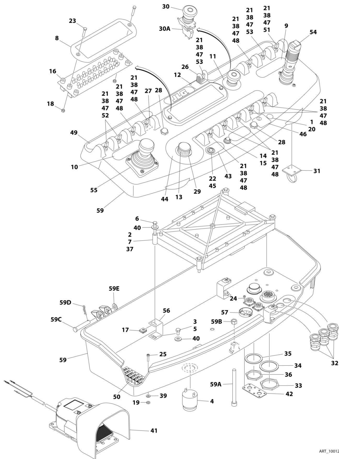
FIGURE 5-28. PLATFORM CONSOLE ASSEMBLY - WITH SKYGUARD (SN 0300218318 through 0300234076)
