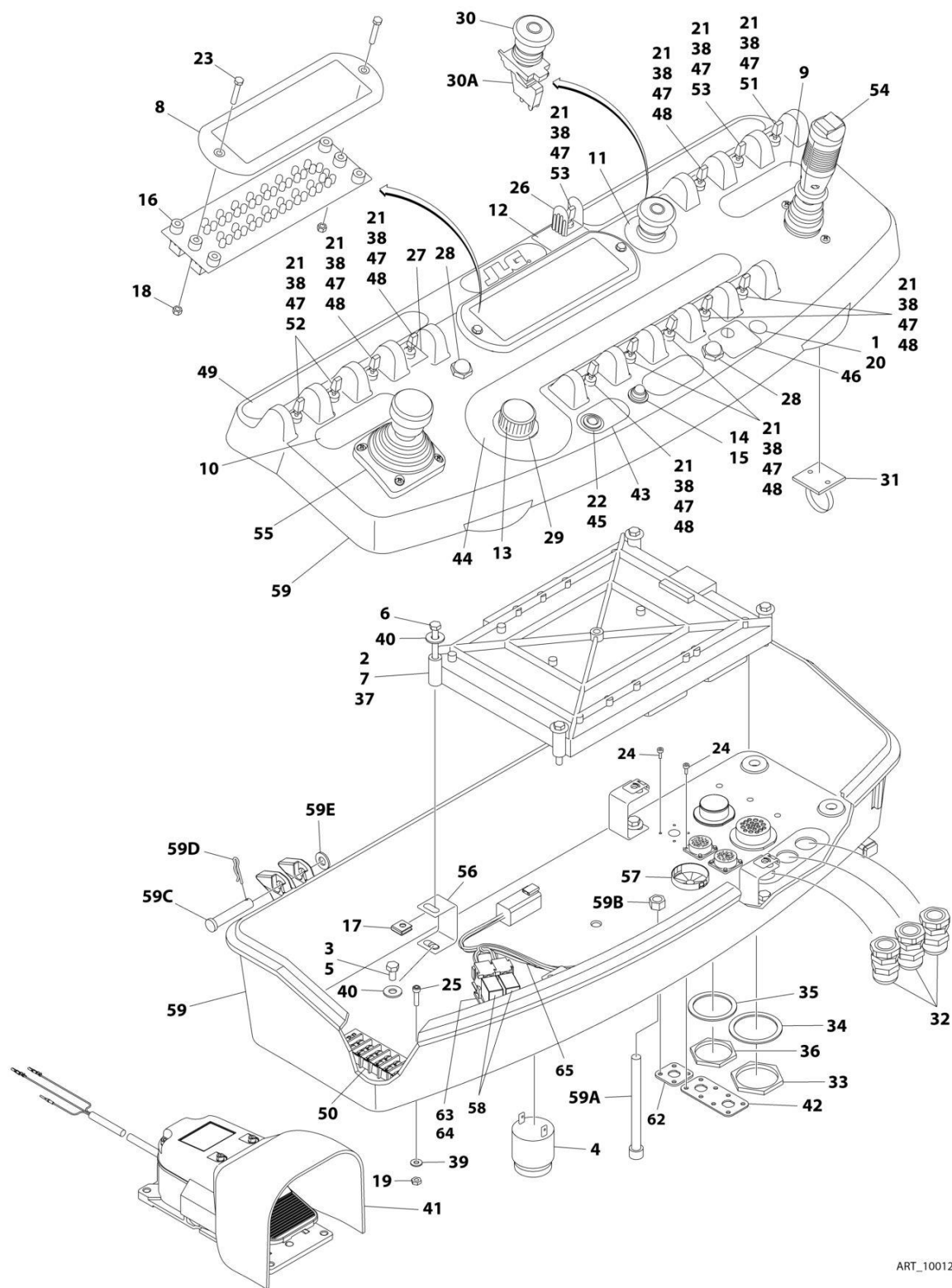
FIGURE 5-29. PLATFORM CONSOLE ASSEMBLY - WITH SKYGUARD (SN 0300234077 through 0300259338)
