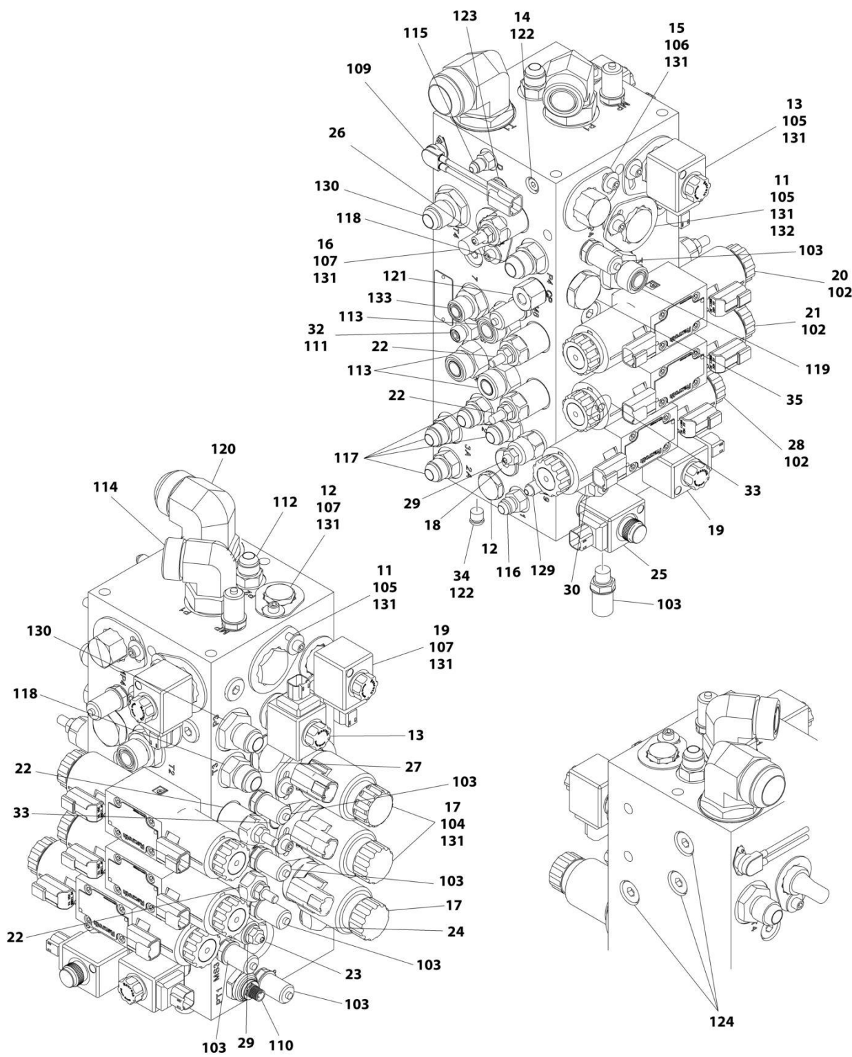
FIGURE 2-4. MAIN VALVE ASSEMBLY (SN 0300247850 through 0300271492)
