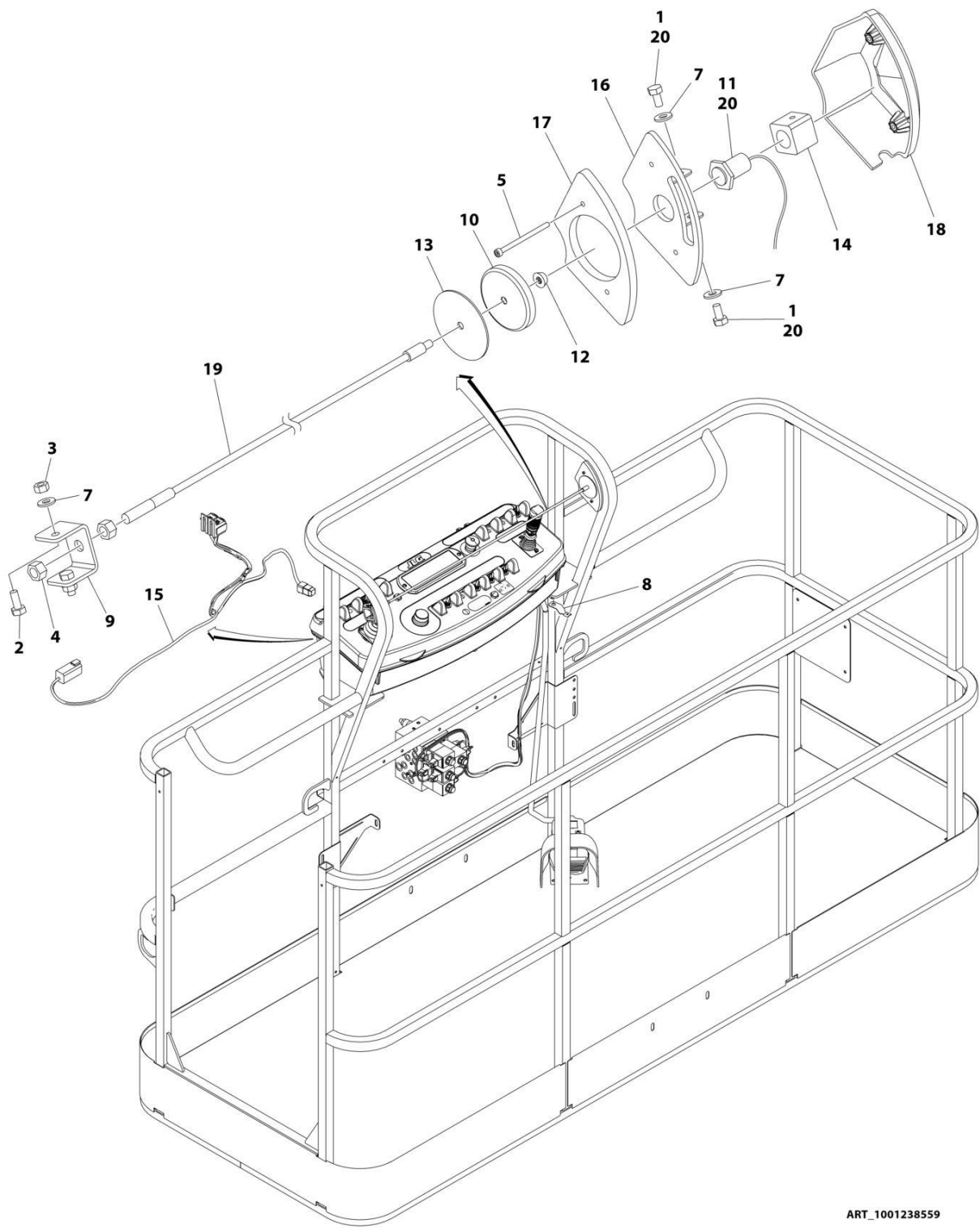
FIGURE 5-68. SKYLINE INSTALLATION (1850SJ)
