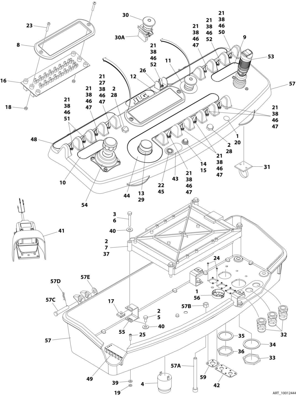
FIGURE 5-30. PLATFORM CONSOLE ASSEMBLY - WITH SKYGUARD (SN 0300229339 through 0300271492)
