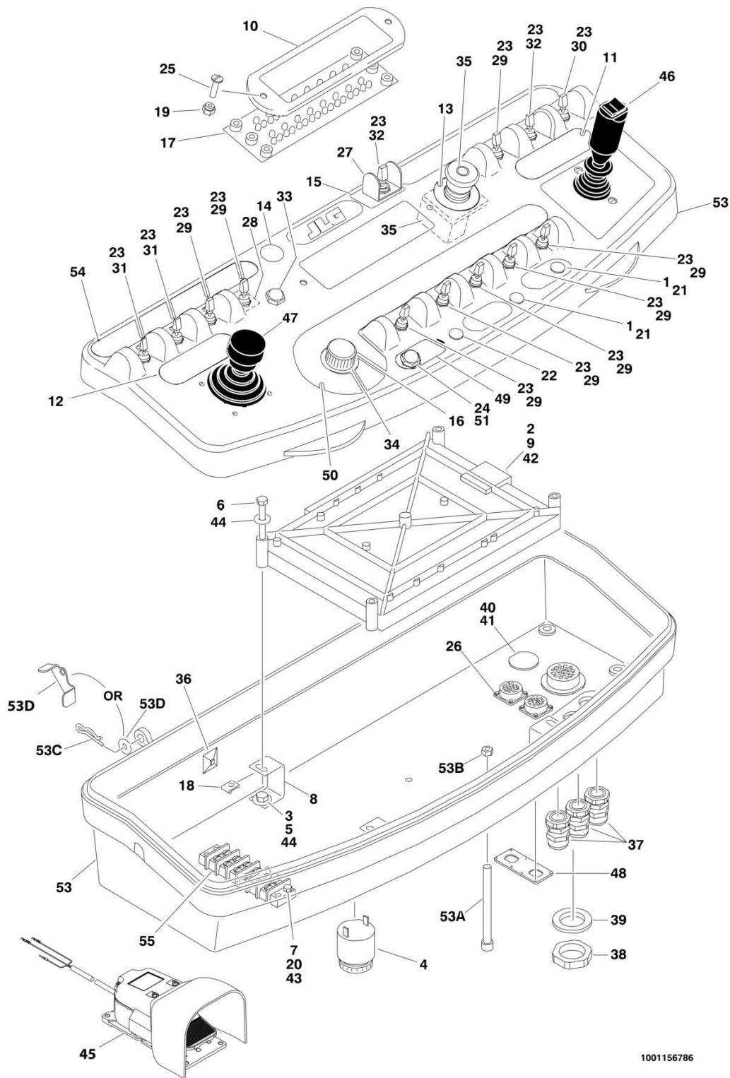
FIGURE 5-23. PLATFORM CONSOLE ASSEMBLY - WITHOUT SKYGUARD (SN 0300000100 through 0300212338)
