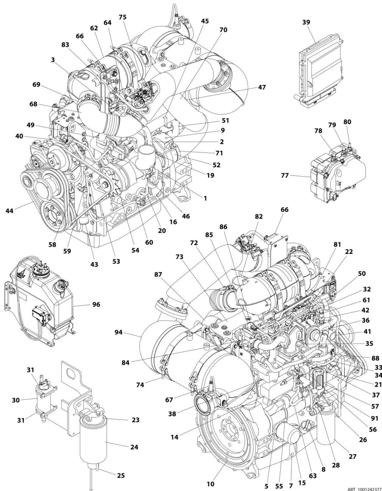
FIGURE 3-39. DEUTZ T4F ENGINE COMPONENTS (SN 0300255121 through 0300271492)
