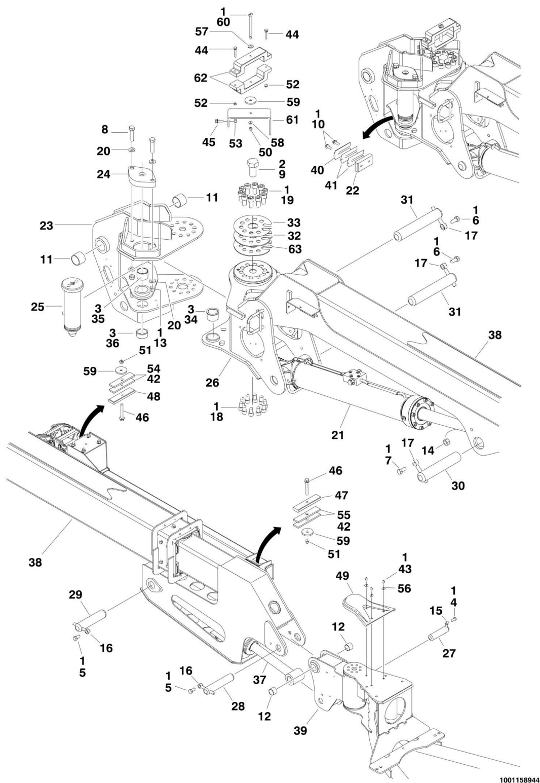
FIGURE 4-3. JIB INSTALLATION
