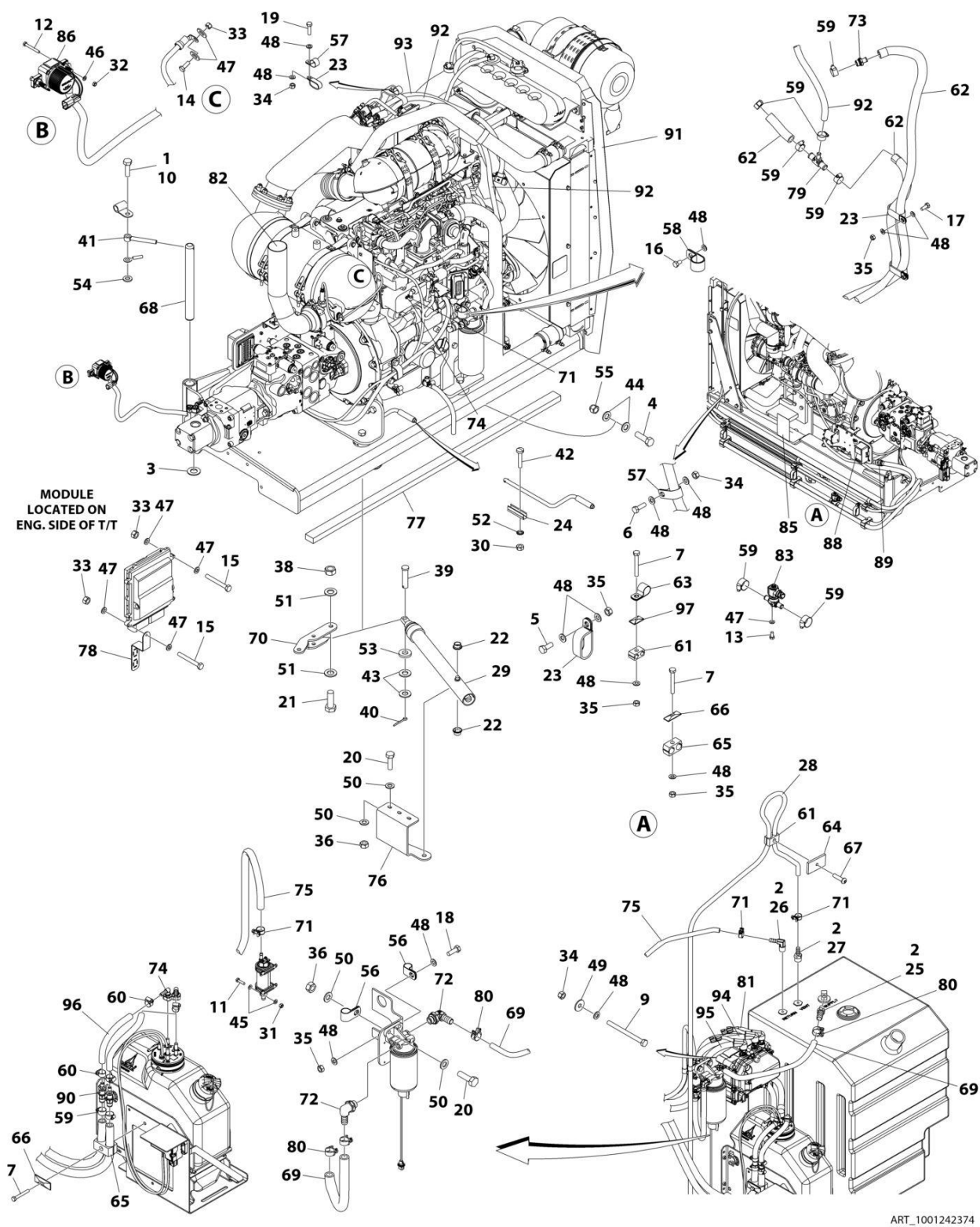
FIGURE 3-27. DEUTZ T4F ENGINE INSTALLATION - NO COLD WEATHER PKG (SN 0300255121 through 0300271492)
