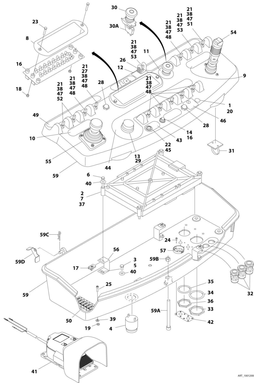
FIGURE 5-27. PLATFORM CONSOLE ASSEMBLY - WITH SKYGUARD (SN 0300212338 through 0300218317)
