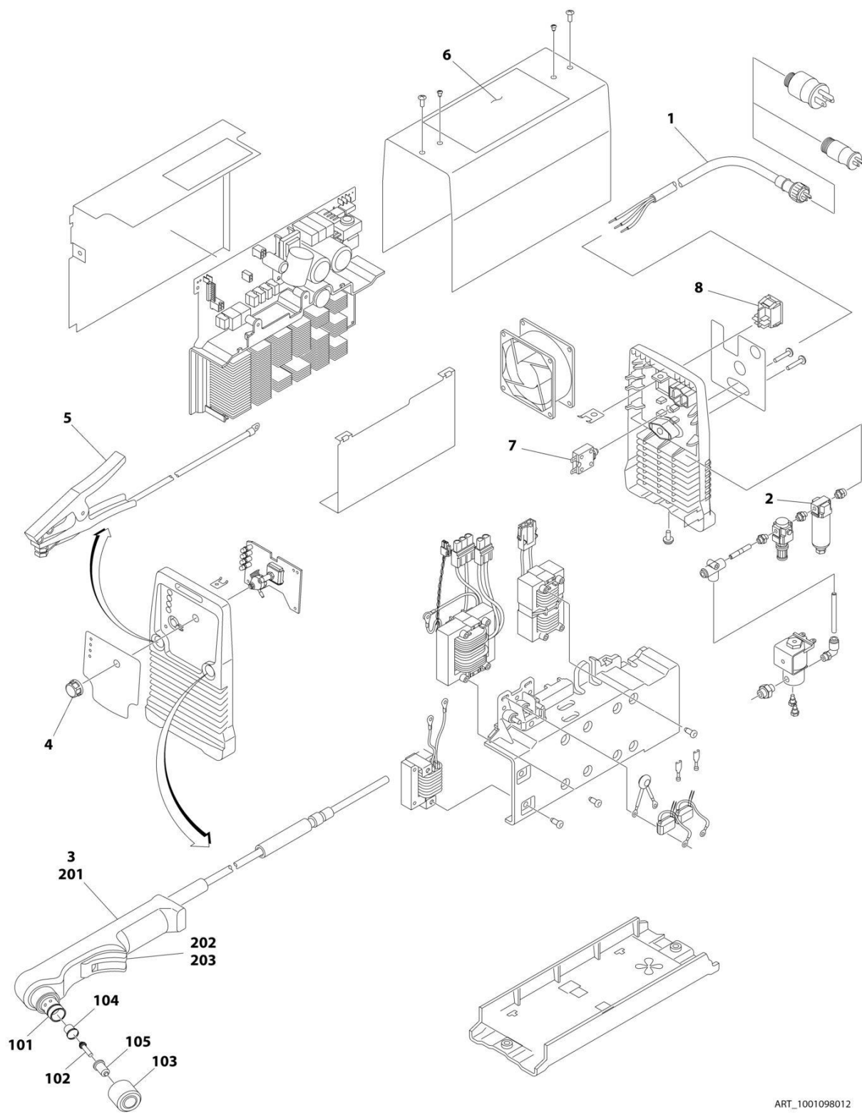
FIGURE 5-74. PLASMA CUTTER ASSEMBLY
