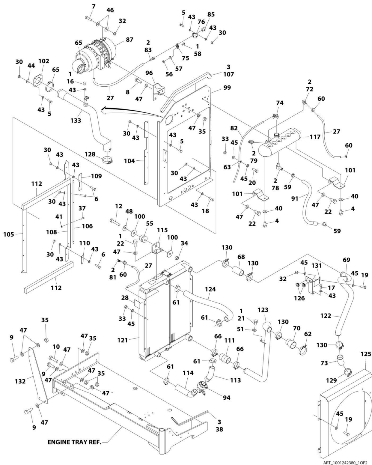
FIGURE 3-37. DEUTZ T4F ENGINE ASSEMBLY - WITH COLD WEATHER PKG (SN 0300255121 through 0300271492)
