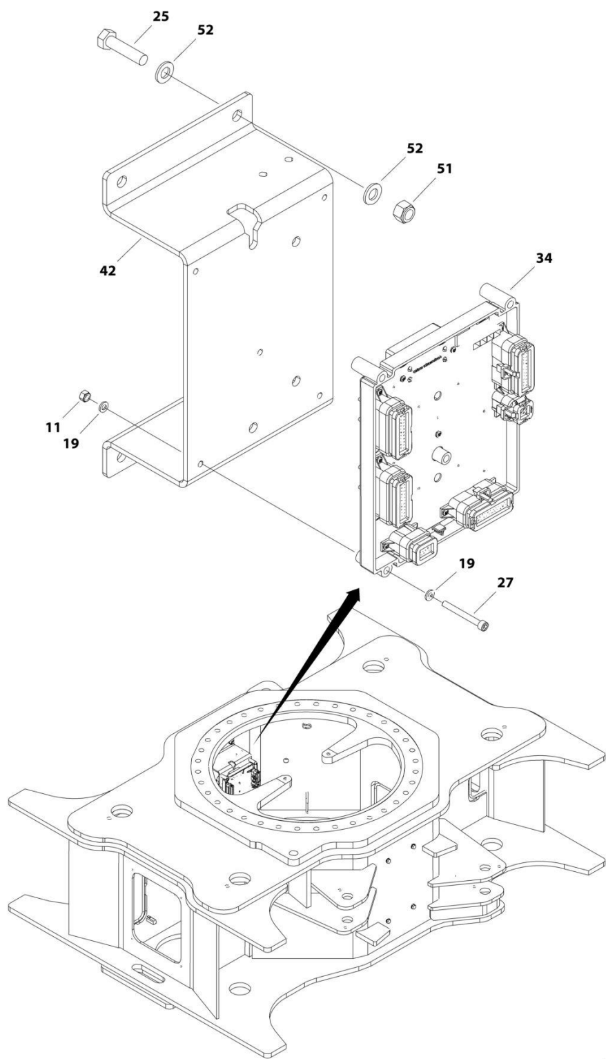
FIGURE 1-15. ELECTRICAL COMPONENTS INSTALLATION - FRAME (ANSI, ANSI EXPORT (HRC), CSA AND JAPANESE SPECS) (SN 0300210987 through 0300271492)
