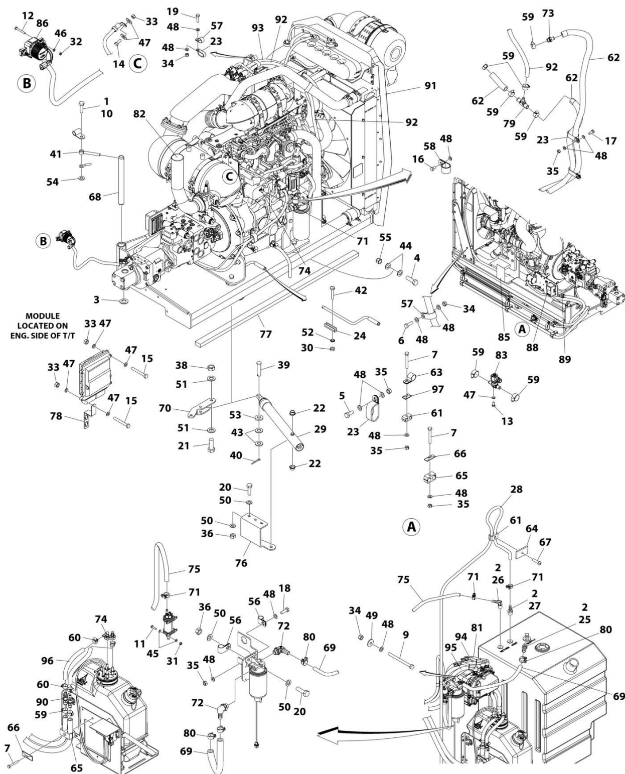
FIGURE 3-33. DEUTZ T4F ENGINE INSTALLATION - WITH COLD WEATHER PKG (SN 0300255121 through 0300271492)
