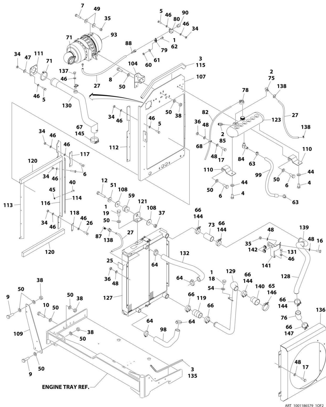
FIGURE 3-30. DEUTZ T4F ENGINE ASSEMBLY - NO COLD WEATHER PKG (SN 0300000100 through 0300255121)
