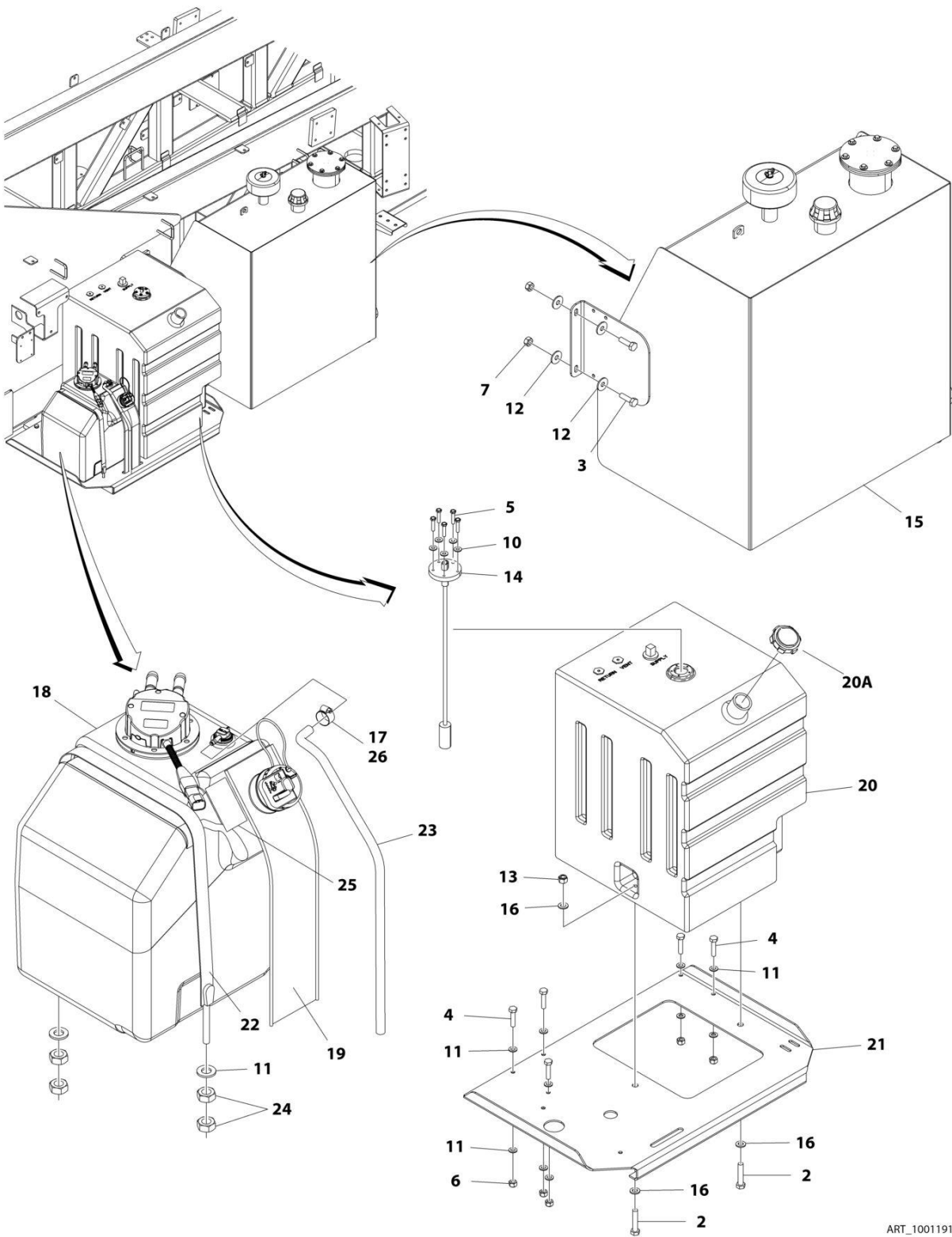
FIGURE 2-13. TANKS INSTALLATION - WITH DIESEL EXHAUST FLUID TANK (SN 0300210987 through 0300255120)
