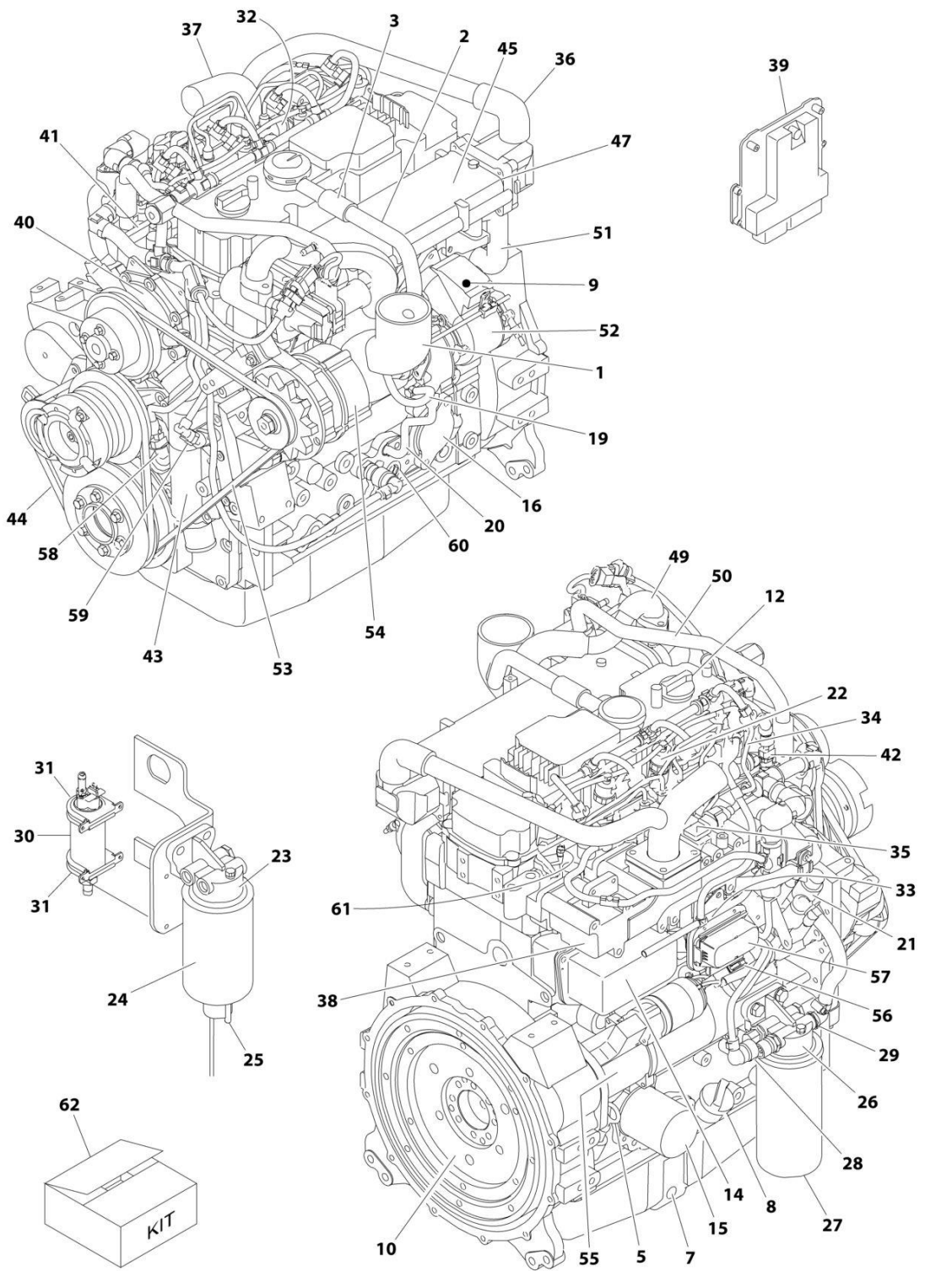
FIGURE 3-7. DEUTZ LRC ENGINE COMPONENTS
