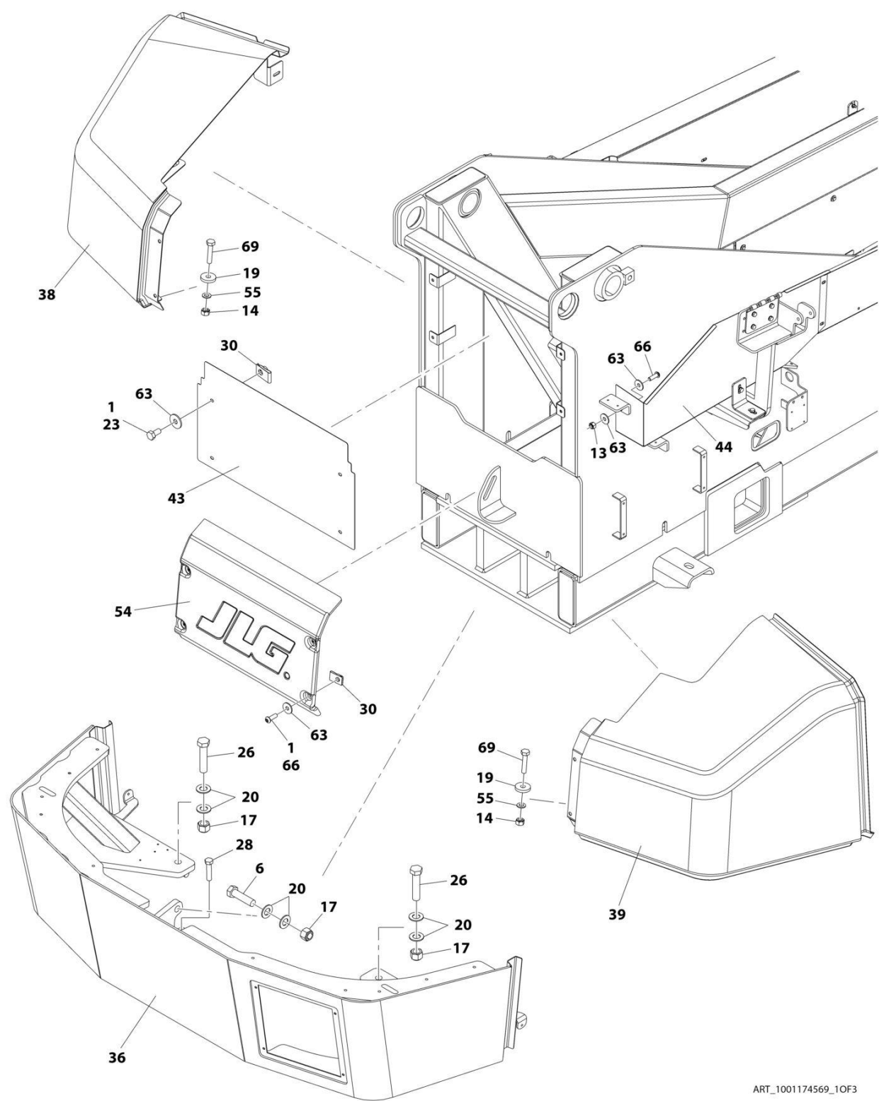
FIGURE 2-43. HOOD INSTALLATION (SN 0300205509 through 0300210986)
