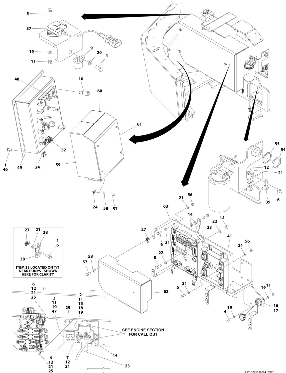
FIGURE 2-22. TURNTABLE ELECTRICAL COMPONENTS INSTALLATION (CE SPECS) (SN 0300210988 through 0300271492)
