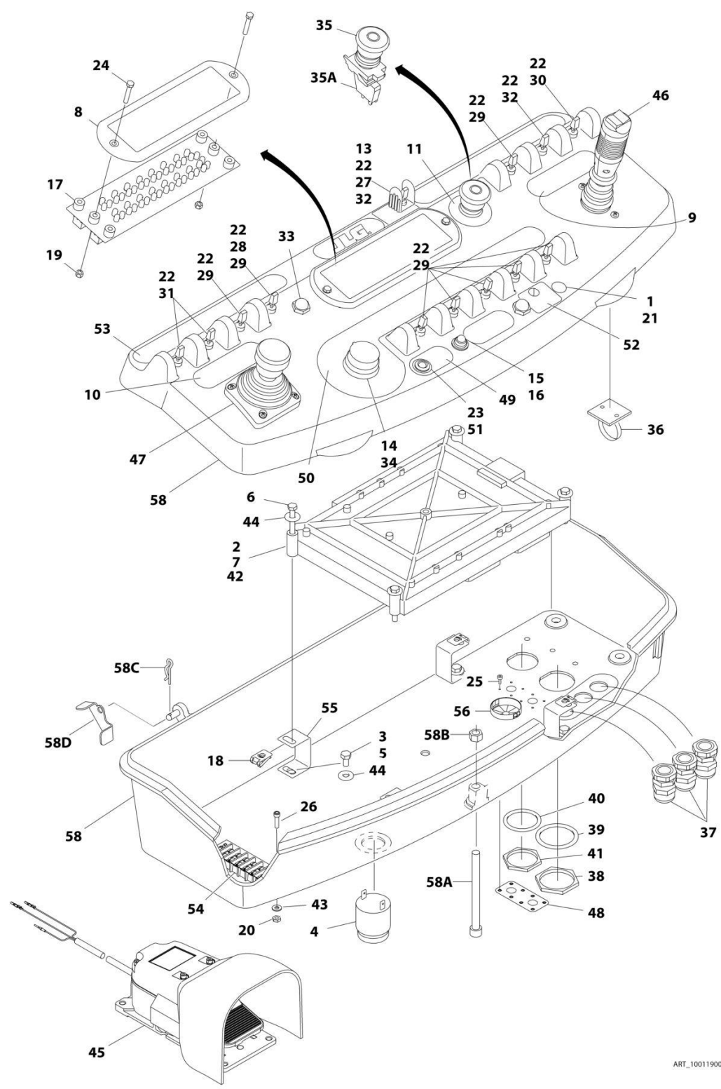
FIGURE 5-26. PLATFORM CONSOLE ASSEMBLY - WITH SKYGUARD (SN 0300000100 through 0300212338)
