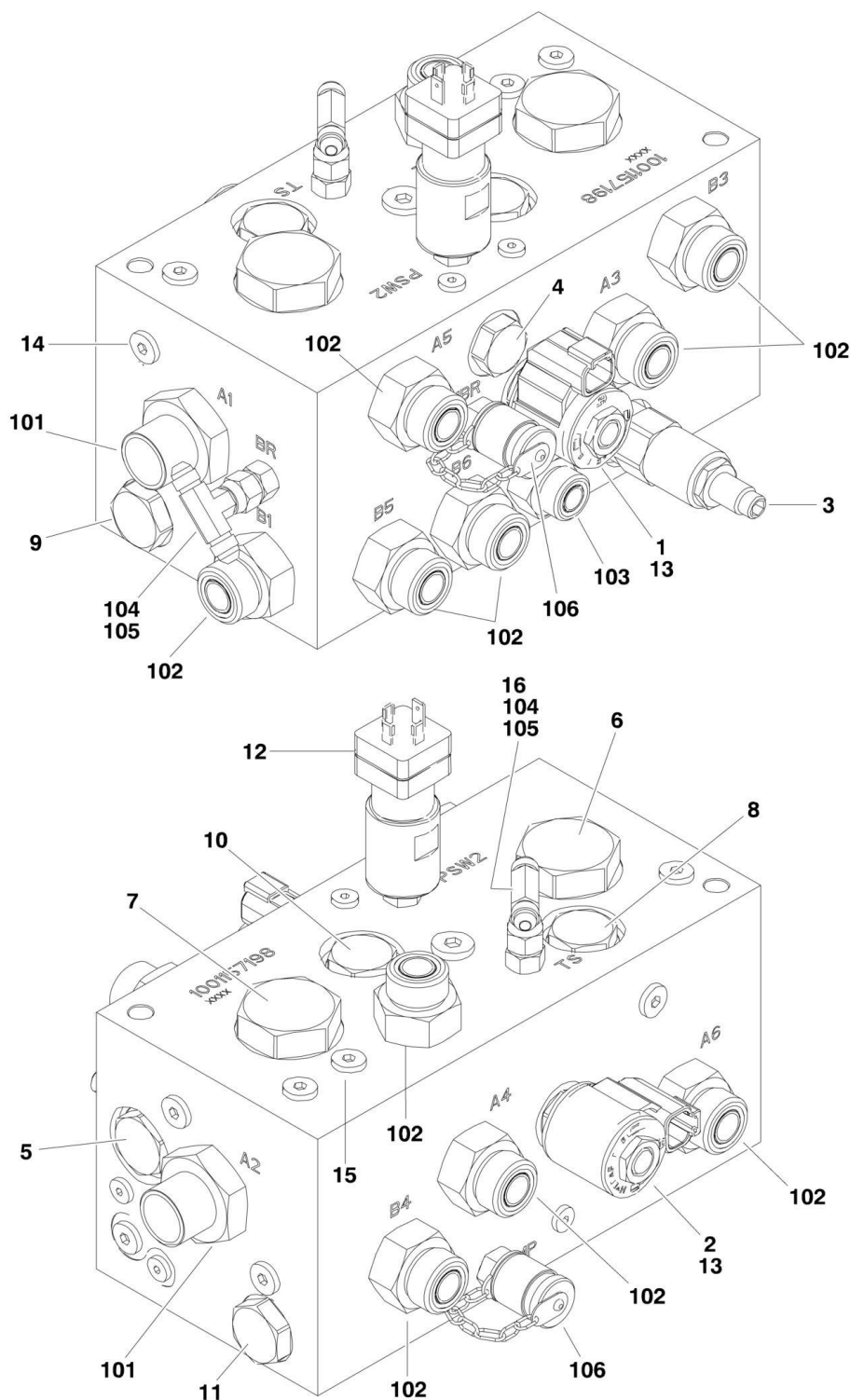
FIGURE 1-11. TRACTION VALVE ASSEMBLY (SN 0300000100 through 0300224866)
