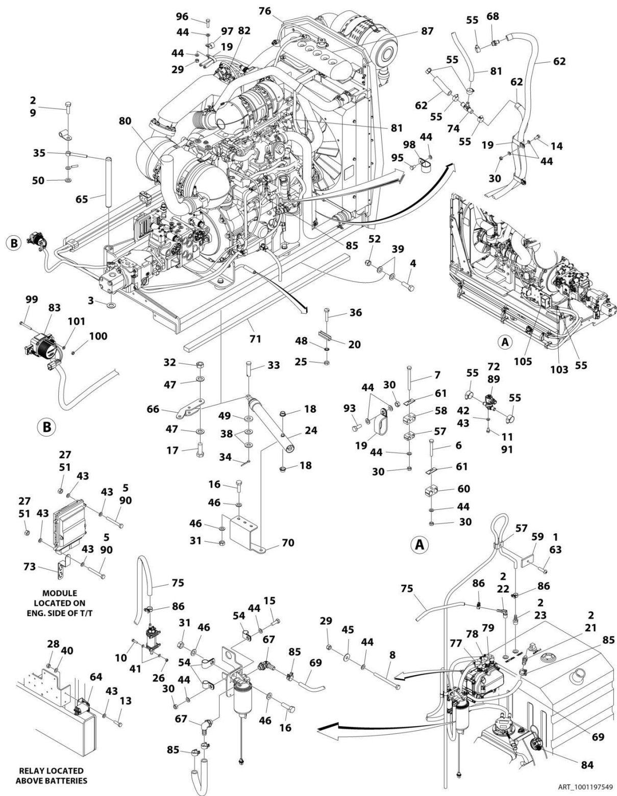
FIGURE 3-32. DEUTZ T4F ENGINE INSTALLATION - WITH COLD WEATHER PKG (SN 0300000100 through 0300255121)
