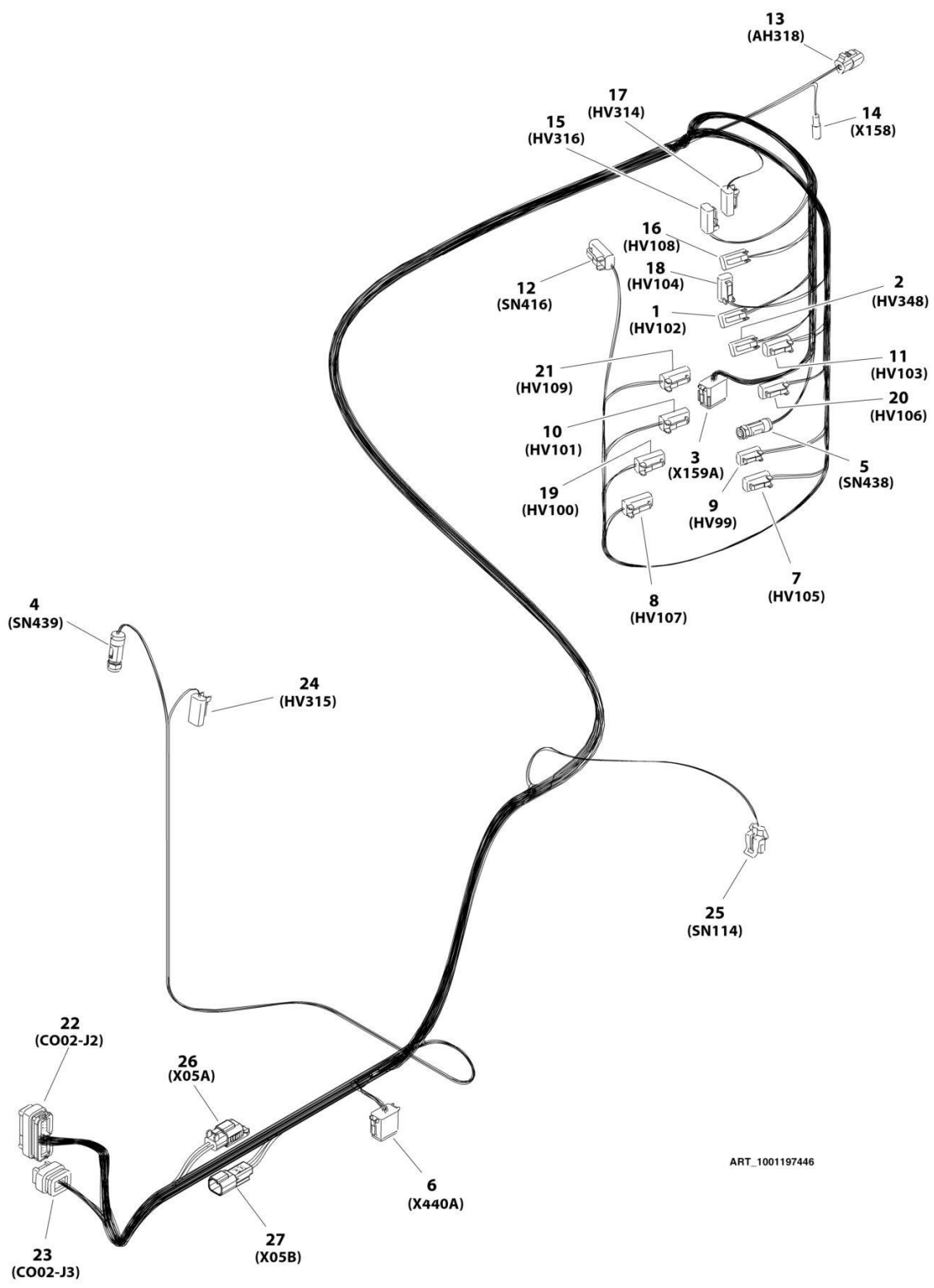
FIGURE 8-66. VALVE BANK HARNESS (SN 0300201023 through 0300271492)
