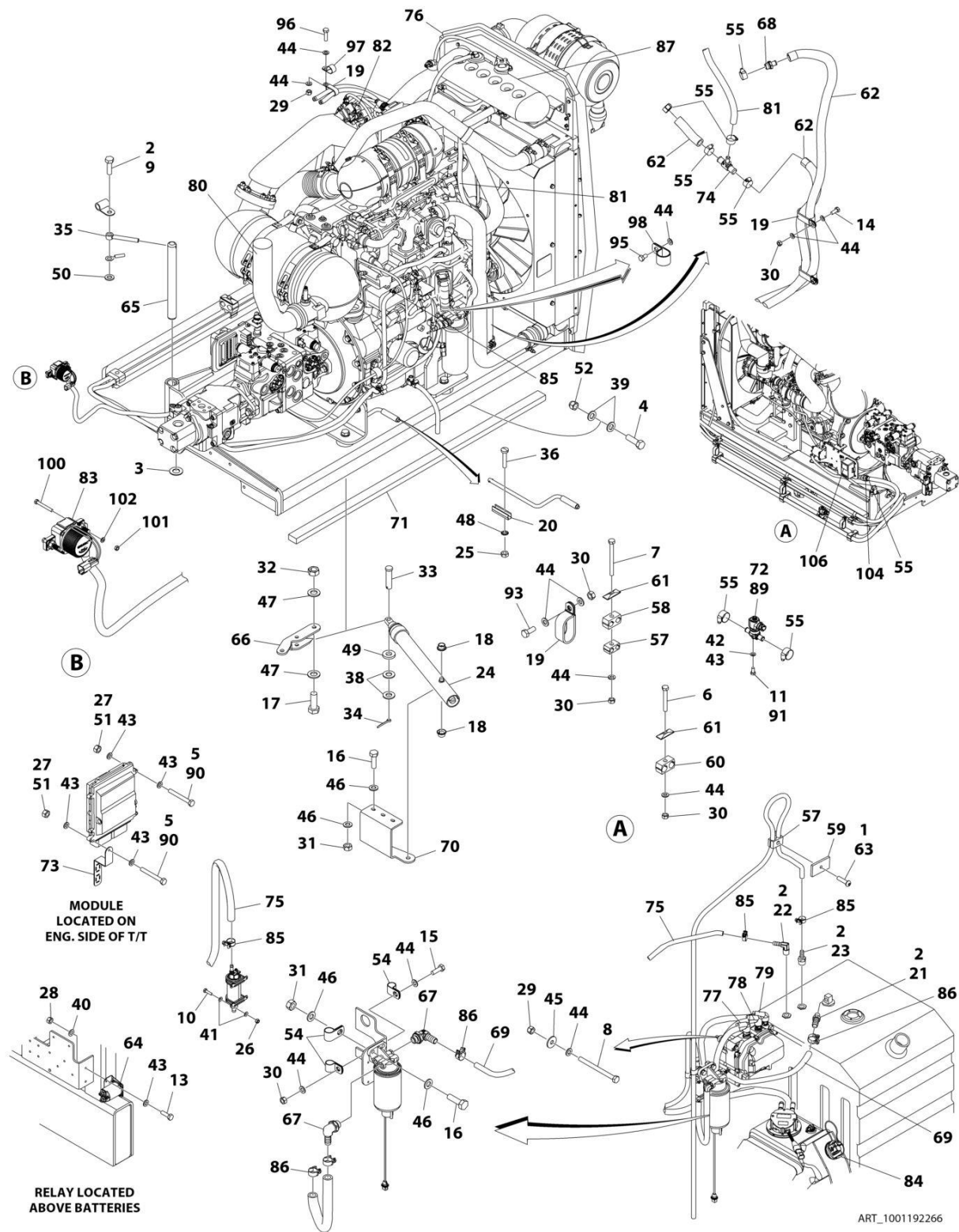
FIGURE 3-26. DEUTZ T4F ENGINE INSTALLATION - NO COLD WEATHER PKG (SN 0300000100 through 0300255121)
