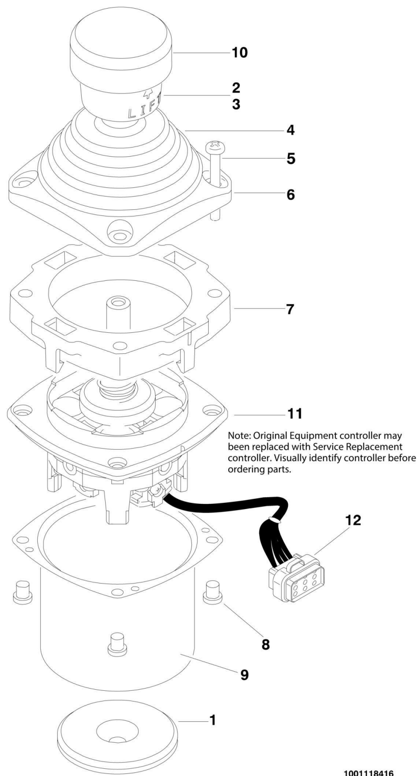
FIGURE 5-35. LIFT AND SWING CONTROLLER ASSEMBLY (SN 0300000100 through 0300188926)
