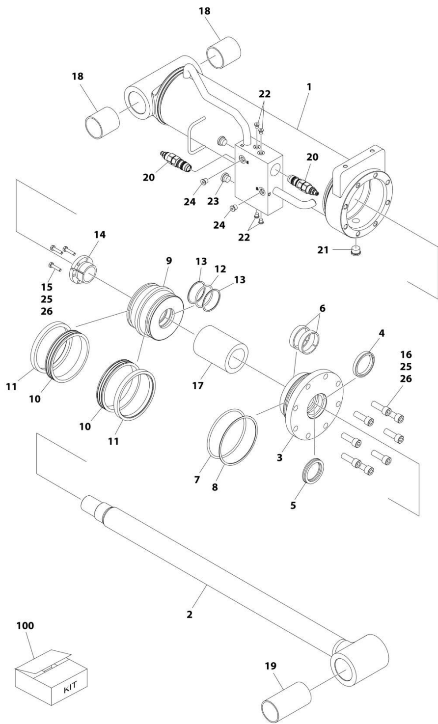
FIGURE 6-2. AXLE EXTEND CYLINDER ASSEMBLY (SN 0300239676 through 0300271492)
