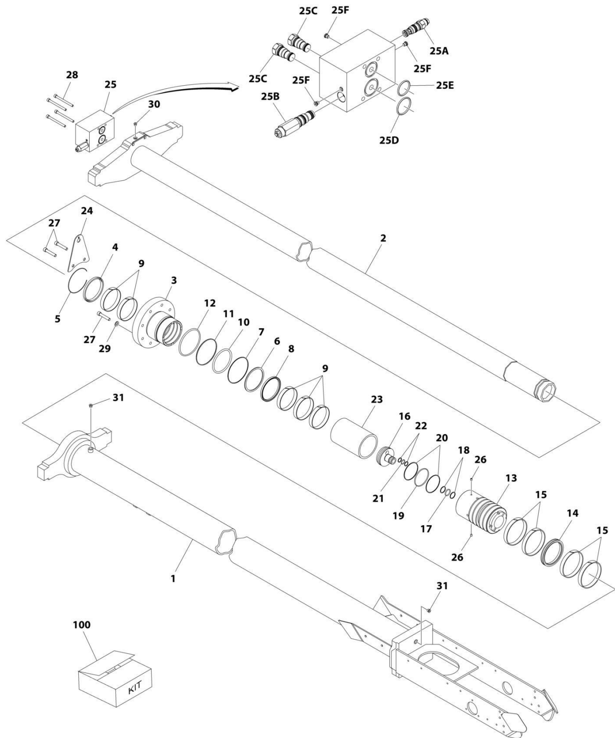
FIGURE 6-16. TELESCOPE CYLINDER ASSEMBLY - BOOM (SN 0300244678 through 0300271492)
