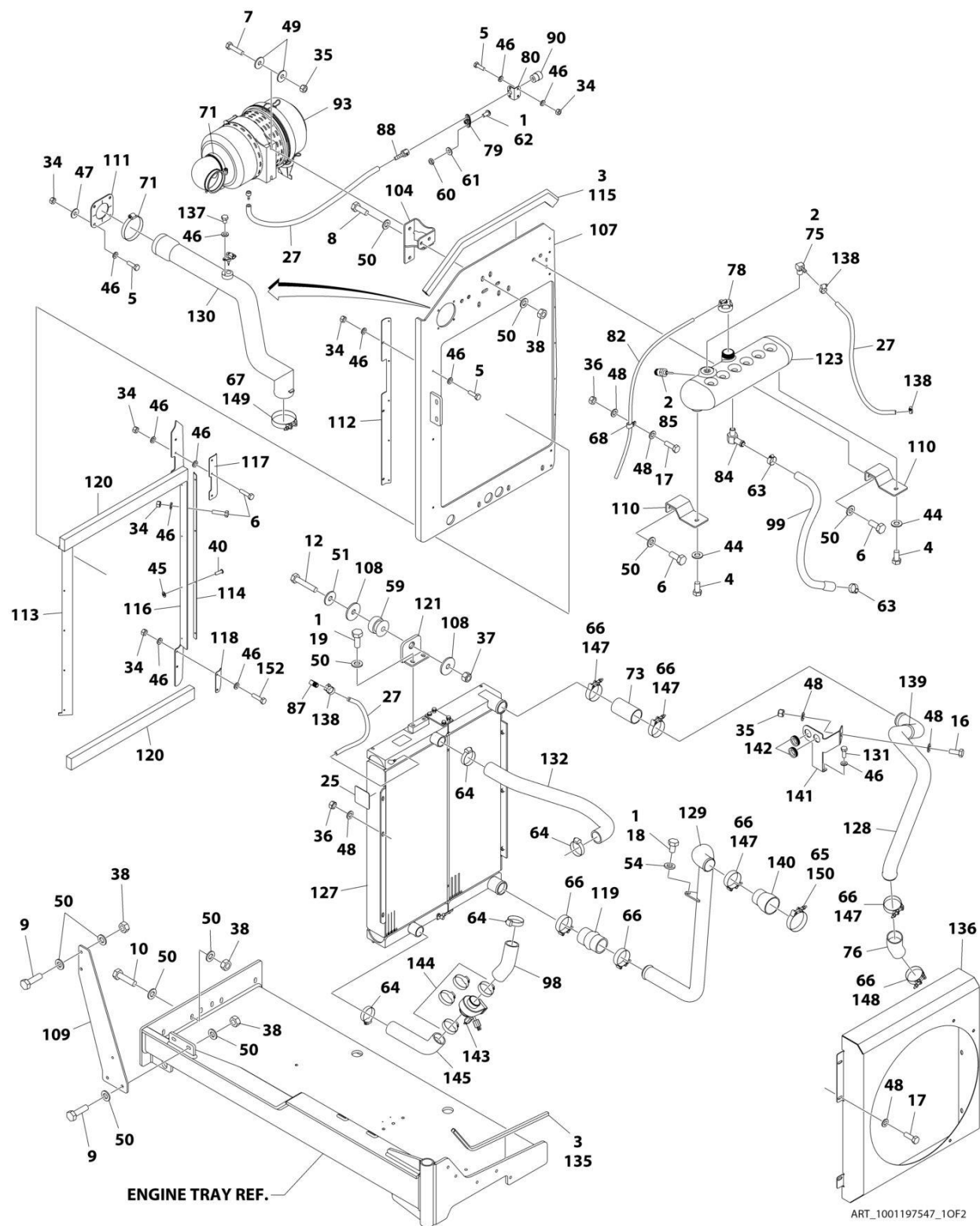
FIGURE 3-36. DEUTZ T4F ENGINE ASSEMBLY - WITH COLD WEATHER PKG (SN 0300000100 through 0300255121)
