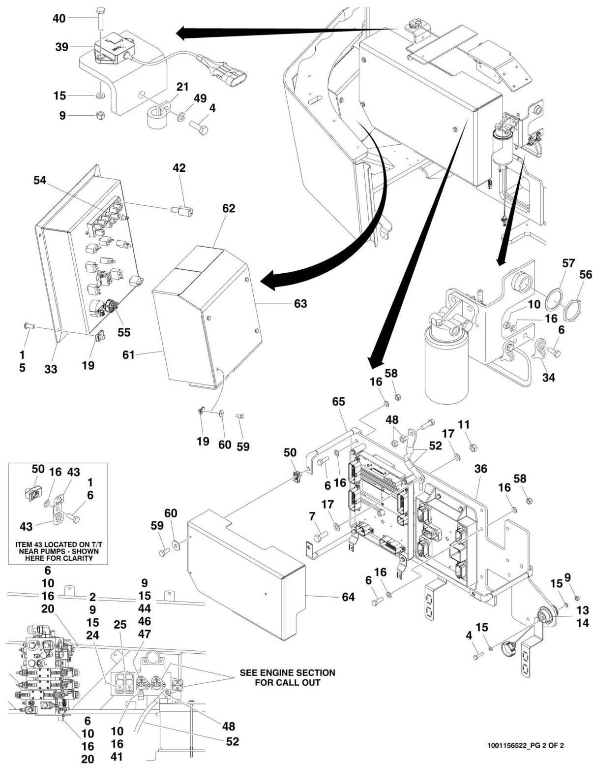
FIGURE 2-19. TURNTABLE ELECTRICAL COMPONENTS INSTALLATION
