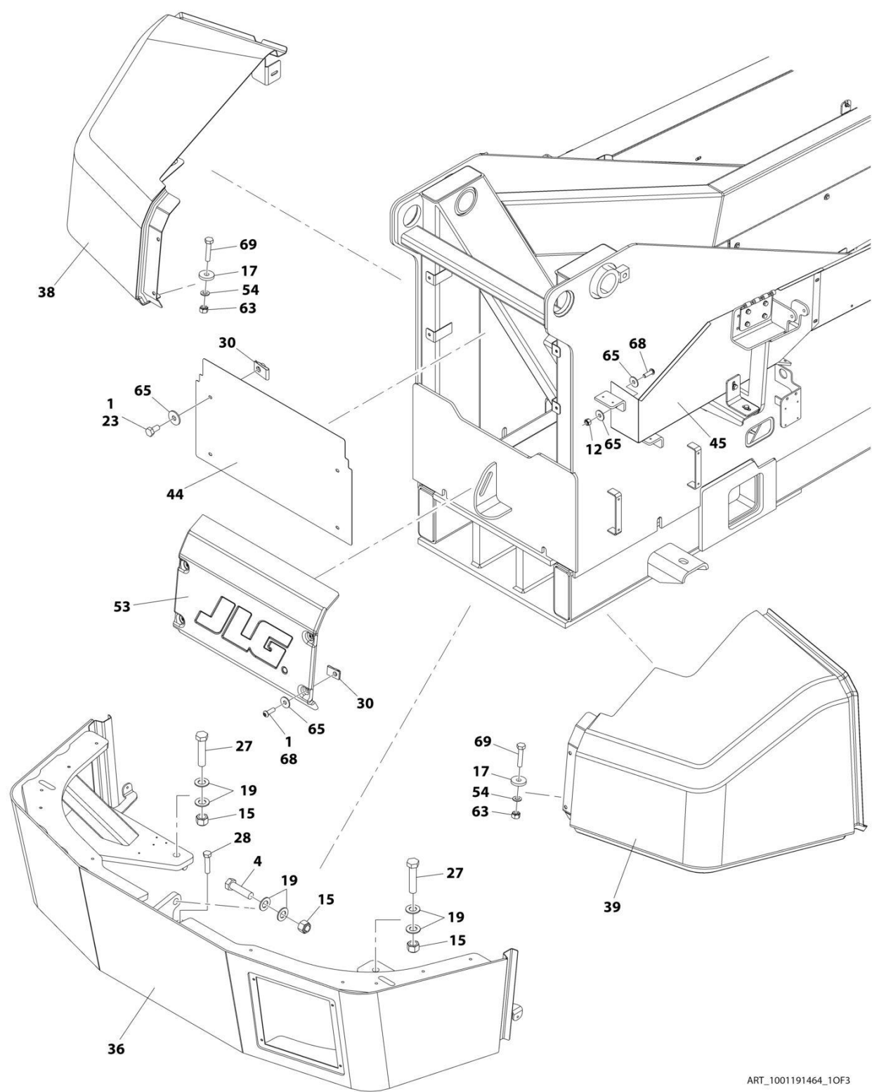
FIGURE 2-44. HOOD INSTALLATION (SN 0300210987 through 0300271492)
