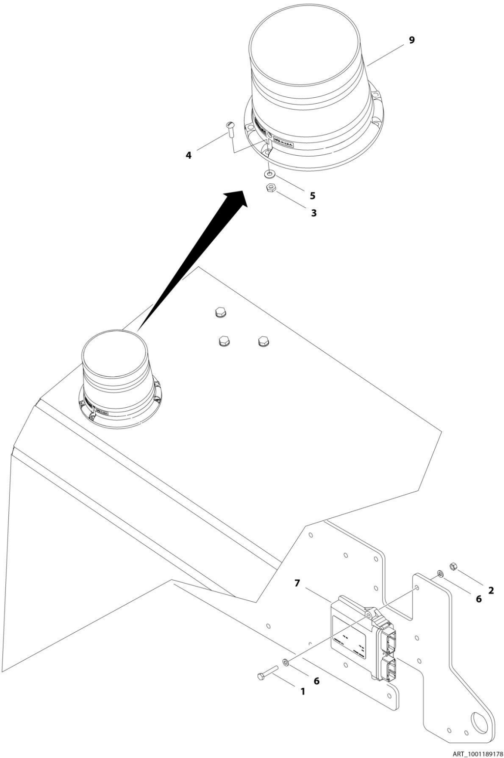
FIGURE 2-36. STROBE LIGHT INSTALLATION - BLUE (SN 0300000100 through 0300217096)
