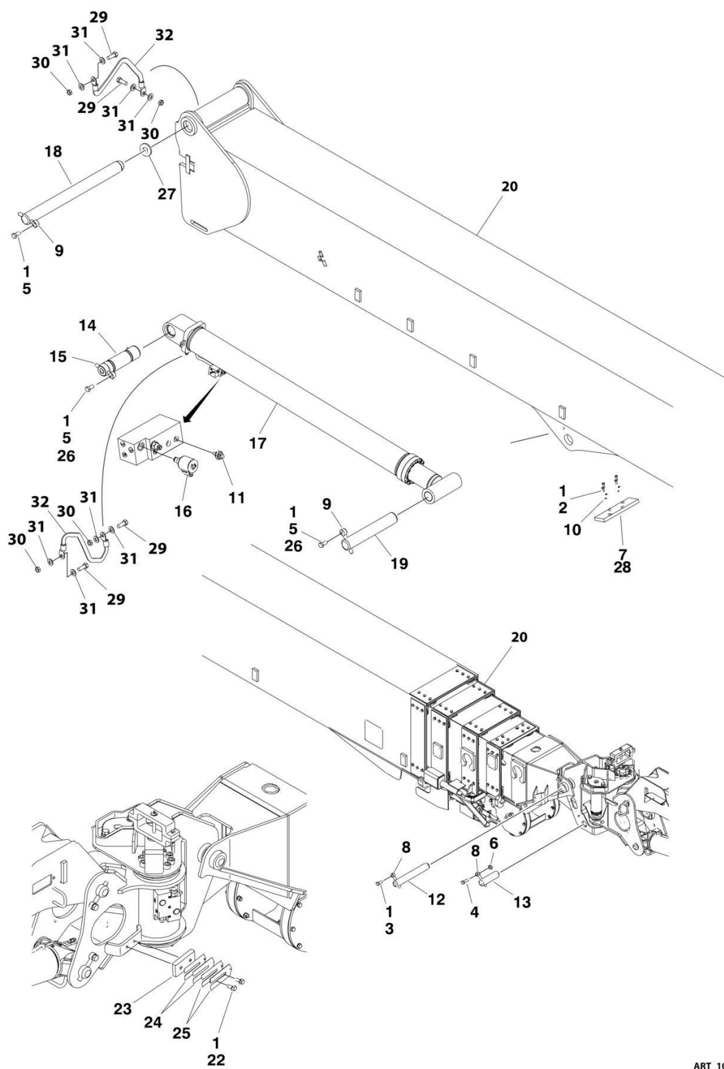
FIGURE 4-1. BOOM INSTALLATION
