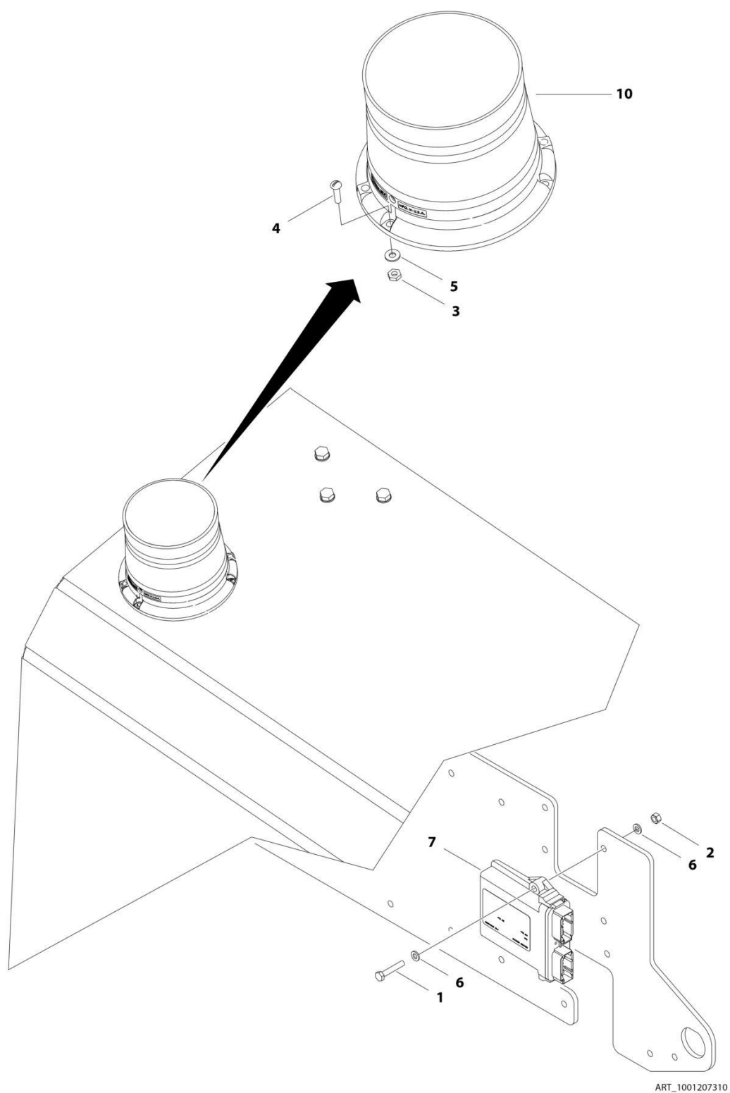
FIGURE 2-39. STROBE LIGHT INSTALLATION - RED (SN 0300000100 through 0300217096)
