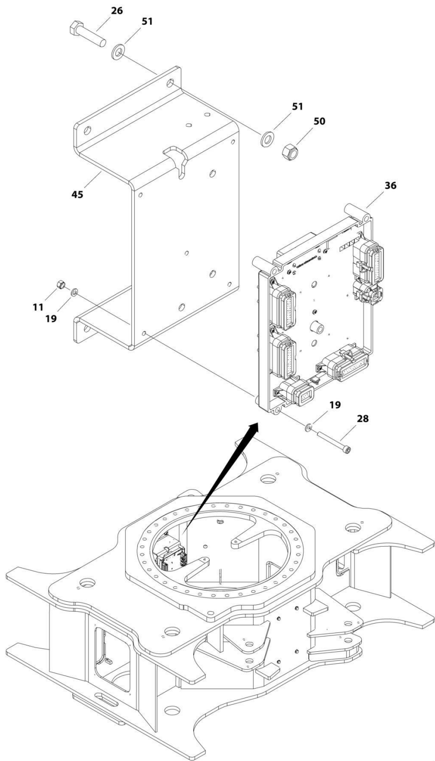
FIGURE 1-17. ELECTRICAL COMPONENTS INSTALLATION - FRAME (CE SPECS) (SN 0300210988 through 0300271492)
