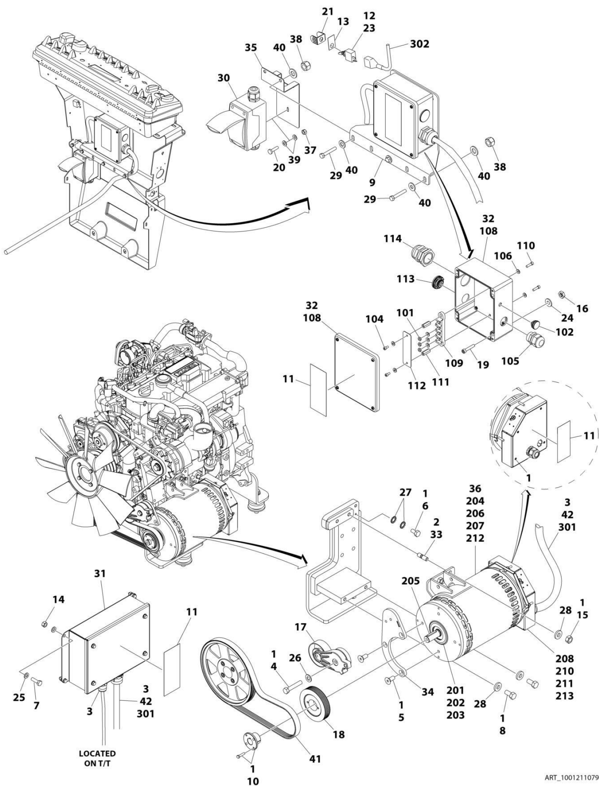
FIGURE 3-47. 4000W GENERATOR INSTALLATION - 50HZ SPEC (OPTIONAL)
