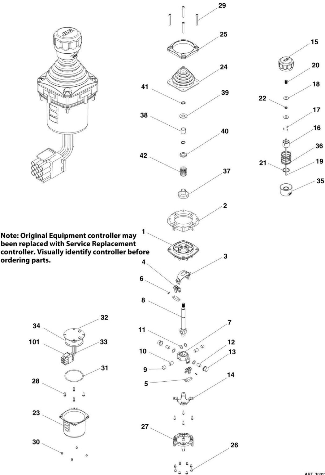
FIGURE 5-36. CONTROLLER ASSEMBLY (LIFT AND SWING) (SN 0300188926 through 0300271492)
