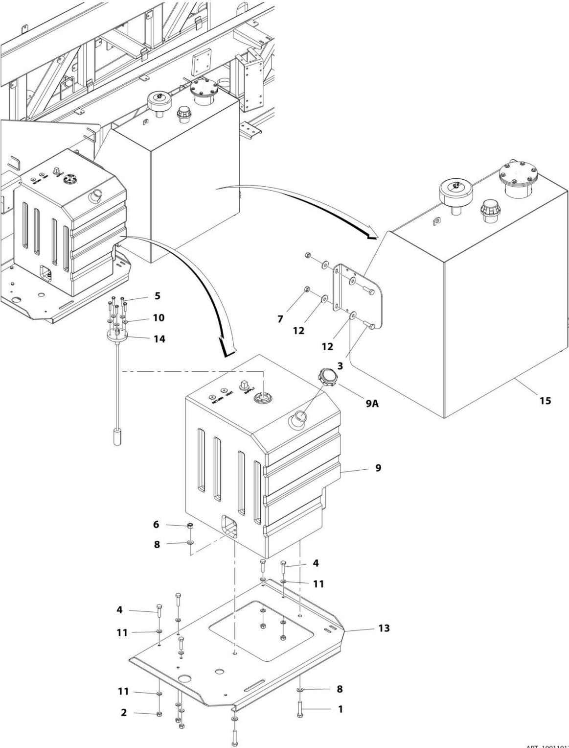
FIGURE 2-12. TANKS INSTALLATION (SN 0300210987 through 0300271492)
