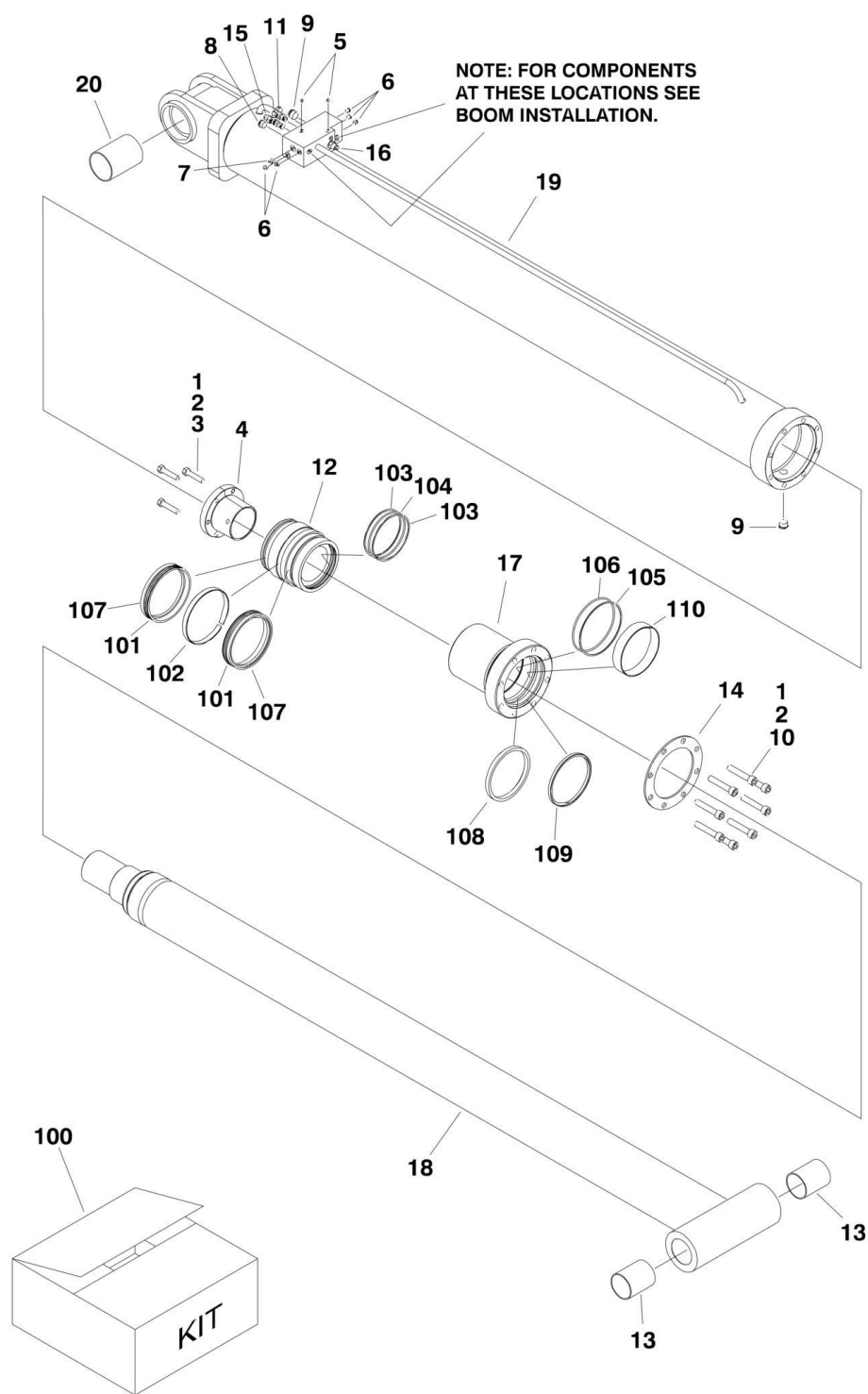
FIGURE 6-7. LIFT CYLINDER ASSEMBLY - BOOM (SN 0300000100 through 0300239676)
