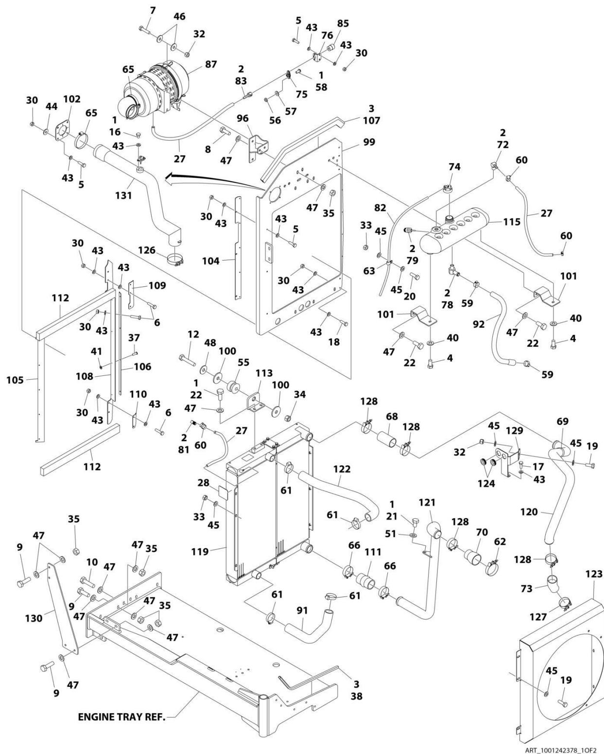
FIGURE 3-31. DEUTZ T4F ENGINE ASSEMBLY - NO COLD WEATHER PKG (SN 0300255121 through 0300271492)
