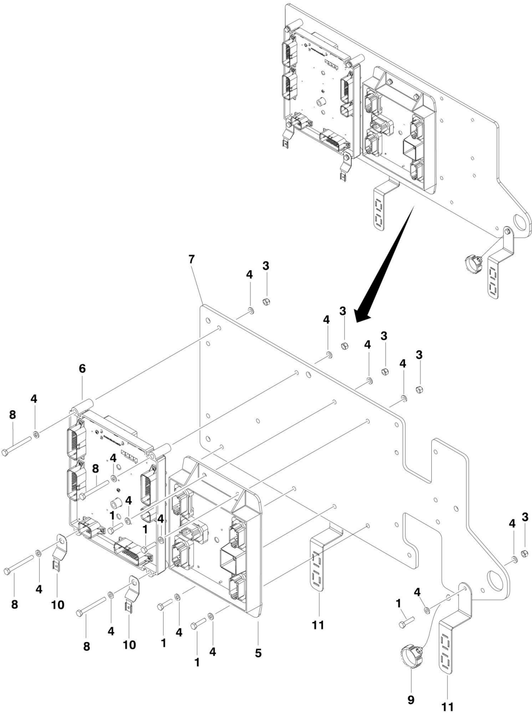
FIGURE 2-33. ELECTRICAL PANEL ASSEMBLY
