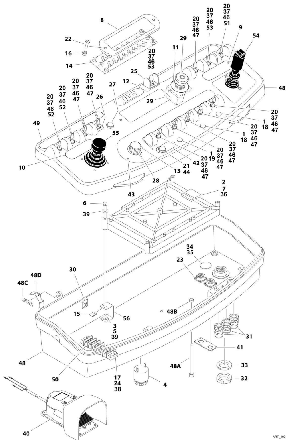
FIGURE 5-24. PLATFORM CONSOLE ASSEMBLY - WITHOUT SKYGUARD (SN 0300212338 through 0300218317)
