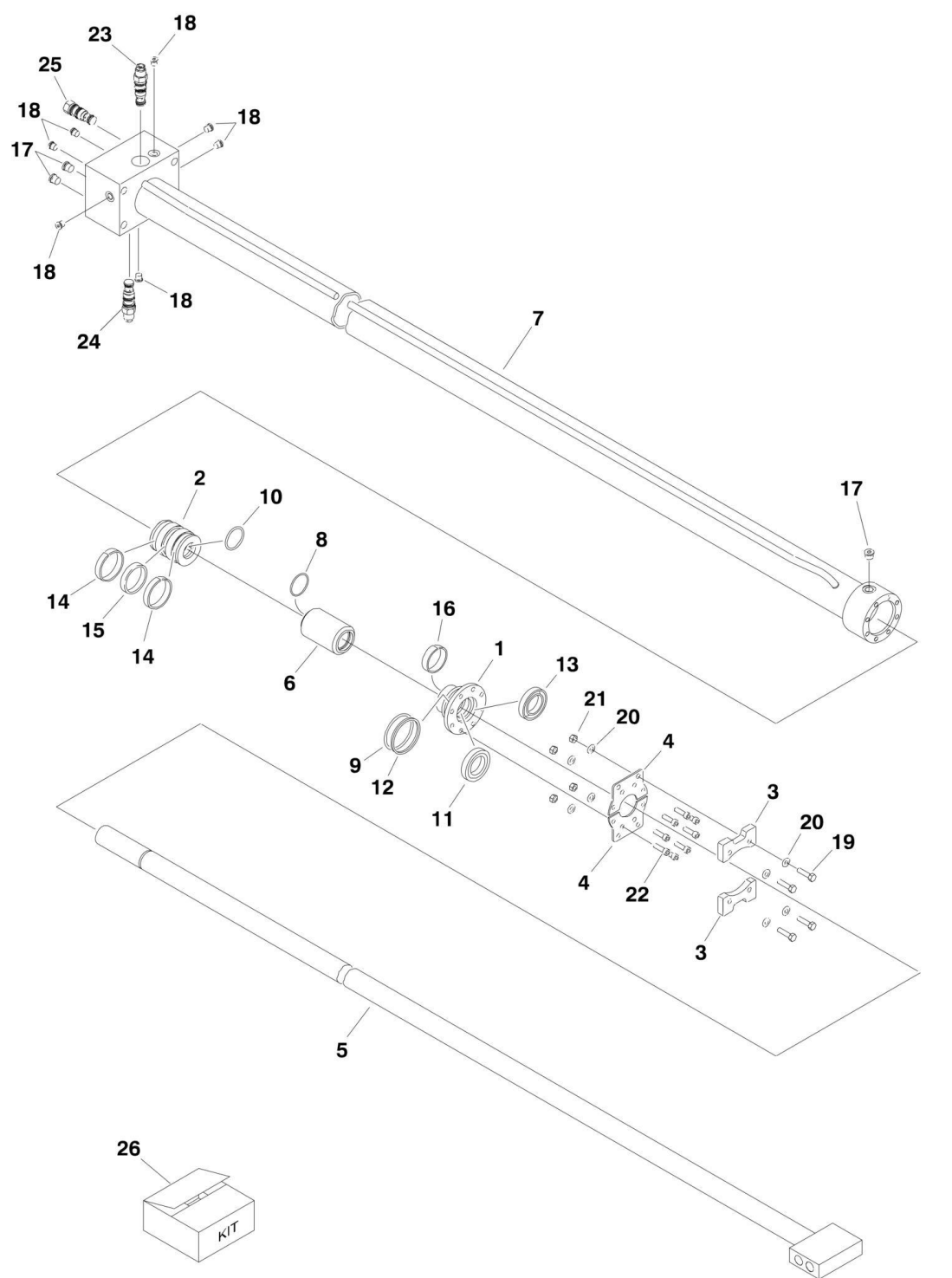
FIGURE 6-17. TELESCOPE CYLINDER ASSEMBLY - JIB
