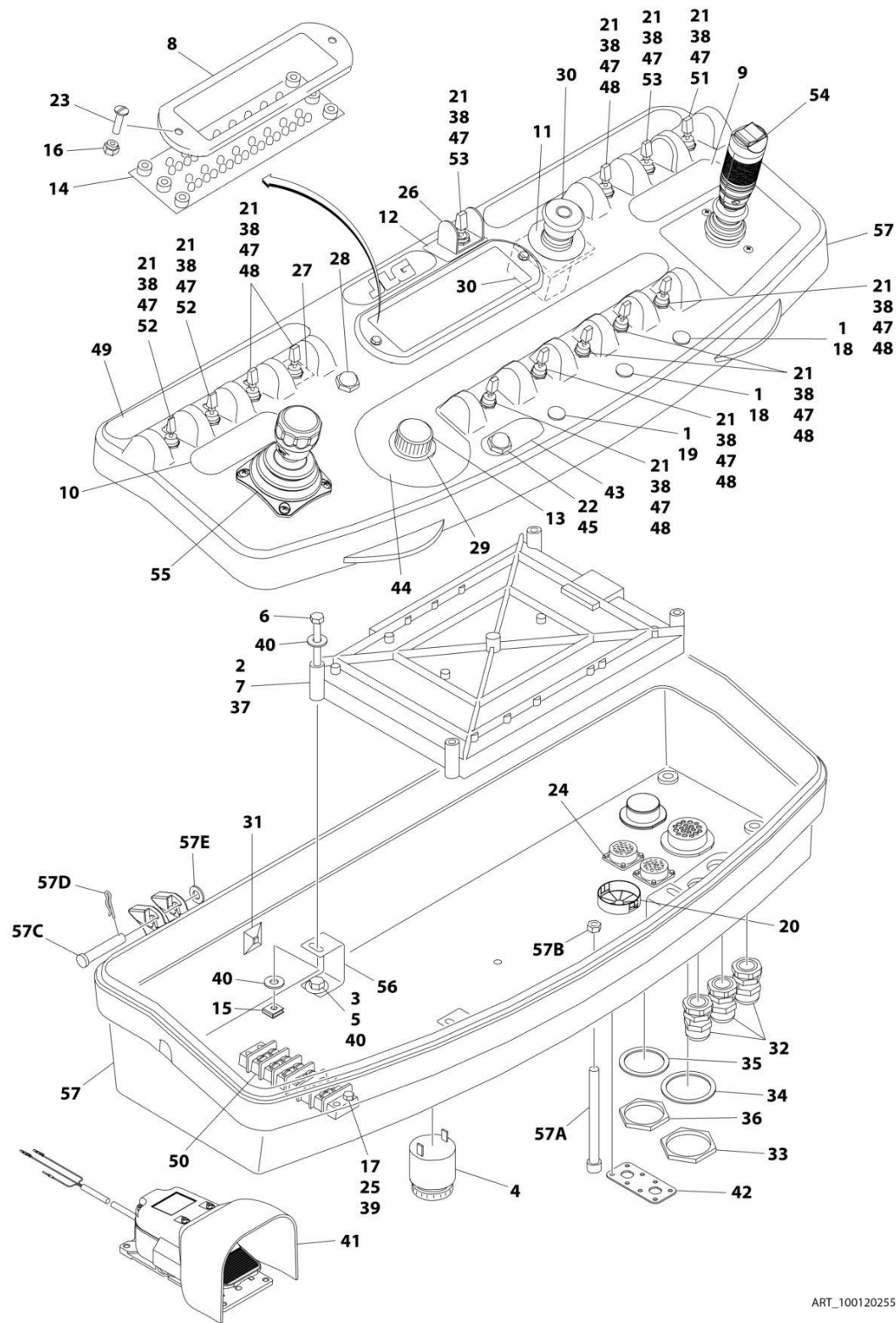
FIGURE 5-25. PLATFORM CONSOLE ASSEMBLY - WITHOUT SKYGUARD (SN 0300218318 through 0300271492)
