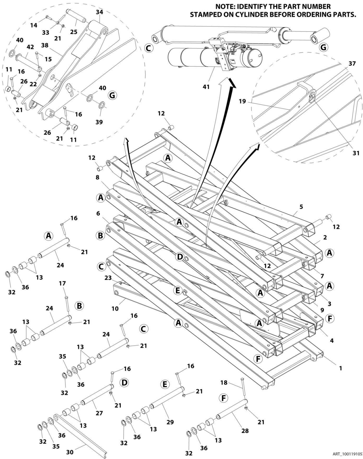
FIGURE 3-16. SCISSORS ARMS ASSEMBLY - BIODEGRADEABLE HYDRAULIC OIL (CHINA BUILT MACHINES) (2646ES) (SN B200020982 to Present)
