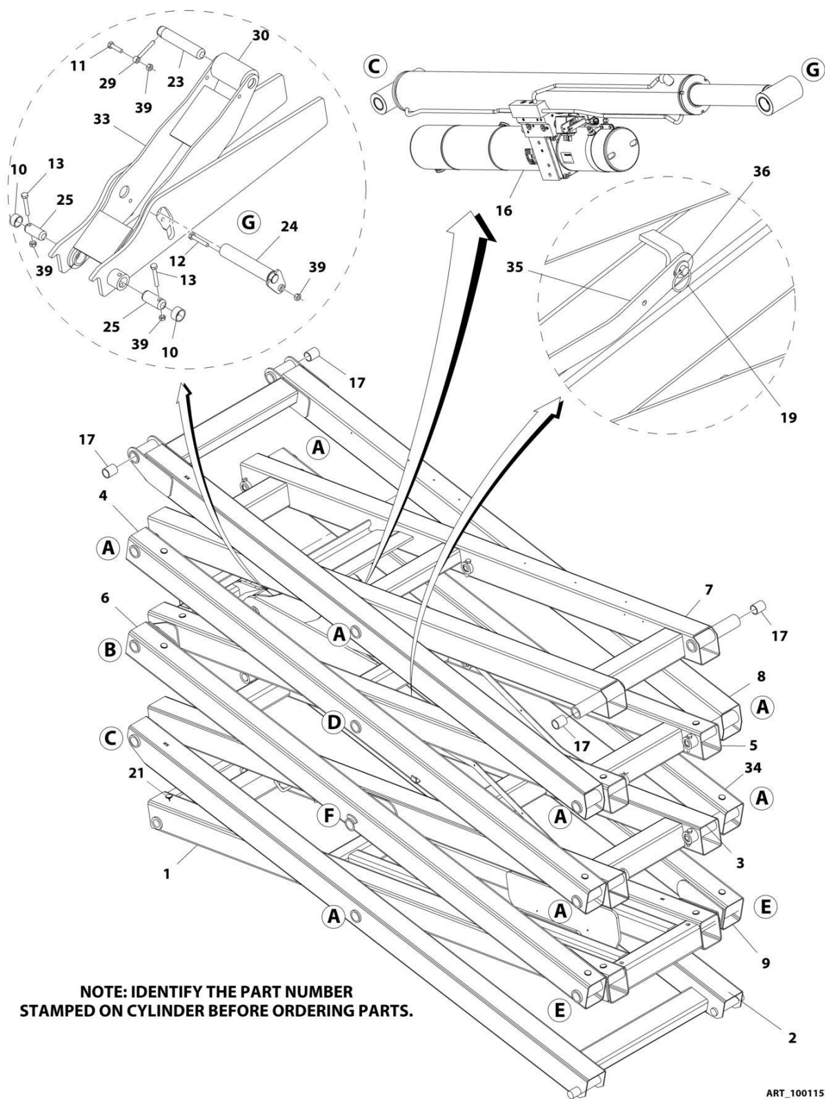
FIGURE 3-18. SCISSORS ARMS ASSEMBLY - STANDARD HYDRAULIC OIL (USA BUILT MACHINES) (3246ES) (SN 0200239382 through 0200241220)
