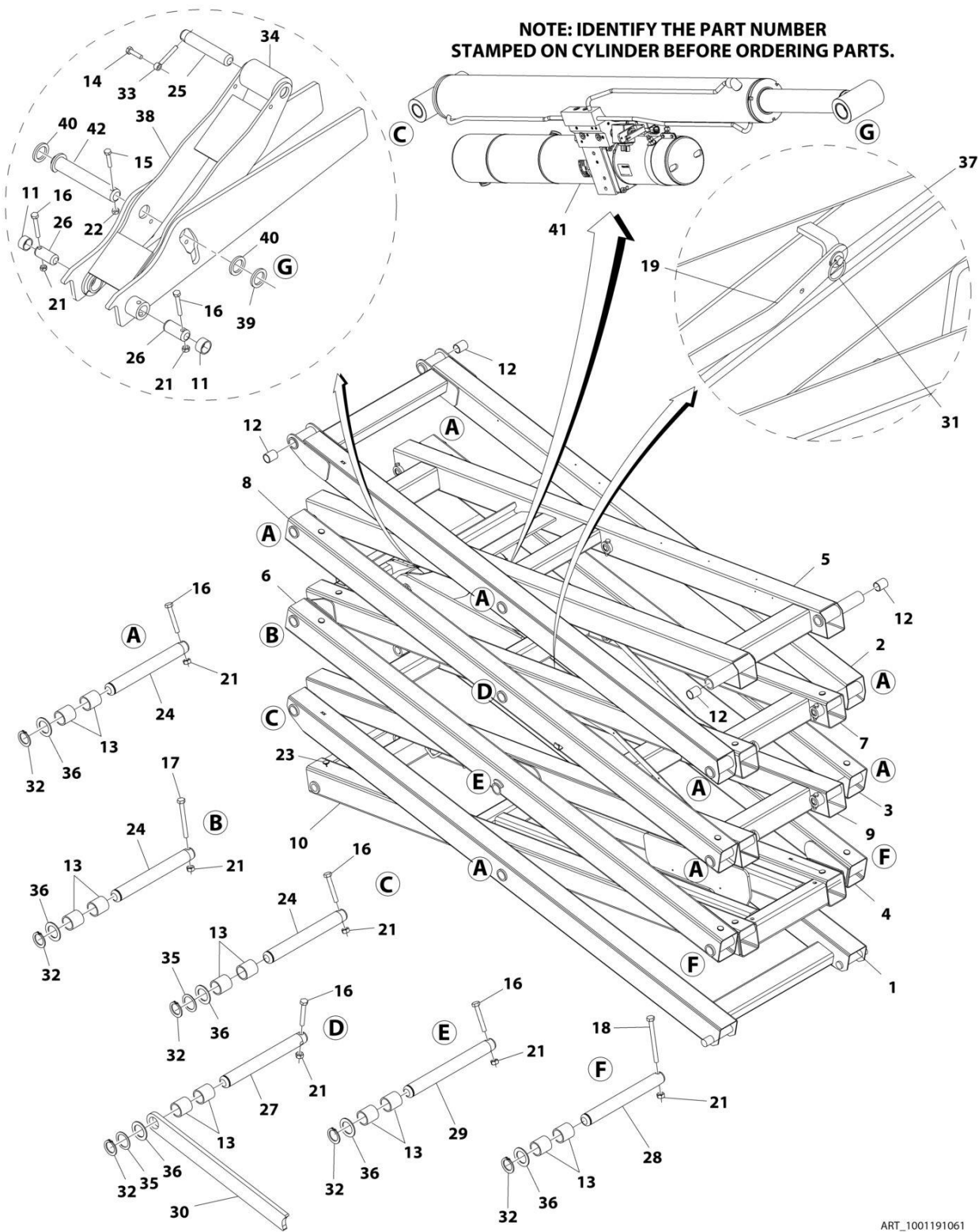
FIGURE 3-12. SCISSORS ARMS ASSEMBLY - BIODEGRADEABLE HYDRAULIC OIL (USA AND MEXICO BUILT MACHINES) (2646ES) (SN 0200241221 to Present, SN M200000100 through M200039292)
