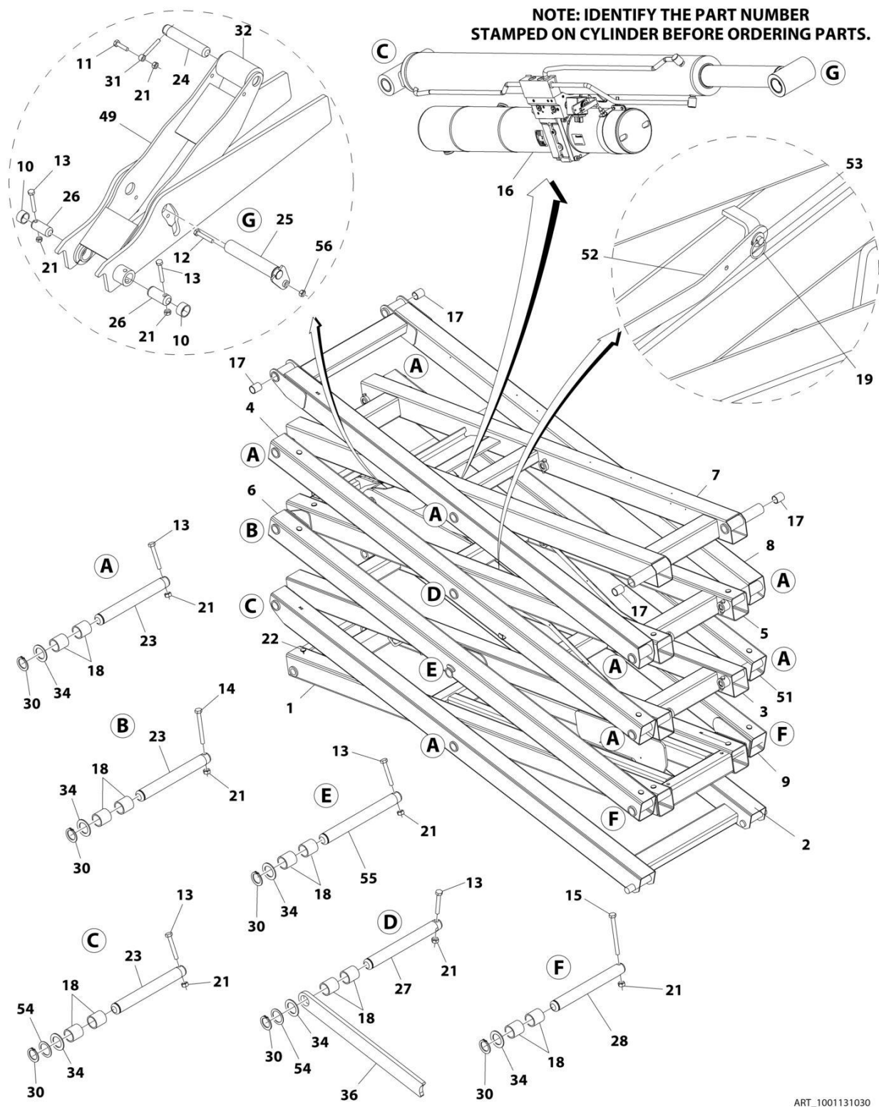
FIGURE 3-14. SCISSORS ARMS ASSEMBLY - BIODEGRADEABLE HYDRAULIC OIL (CHINA BUILT MACHINES) (2646ES) (SN B200020297 through B200020981)
