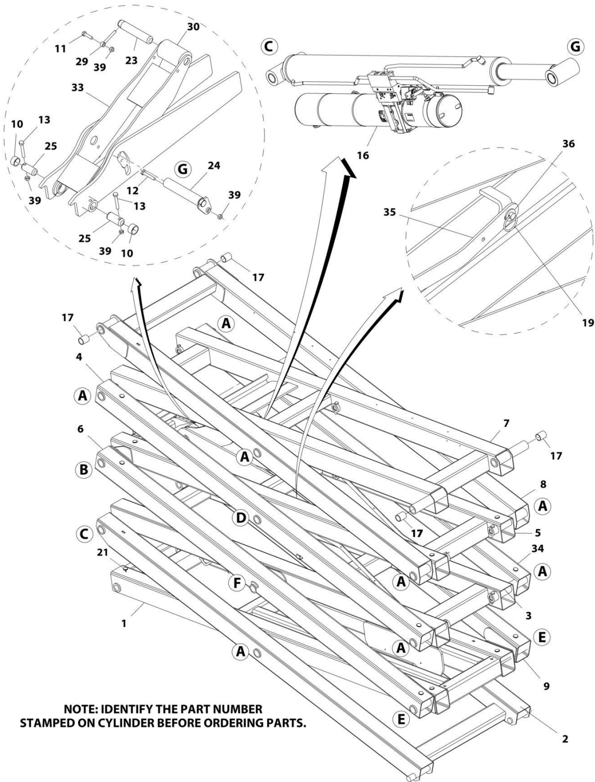
FIGURE 3-26. SCISSORS ARMS ASSEMBLY - BIODEGRADABLE HYDRAULIC OIL (USA BUILT MACHINES) (3246ES) (SN 0200239382 through 0200241220)
