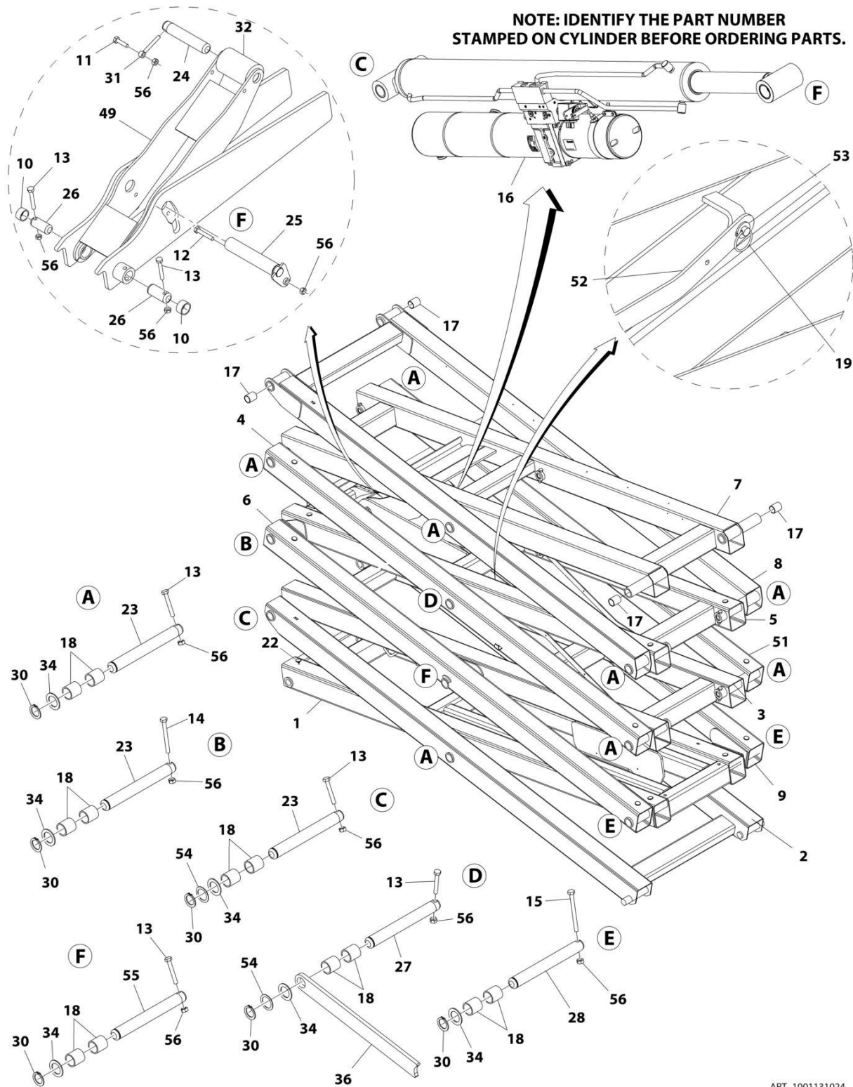
FIGURE 3-6. SCISSORS ARMS ASSEMBLY - STANDARD HYDRAULIC OIL (CHINA BUILT MACHINES) (2646ES) (SN B200020297 through B200020981)
