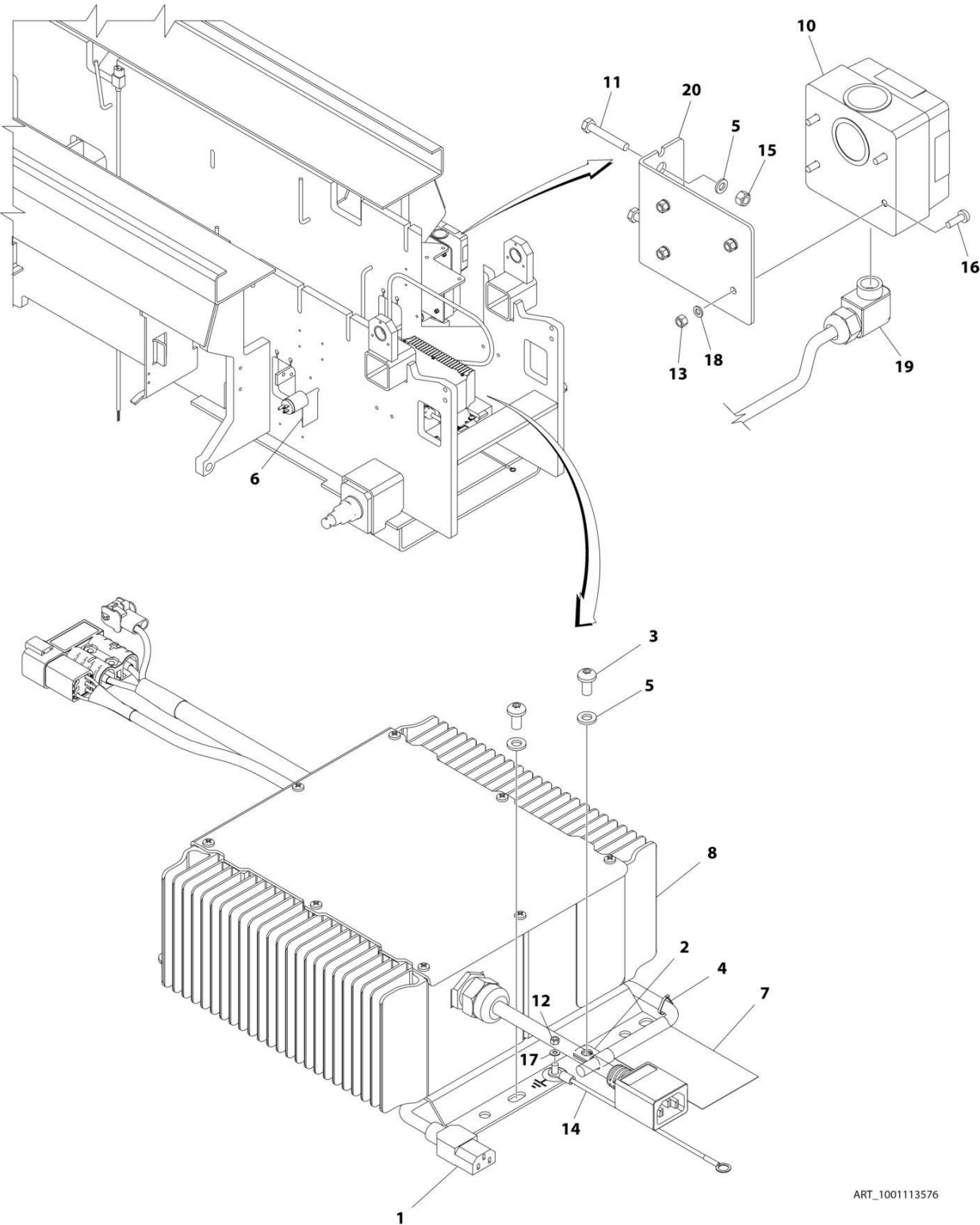
FIGURE 1-14. BATTERY CHARGER INSTALLATION WITH LOCALLY SUPPLIED PLUG (AUSTRALIAN SPEC) (SN 0200239382 to Present, SN B200020297 through B200061738, SN M200000100 to Present, SN 1200025021 to Present)
