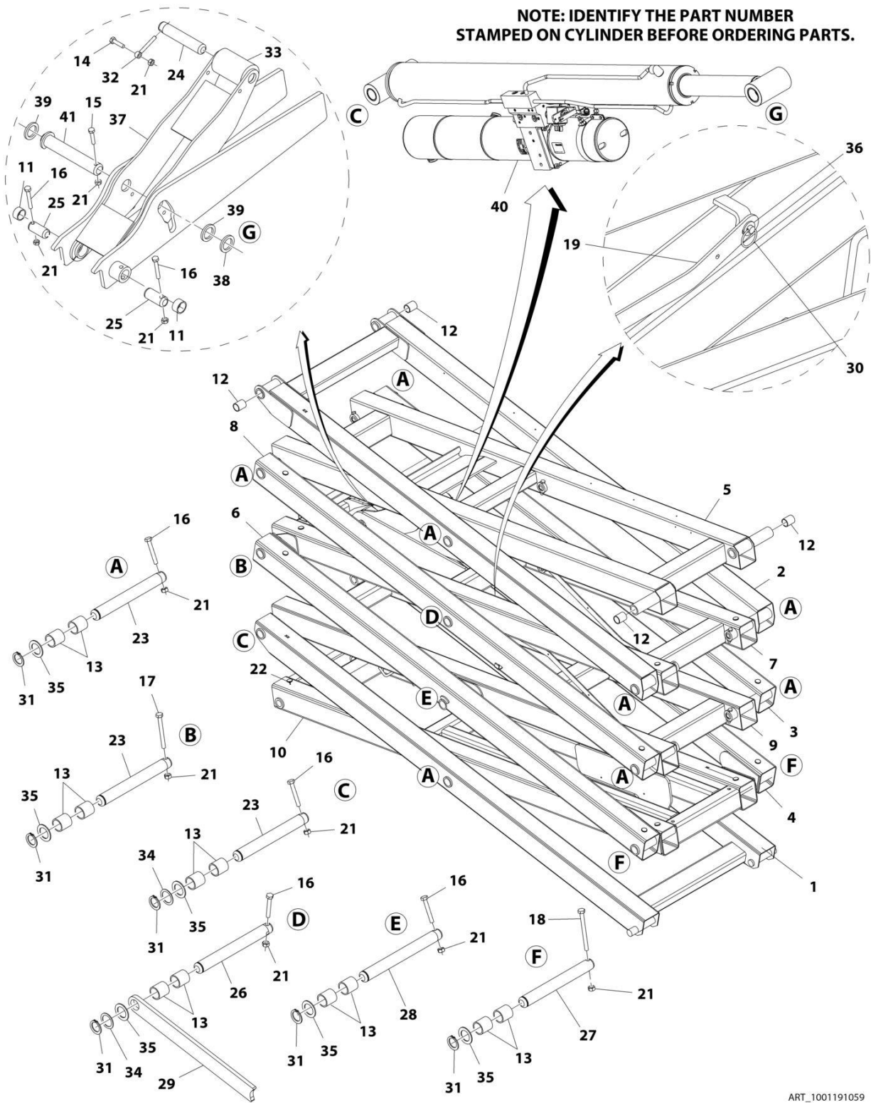
FIGURE 3-4. SCISSORS ARMS ASSEMBLY - STANDARD HYDRAULIC OIL (USA AND MEXICO BUILT MACHINES) (2646ES) (SN 0200241221 to Present, SN M200000100 through M200039292)
