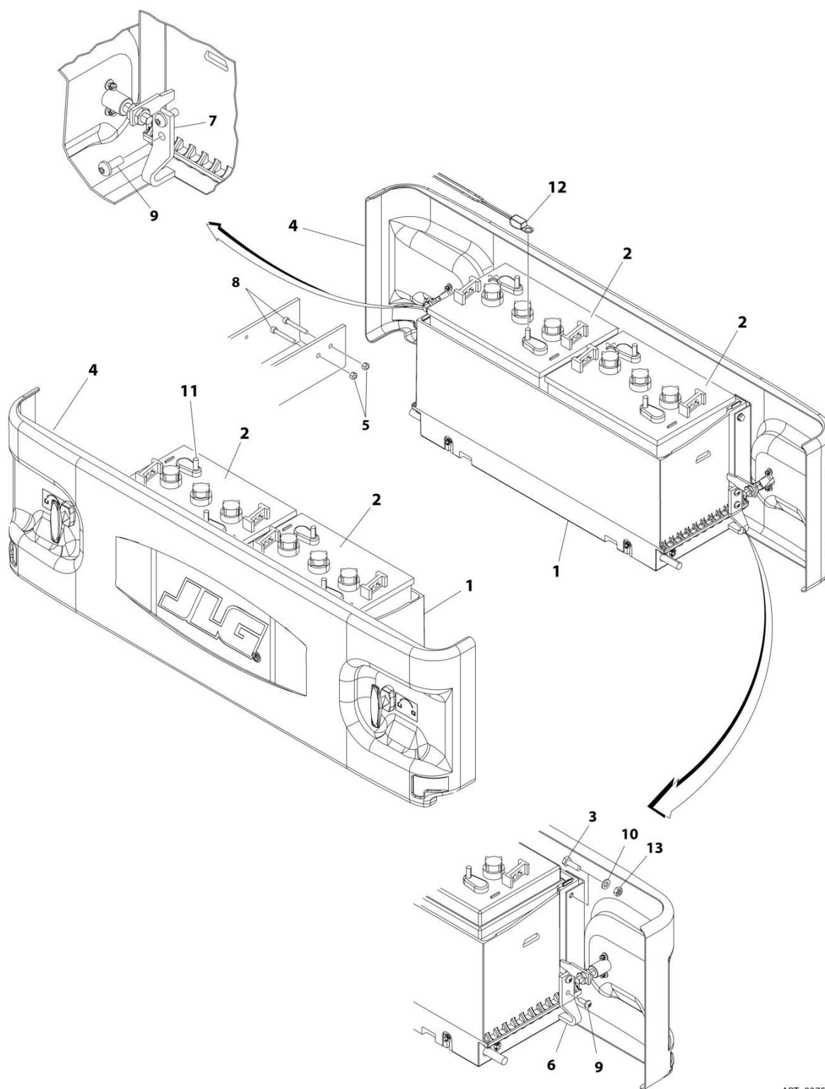
FIGURE 2-23. BATTERIES INSTALLATION - EV TYPE - 244 AH RATING (UL LOCKING COVERS)
