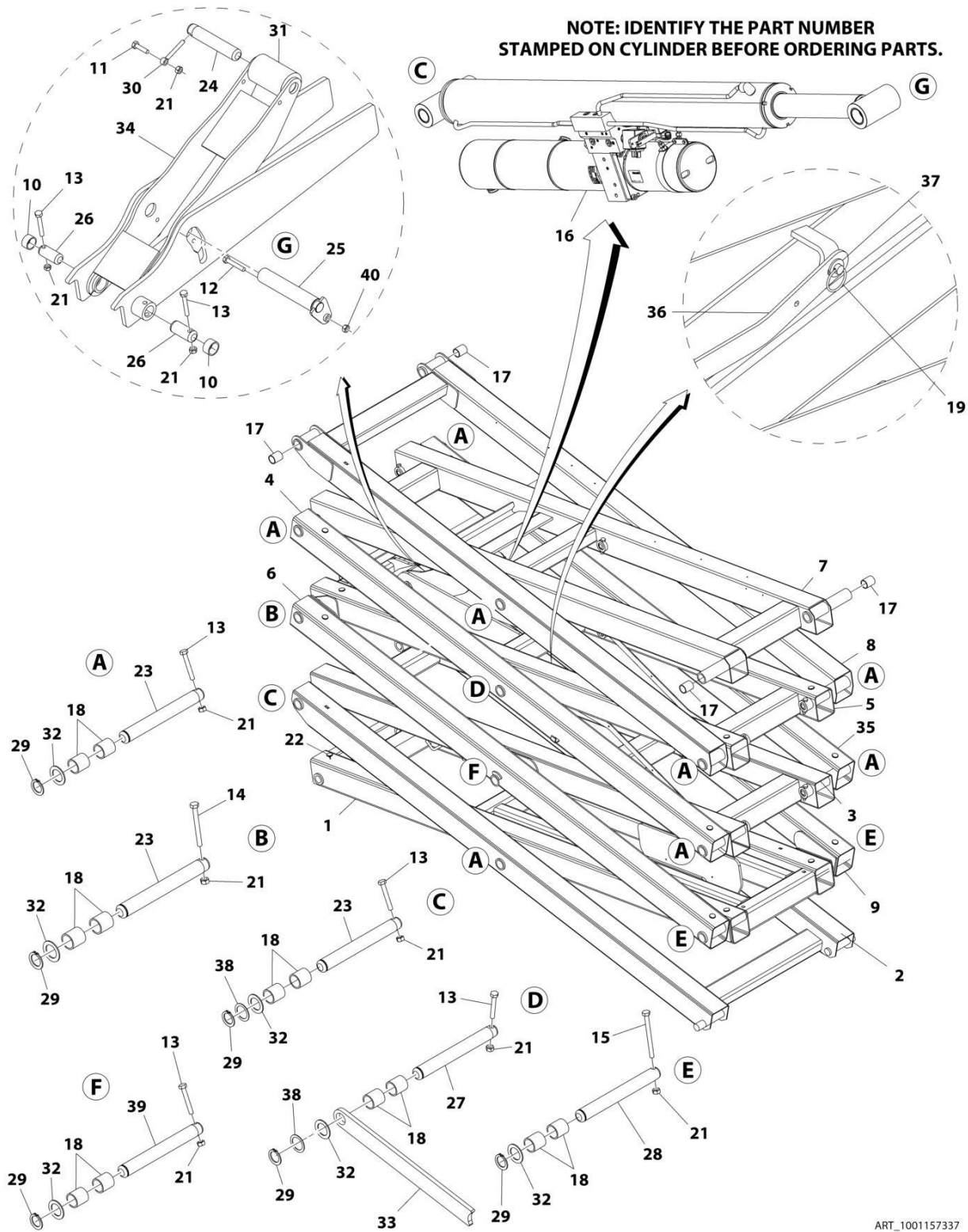
FIGURE 3-10. SCISSORS ARMS ASSEMBLY - BIODEGRADABLE HYDRAULIC OIL (USA BUILT MACHINES) (2646ES) (SN 0200239382 through 0200241220)
