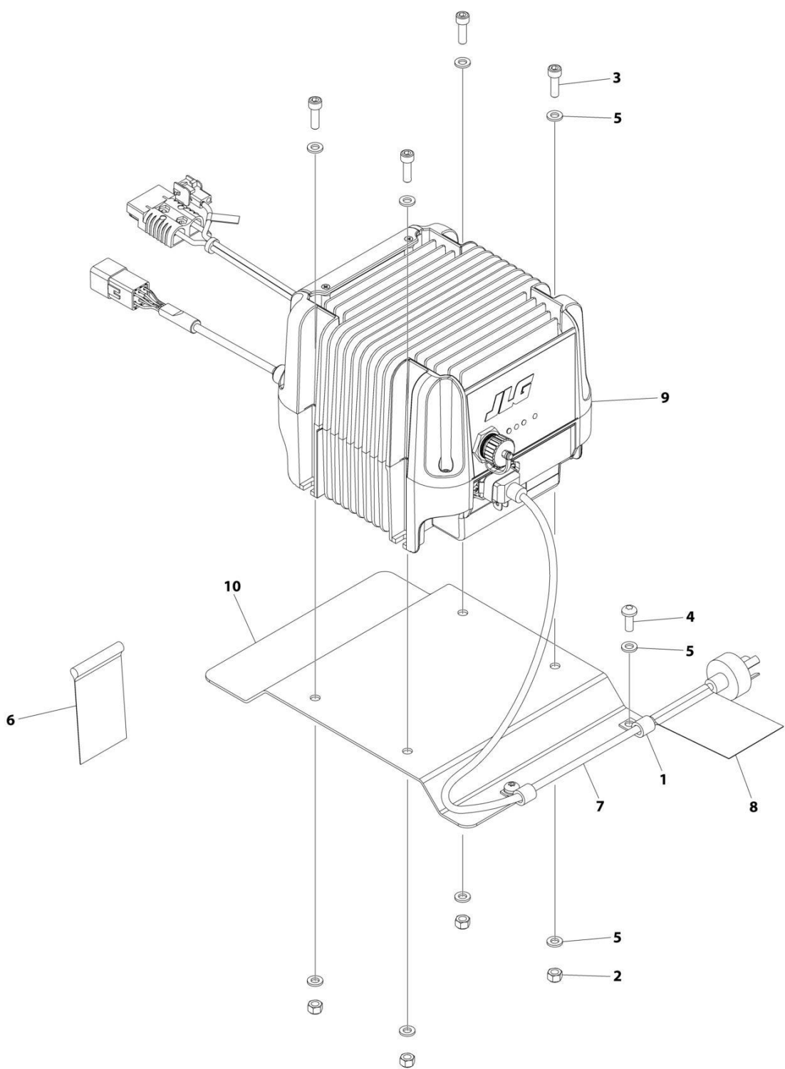
FIGURE 1-23. BATTERY CHARGER INSTALLATION - GREEN POWER (CHINESE PLUG) (CHINESE SPECS) (SN 0200238382 through 0200261035, SN B200020297 through B200036742, SN M200000100 through M200007339)
