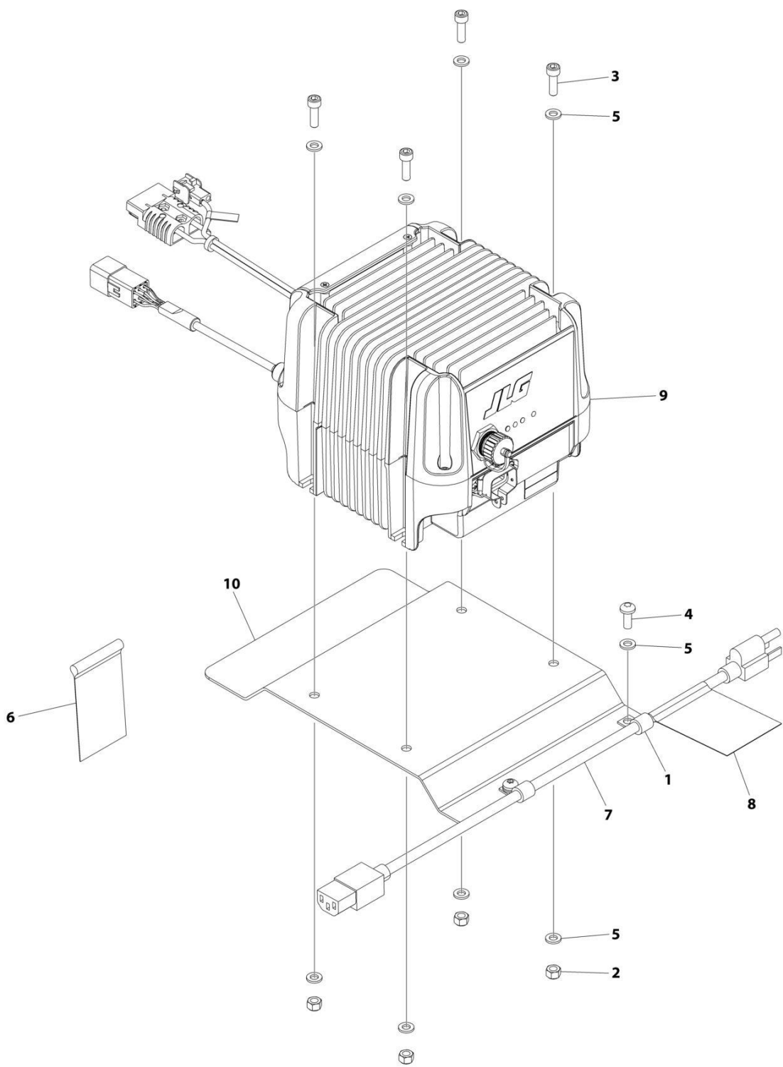
FIGURE 1-26. BATTERY CHARGER INSTALLATION - GREEN POWER (110V PLUG) (JAPANESE SPECS)
