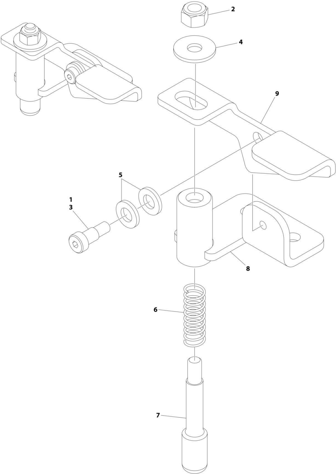
FIGURE 4-8. LATCH ASSEMBLY - WITH INSIDE EXTENSION RAILS (SN 1200030234 to Present, SN B200051185 to Present, SN M200021521 through M200039292)
