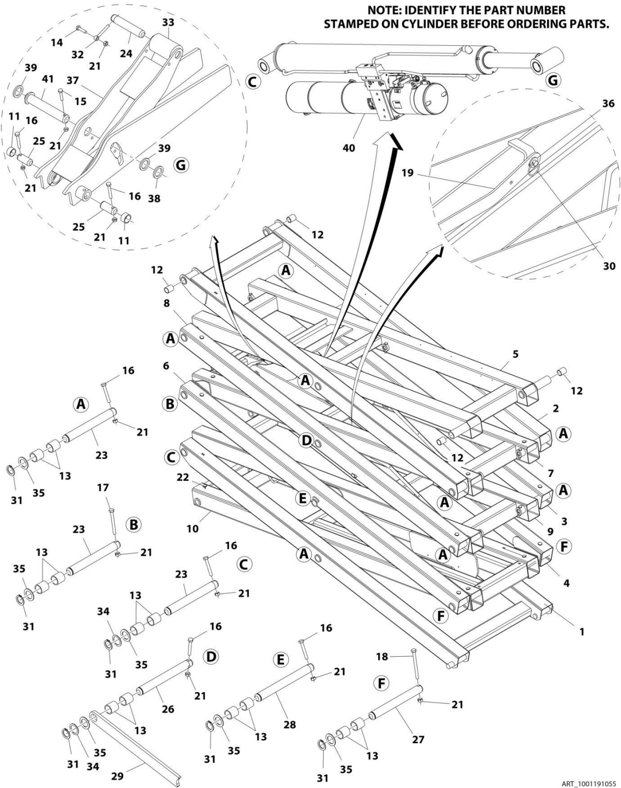
FIGURE 3-8. SCISSORS ARMS ASSEMBLY - STANDARD HYDRAULIC OIL (CHINA BUILT MACHINES) (2646ES) (SN B200020982 to Present)
