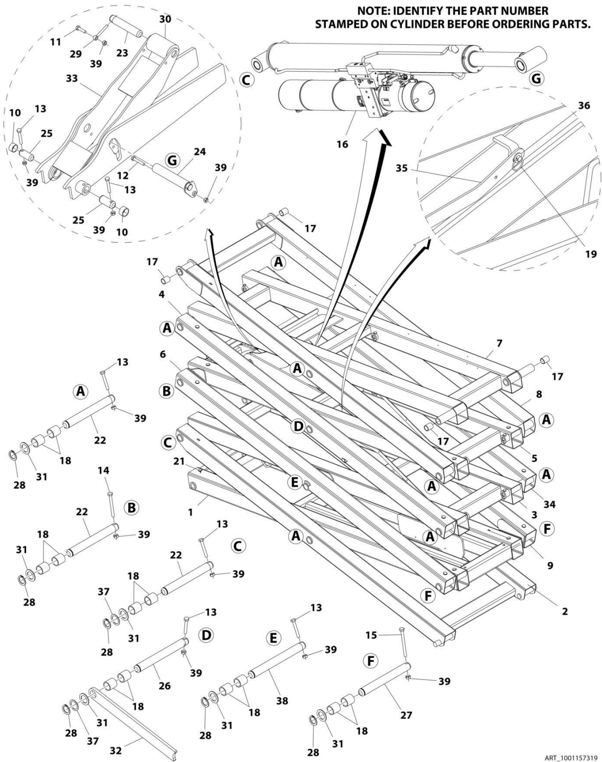
FIGURE 3-2. SCISSORS ARMS ASSEMBLY - STANDARD HYDRAULIC OIL (USA BUILT MACHINES) (2646ES) (SN 0200239382 through 0200241220)
