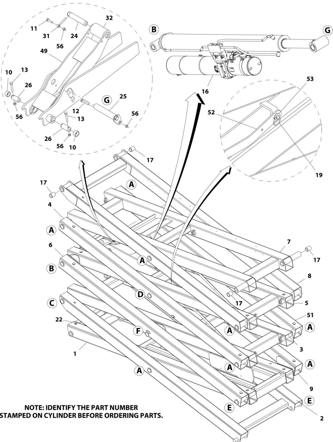
FIGURE 3-30. SCISSORS ARMS ASSEMBLY - BIODEGRADABLE HYDRAULIC OIL (CHINA BUILT MACHINES) (3246ES) (SN B200020297 through B200020981)
