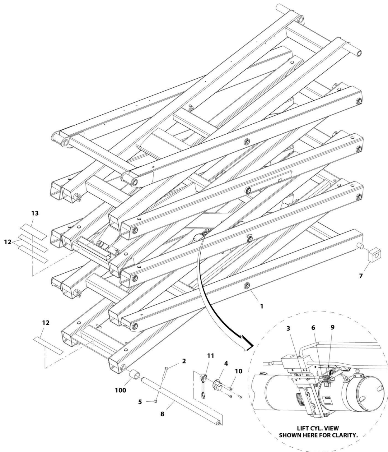
FIGURE 3-25. SCISSOR ARMS INSTALLATION - BIODEGRADEABLE HYDRAULIC OIL (USA BUILT MACHINES) (3246ES) (SN 0200239382 through 0200241220)
