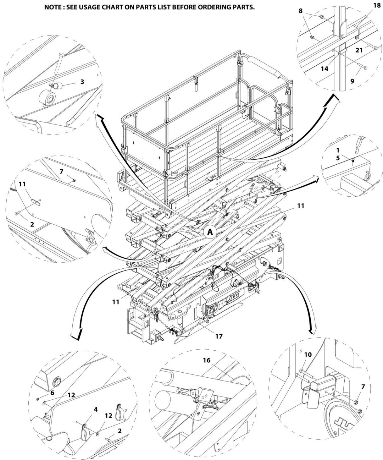
DETAIL A
