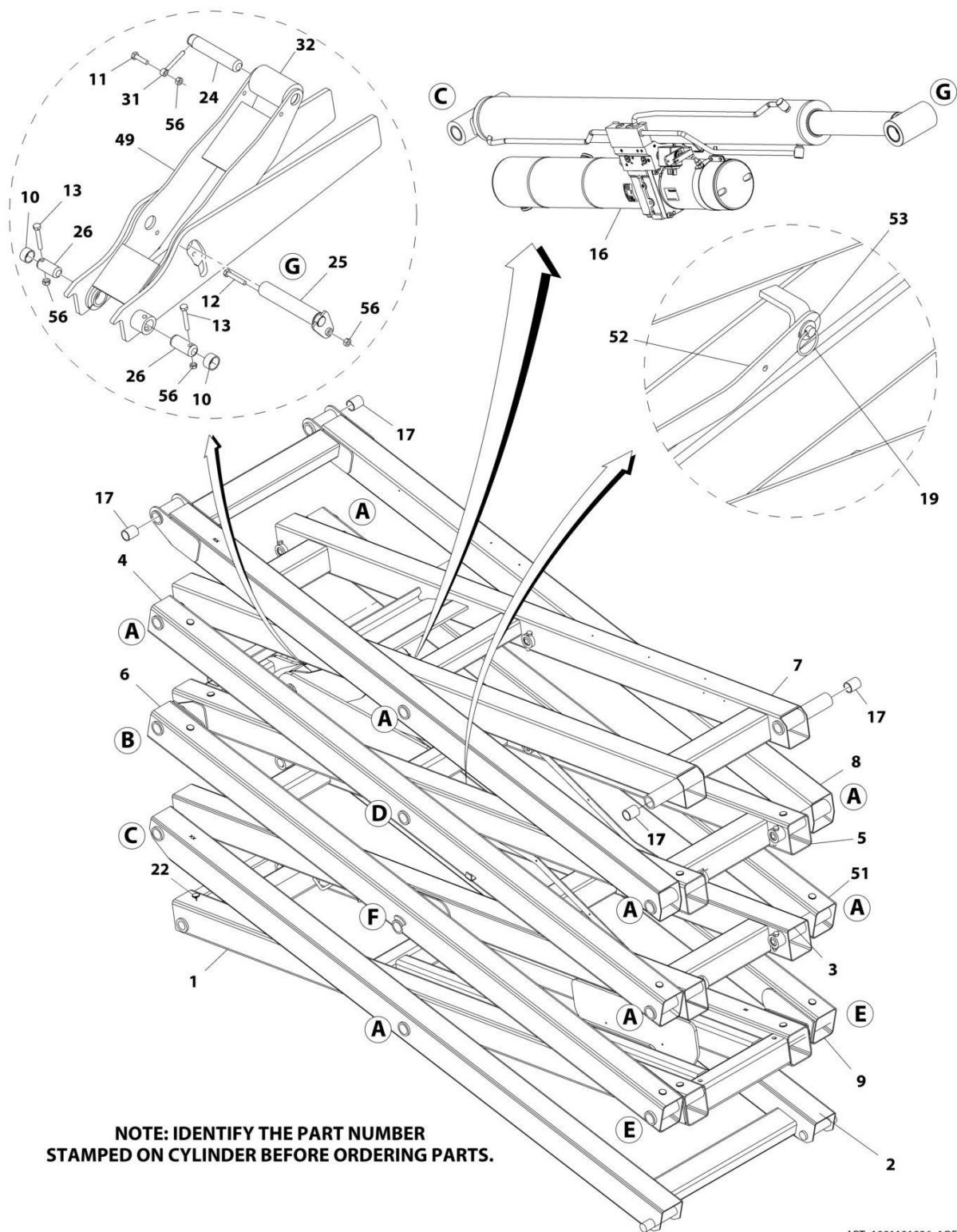
FIGURE 3-22. SCISSORS ARMS ASSEMBLY - STANDARD HYDRAULIC OIL (CHINA BUILT MACHINES) (3246ES) (SN B200020297 through B200020981)
