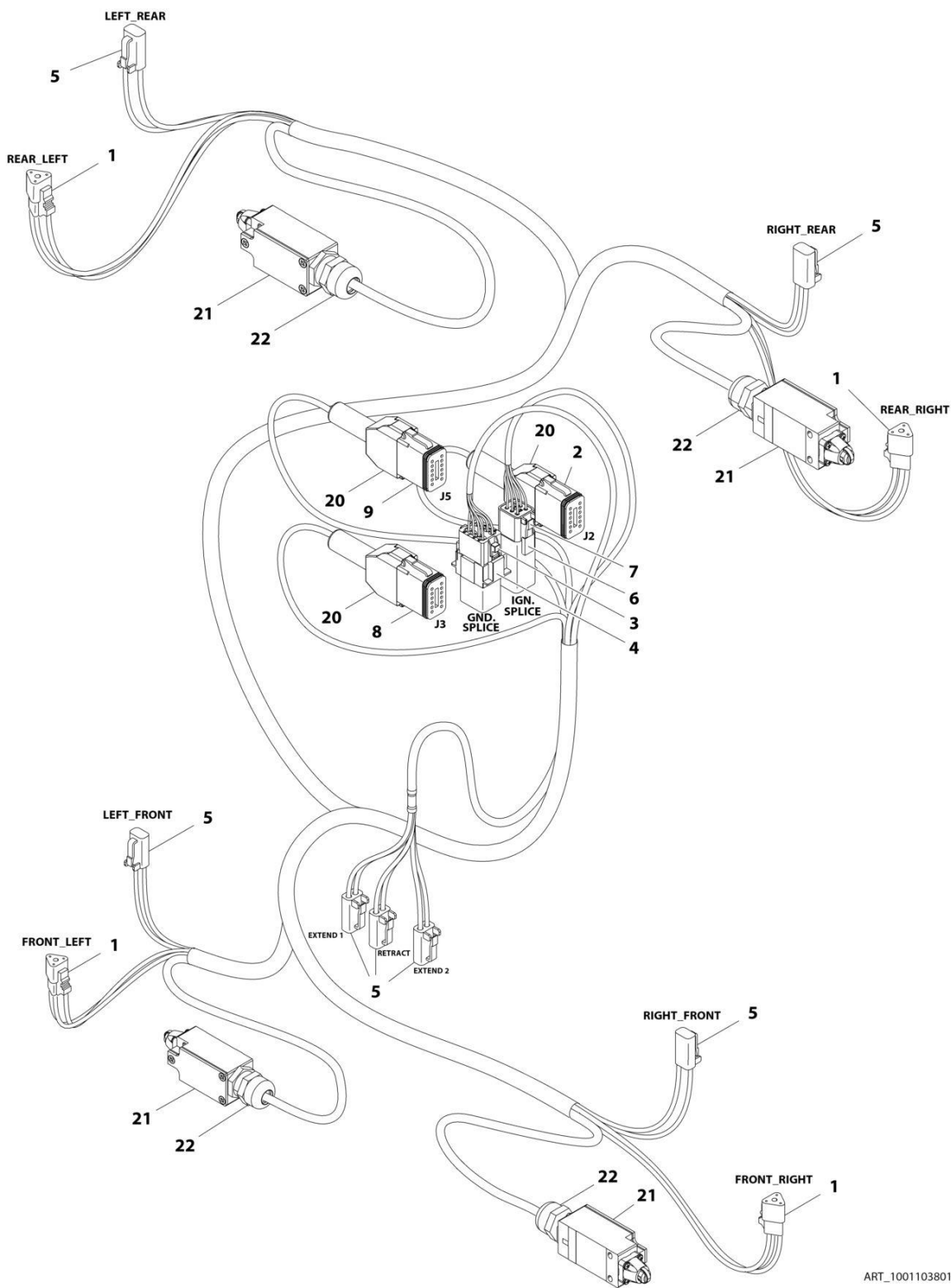
FIGURE 8-39. LEVELING JACK HARNESS
