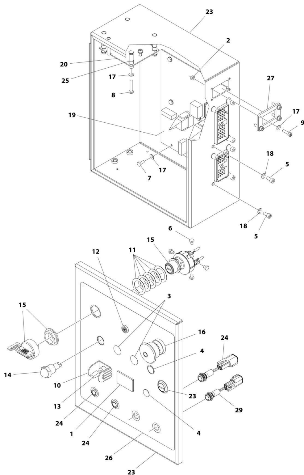
FIGURE 2-12. GROUND CONTROL BOX ASSEMBLY - KUBOTA GASOLINE
