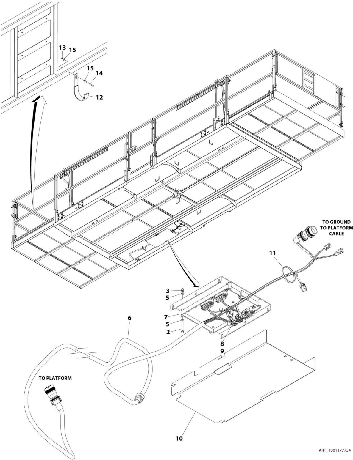
FIGURE 5-10. PLATFORM MODULE INSTALLATION
