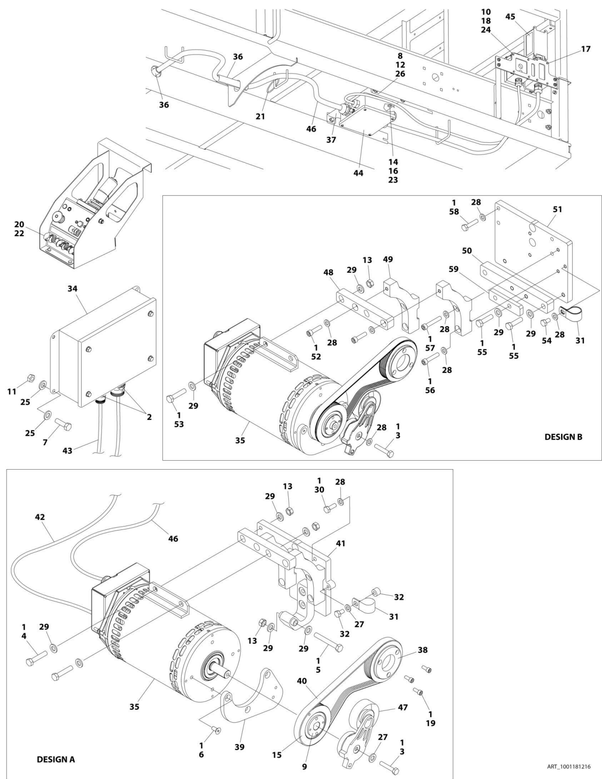
FIGURE 3-22. GENERATOR INSTALLATION - 4000W (KUBOTA GASOLINE) (DUAL FUEL)
