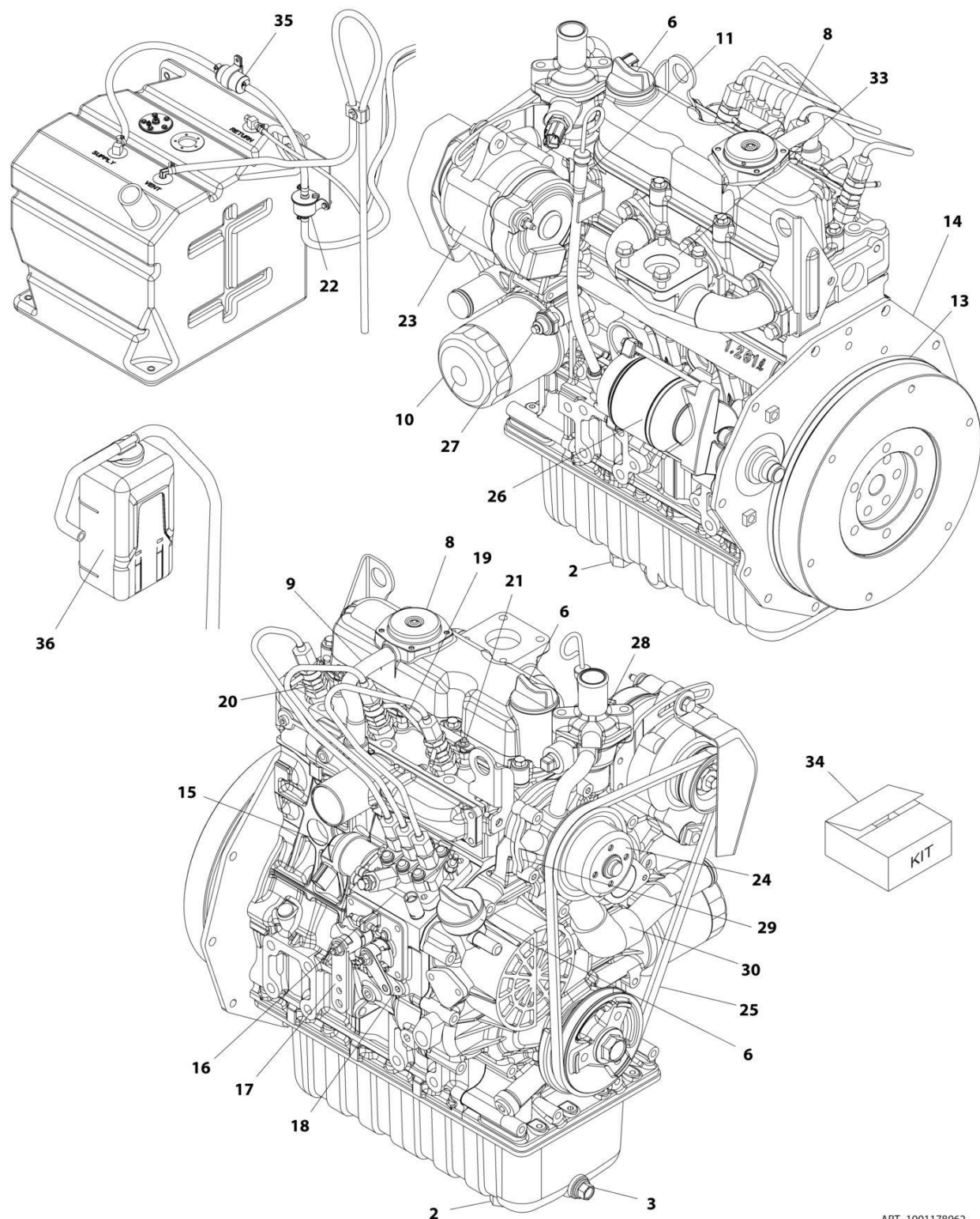
FIGURE 3-8. ENGINE COMPONENTS - KUBOTA DIESEL T4F
