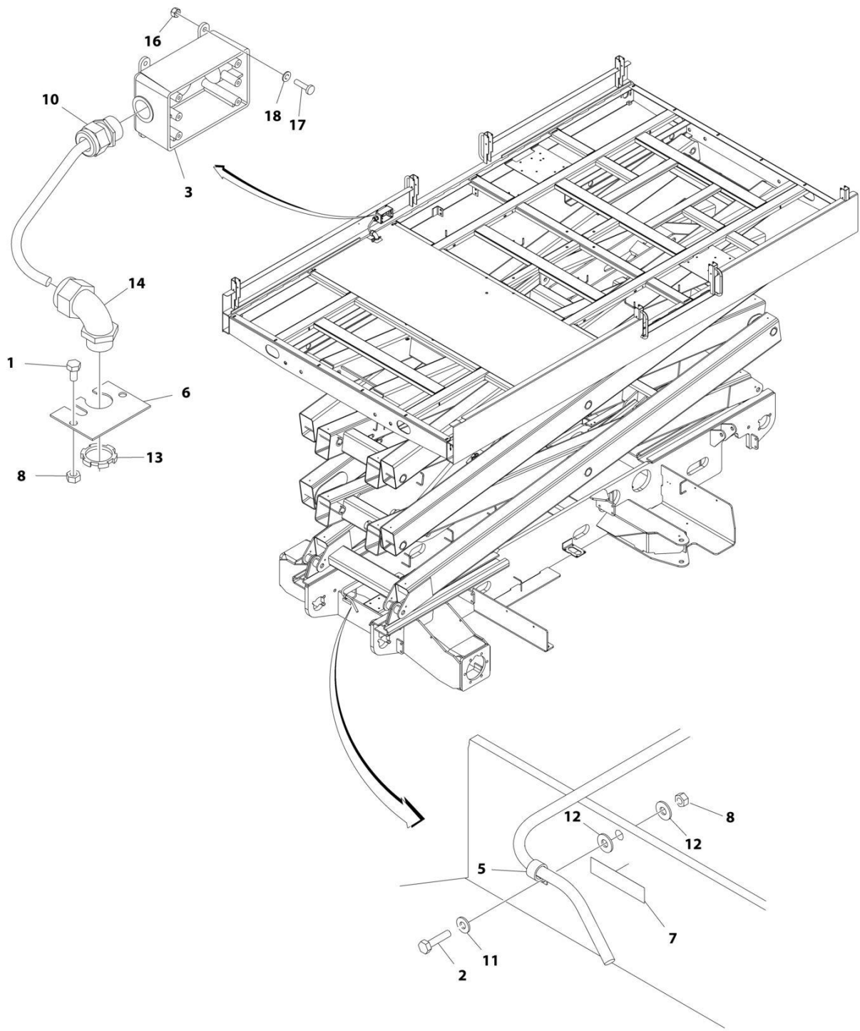
FIGURE 8-4. AC BOX AT PLATFORM INSTALLATION - 220V (ANSI AND ANSI EXPORT SPECS) (Prior to SN E200000130)
