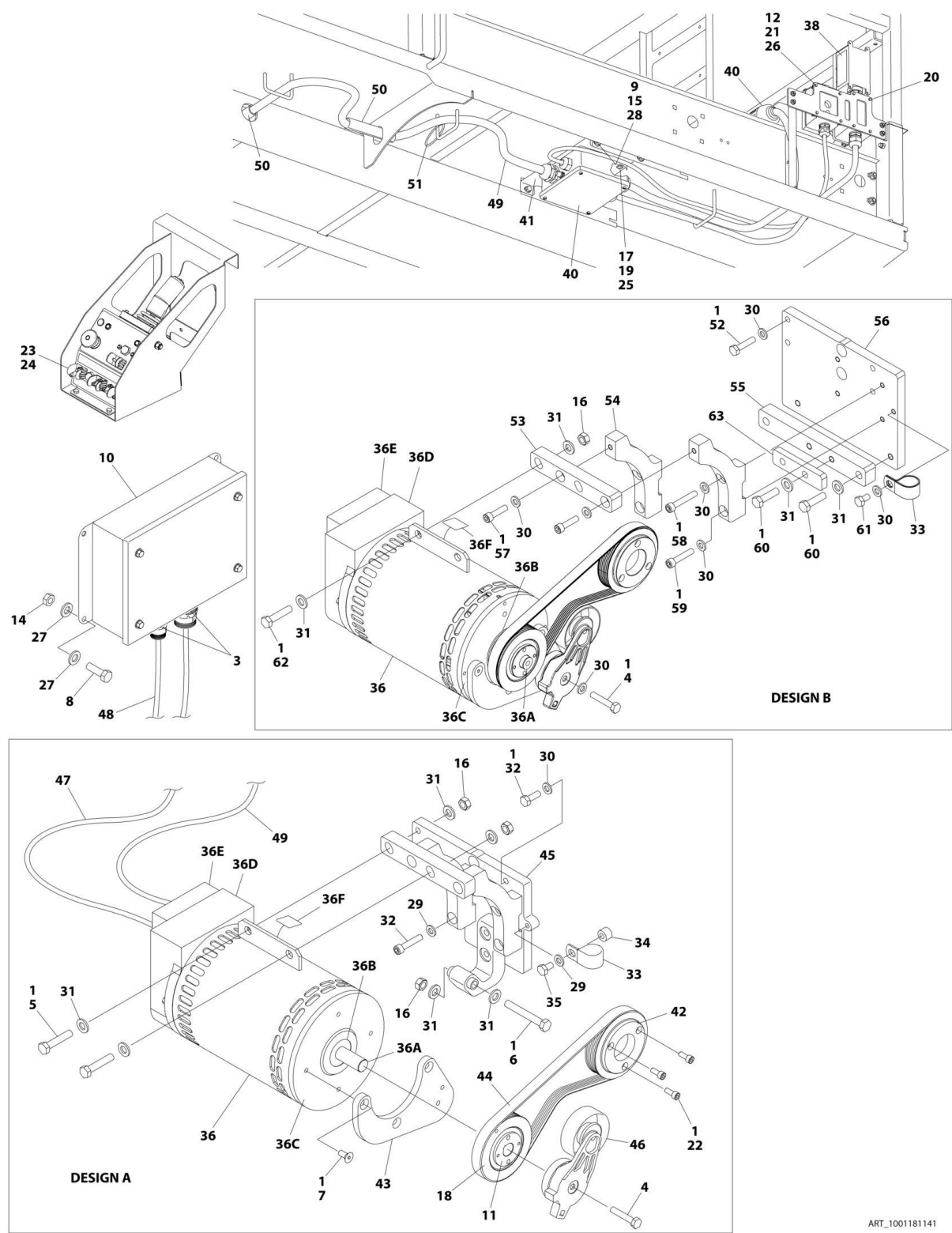
FIGURE 3-25. GENERATOR INSTALLATION - 7500W (KUBOTA GASOLINE) (DUAL FUEL)
