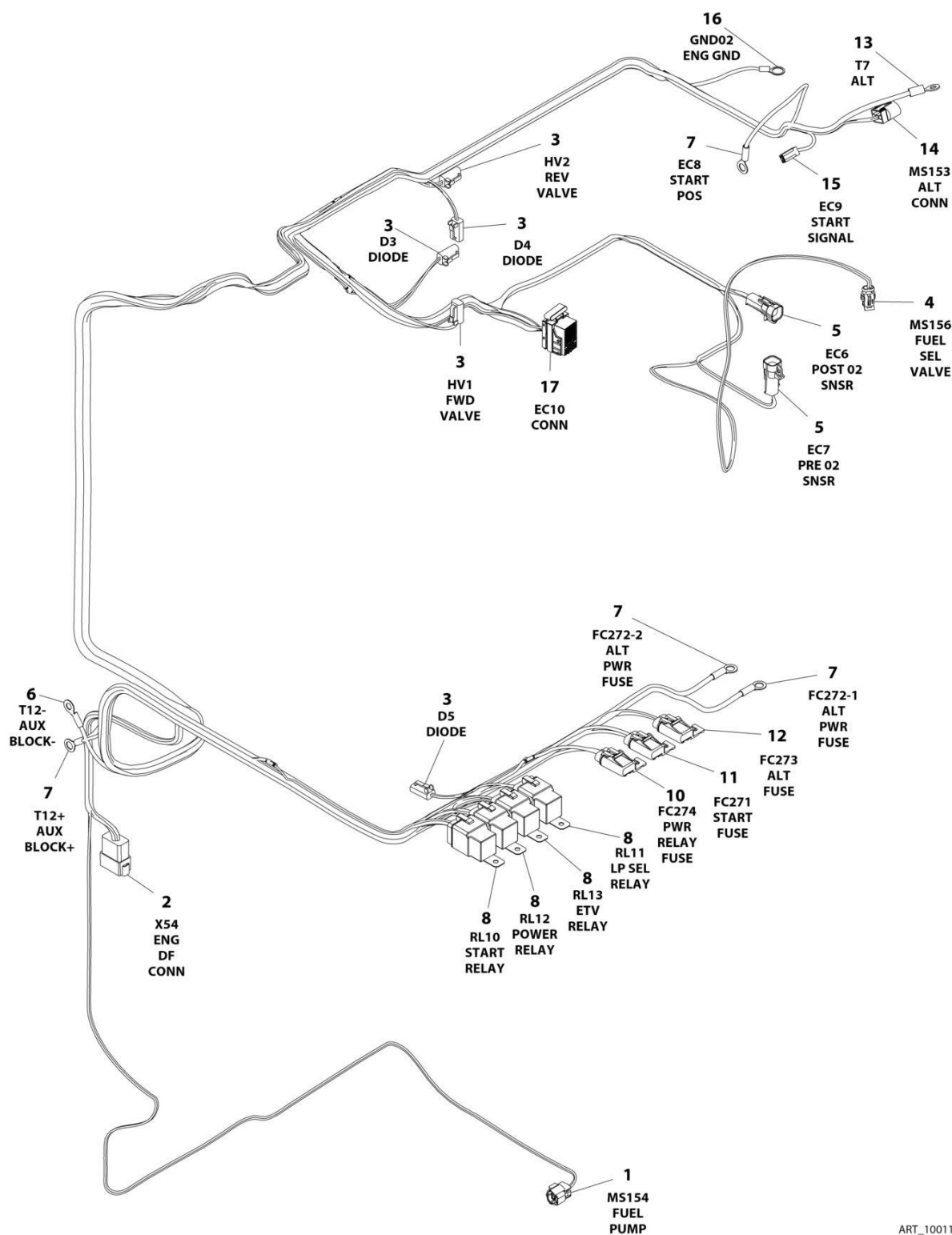
FIGURE 8-28. ENGINE HARNESS - KUBOTA GASOLINE
