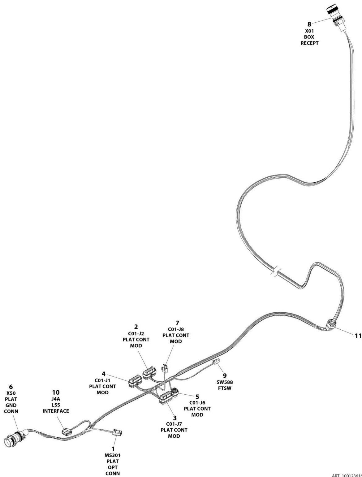
FIGURE 8-36. PLATFORM MODULE TO CONSOLE BOX HARNESS
