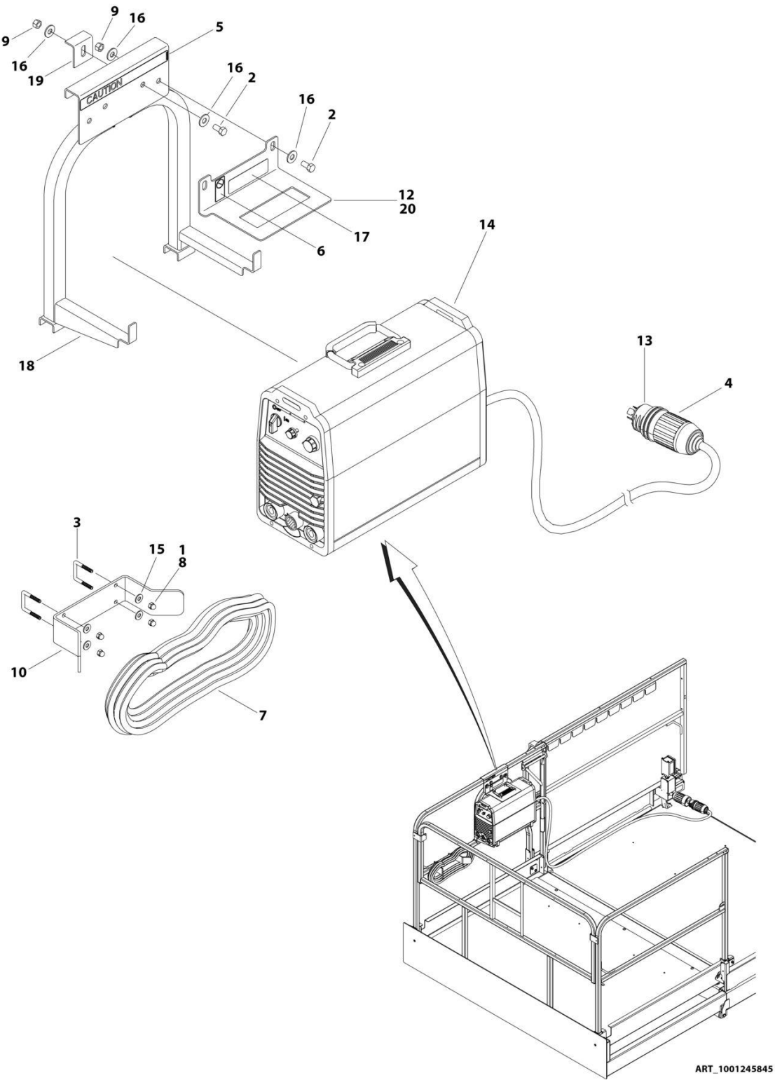
FIGURE 5-12. SKYWELDER INSTALLATION (OPTIONAL) (ANSI SPECS)
