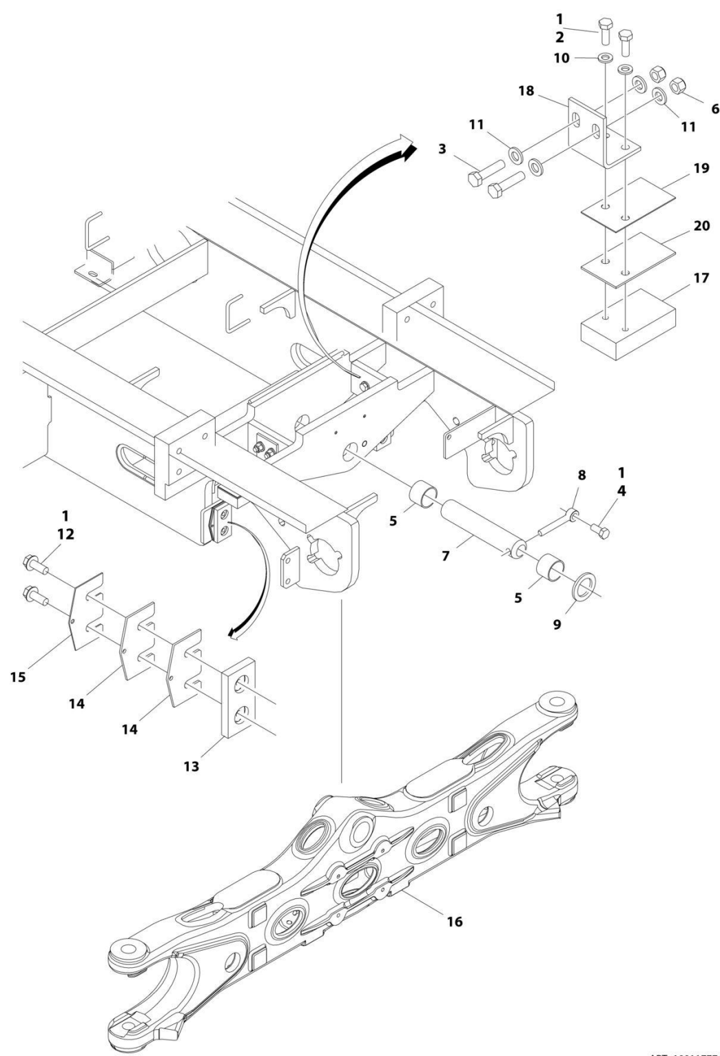
FIGURE 1-1. AXLE INSTALLATION - FIXED
