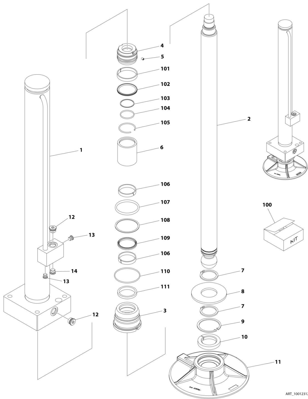
FIGURE 6-5. LEVELING JACK CYLINDER ASSEMBLY (SN E200000706 through E200000900)
