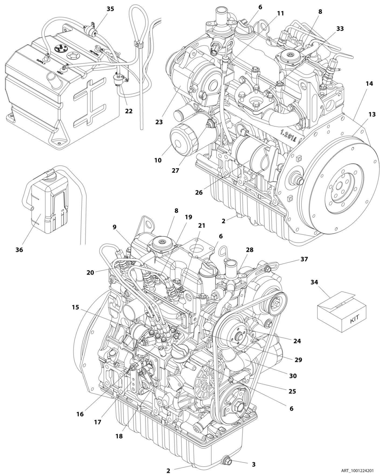
FIGURE 3-7. ENGINE COMPONENTS - KUBOTA DIESEL STAGE III (SN E200000676 through E200000730)
