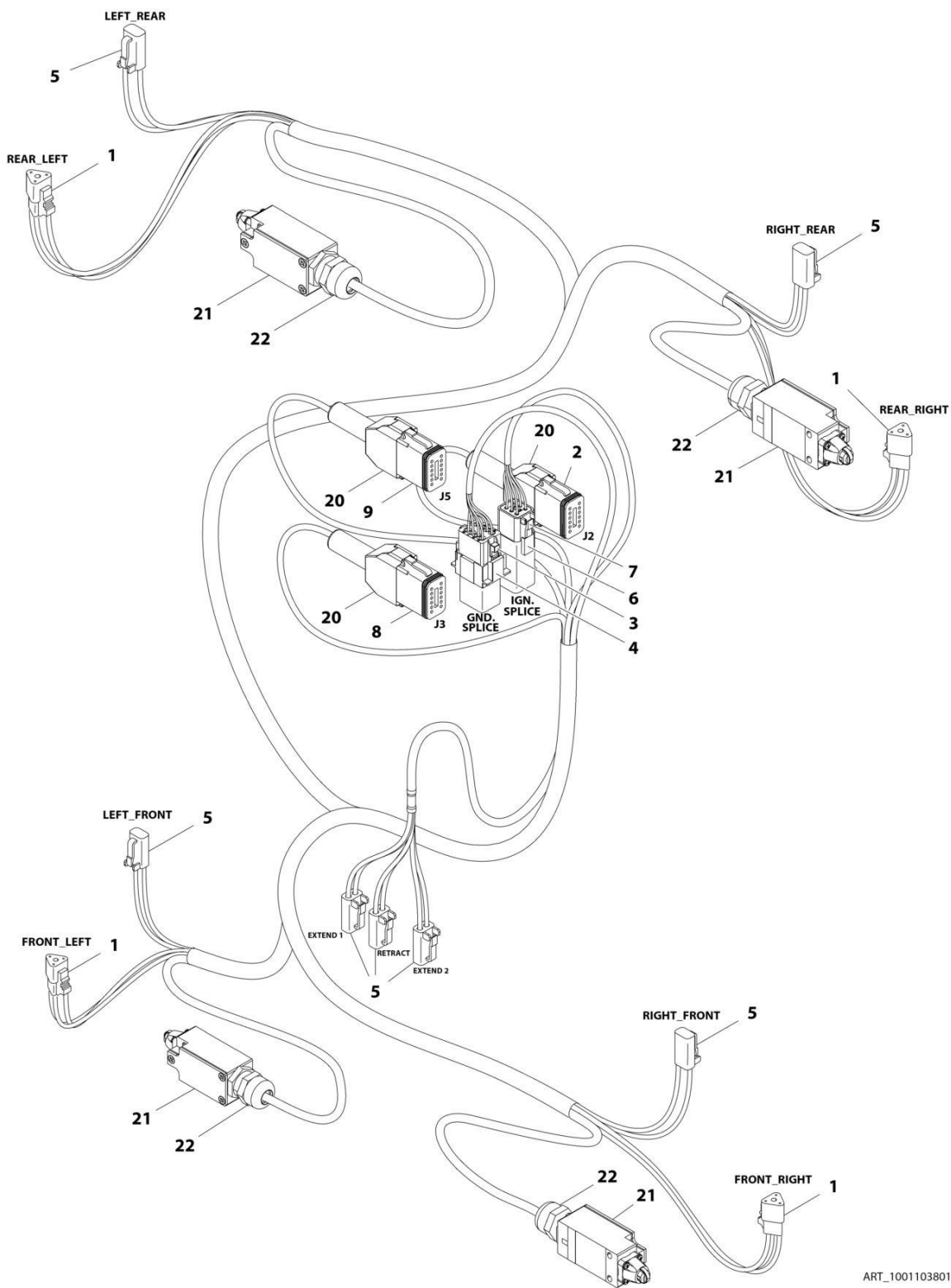
FIGURE 8-32. LEVELING JACK HARNESS
