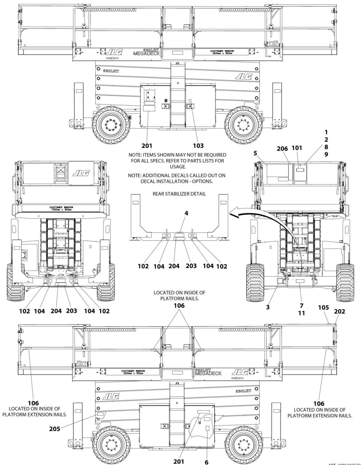
FIGURE 9-8. ECAL INSTALLATION - LATIN AMERICAN SPECS (ENGLISH/SPANISH)
