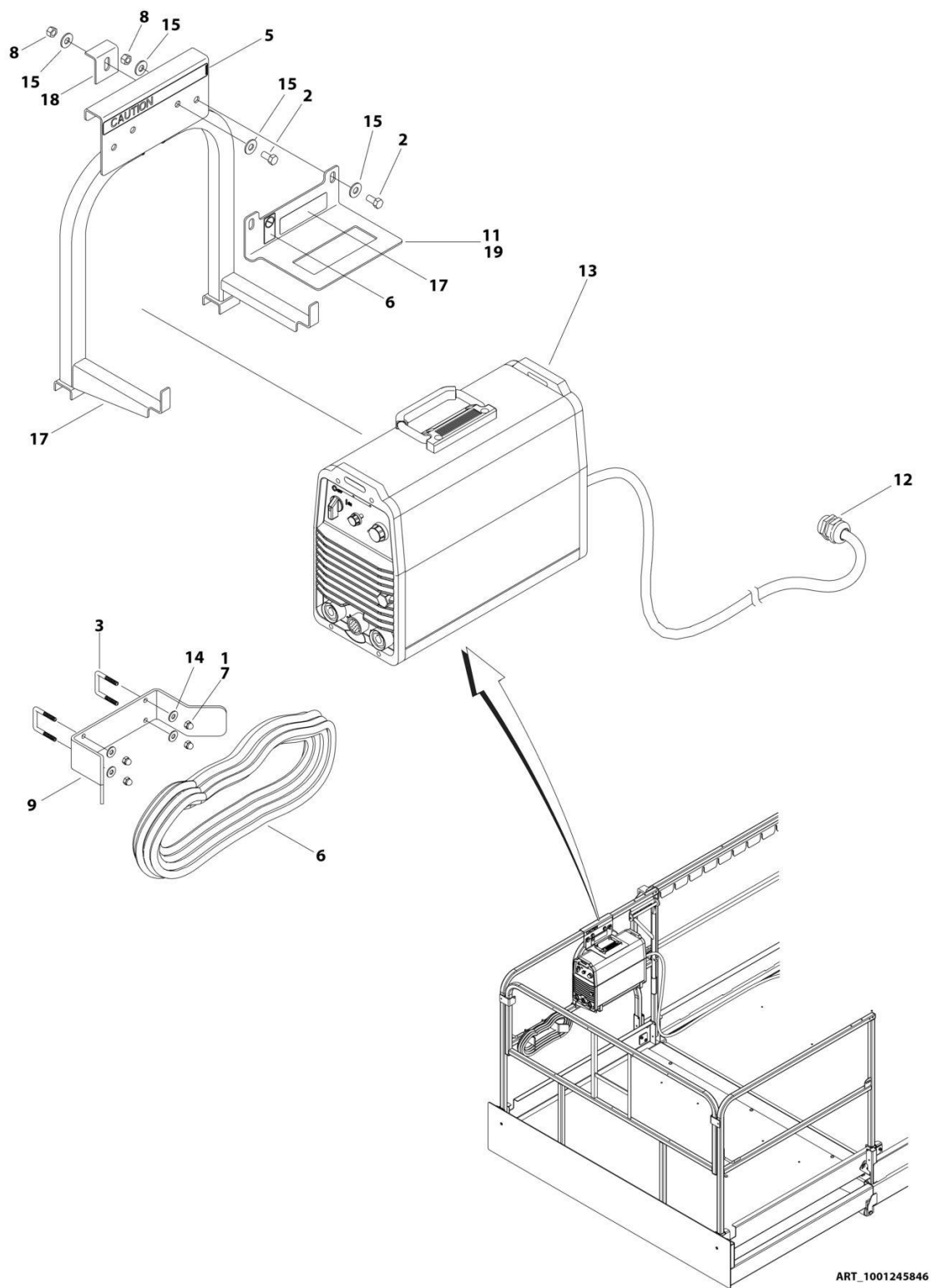
FIGURE 5-13. SKYWELDER INSTALLATION (OPTIONAL) (CE SPECS)
