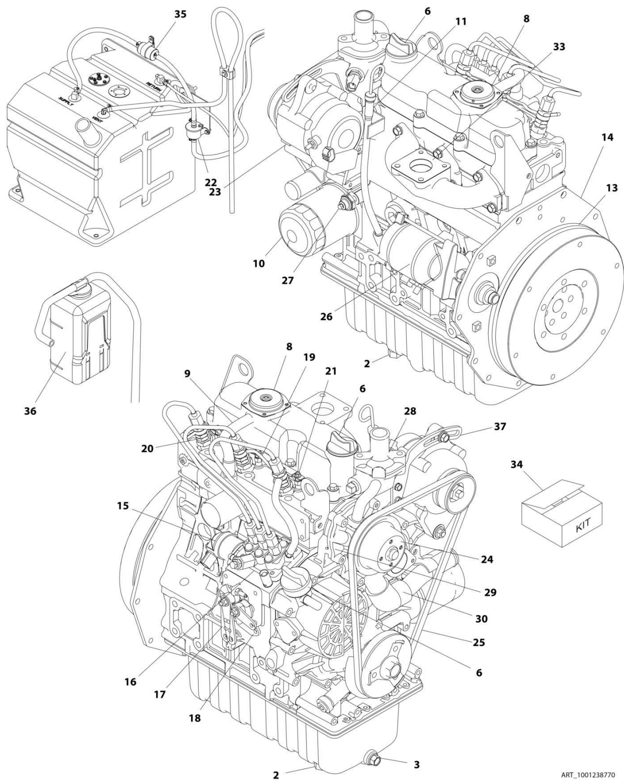
FIGURE 3-19. ENGINE COMPONENTS - KUBOTA DIESEL T4F (SN E200000723 through E200000900)
