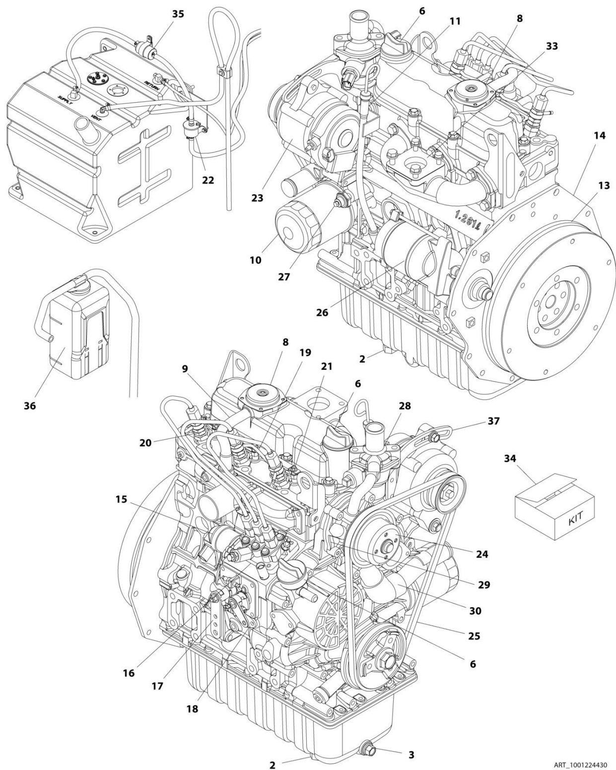
FIGURE 3-18. ENGINE COMPONENTS - KUBOTA DIESEL T4F (SN E200000676 through E200000722)
