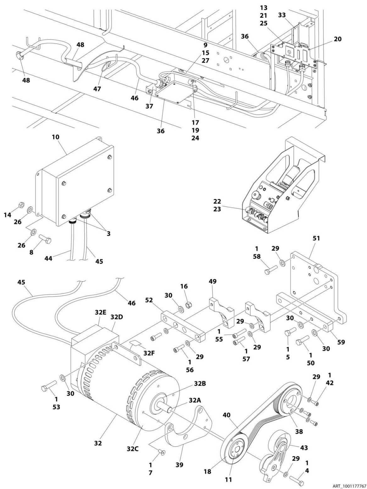
FIGURE 3-37. GENERATOR INSTALLATION - 7500W (KUBOTA DIESEL T4F)
