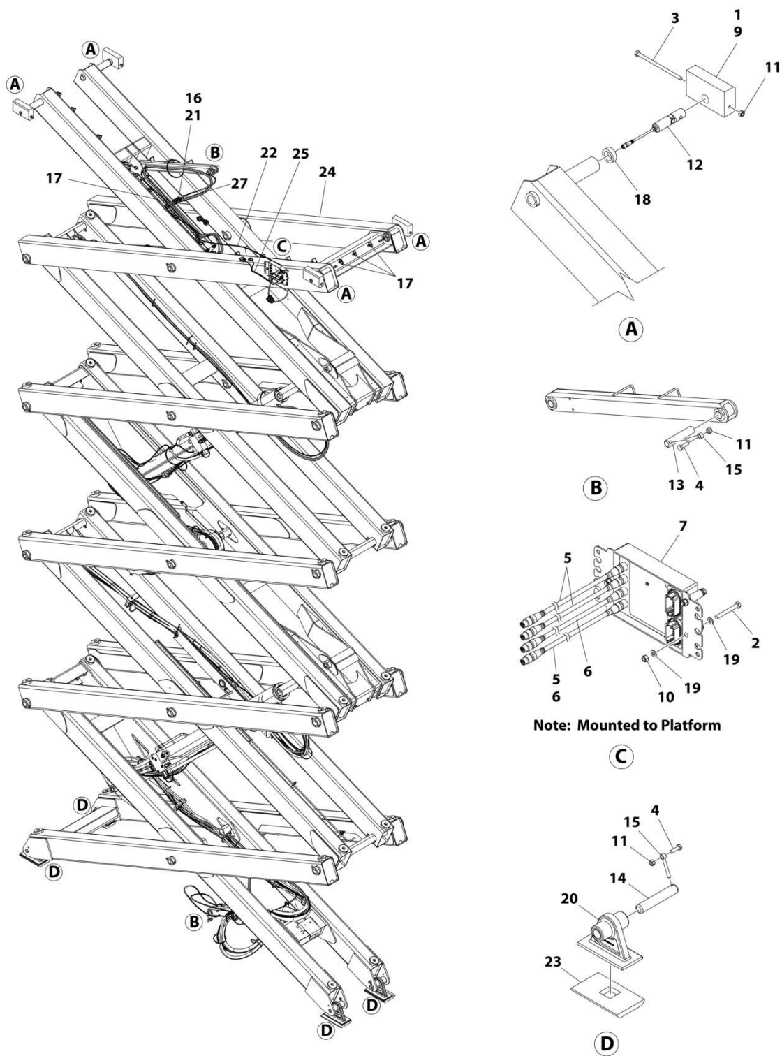
FIGURE 4-2. SCISSORS ARMS INSTALLATION WITH AC CABLE
