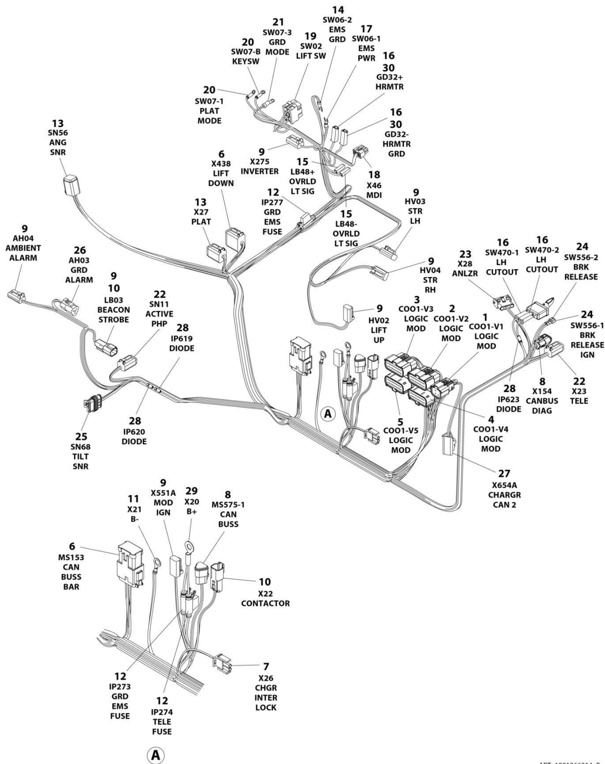
FIGURE 7-25. CHASSIS HARNESS (WITH LSS WITH PLATFORM DRIVE SELECT SWITCH) (CHINA & MEXICO BUILT MACHINES) (SN B200059250 to Present)
