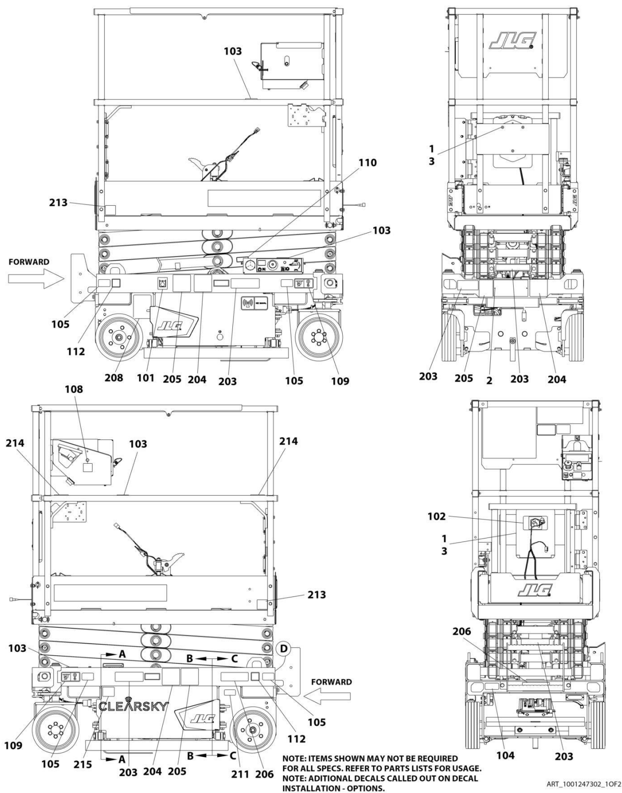
FIGURE 8-6. DECALS INSTALLATION (KOREAN SPECS)
