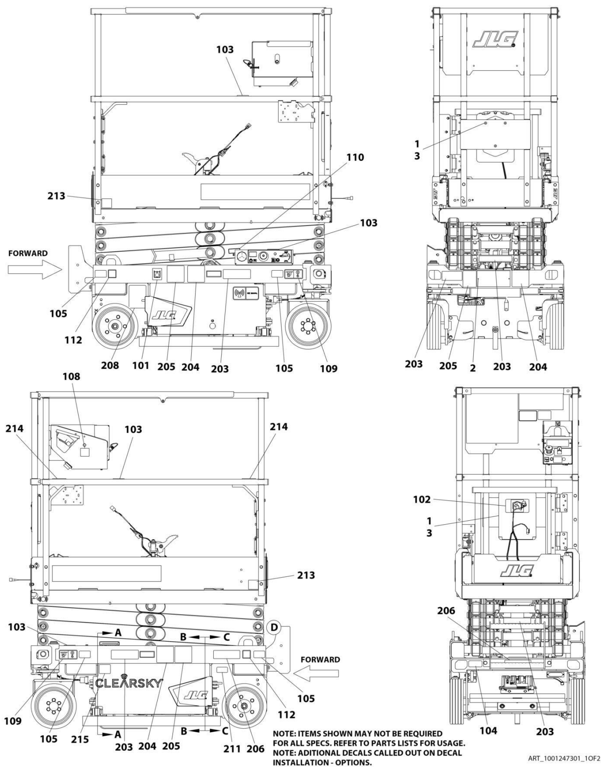
FIGURE 8-1. DECALS INSTALLATION (ANSI SPECS)
