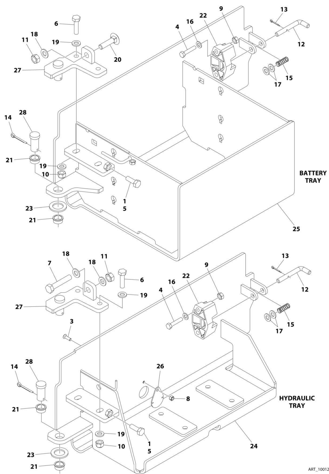
FIGURE 2-16. DOORS INSTALLATION
