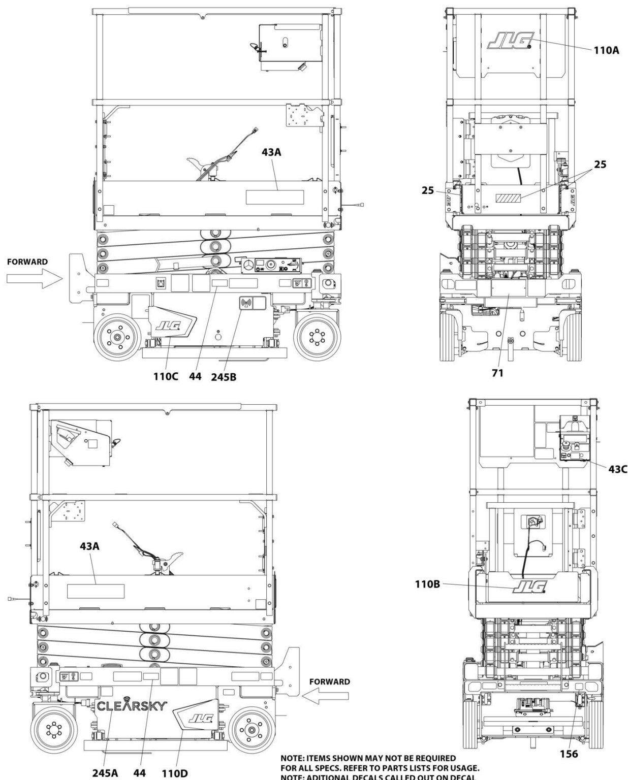
FIGURE 8-7. DECAL INSTALLATION - OPTIONS
