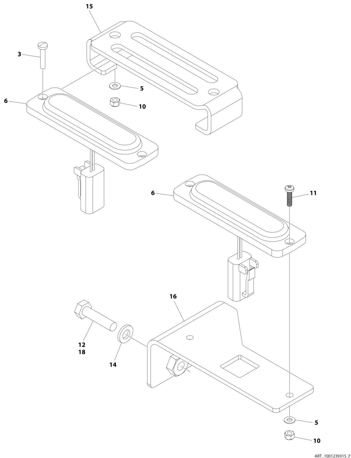
FIGURE 1-24. STROBE LIGHT INSTALLATION - DUAL (AMBER) (WITH GUARD) (SN B200062116 through B200065232)
