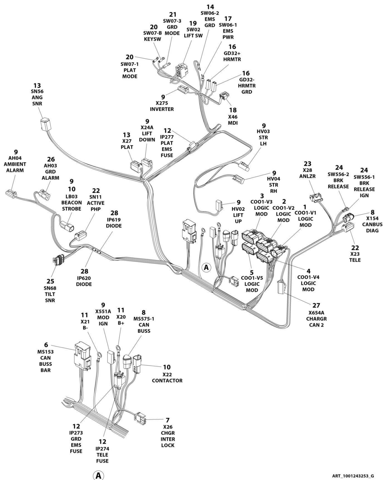
FIGURE 7-22. CHASSIS HARNESS (WITHOUT LSS WITHOUT PLATFORM DRIVE SELECT SWITCH) (CHINA BUILT MACHINES) (Prior to SN B200059250)
