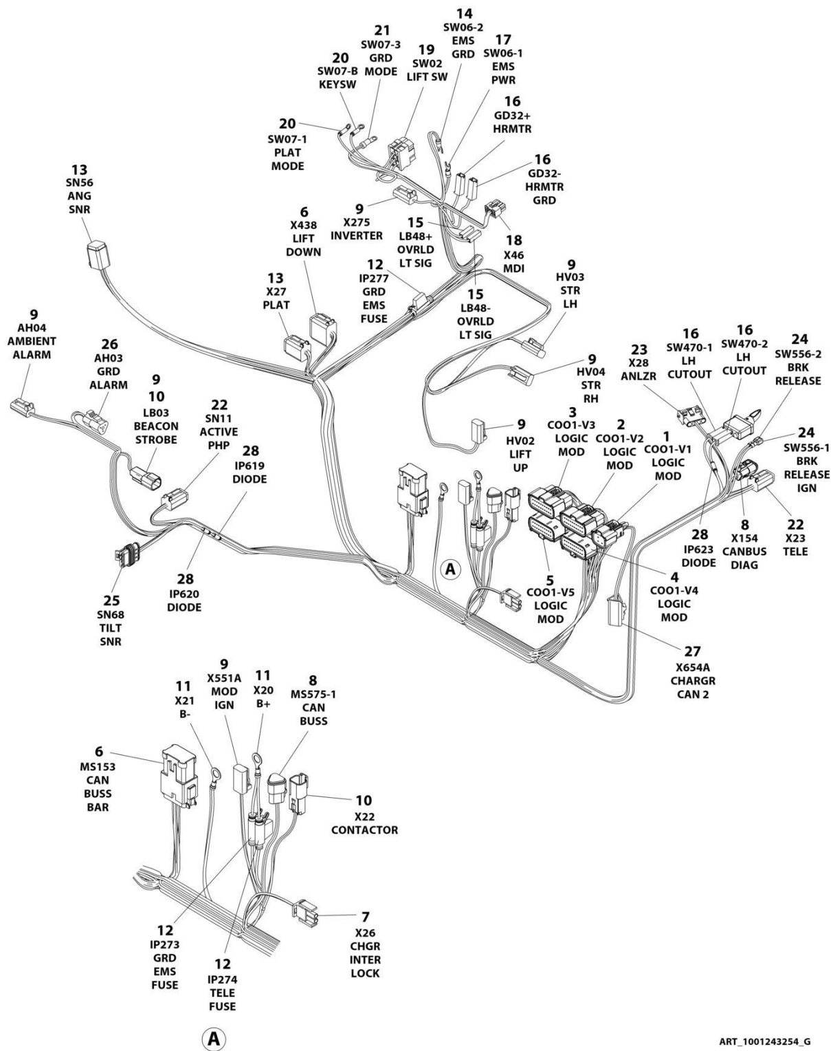
FIGURE 7-24. CHASSIS HARNESS (WITH LSS WITHOUT PLATFORM DRIVE SELECT SWITCH) (CHINA BUILT MACHINES) (Prior to SN B200059250)
