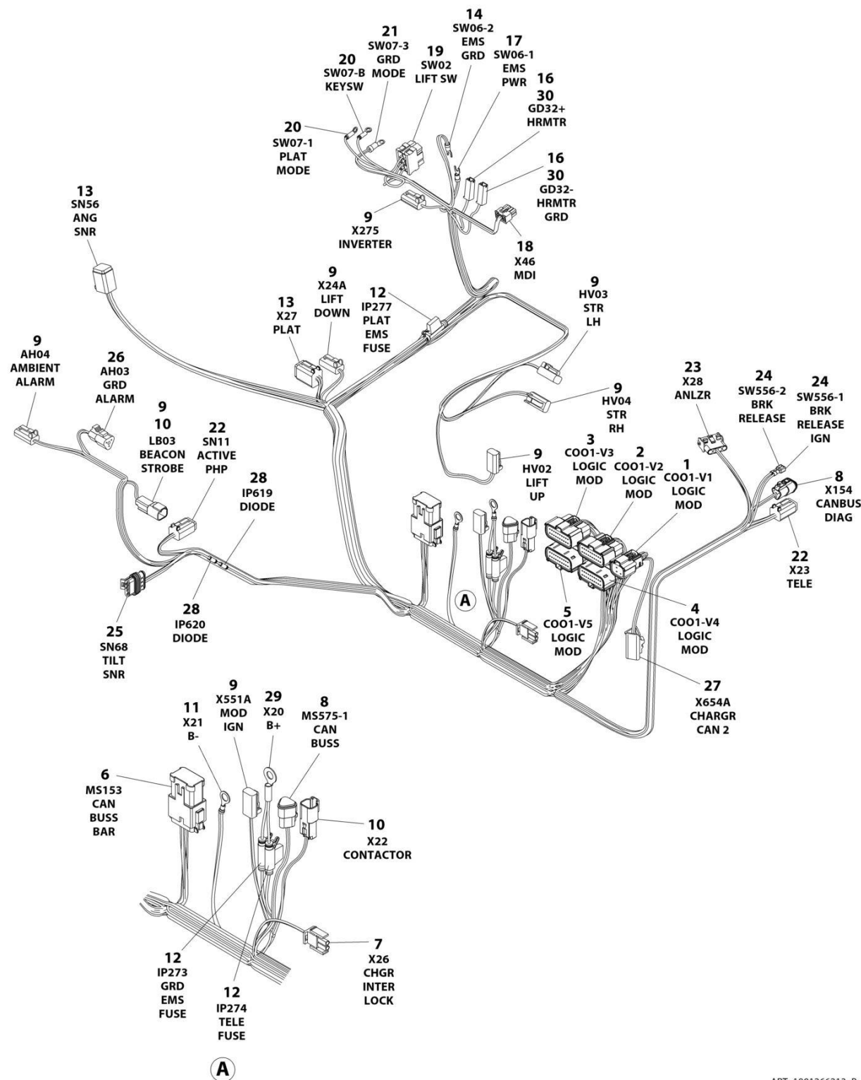
FIGURE 7-23. CHASSIS HARNESS (WITHOUT LSS WITH PLATFORM DRIVE SELECT SWITCH) (CHINA & MEXICO BUILT MACHINES) (SN B200059250 to Present)
