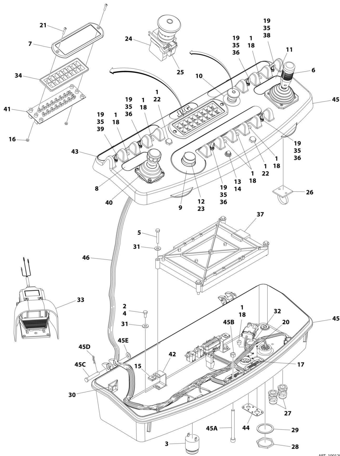
FIGURE 5-16. CONSOLE BOX ASSEMBLY (SN 0300259635 through 0300272447)
