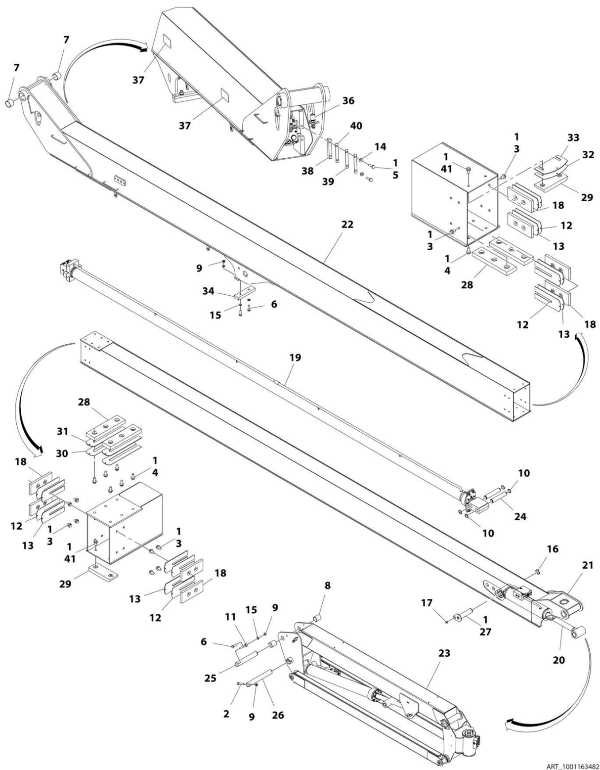
FIGURE 4-6. MAIN BOOM ASSEMBLY - 460SJC
