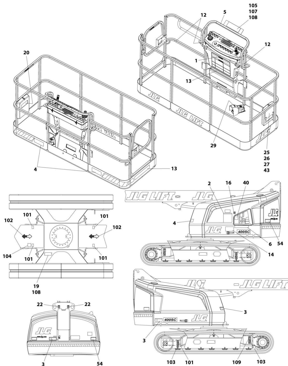
FIGURE 9-2. DECAL INSTALLATION - ANSI EXPORT - 400SC (SN 0300224020 through 0300272447)
