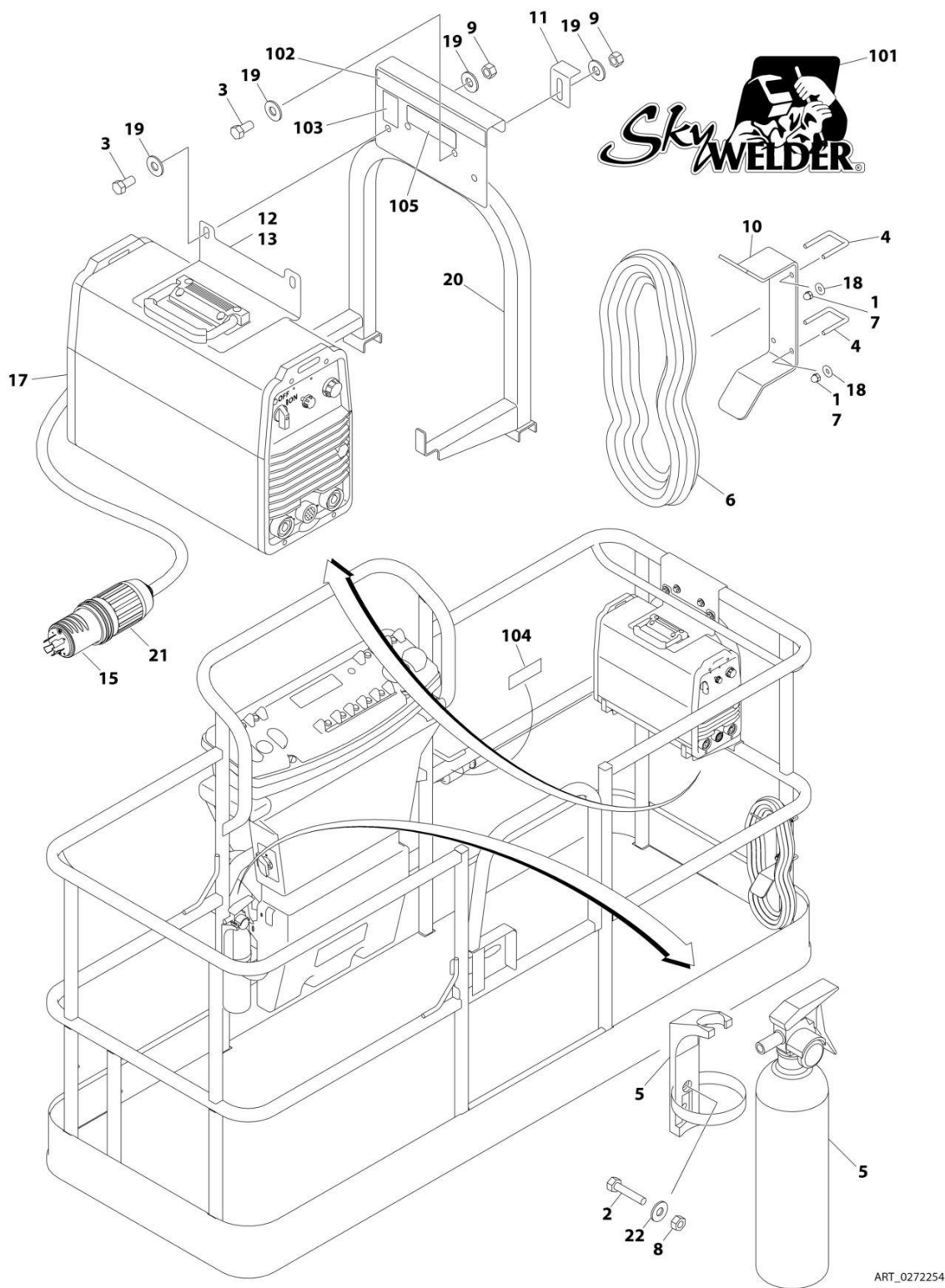
FIGURE 5-30. SKYWELDER INSTALLATION (60HZ) (ANSI EXPORT SPECS) (SN 0300224020 through 0300272447)
