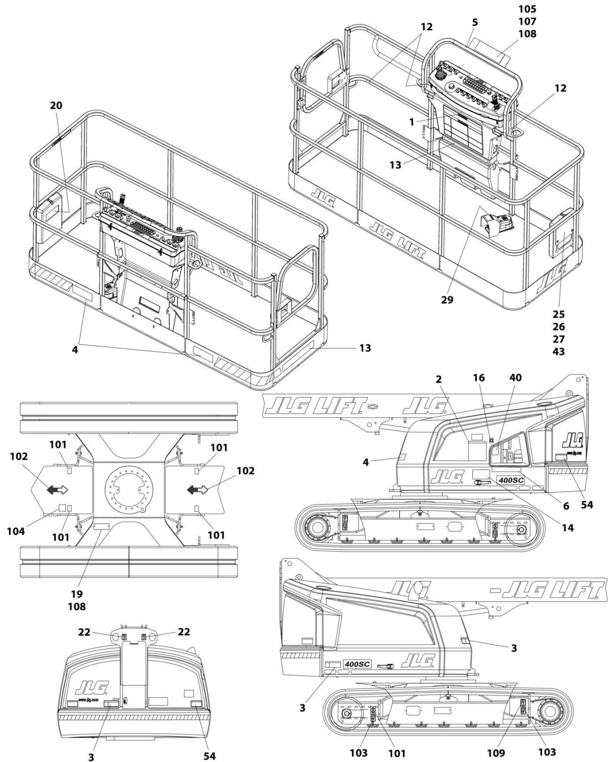
FIGURE 9-4. DECAL INSTALLATION - ANSI EXPORT - 460SJC (SN 0300224020 through 0300272447)
