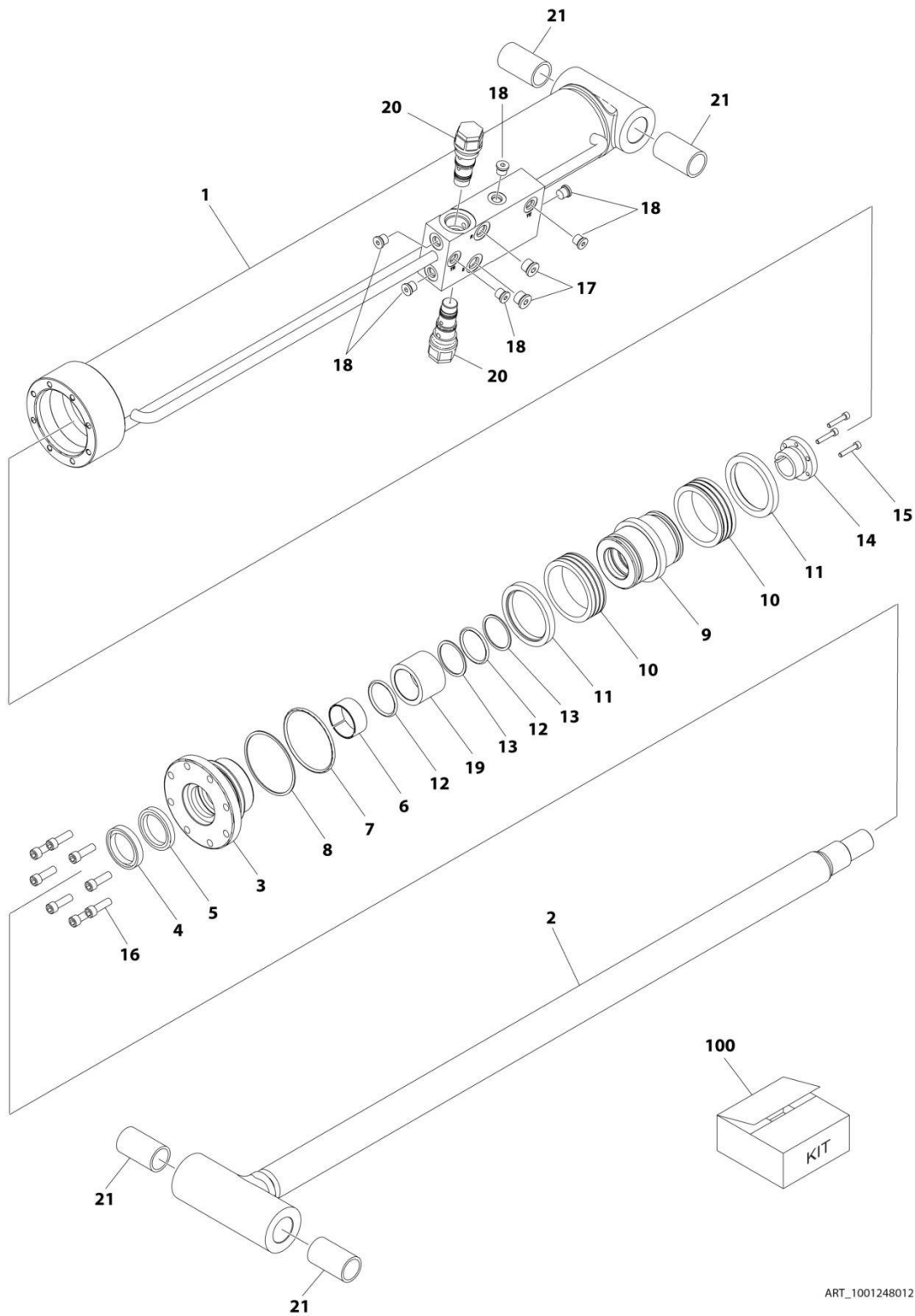
FIGURE 6-8. LIFT CYLINDER ASSEMBLY - JIB - 460SJC (USAGE MAY VARY) (SN 0300245252 through 0300272447)
