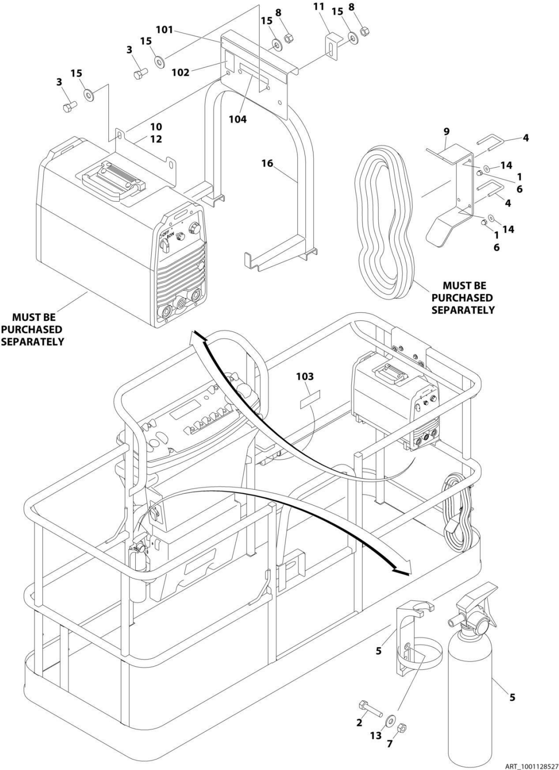
FIGURE 5-31. SKYWELDER PREP PACKAGE (60HZ) (ANSI EXPORT SPECS) (SN 0300224020 through 0300272447)
