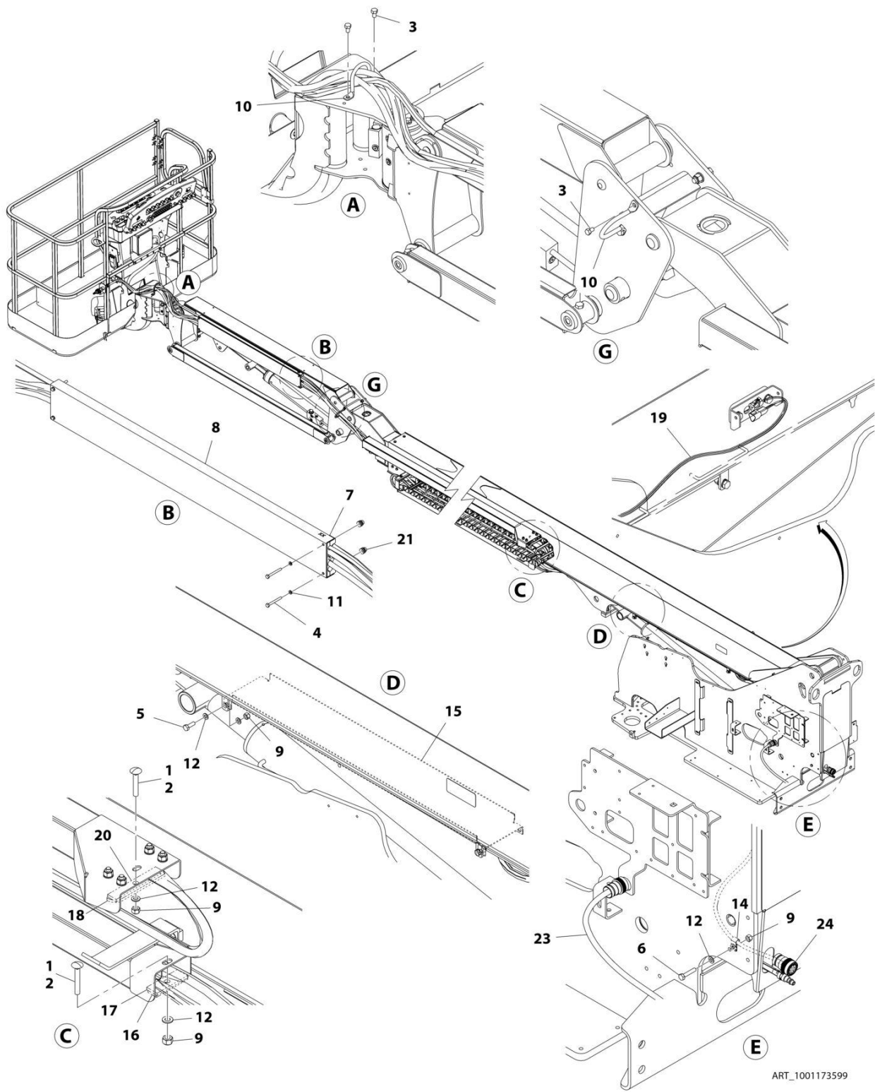
FIGURE 4-22. CABLES AND CLAMPS INSTALLATION - 460SJC - CE SPECS
