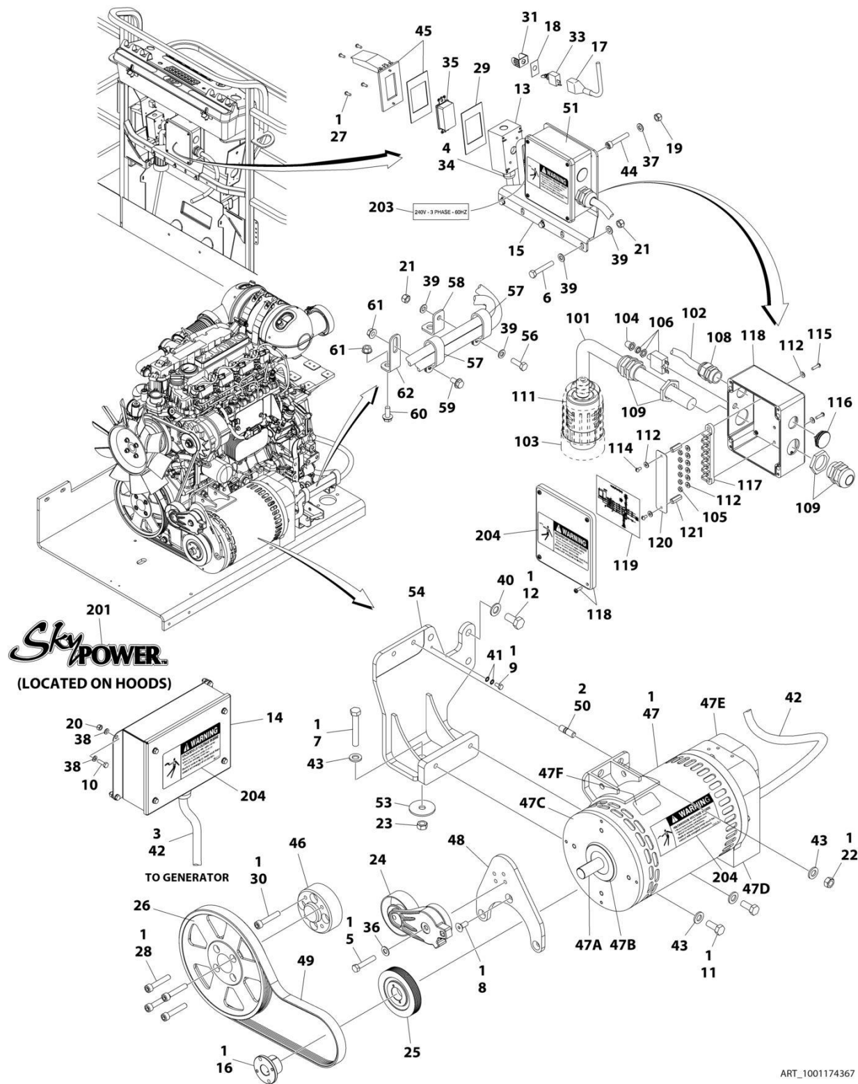
FIGURE 3-38. GENERATOR INSTALLATION - 7500W/60HZ (DEUTZ D2.9L4) (ANSI, ANSI EXPORT AND CSA SPECS) (SN 0300224020 through 0300272447)
