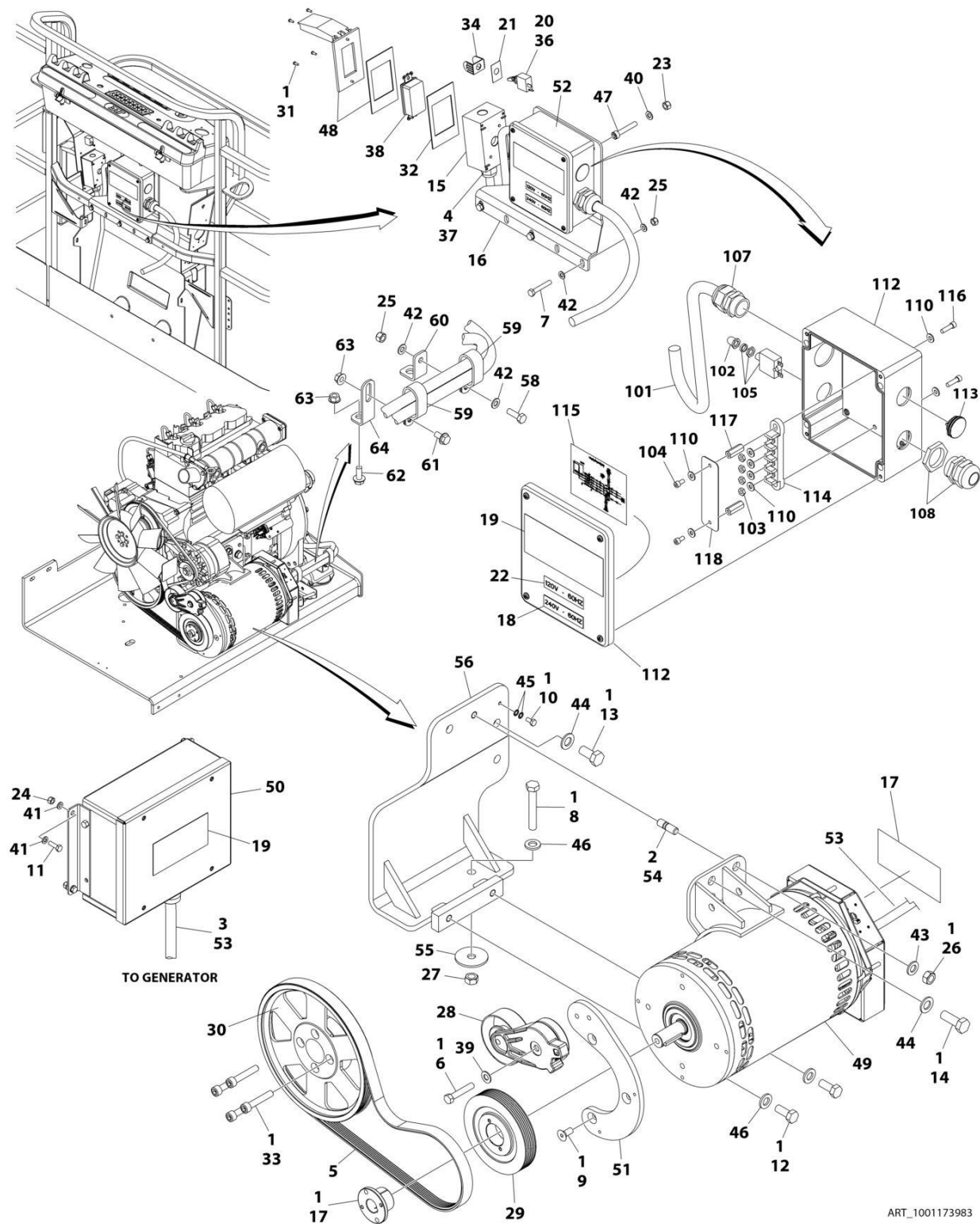
FIGURE 3-32. GENERATOR INSTALLATION - 4000W/60HZ (DEUTZ D2.3L3 ENGINE) (ANSI EXPORT SEPC) (SN 0300234013 through 0300272447)
