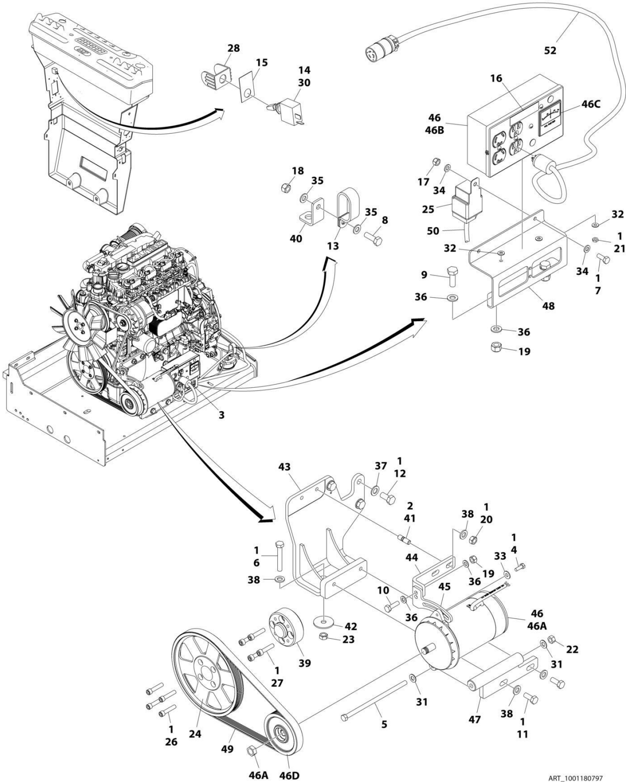
FIGURE 3-33. GENERATOR INSTALLATION - 2500W/60HZ (DEUTZ D2.9L4 ENGINE) (ANSI, ANSI EXPORT AND CSA SPECS) (SN 0300224020 through 0300272447)
