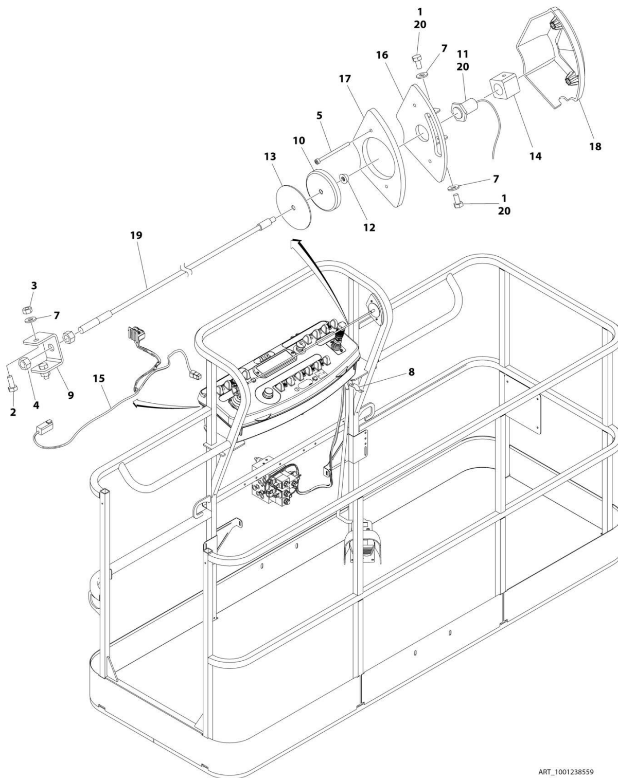
FIGURE 5-34. SKYLINE INSTALLATION
