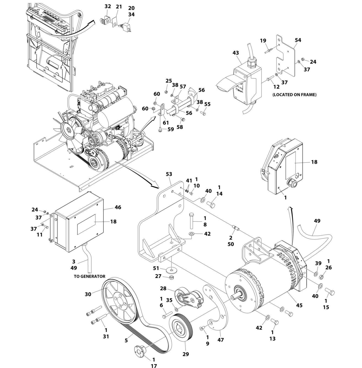
FIGURE 3-34. GENERATOR INSTALLATION - 4000W/50HZ (DEUTZ D2.3L3 ENGINE) (ANSI EXPORT AND CE SPECS) (SN 0300000100 through 0300237337)
