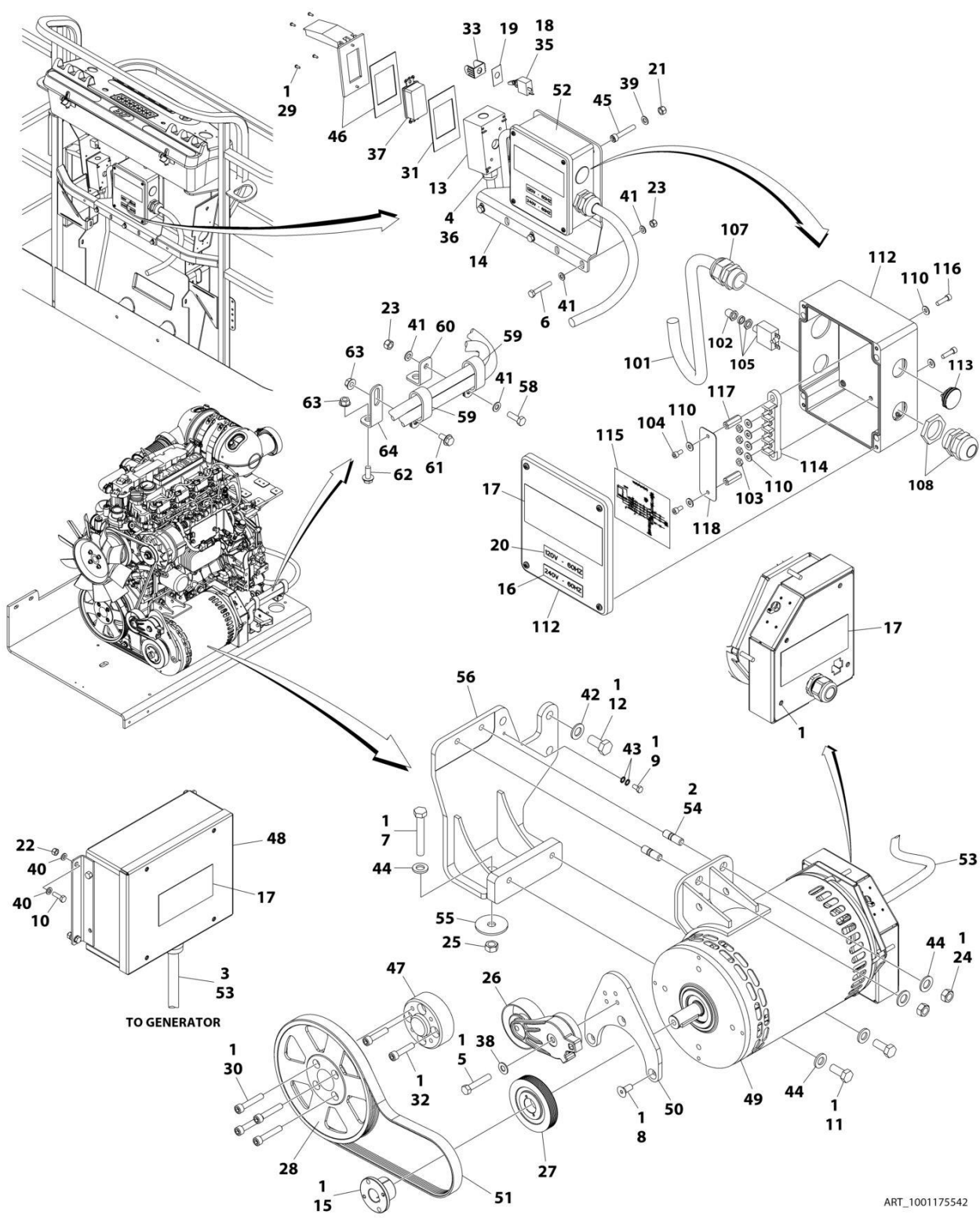
FIGURE 3-36. GENERATOR INSTALLATION - 4000W/60HZ (DEUTZ D2.9L4 ENGINE) (ANSI, ANSI EXPORT AND CSA SPECS) (SN 0300224020 through 0300272447)
