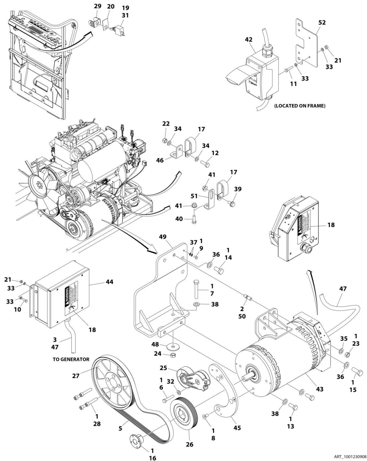
FIGURE 3-35. GENERATOR INSTALLATION - 4000W/50HZ (DEUTZ D2.3L3 ENGINE) (ANSI EXPORT AND CE SPECS) (SN 0300237337 through 0300272447)
