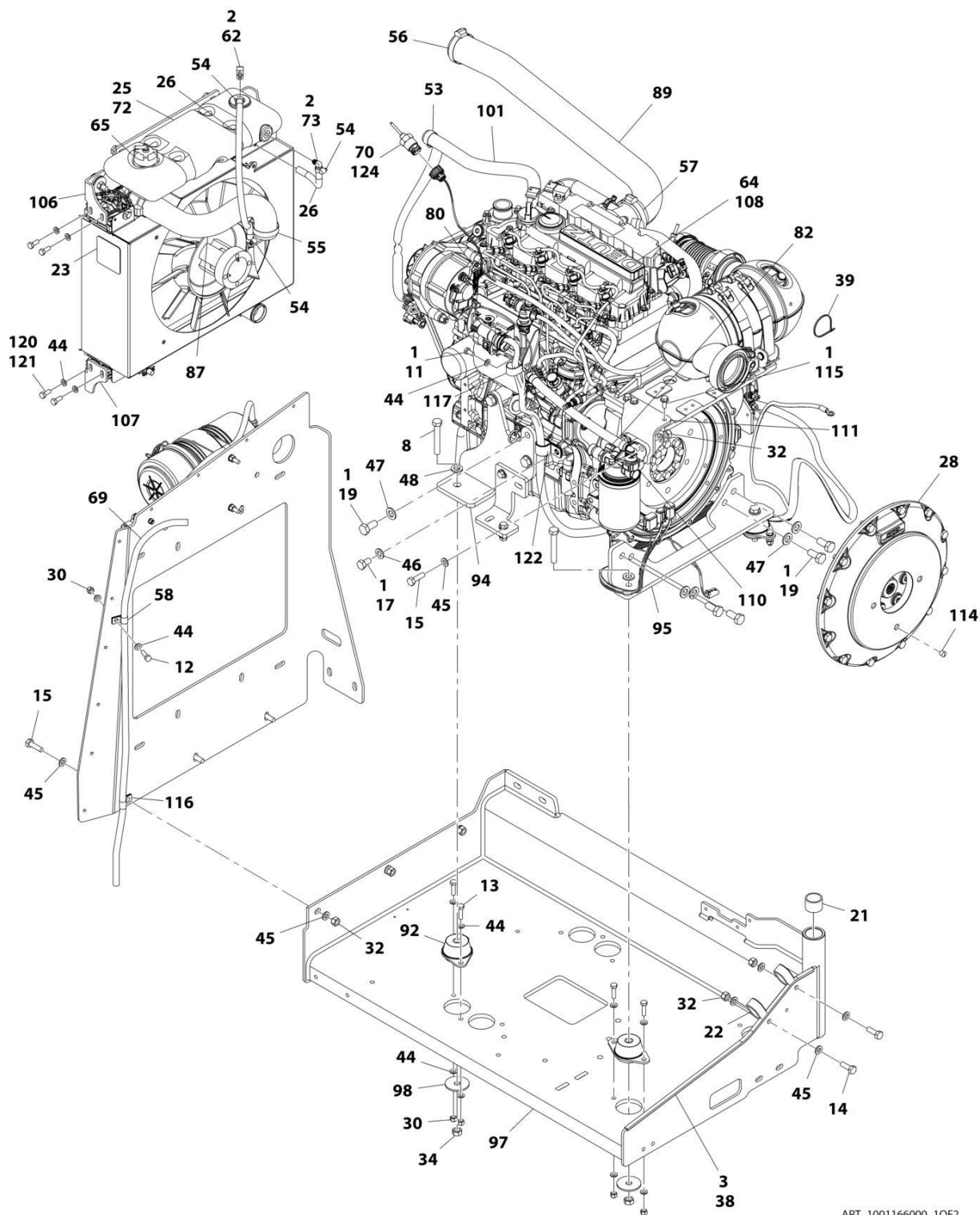
FIGURE 3-13. ENGINE ASSEMBLY - (DEUTZ D2.9L) (T4F) (ANSI, CSA AND ANSI EXPORT SPECS) (SN 0300224020 through 0300272447)
