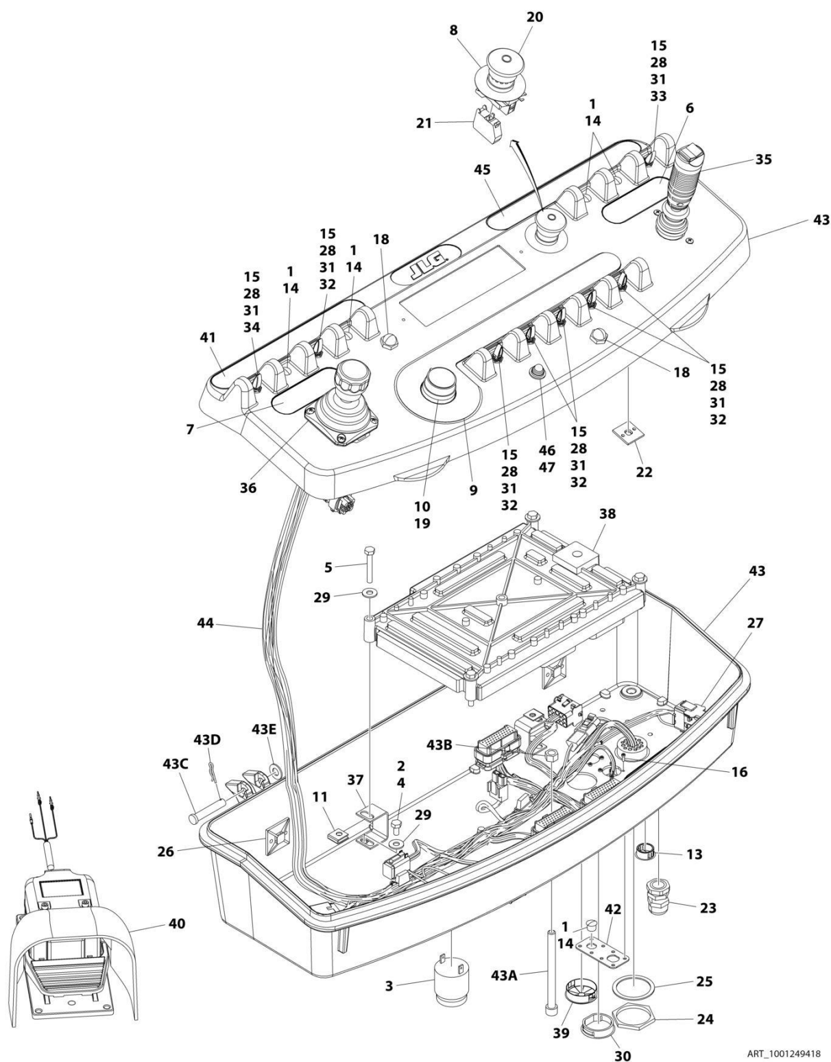
FIGURE 4-9. CONSOLE BOX ASSEMBLY - E300AJP
