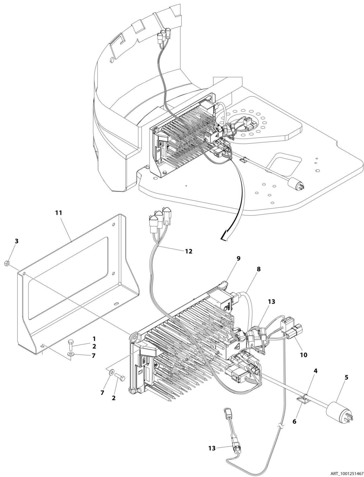
FIGURE 2-23. BATTERY CHARGER INSTALLATION - WITH PLUG (ALL SPECS EXCEPT CE SPECS)
