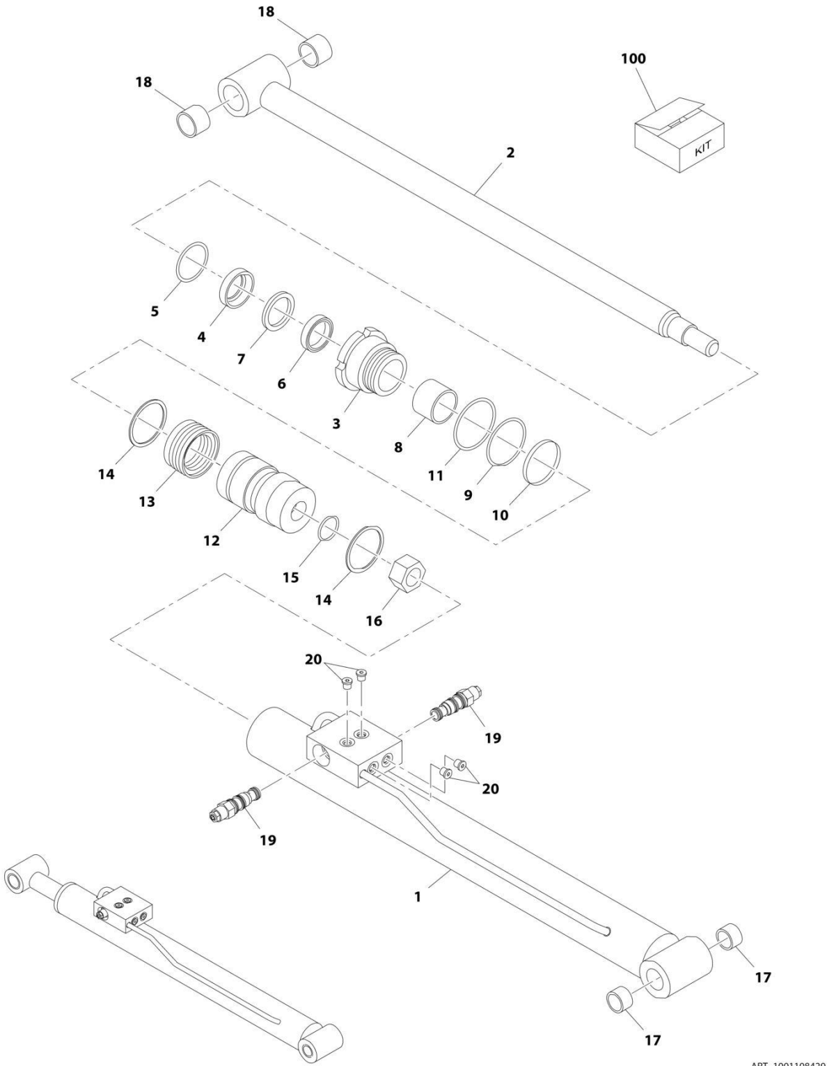
FIGURE 5-2. LIFT CYLINDER ASSEMBLY - JIB
