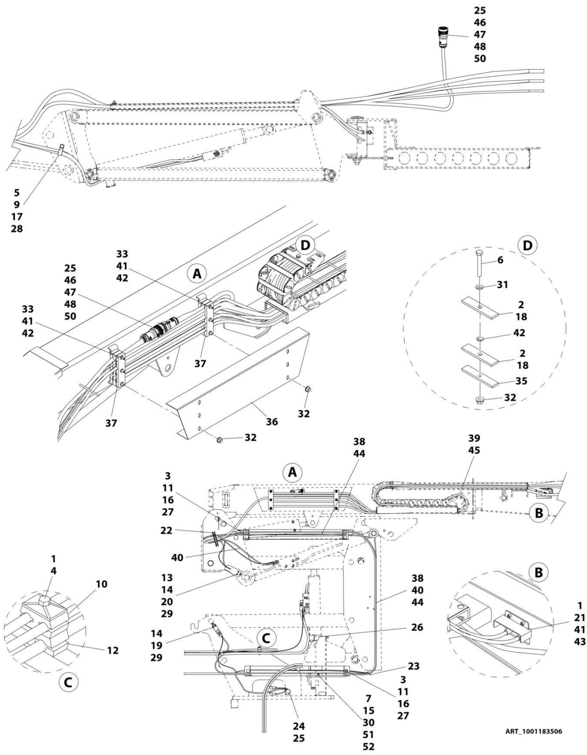
FIGURE 7-14. BOOM CABLES AND CLAMPS INSTALLATION - E300AJ
