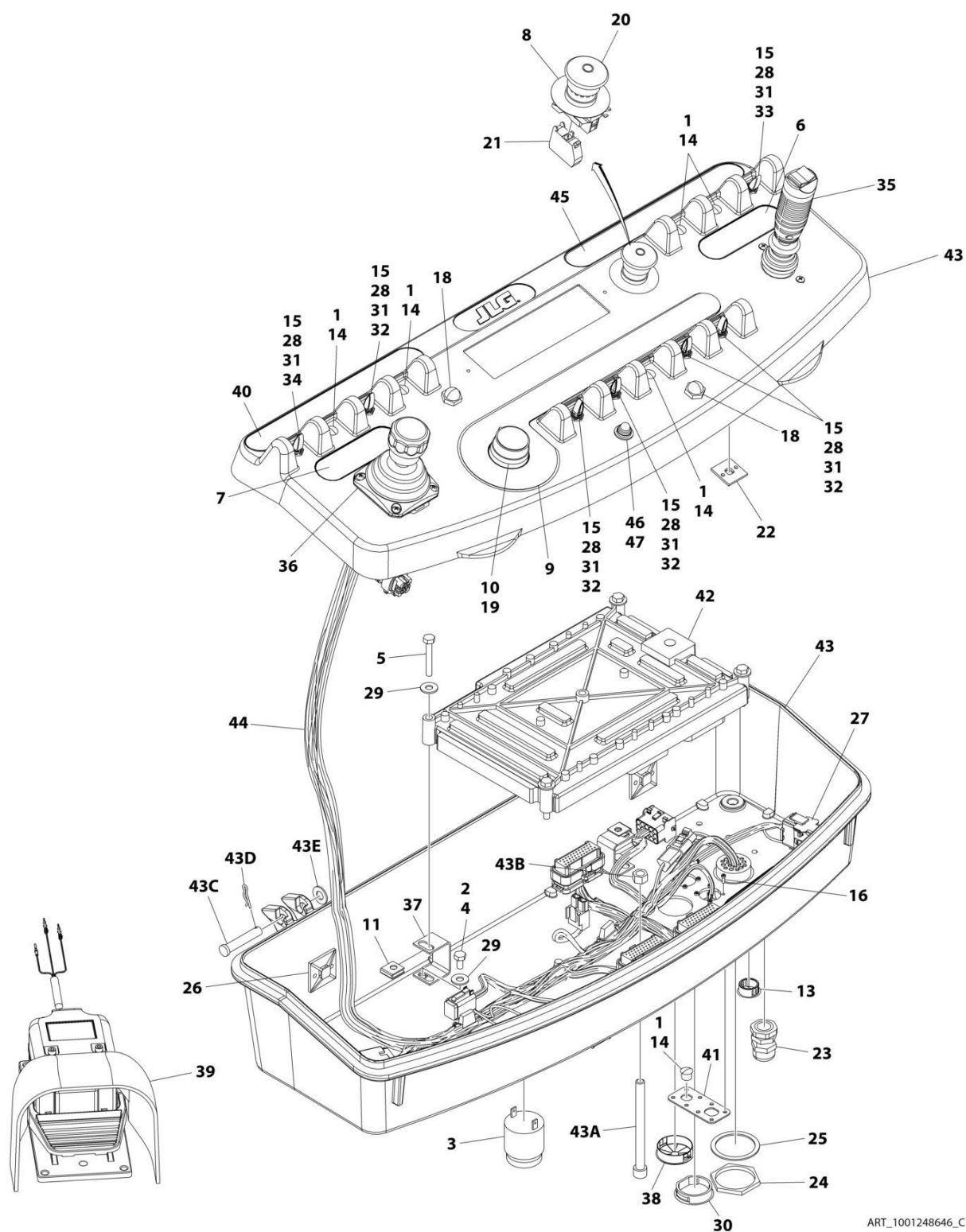
FIGURE 4-8. CONSOLE BOX ASSEMBLY - E300AJ WITH UL SPECS
