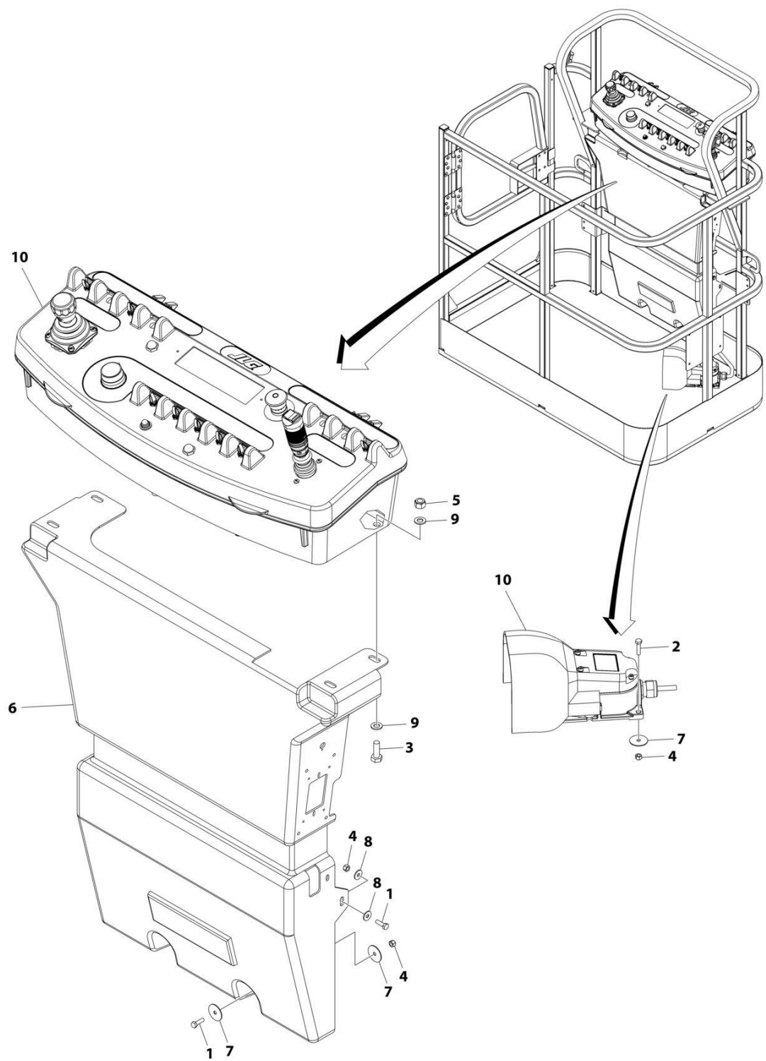
FIGURE 4-6. PLATFORM CONSOLE AND FOOTSWITCH INSTALLATION - E300AJP WITH UL SPECS
