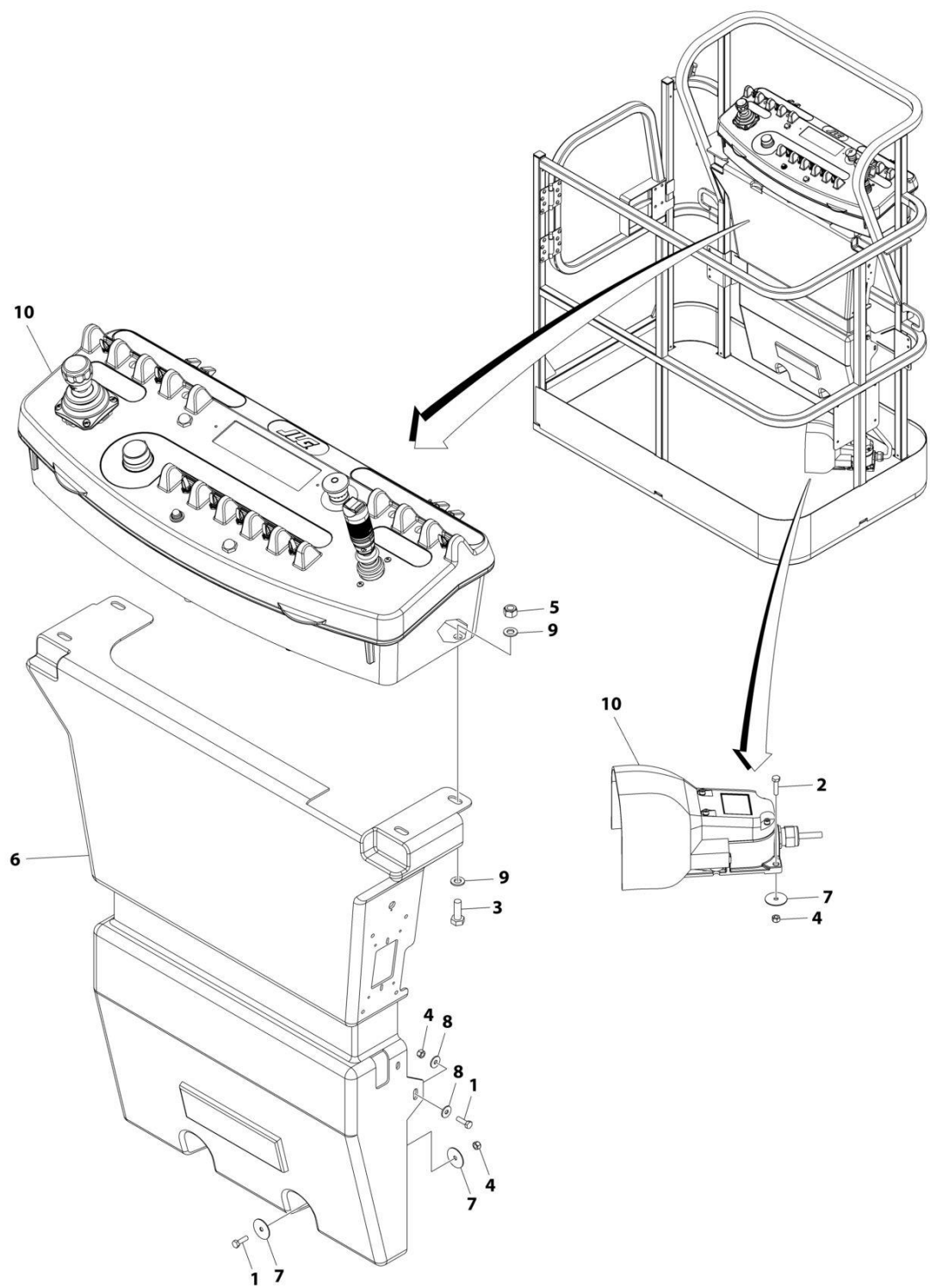
FIGURE 4-5. PLATFORM CONSOLE AND FOOTSWITCH INSTALLATION - E300AJP
