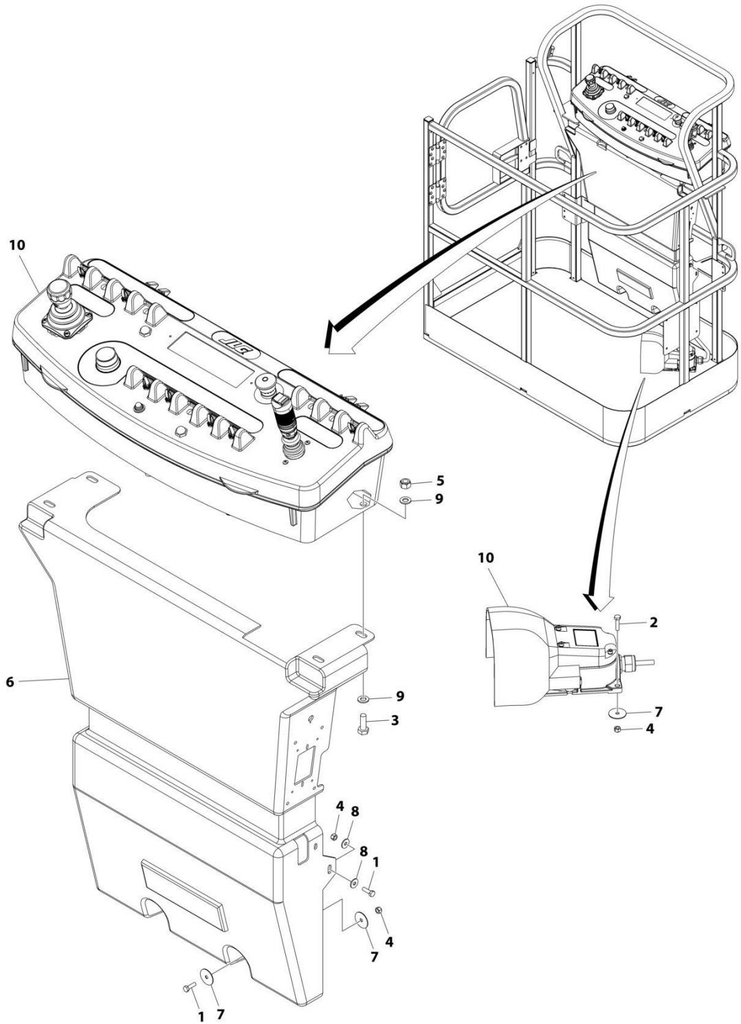
FIGURE 4-3. PLATFORM CONSOLE AND FOOTSWITCH INSTALLATION - E300AJ
