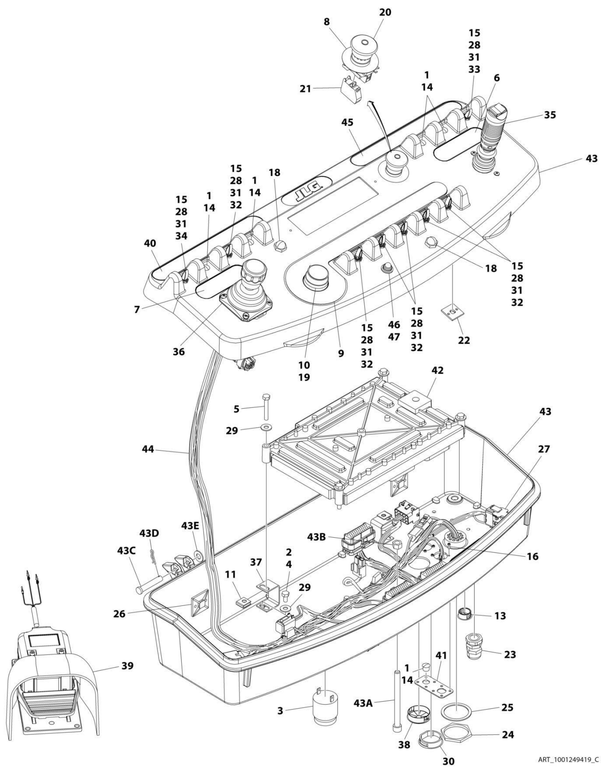
FIGURE 4-10. CONSOLE BOX ASSEMBLY - E300AJP WITH UL SPECS
