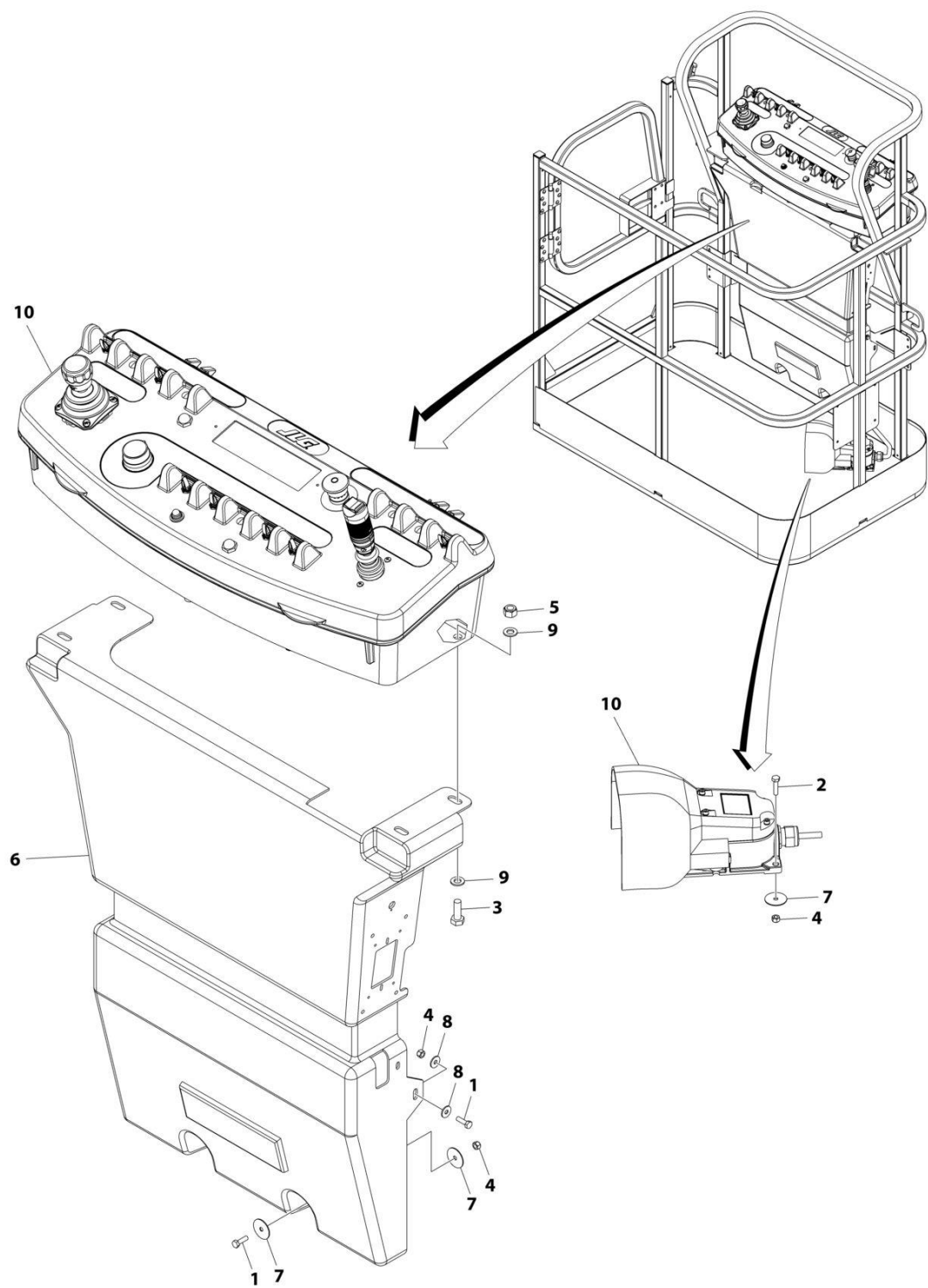
FIGURE 4-4. PLATFORM CONSOLE AND FOOTSWITCH INSTALLATION - E300AJ WITH UL SPECS
