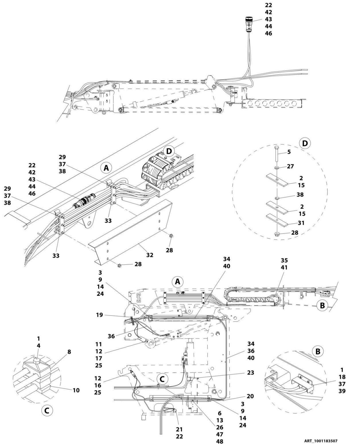
FIGURE 7-15. BOOM CABLES AND CLAMPS INSTALLATION - E300AJP
