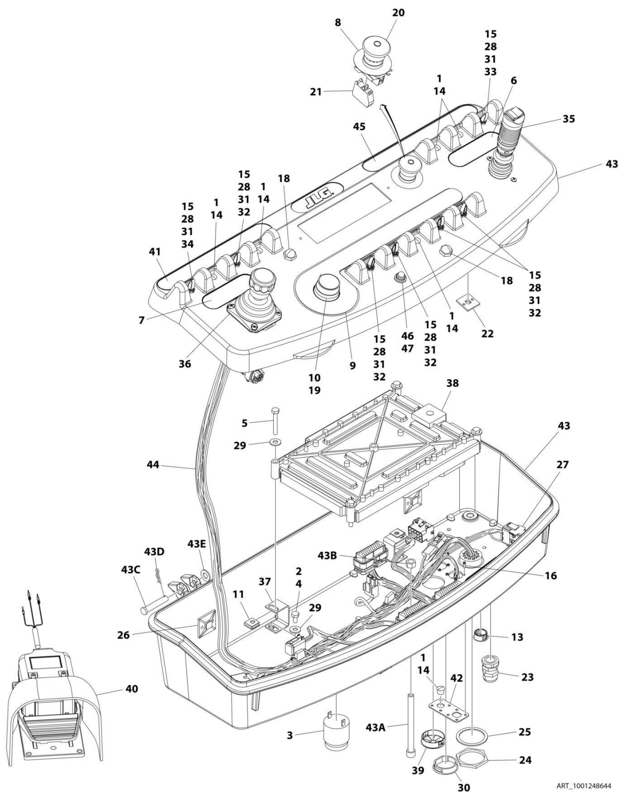
FIGURE 4-7. CONSOLE BOX ASSEMBLY - E300AJ
