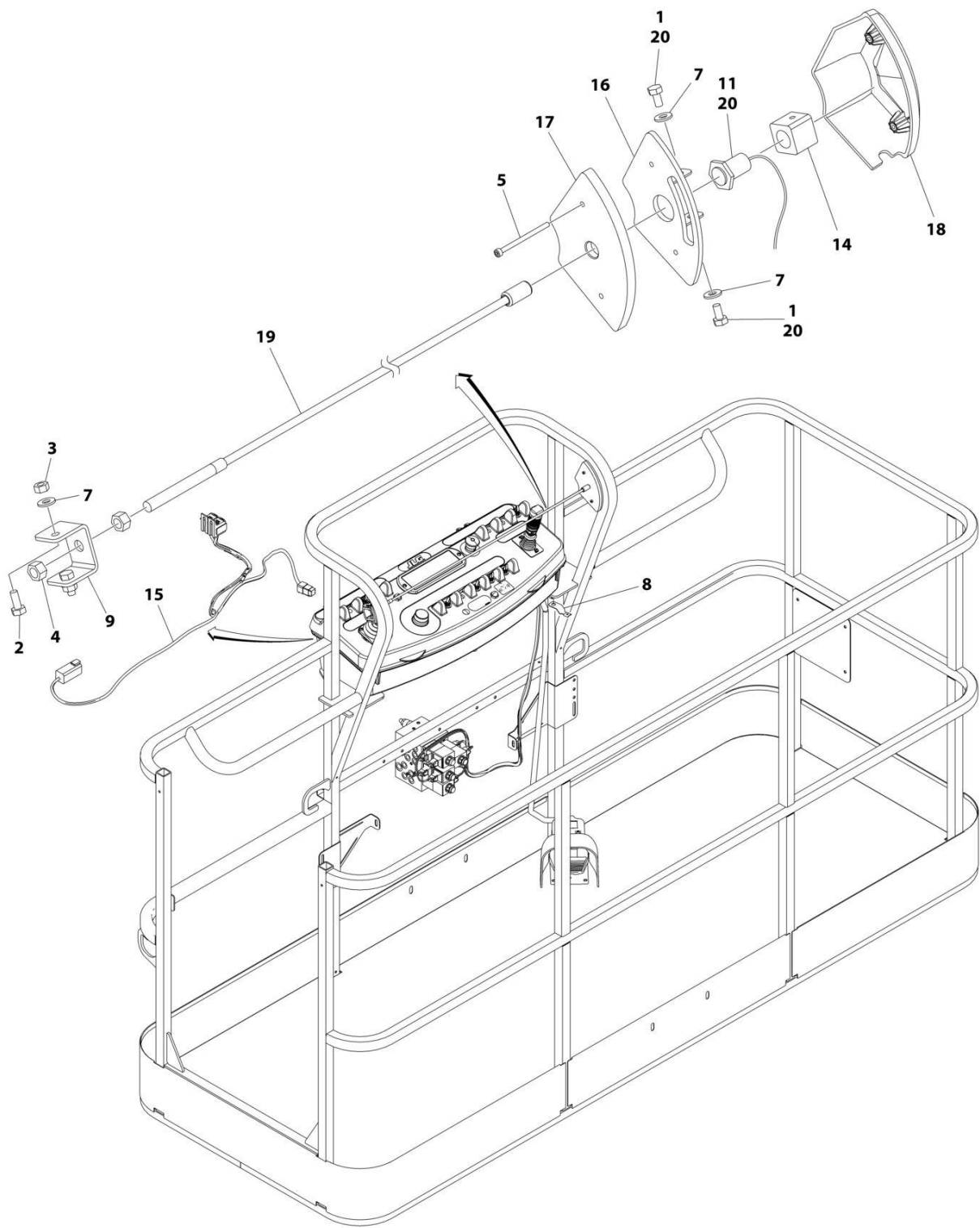
FIGURE 5-15. SKYLINE INSTALLATION
