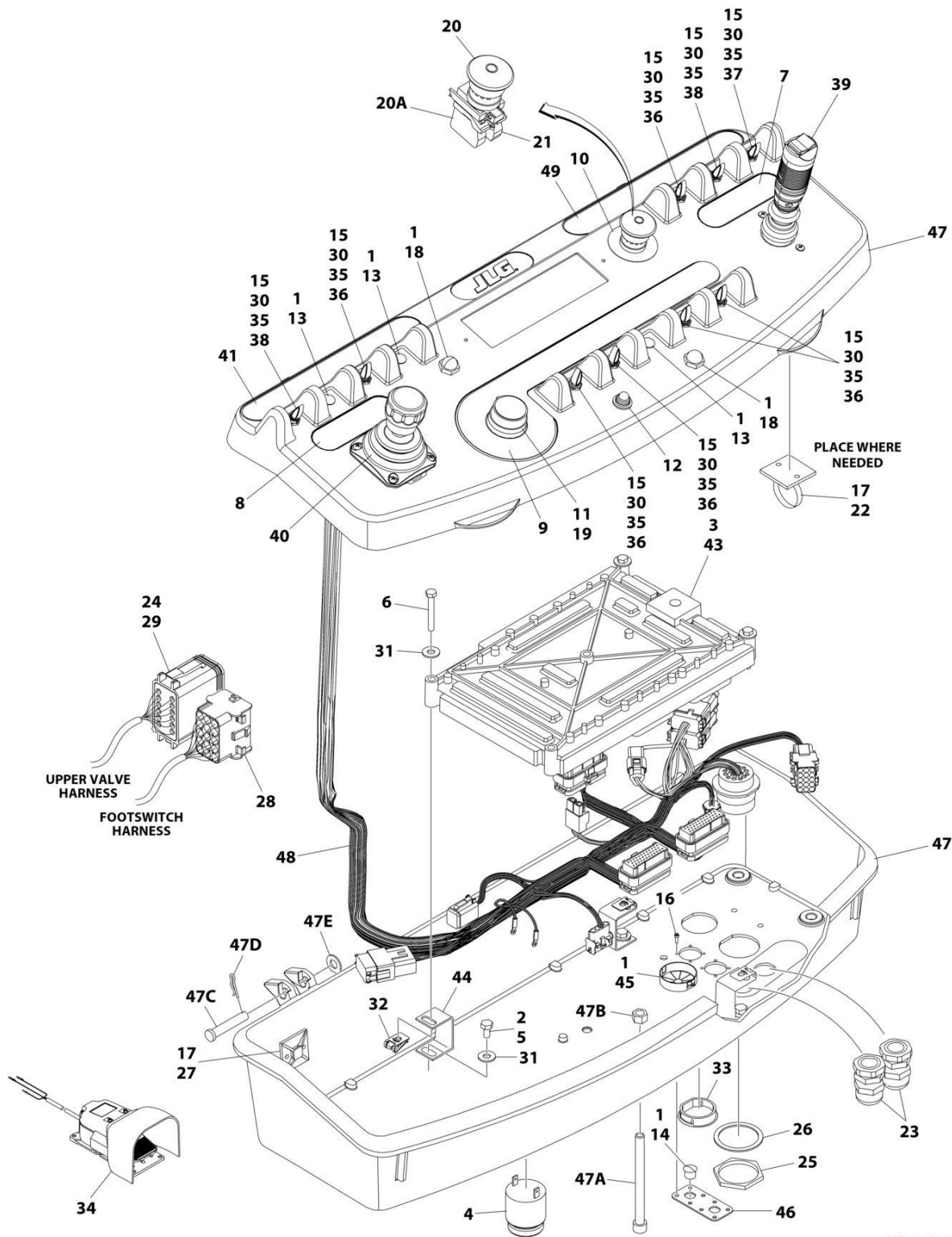
FIGURE 5-8. CONSOLE AND FOOTSWITCH ASSEMBLY
