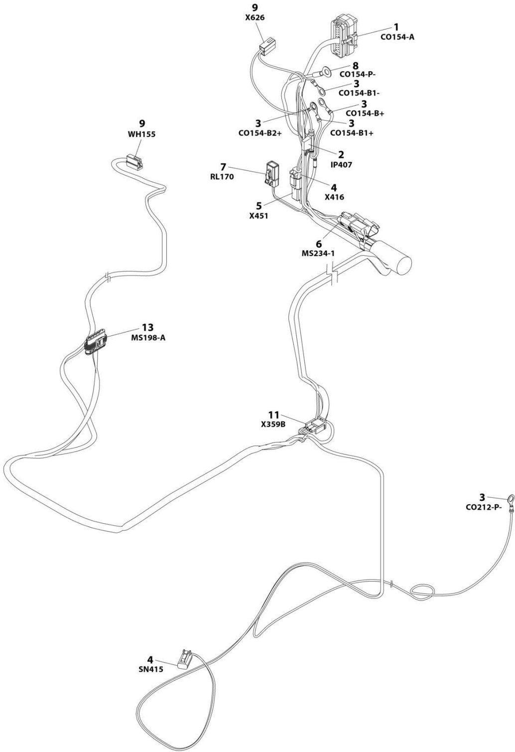
FIGURE 8-29. GENERATOR HARNESS
