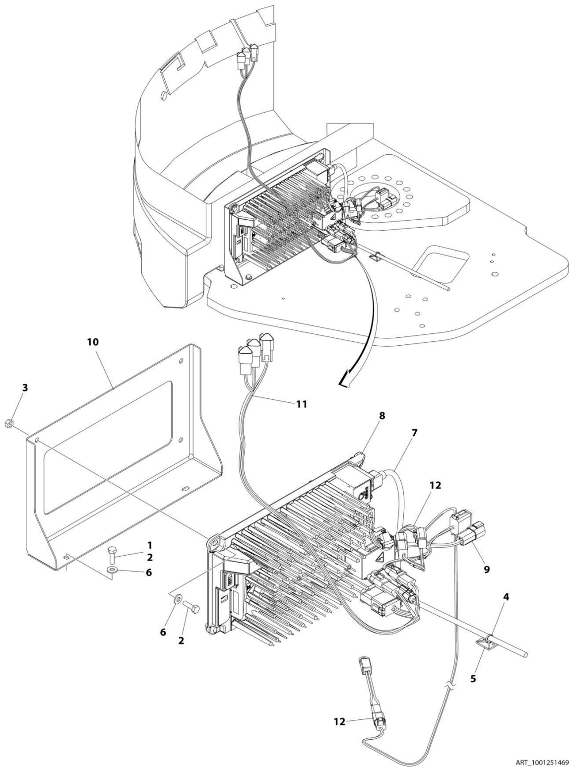
FIGURE 2-19. BATTERY CHARGER INSTALLATION - WITHOUT PLUG
