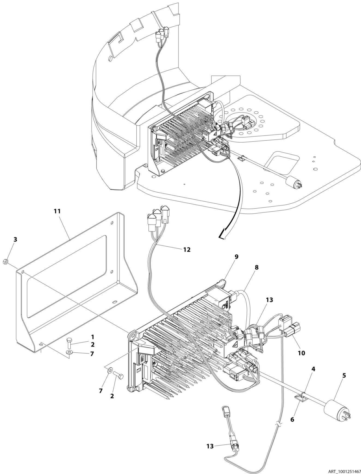
FIGURE 2-17. BATTERY CHARGER INSTALLATION - WITH PLUG (ALL SPECS EXCEPT CE & UK CA SPECS)
