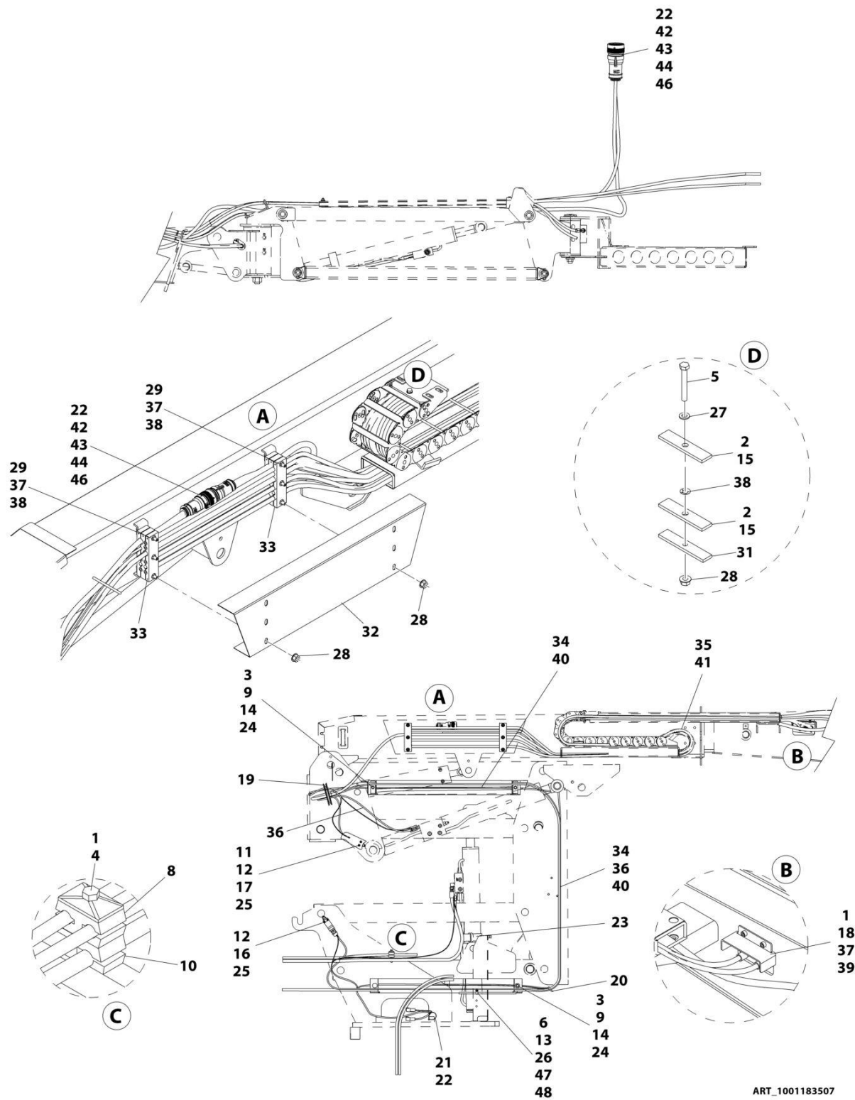
FIGURE 7-14. BOOM CABLES AND CLAMPS INSTALLATION
