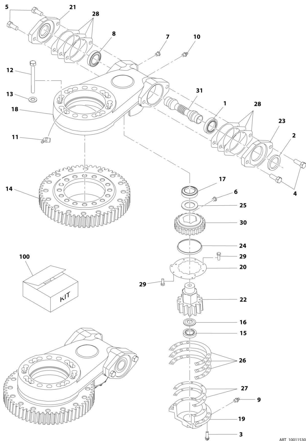
FIGURE 2-5. TURNTABLE BEARING ASSEMBLY
