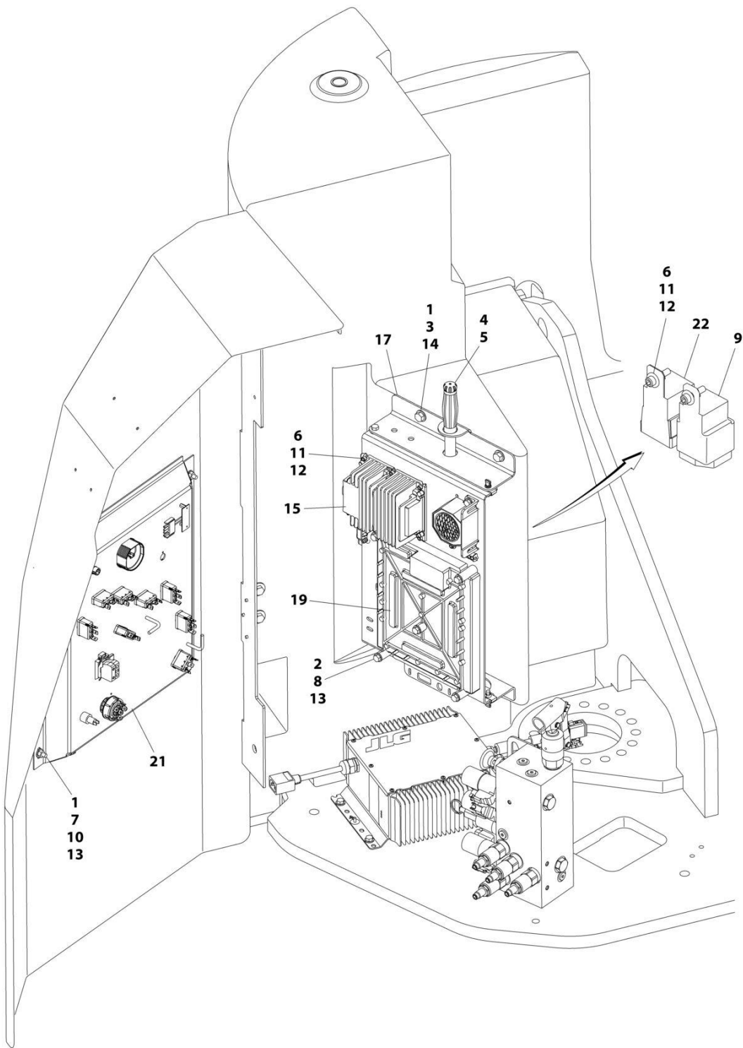
FIGURE 2-9. ELECTRICAL COMPONENTS INSTALLATION (CE & UK CA SPECS)
