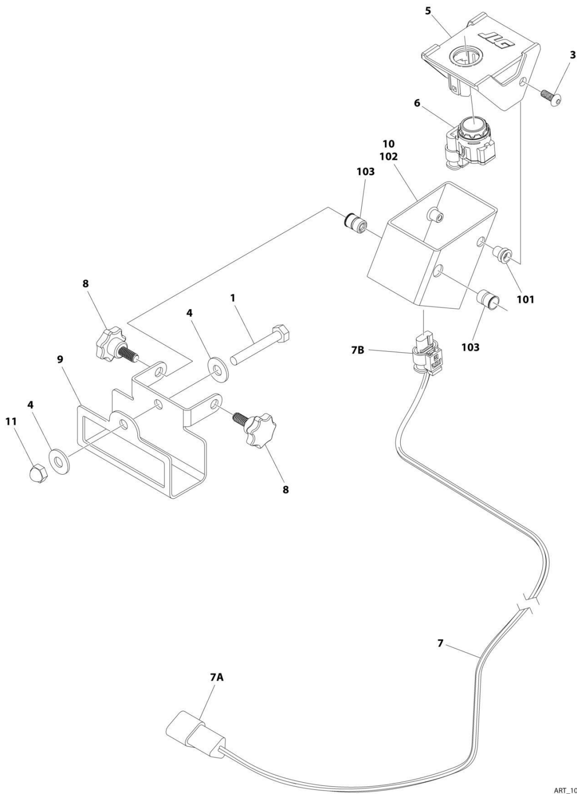
FIGURE 4-17. SKYSENSE OVERHEAD SENSOR ASSEMBLY
