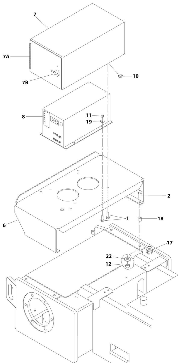
FIGURE 1-13. INVERTER INSTALLATION - OPTIONAL
