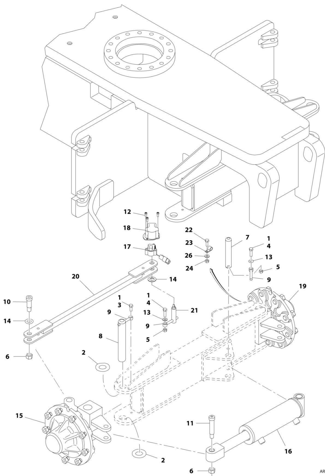
FIGURE 1-1. STEER INSTALLATION
