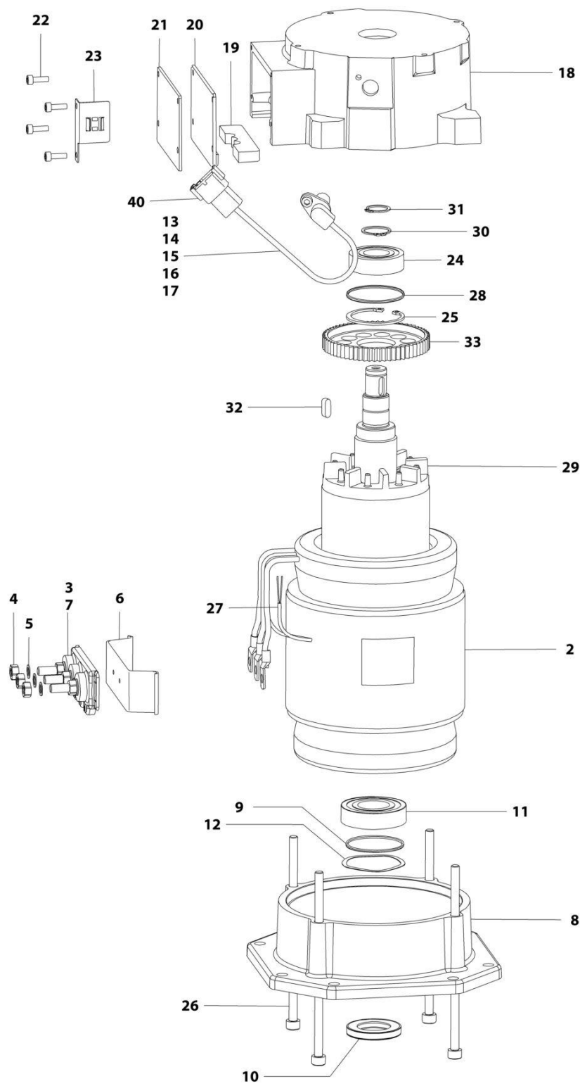
FIGURE 1-6. DRIVE MOTOR ASSEMBLY
