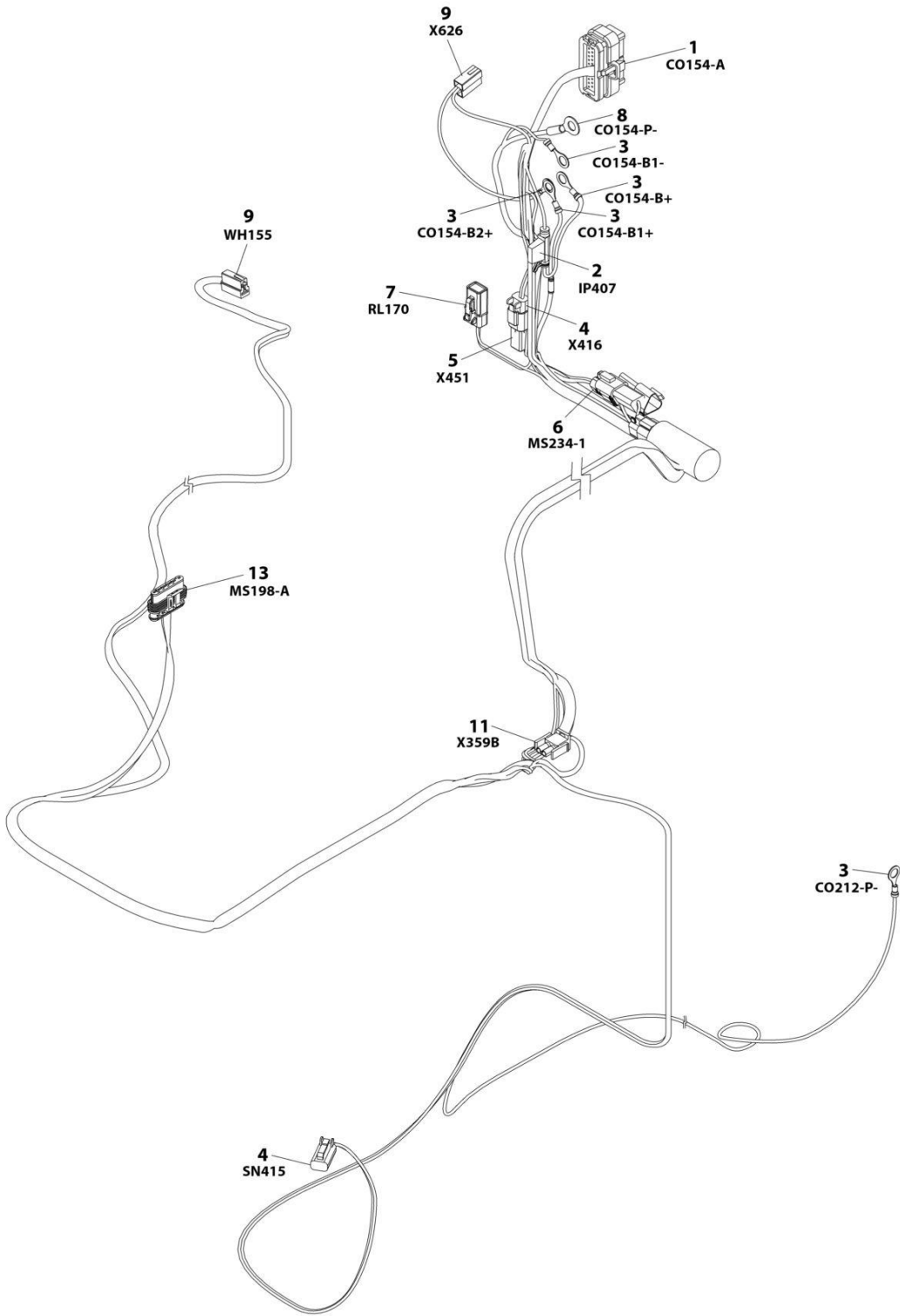
FIGURE 8-29. GENERATOR HARNESS
