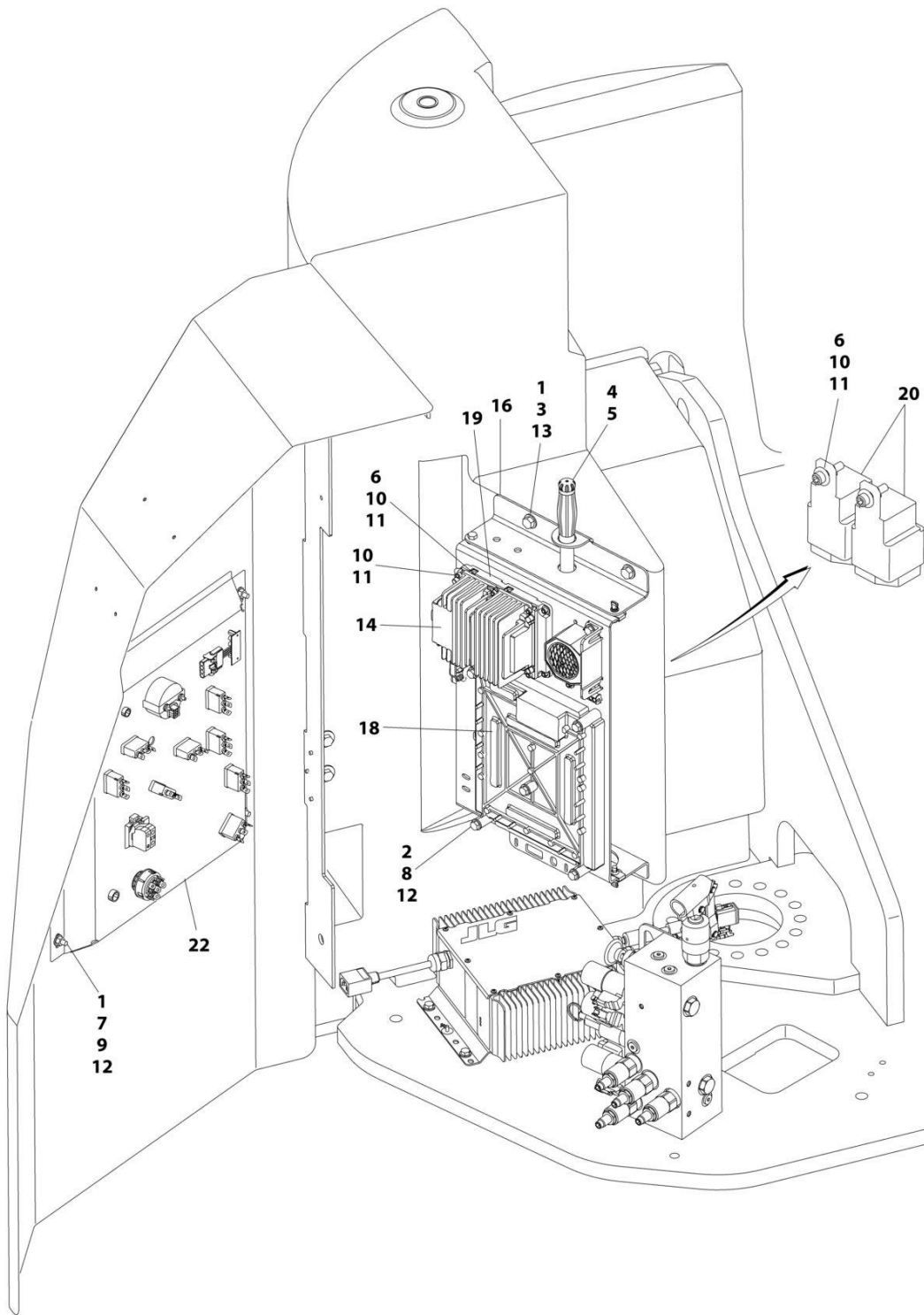
FIGURE 2-12. ELECTRICAL COMPONENTS INSTALLATION (UL SPECS) (Prior to SN 0300291030, Excluding 0300284206)
