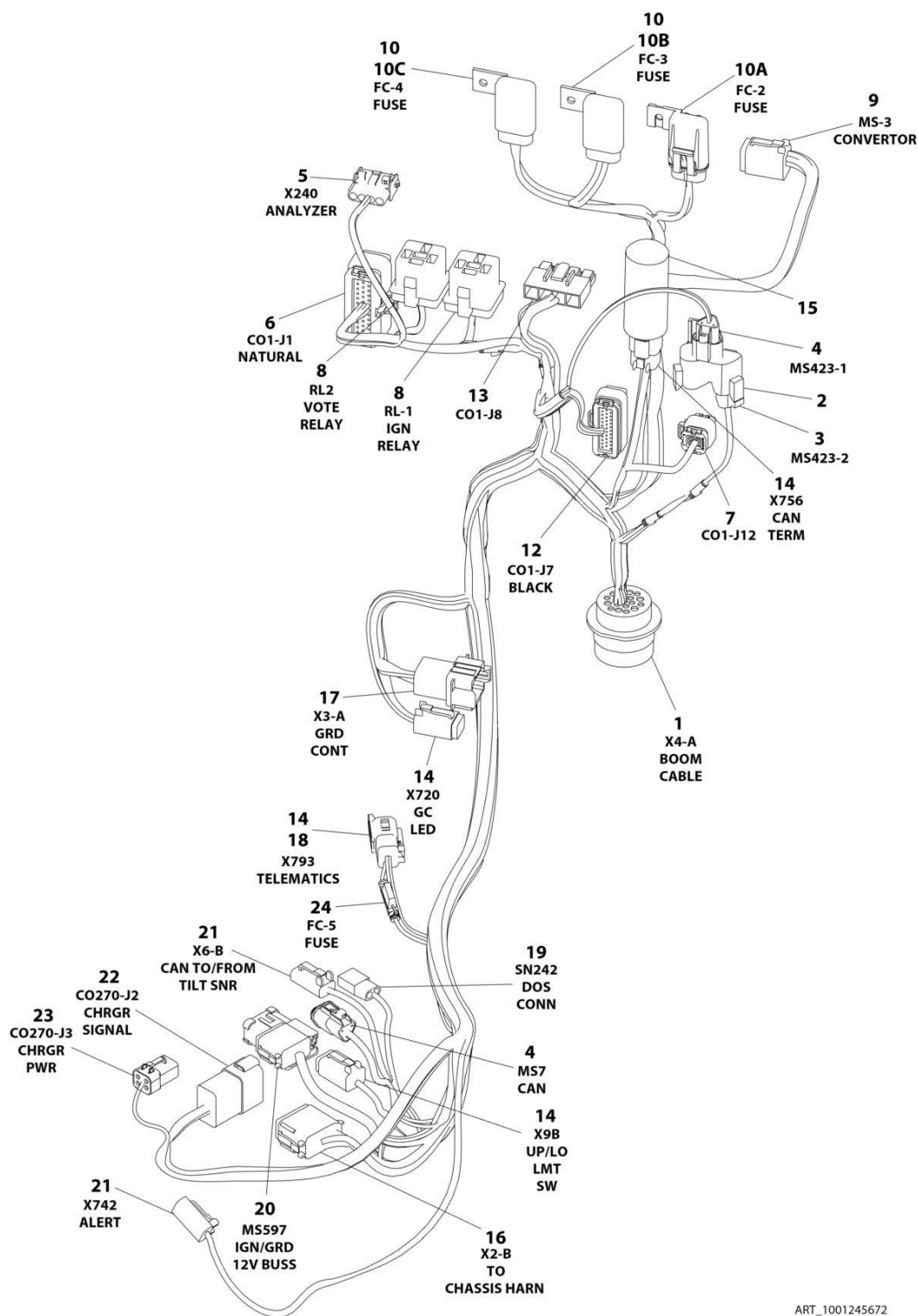
FIGURE 7-46. TURNTABLE HARNESS
