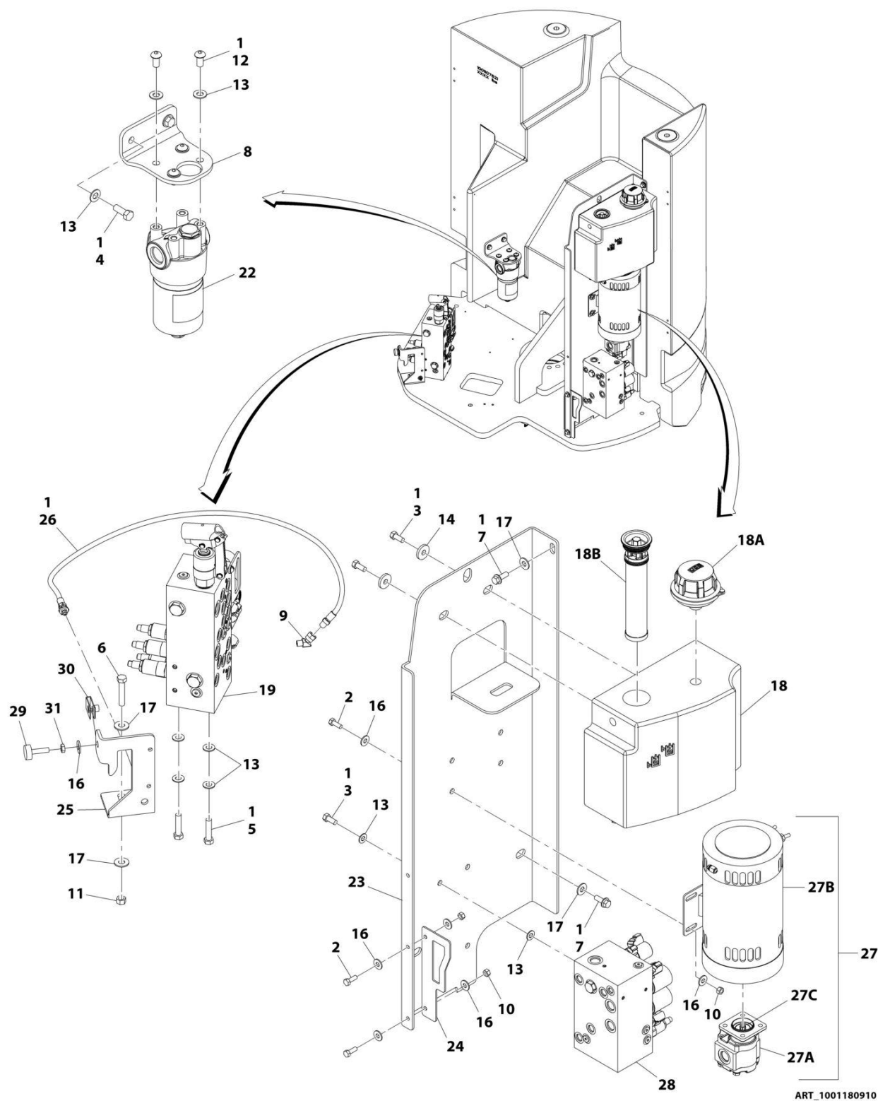
FIGURE 2-1. VALVES, TANK AND MOTOR INSTALLATION
