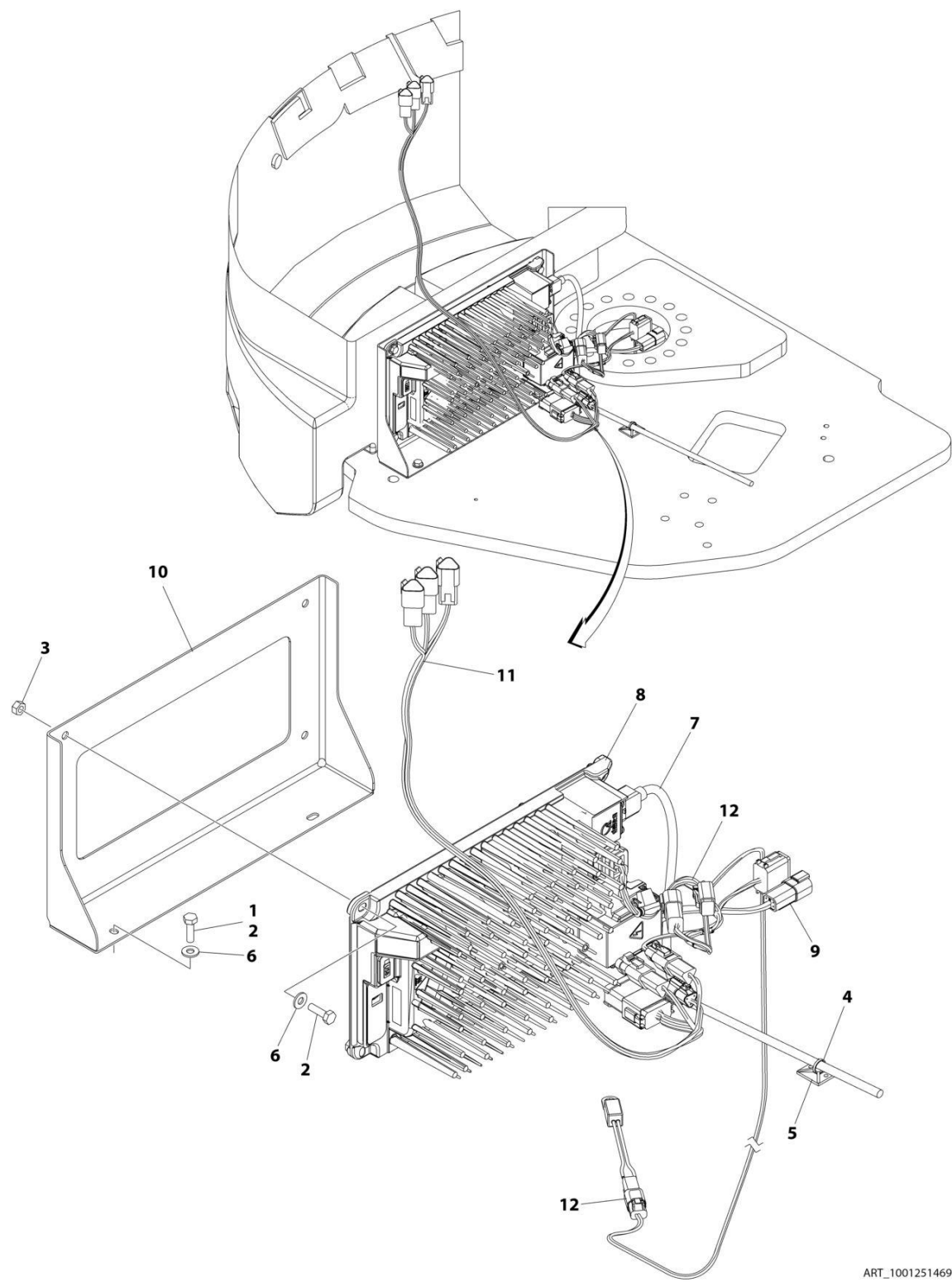
FIGURE 2-20. BATTERY CHARGER INSTALLATION - WITHOUT PLUG
