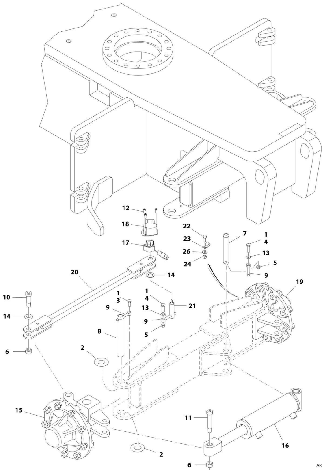
FIGURE 1-1. STEER INSTALLATION
