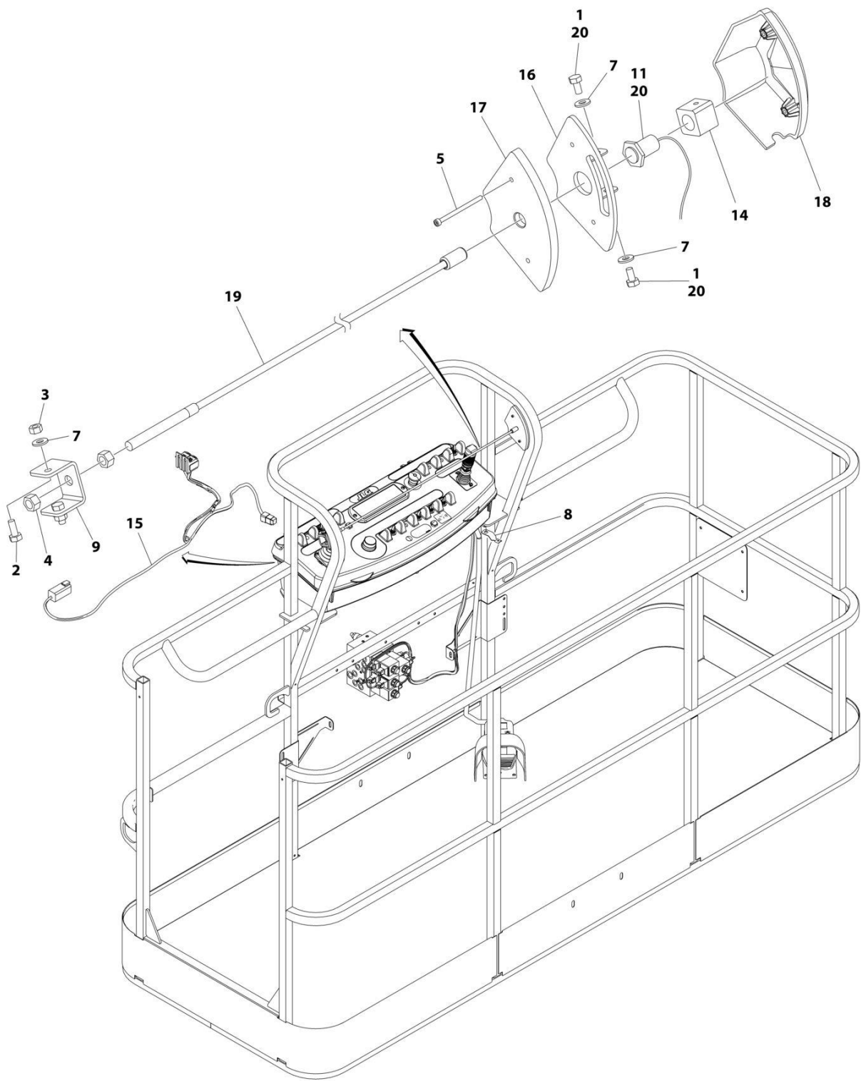
FIGURE 4-14. SKYLINE INSTALLATION
