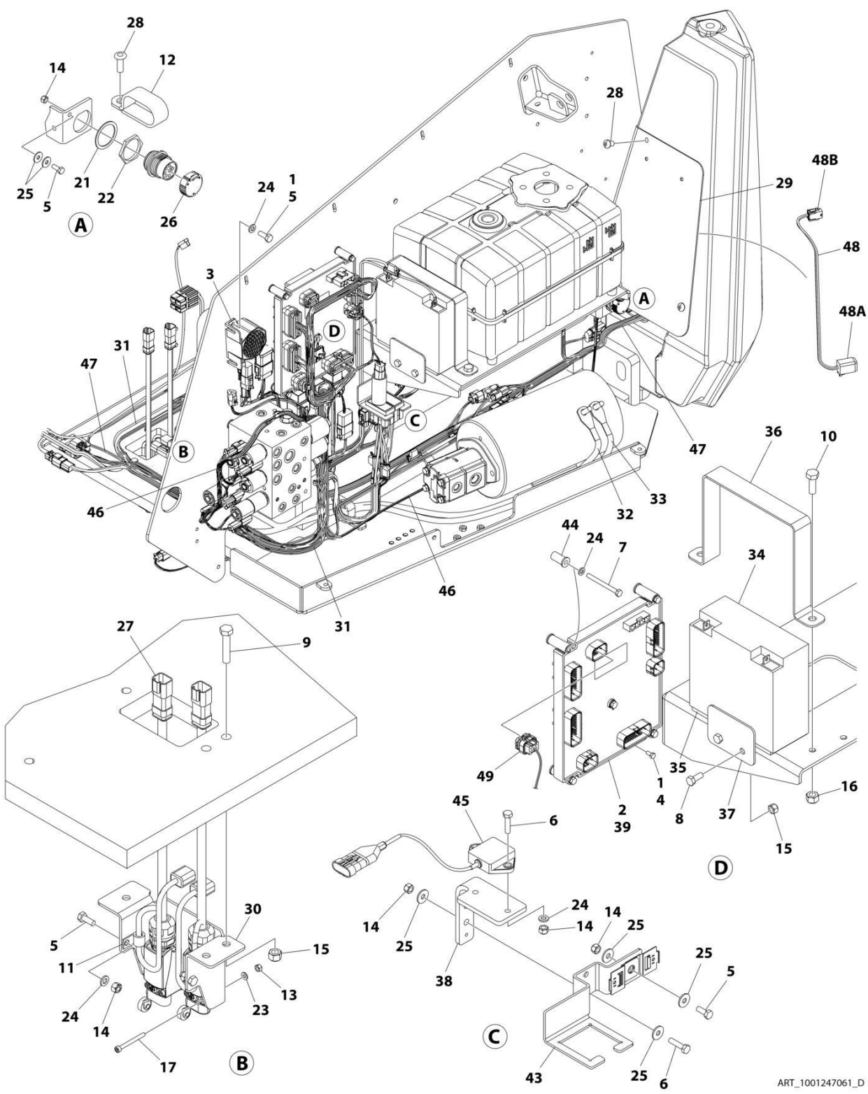
FIGURE 2-19. ELECTRICAL COMPONENTS INSTALLATION (SN 0300292053 to Present)
