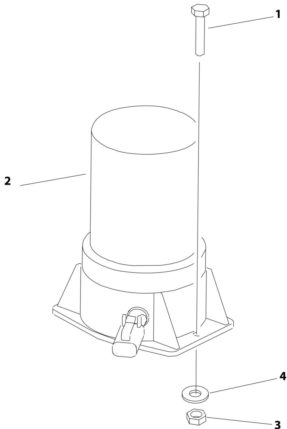
FIGURE 2-20. BEACON LIGHT INSTALLATION - AMBER (OPTIONAL)
