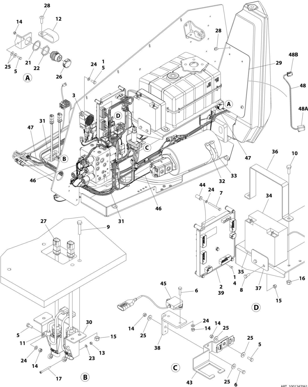
FIGURE 2-18. ELECTRICAL COMPONENTS INSTALLATION (Prior to SN 0300292053)
