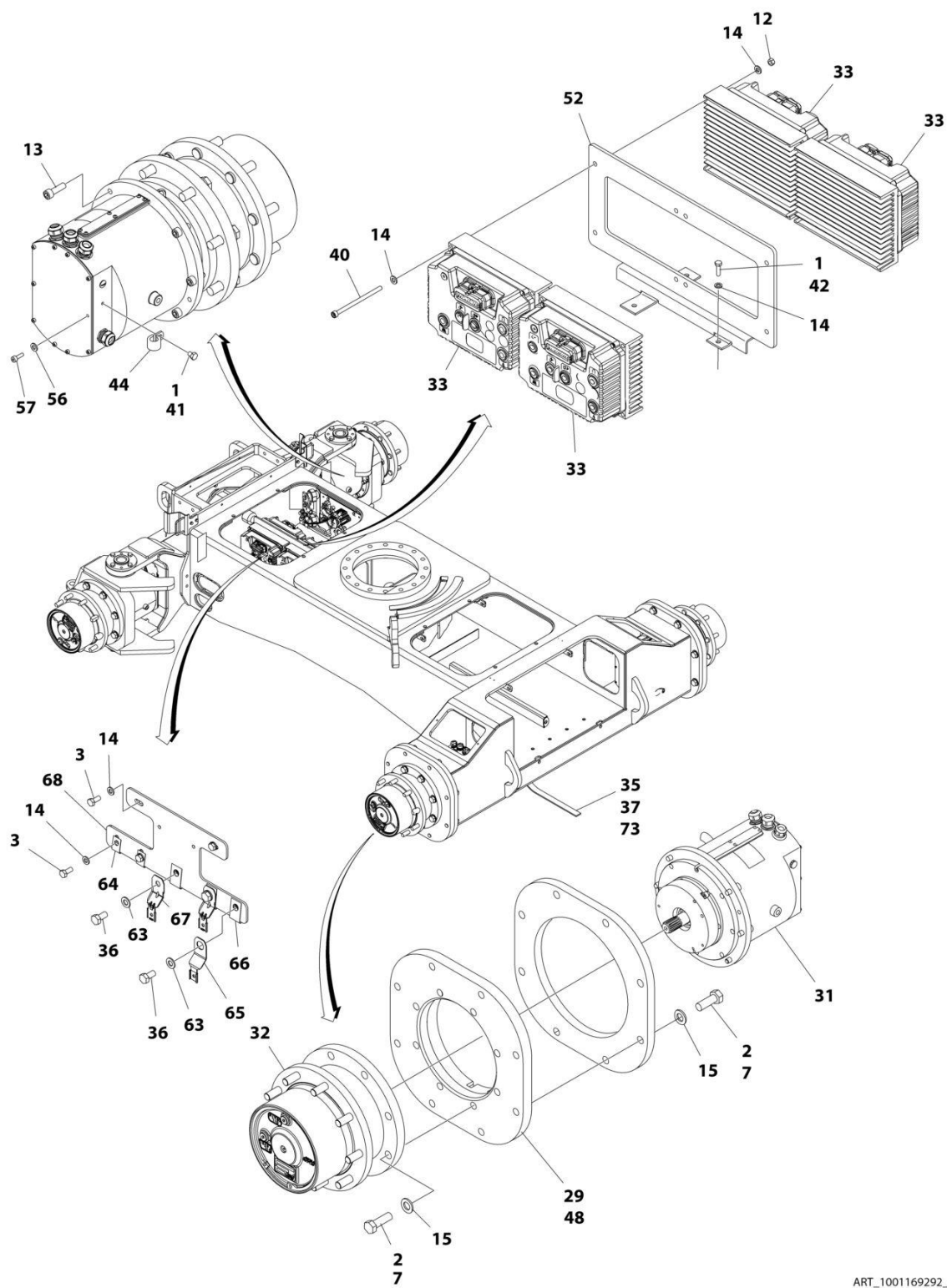
FIGURE 1-5. DRIVE INSTALLATION
