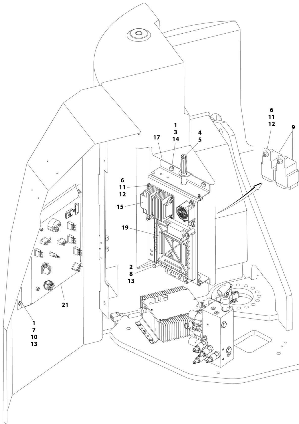
FIGURE 2-13. ELECTRICAL COMPONENTS INSTALLATION - E300AJP (ALL SPECS EXCEPT CE & UL SPECS)
