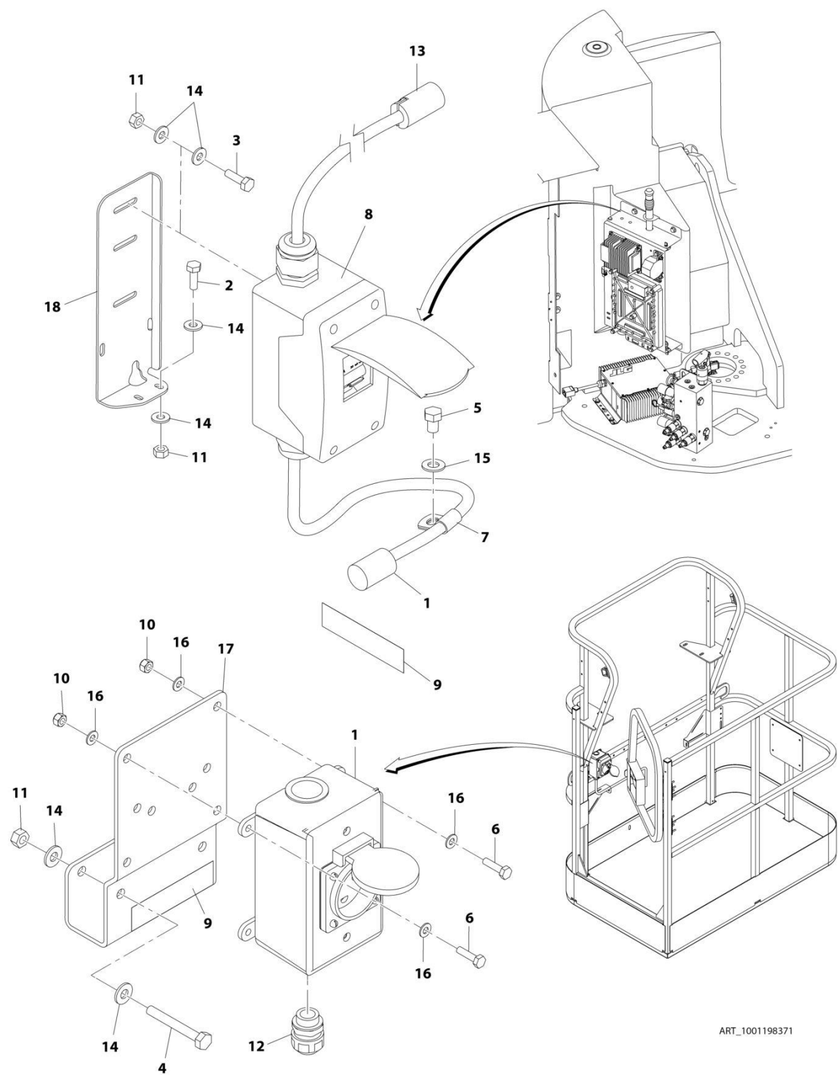
FIGURE 7-7. AC BOX AT PLATFORM INSTALLATION - 220V CEE7 POST GROUND (CE SPECS)
