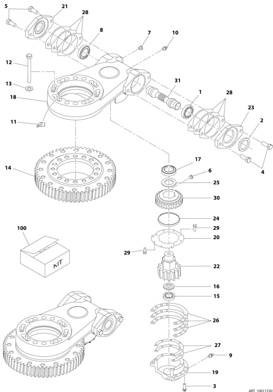
FIGURE 2-7. TURNTABLE BEARING ASSEMBLY
