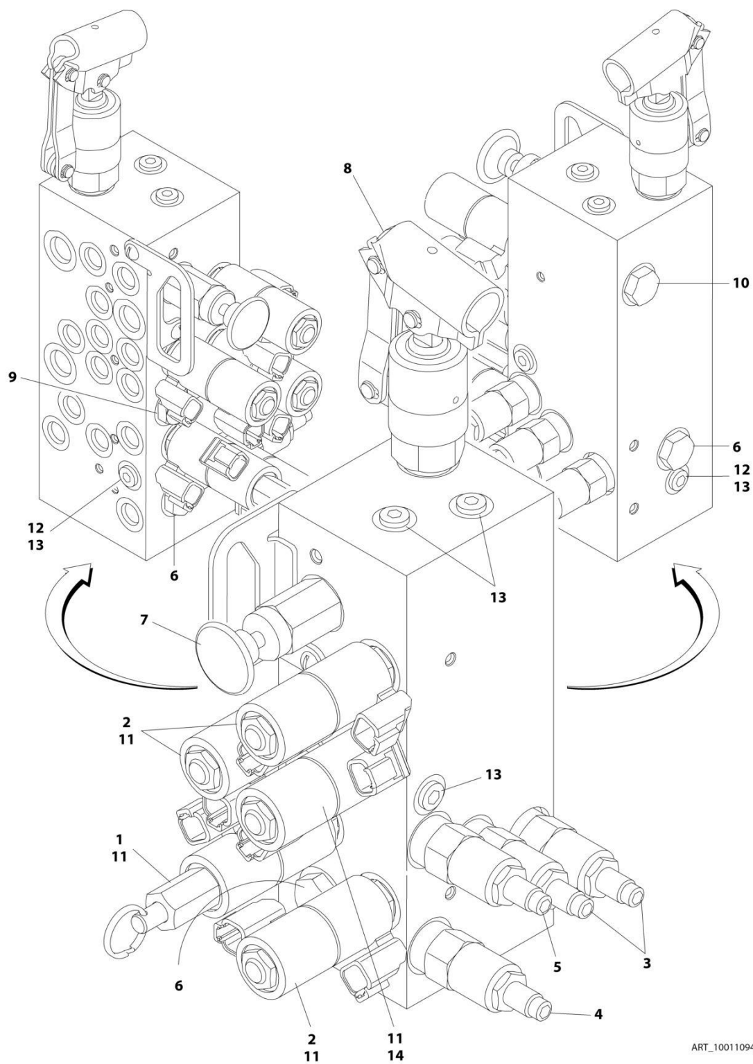
FIGURE 2-5. BOOM VALVE ASSEMBLY - E300AJP
