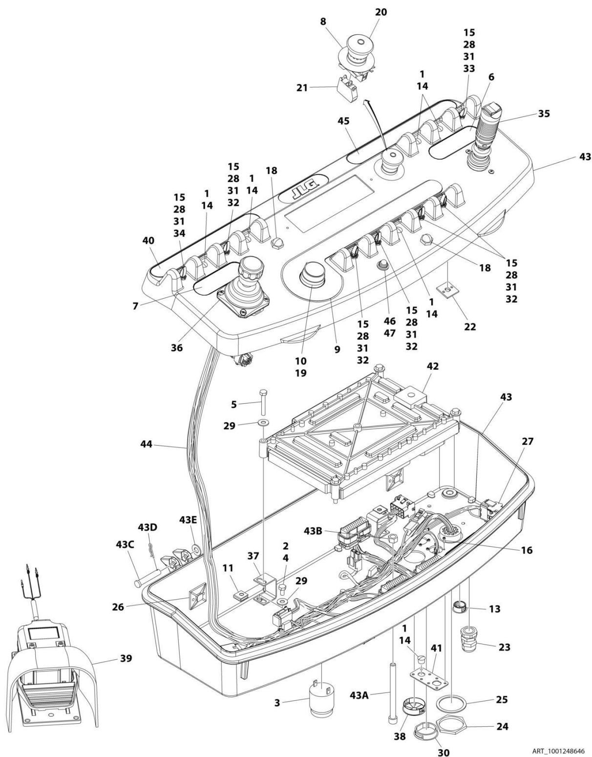
FIGURE 4-8. CONSOLE BOX ASSEMBLY - E300AJ (UL SPECS)
