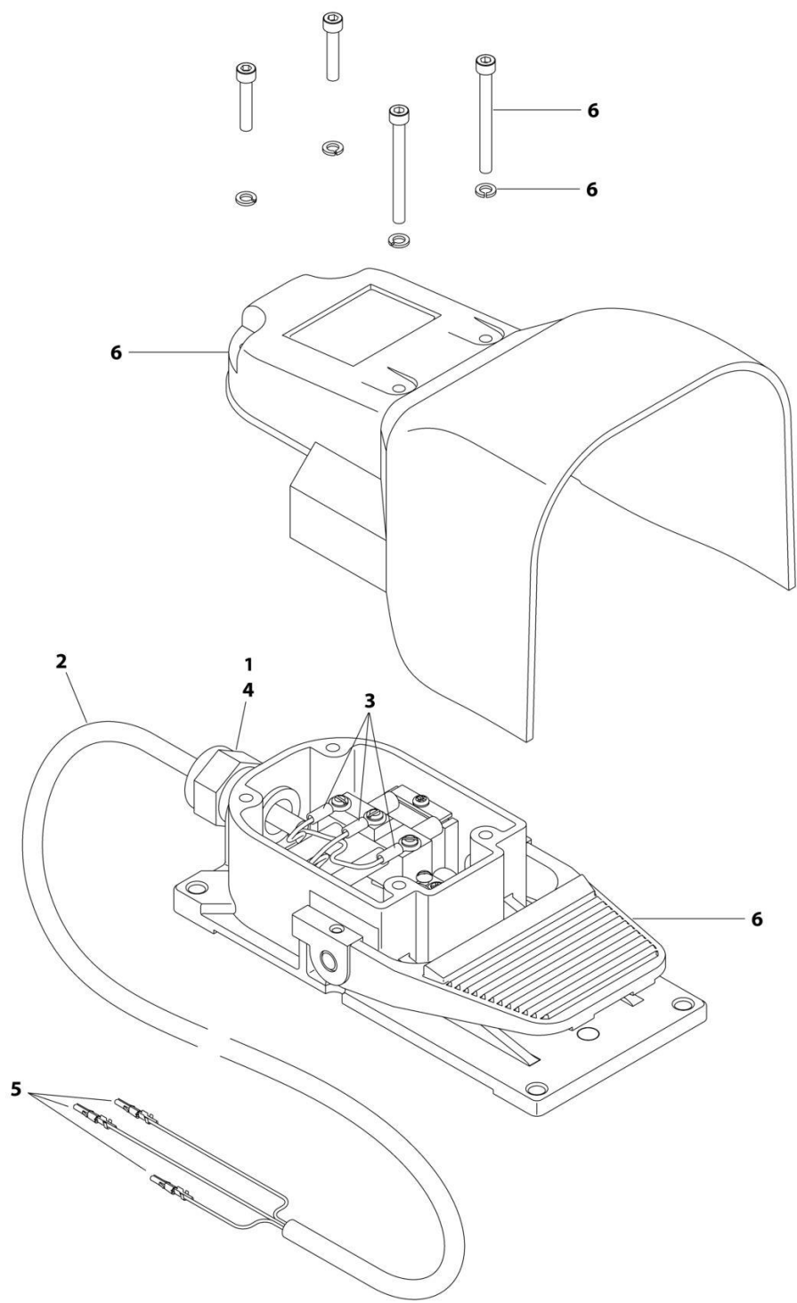
FIGURE 4-13. FOOTSWITCH ASSEMBLY
