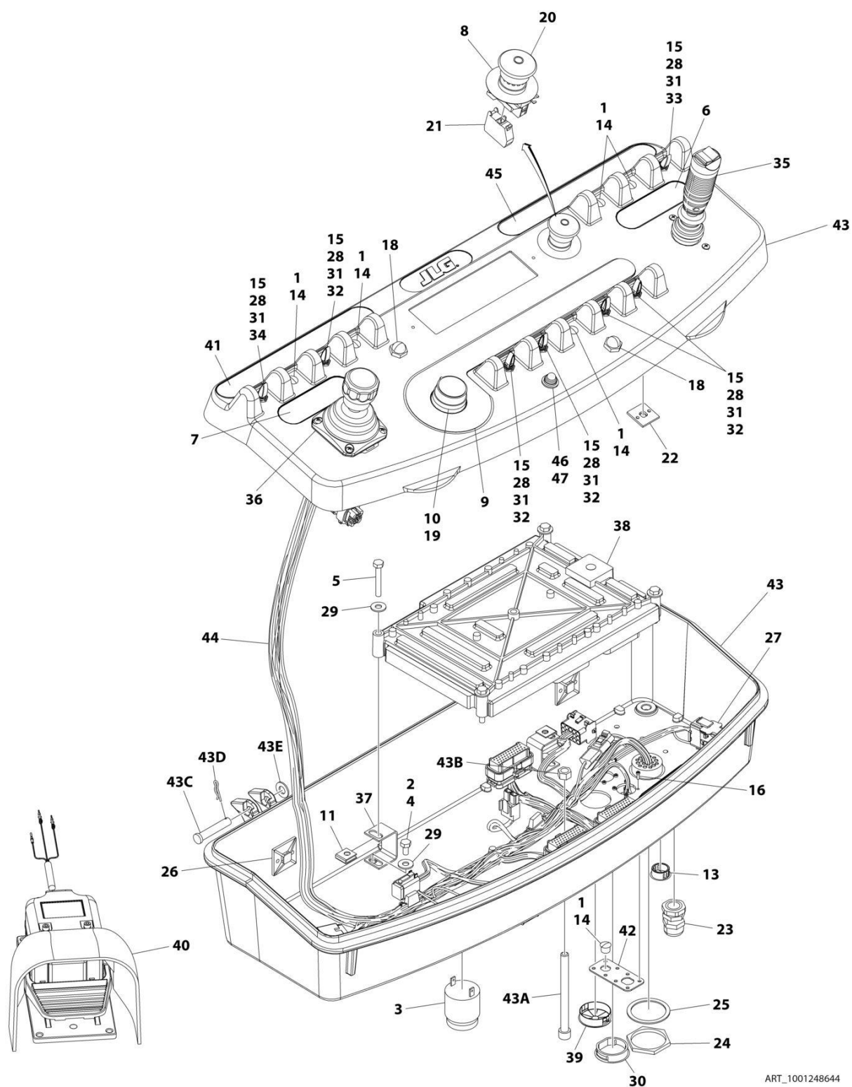
FIGURE 4-7. CONSOLE BOX ASSEMBLY - E300AJ (ALL SPECS EXCEPT UL SPECS)
