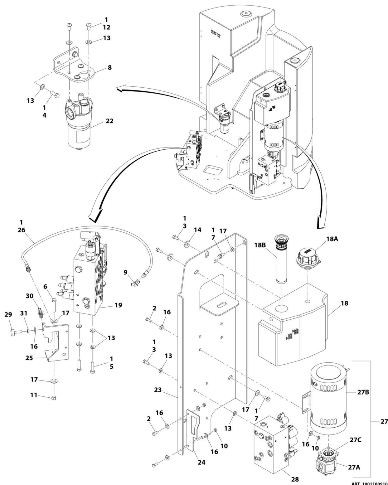
FIGURE 2-2. VALVES, TANK AND MOTOR INSTALLATION - E300AJP
