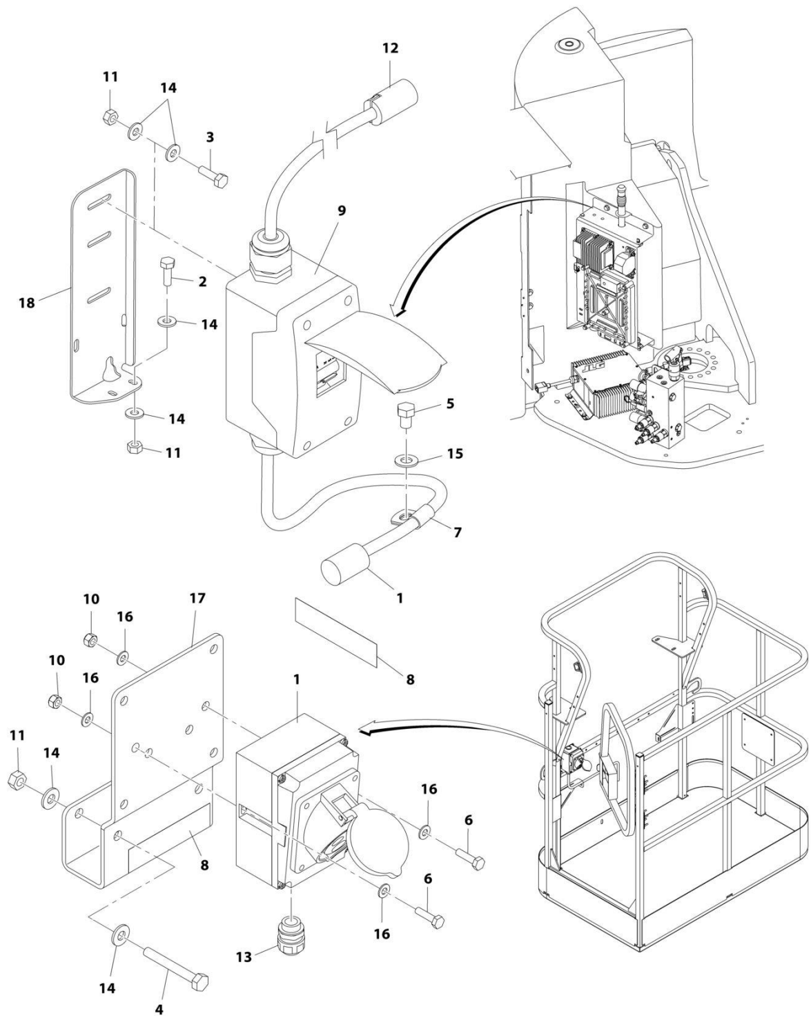
FIGURE 7-4. AC BOX AT PLATFORM INSTALLATION - 110V IEC YELLOW (CE SPECS)
