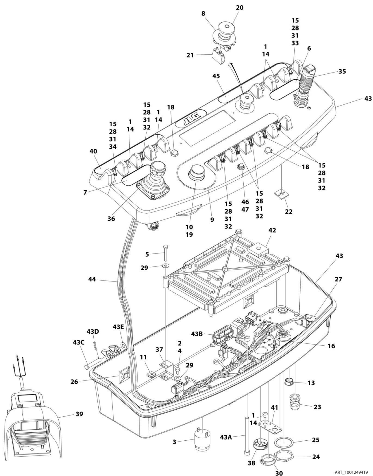
FIGURE 4-10. CONSOLE BOX ASSEMBLY - E300AJP (UL SPECS)
