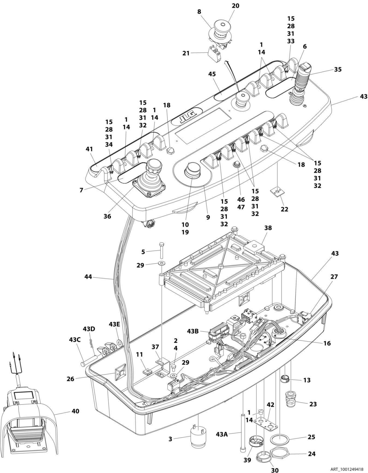
FIGURE 4-9. CONSOLE BOX ASSEMBLY - E300AJP (ALL SPECS EXCEPT UL SPECS)
