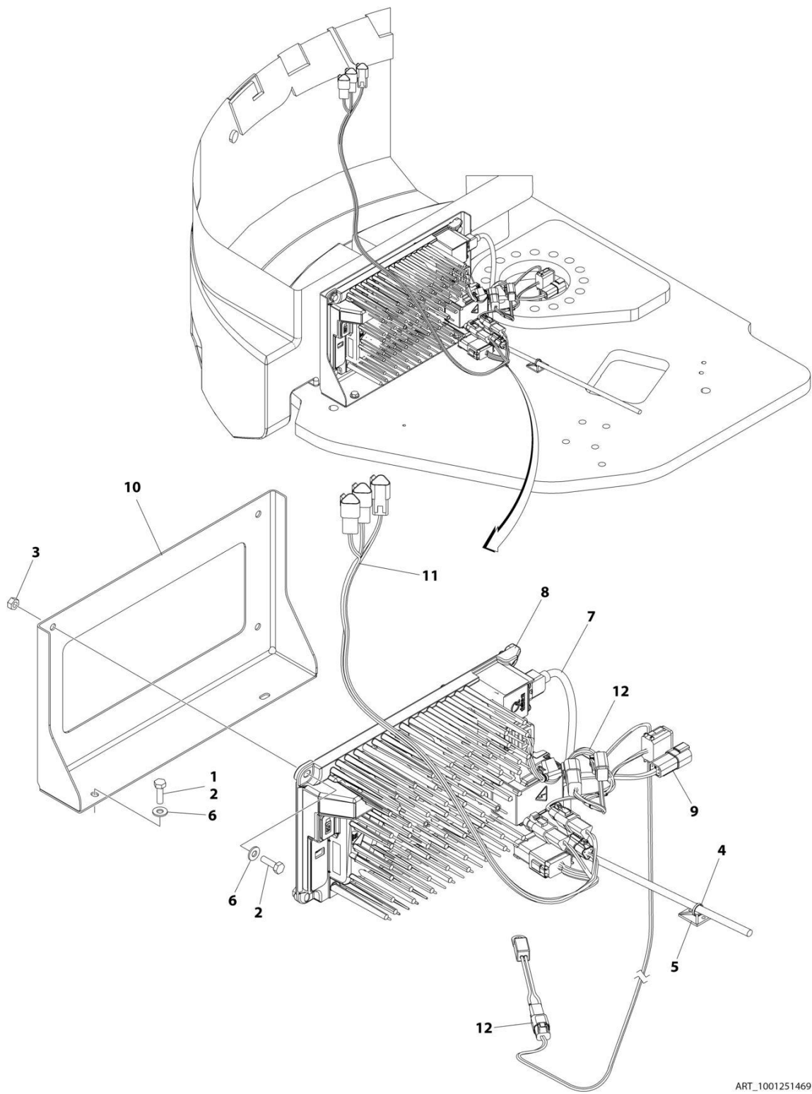
FIGURE 2-25. BATTERY CHARGER INSTALLATION - WITHOUT PLUG (PVC 2007)
