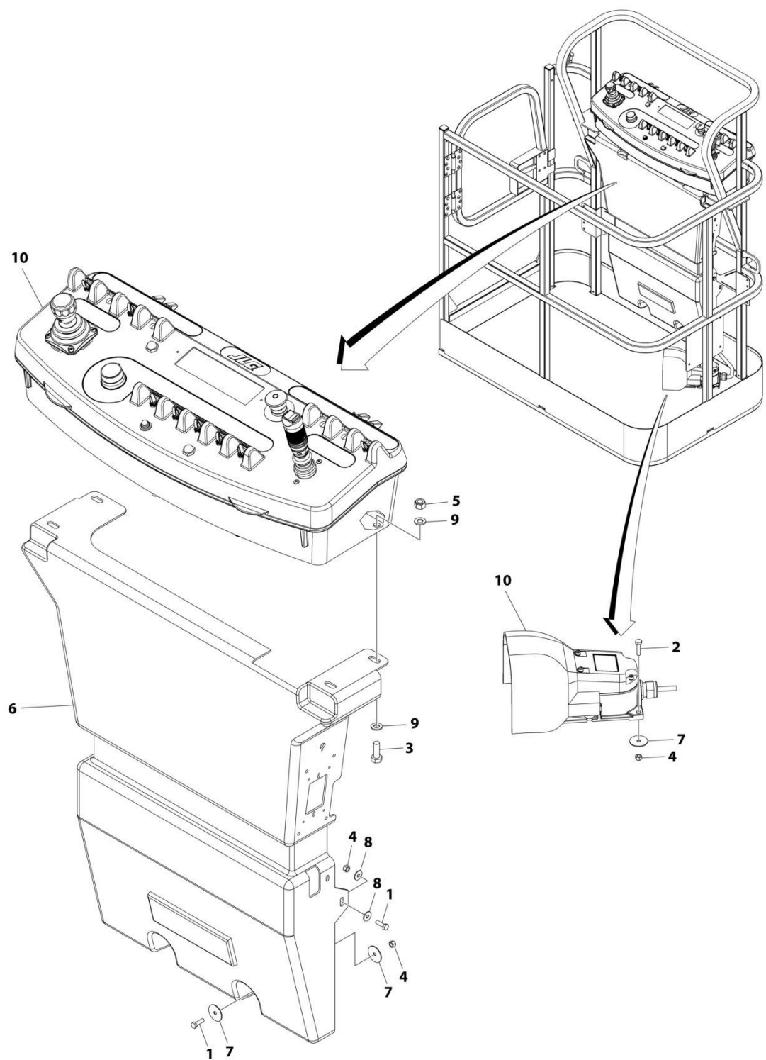
FIGURE 4-5. PLATFORM CONSOLE AND FOOTSWITCH INSTALLATION - E300AJP (ALL SPECS EXCEPT UL SPECS)
