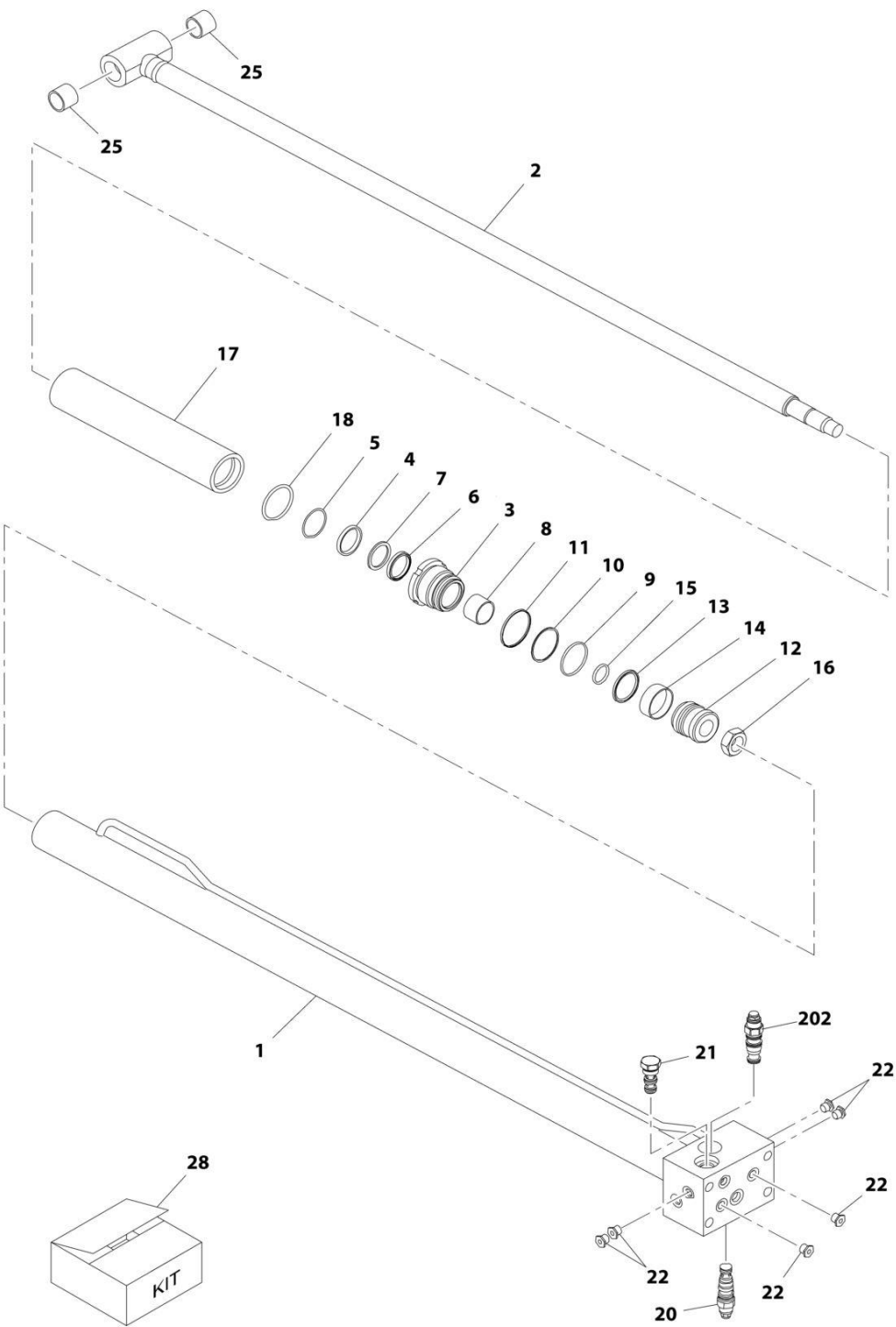
FIGURE 5-7. TELESCOPE CYLINDER ASSEMBLY - E300AJ
