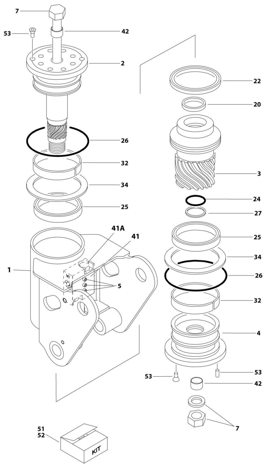
FIGURE 3-10. ROTATOR ASSEMBLY - JIB SWING
