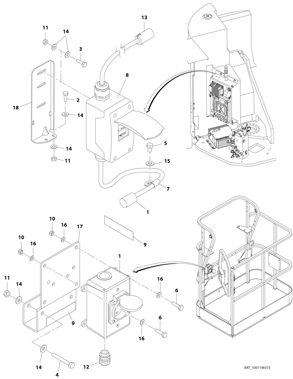
FIGURE 7-6. AC BOX AT PLATFORM INSTALLATION - 220V AFSINT107 KEYED GROUND (CE SPECS)
