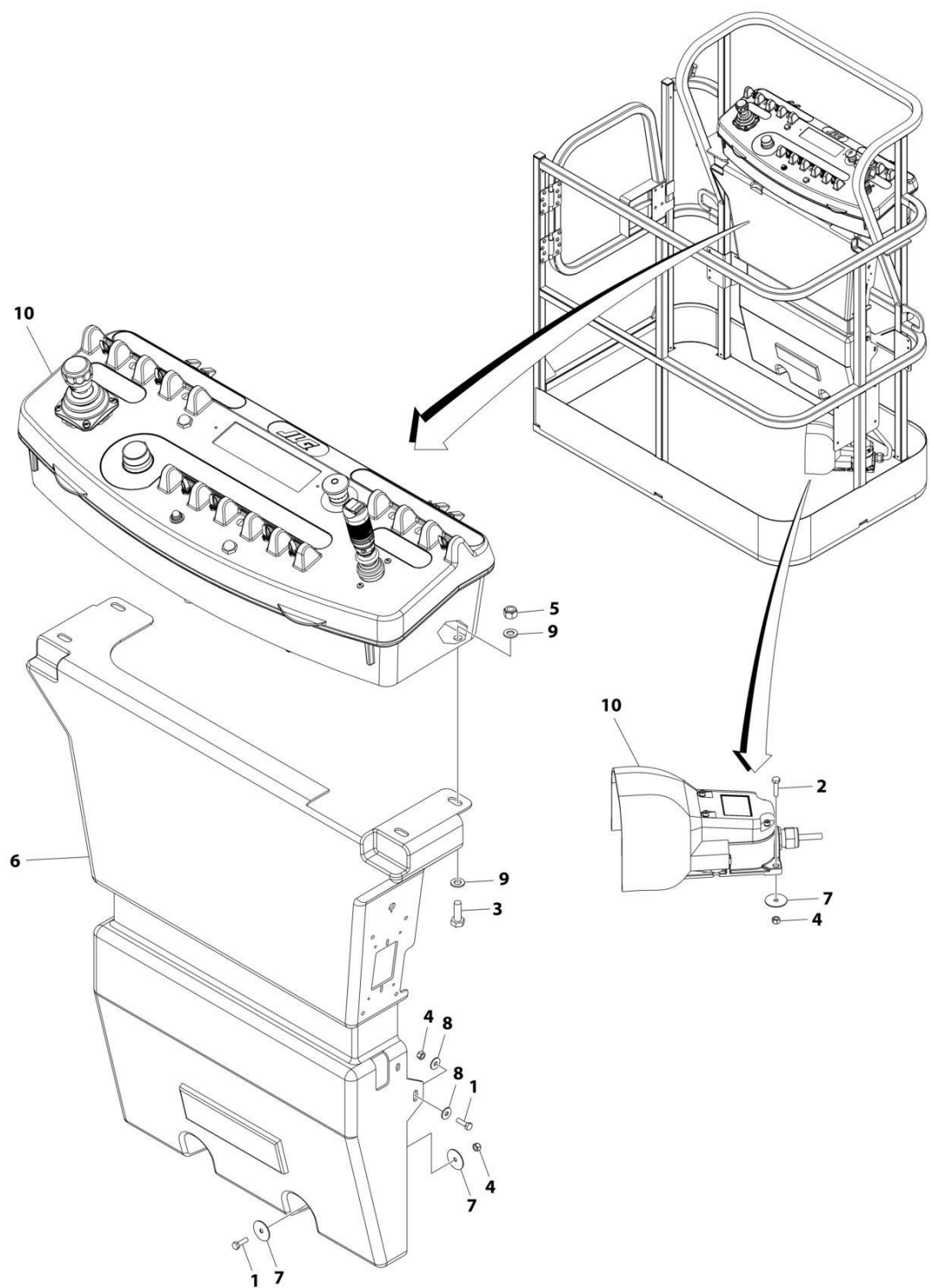
FIGURE 4-3. PLATFORM CONSOLE AND FOOTSWITCH INSTALLATION - E300AJ (ALL SPECS EXCEPT UL SPECS)
