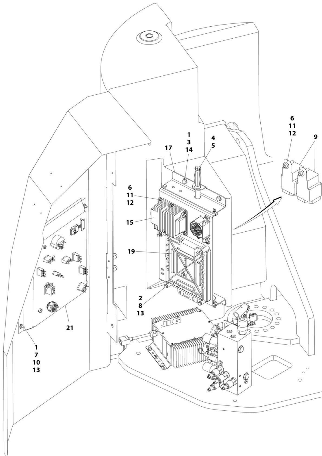
FIGURE 2-10. ELECTRICAL COMPONENTS INSTALLATION - E300AJ (ALL SPECS EXCEPT CE & UL SPECS)
