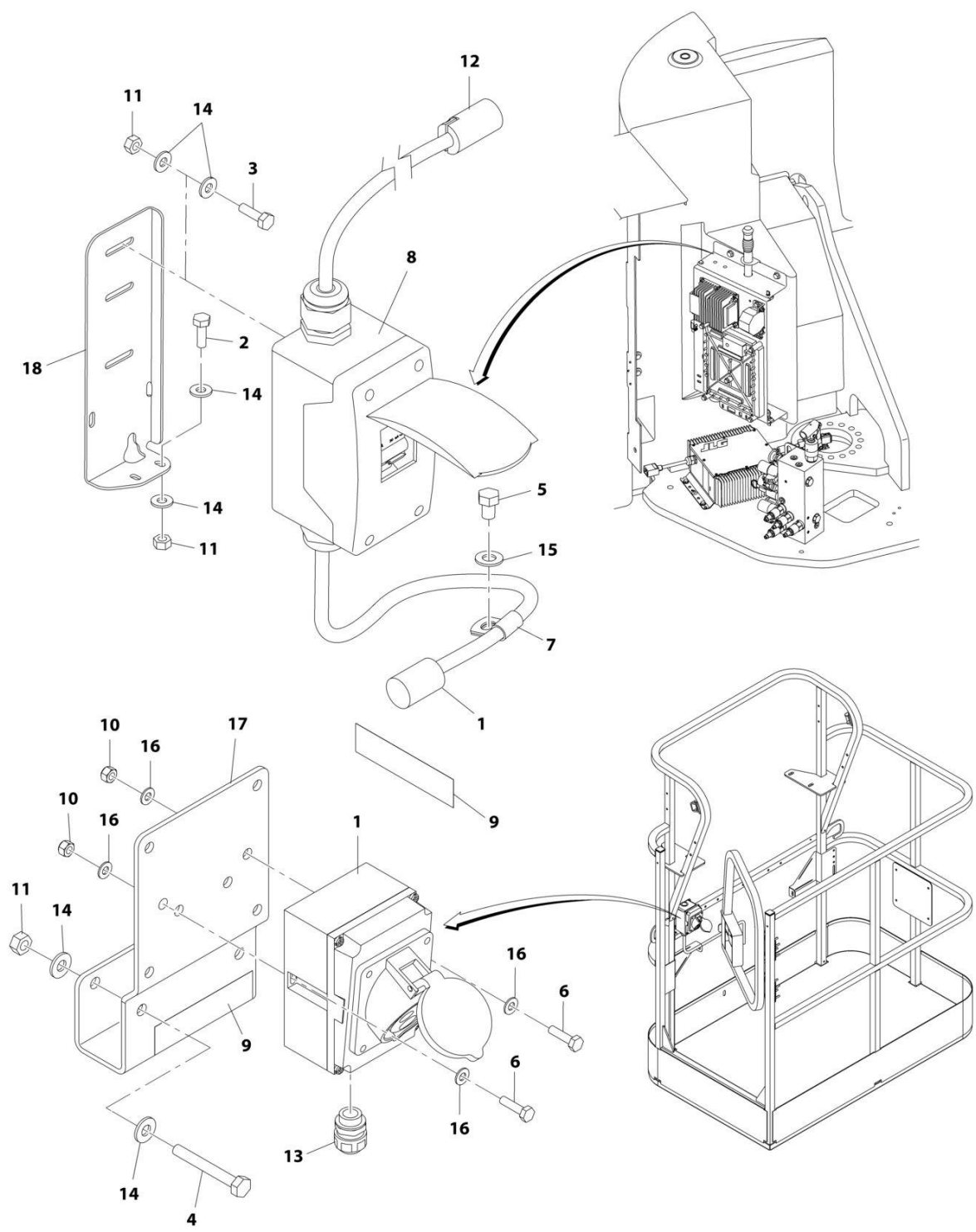
FIGURE 7-5. AC BOX AT PLATFORM INSTALLATION - 220V IEC BLUE (CE SPECS)
