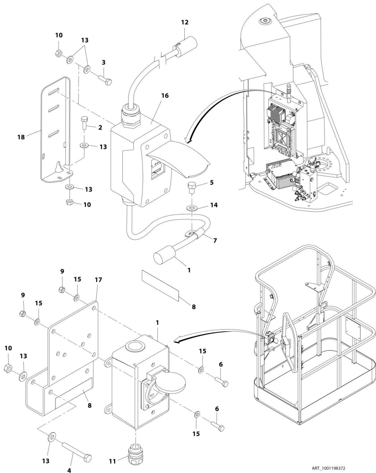
FIGURE 7-8. AC BOX AT PLATFORM INSTALLATION - 220V CEE7 SIDE GROUND (CE SPECS)
