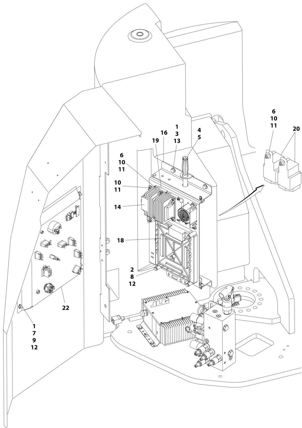
FIGURE 2-12. ELECTRICAL COMPONENTS INSTALLATION - E300AJ (UL SPECS)
