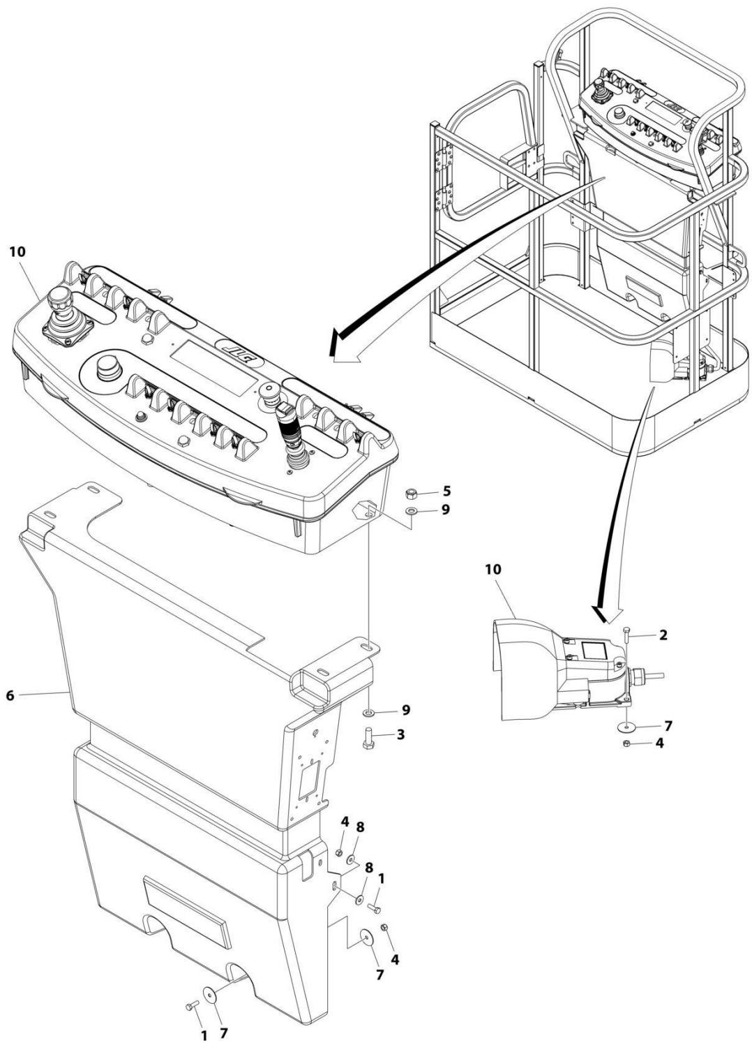
FIGURE 4-4. PLATFORM CONSOLE AND FOOTSWITCH INSTALLATION - E300AJ (UL SPECS)
