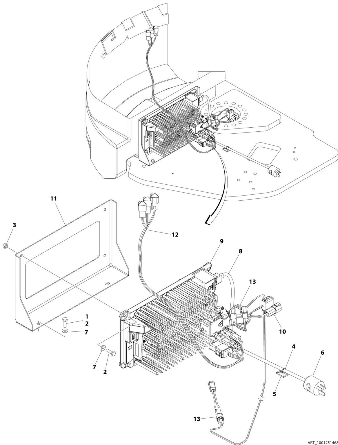
FIGURE 2-23. BATTERY CHARGER INSTALLATION - WITH PLUG (CE SPECS) (PVC 2007)
