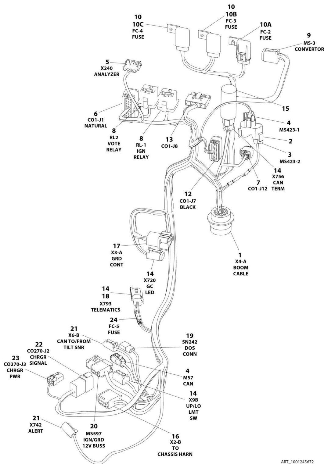
FIGURE 7-45. TURNTABLE HARNESS
