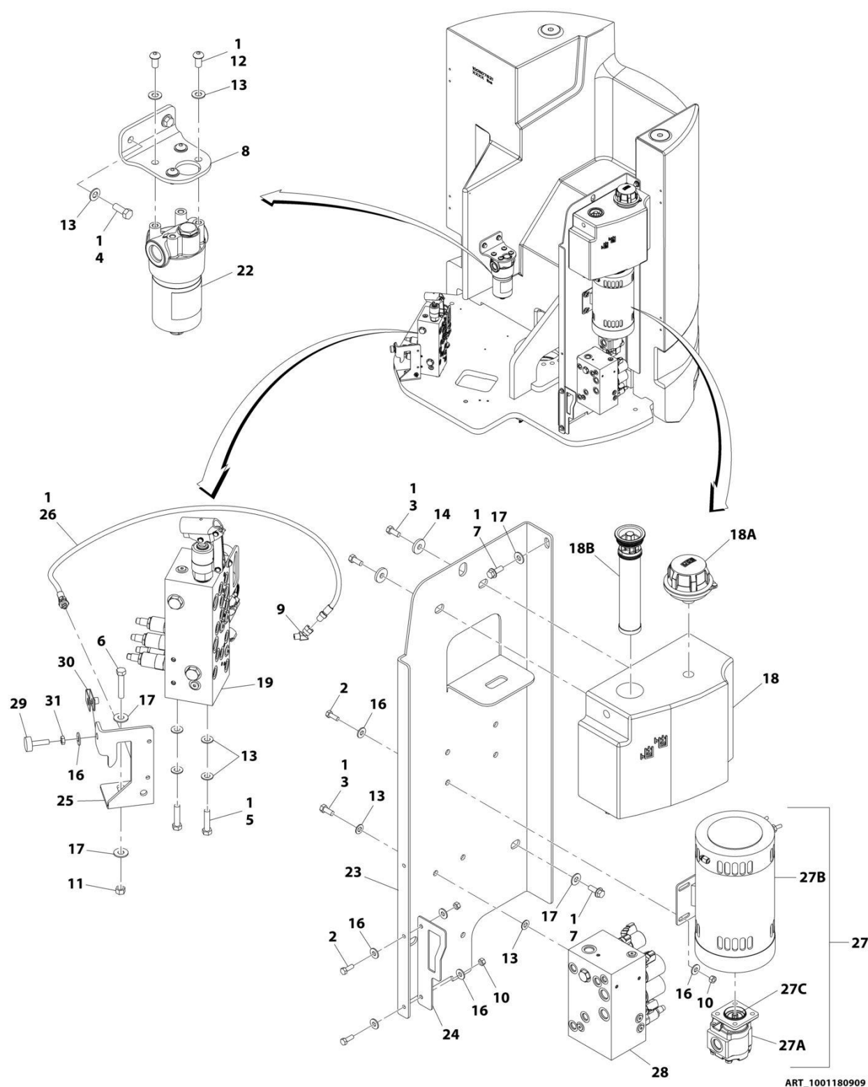
FIGURE 2-1. VALVES, TANK AND MOTOR INSTALLATION - E300AJ
