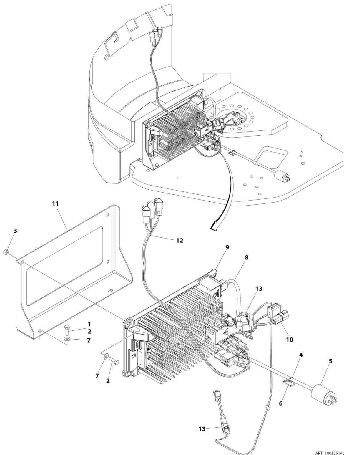
FIGURE 2-21. BATTERY CHARGER INSTALLATION - WITH PLUG (ALL SPECS EXCEPT CE SPECS) (PVC 2007)
