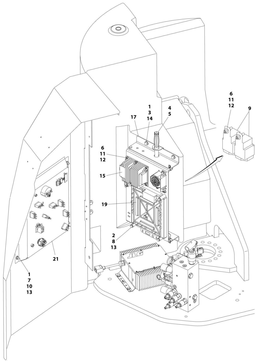
FIGURE 2-11. ELECTRICAL COMPONENTS INSTALLATION - E300AJ (CE SPECS)
