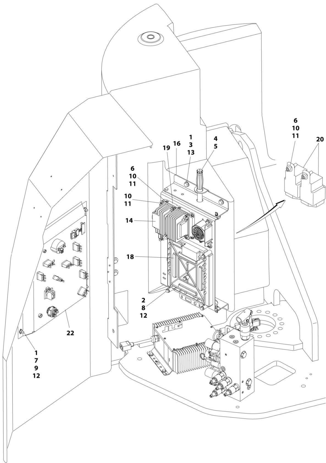
FIGURE 2-15. ELECTRICAL COMPONENTS INSTALLATION - E300AJP (UL SPECS)
