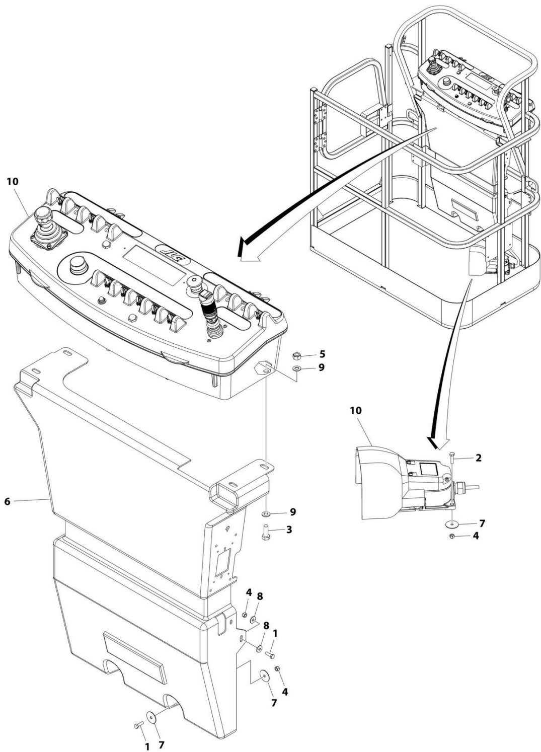
FIGURE 4-6. PLATFORM CONSOLE AND FOOTSWITCH INSTALLATION - E300AJP (UL SPECS)
