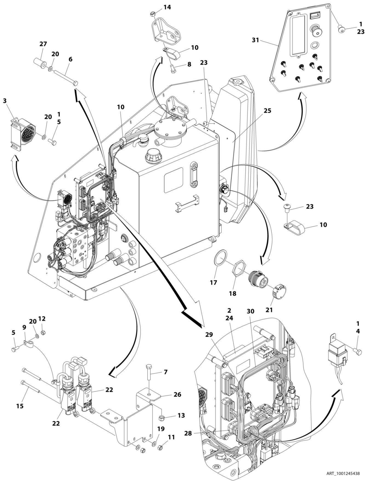
FIGURE 2-11. ELECTRICAL COMPONENTS INSTALLATION (ALL SPECS EXCEPT CE) (PVC 2001)
