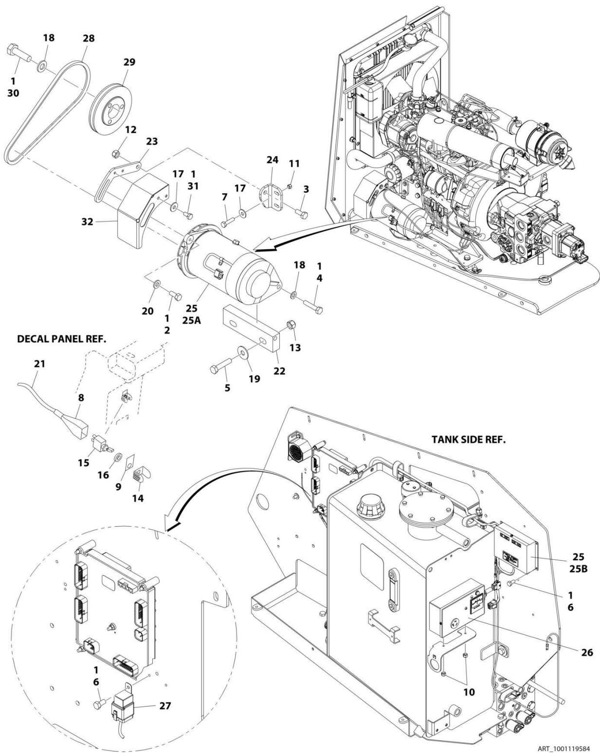
FIGURE 3-28. 3500W GENERATOR INSTALLATION - KUBOTA ENGINE MACHINES 220V/60HZ GENERATOR (ANSI EXPORT, CHINA AND CSA SPECS)
