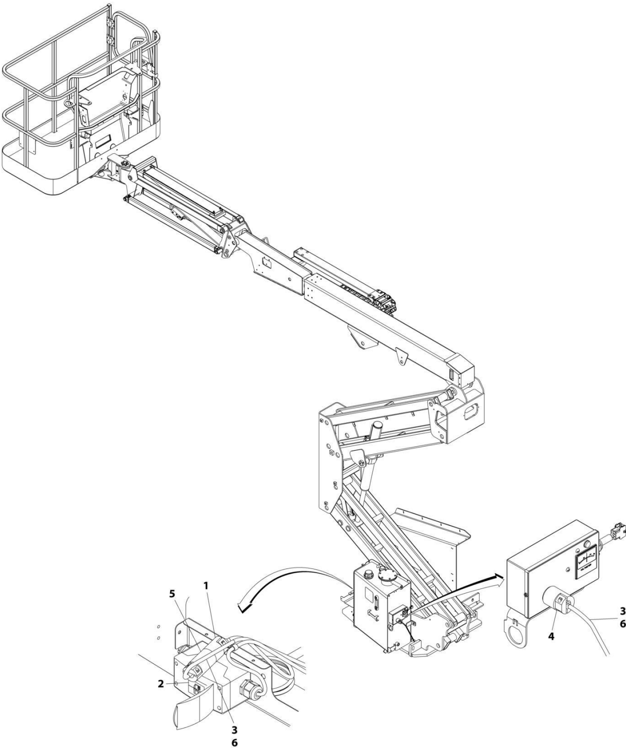
FIGURE 8-41. GENERATOR TO AC PLUG HARNESS - 2800W GENERATOR 220/50HZ (ANSI EXPORT, AUSTRALIAN, CE AND CHINA SPECS)
