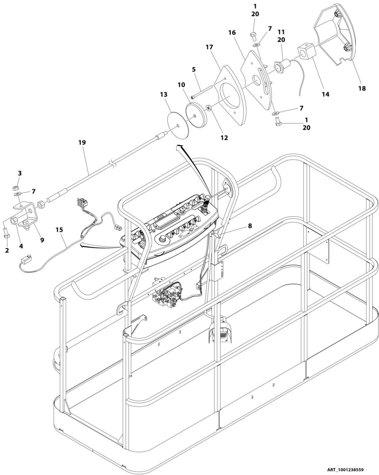
FIGURE 5-15. SKYLINE INSTALLATION
