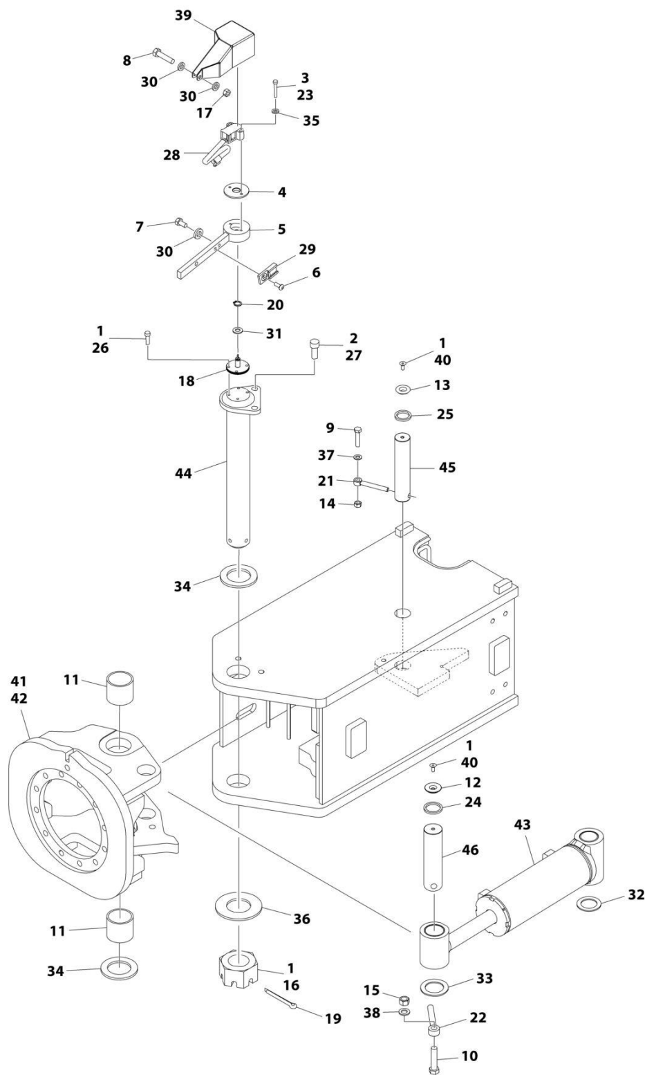
FIGURE 1-3. STEER INSTALLATION - 2WS
