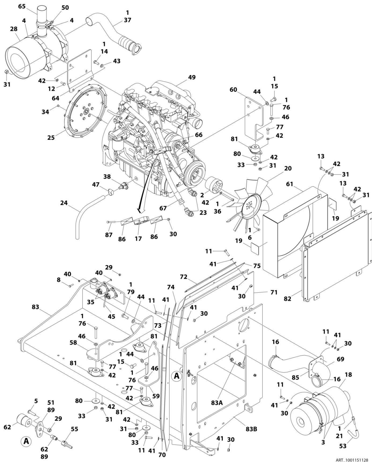
FIGURE 3-3. DEUTZ TD2011 ENGINE ASSEMBLY (PVC2001)
