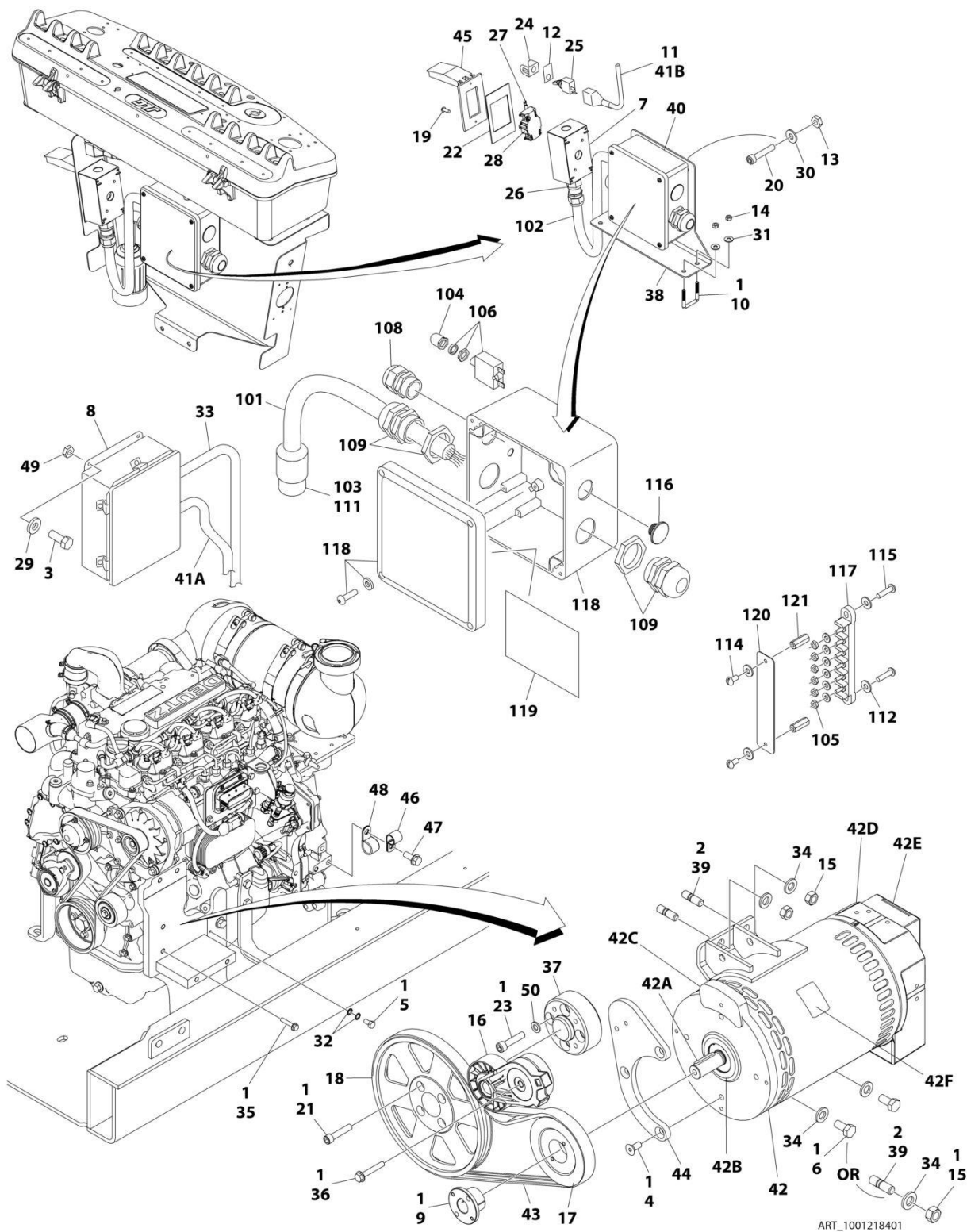
FIGURE 3-21. 7500W SKYPOWER GENERATOR INSTALLATION - 60HZ/240V (DEUTZ TD2.9L4 T4F ENGINES) (OPTIONAL)
