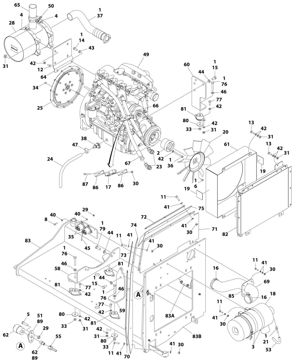
FIGURE 3-4. DEUTZ TD2011 ENGINE ASSEMBLY (PVC2007)
