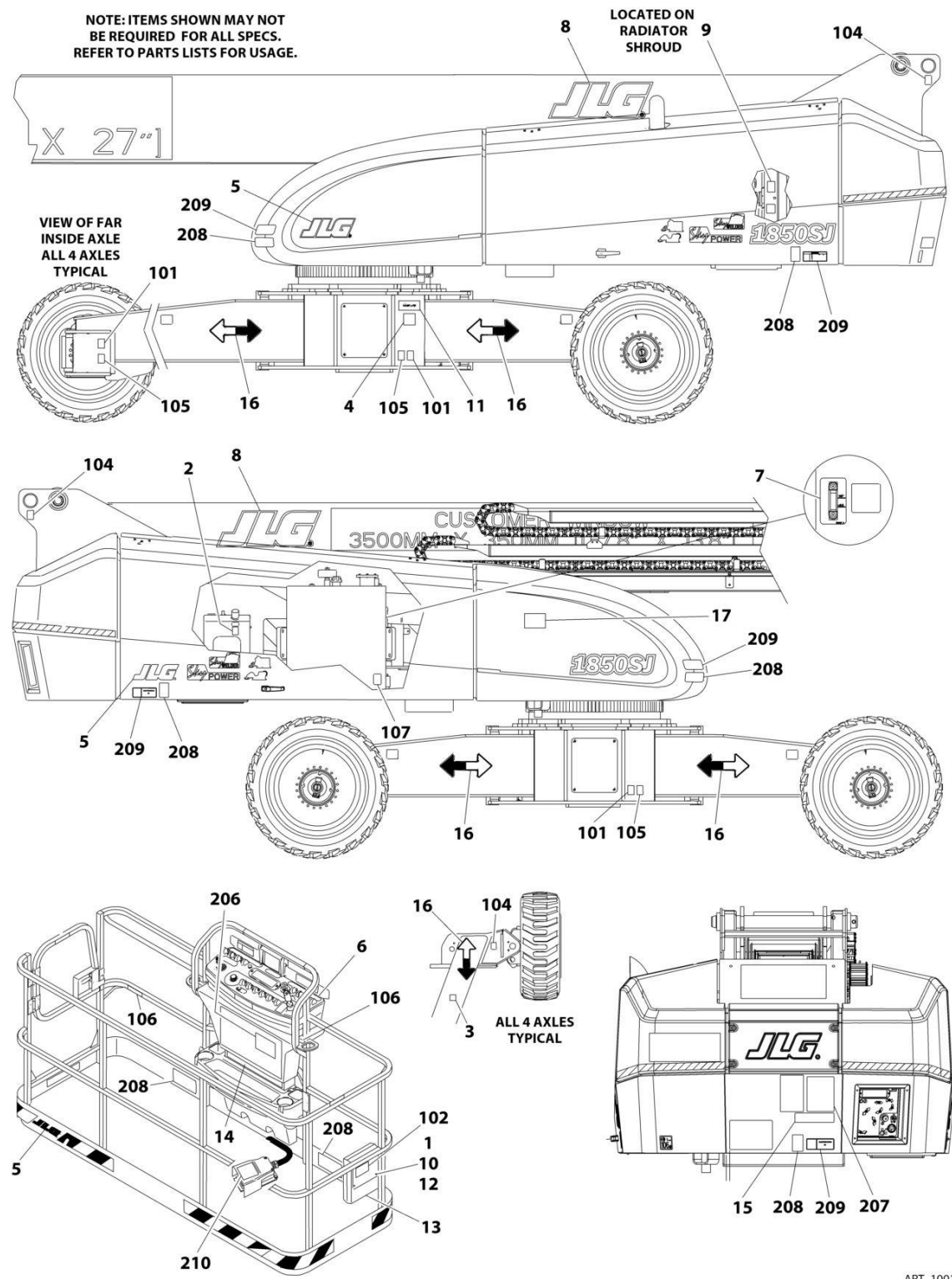
FIGURE 9-5. DECAL INSTALLATION - CE SPECS
