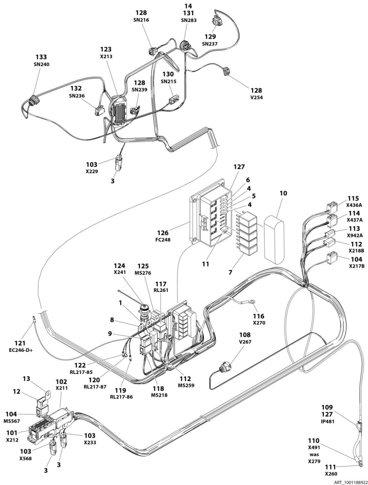
FIGURE 8-33. ENGINE HARNESS - DEUTZ HRC ENGINES
