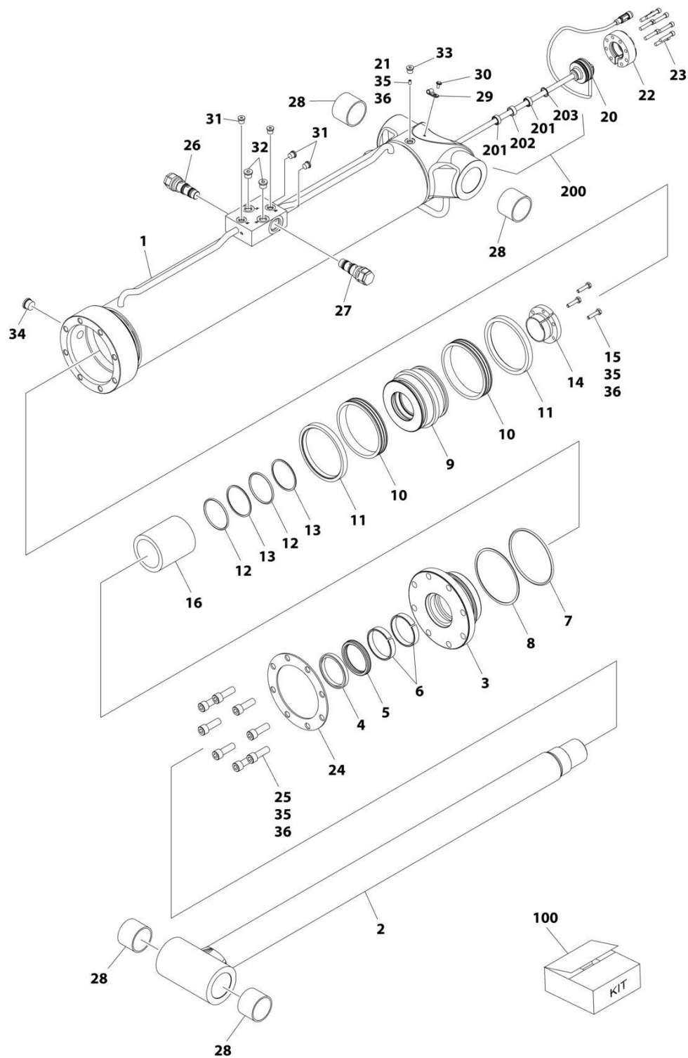
FIGURE 6-5. LIFT CYLINDER ASSEMBLY - JIB
