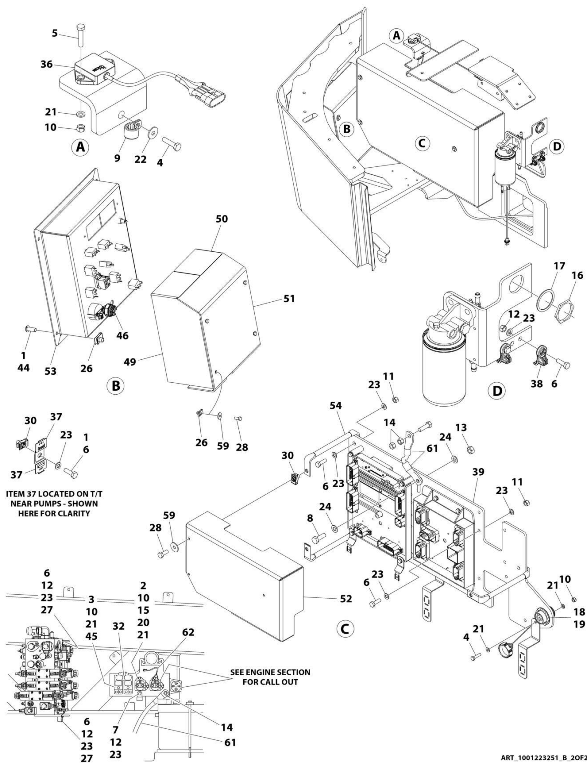
FIGURE 2-16. TURNTABLE ELECTRICAL COMPONENTS INSTALLATION (CE (LRC) SPECS)
