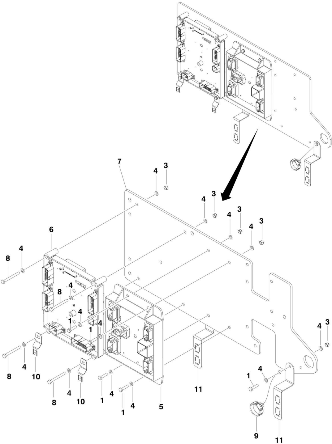
FIGURE 2-24. ELECTRICAL PANEL ASSEMBLY
