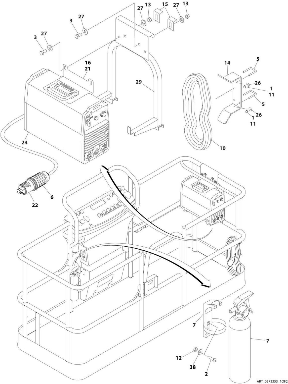
FIGURE 5-23. SKYWELDER/SKYCUTTER COMBO INSTALLATION (60HZ) (ANSI, ANSI EXPORT, CHINA CSA AND JAPANESE SPECS)
