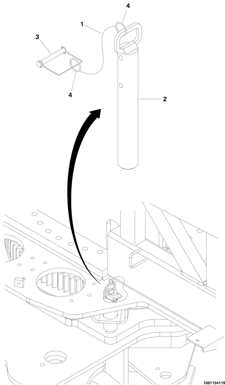
FIGURE 2-4. TURNTABLE LOCK INSTALLATION
