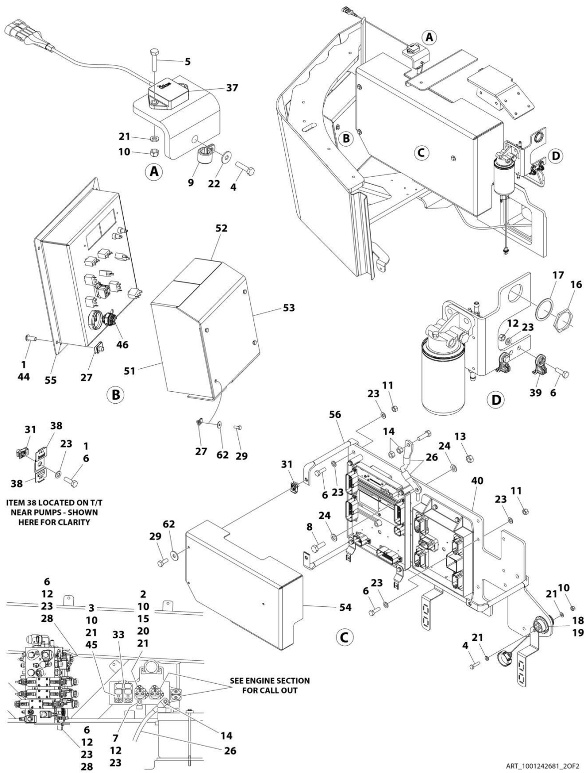
FIGURE 2-15. TURNTABLE ELECTRICAL COMPONENTS INSTALLATION (ANSI, ANSI EXPORT (HRC), CSA AND JAPANESE SPECS)
