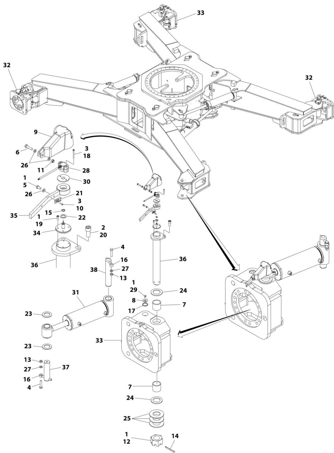
FIGURE 1-2. STEERING INSTALLATION
