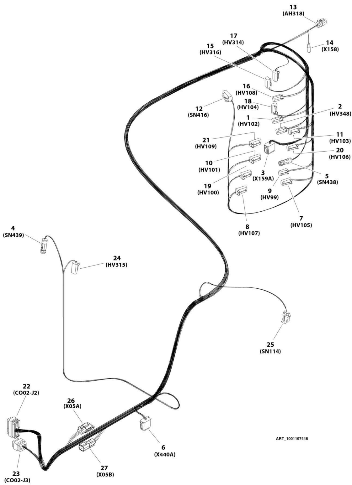
FIGURE 8-67. VALVE BANK HARNESS
