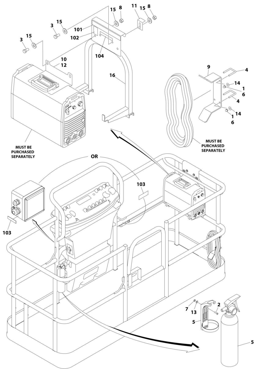
FIGURE 5-38. SKYWELDER PREP PACKAGE (60HZ) (ANSI, ANSI EXPORT, CHINA AND CSA SPECS)
