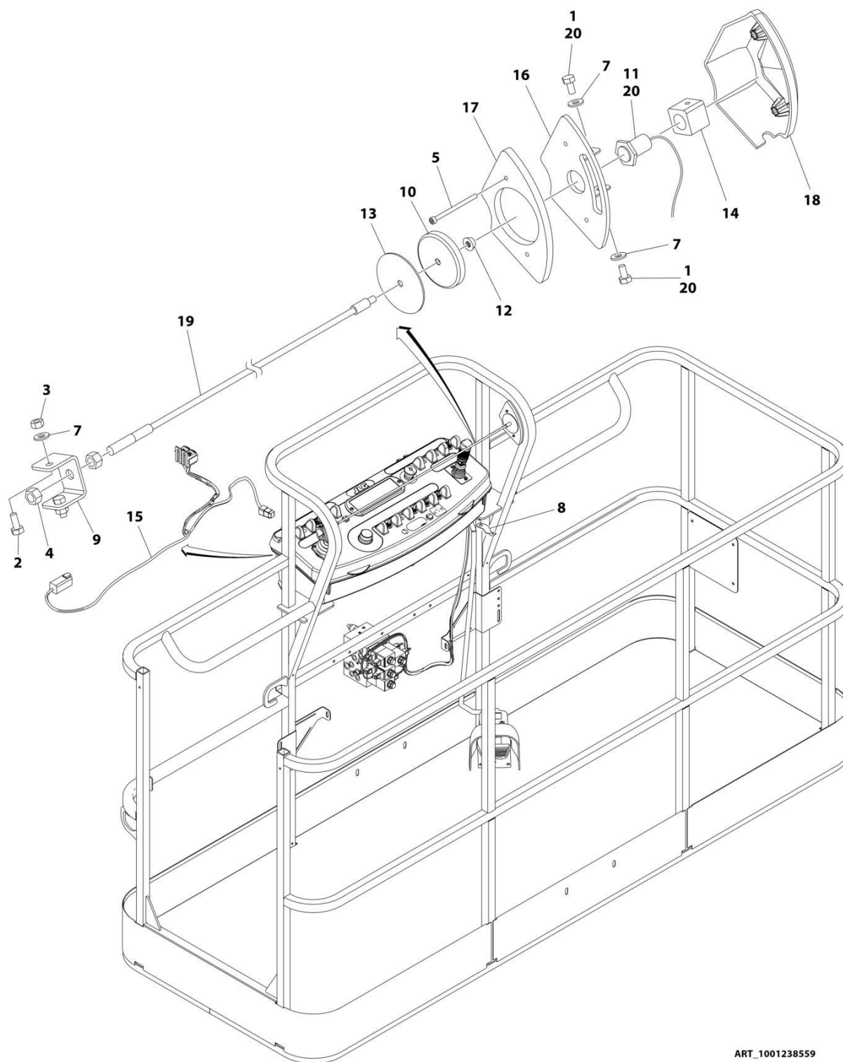
FIGURE 5-35. SKYLINE INSTALLATION
