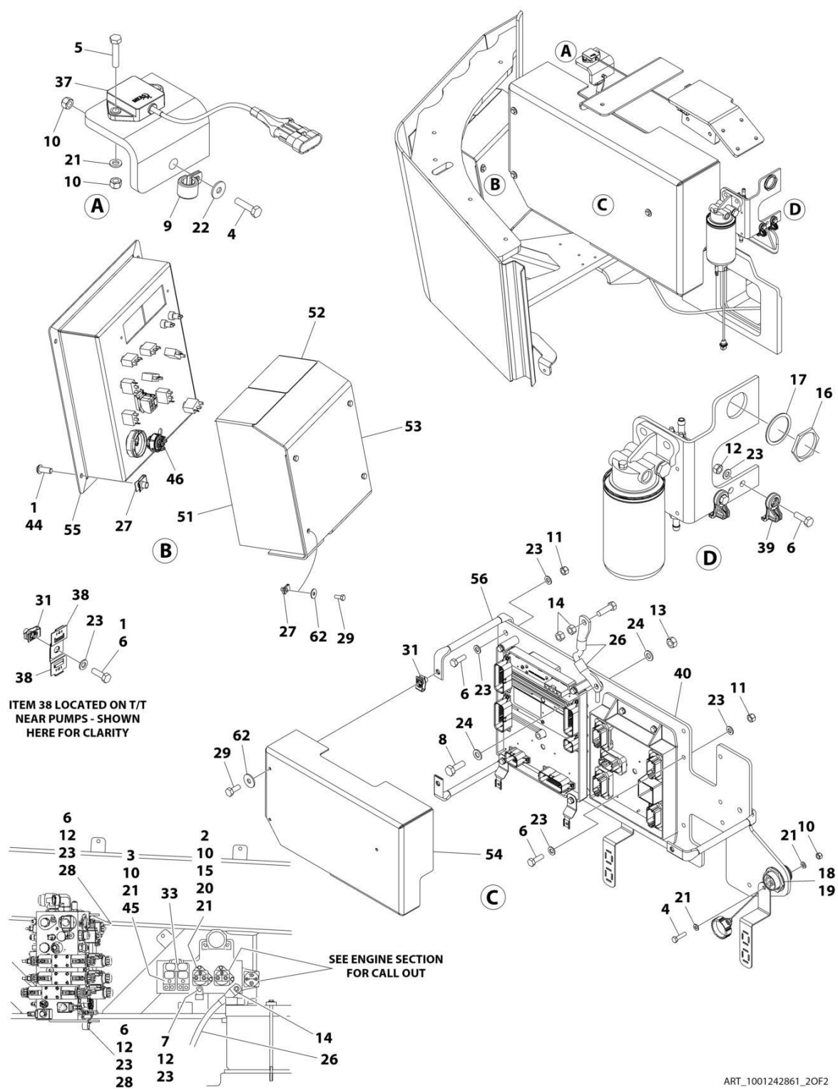
FIGURE 2-17. TURNTABLE ELECTRICAL COMPONENTS INSTALLATION (CE SPECS)
