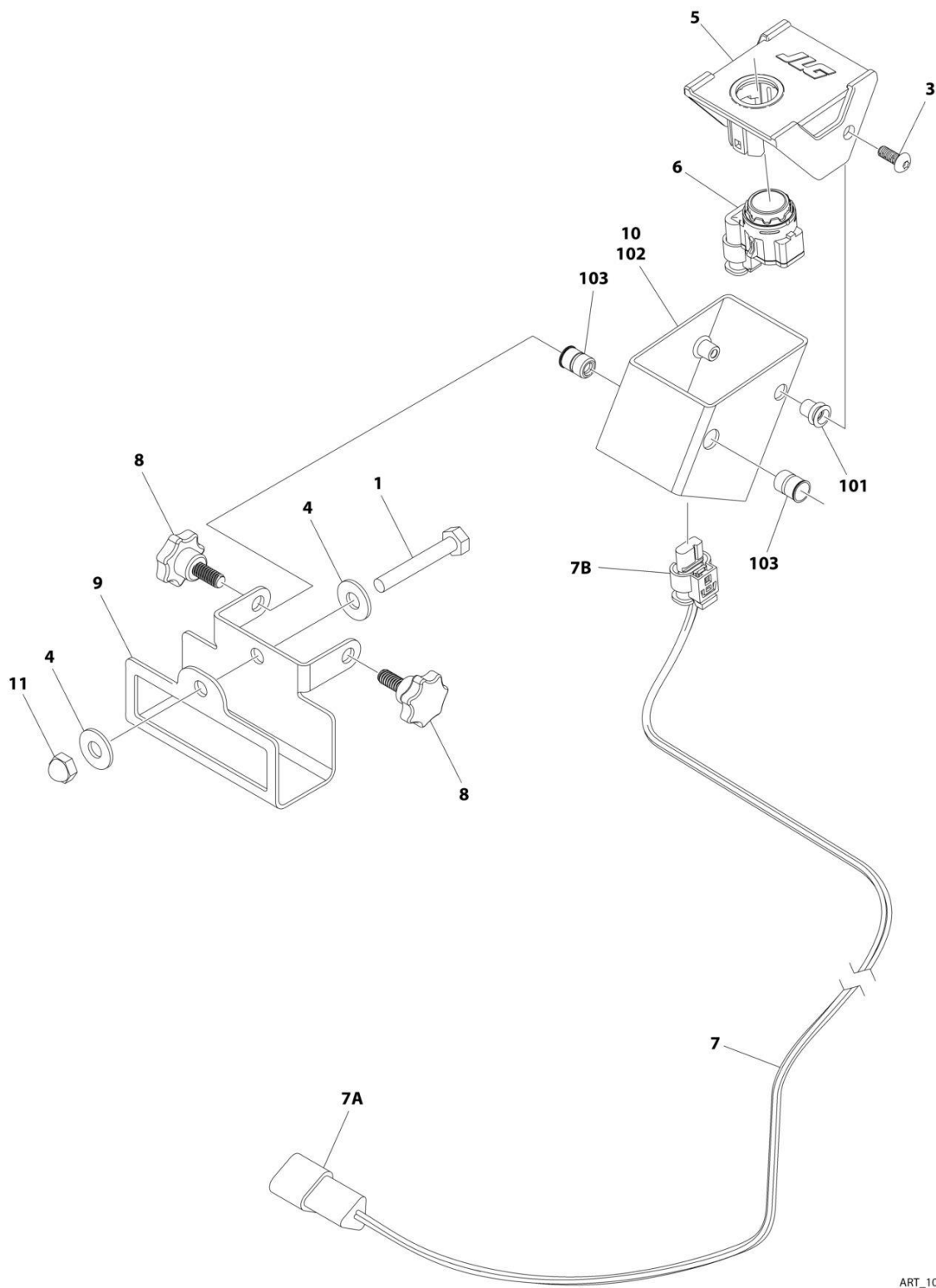
FIGURE 5-34. SKYSENSE OVERHEAD SENSOR ASSEMBLY
