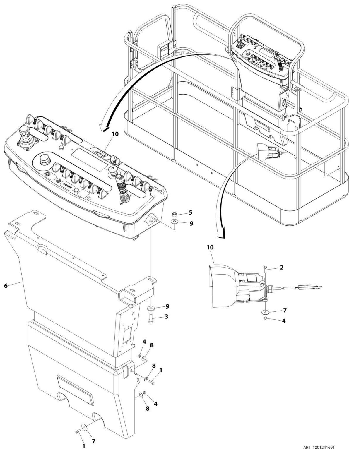
FIGURE 5-12. PLATFORM CONTROLS INSTALLATION - WITH SKYGUARD
