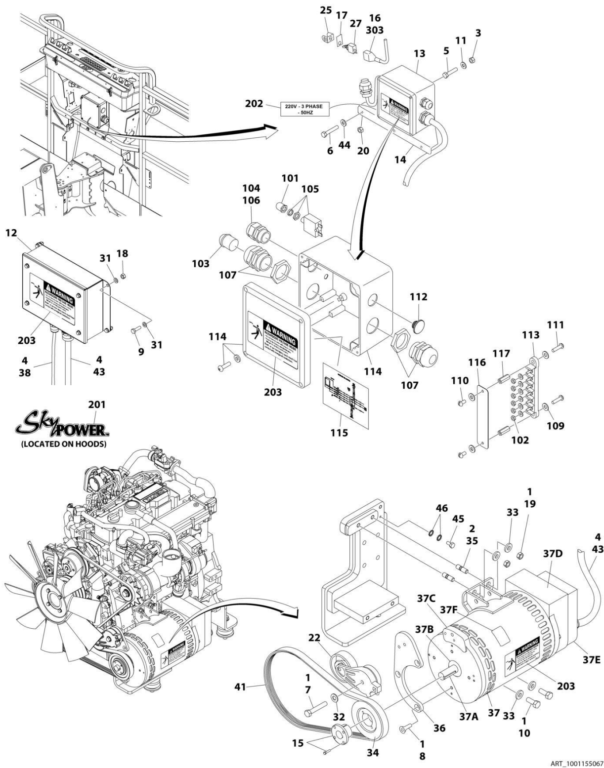
FIGURE 3-29. 7500W SKYPOWER GENERATOR INSTALLATION - 50HZ (OPTIONAL)
