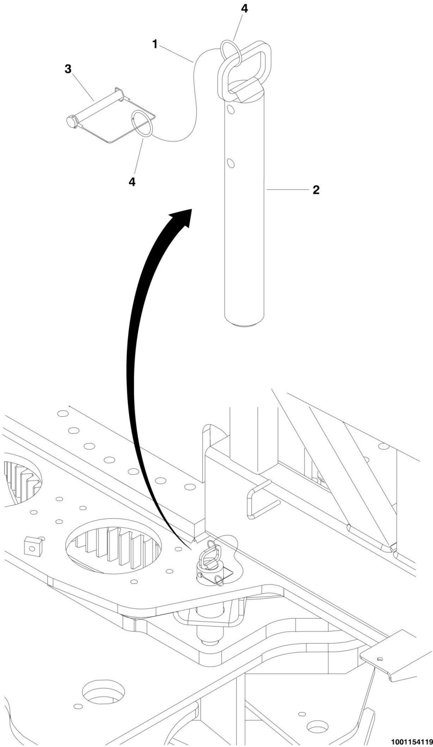
FIGURE 2-4. TURNTABLE LOCK INSTALLATION
