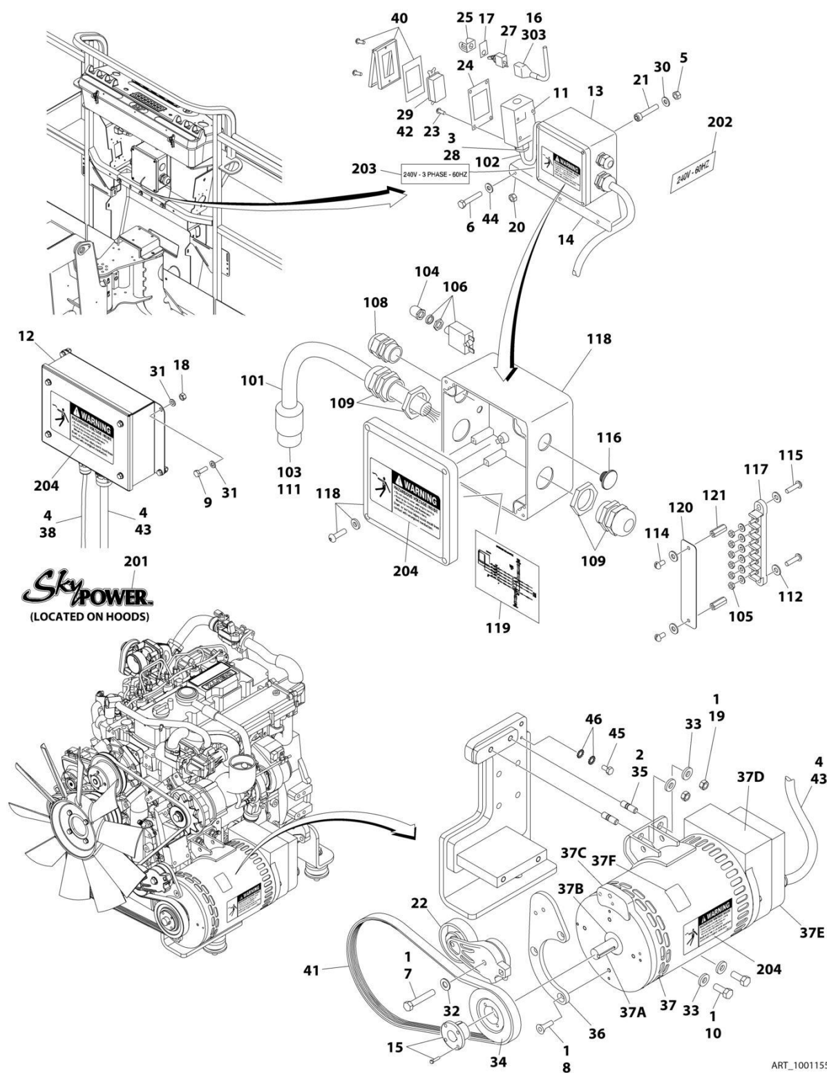
FIGURE 3-28. 7500W SKYPOWER GENERATOR INSTALLATION - 60HZ (OPTIONAL)
