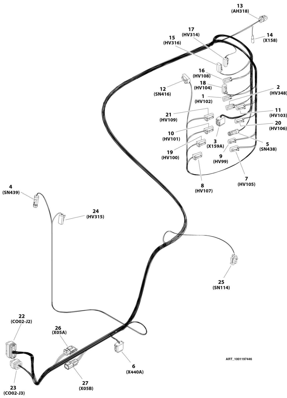
FIGURE 8-68. VALVE BANK HARNESS
