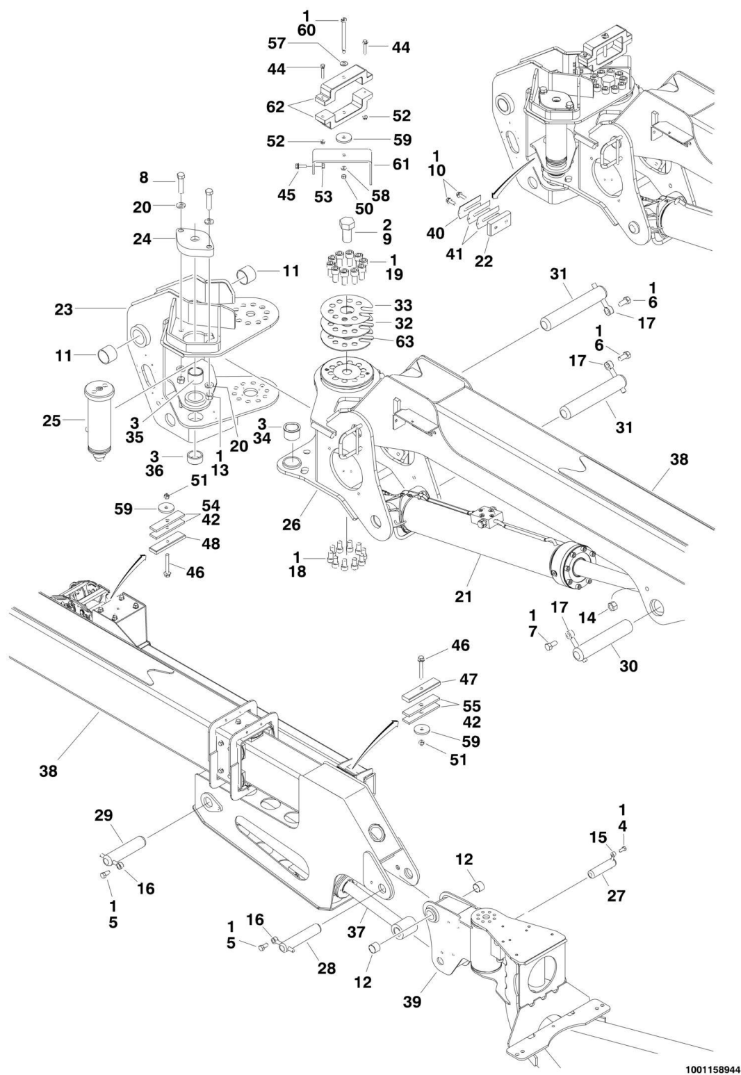
FIGURE 4-3. JIB INSTALLATION
