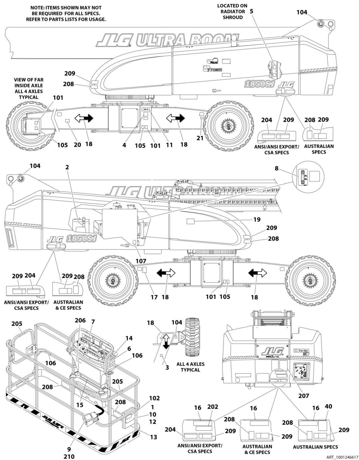
FIGURE 9-3. DECAL INSTALLATION - AUSTRALIAN SPECS
