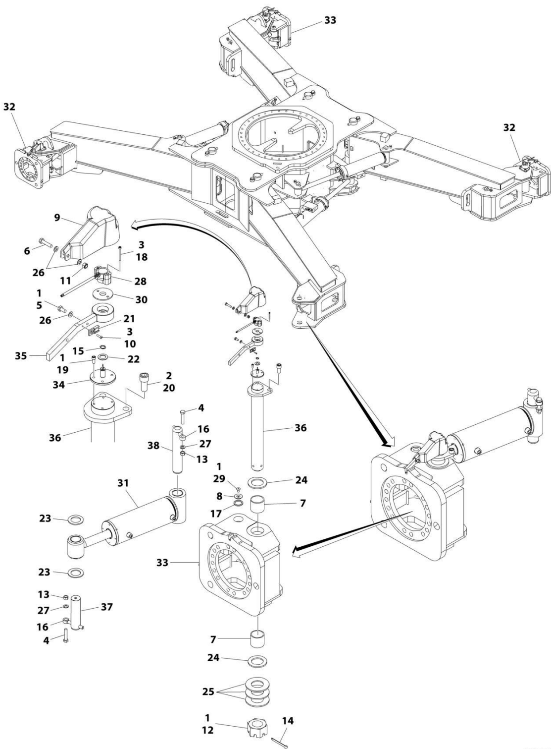
FIGURE 1-2. STEERING INSTALLATION
