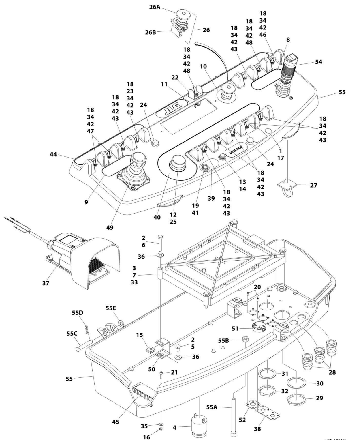
FIGURE 5-13. PLATFORM CONSOLE ASSEMBLY - WITH SKYGUARD
