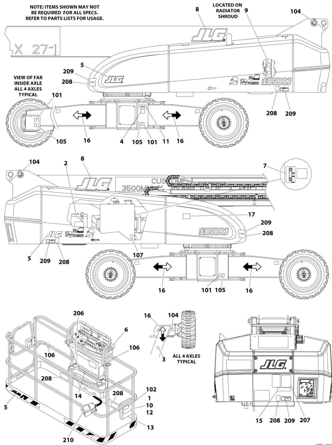
FIGURE 9-5. DECAL INSTALLATION - CE & UK CA SPECS
