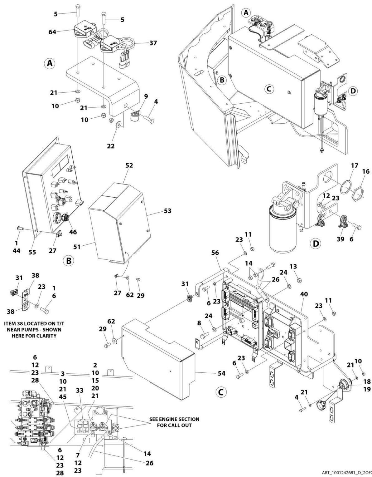
FIGURE 2-15. TURNTABLE ELECTRICAL COMPONENTS INSTALLATION (ANSI, ANSI EXPORT (HRC), CSA AND JAPANESE SPECS)
