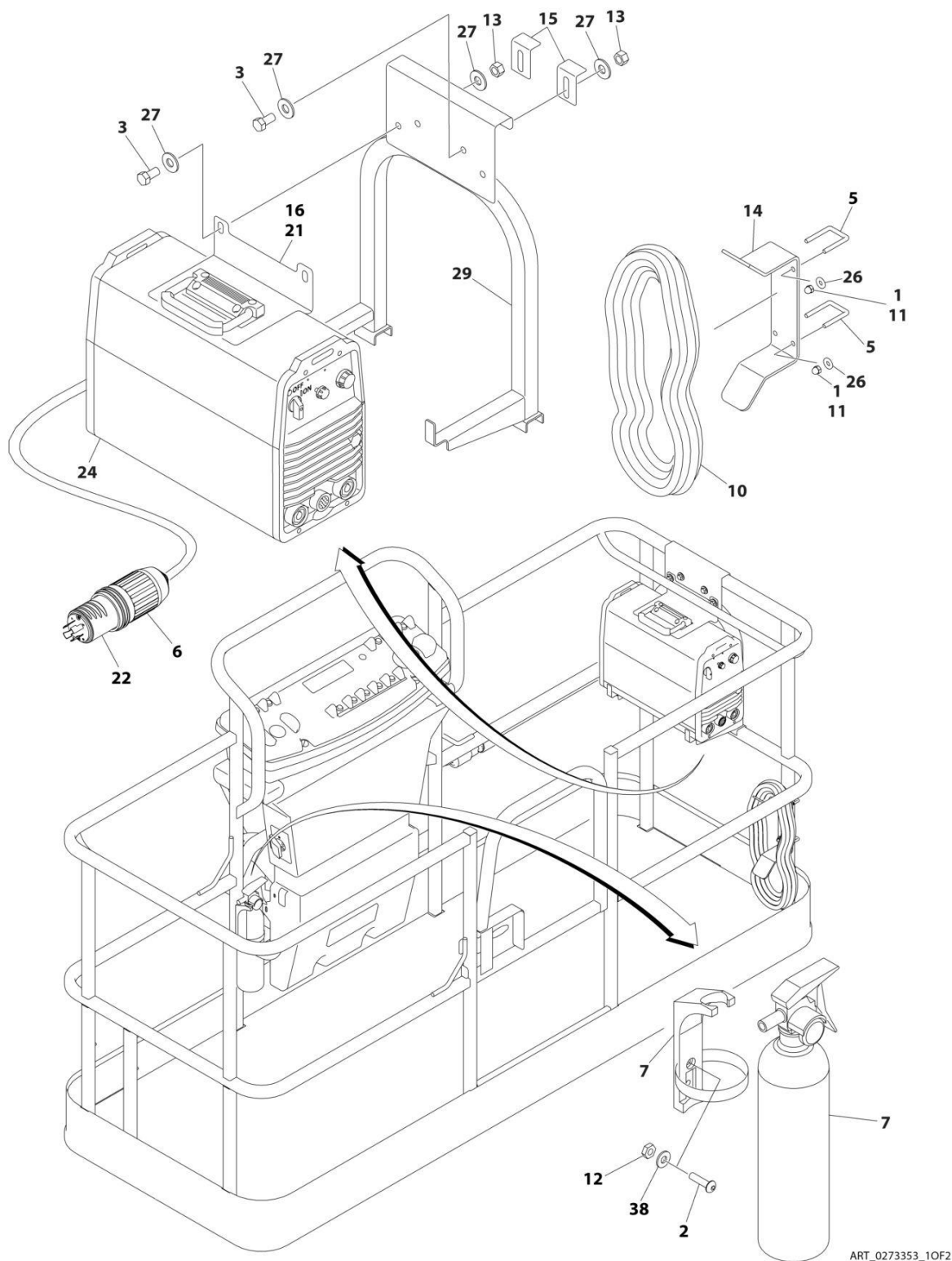
FIGURE 5-38. SKYWELDER/SKYCUTTER COMBO INSTALLATION (60HZ) (ANSI, ANSI EXPORT, CHINA, CSA & JAPANESE SPECS)
