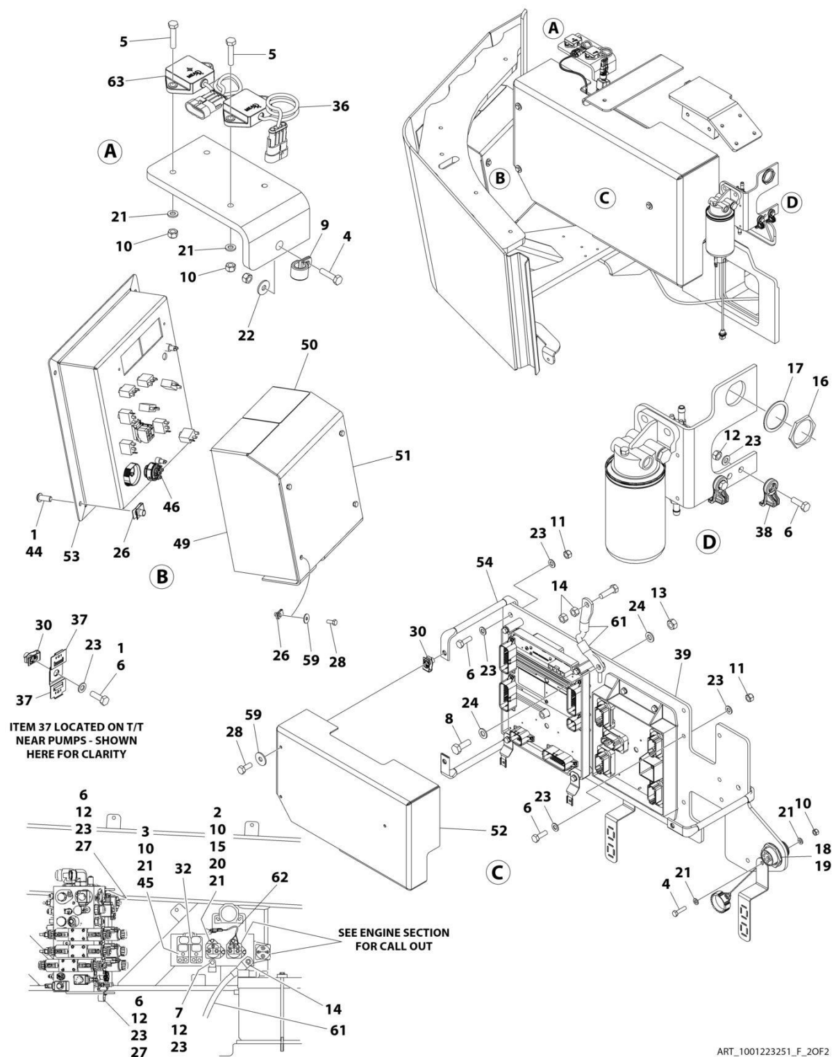
FIGURE 2-16. TURNTABLE ELECTRICAL COMPONENTS INSTALLATION (CE & UK CA (LRC) SPECS)
