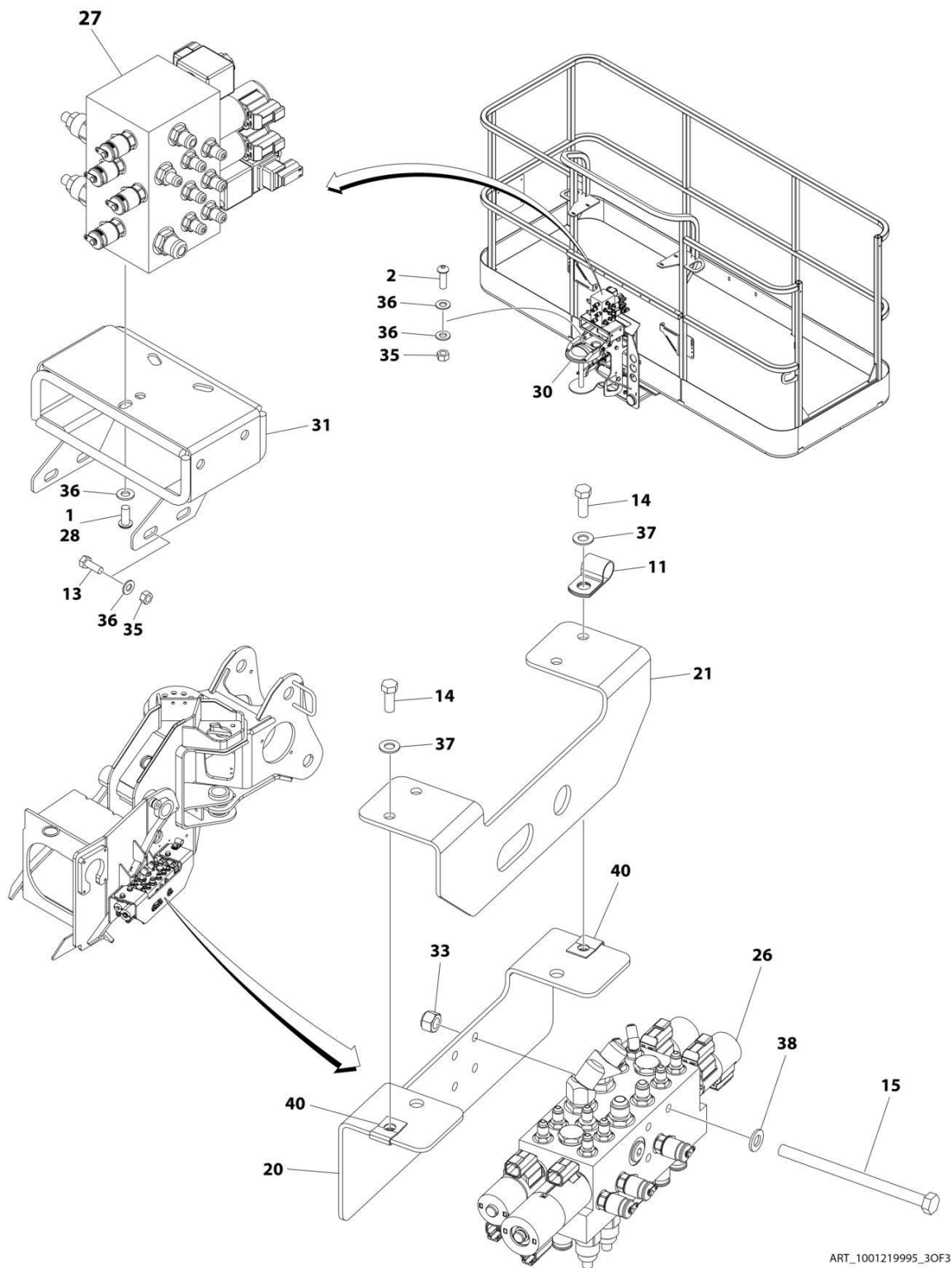
FIGURE 4-9. VALVES INSTALLATION - BOOM (WITH LSS)
