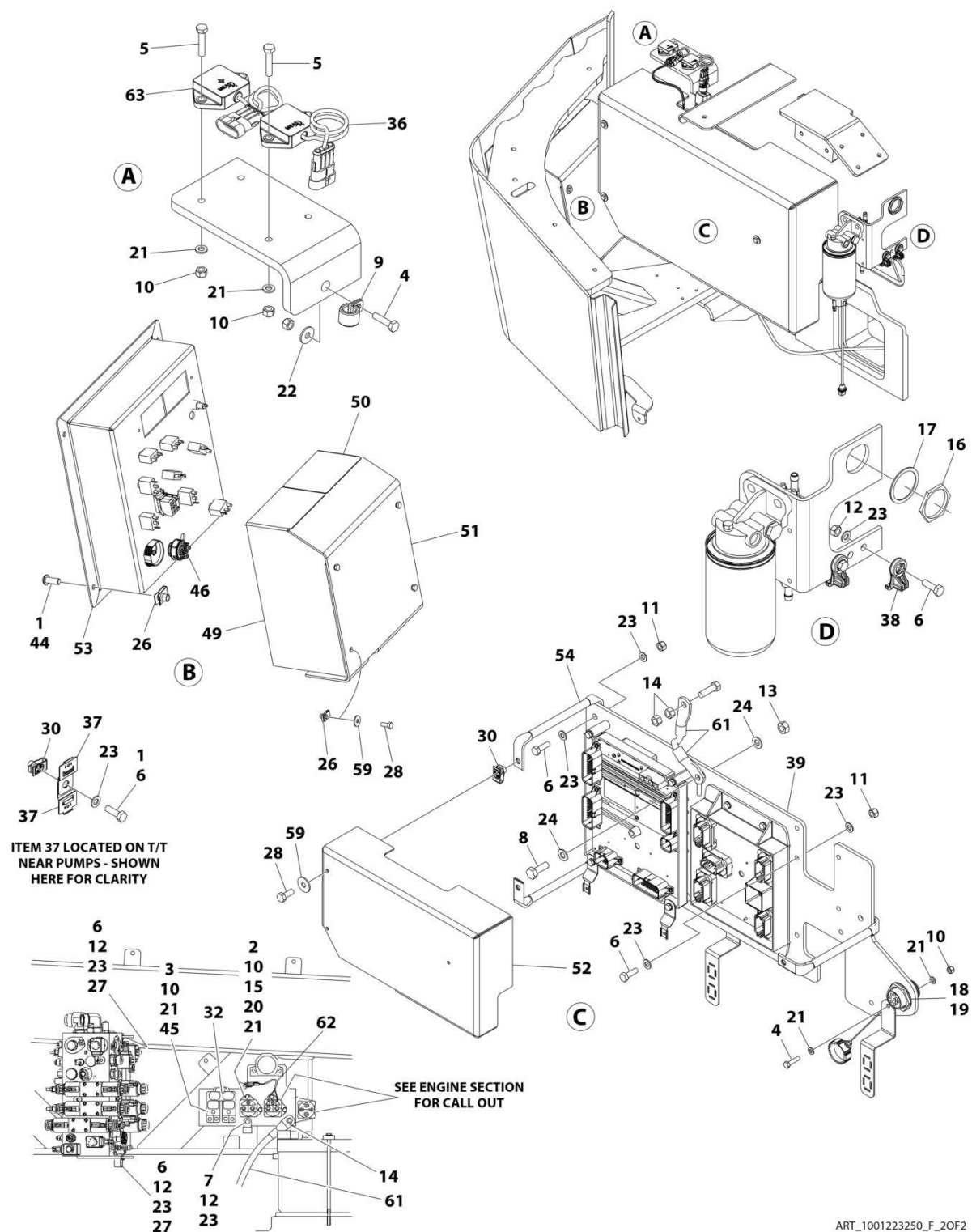
FIGURE 2-14. TURNTABLE ELECTRICAL COMPONENTS INSTALLATION (ANSI EXPORT (LRC), AUSTRALIAN AND CHINA SPECS)
