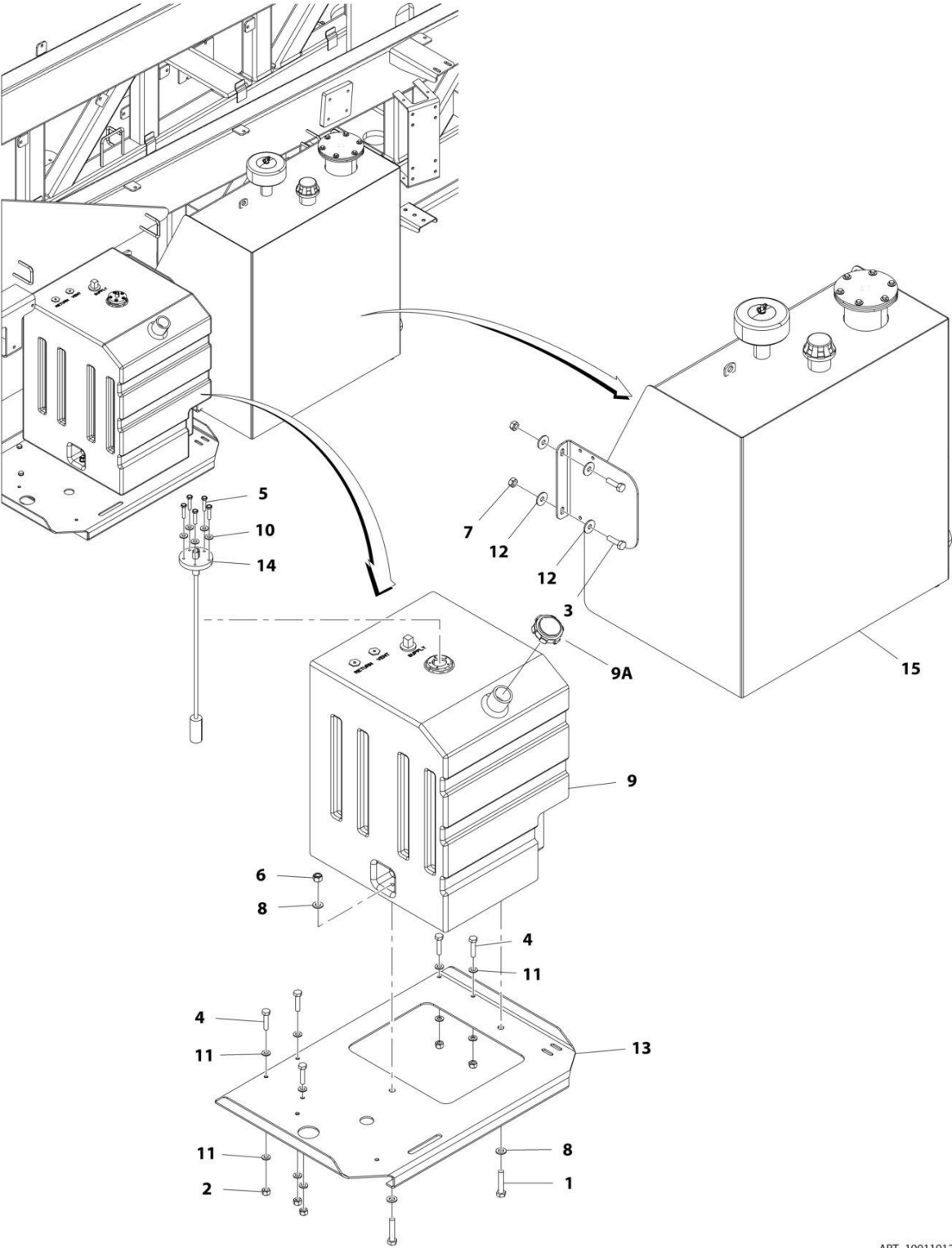
FIGURE 2-9. TANKS INSTALLATION
