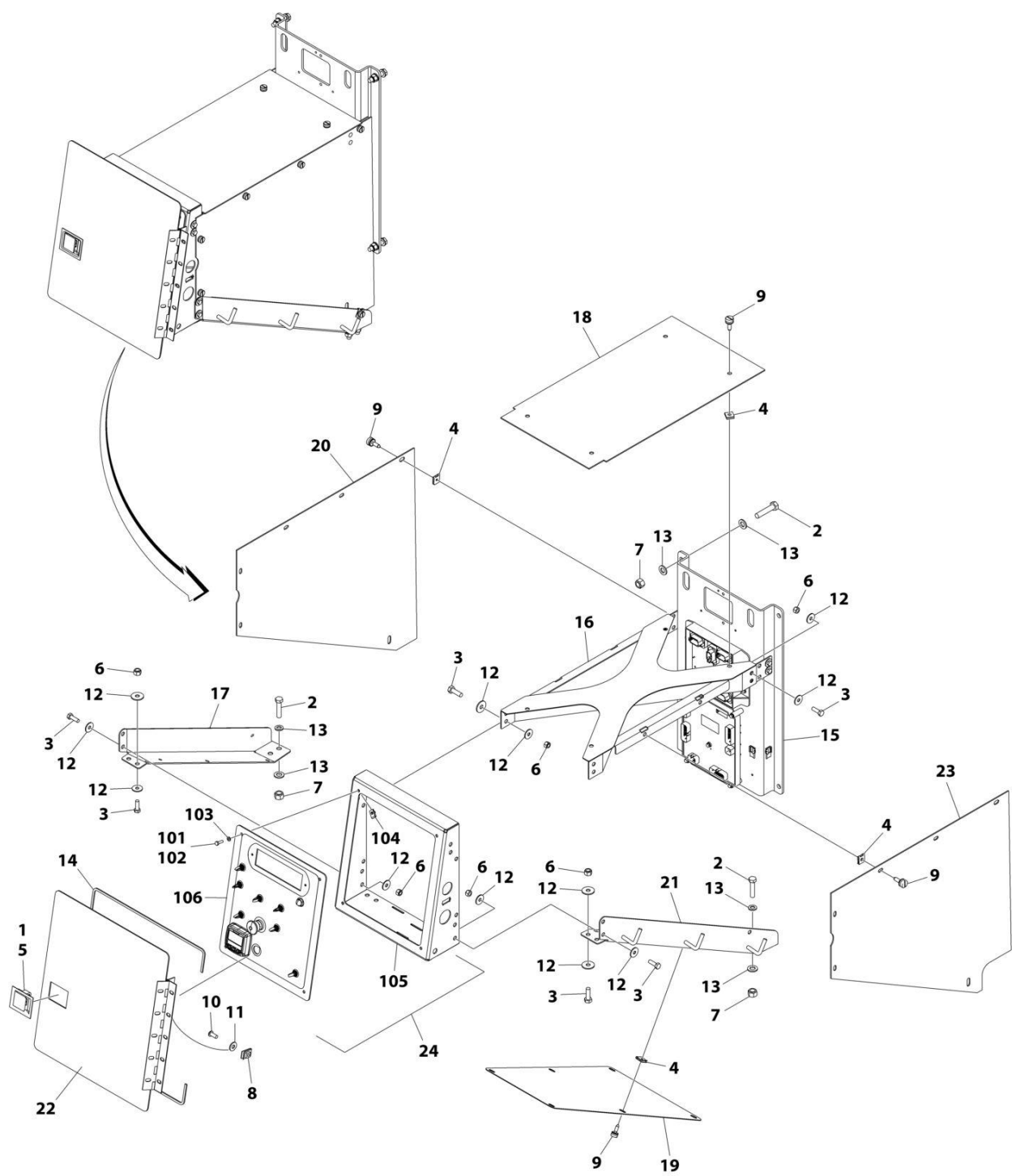
FIGURE 2-16. ELECTRICAL COMPONENTS INSTALLATION
