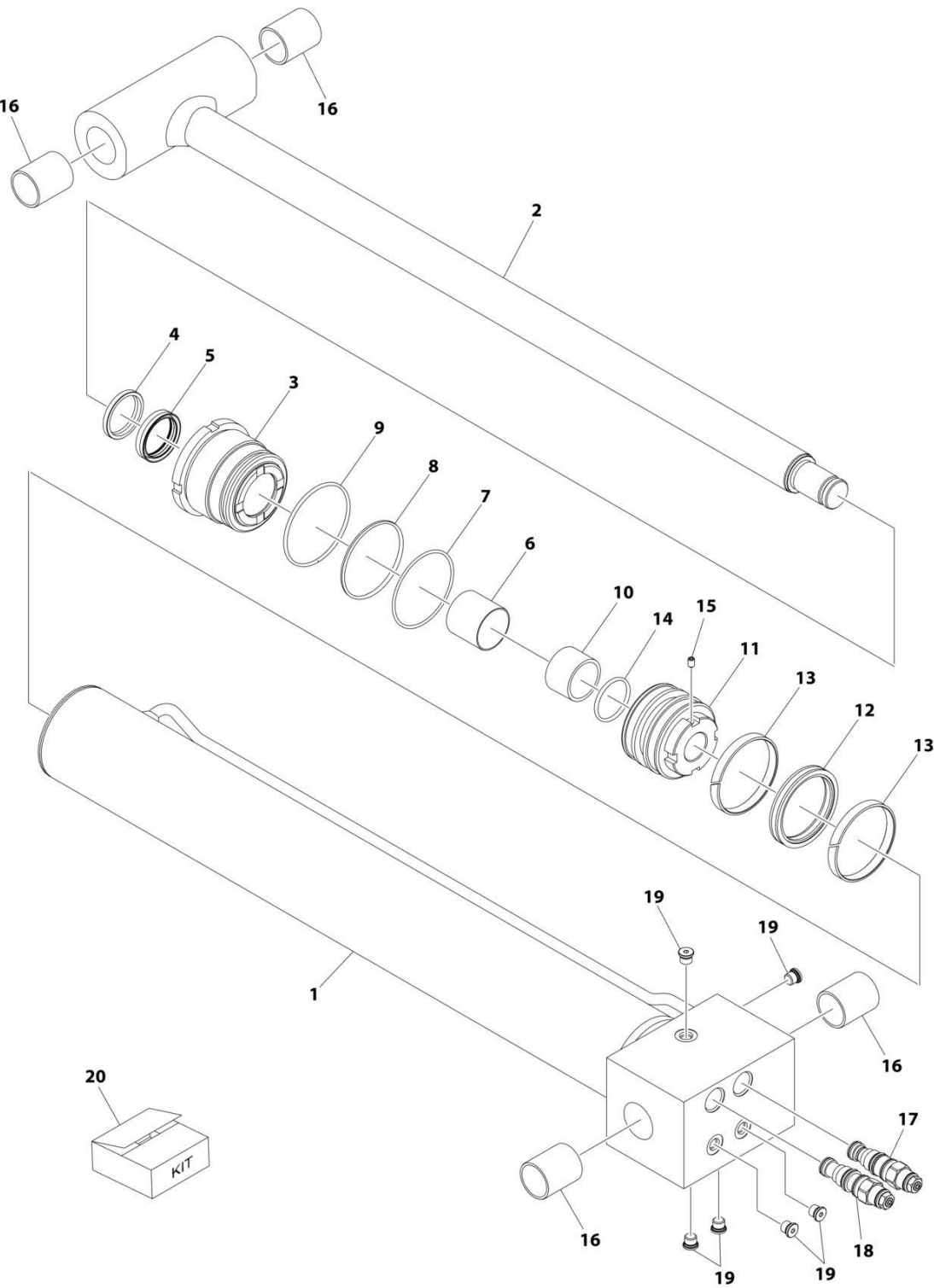
FIGURE 6-4. LIFT CYLINDER ASSEMBLY - JIB
