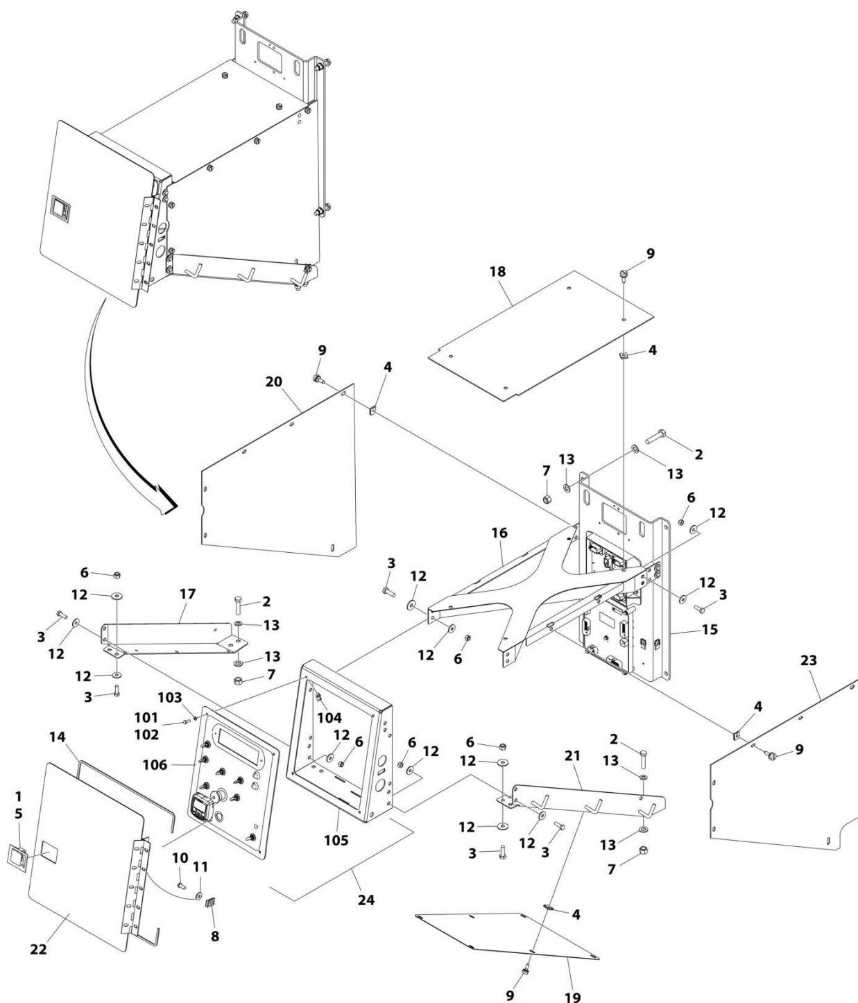
FIGURE 2-17. ELECTRICAL COMPONENTS INSTALLATION (CHINA IV SPECS)
