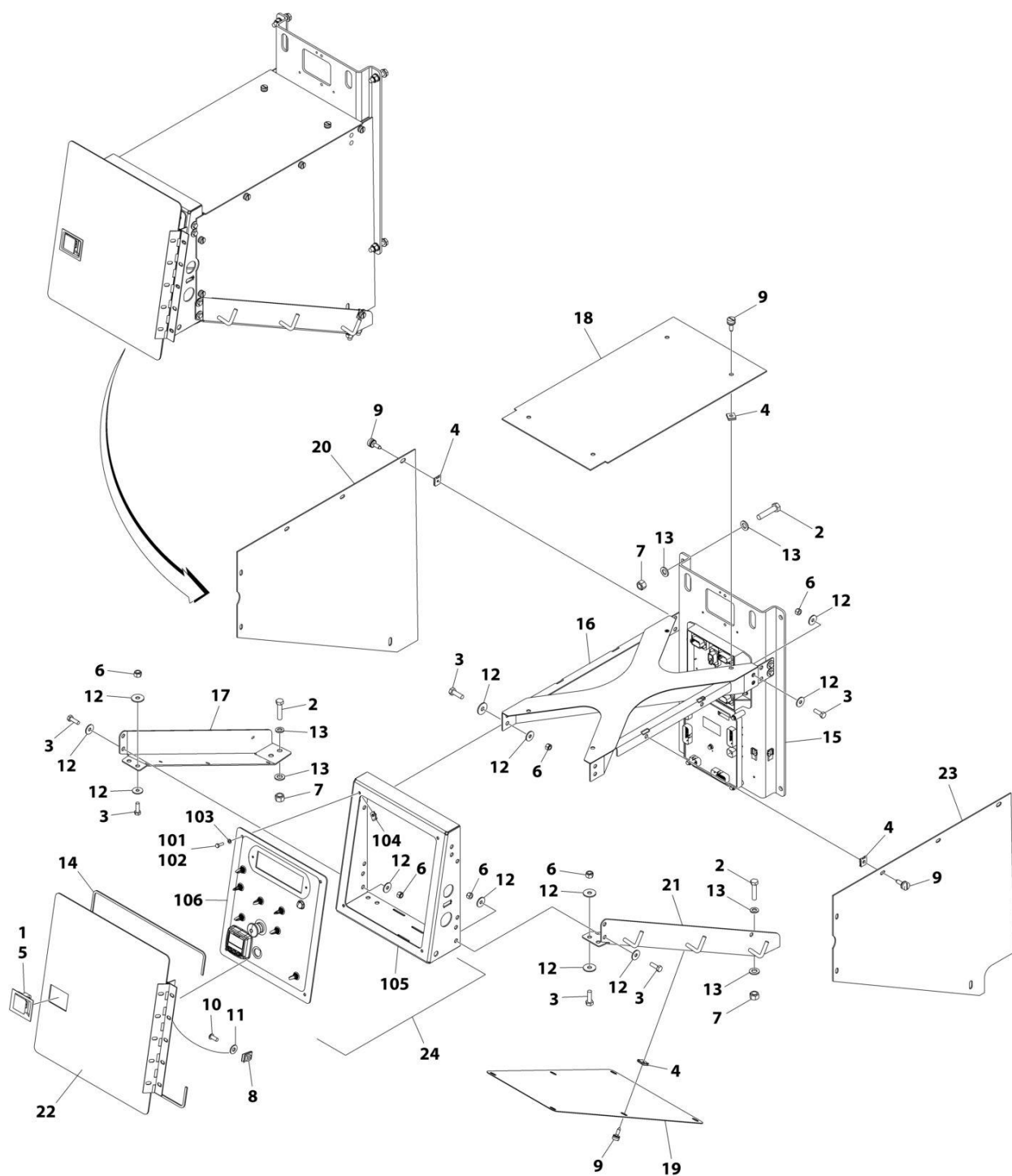
FIGURE 2-16. ELECTRICAL COMPONENTS INSTALLATION (ALL SPEC EXCEPT CHINA IV SPECS)
