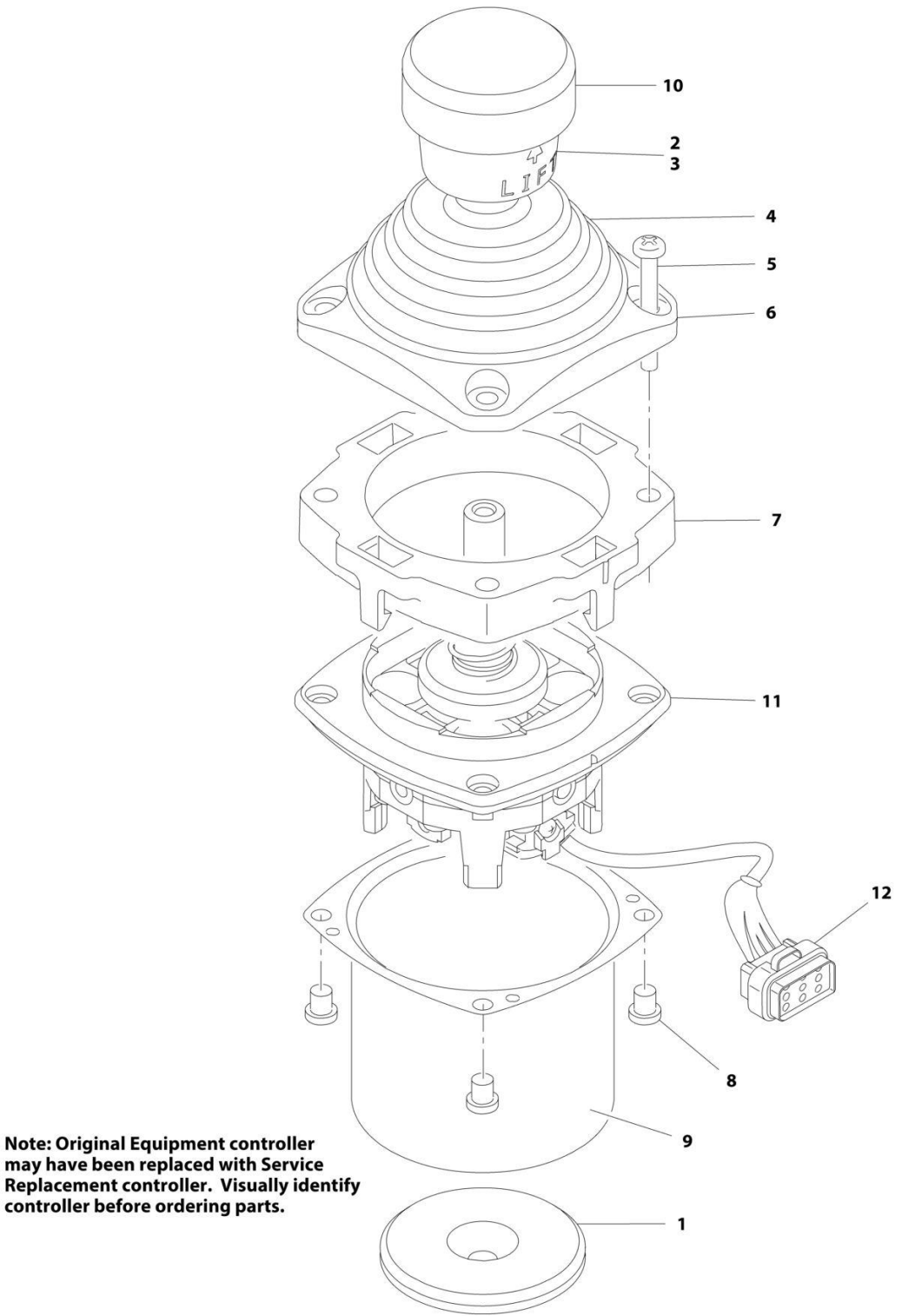
FIGURE 5-14. CONTROLLER ASSEMBLY (LIFT AND SWING)
