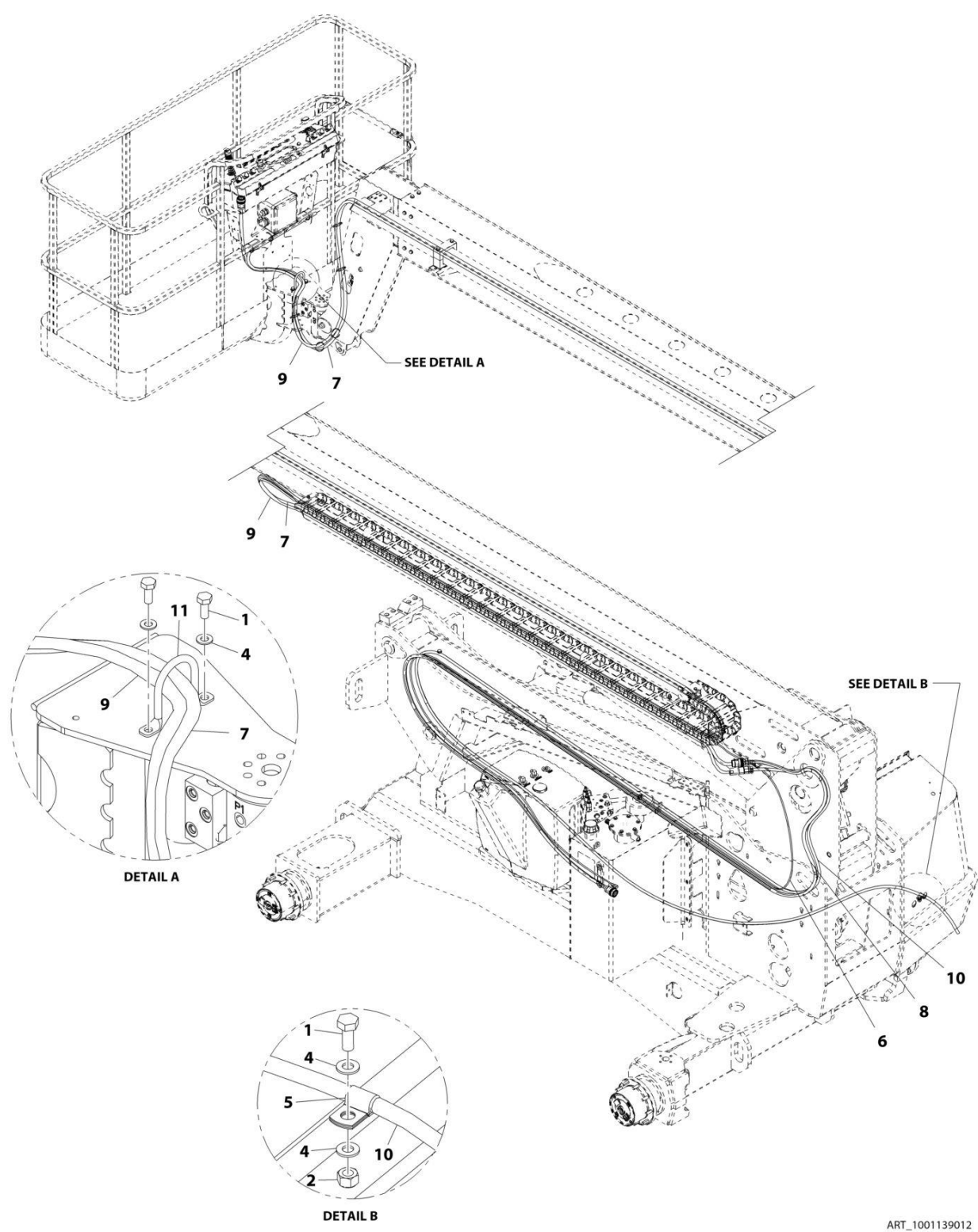
FIGURE 8-15. BOOM CABLES INSTALLATION WITHOUT SKYPOWER (24RS)
