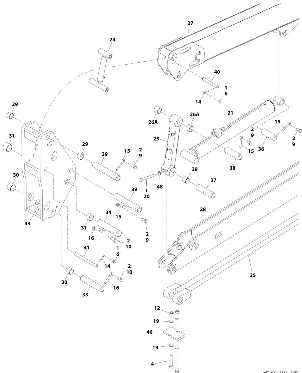
FIGURE 4-1. BOOM AND CYLINDERS INSTALLATION (24RS)
