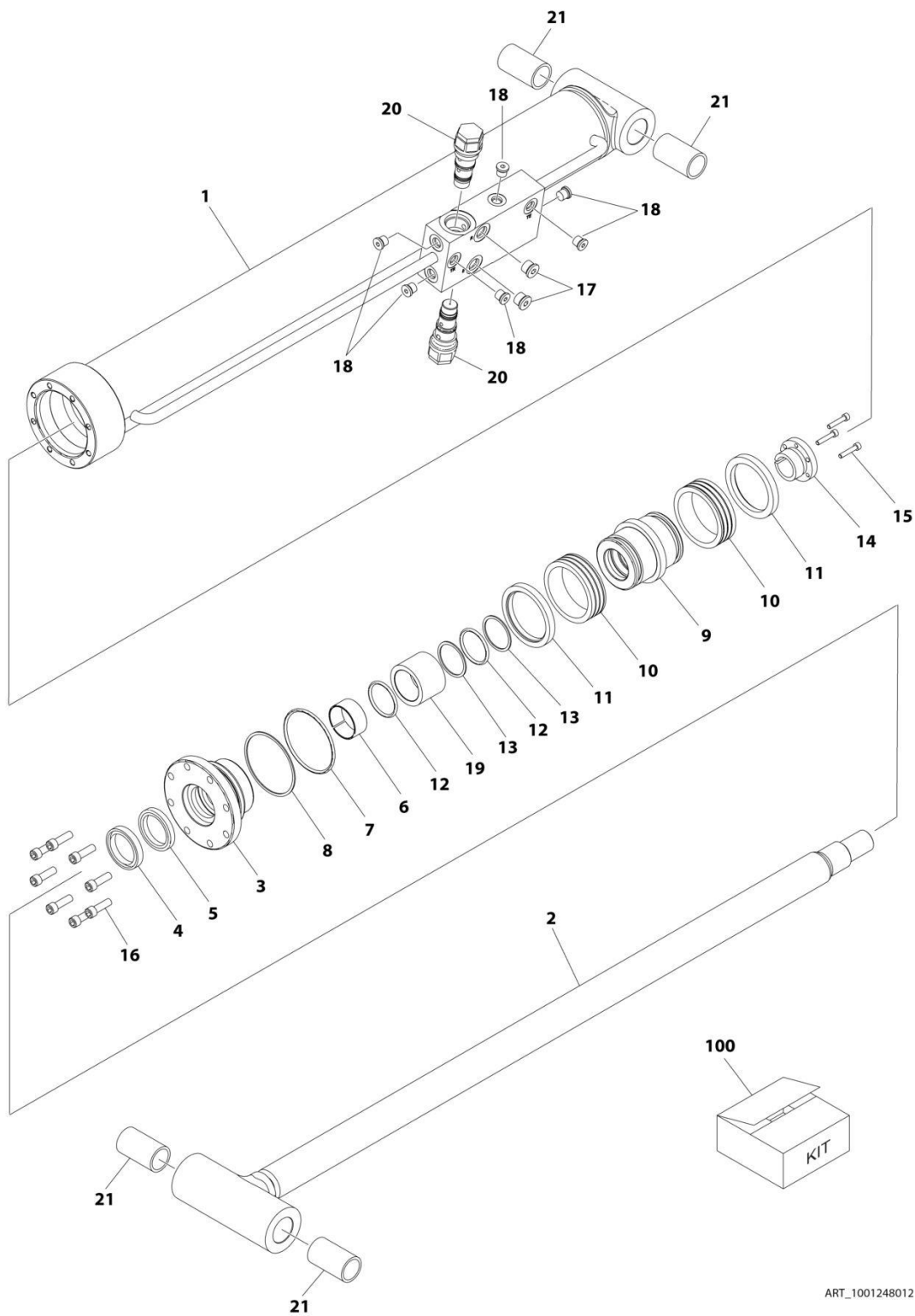
FIGURE 6-4. LIFT CYLINDER ASSEMBLY - JIB (SN B300002343 through B300002879)
