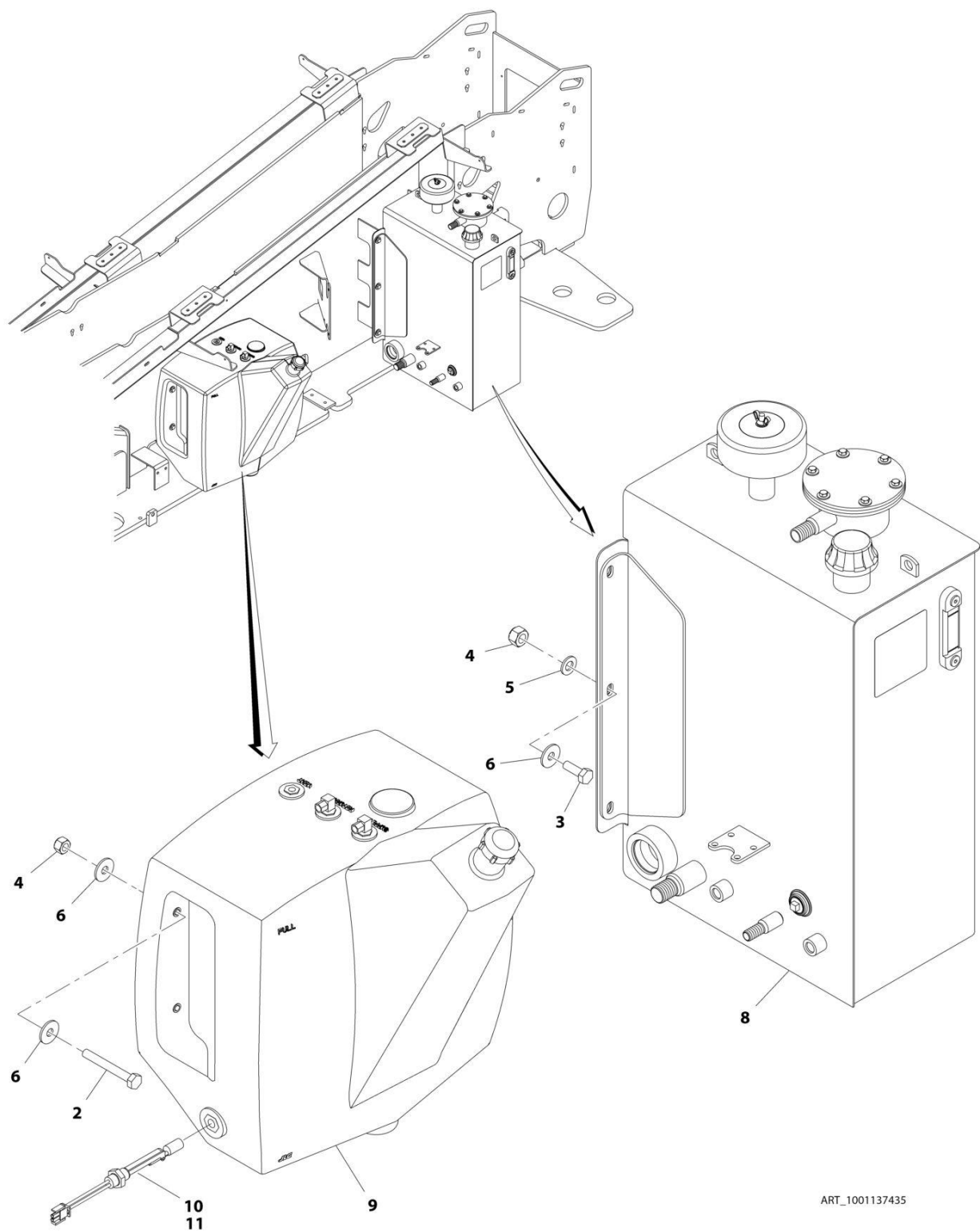
FIGURE 2-11. TANK INSTALLATIONS
