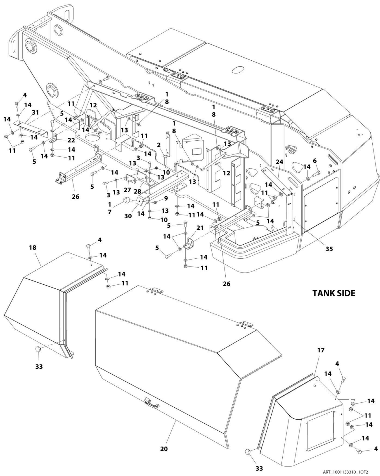
FIGURE 2-26. HOODS INSTALLATION
