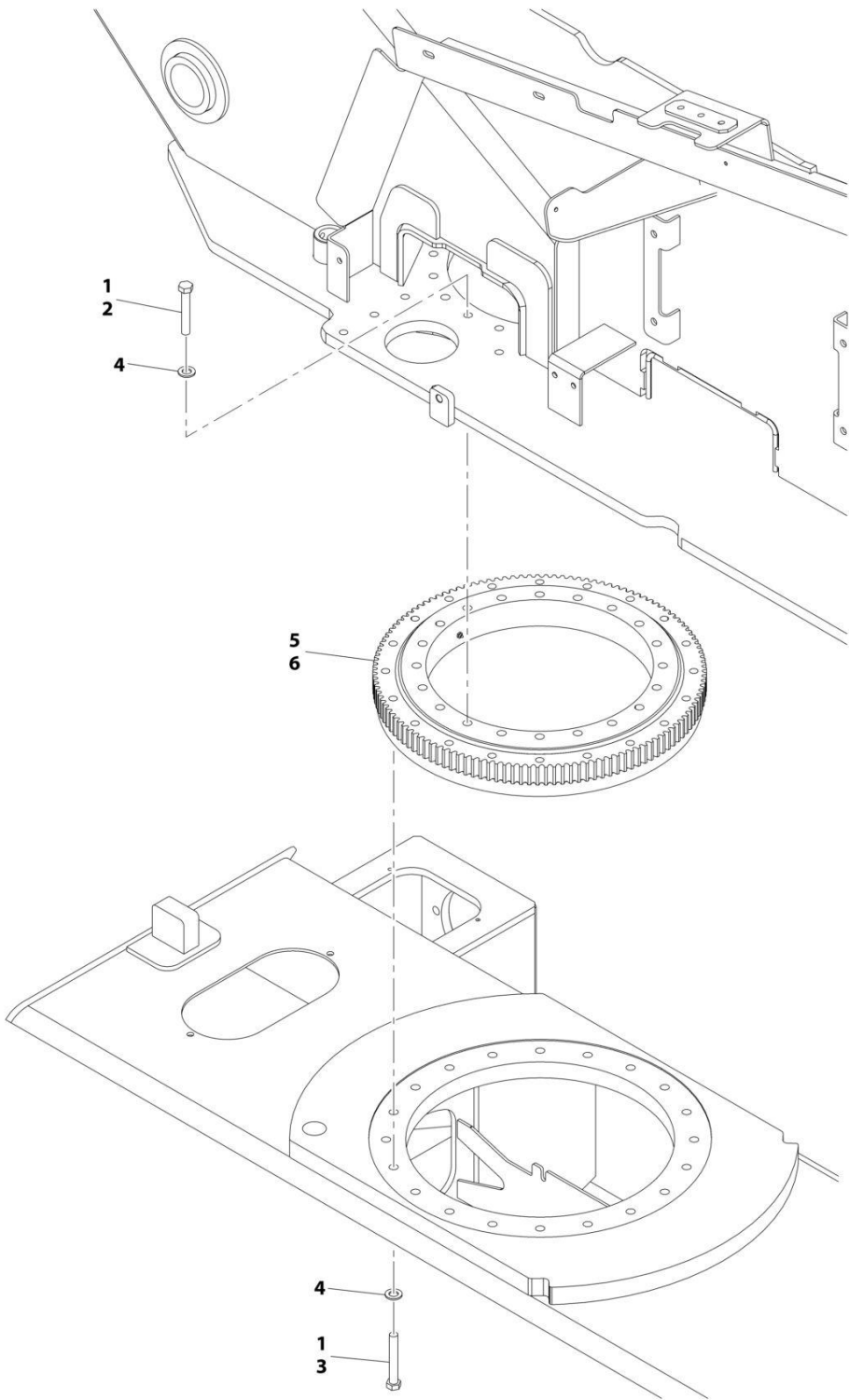
FIGURE 2-9. TURNTABLE BEARING INSTALLATION
