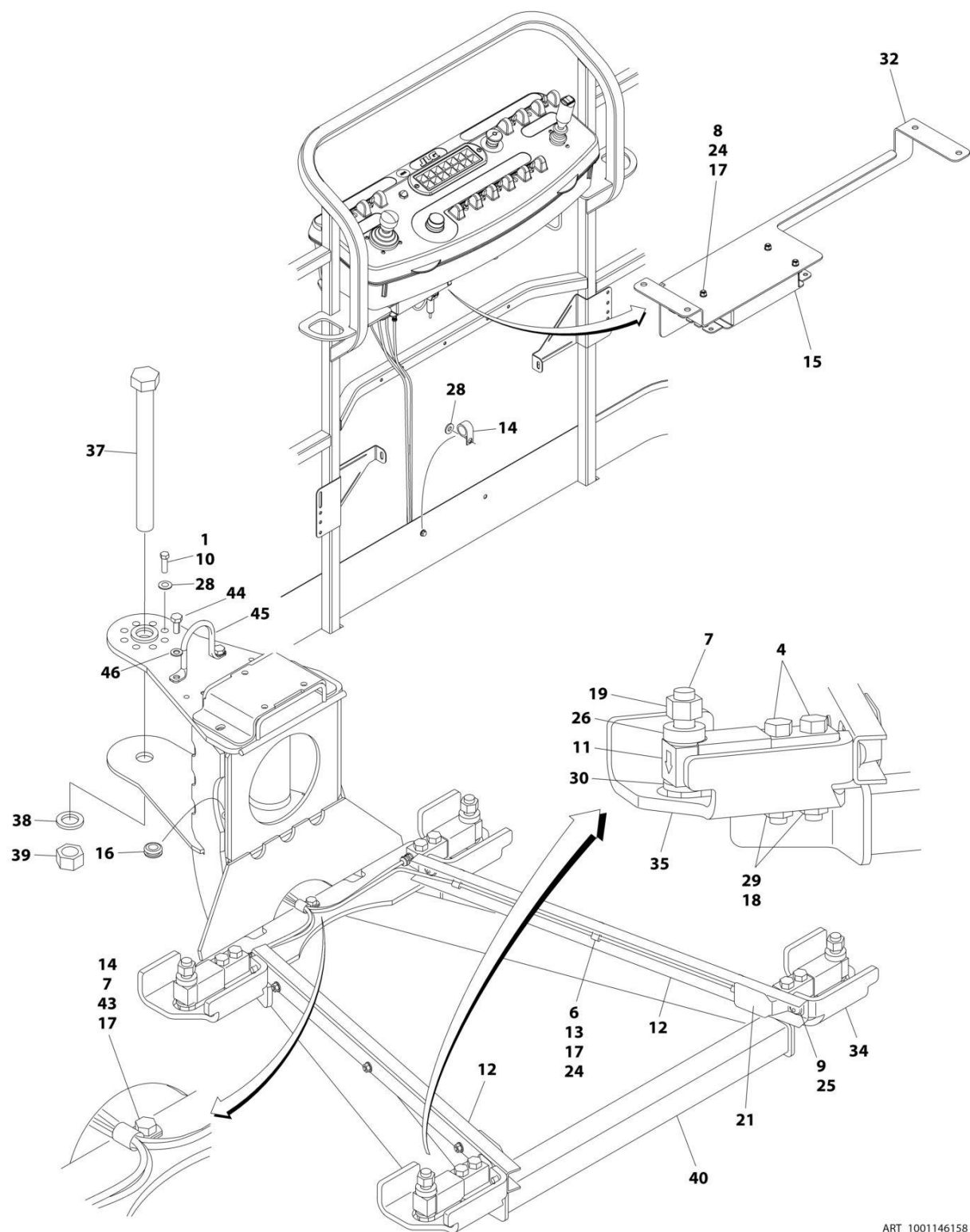
FIGURE 4-13. PLATFORM SUPPORT INSTALLATION - WITH LSS (24RS)
