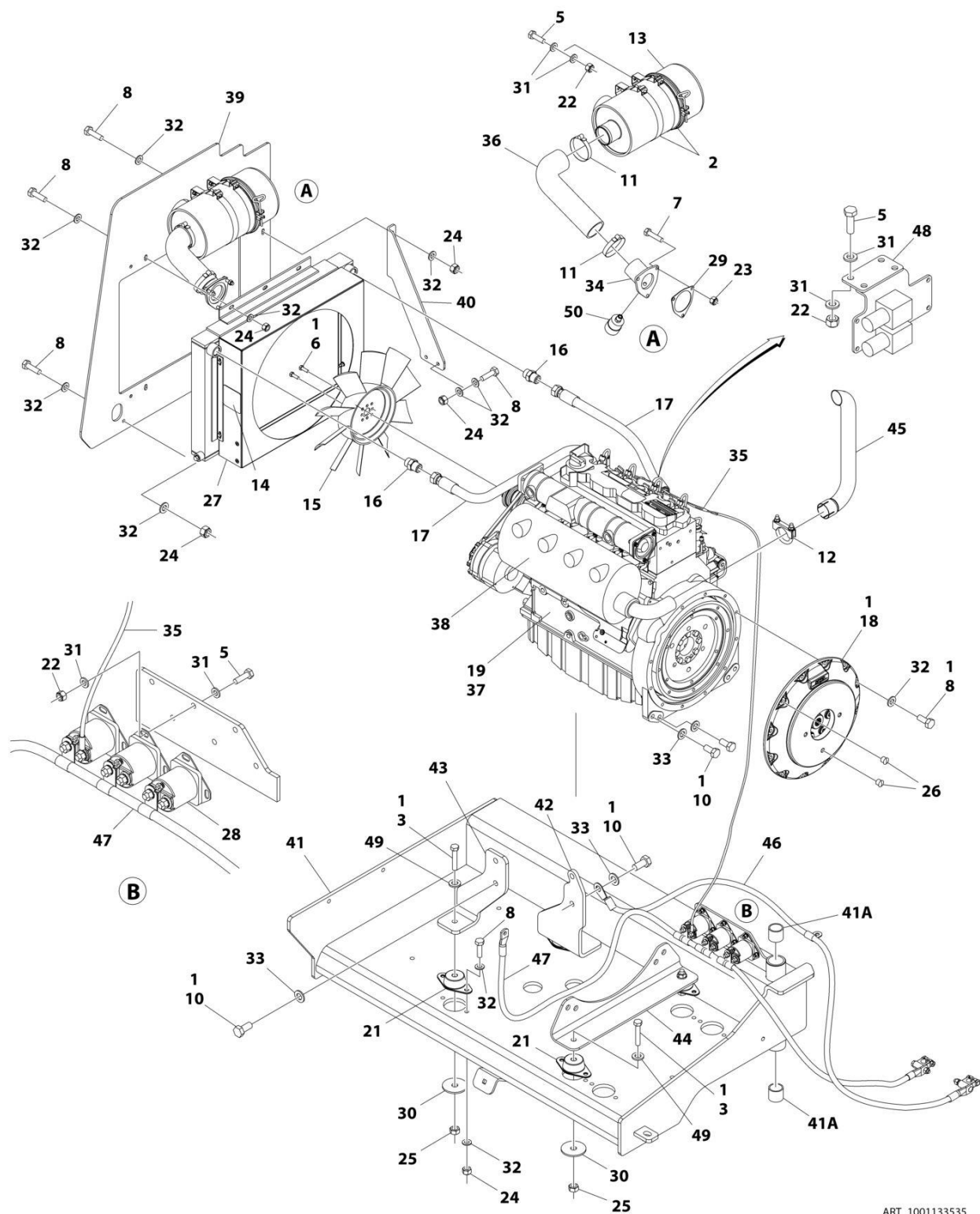
FIGURE 3-3. ENGINE ASSEMBLY
