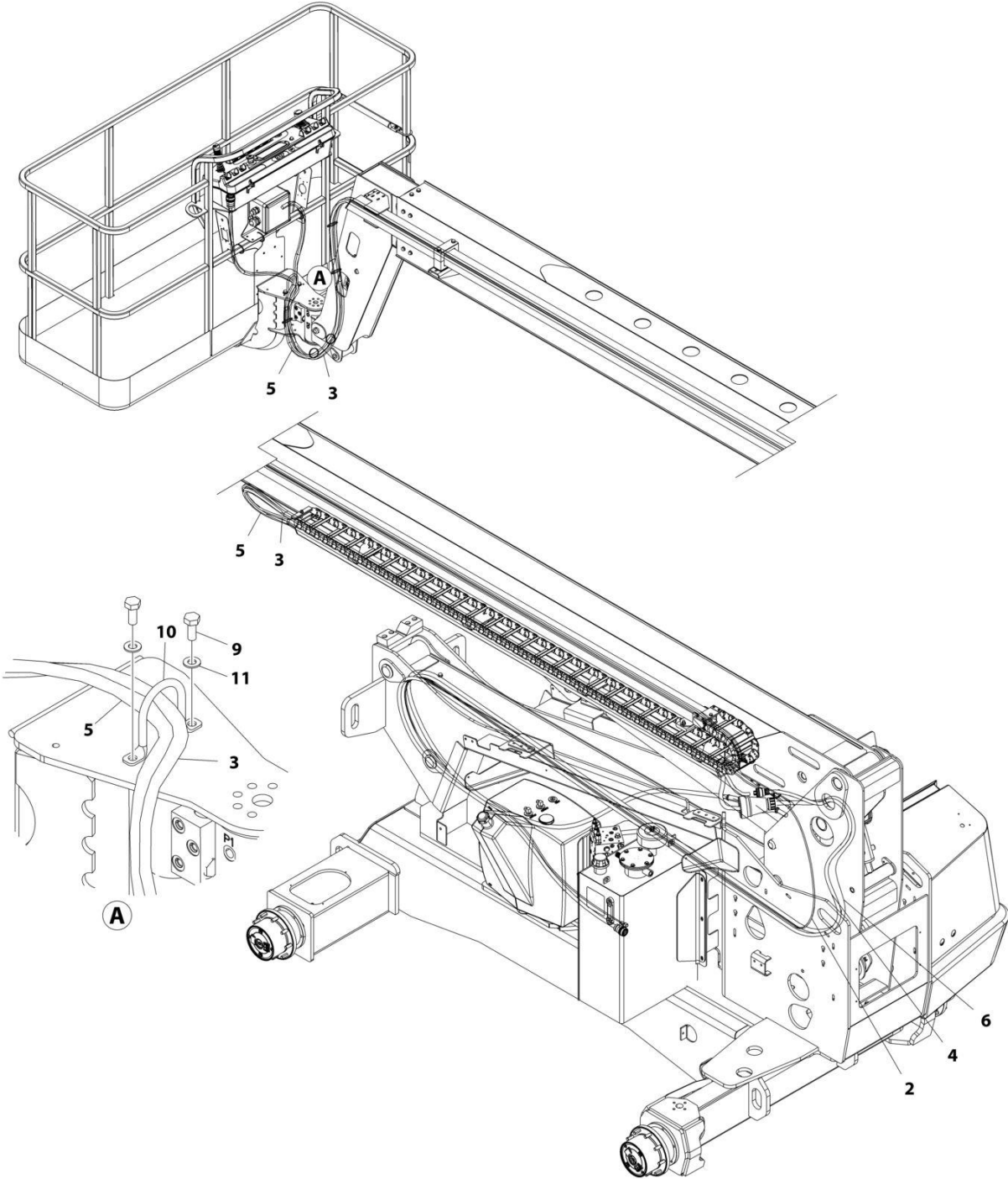
FIGURE 8-16. BOOM CABLES INSTALLATION WITH SKYPOWER (24RS)
