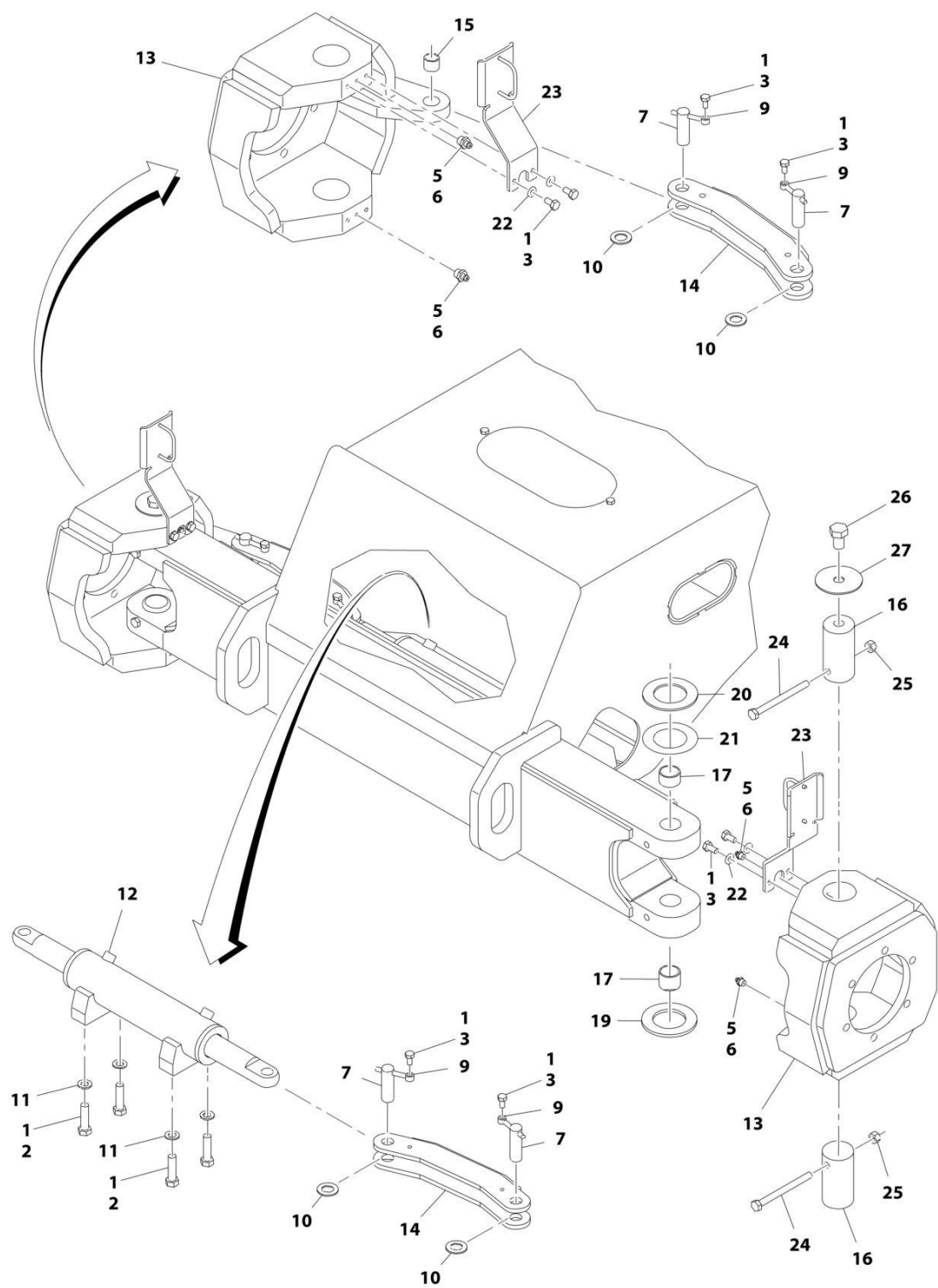
FIGURE 1-1. STEERING INSTALLATION
