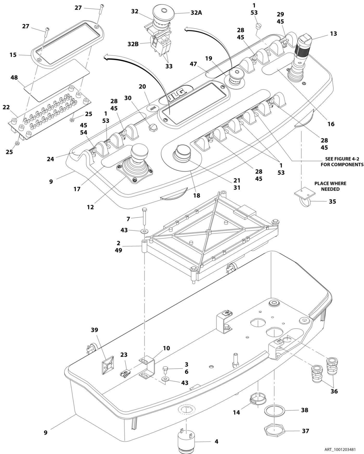
FIGURE 5-9. PLATFORM CONSOLE ASSEMBLY (24RSJ)
