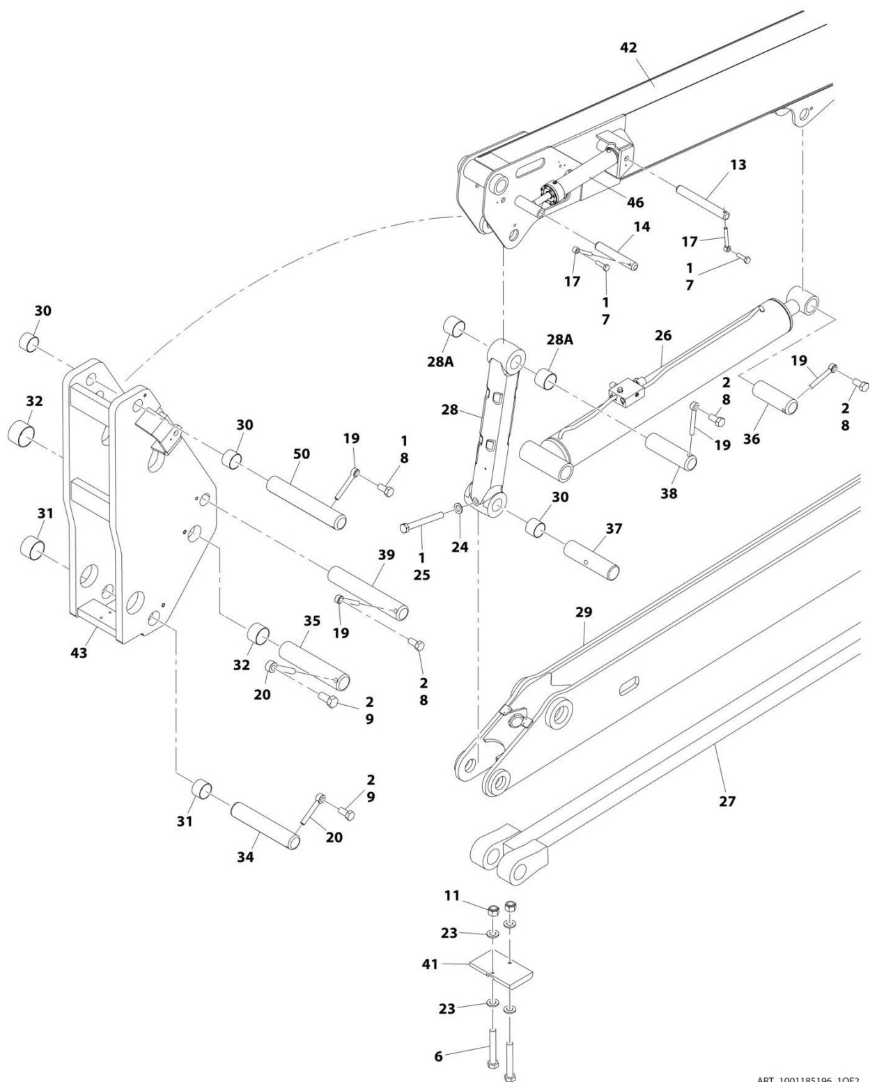
FIGURE 4-2. BOOM AND CYLINDERS INSTALLATION (24RSJ)
