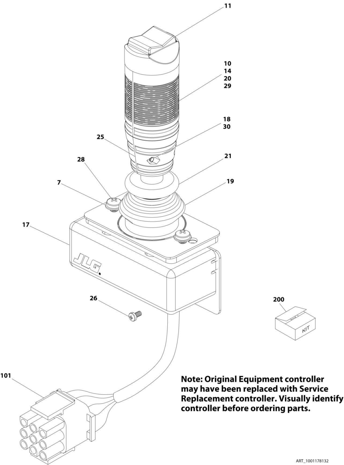
FIGURE 4-11. CONTROLLER ASSEMBLY (DRIVE AND STEER) (SN 0300194271 through 0300219271)
