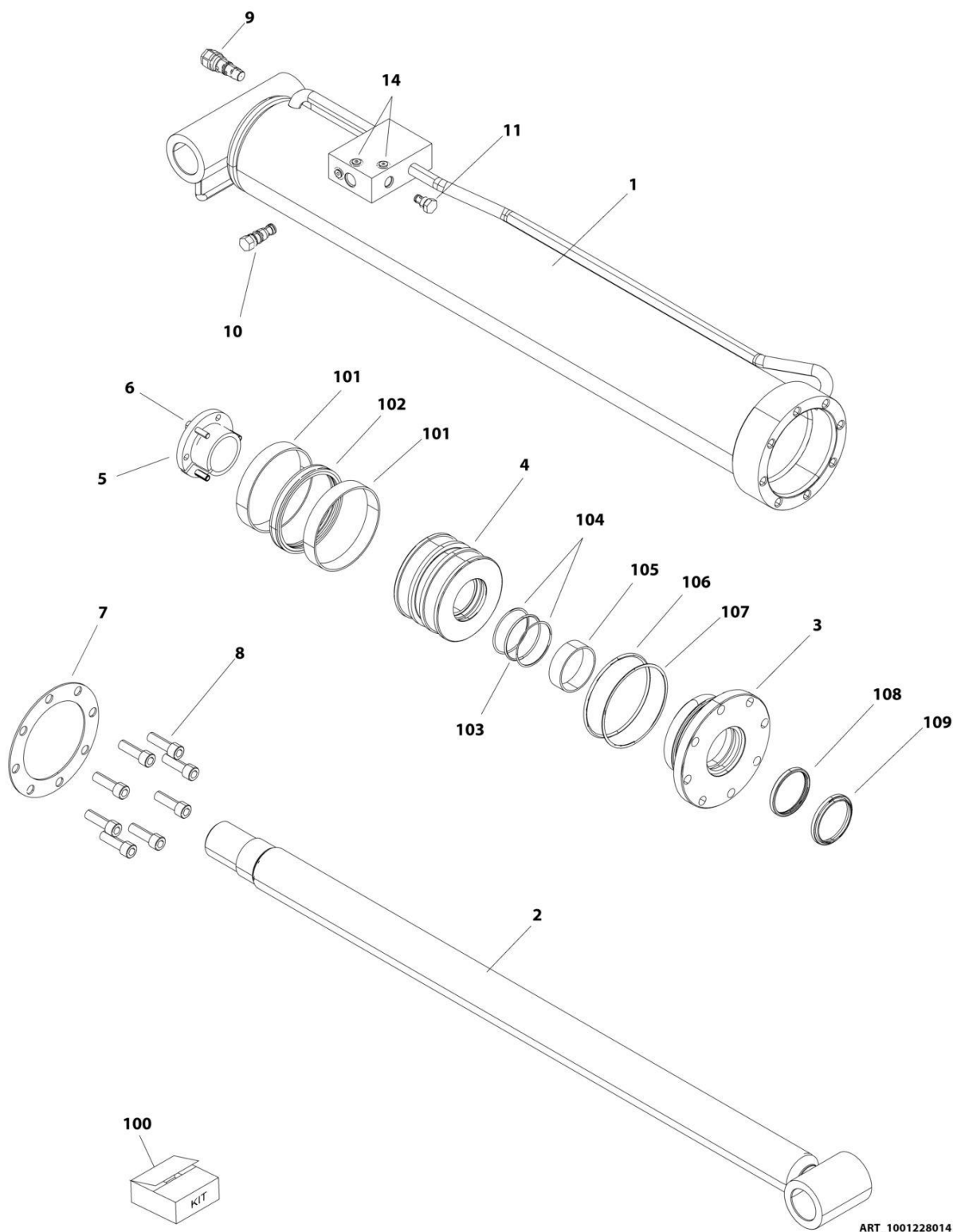
FIGURE 6-6. LIFT CYLINDER ASSEMBLY - MAIN (SN 0300239696 through 0300270877)
