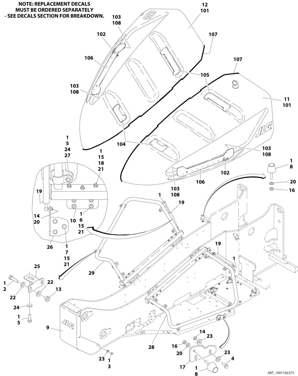
FIGURE 2-43. HOODS INSTALLATION
