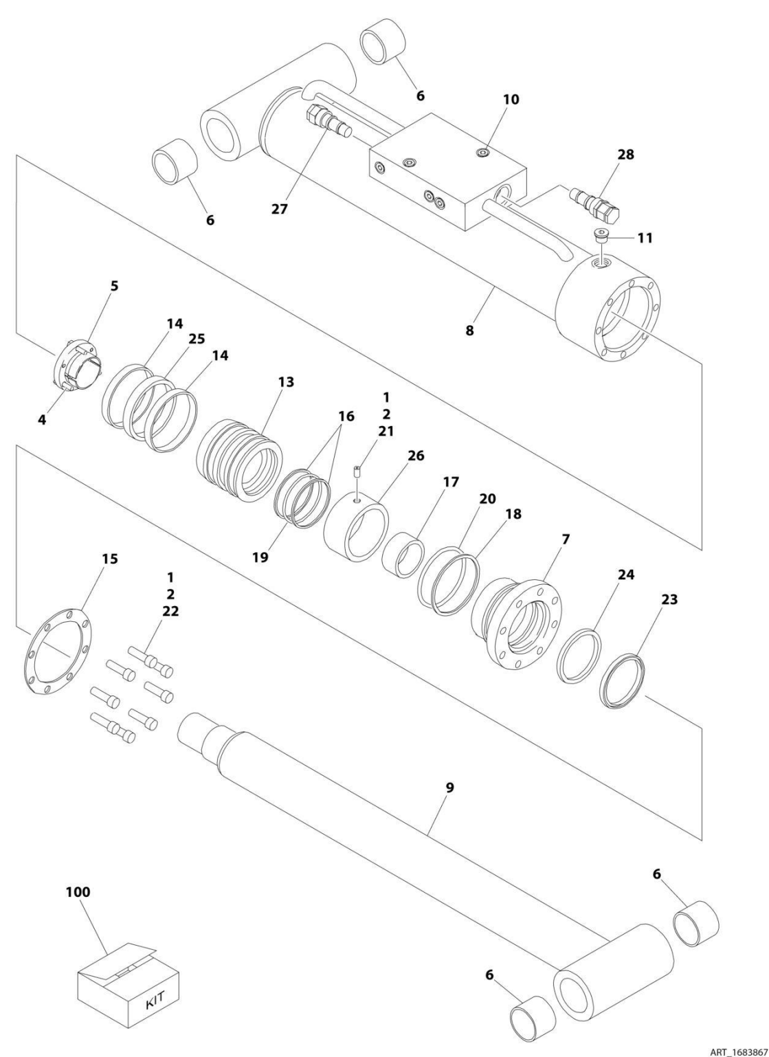
FIGURE 6-2. LEVEL (PLATFORM SLAVE) CYLINDER ASSEMBLY (E600/M600)
