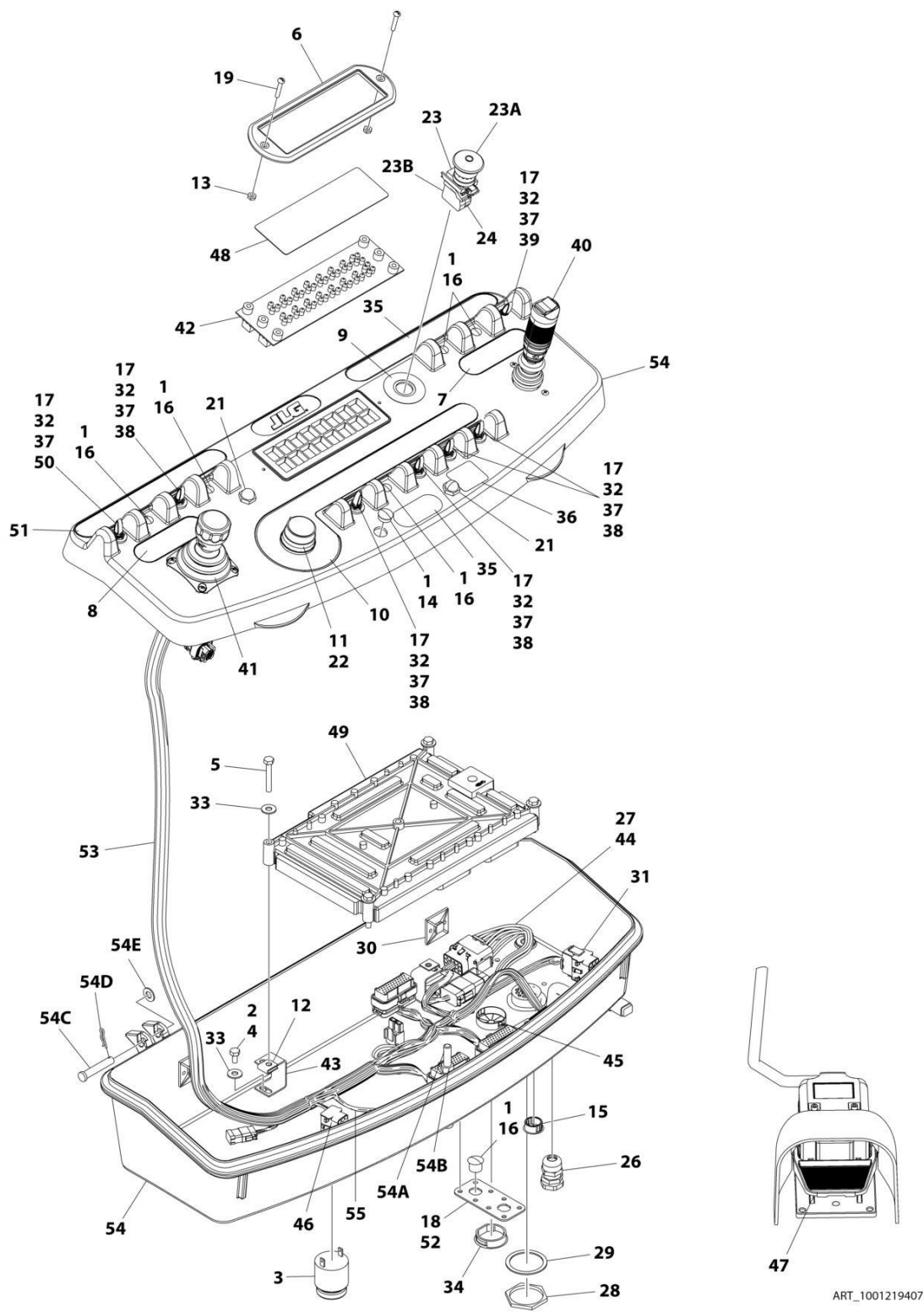
FIGURE 5-46. 4WD PLATFORM CONSOLE BOX ASSEMBLY - WITH 1 CELL LSS - WITH SKYGUARD (NON UL SPECS) (E600J/E600JP/M600J/M600JP) (SN 0300219271 through 0300256397)
