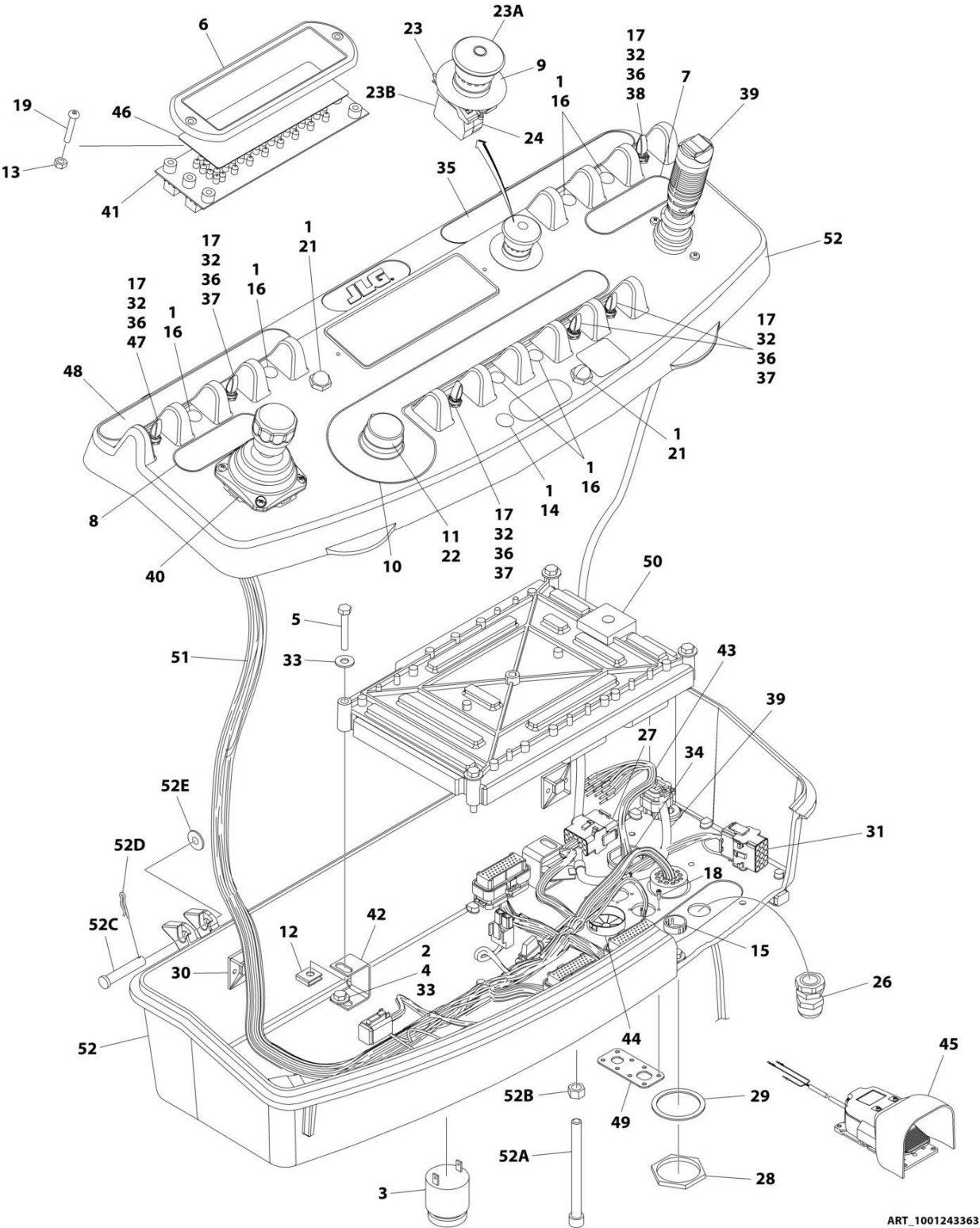
FIGURE 5-37. 4WD PLATFORM CONSOLE BOX ASSEMBLY - WITHOUT LSS OR WITH 1 CELL LSS (UL SPECS) (E600J/E600JP) (SN 0300256398 to Present)
