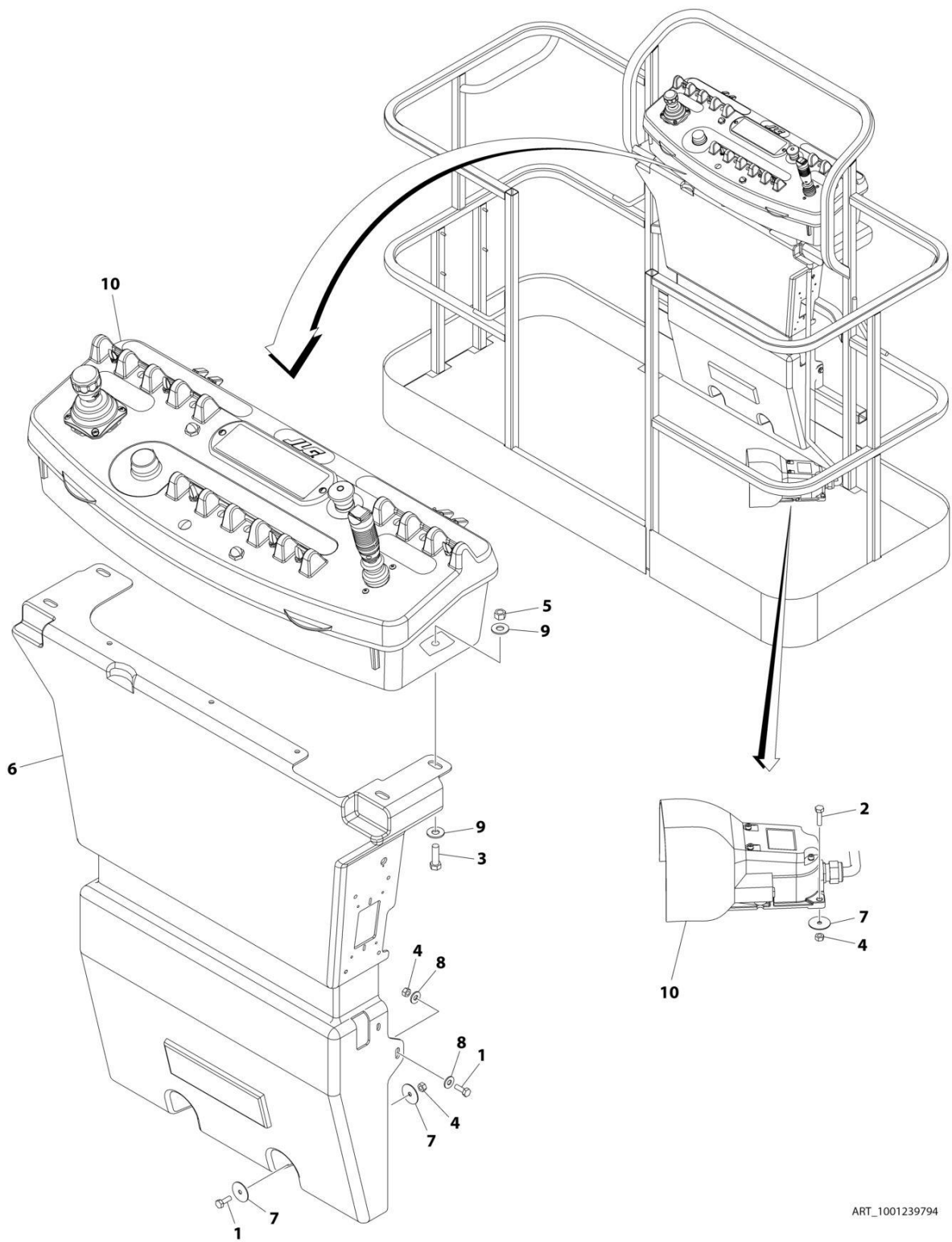
FIGURE 5-26. 2WD PLATFORM CONSOLE BOX INSTALLATION - WITH 1 CELL LSS - WITH SKYGUARD (NON UL SPECS) (E600J/E600JP/M600J/M600JP) (SN 0300256398 to Present)
