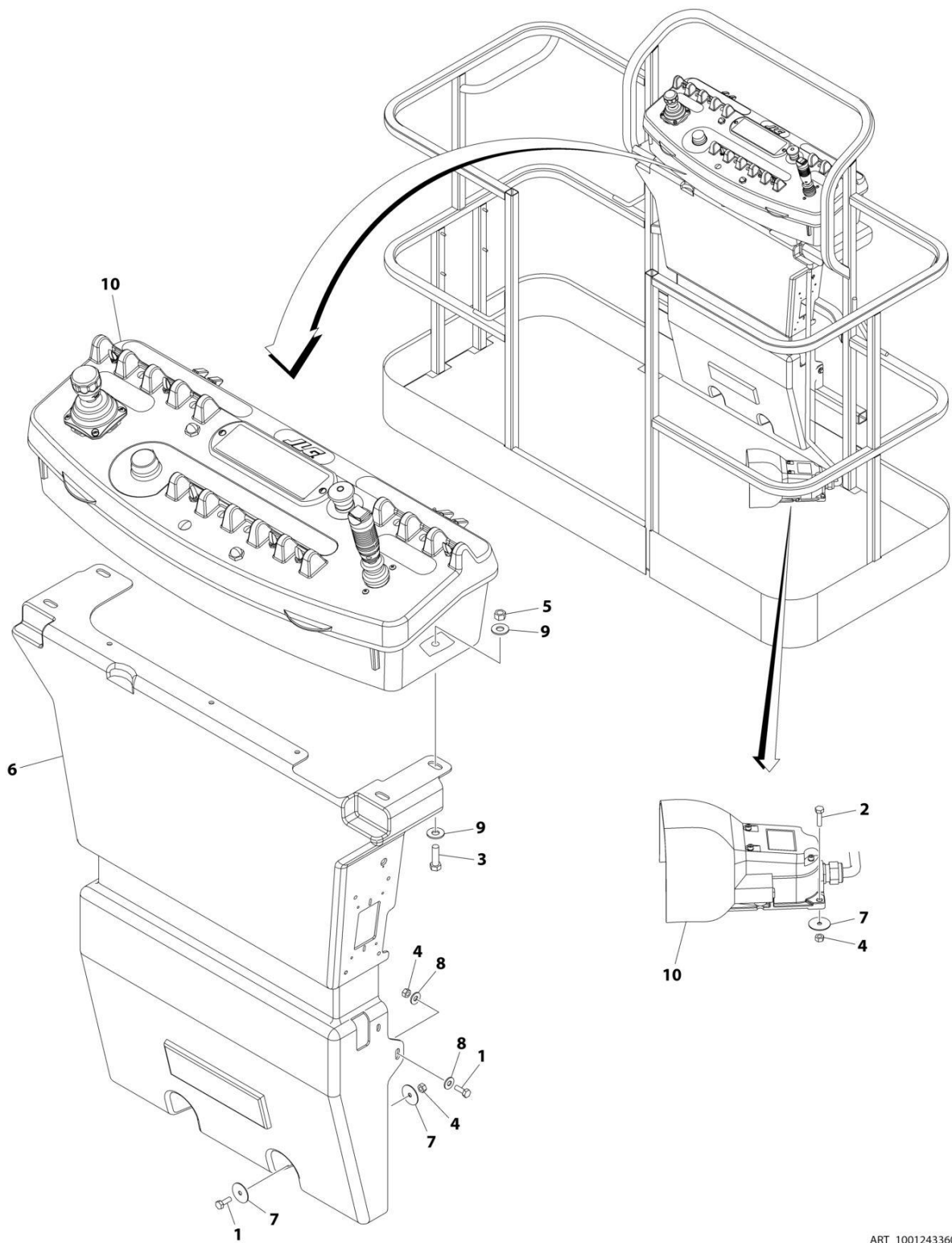
FIGURE 5-29. 4WD PLATFORM CONSOLE BOX INSTALLATION - WITH 1 CELL LSS - WITH SKYGUARD (NON UL SPECS) (E600J/E600JP/M600J/M600JP) (SN 0300256398 to Present)
