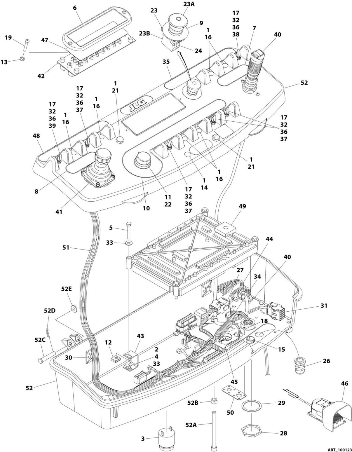
FIGURE 5-33. 2WD PLATFORM CONSOLE BOX ASSEMBLY - WITHOUT LSS OR WITH 1 CELL LSS (UL SPECS) (E600J/E600JP) (SN 0300256398 to Present)
