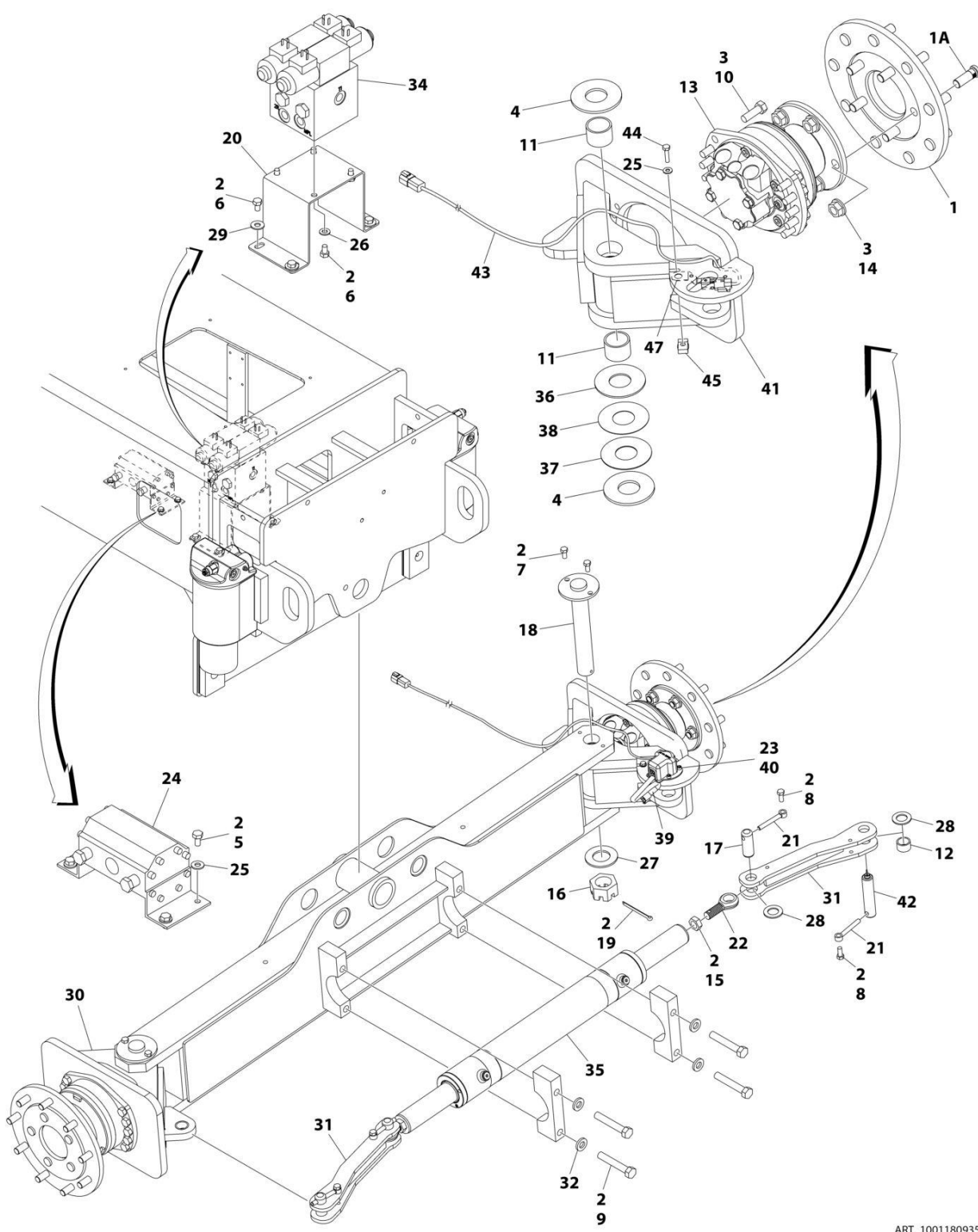
FIGURE 1-11. STEER INSTALLATION - (4WD/2WS) (E600/E600J & M600/M600J)
