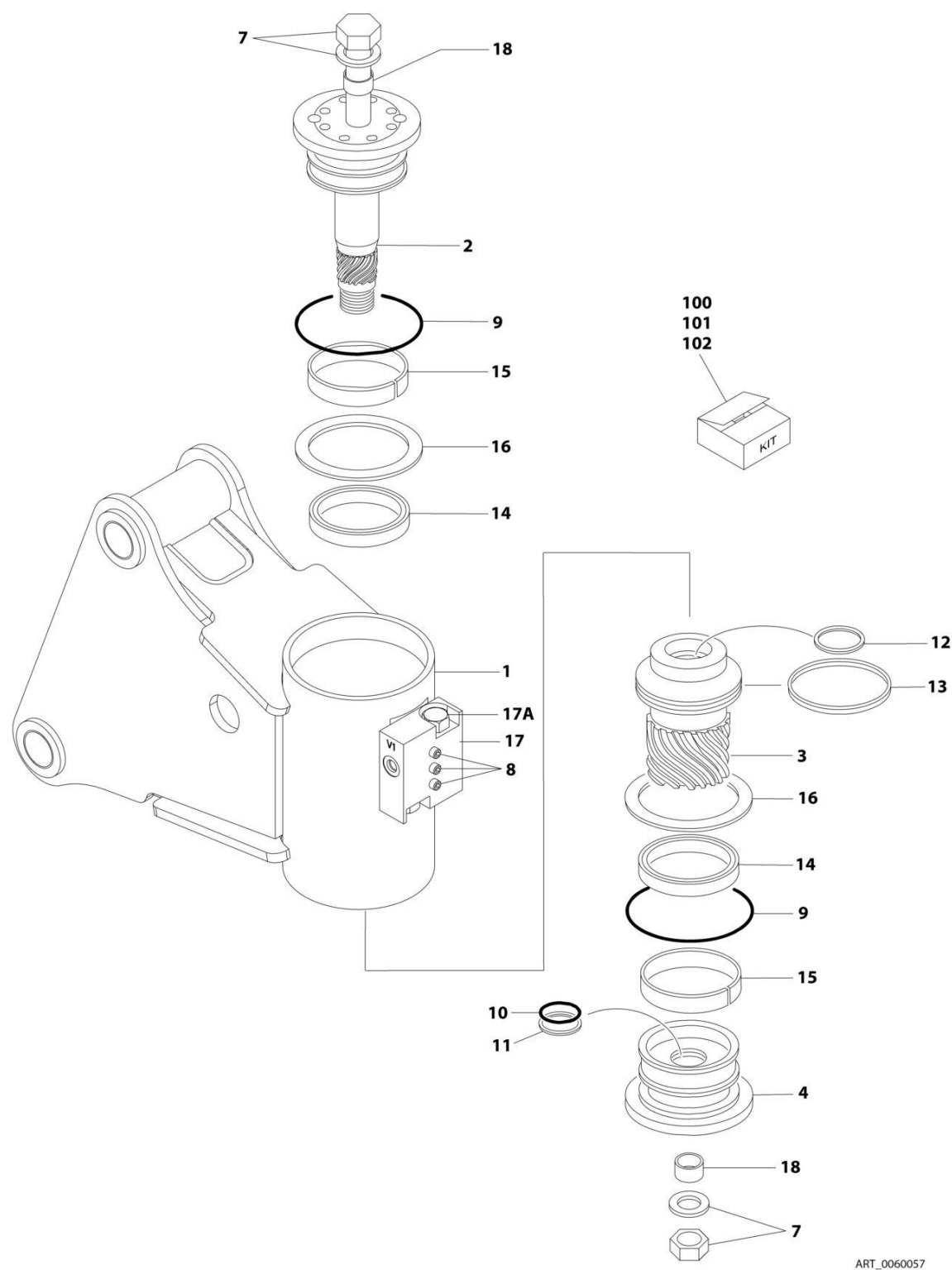
FIGURE 4-14. ROTATOR ASSEMBLY - SIDE SWING ROTATE (E600JP/M600JP)
