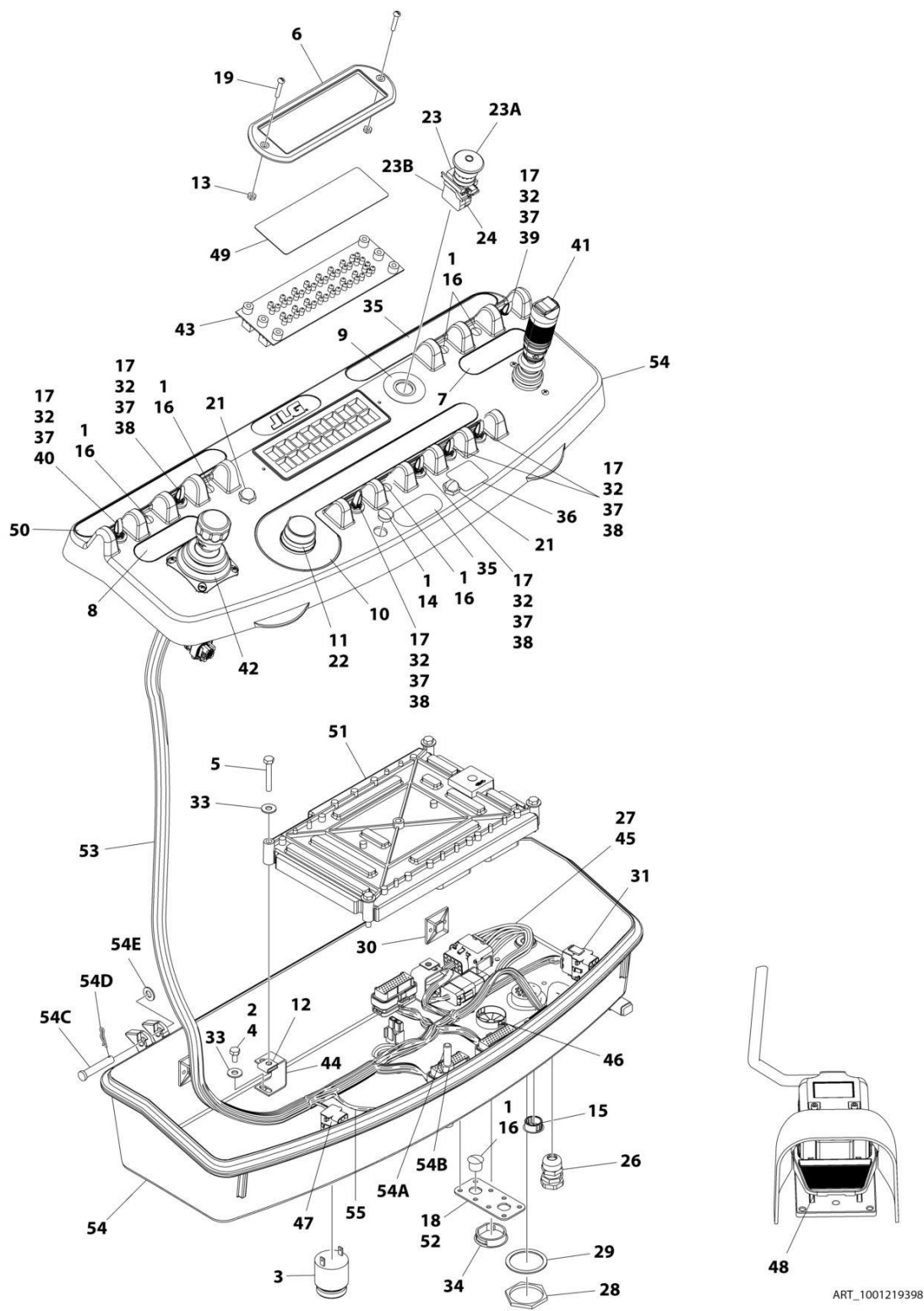
FIGURE 5-43. 2WD PLATFORM CONSOLE BOX ASSEMBLY - WITH 1 CELL LSS - WITH SKYGUARD (NON UL SPECS) (E600J/E600JP/M600J/M600JP) (SN 0300219271 through 0300256397)
