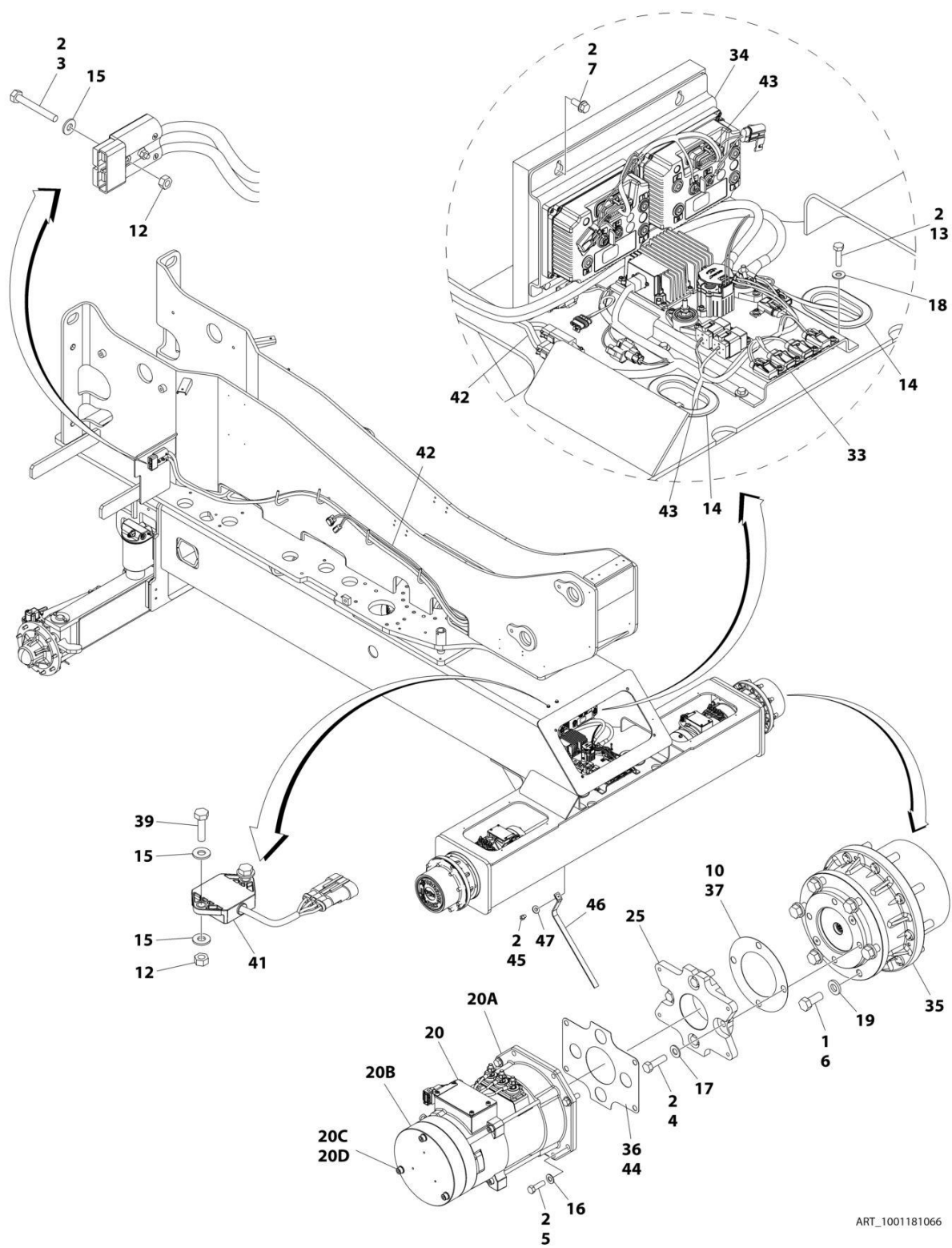
FIGURE 1-17. WHEEL DRIVE INSTALLATION (NON UL SPECS)
