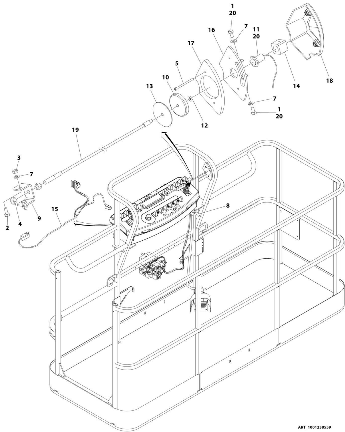
FIGURE 5-64. SKYLINE INSTALLATION
