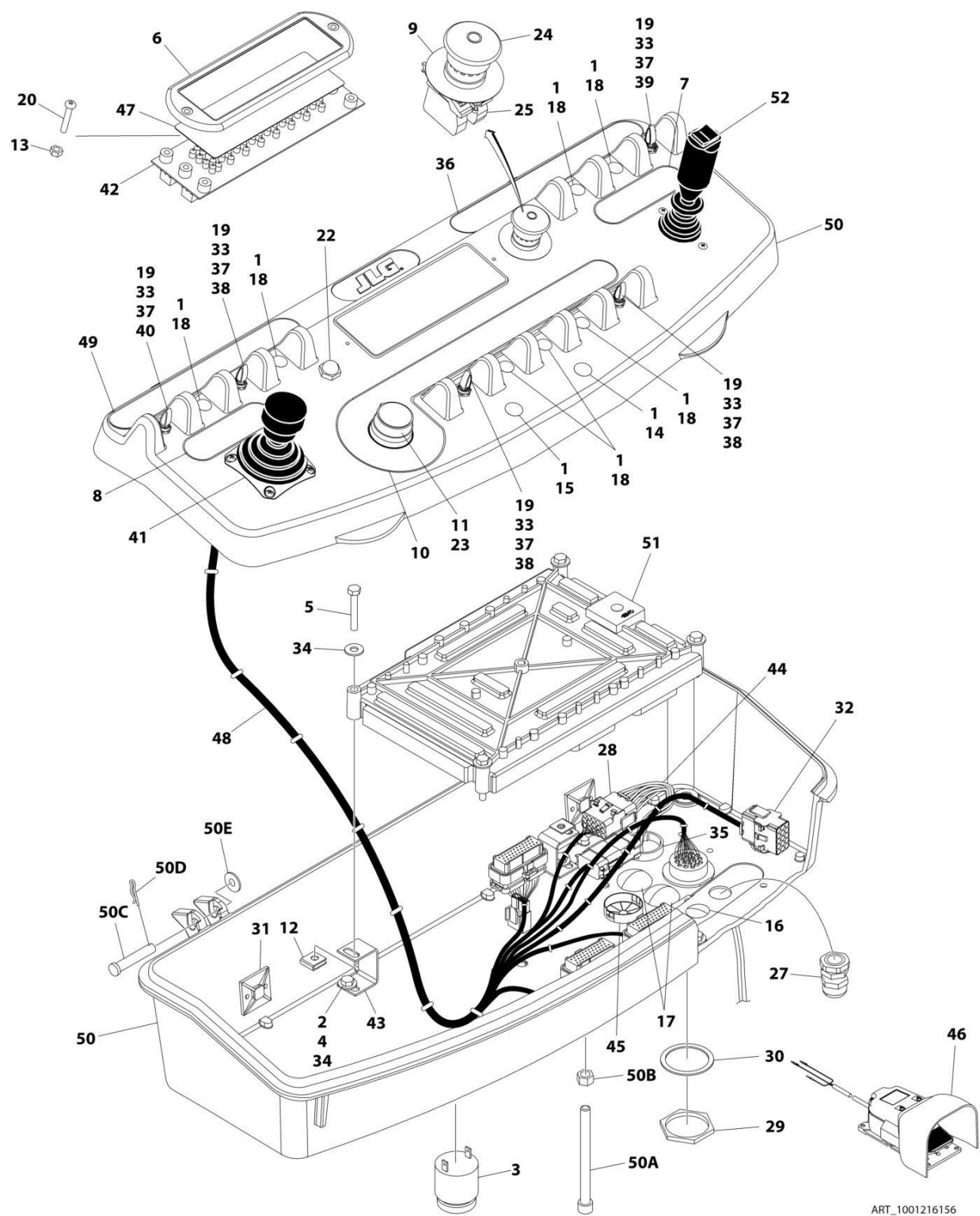
FIGURE 5-31. 2WD PLATFORM CONSOLE BOX ASSEMBLY - WITHOUT LSS OR WITH 4 CELL LSS - WITHOUT SKYGUARD (UL SPECS) (E600)
