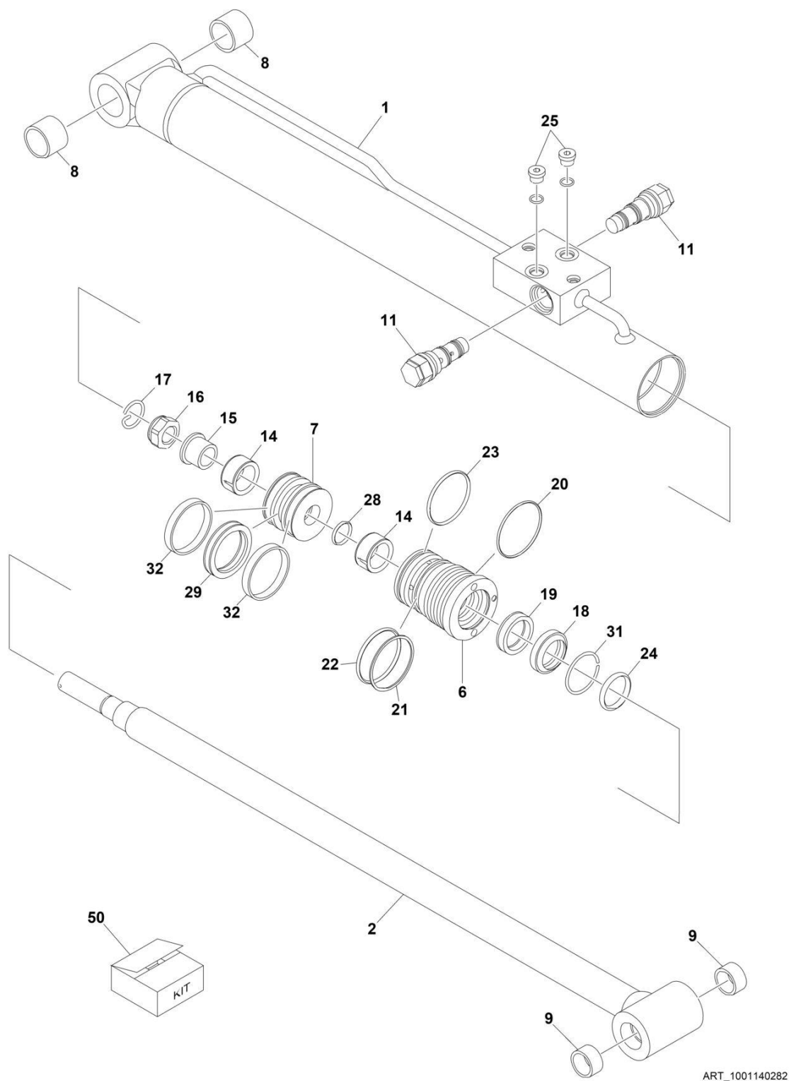
FIGURE 6-4. LIFT CYLINDER ASSEMBLY - JIB (E600J/E600JP/M600J/M600JP)
