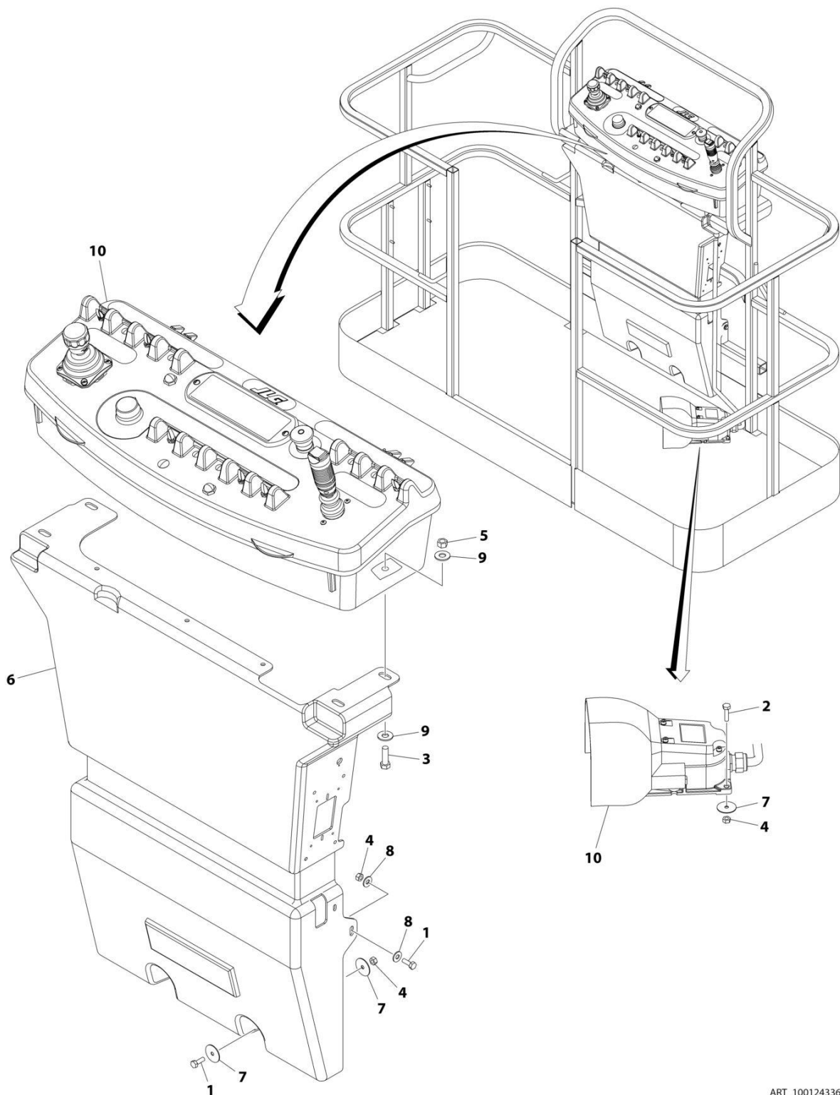
FIGURE 5-19. 4WD PLATFORM CONSOLE BOX INSTALLATION - WITHOUT LSS OR WITH 1 CELL LSS (UL SPECS) (E600J/E600JP) (SN 0300256398 to Present)
