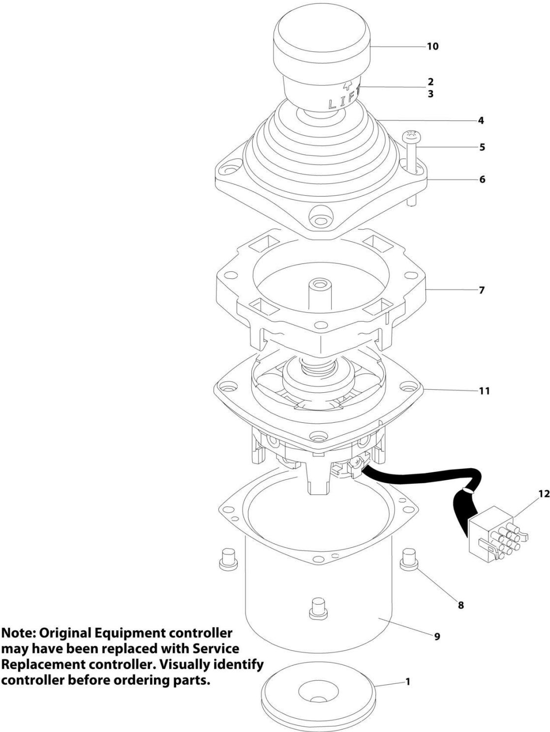
FIGURE 4-6. CONTROLLER ASSEMBLY (SWING AND LIFT) (SN 0300146804 through 0300194270)
