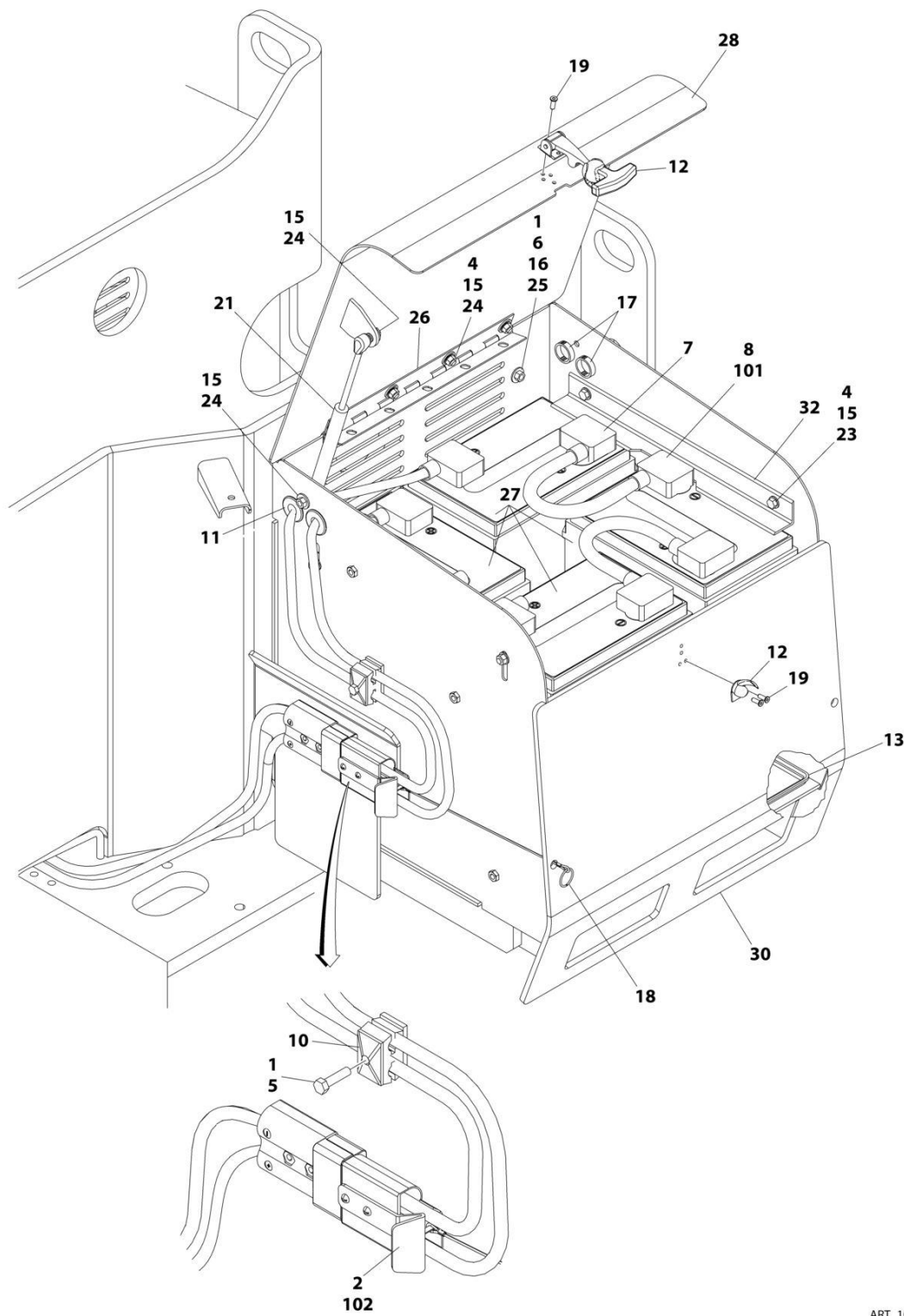
FIGURE 2-25. BATTERY BOX INSTALLATION - AGM BATTERIES
