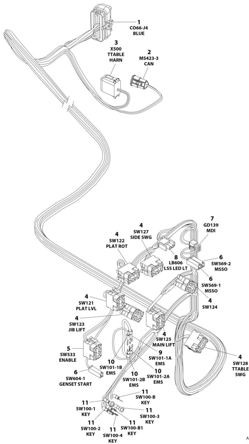
FIGURE 8-41. GROUND CONTROL HARNESS
