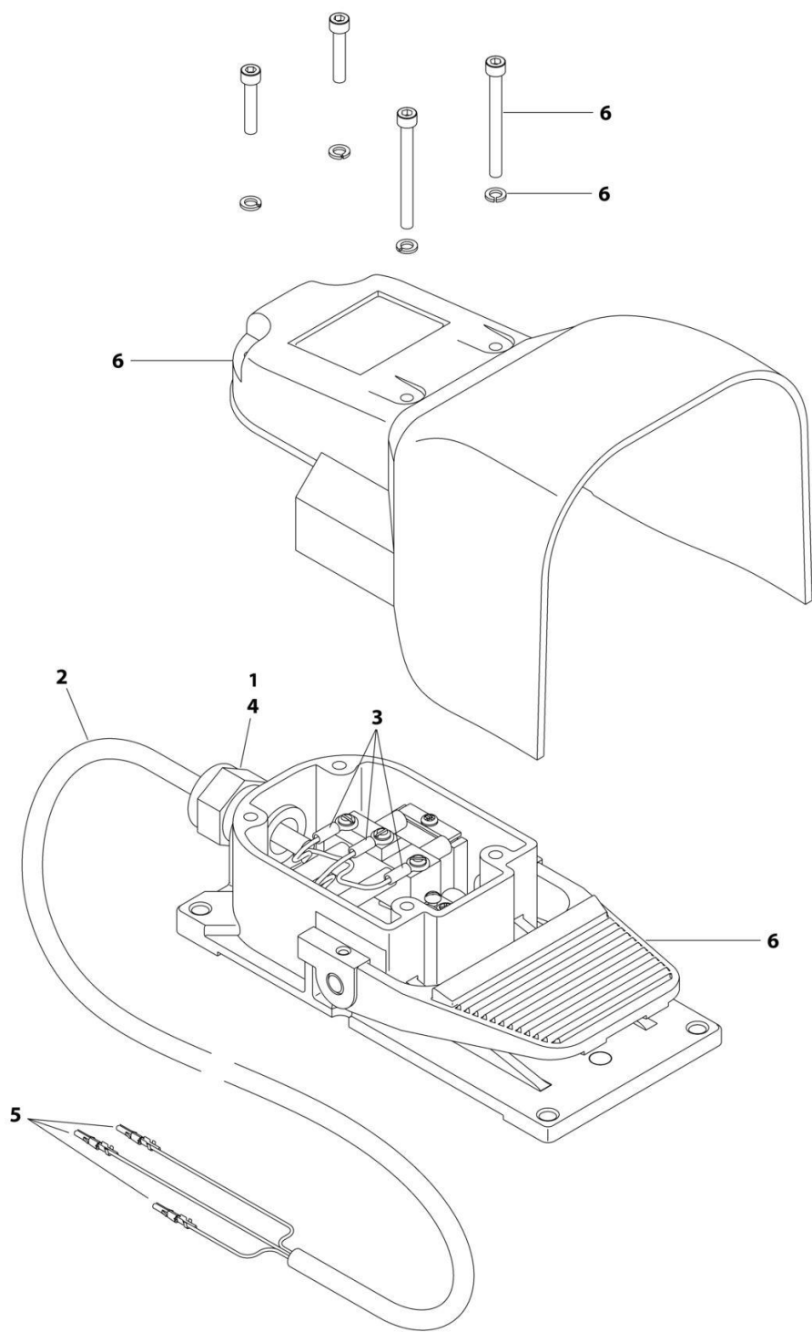
FIGURE 5-22. FOOTSWITCH ASSEMBLY
