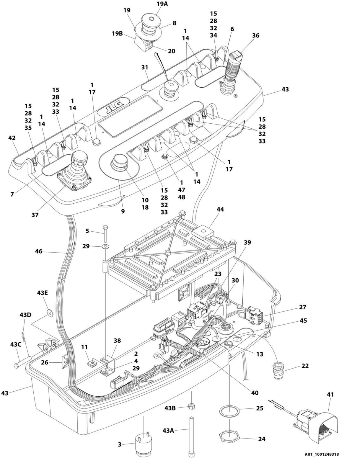
FIGURE 5-17. PLATFORM CONSOLE ASSEMBLY - 2WD (UL SPECS)
