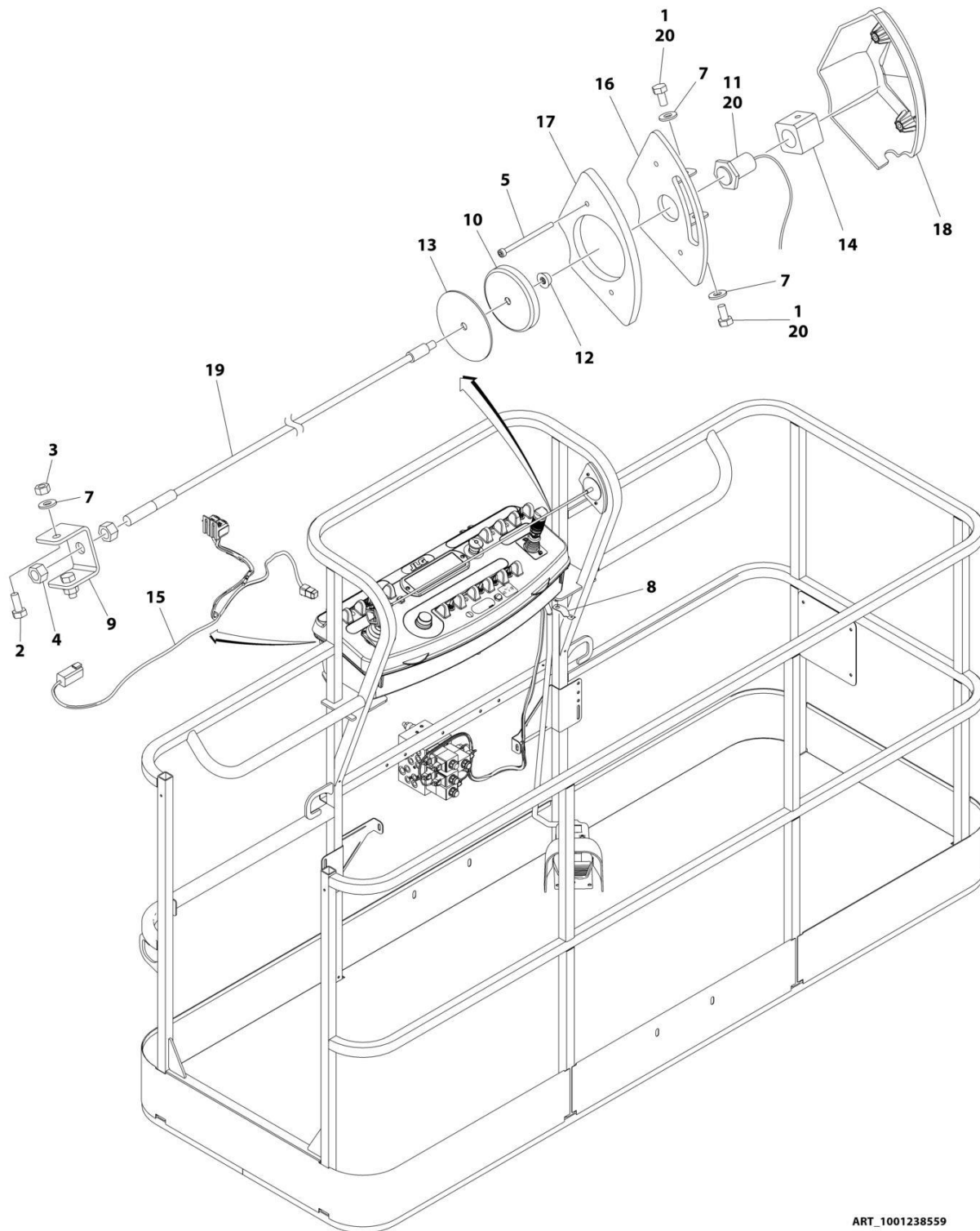
FIGURE 5-30. SKYLINE INSTALLATION
