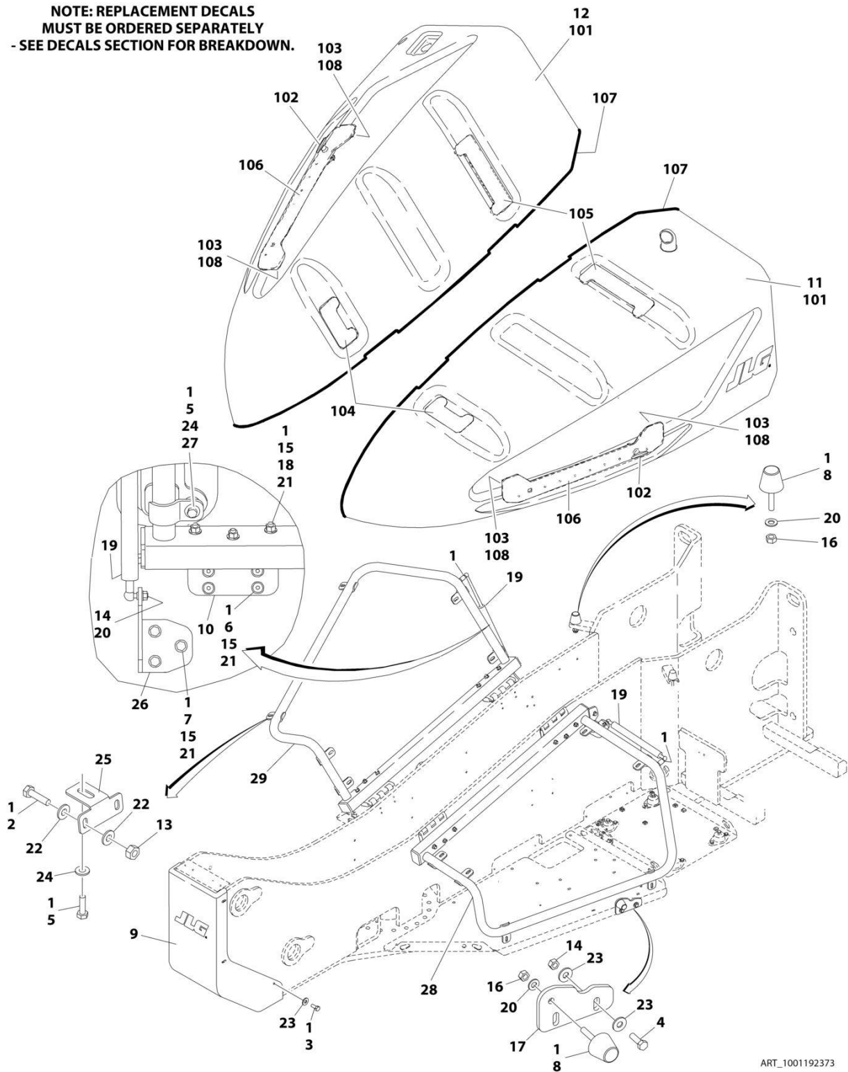
FIGURE 2-42. HOODS INSTALLATION
