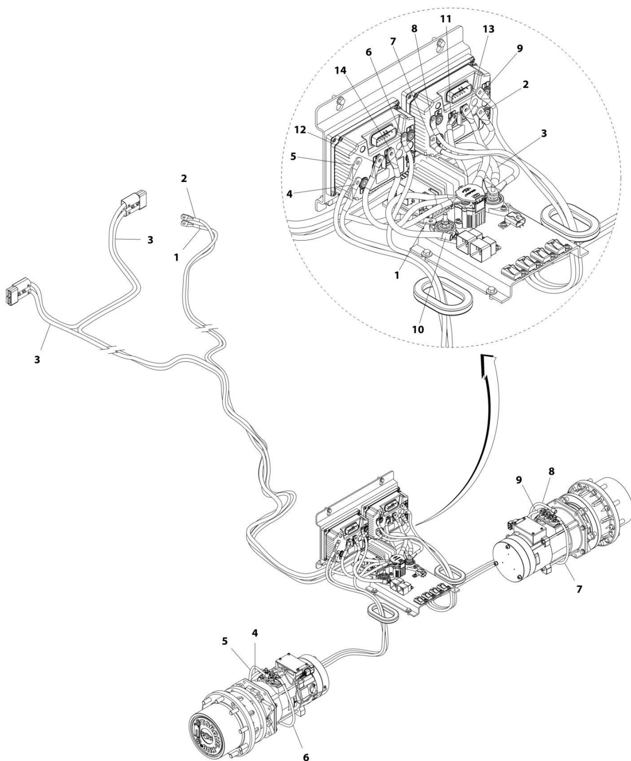
FIGURE 8-37. DRIVE CABLE KIT (ALL SPECS EXCPET UL SPECS)
