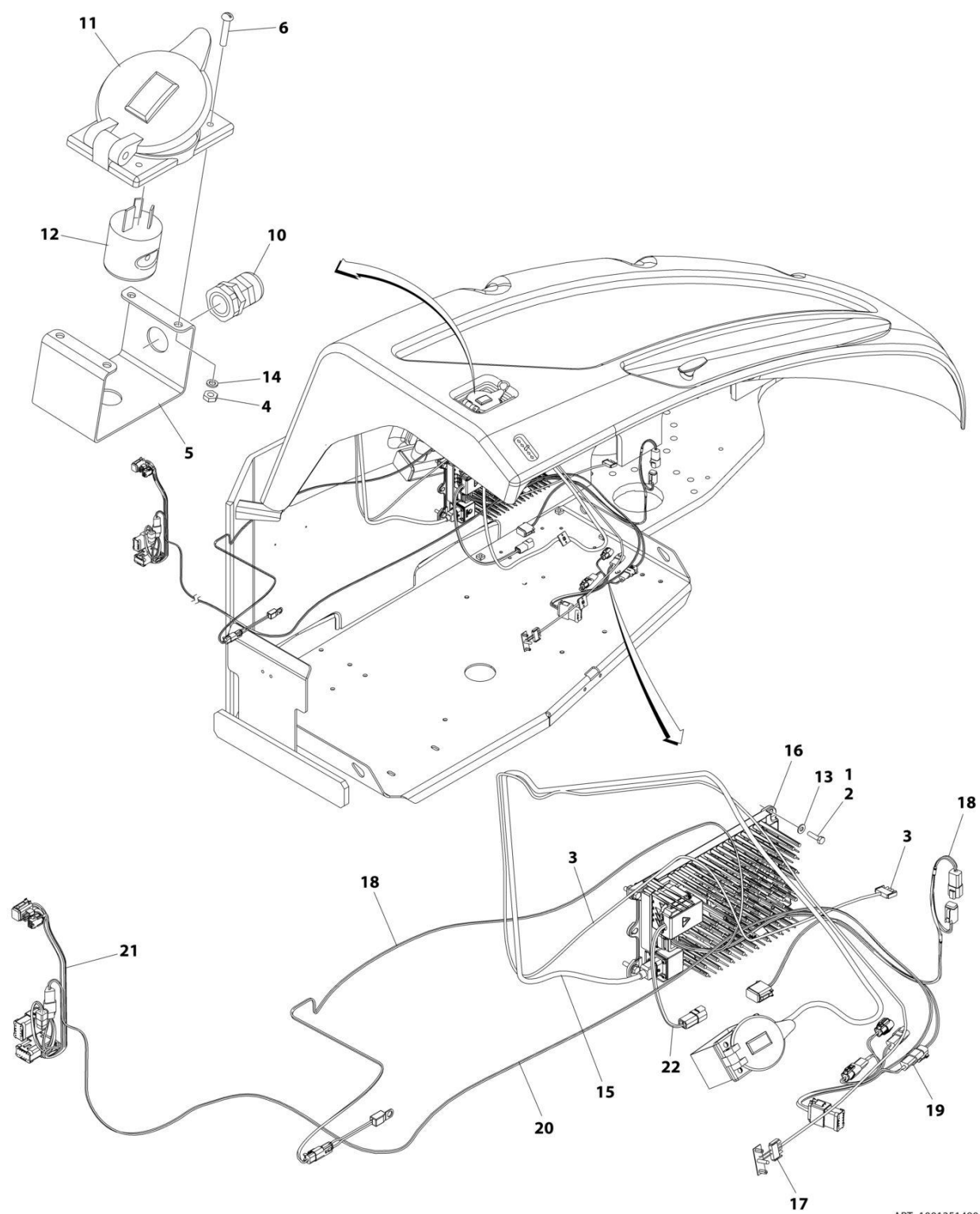
FIGURE 2-23. BATTERY CHARGER INSTALLATION - 250V/50HZ (ANSI EXPORT, AUSTRALIAN AND CHINA SPECS) (PVC 2007)
