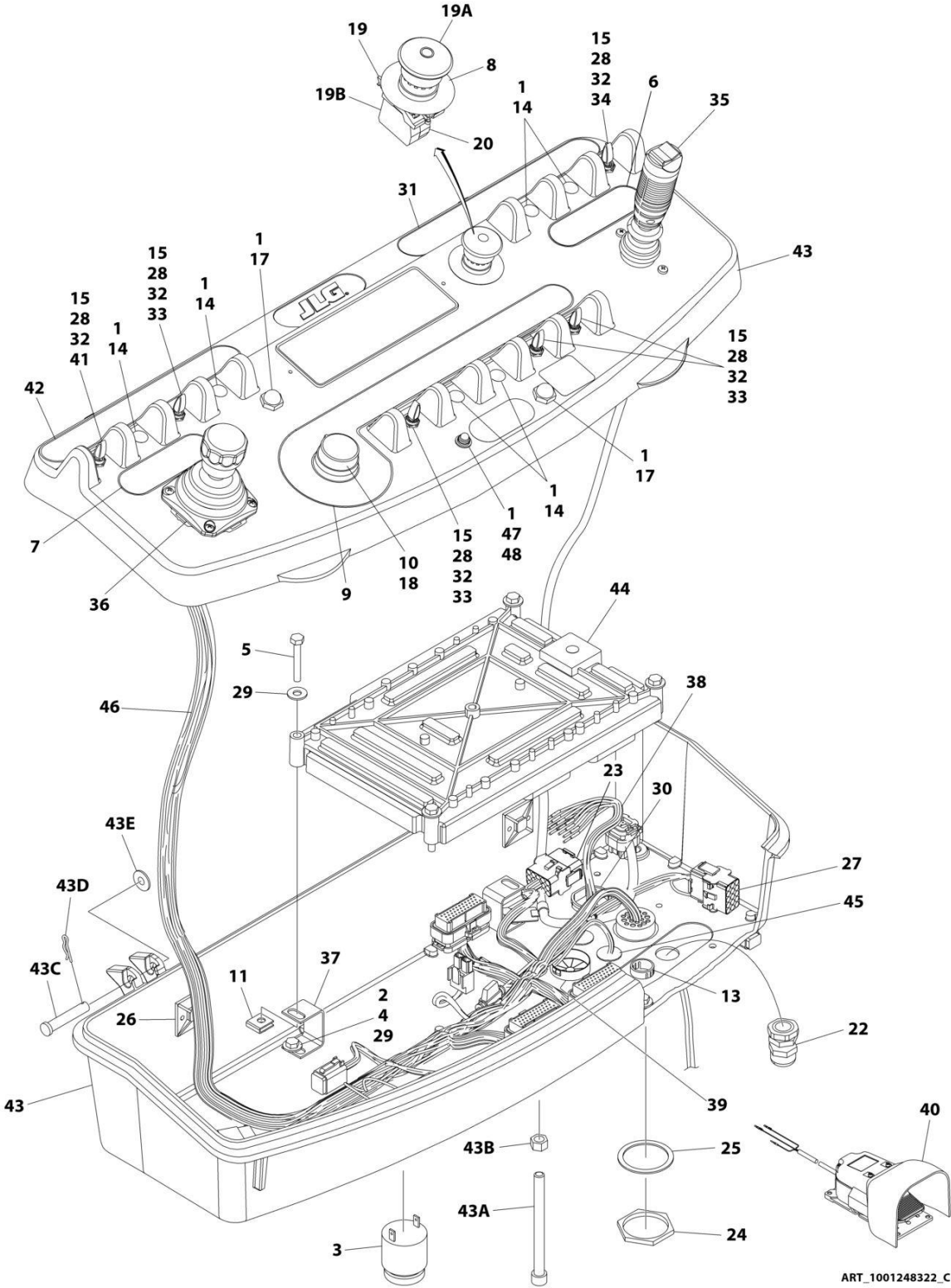
FIGURE 5-19. PLATFORM CONSOLE ASSEMBLY - 4WD (UL SPECS)
