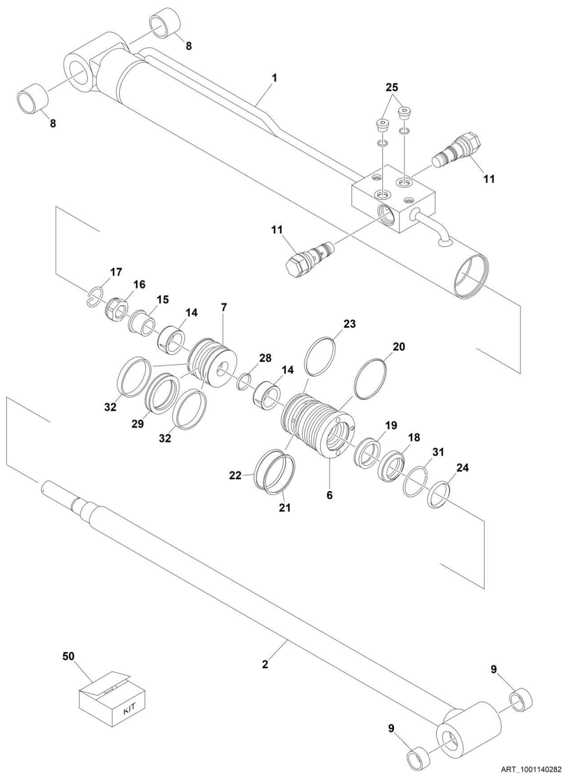
FIGURE 6-3. LIFT CYLINDER ASSEMBLY - JIB
