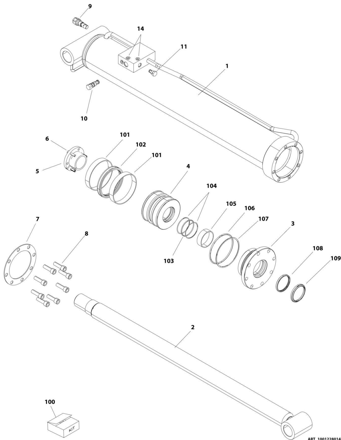
FIGURE 6-4. LIFT CYLINDER ASSEMBLY - MAIN (PRIOR TO PVC 2001)
