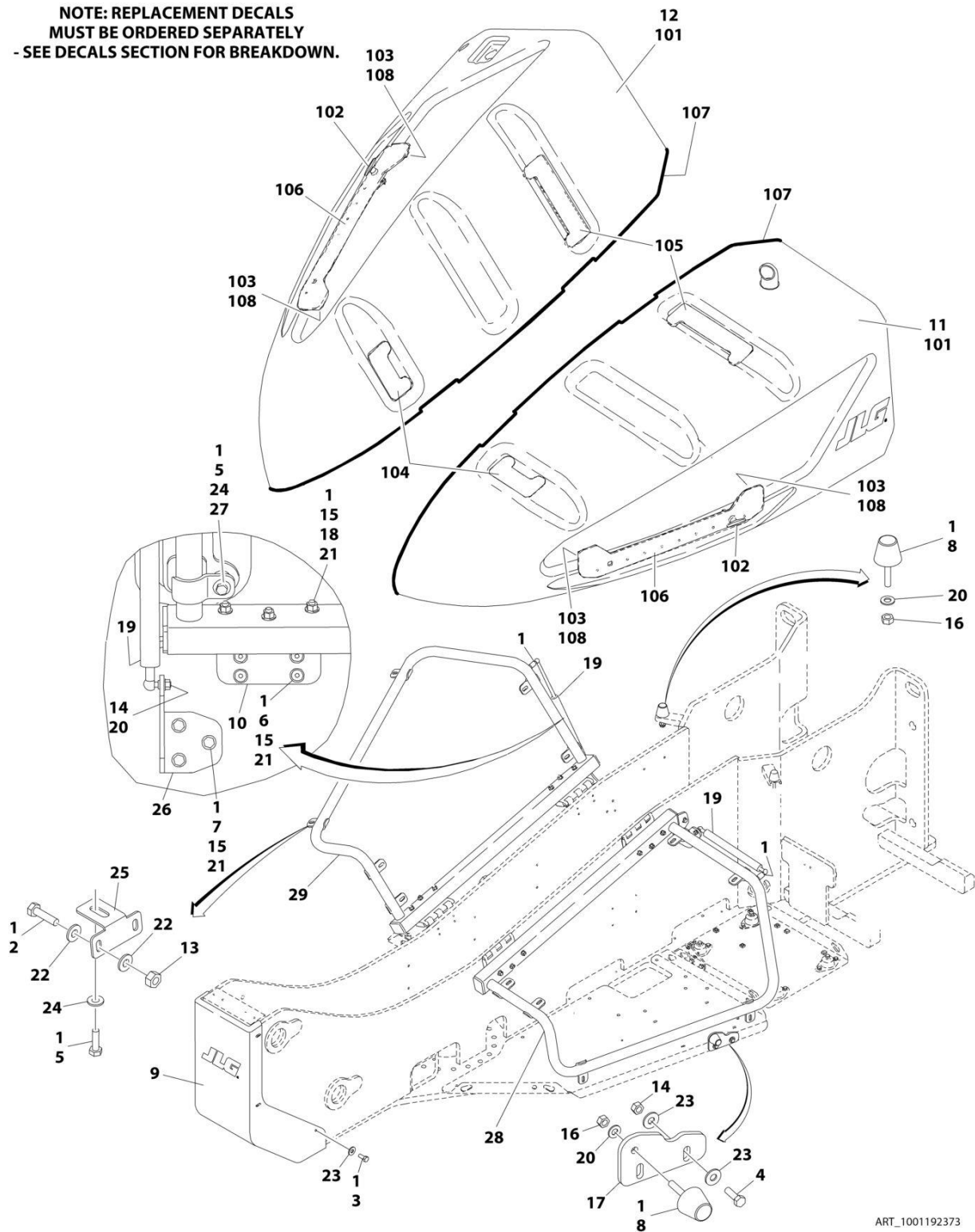
FIGURE 2-37. HOODS INSTALLATION
