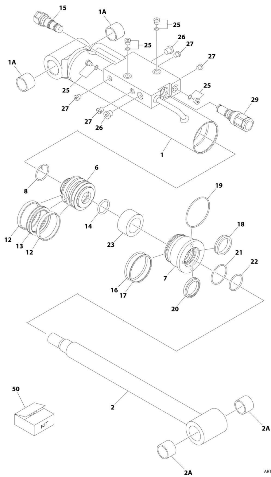
FIGURE 6-2. LEVEL CYLINDER ASSEMBLY - PLATFORM SLAVE
