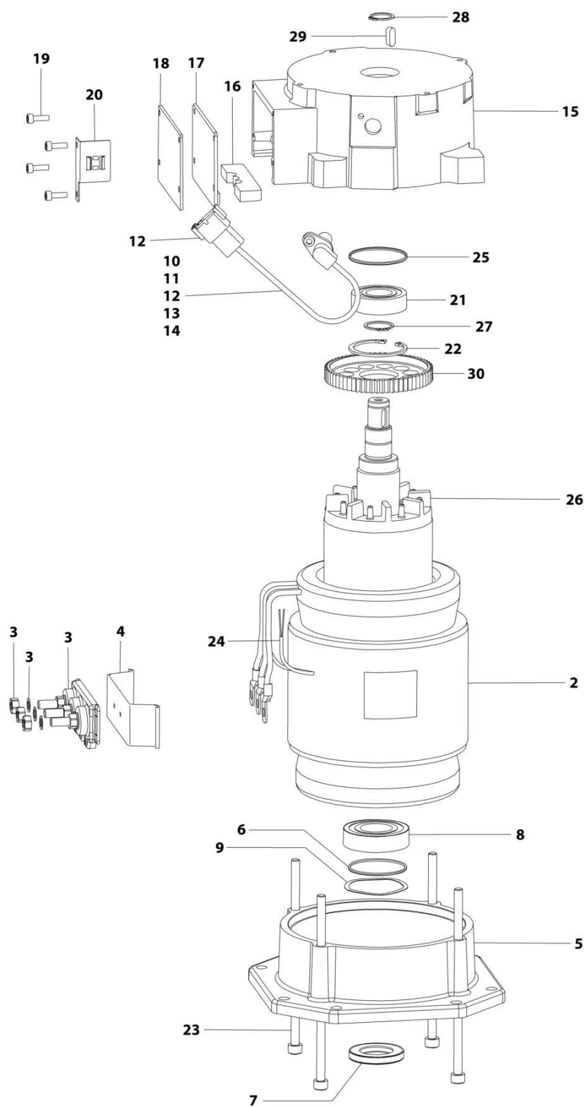
FIGURE 1-17. DRIVE MOTOR ASSEMBLY (REAR)
