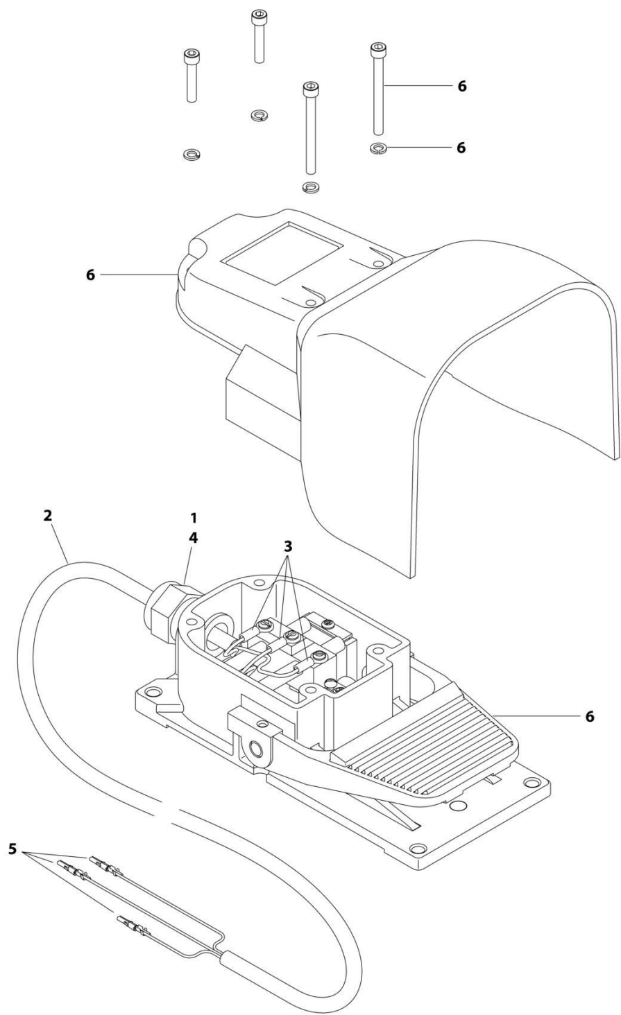
FIGURE 5-22. FOOTSWITCH ASSEMBLY
