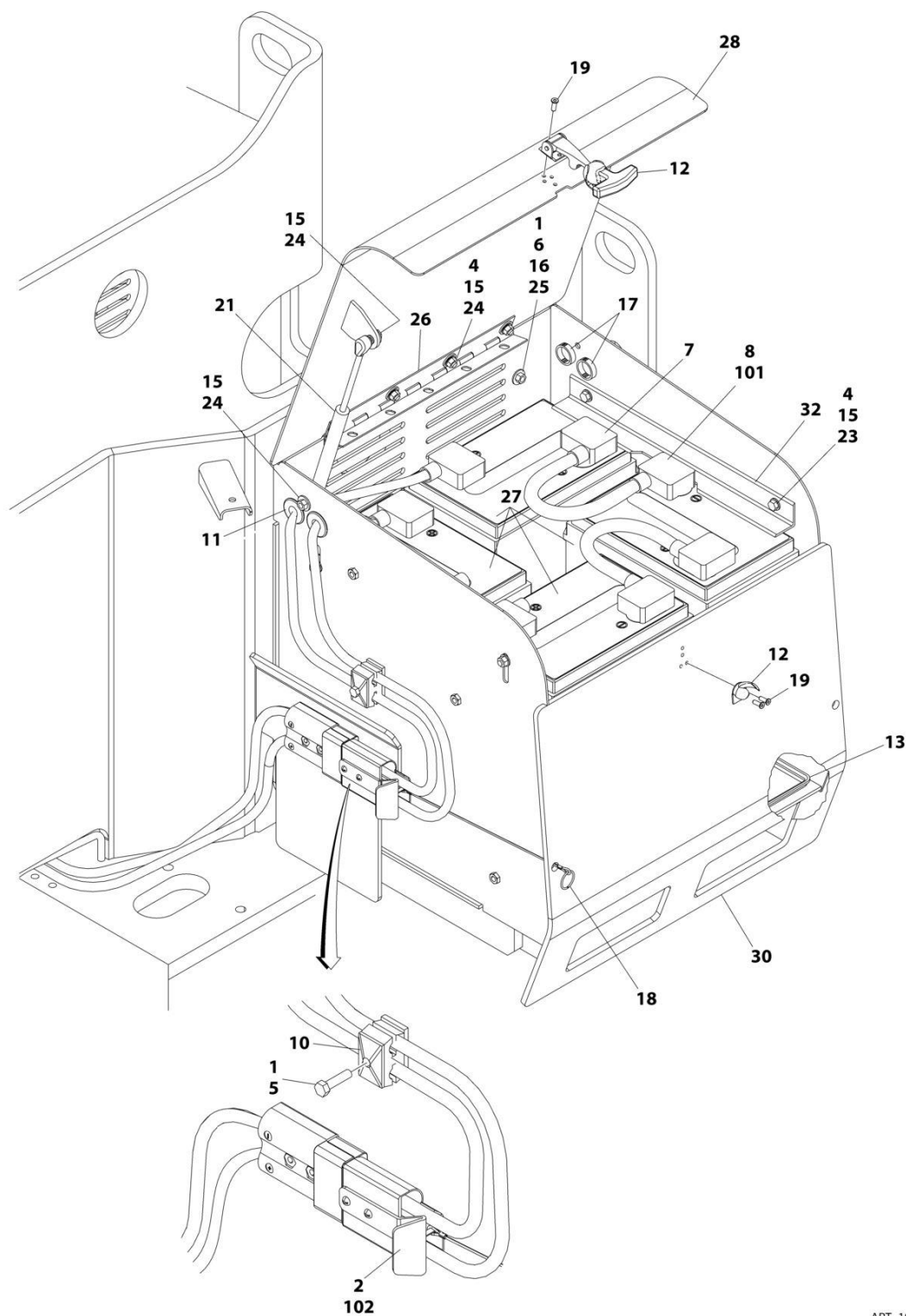
FIGURE 2-20. BATTERY BOX INSTALLATION - AGM BATTERIES
