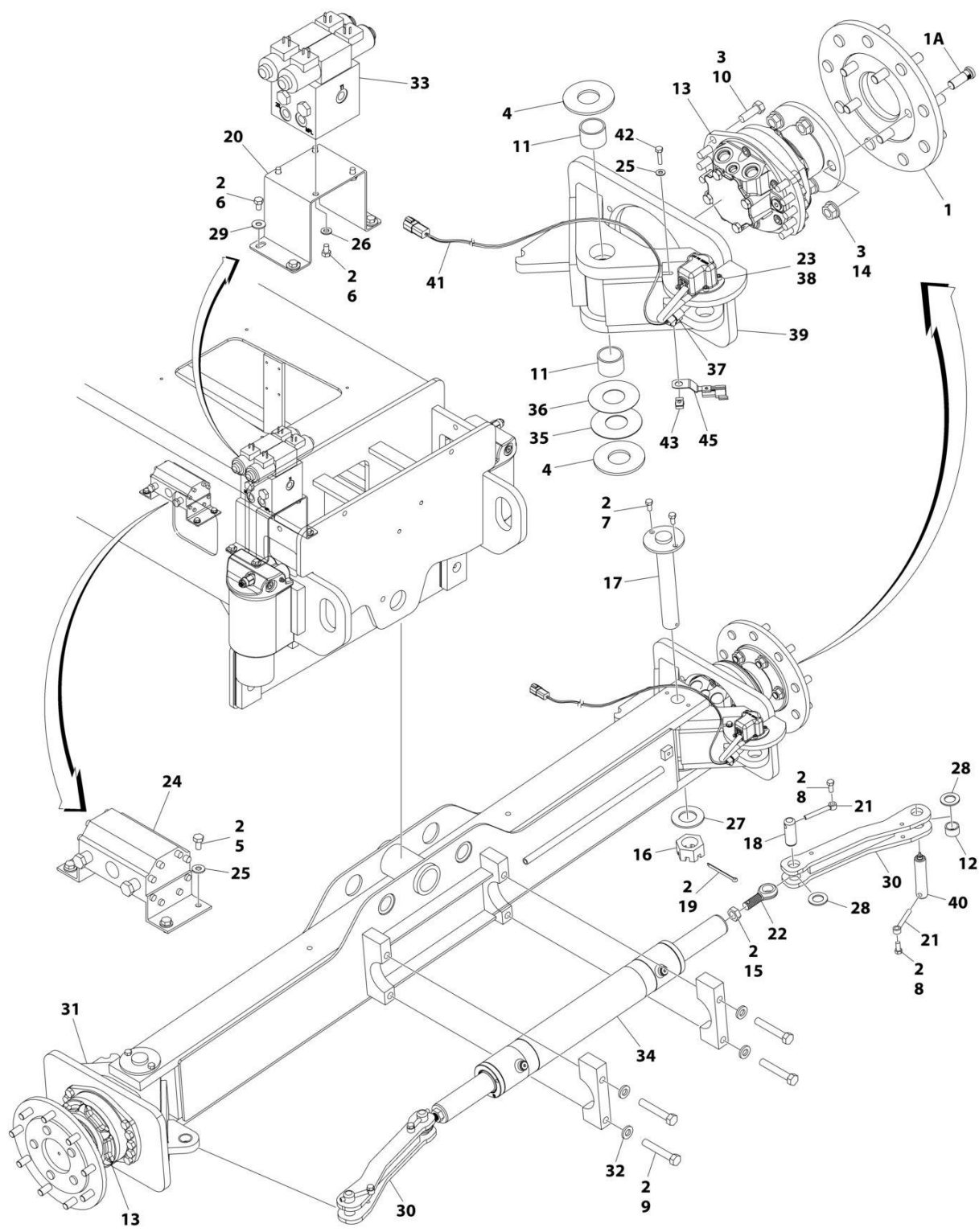
FIGURE 1-10. STEER INSTALLATION - (4WD/2WS) (EC600SJP/H600SJP)
