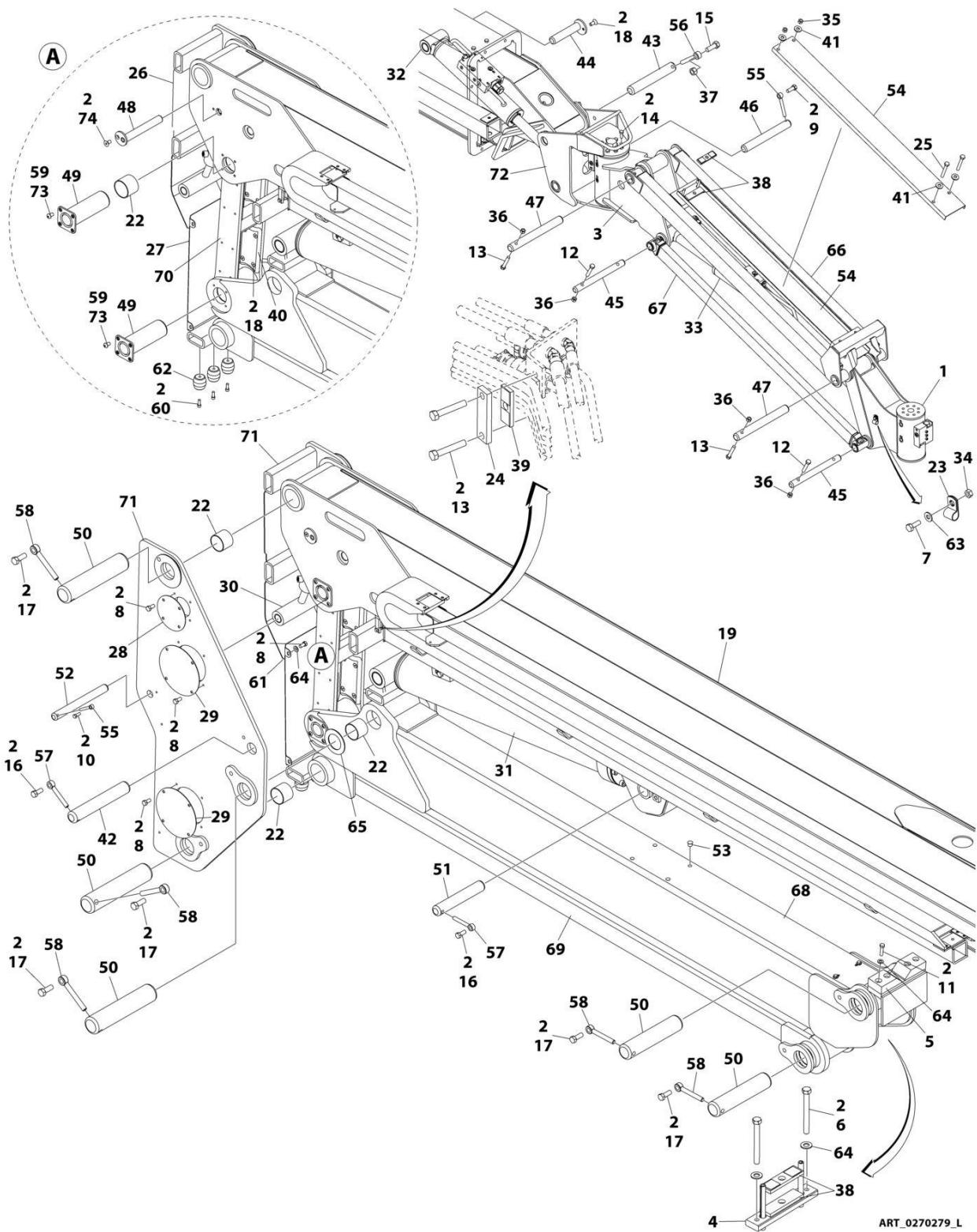
FIGURE 4-2. BOOM INSTALLATION (EC600SJP/H600SJP)
