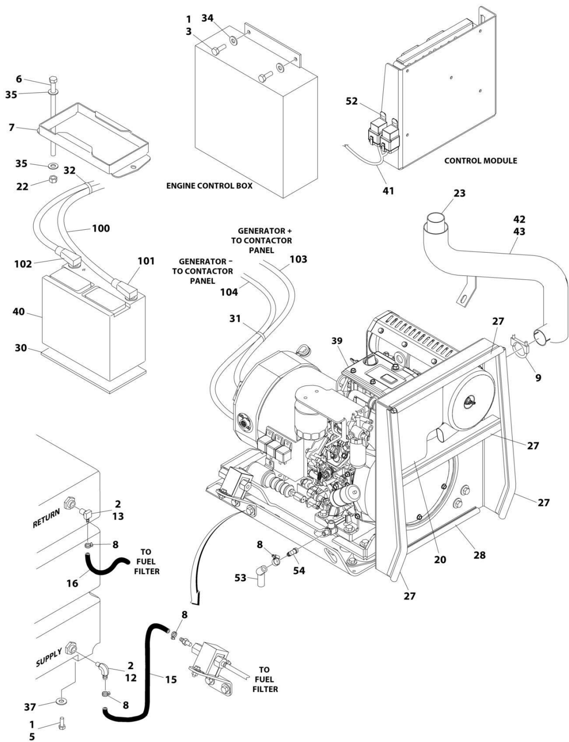
FIGURE 3-2. ENGINE AND GENERATOR INSTALLATION - WITH AGM BATTERIES (H600SJ/H600SJP ONLY)
