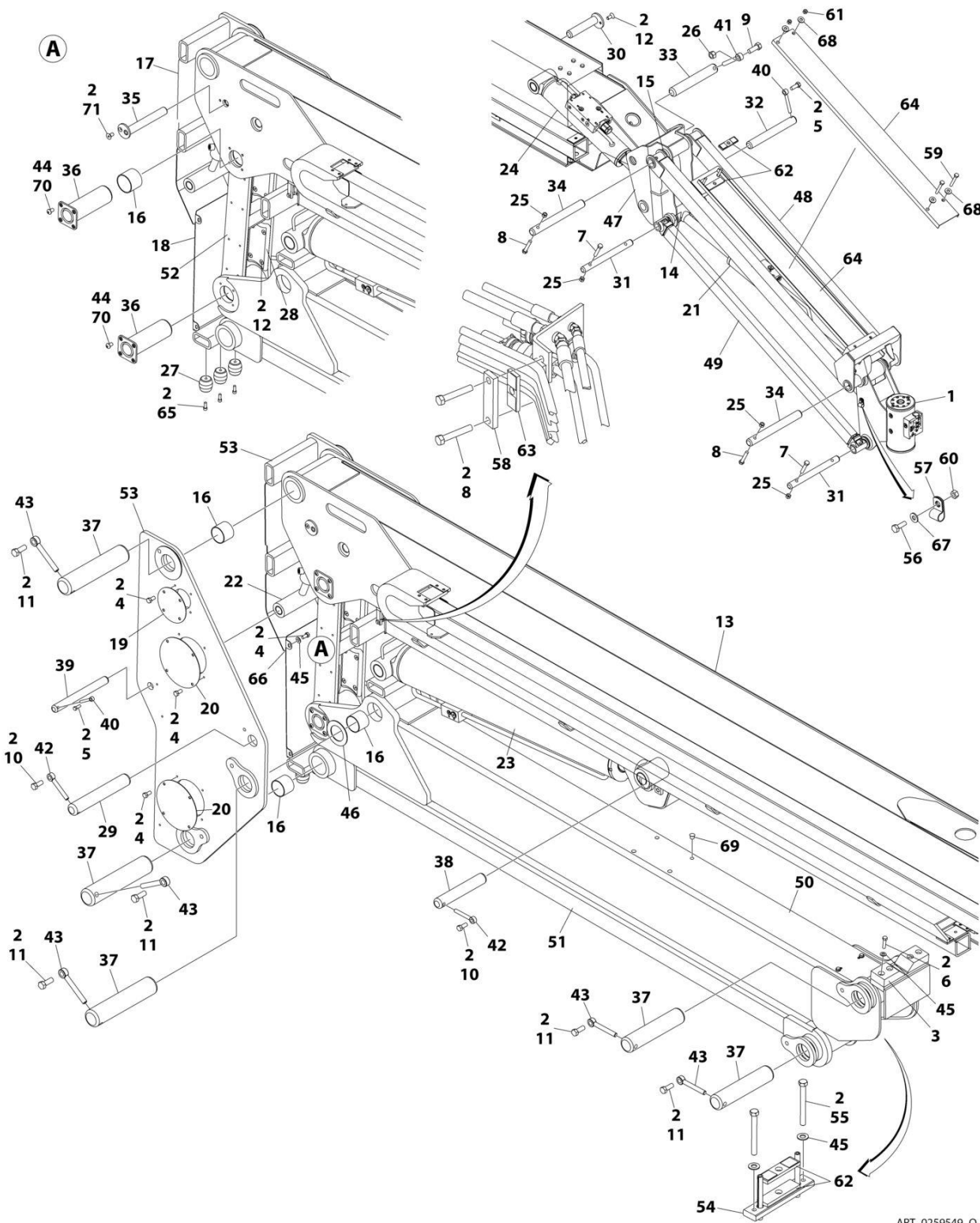
FIGURE 4-1. BOOM INSTALLATION (EC600SJ/H600SJ)
