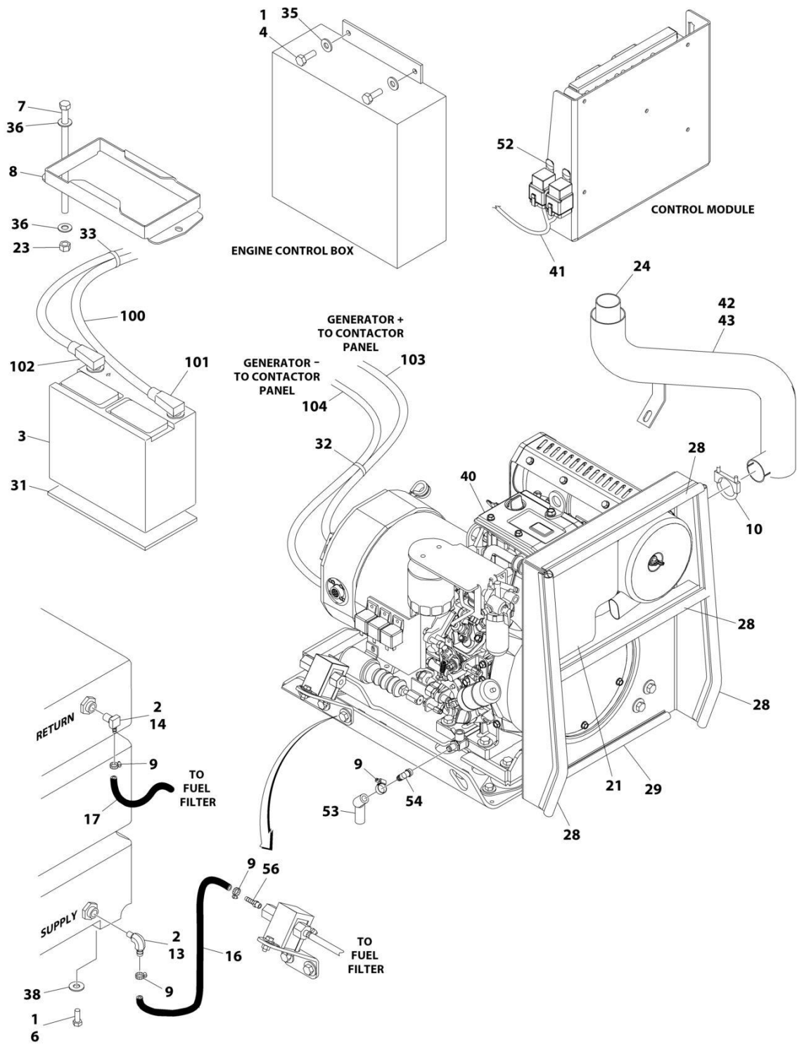
FIGURE 3-1. ENGINE AND GENERATOR INSTALLATION - WITH STANDARD BATTERIES (H600SJ/H600SJP ONLY)
