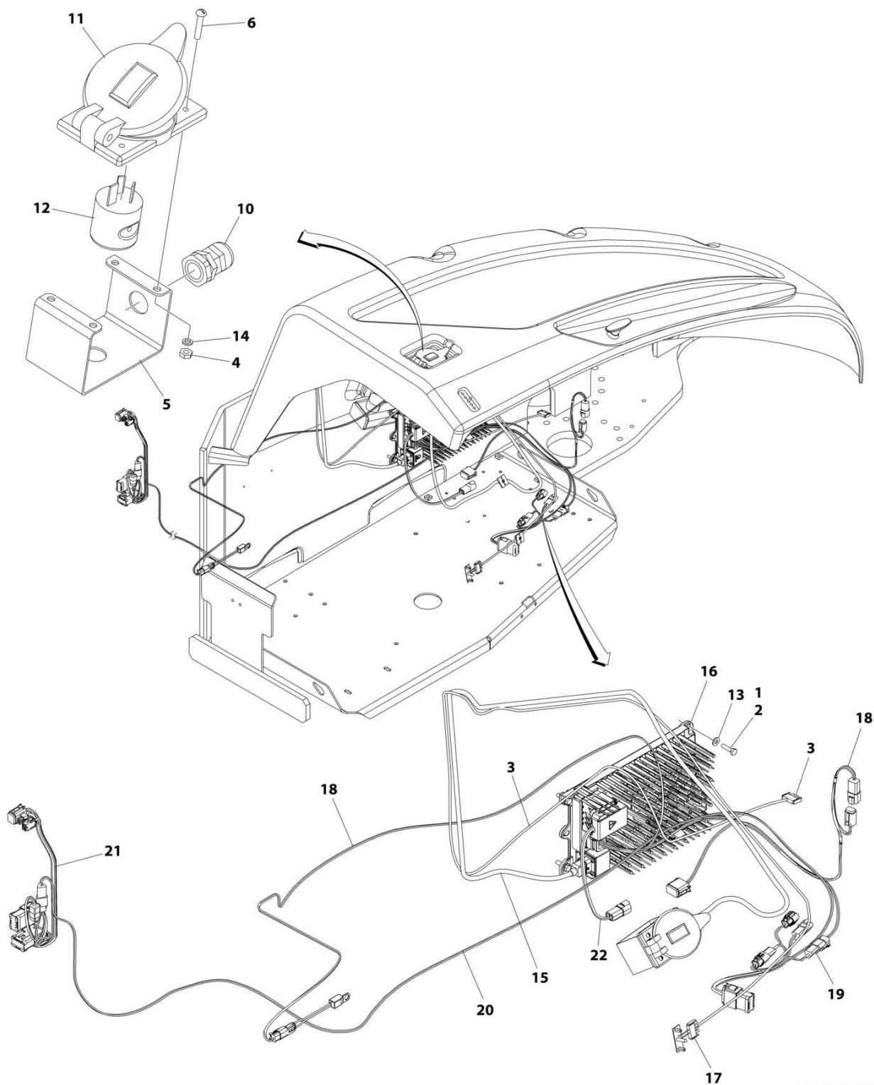
FIGURE 2-18. BATTERY CHARGER INSTALLATION - 250V/50HZ (ANSI EXPORT, AUSTRALIAN AND CHINA SPECS)
