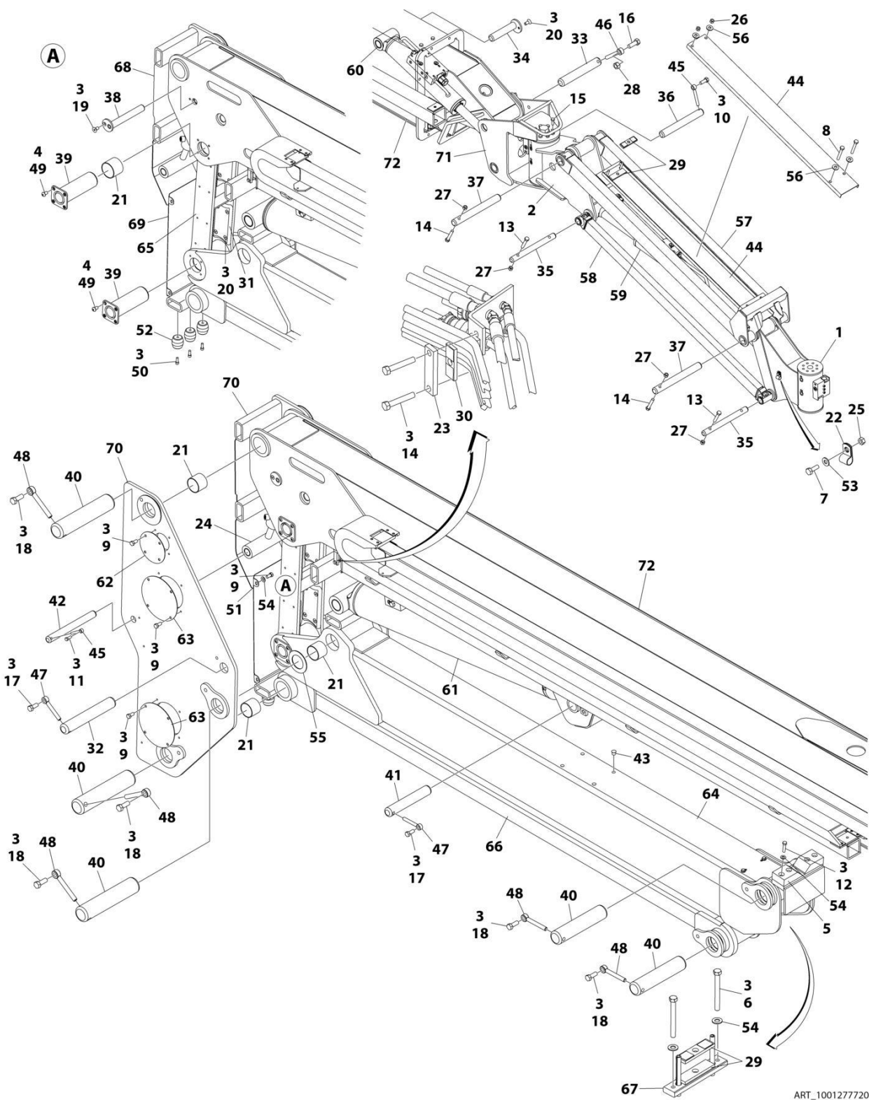
FIGURE 4-4. BOOM INSTALLATION (EC600SJP/H600SJP) (MACHINES WITH SN STARTING WITH B3)
