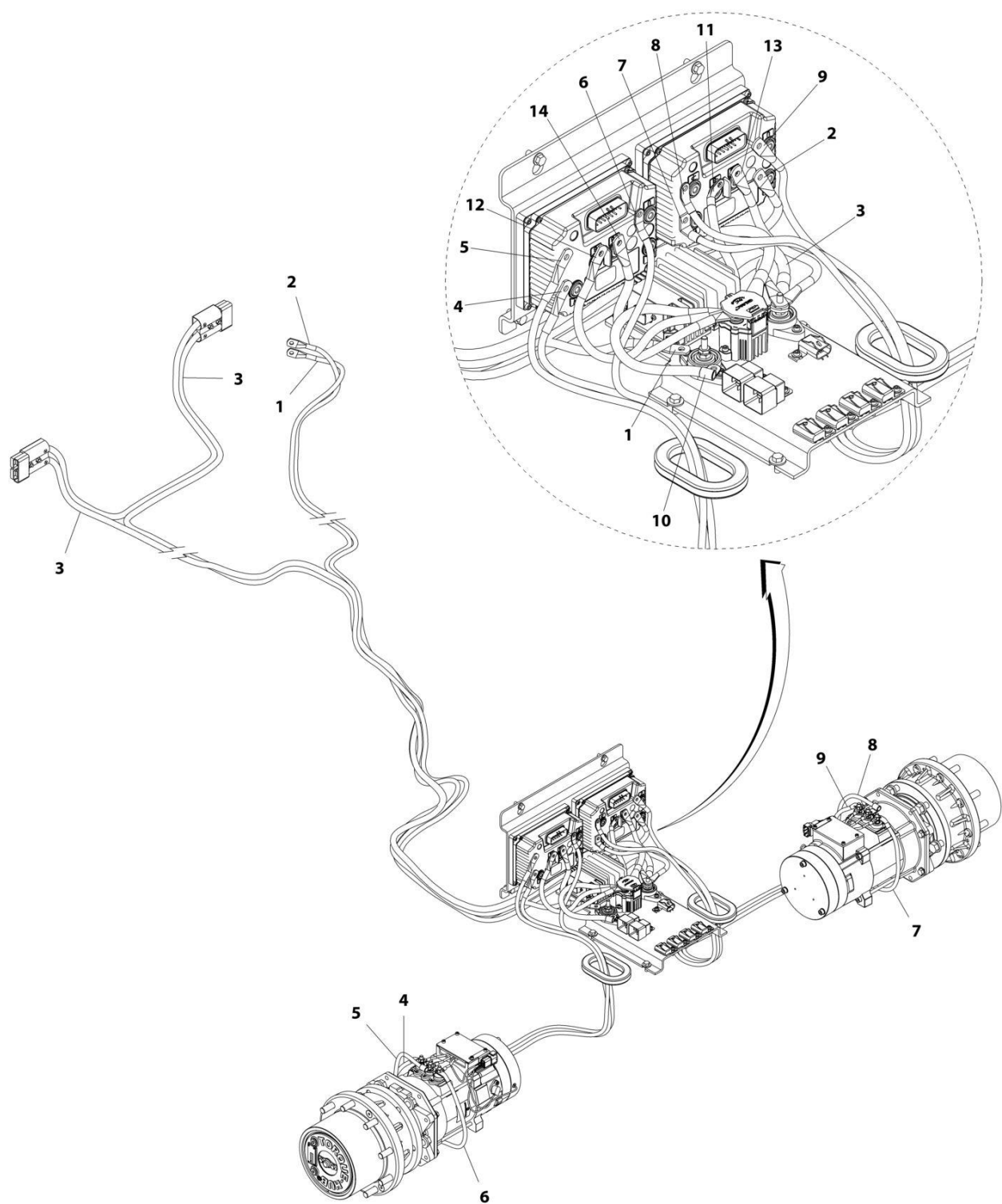
FIGURE 8-39. DRIVE CABLE KIT (ALL SPECS EXCPET UL SPECS)
