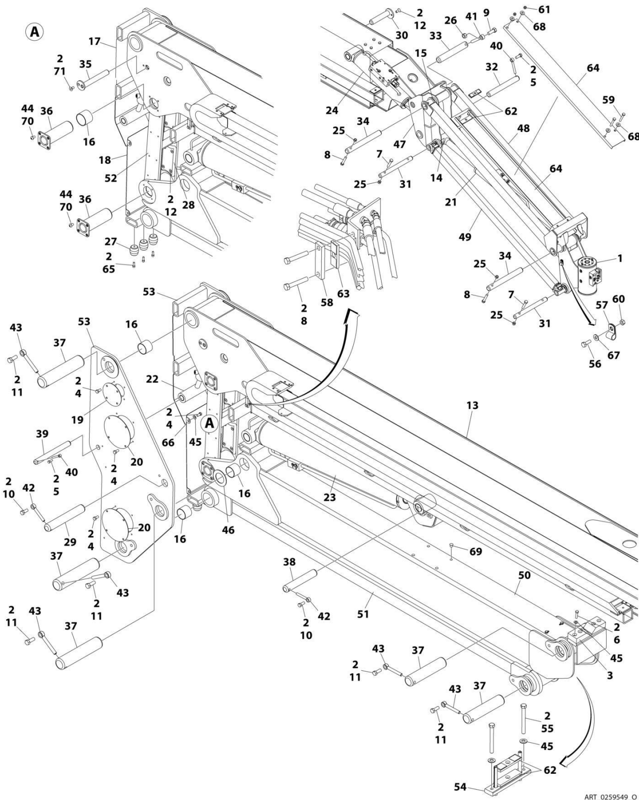
FIGURE 4-1. BOOM INSTALLATION (EC600SJ/H600SJ) (MACHINES WITH SN STARTING WITH 03)
