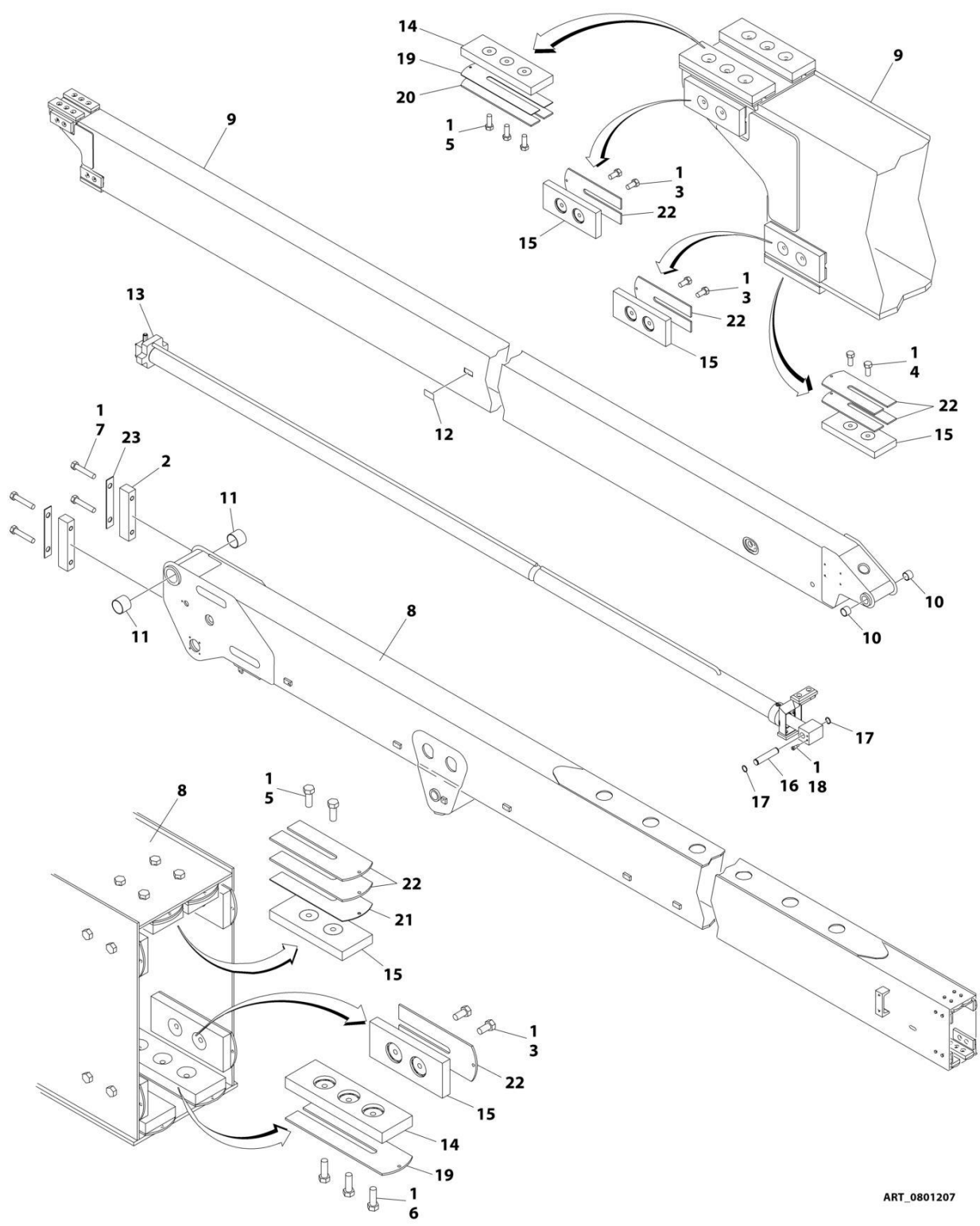
FIGURE 4-5. MAIN BOOM ASSEMBLY (EC600SJ/H600SJ) (MACHINES WITH SN STARTING WITH 03)
