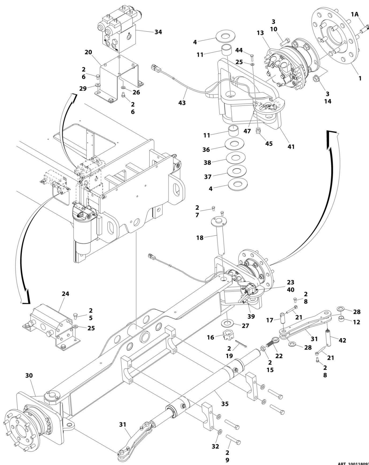
FIGURE 1-11. STEER INSTALLATION - (4WD/2WS) (EC600SJ/H600SJ)
