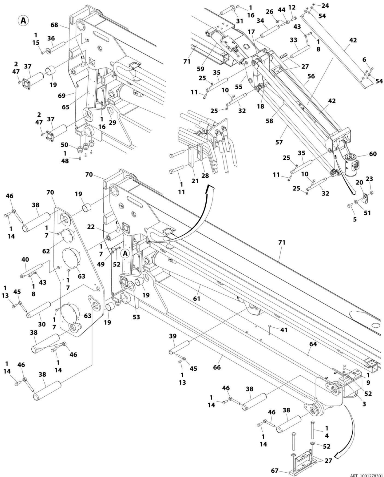
FIGURE 4-2. BOOM INSTALLATION (EC600SJ/H600SJ) (MACHINES WITH SN STARTING WITH B3)
