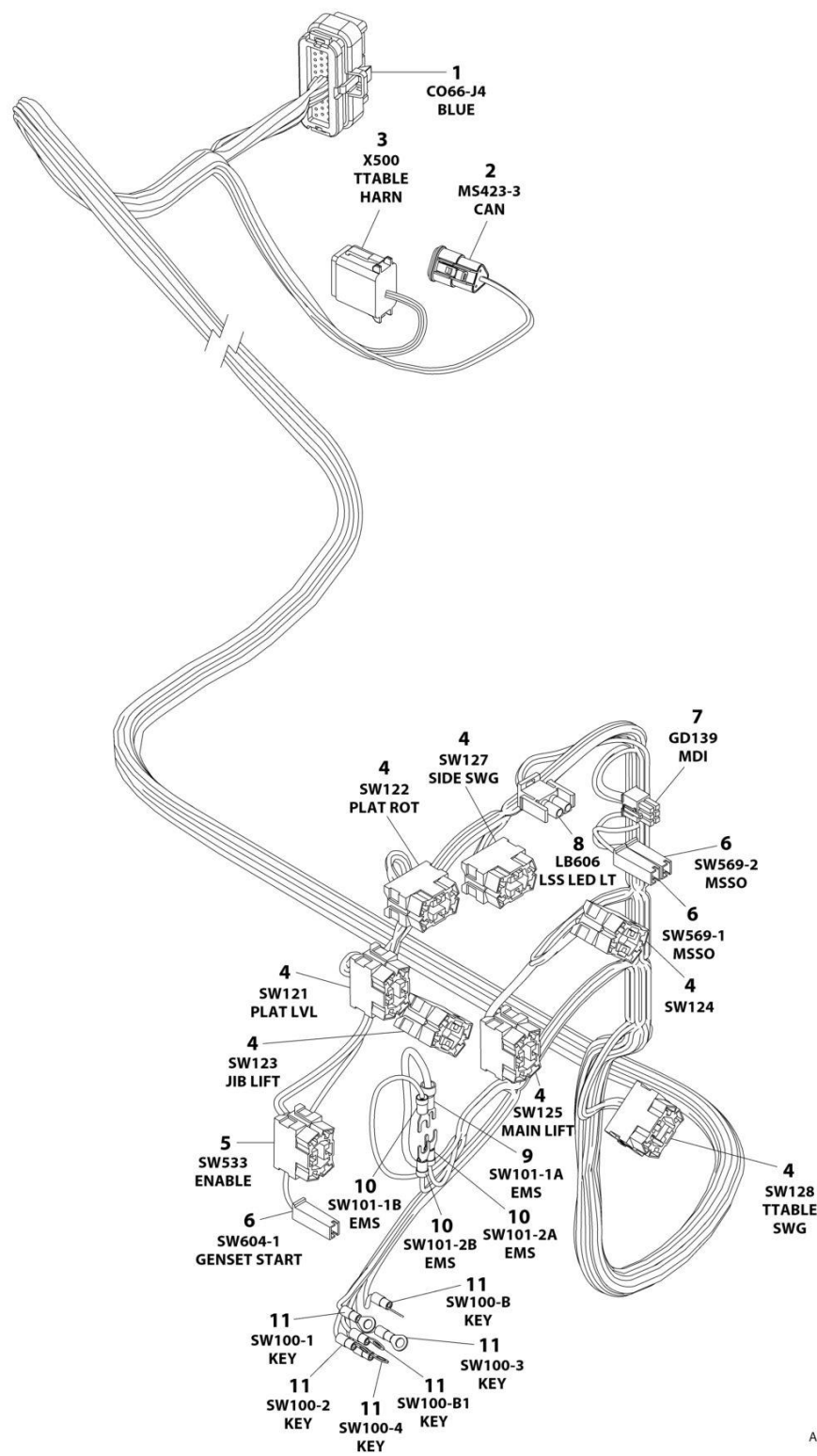
FIGURE 8-43. GROUND CONTROL HARNESS
