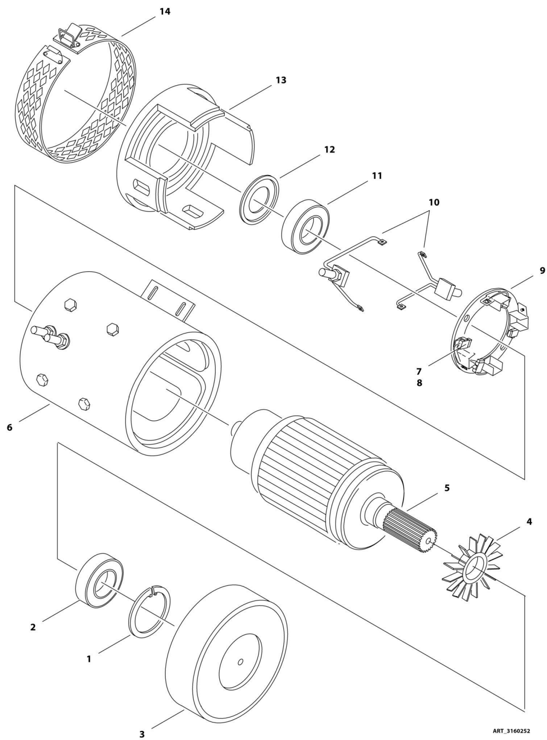
FIGURE 2-11. ELECTRIC MOTOR ASSEMBLY
