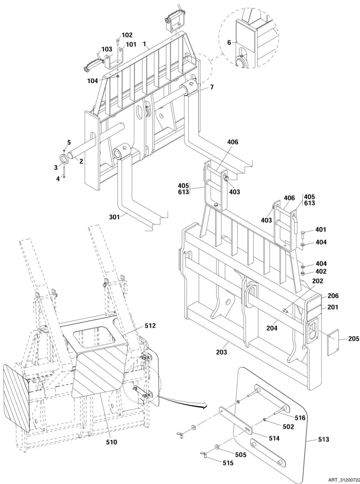
FIGURE 3-1. CARRIAGE ASSEMBLY
