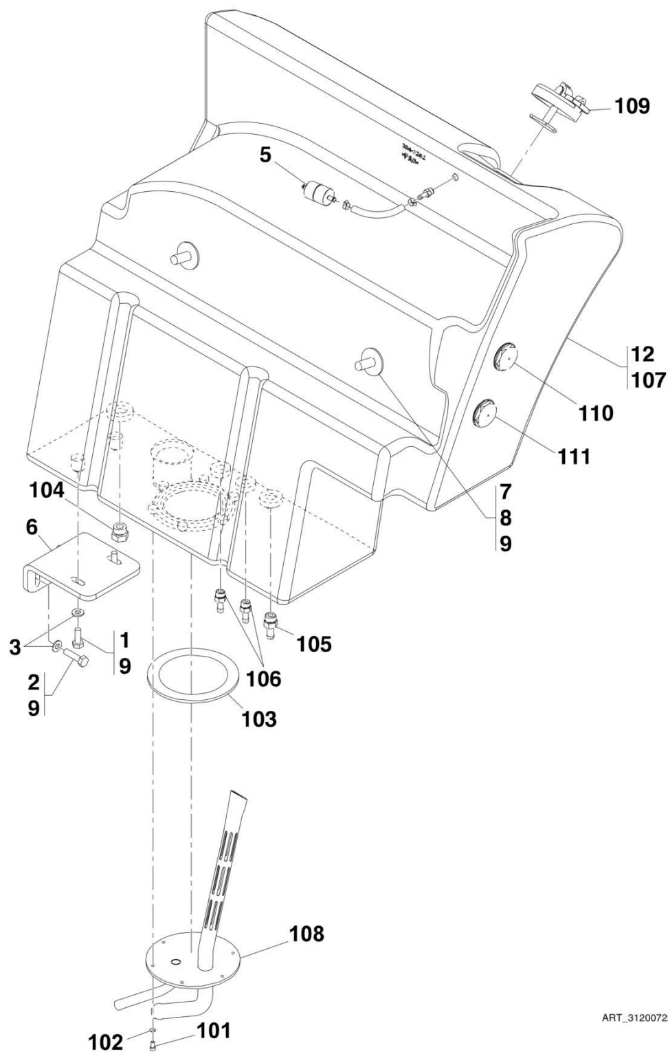
FIGURE 9-10. HYDRAULIC TANK
