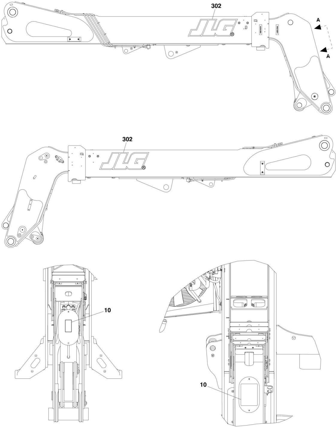
VIEW A-A (3706PS, 3707PS, 33.7, 37.6 & 37.7)
