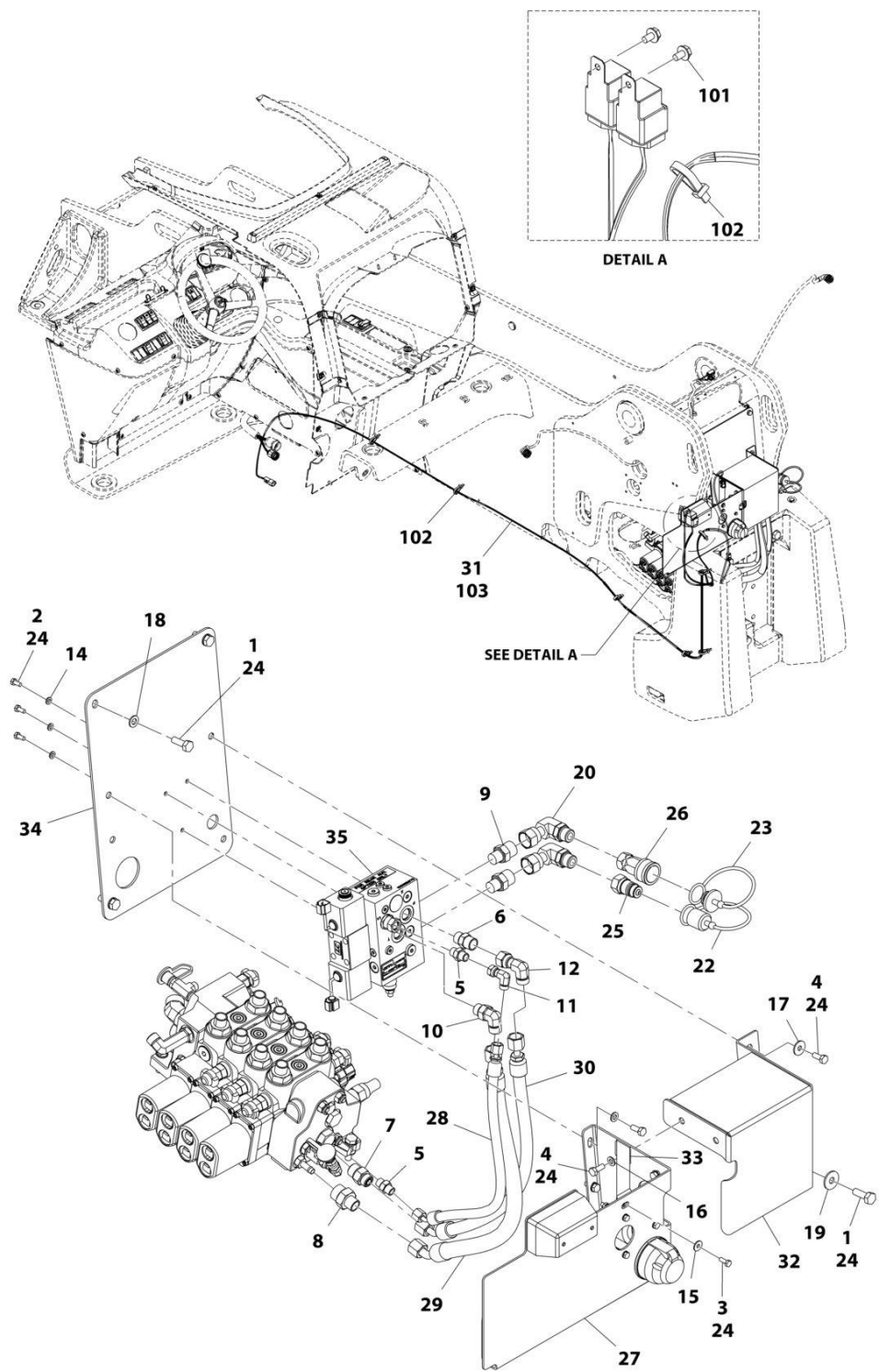
FIGURE 8-14. TRAILER BRAKES (33.7,37.6,37.7,3706PS,3707PS)
