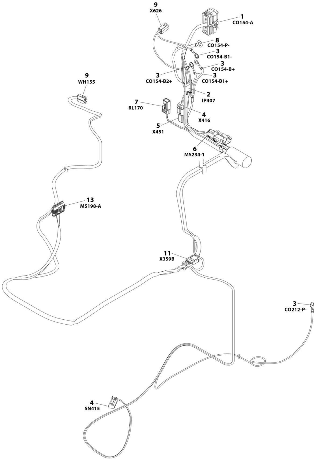
FIGURE 8-30. GENERATOR HARNESS
