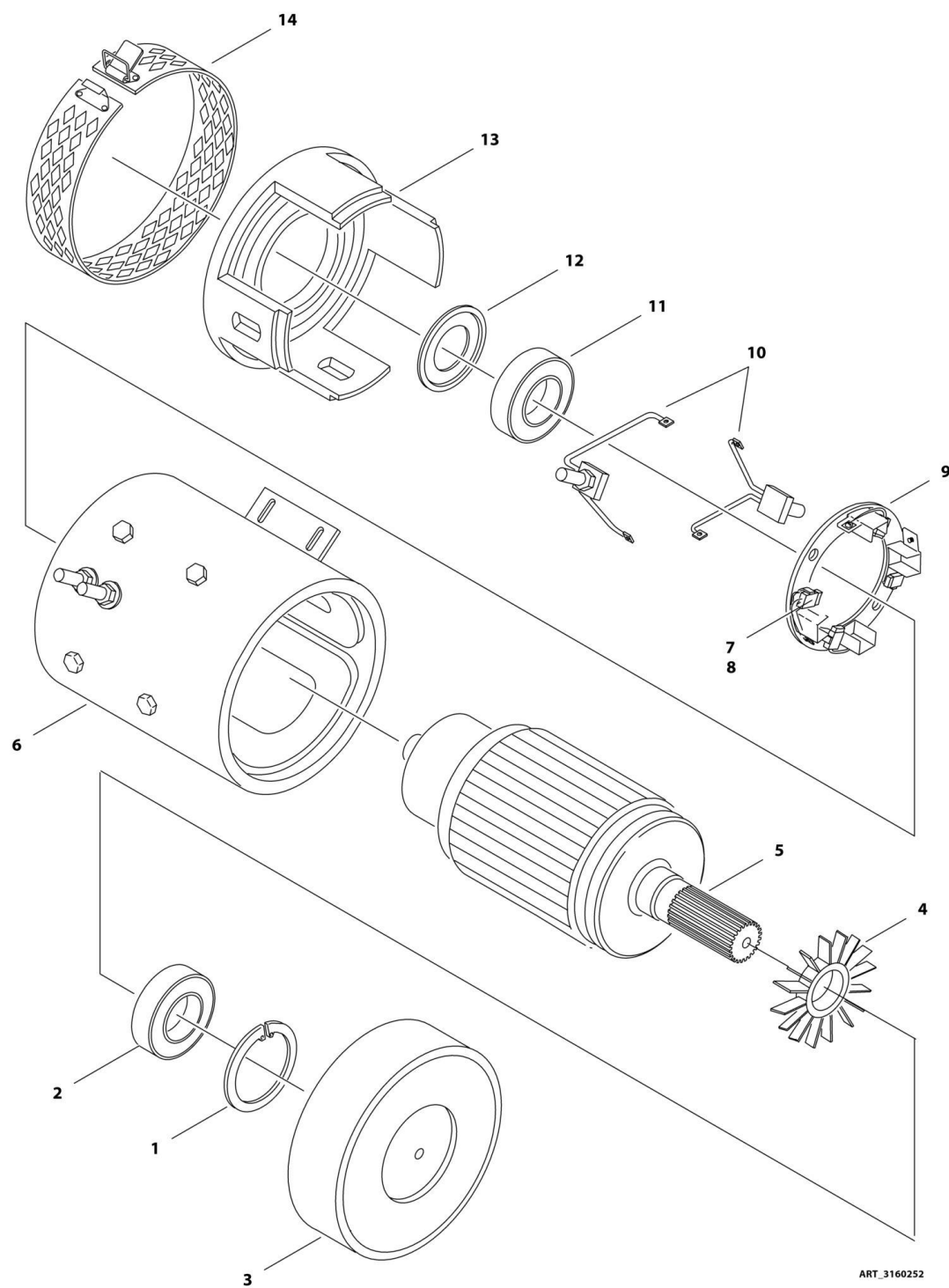
FIGURE 2-7. HYDRAULIC PUMP MOTOR ASSEMBLY
