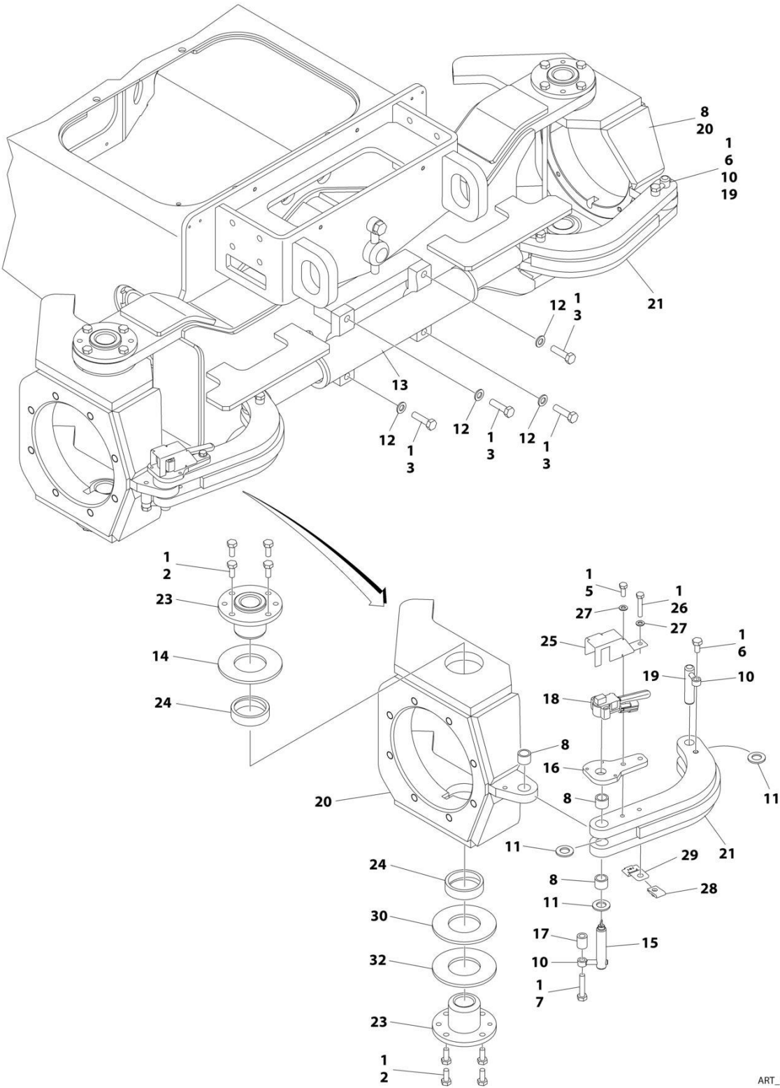
FIGURE 1-1. STEERING INSTALLATION
