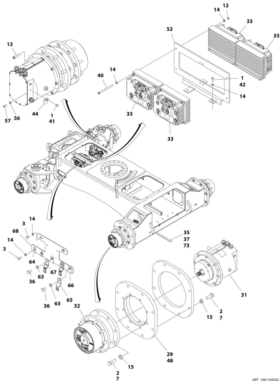
FIGURE 1-5. DRIVE INSTALLATION
