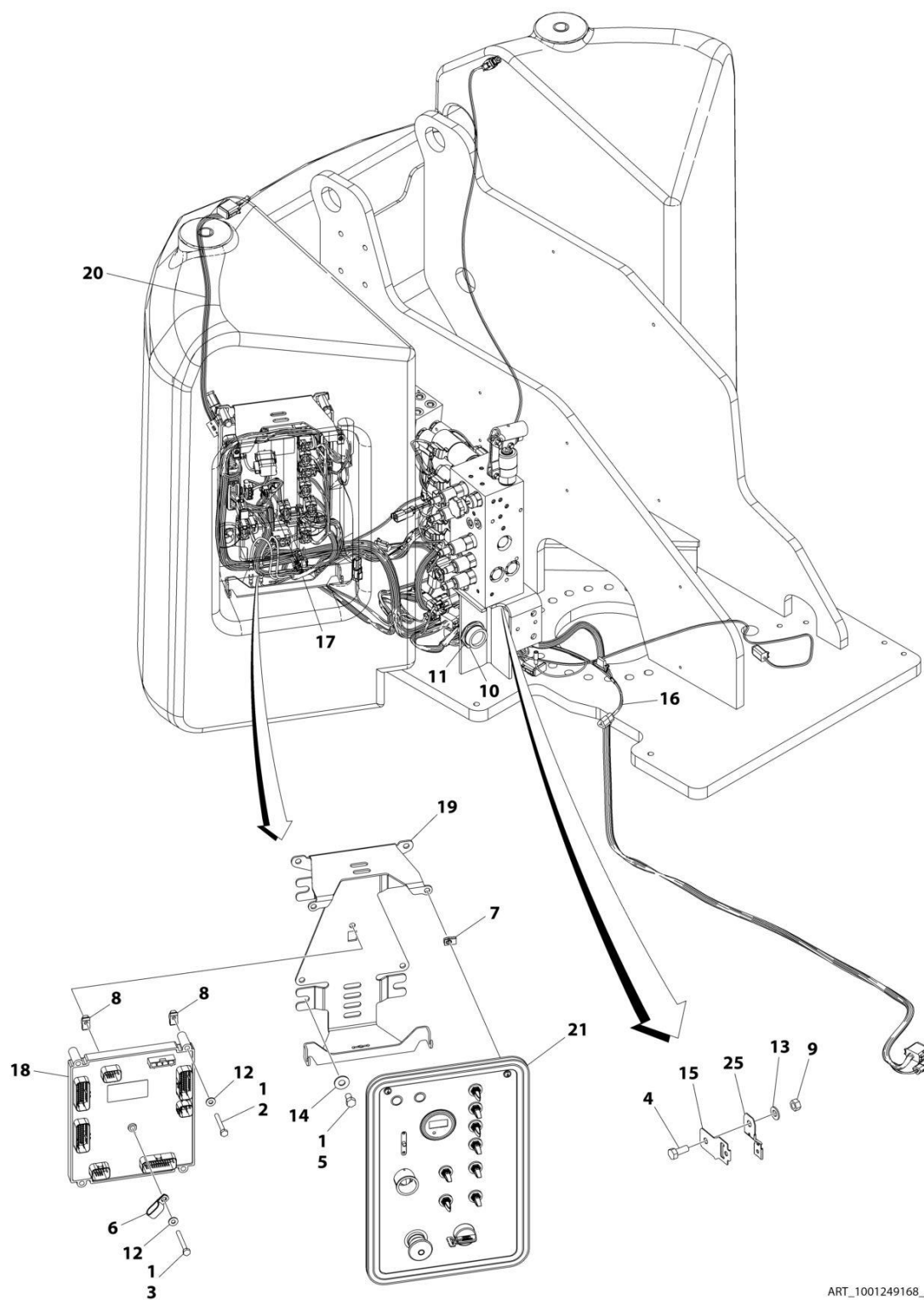
FIGURE 2-15. GROUND CONTROL BOX INSTALLATION (CE & UK CA SPEC) (E400AJPNARROW)
