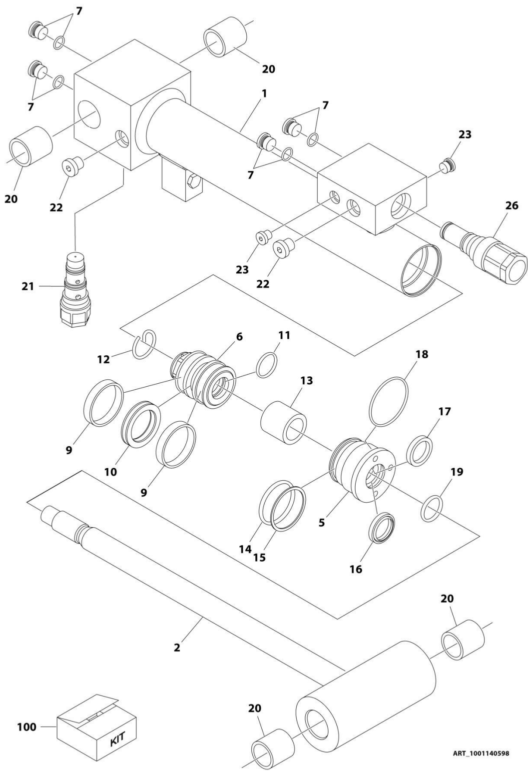
FIGURE 5-1. LEVEL (PLATFORM SLAVE) CYLINDER ASSEMBLY (E400ANARROW)
