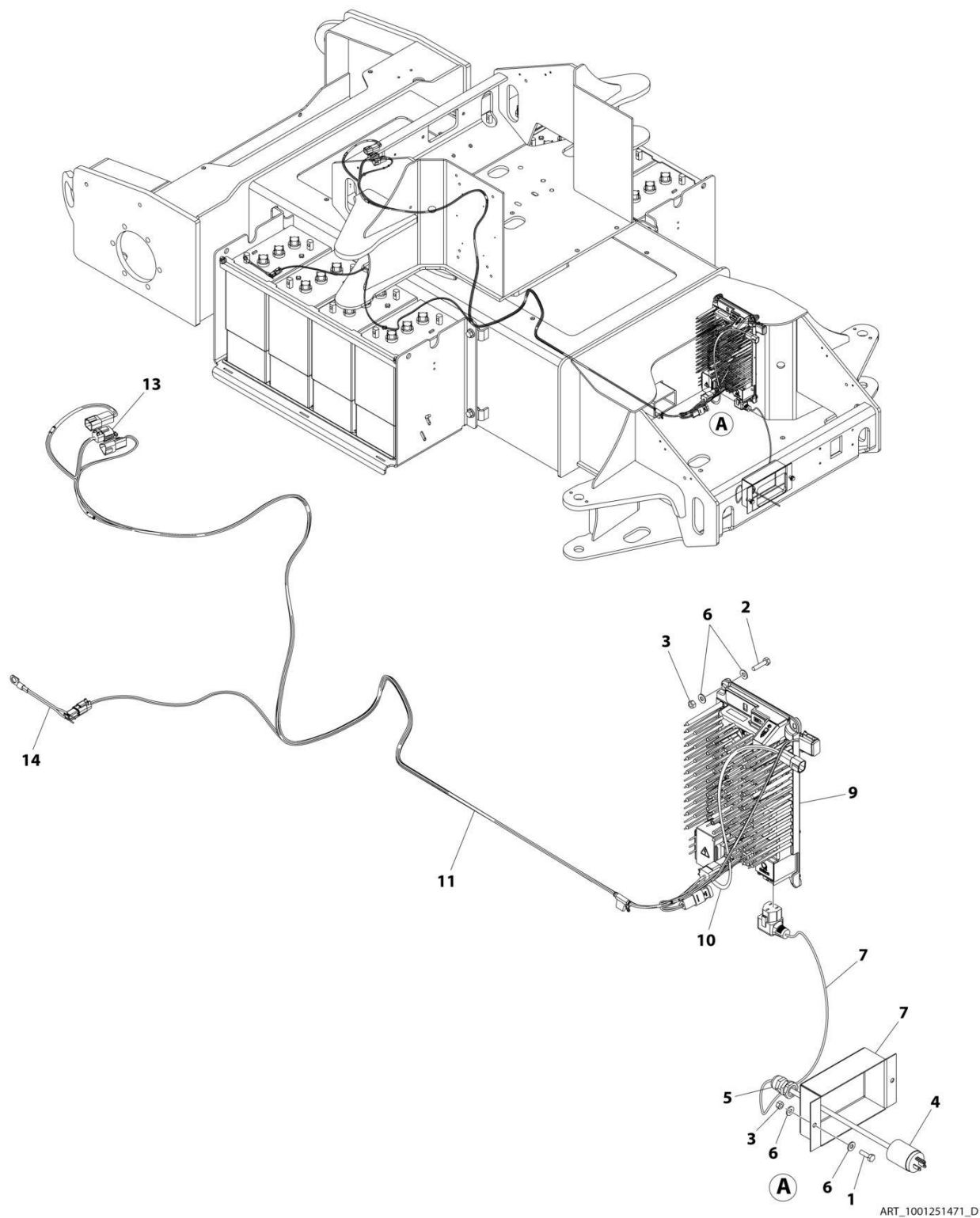
FIGURE 1-22. BATTERY CHARGER INSTALLATION (ALL SPECS EXCEPT AUSTRALIAN, CE & UK CA SPECS)
