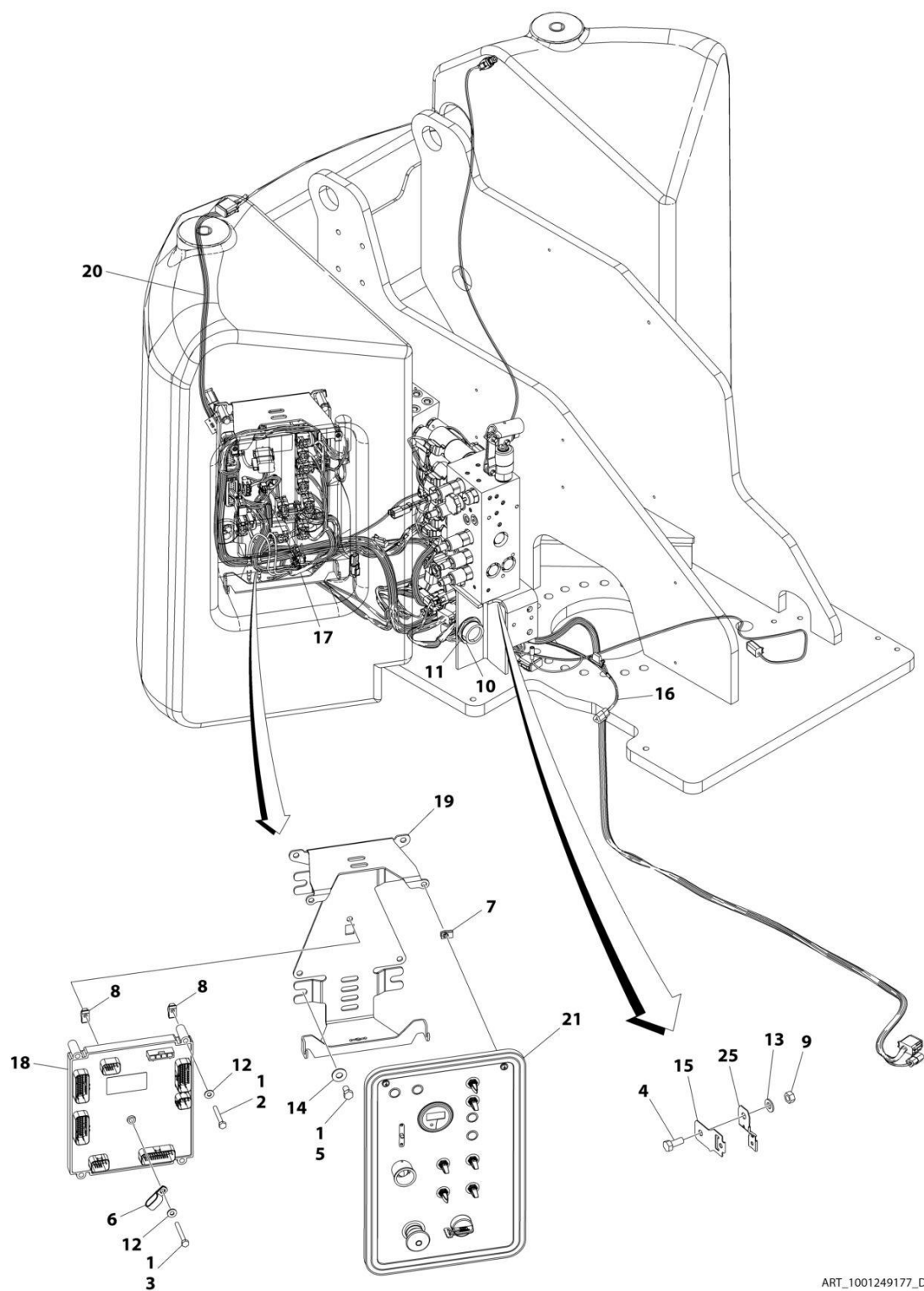
FIGURE 2-13. GROUND CONTROL BOX INSTALLATION (CE & UK CA SPEC) (E400ANARROW)
