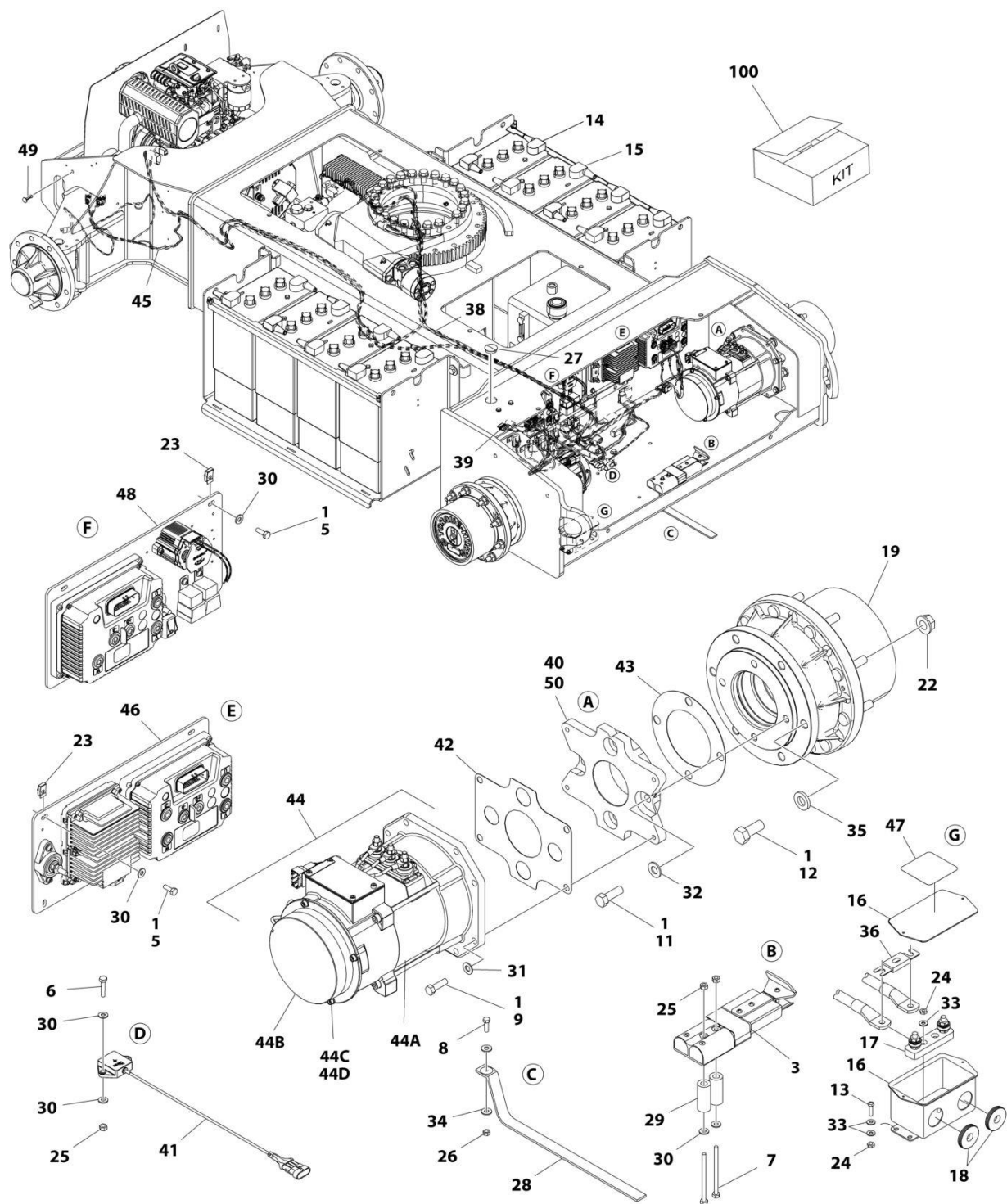
FIGURE 1-5. DRIVE INSTALLATION - UL SPECS
