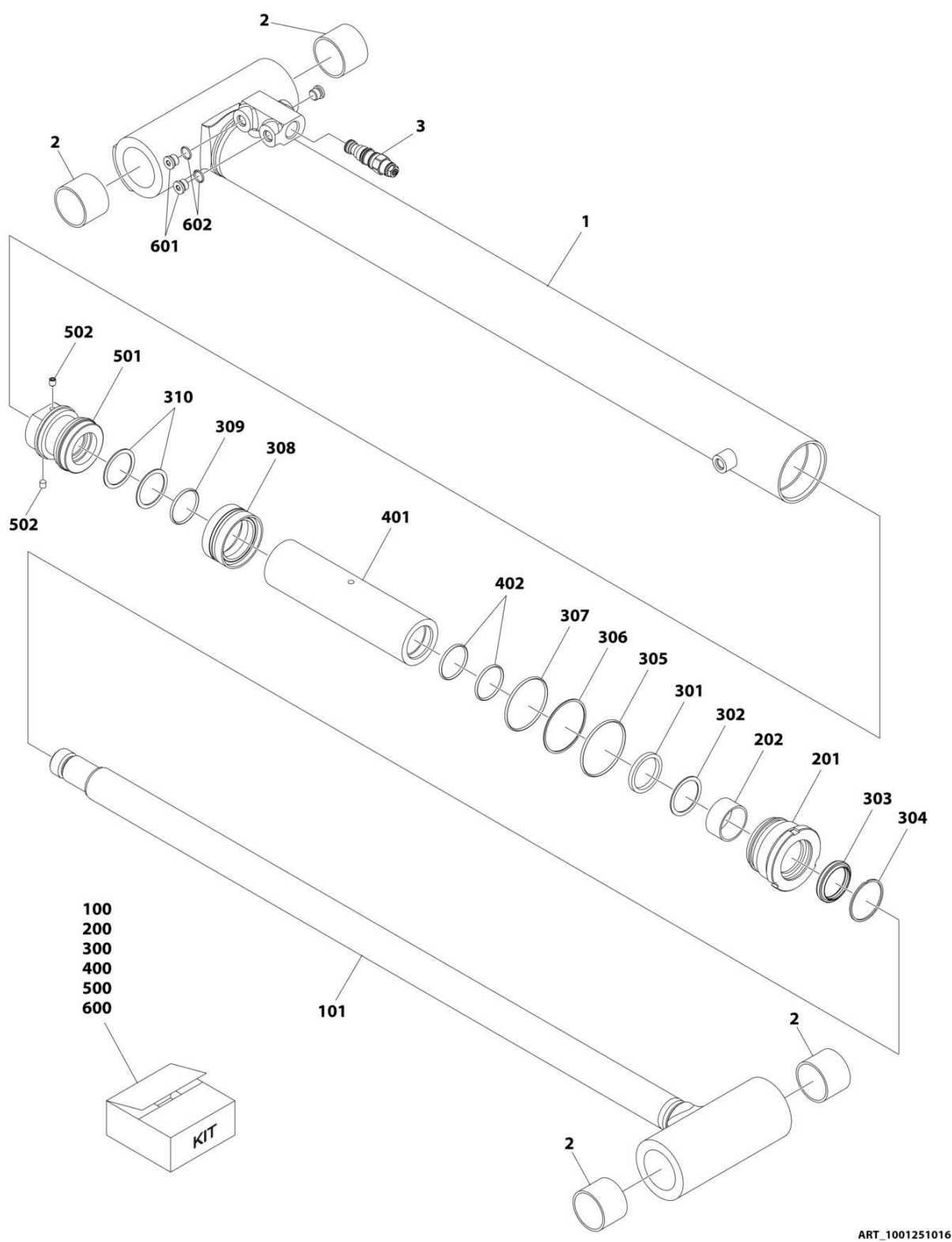
FIGURE 5-9. LIFT CYLINDER - UPPER (E400AJPNARROW)
