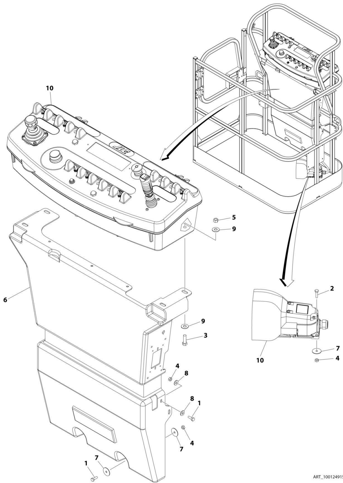
FIGURE 4-7. PLATFORM CONSOLE AND FOOTSWITCH INSTALLATION - NON-UL LISTED (ALL SPESC EXCEPT AUSTRALIAN AND UL SPECS) (E400ANARROW)
