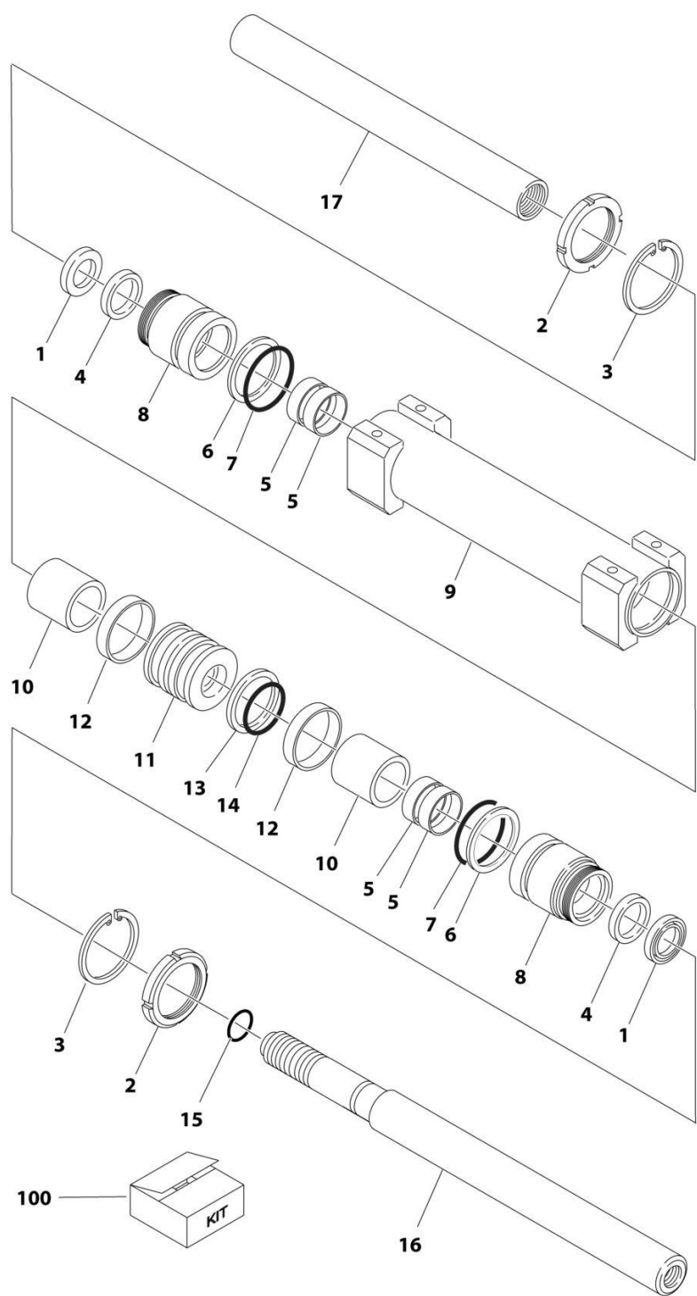
FIGURE 5-12. STEER CYLINDER ASSEMBLY
