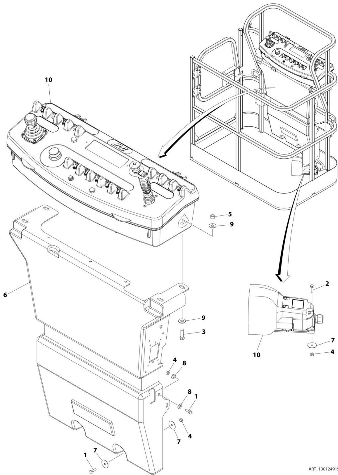
FIGURE 4-10. PLATFORM CONSOLE AND FOOTSWITCH INSTALLATION - UL LISTED (ALL SPECS EXCEPT AUSTRALIAN, CE, JAPANESE & UK CA SPECS) (E400AJPNARROW)
