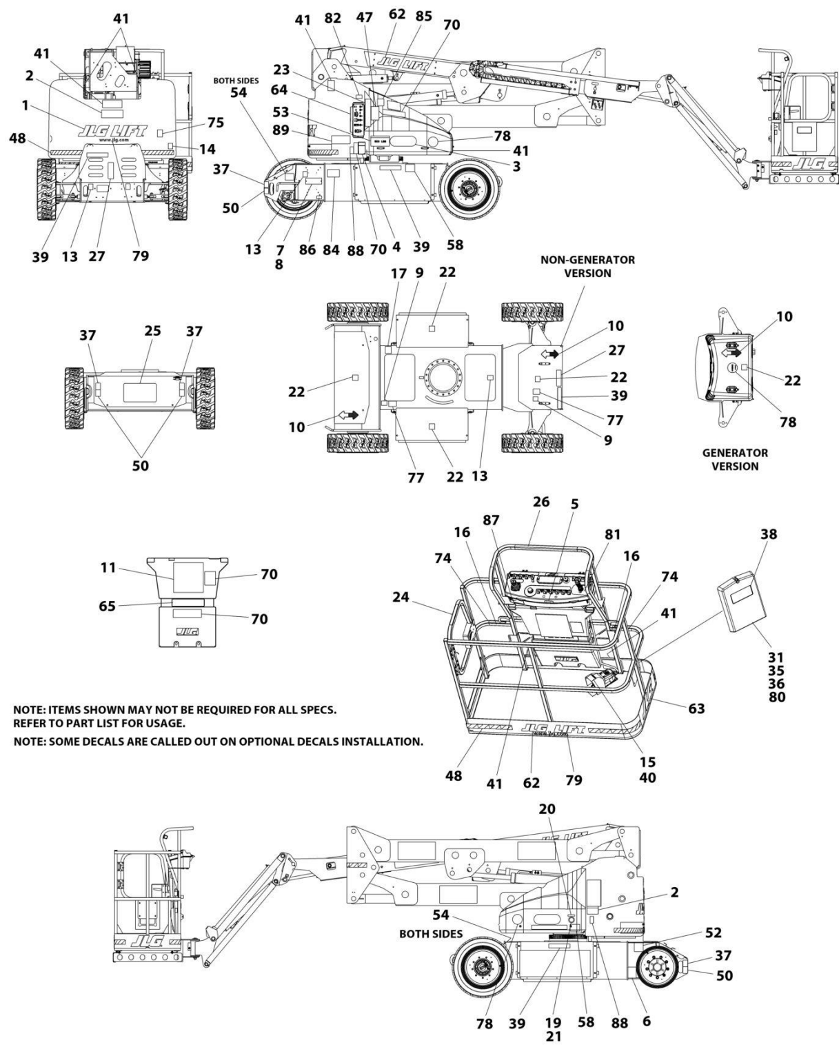
FIGURE 8-8. DECAL INSTALLATION - SPANISH/ENGLISH SPECS
