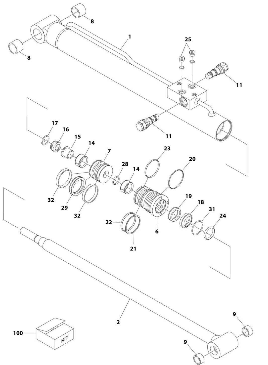
FIGURE 5-3. LIFT CYLINDER ASSEMBLY - JIB (E400AJPNARROW)
