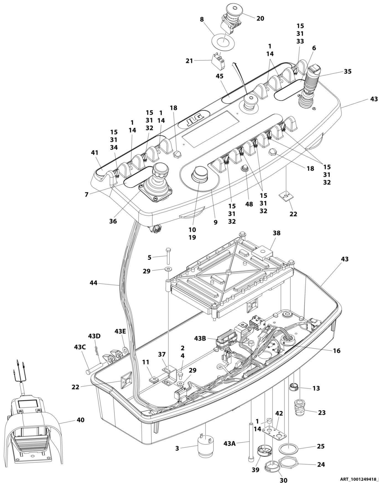
FIGURE 4-14. PLATFORM CONSOLE ASSEMBLY - NON-UL LISTED (ALL SPECS EXCEPT UL SPECS) (E400AJPNARROW)
