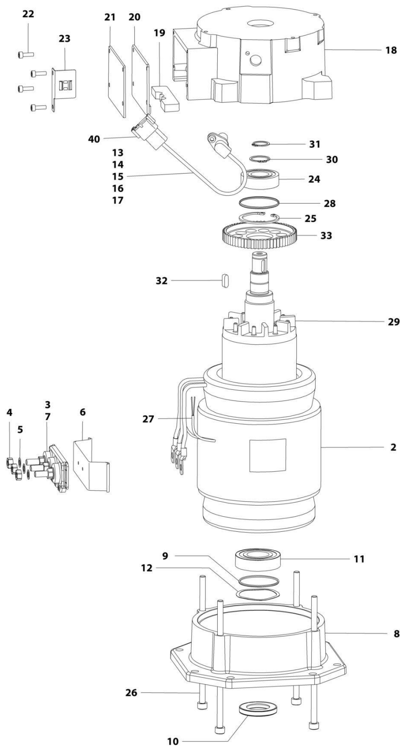
FIGURE 1-7. DRIVE MOTOR ASSEMBLY
