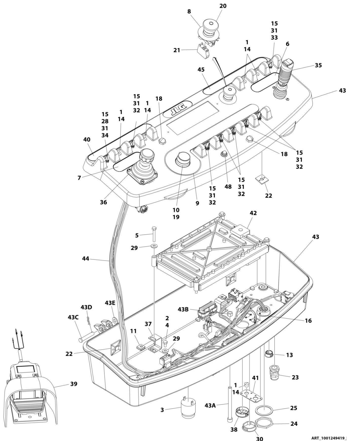
FIGURE 4-13. PLATFORM CONSOLE ASSEMBLY - UL LISTED (ALL SPECS EXCEPT AUSTRALIAN, CE, JAPANESE & UK CA SPECS)
