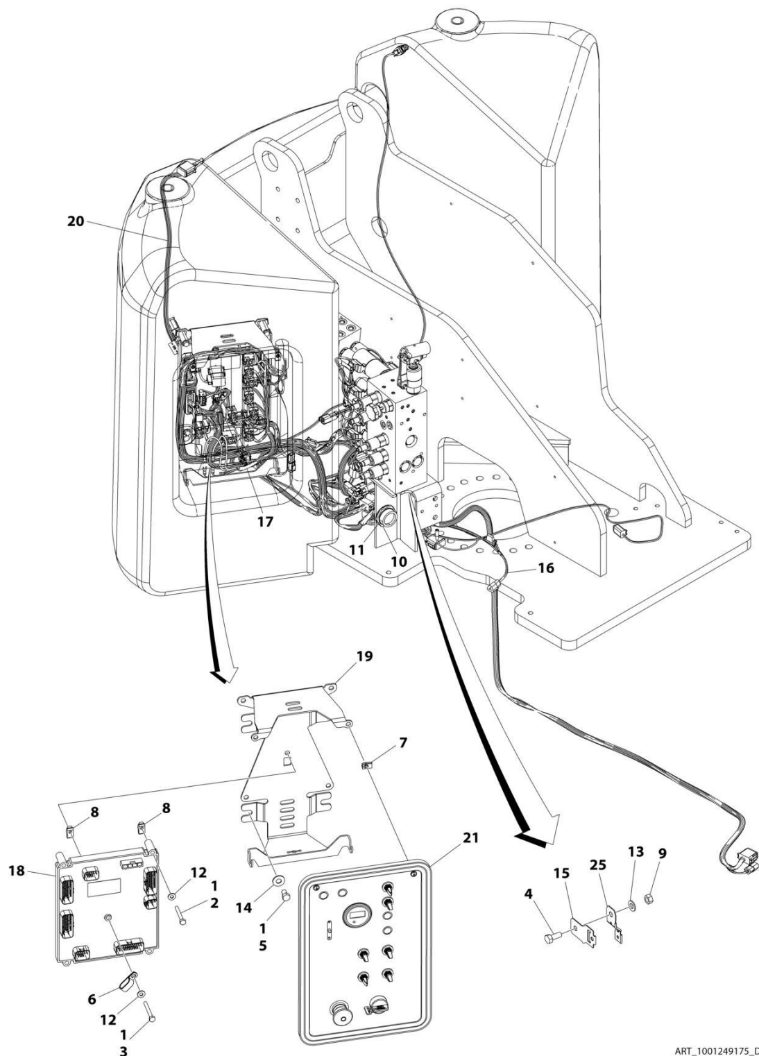
FIGURE 2-12. GROUND CONTROL BOX INSTALLATION (ALL SPECS EXCEPT AUSTRALIAN, CE & UK CA SPECS) (E400ANARROW)
