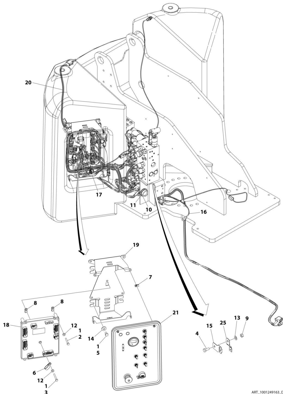
FIGURE 2-14. GROUND CONTROL BOX INSTALLATION (ALL SPECS EXCEPT CE & UK CA SPEC) (E400AJPNARROW)
