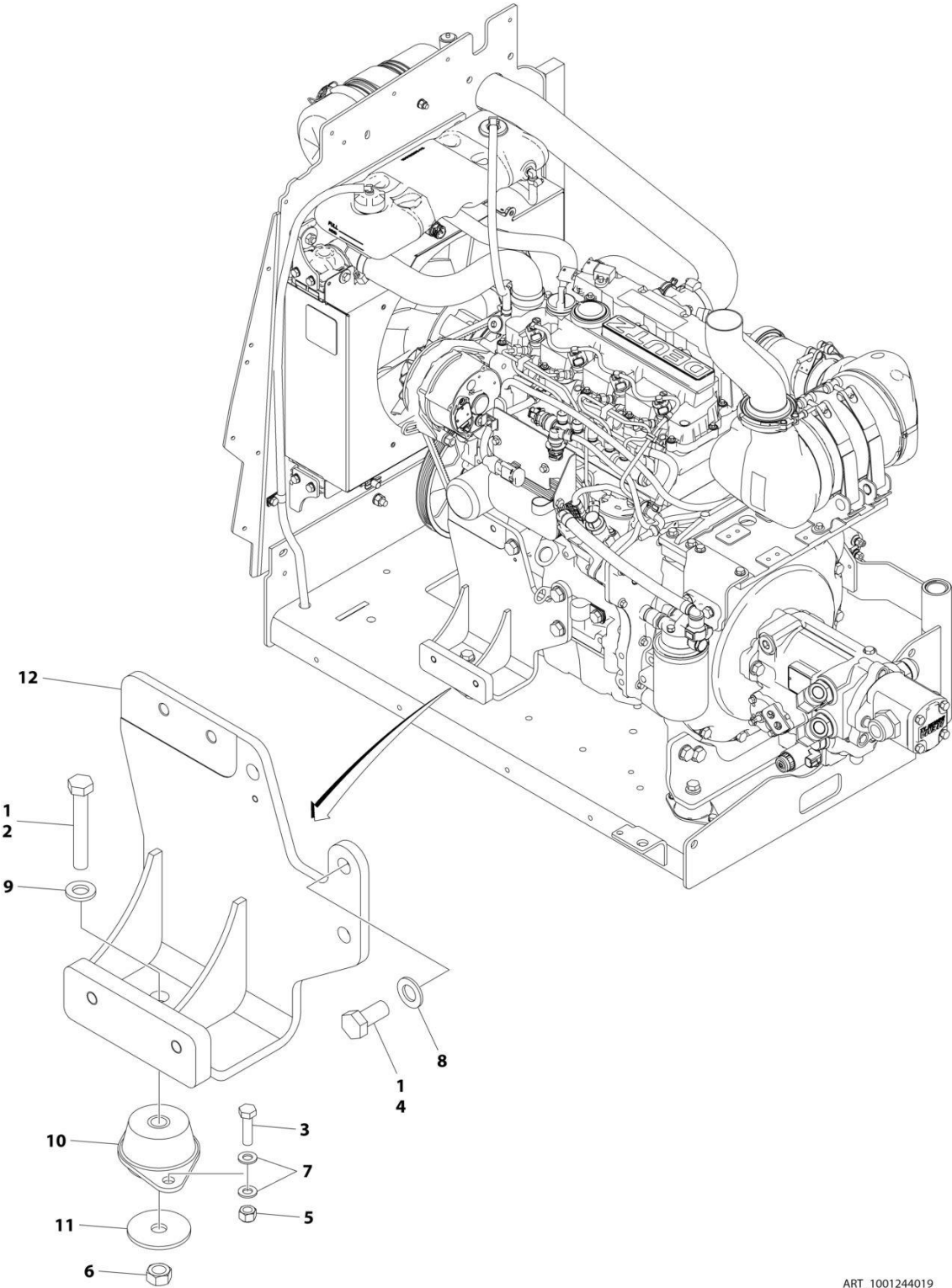
FIGURE 3-26. MOTOR MOUNT INSTALLATION - STAGE V ENGINE (WITHOUT GENERATOR)
