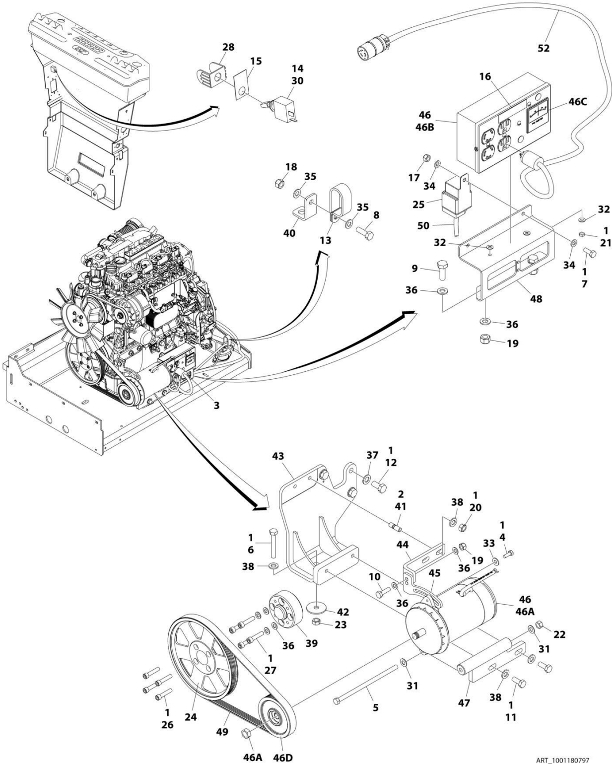
FIGURE 3-39. GENERATOR INSTALLATION - 2500W/60HZ (DEUTZ D2.9L4 ENGINE) (ANSI, ANSI EXPORT, CSA AND JAPAN SPECS)
