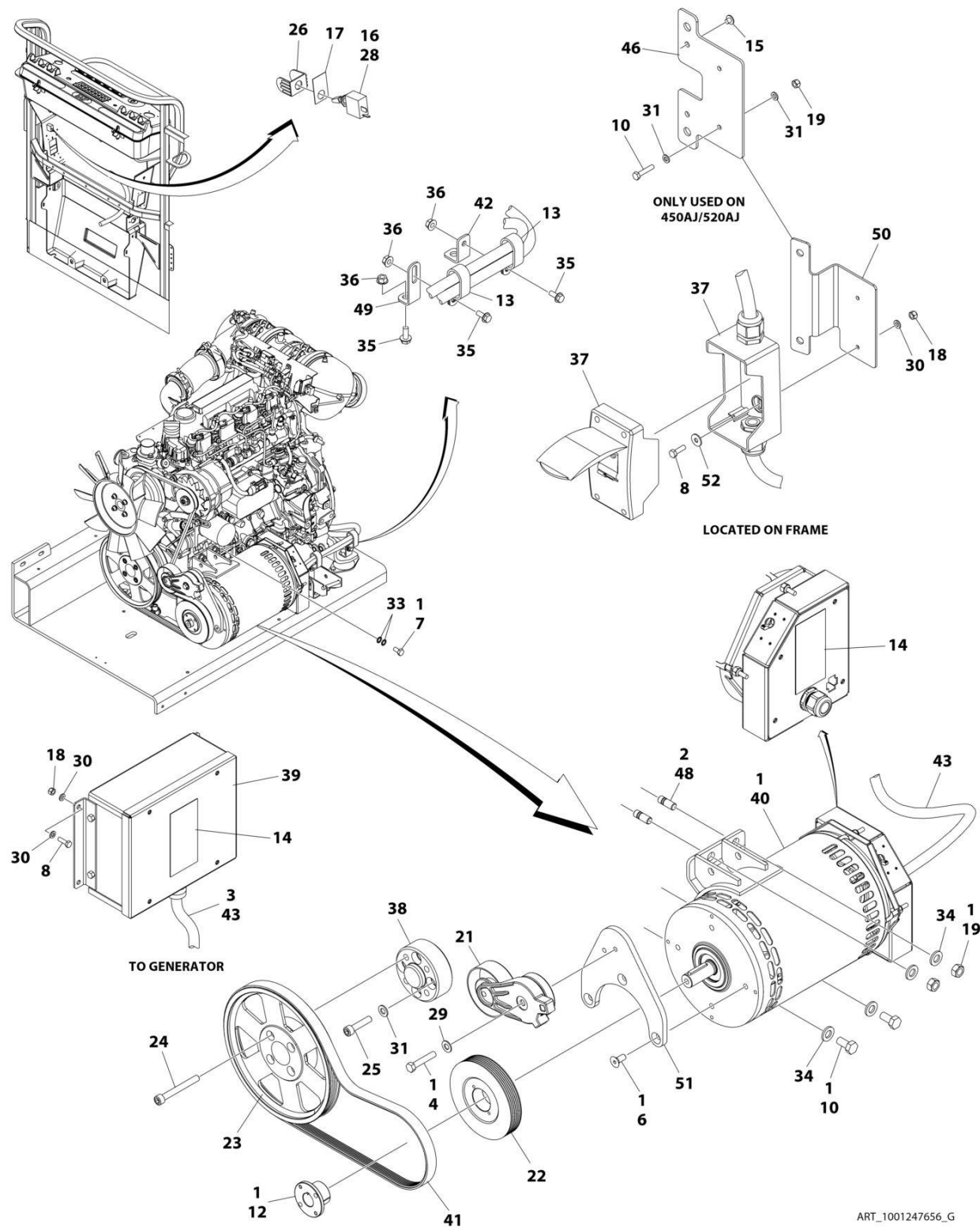
FIGURE 3-43. GENERATOR INSTALLATION - 4000W/50HZ (DEUTZ (STAGE V) ENGINE) (CE & UK CA SPEC)
