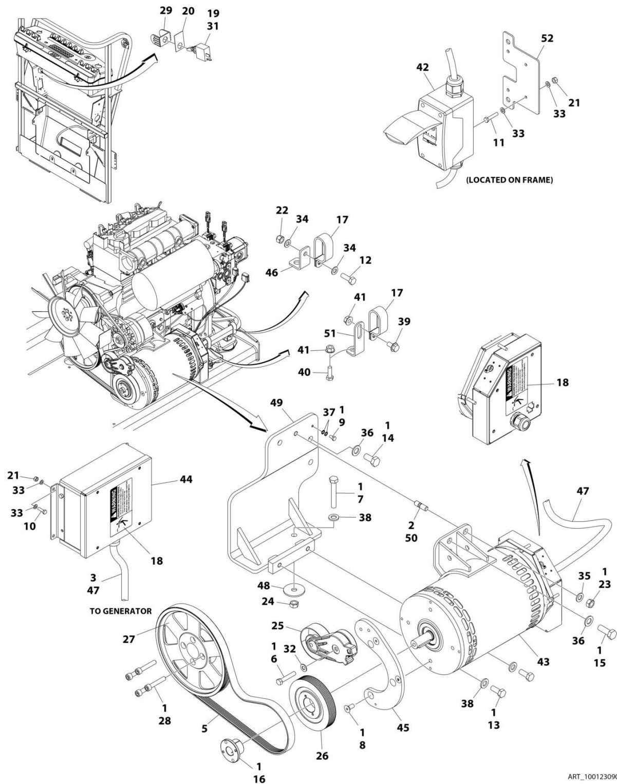
FIGURE 3-41. GENERATOR INSTALLATION - 4000W/50HZ (DEUTZ D2011 ENGINE) (ANSI EXPORT, CE & UK CA (LRC) SPECS)
