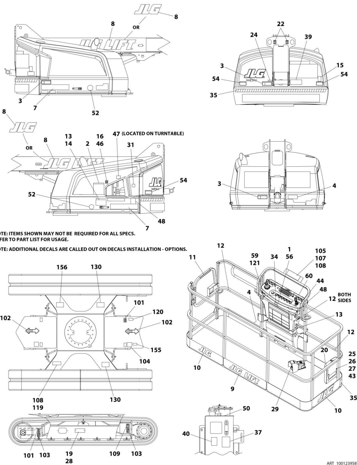
FIGURE 9-7. DECAL INSTALLATION - ANSI EXPORT - (JAPANESE SPECS) (400SC)
