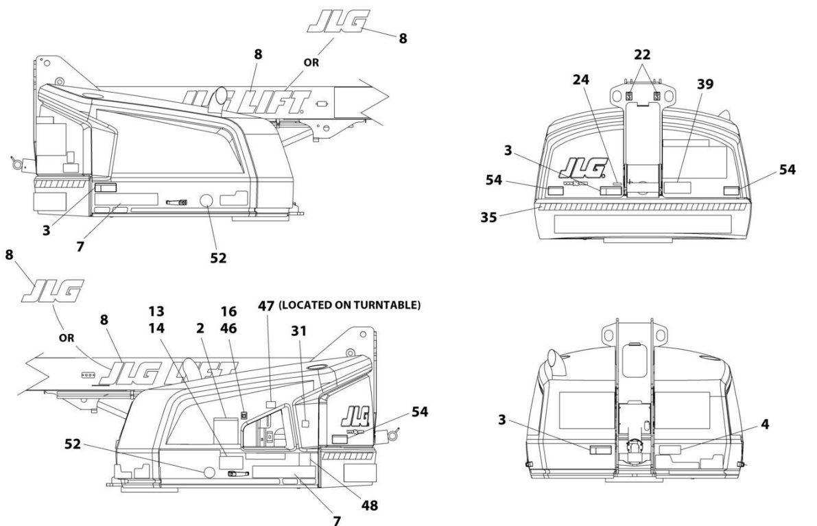
FIGURE 9-4. DECAL INSTALLATION - CE & UK CA SPEC (460SJC)
