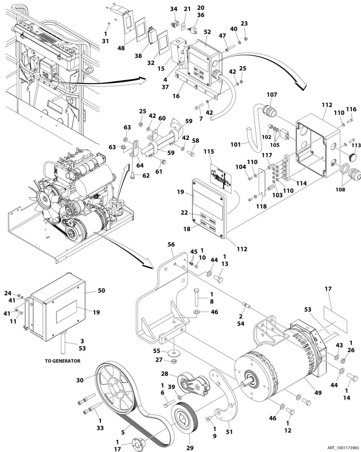
FIGURE 3-40. GENERATOR INSTALLATION - 4000W/60HZ (DEUTZ D2011 ENGINE) (ANSI EXPORT SPEC)
