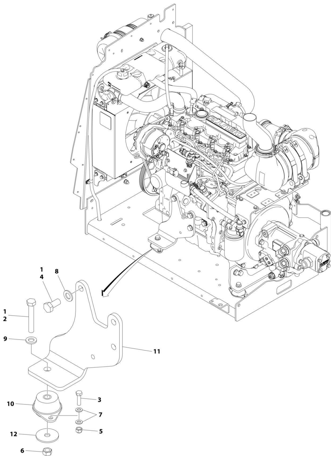
FIGURE 3-27. MOTOR MOUNT INSTALLATION - STAGE V ENGINE (WITH GENERATOR)
