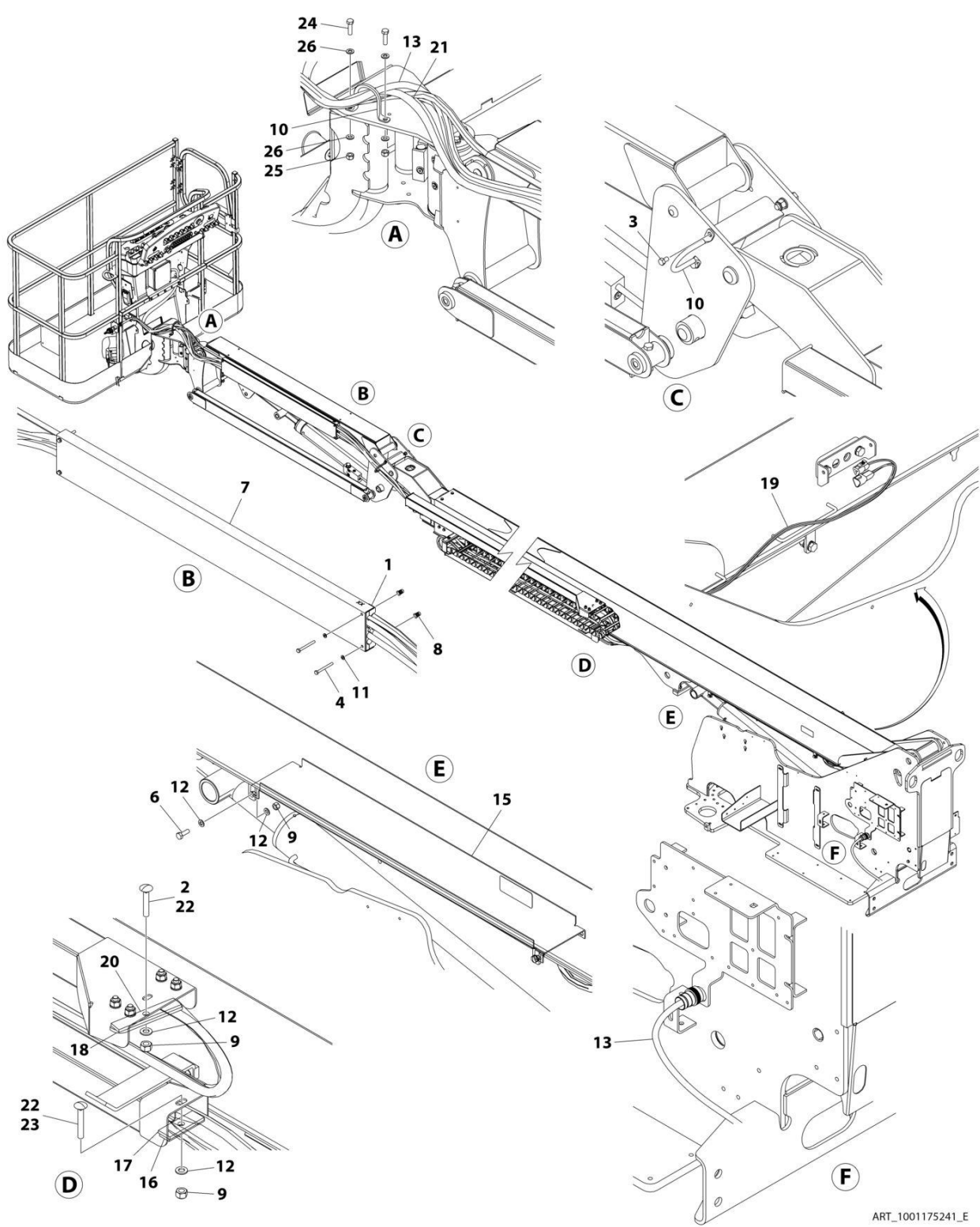
FIGURE 8-33. CABLES AND CLAMPS INSTALLATION -WITH 4000W GENERATOR 60HZ (460SJC)
