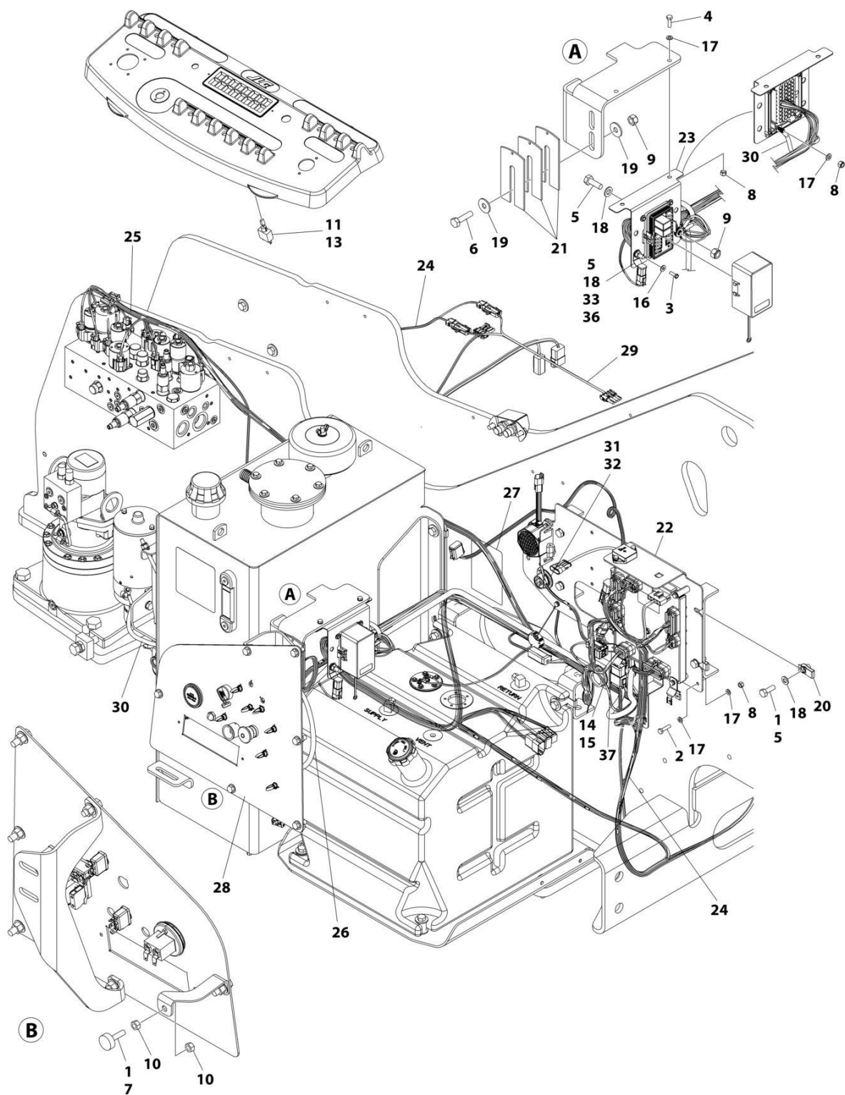
FIGURE 2-20. ELECTRICAL INSTALLATION - WITH DEUTZ (STAGE V) ENGINE (460SJC)
