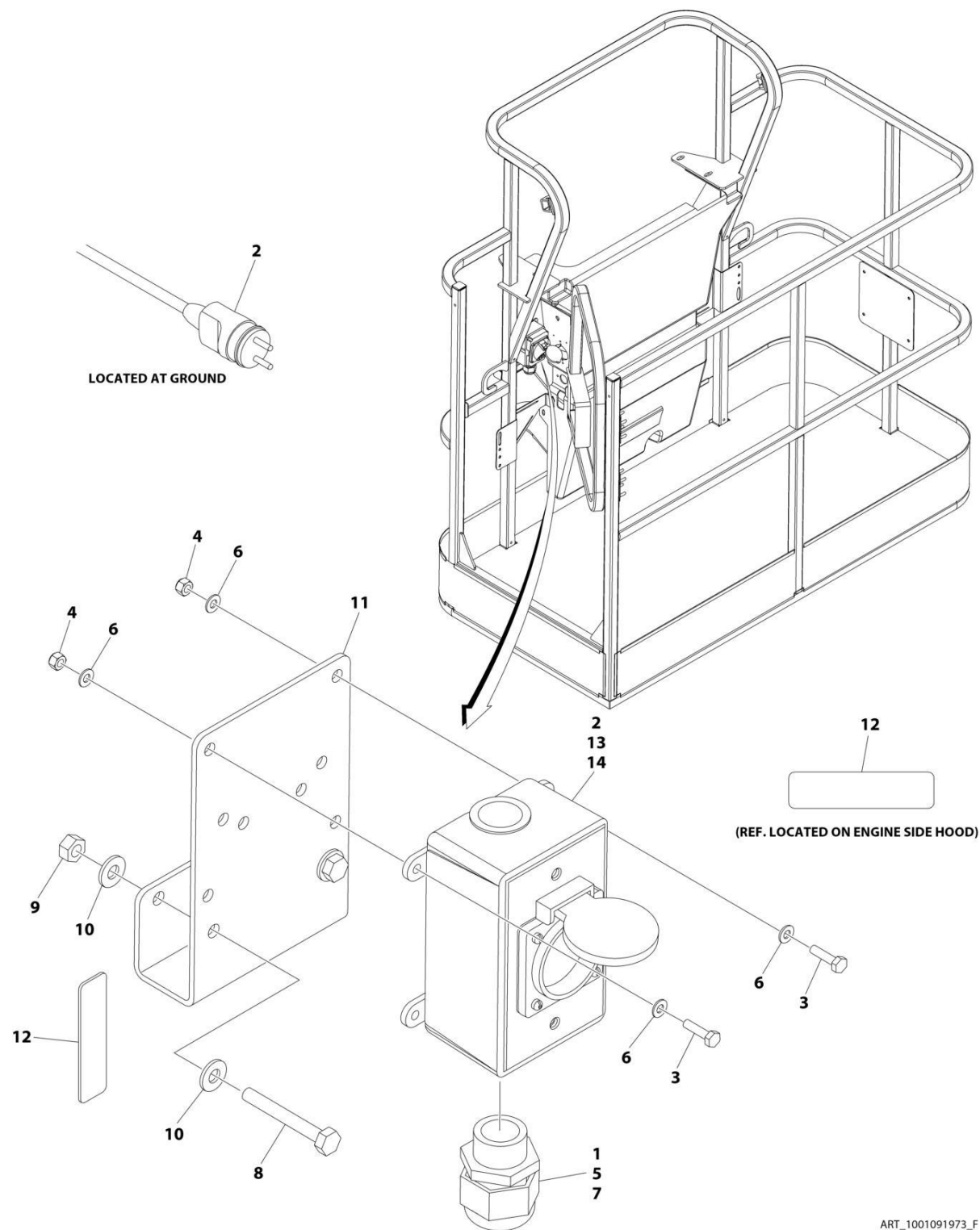
FIGURE 8-6. AC BOX AT PLATFORM - 220V CEE7 2IN X 4IN POST GROUND (CE & UK CA SPEC WITHOUT GENERATOR)
