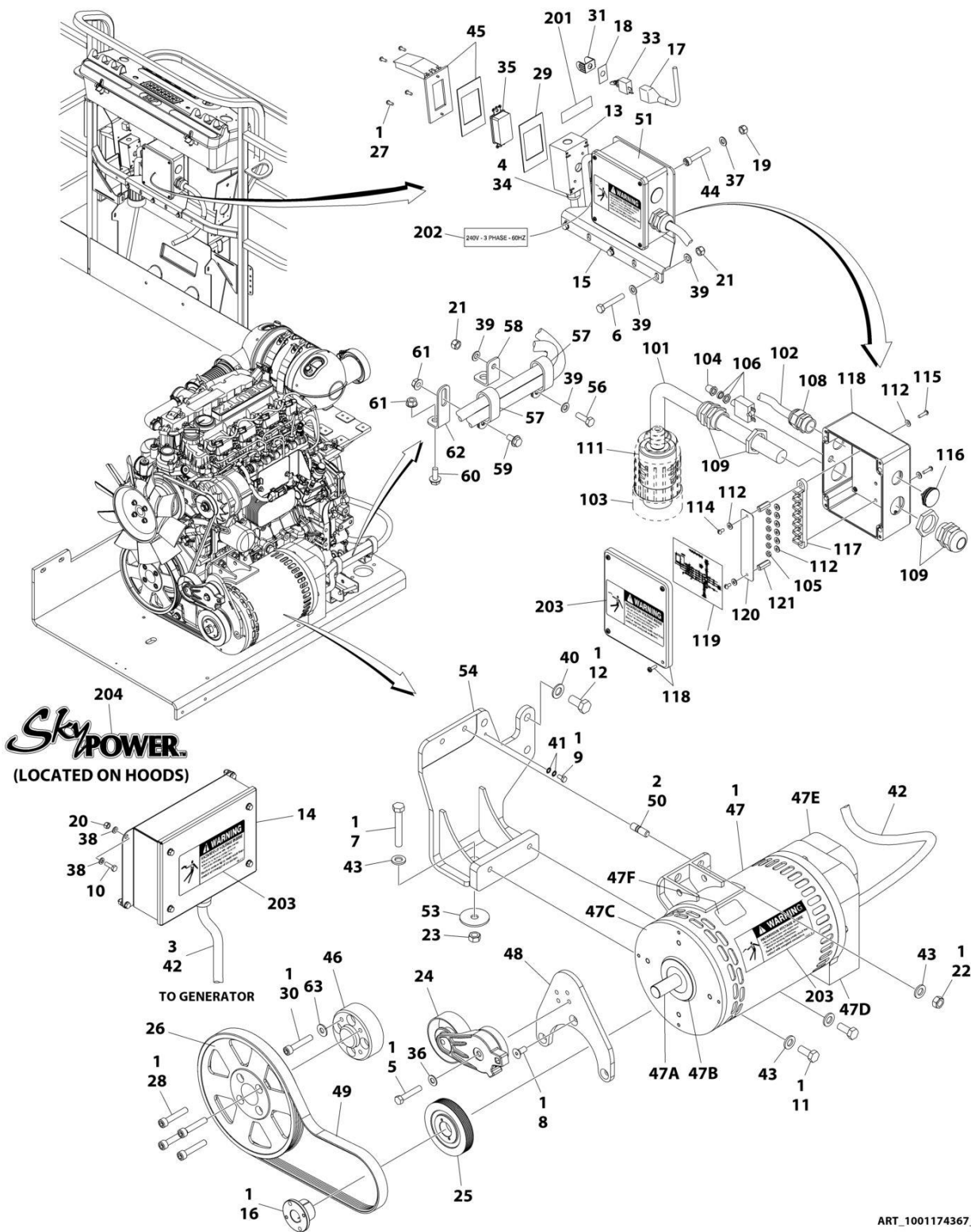
FIGURE 3-46. GENERATOR INSTALLATION - 7500W/60HZ (DEUTZ D2.9L4) (ANSI, ANSI EXPORT, CSA AND JAPAN SPECS)
