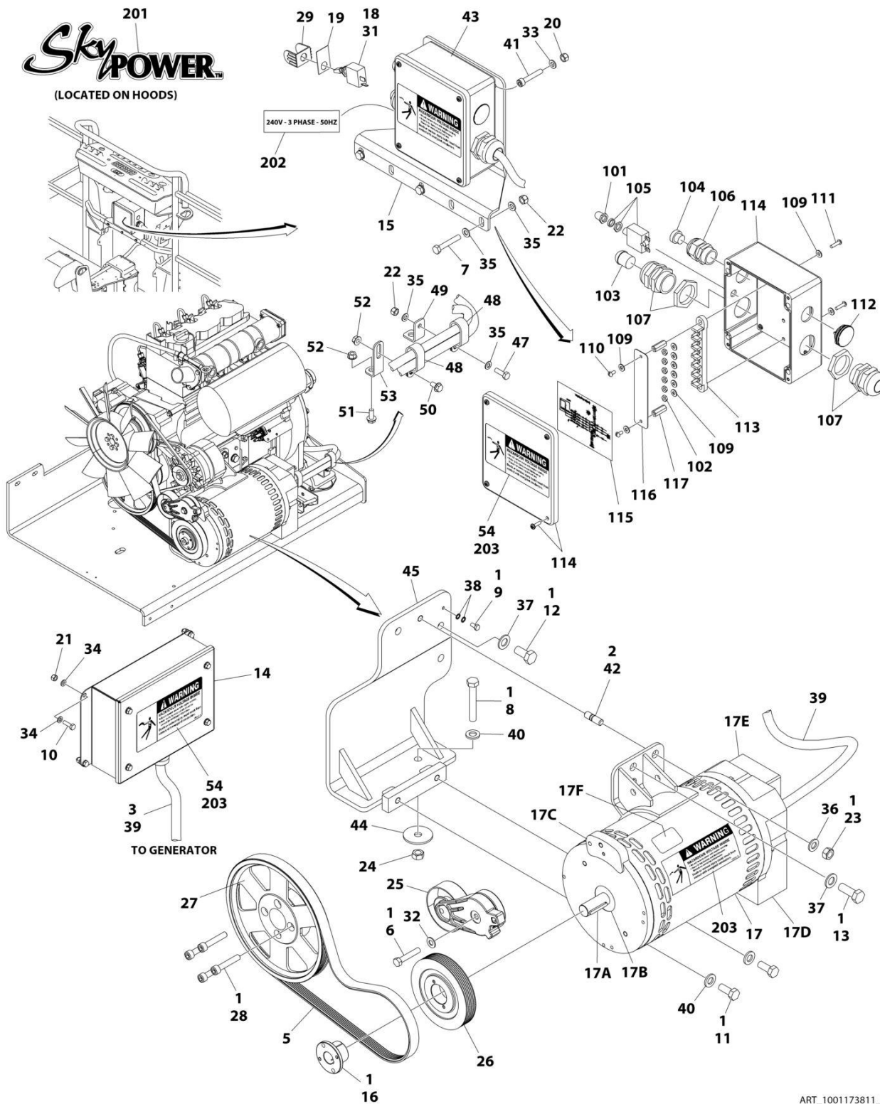
FIGURE 3-44. GENERATOR INSTALLATION - 7500W/50HZ (DEUTZ D2011 ENGINE) (ANSI EXPORT SPECS)
