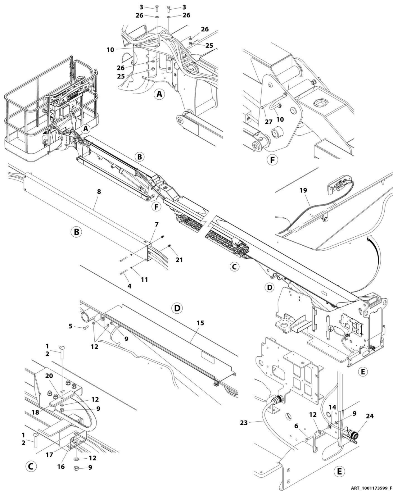
FIGURE 8-32. CABLES AND CLAMPS INSTALLATION - WITH 4000W GENERATOR 50HZ (460SJC)
