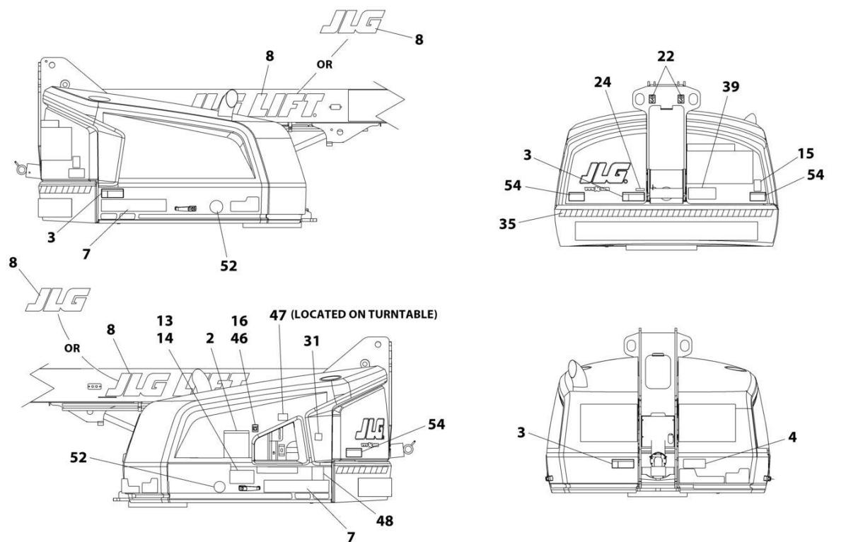
FIGURE 9-8. DECAL INSTALLATION - ANSI EXPORT - (JAPANESE SPECS) (460SJC)
