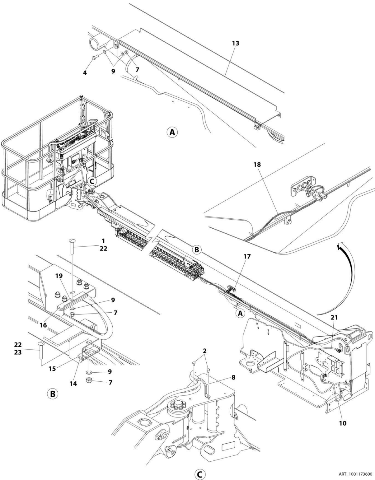
FIGURE 8-30. CABLES AND CLAMPS INSTALLATION -WITH 7500W GENERATOR (400SC)
