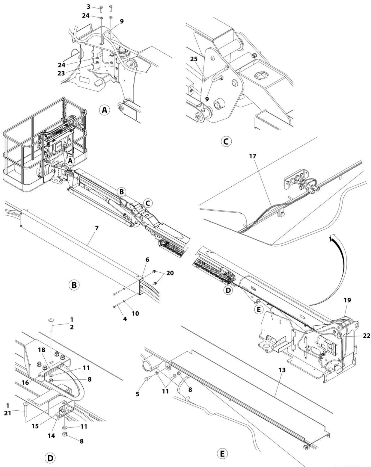
FIGURE 8-34. CABLES AND CLAMPS INSTALLATION - WITH 7500W GENERATOR (460SJC)
