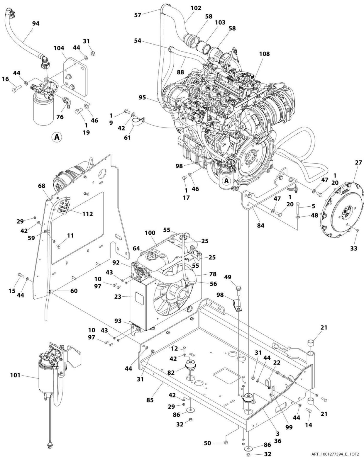
FIGURE 3-24. ENGINE ASSEMBLY - DEUTZ D2.9L4 (STAGE V) ENGINE (WITHOUT ARCTIC PACKAGE) (CE & UK CA SPECS)
