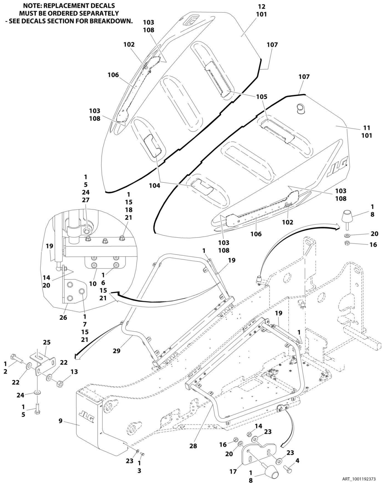
FIGURE 2-44. HOODS INSTALLATION
