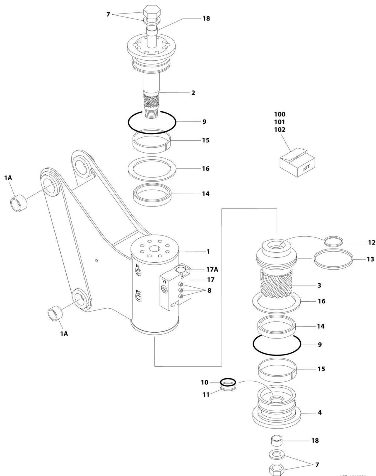
FIGURE 4-12. ROTATOR ASSEMBLY - PLATFORM ROTATE (EC600SJP/H600SJP) (E600JP,EC600SJP,H600SJP,M600JP)
