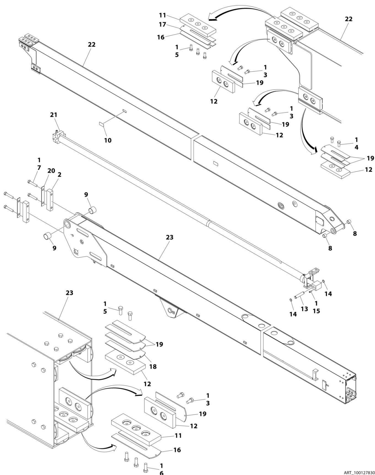
FIGURE 4-6. BOOM ASSEMBLY (MACHINES WITH SN STARTING WITH B3) (EC600SJ)
