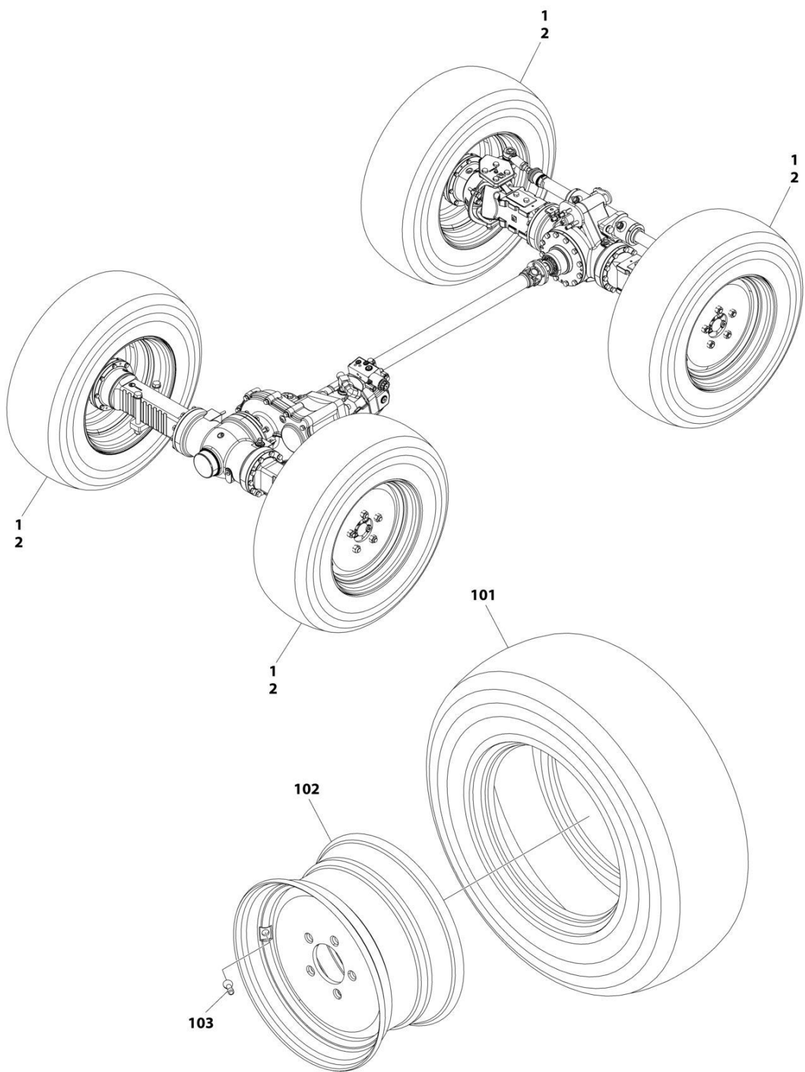
FIGURE 4-20. TIRE INSTALLATION - TURF
