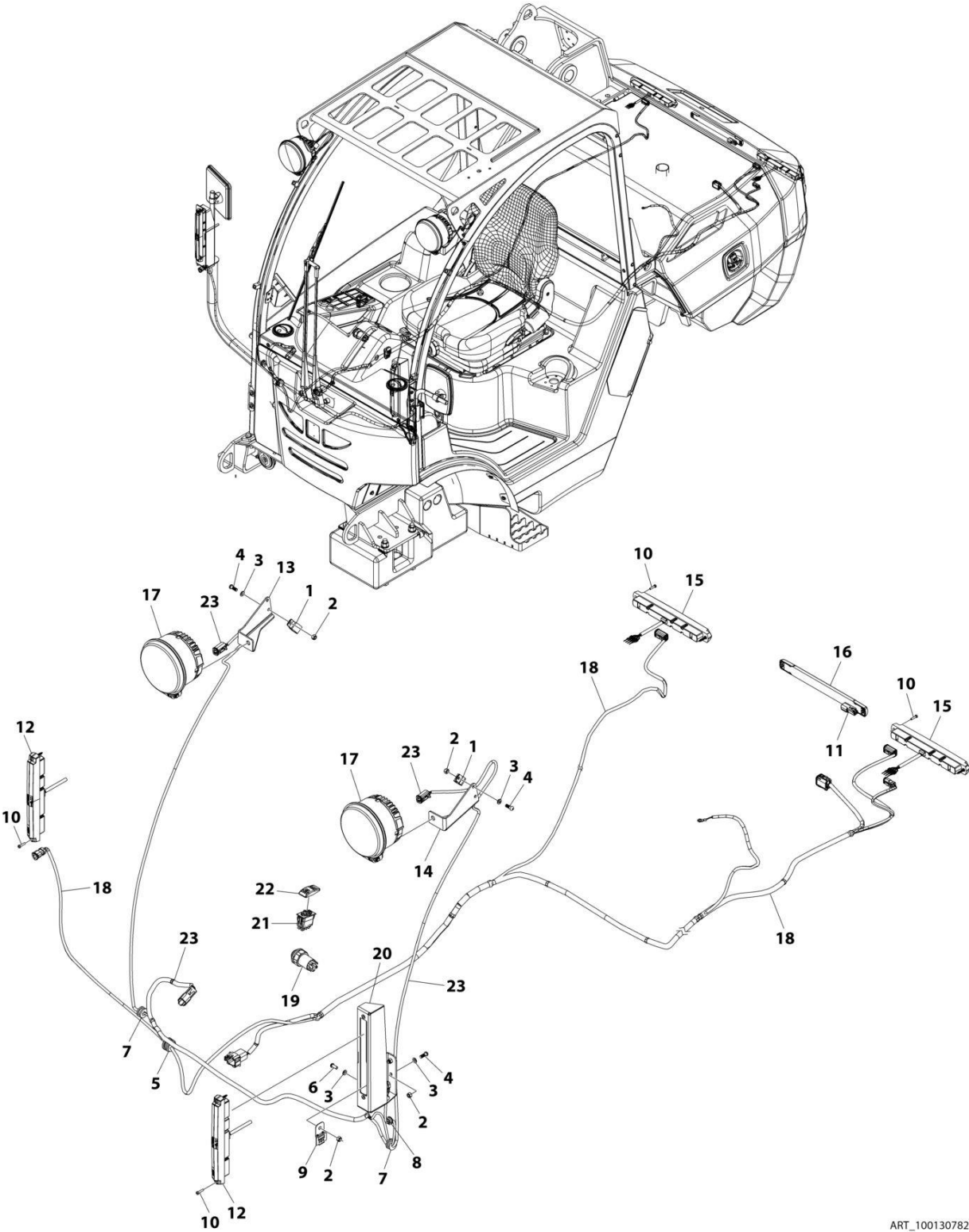
FIGURE 9-17. ROAD LIGHTS INSTALLATION
