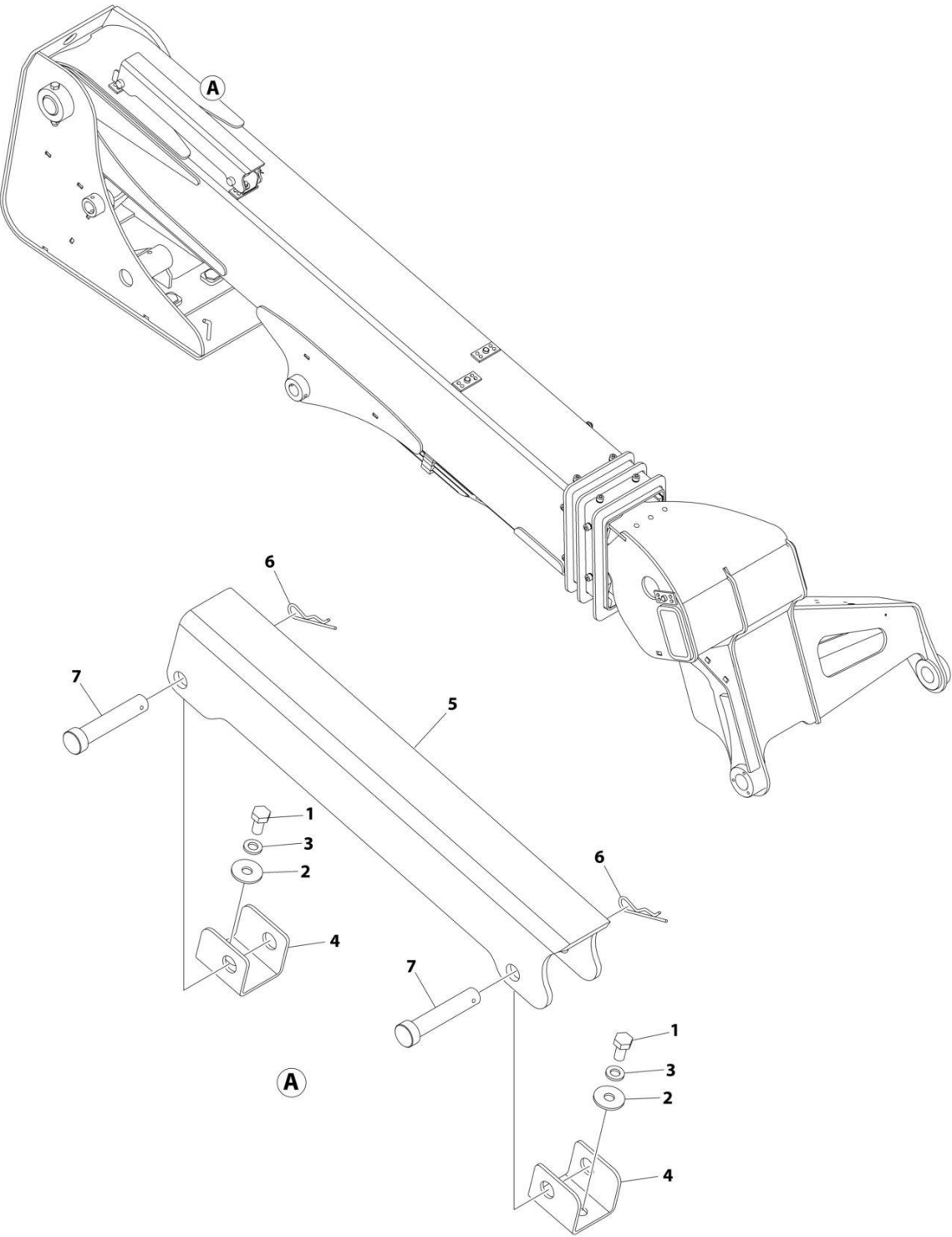
FIGURE 2-5. BOOM PROP INSTALLATION
