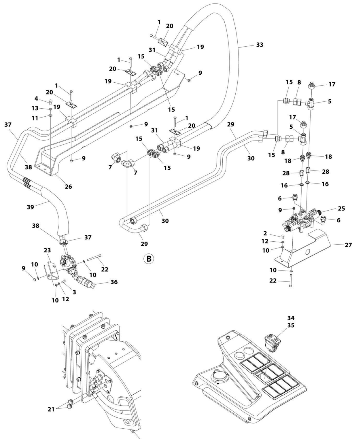
FIGURE 7-2. AUXILIARY HYDRAULICS INSTALLATION - HYDRAULIC COUPLER (HIGH FLOW)
