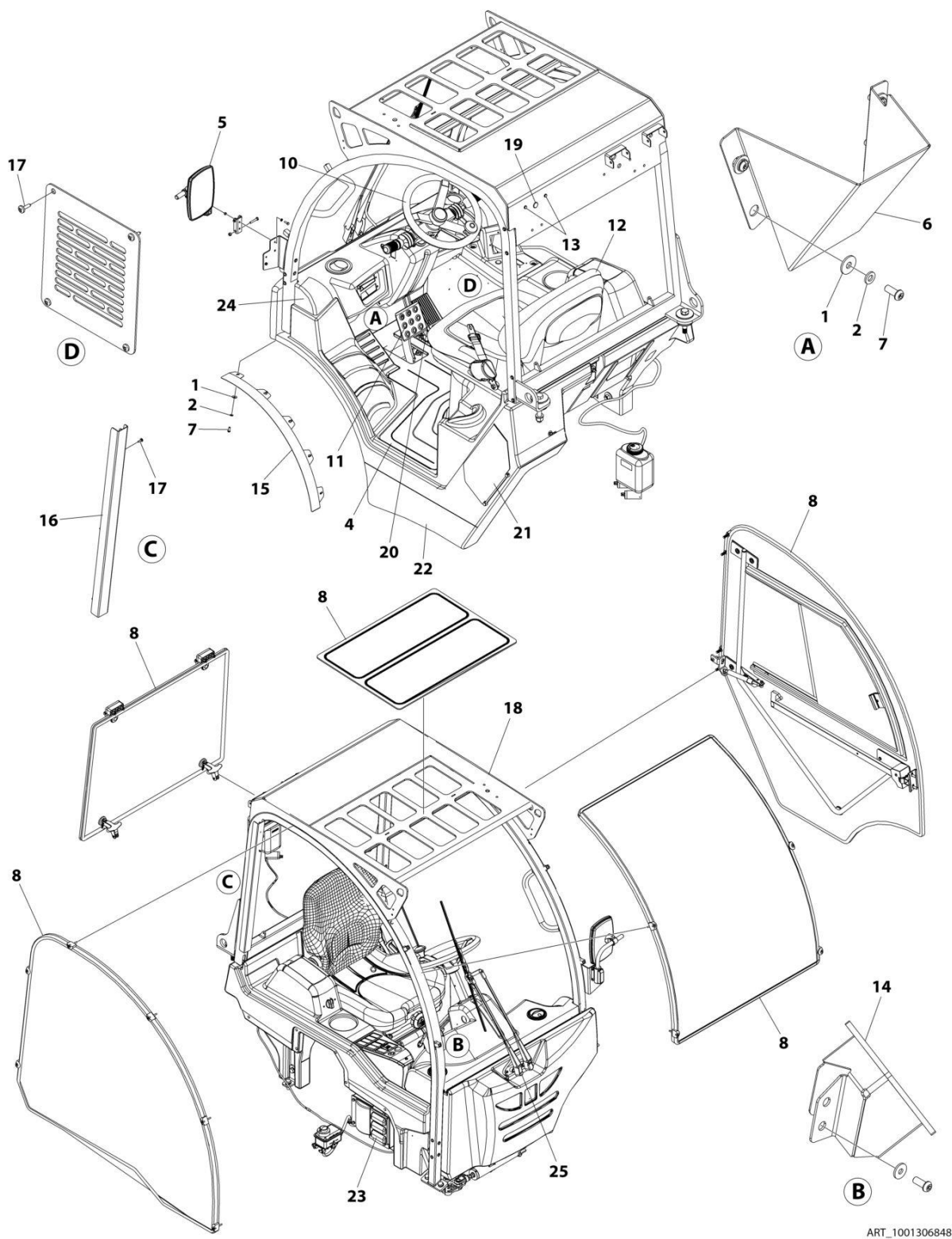
FIGURE 5-1. ENCLOSED CAB INSTALLATION
