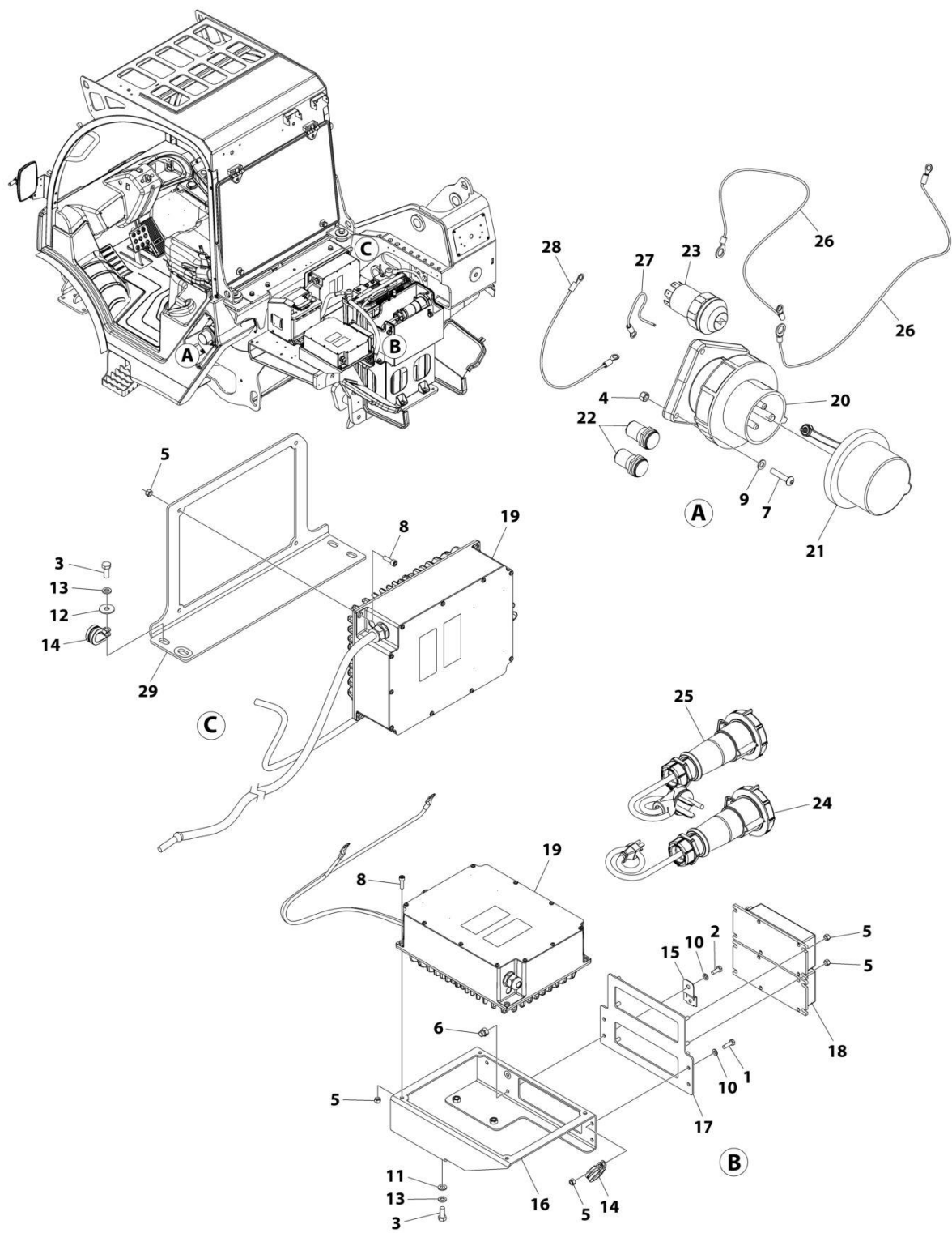
FIGURE 9-9. CHARGER INSTALLATION - DOUBLE
