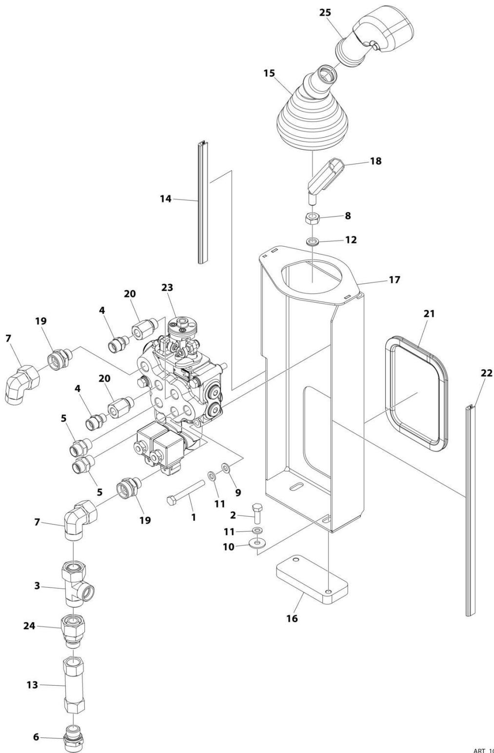
FIGURE 5-15. JOYSTICK INSTALLATION
