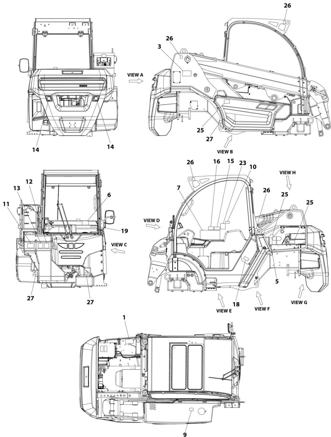
FIGURE 10-5. DECAL INSTALLATION (ISO)
