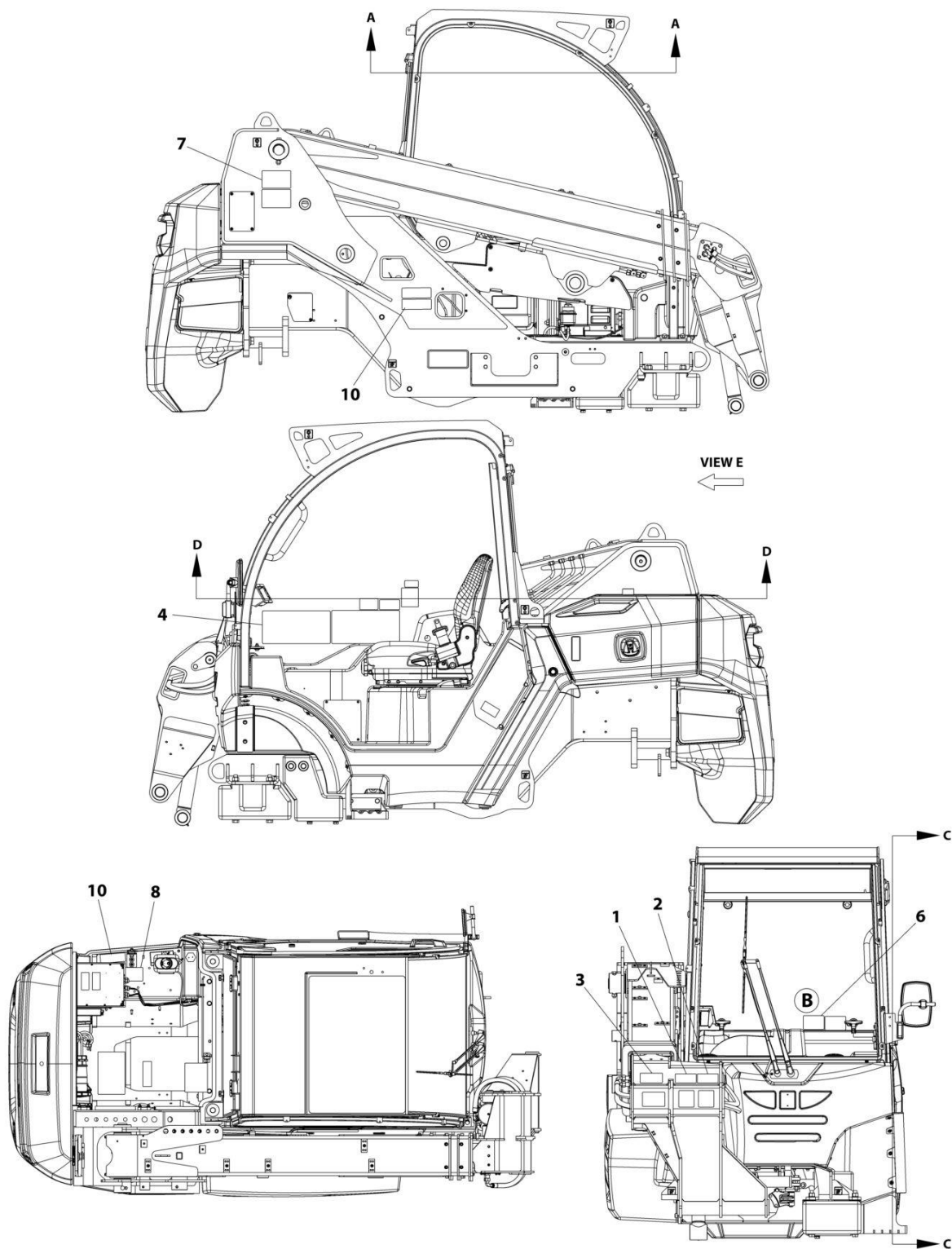
FIGURE 10-4. DECAL INSTALLATION (FRENCH)
