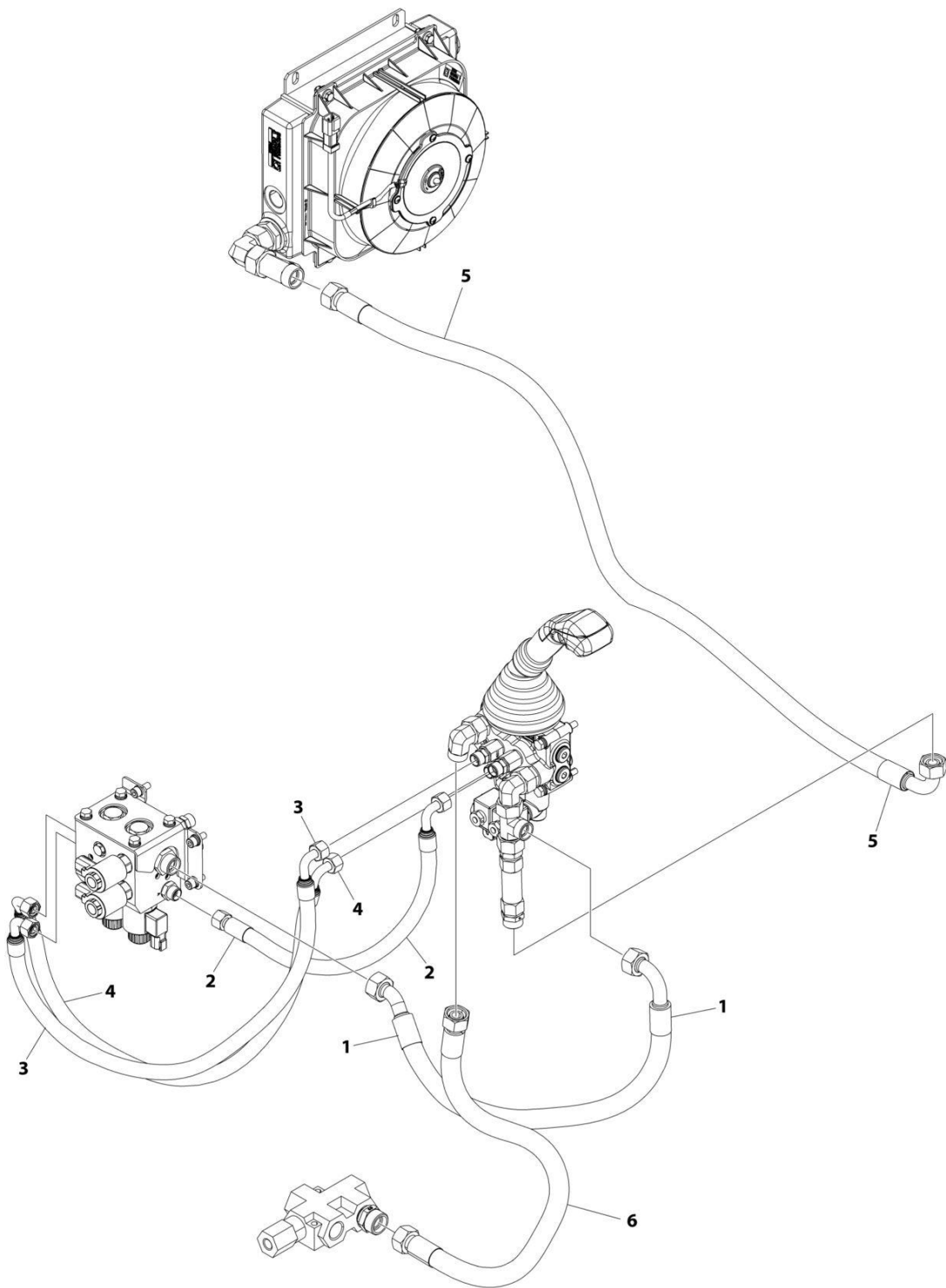
FIGURE 7-12. JOYSTICK HOSES INSTALLATION (HIGH FLOW)
