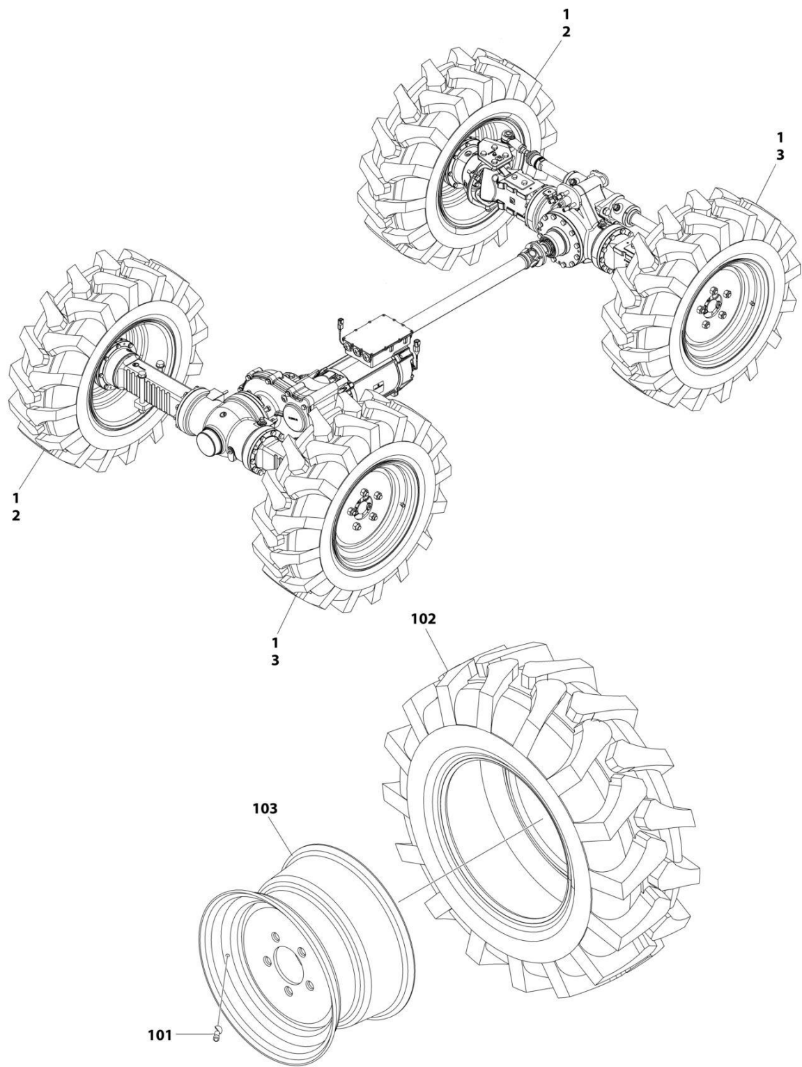
FIGURE 4-19. TIRE INSTALLATION - FOAM FILLED
