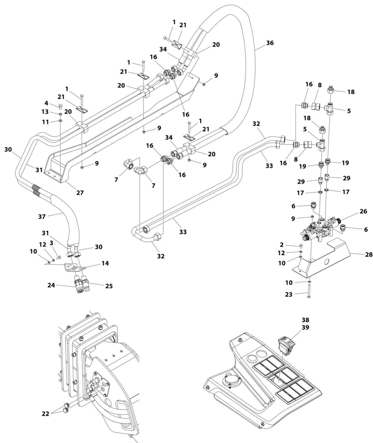
FIGURE 7-4. AUXILIARY HYDRAULICS INSTALLATION - MANUAL COUPLER (HIGH FLOW)
