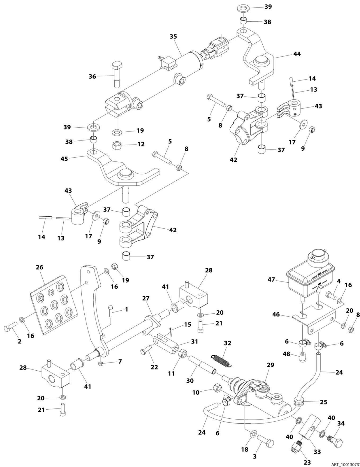
FIGURE 6-1. BRAKE SYSTEM INSTALLATION
