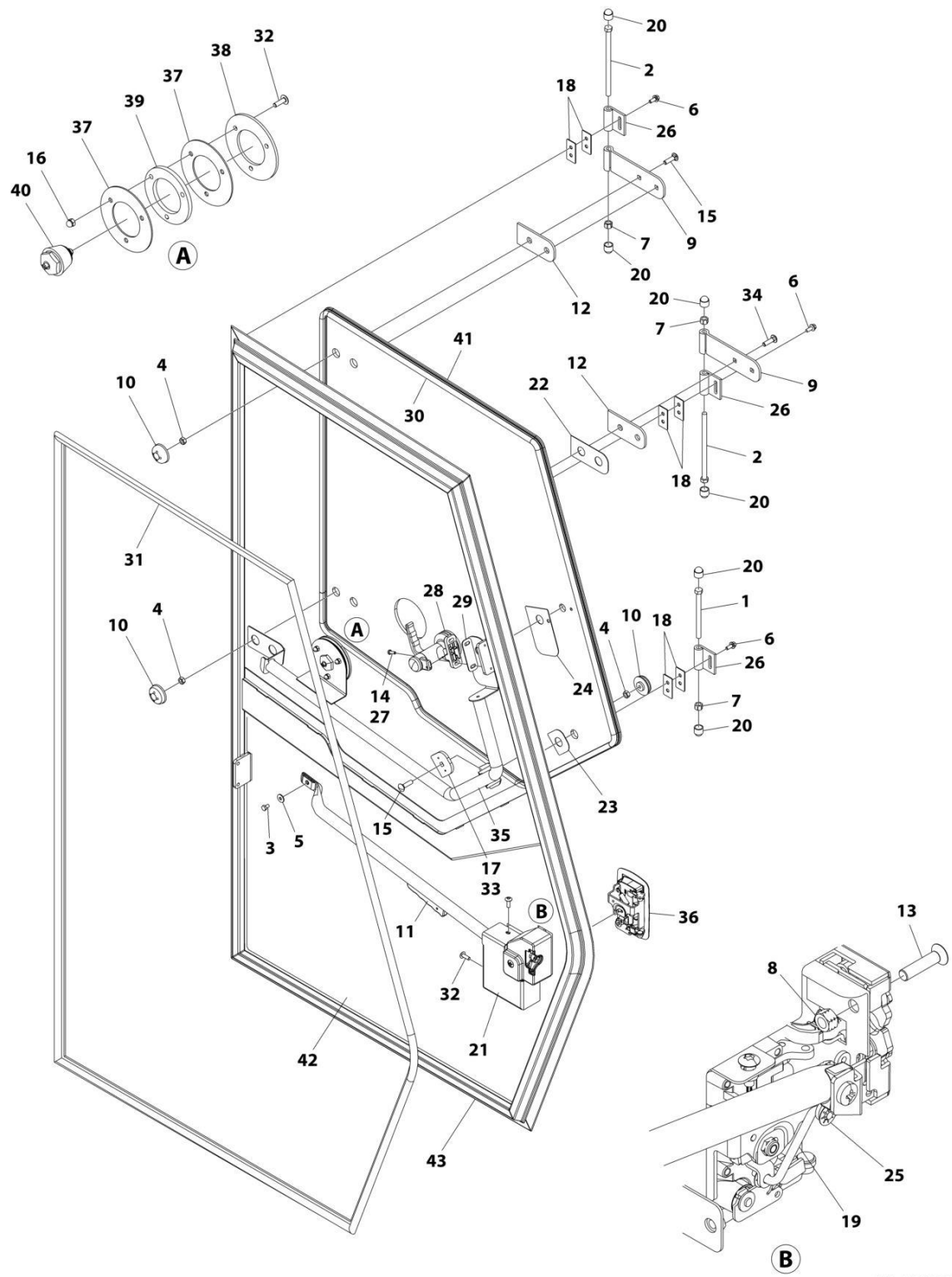
FIGURE 6-8. DOOR ASSEMBLY
