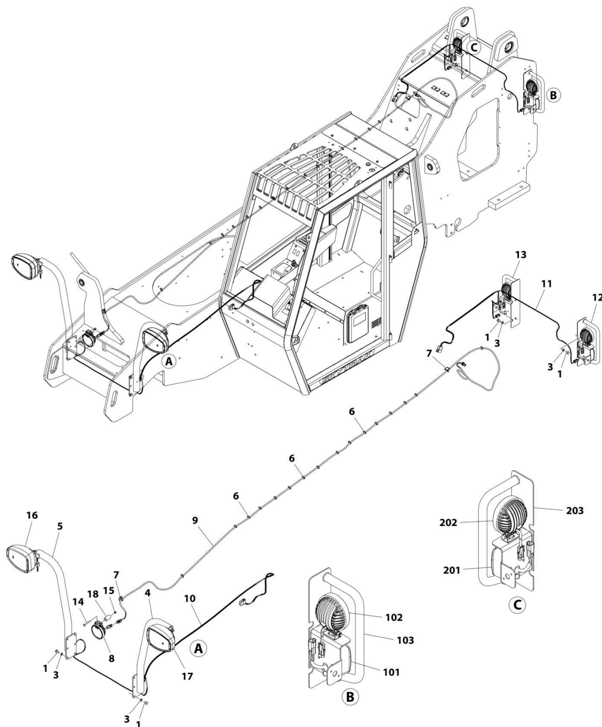
FIGURE 10-31. LIGHTS - ROADLIGHTS INSTALLATION
