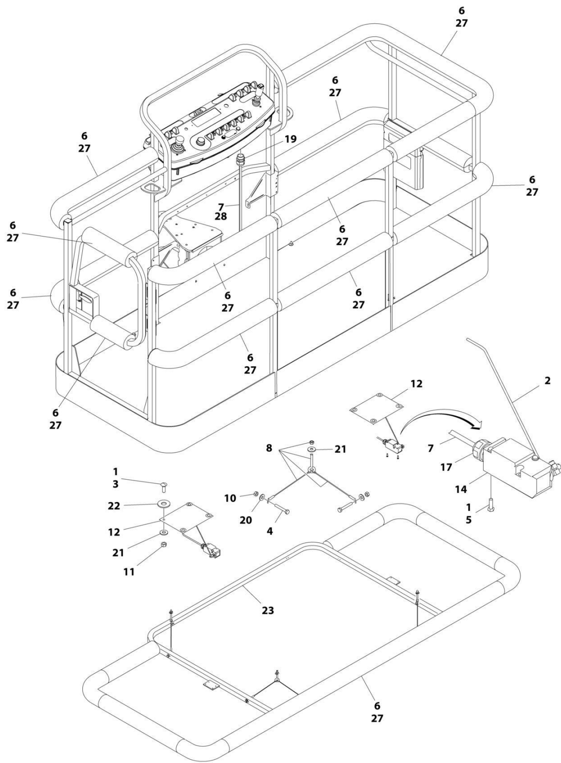
FIGURE 5-26. SOFT TOUCH SYSTEM INSTALLATION - 8FT/2.4M PLATFORMS (OPTIONAL)
