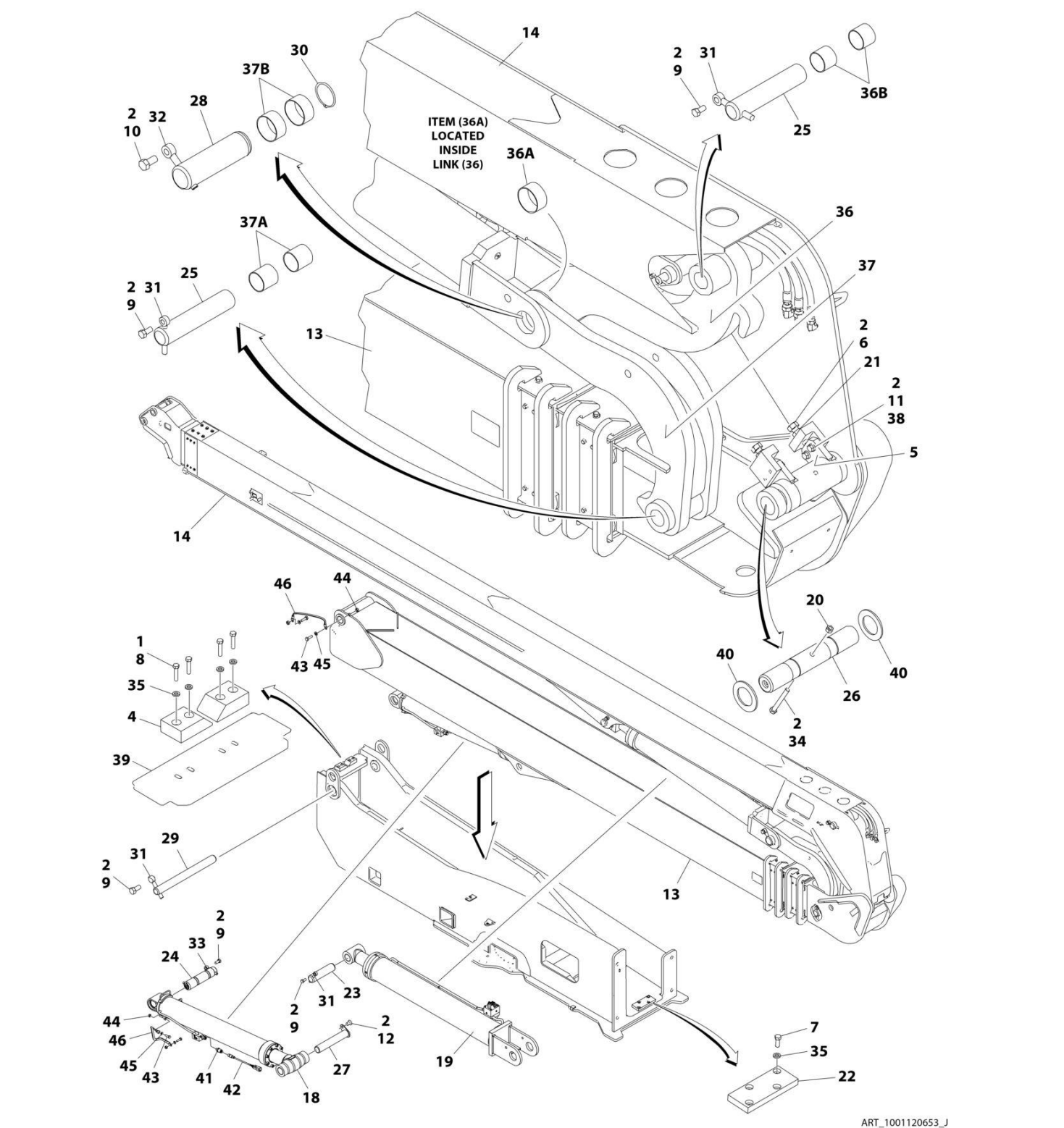
FIGURE 4-1. BOOM AND CYLINDER INSTALLATION - WITHOUT COLD WEATHER PLUS PACKAGE
