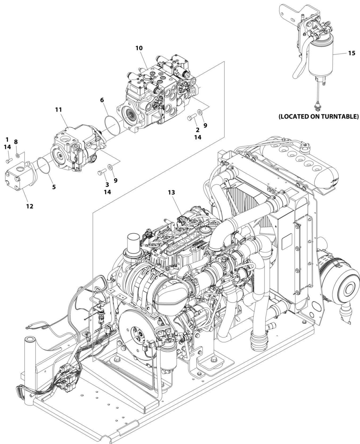
FIGURE 3-21. DEUTZ TCD2.9L4 EMR4 ENGINE SUB-ASSEMBLY - WITH SAUER PUMP (WITHOUT COLD WEATHER PLUS PACKAGE)
