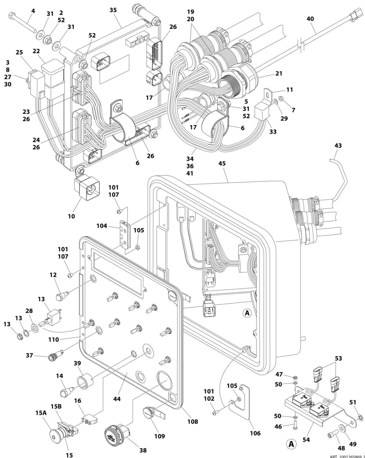
FIGURE 2-43. GROUND CONTROL ASSEMBLY - DEUTZ TCD2.9L4 (STAGE V) (WITH TOWER STOW) (CE & UK CA SPECS)
