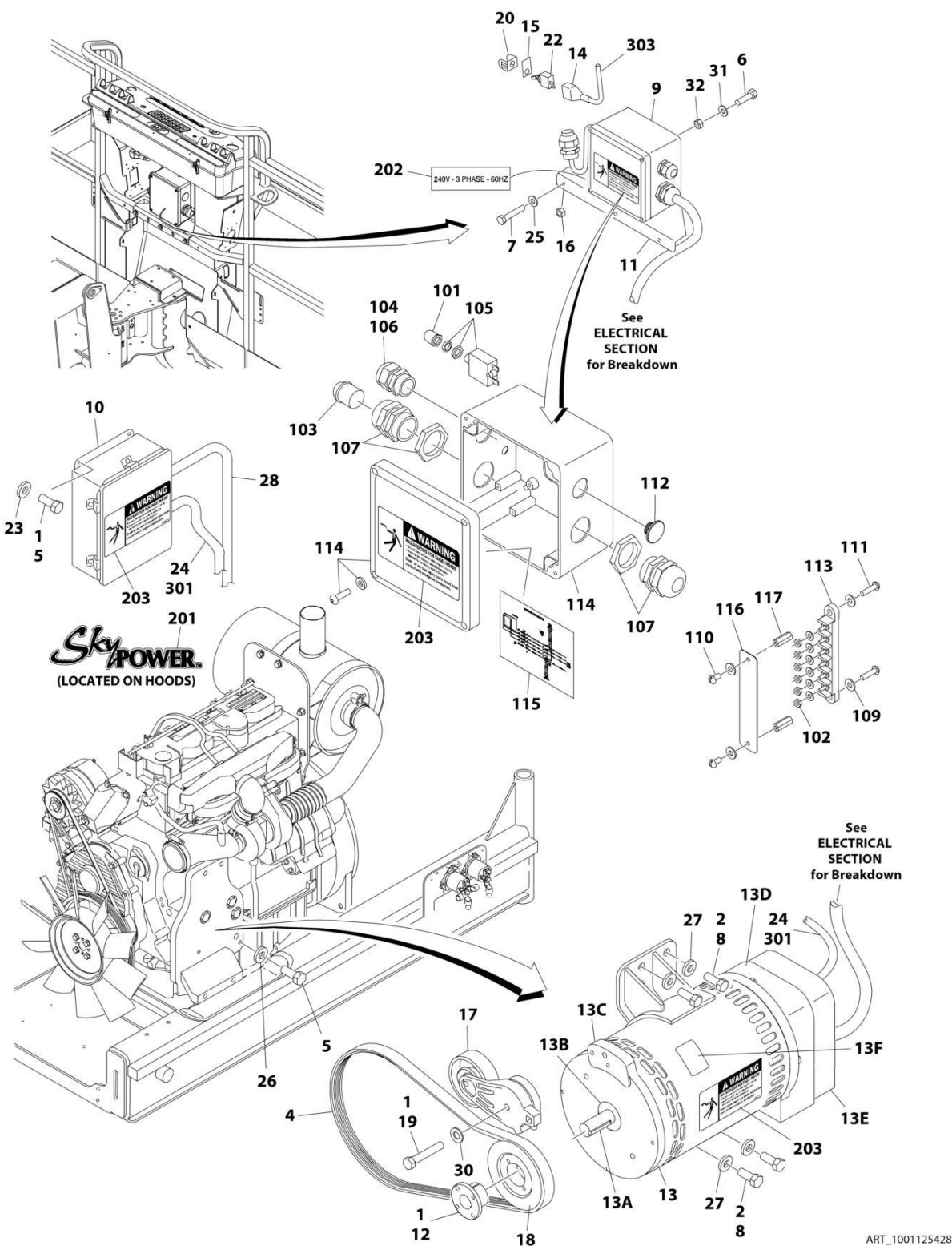
FIGURE 3-79. 7500W SKYPOWER GENERATOR INSTALLATION - 50HZ SPEC (DEUTZ TD2011 ENGINES) (OPTIONAL)
