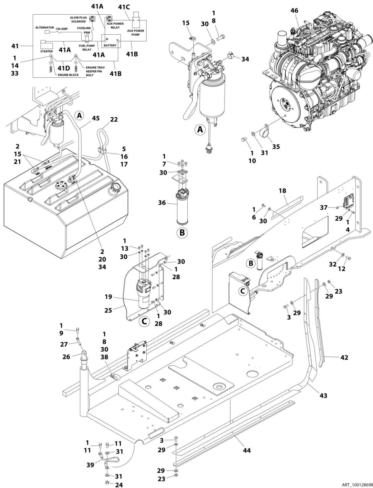
FIGURE 3-31. DEUTZ D2.9L4 - EMR5 ENGINE INSTALLATION WITH PMP PUMPS (WITH COLD WEATHER PLUS PACKAGE)
