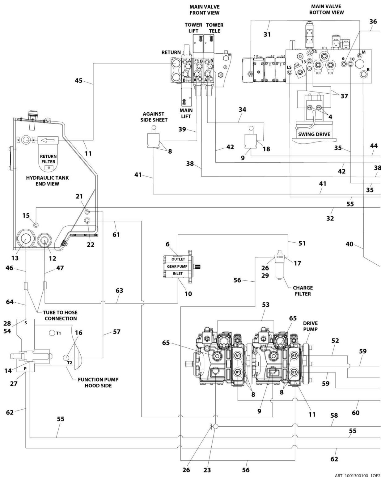
FIGURE 7-12. HYDRAULIC DIAGRAM - TURNTABLE (WITH PMP PUMPS)
