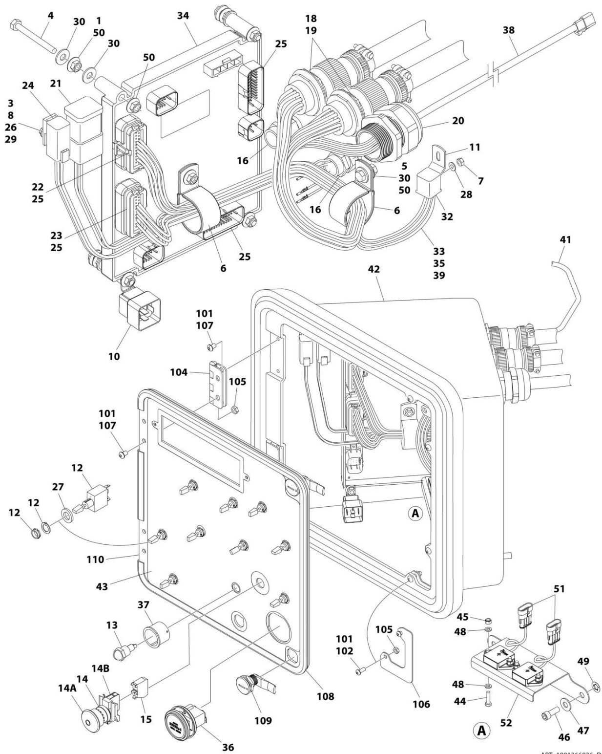
FIGURE 2-40. GROUND CONTROL ASSEMBLY - DEUTZ TD2011 ENGINES (WITHOUT TOWER STOW) (CE & UK CA SPECS)
