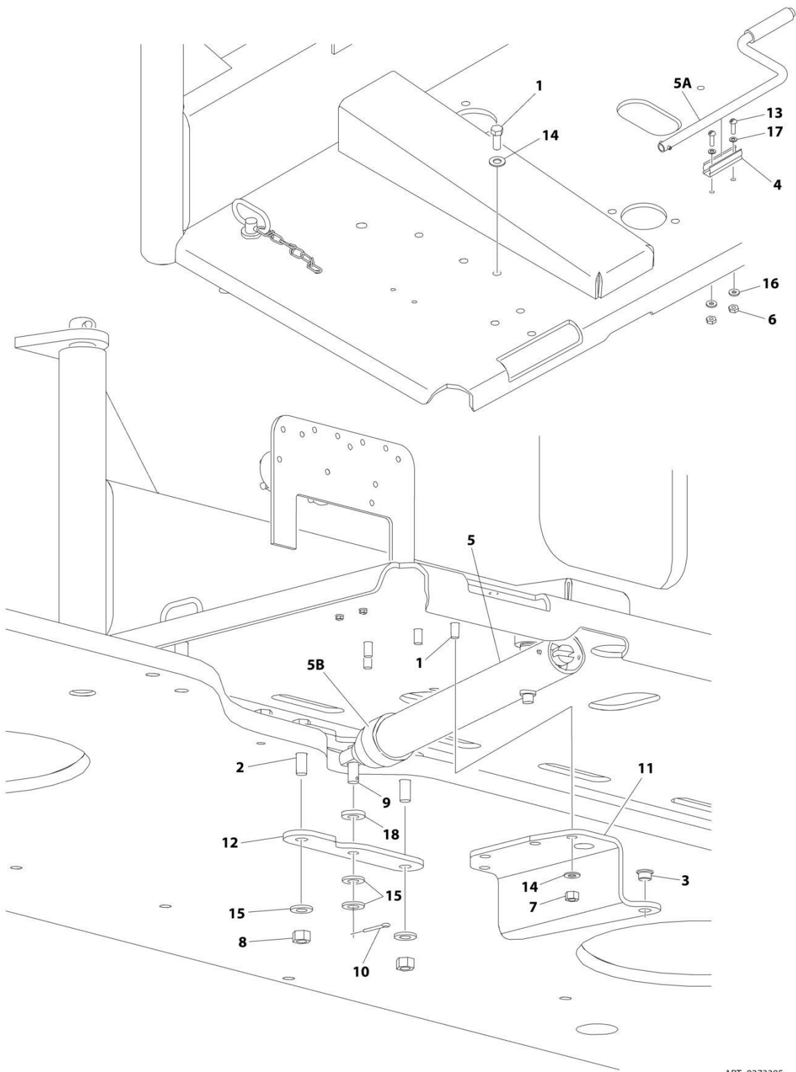
FIGURE 2-54. ENGINE TRAY JACK INSTALLATION - DEUTZ TD2011 ENGINES
