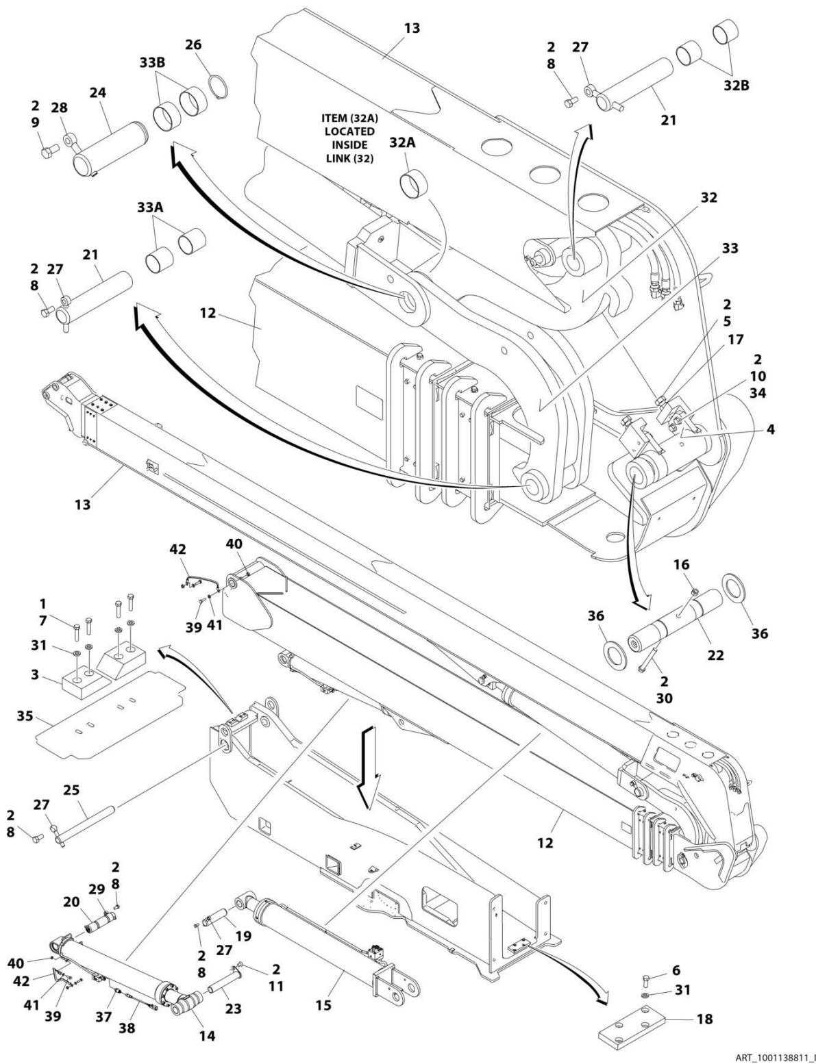
FIGURE 4-2. BOOM AND CYLINDER INSTALLATION - WITH COLD WEATHER PLUS PACKAGE
