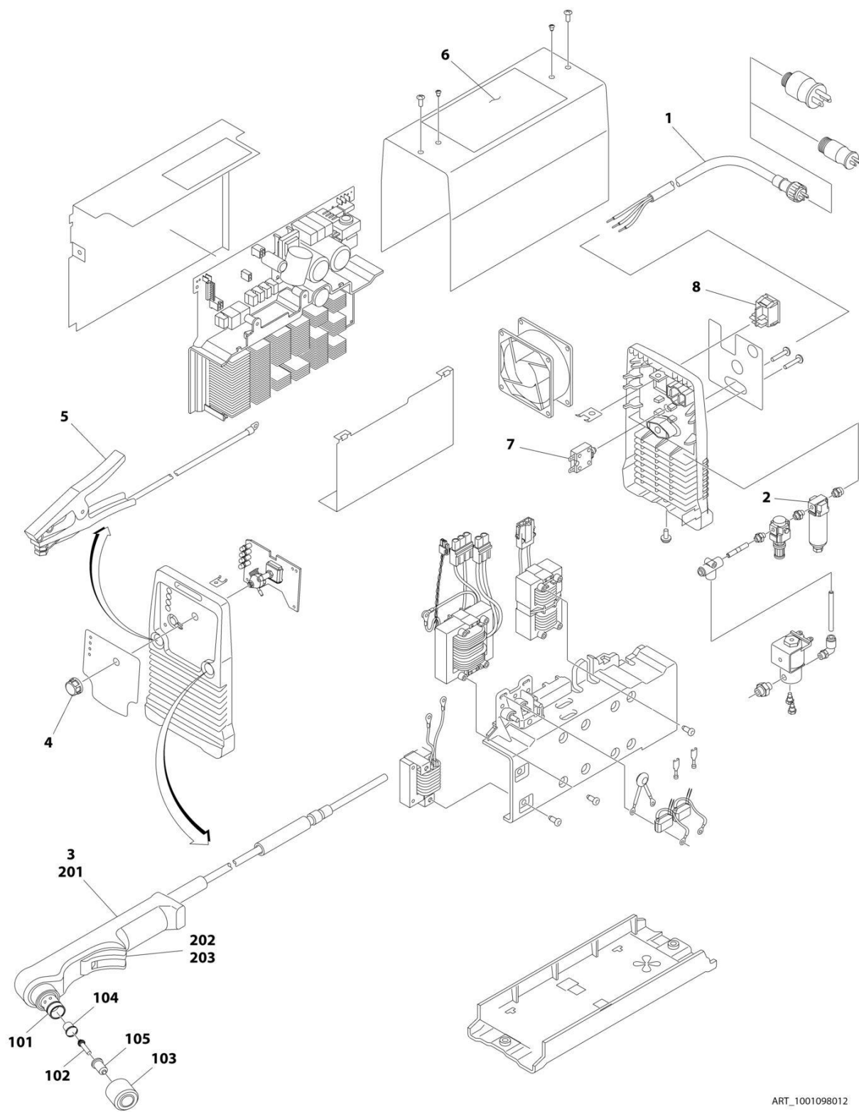
FIGURE 5-40. PLASMA CUTTER ASSEMBLY
