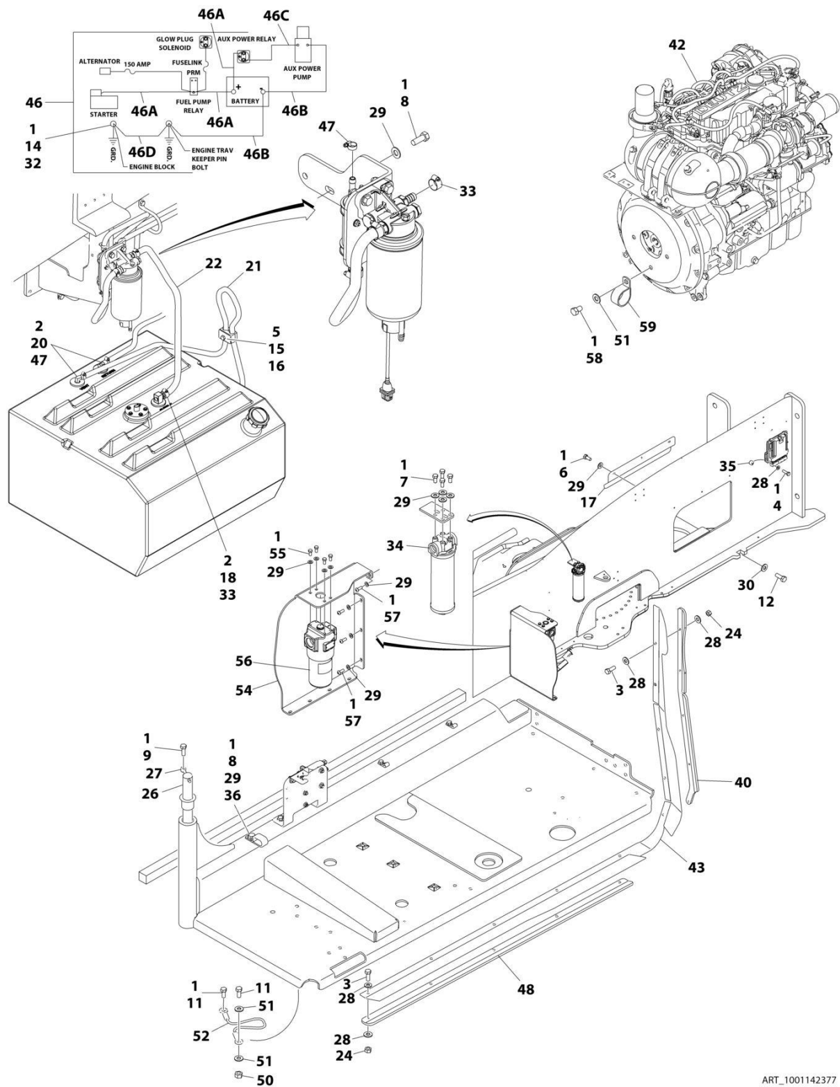
FIGURE 3-17. DEUTZ TCD2.9L4 EMR4 ENGINE INSTALLATION - WITH REXROTH PUMP (WITH COLD WEATHER PLUS PACKAGE)
