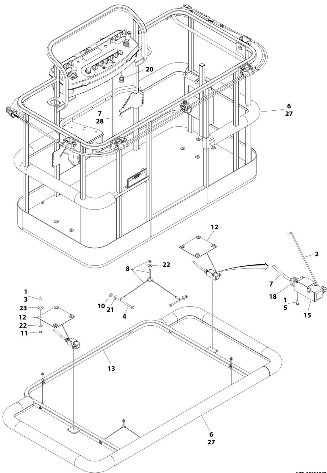
FIGURE 5-25. SOFT TOUCH SYSTEM INSTALLATION - 6FT/1.83M FALL ARREST PLATFORM
