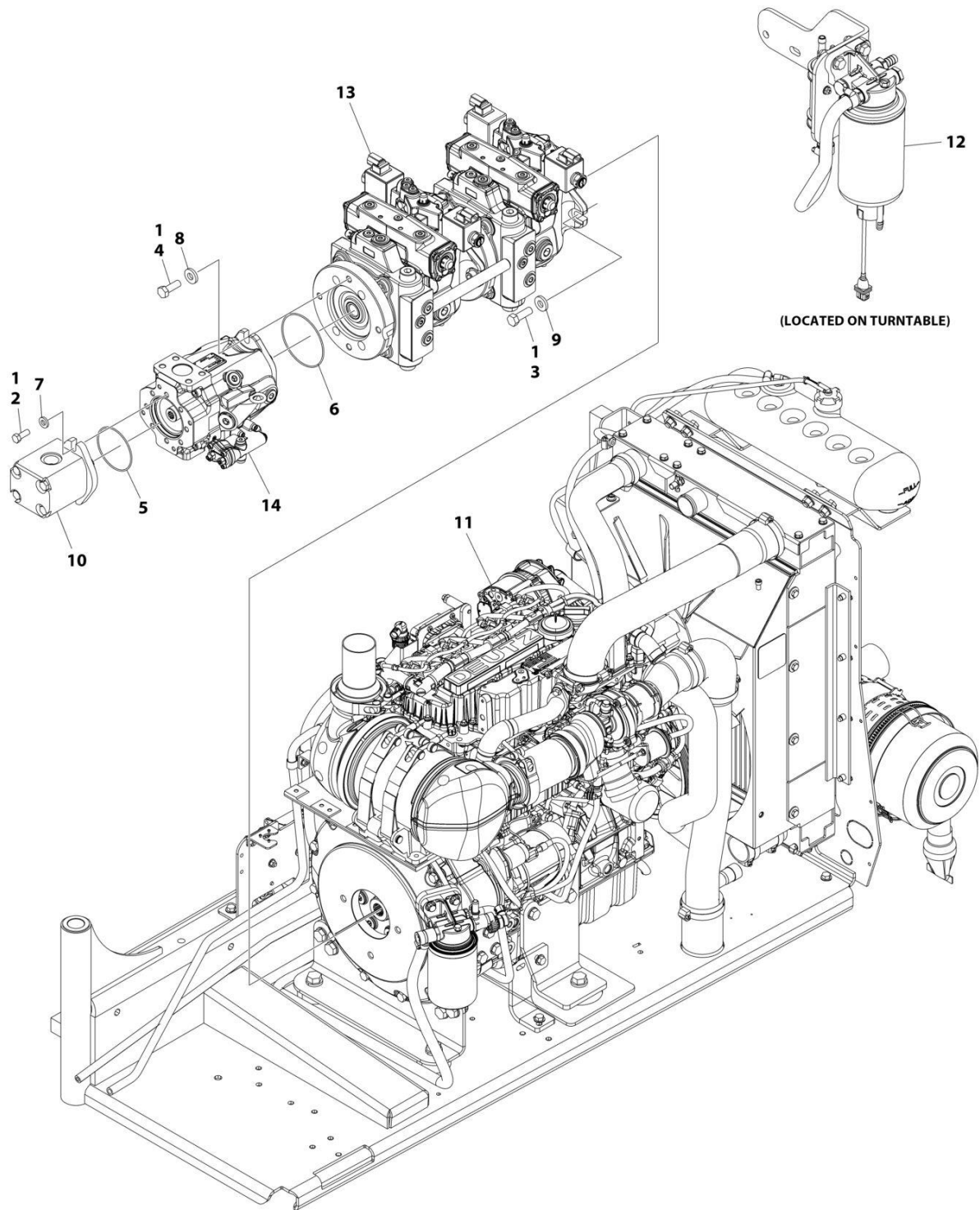
FIGURE 3-25. DEUTZ D2.9L4 (EMR4) ENGINE SUB-ASSEMBLY WITH PMP PUMP AND ABS HOODS (WITHOUT COLD WEATHER PLUS PACKAGE)
