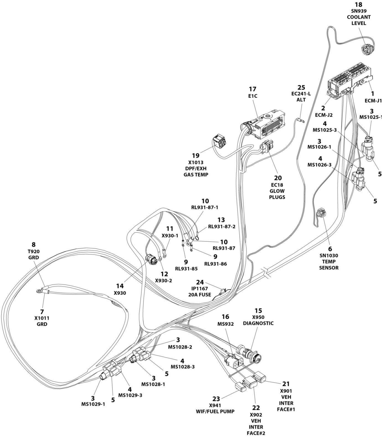
FIGURE 8-51. ENGINE HARNESS - DEUTZ TCD2.9L4 ENGINES AND DEUTZ TCD2.9L4 (STAGE V) ENGINES
