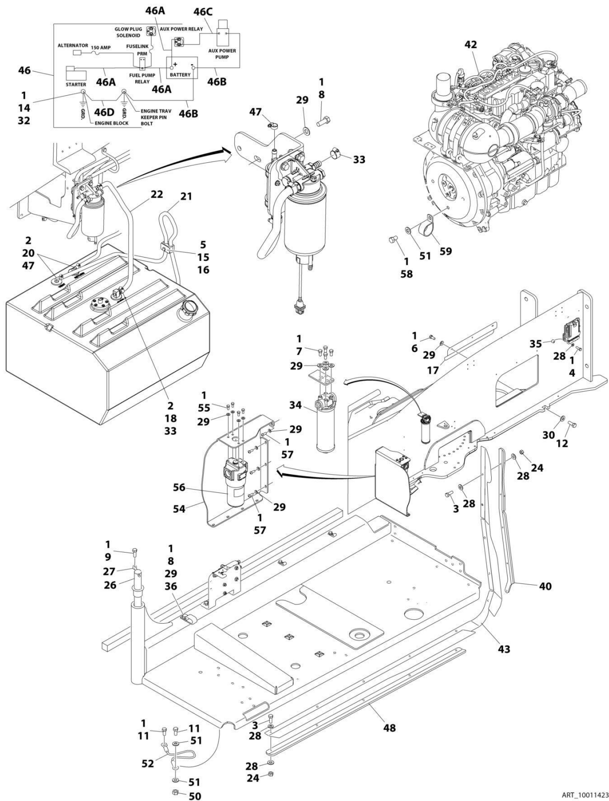
FIGURE 3-14. DEUTZ TCD2.9L4 EMR4 ENGINE INSTALLATION - WITH REXROTH PUMP (WITHOUT COLD WEATHER PLUS PACKAGE)
