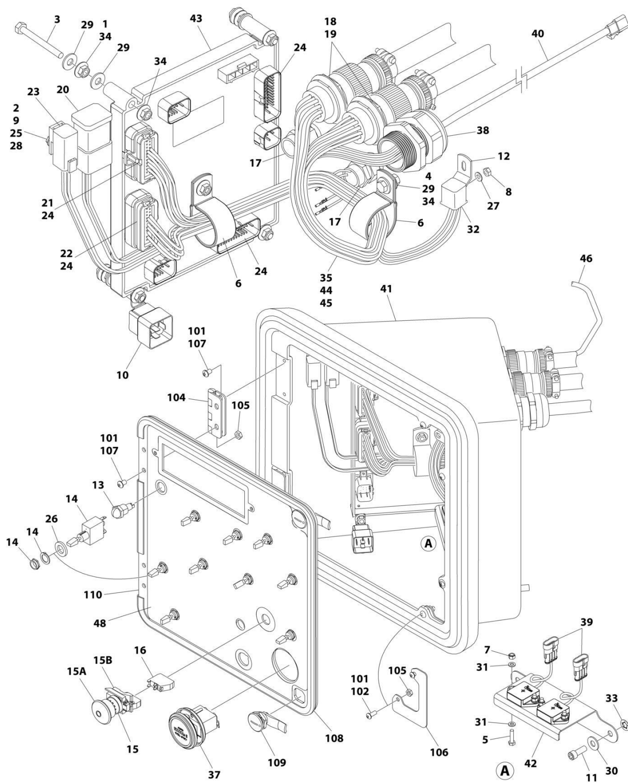
FIGURE 2-44. GROUND CONTROL ASSEMBLY - CHINA IV (CHINESE SPEC)
