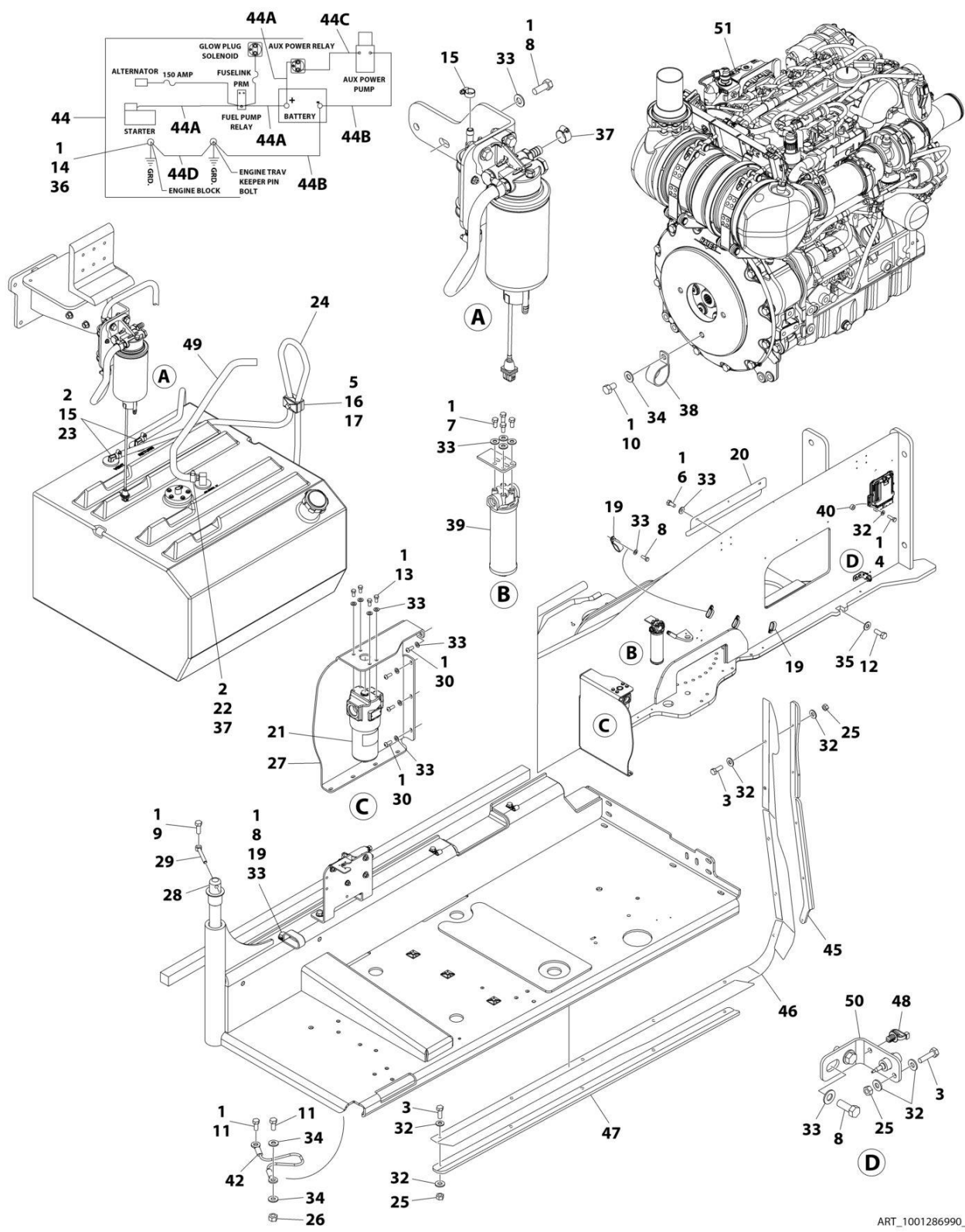
FIGURE 3-37. DEUTZ D2.9L4 - (STAGE V) ENGINE INSTALLATION WITH PMP PUMPS (WITHOUT COLD WEATHER PLUS PACKAGE)
