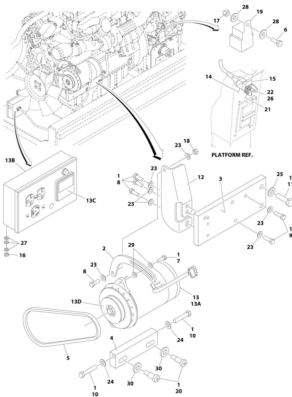
FIGURE 3-73. 2500W GENERATOR INSTALLATION - DEUTZ TD2011 ENGINES (OPTIONAL)
