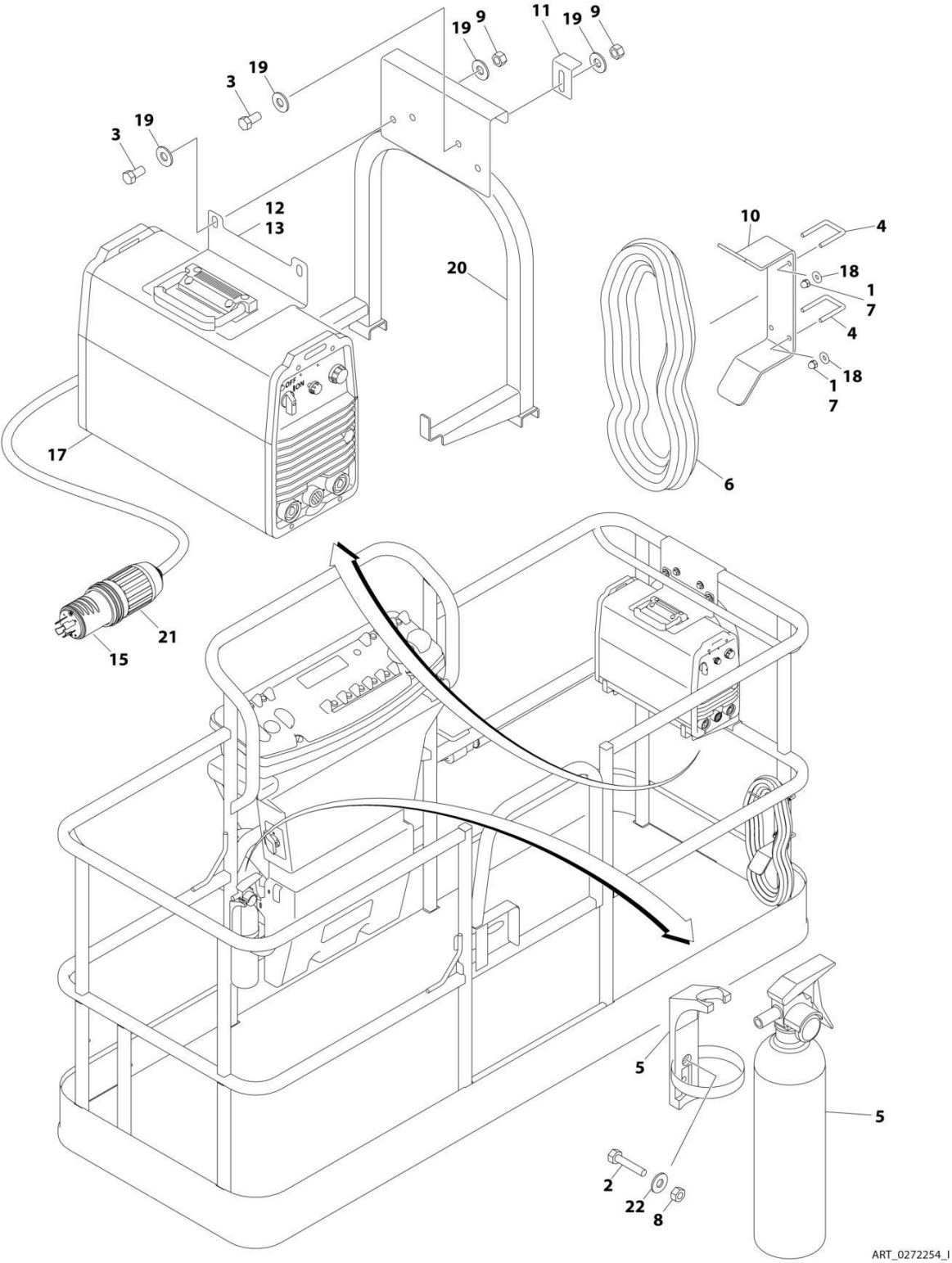
FIGURE 5-42. SKYWELDER INSTALLATION (60HZ)
