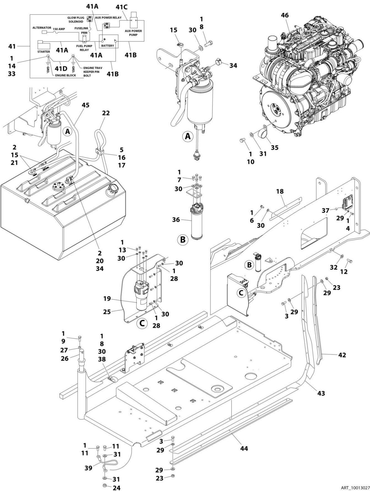
FIGURE 3-33. DEUTZ D2.9L4 - EMR5 ENGINE INSTALLATION WITH SAUER PUMPS (WITHOUT COLD WEATHER PLUS PACKAGE)
