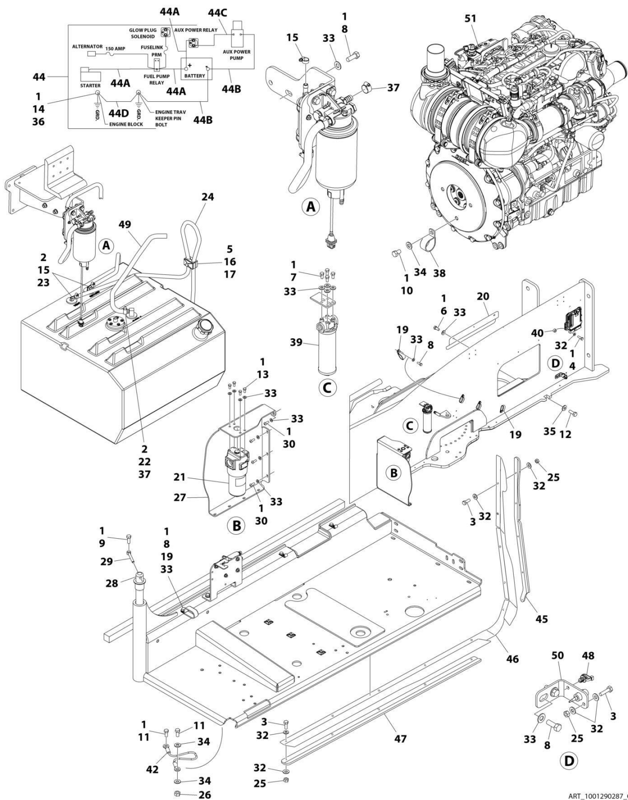
FIGURE 3-54. DEUTZ DIESEL TCD2.9L CHINA IV ENGINE INSTALLATION (CHINESE SPEC)
