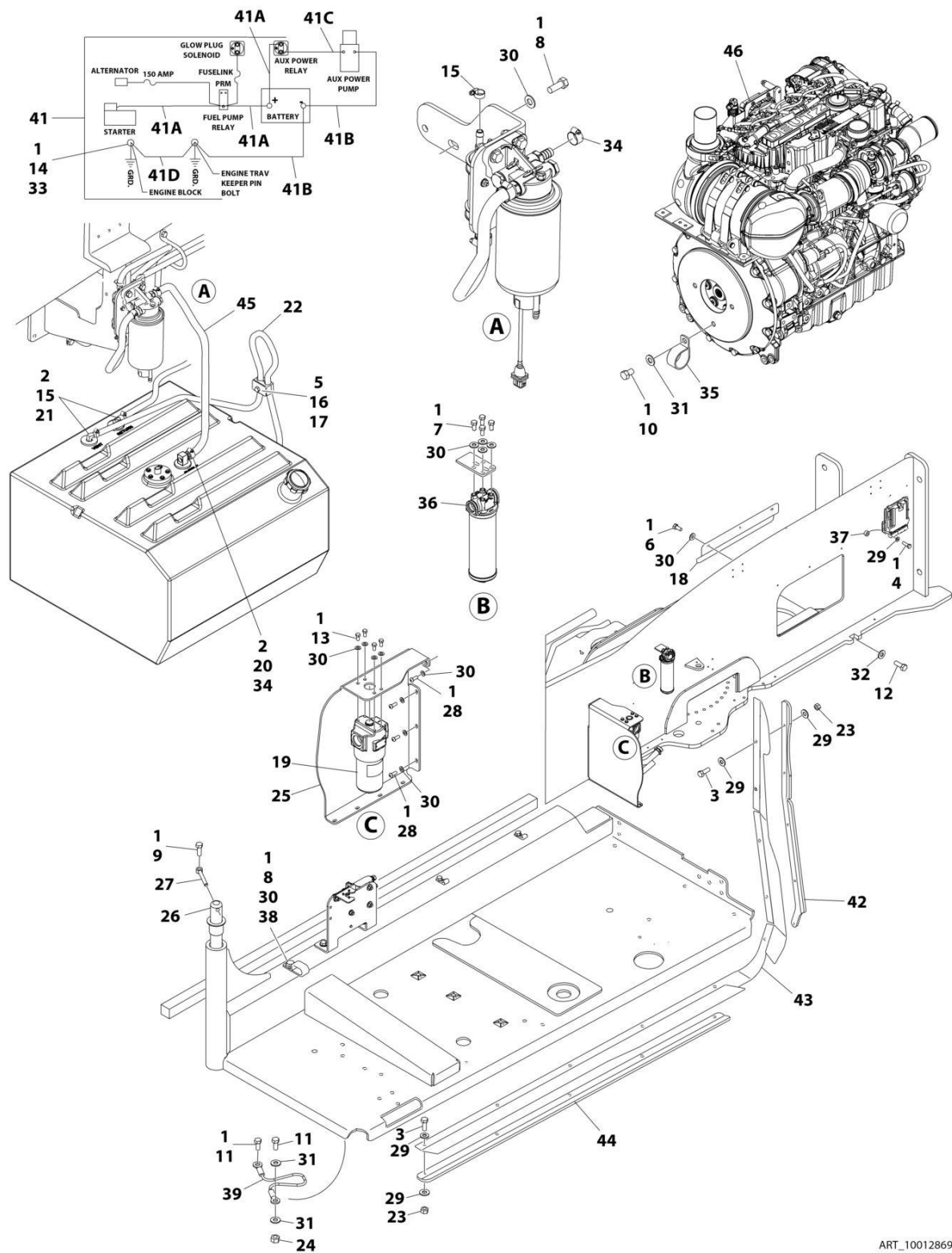
FIGURE 3-32. DEUTZ D2.9L4 - EMR5 ENGINE INSTALLATION WITH PMP PUMPS (WITHOUT COLD WEATHER PLUS PACKAGE)
