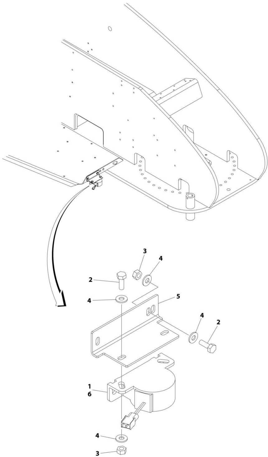
FIGURE 2-49. BACKUP ALARM (WHITE NOISE) INSTALLATION
