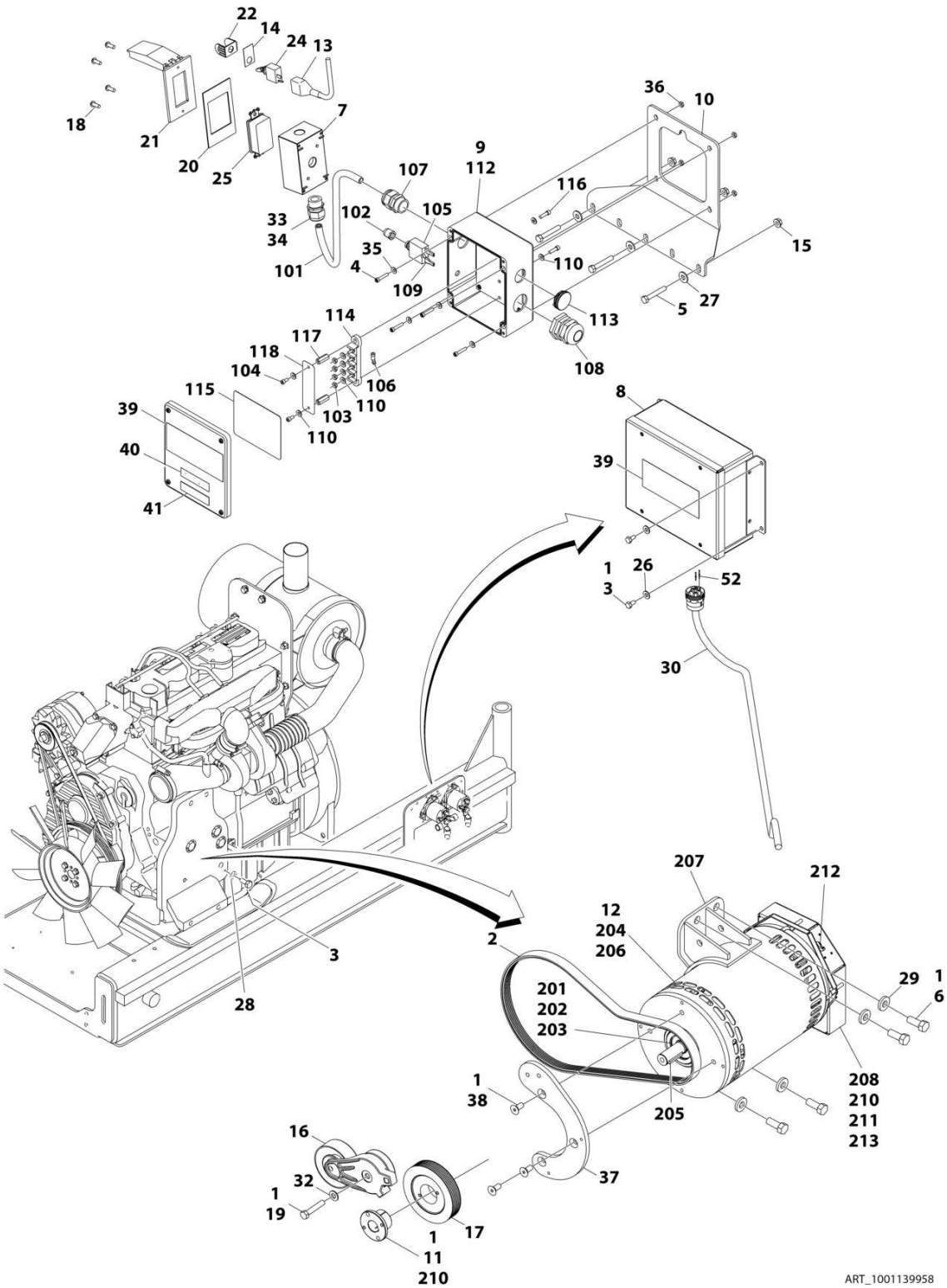
FIGURE 3-74. 4000W GENERATOR INSTALLATION - 60HZ SPEC (DEUTZ TD2011 ENGINES)
