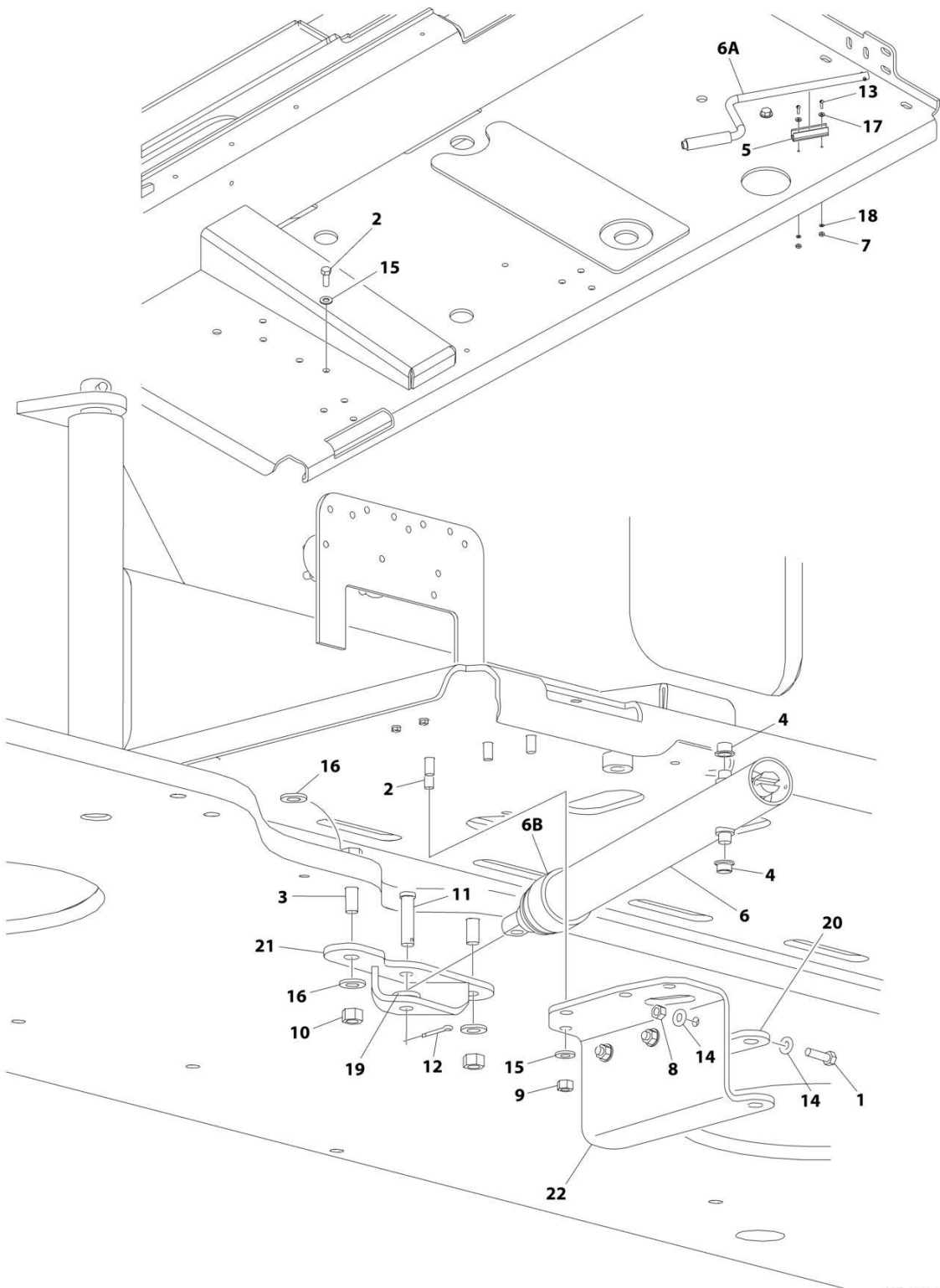
FIGURE 2-55. ENGINE TRAY JACK INSTALLATION - DEUTZ TCD2.9L4 ENGINES AND DEUTZ TCD2.9L4 (STAGE V) ENGINES
