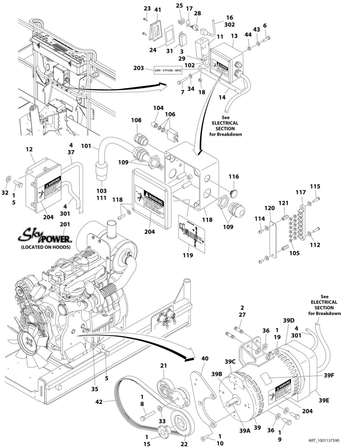
FIGURE 3-80. 7500W SKYPOWER GENERATOR INSTALLATION - 60HZ SPEC (DEUTZ TCD2.9L4 ENGINES) (OPTIONAL)
