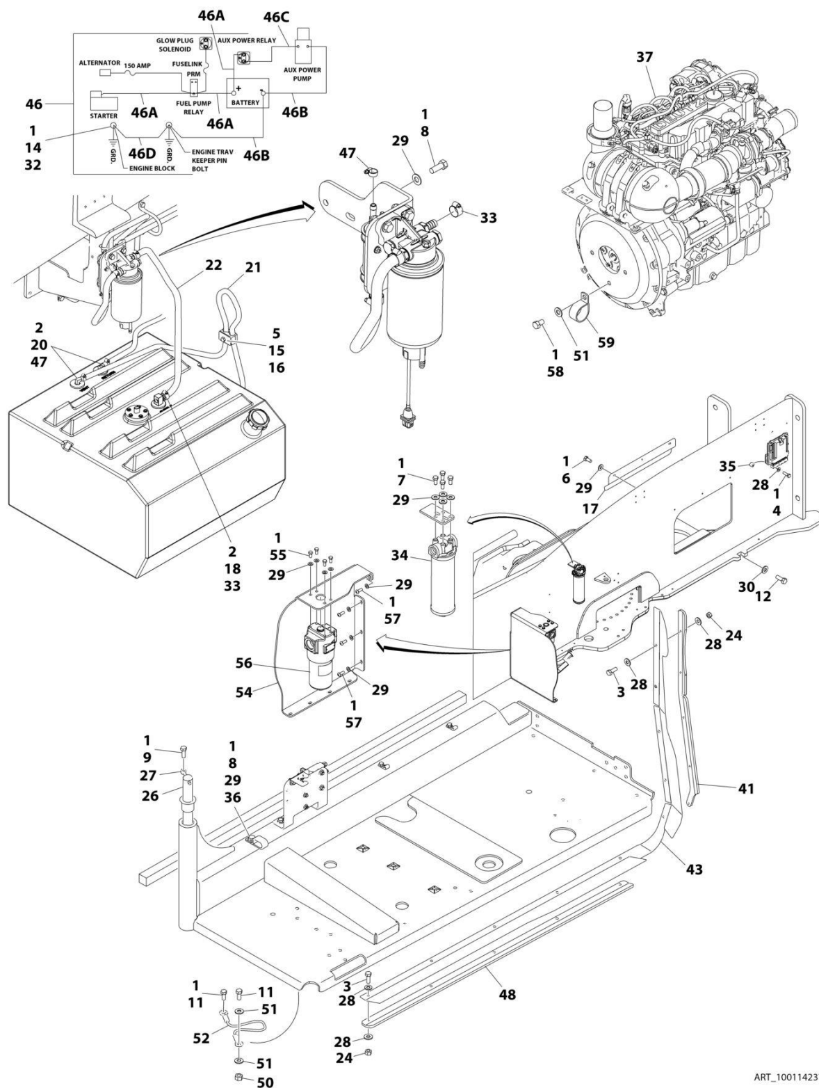
FIGURE 3-20. DEUTZ TCD2.9L4 EMR4 ENGINE INSTALLATION - WITH SAUER PUMPS (WITHOUT COLD WEATHER PLUS PACKAGE)
