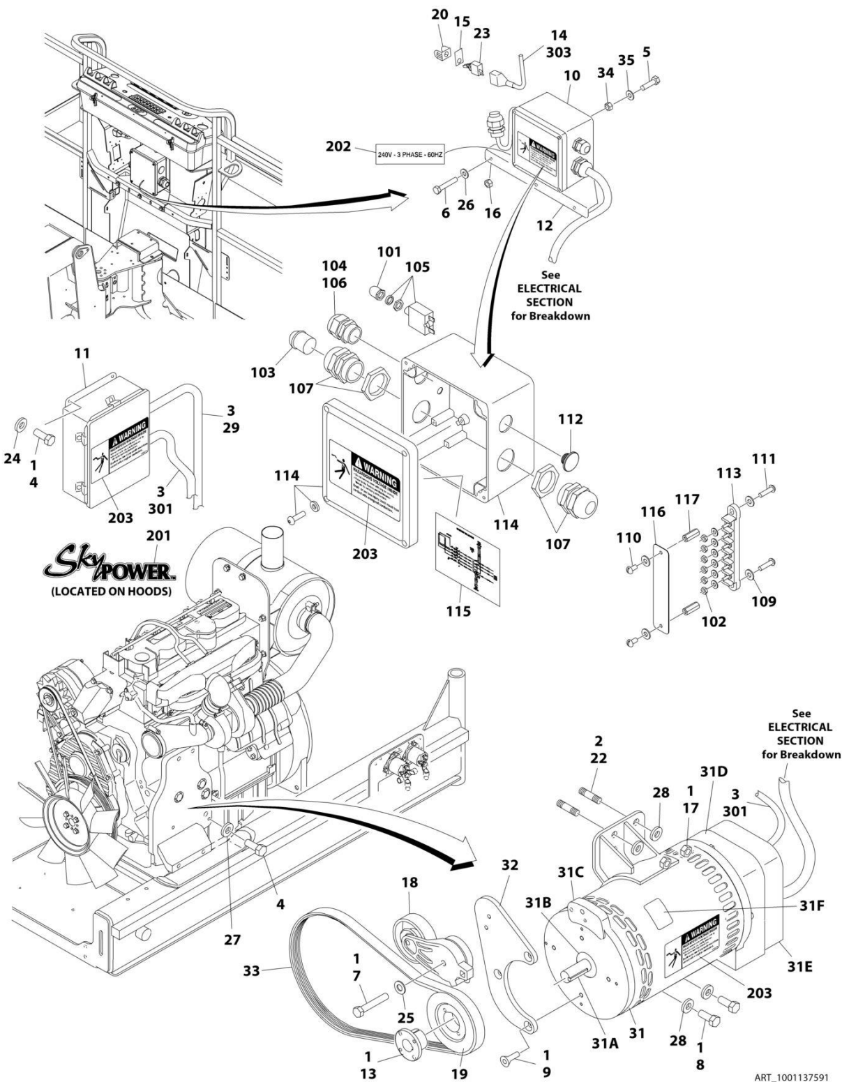
FIGURE 3-81. 7500W SKYPOWER GENERATOR INSTALLATION - 50HZ SPEC (DEUTZ TCD2.9L4 ENGINES AND DEUTZ TCD2.9L4 (STAGE V) ENGINES) (OPTIONAL)
