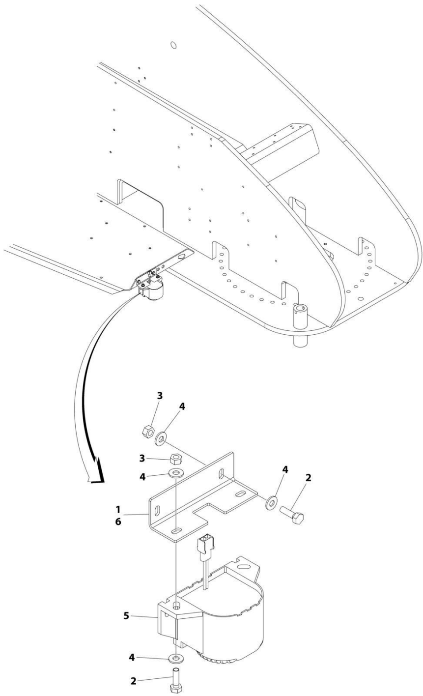
FIGURE 2-50. BACKUP ALARM AMBIENT (WHITE NOISE) INSTALLATION
