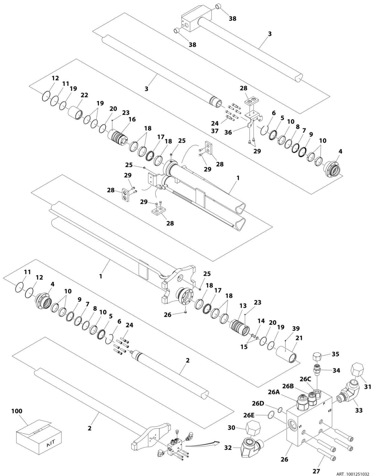
FIGURE 6-9. TELESCOPE CYLINDER ASSEMBLY - TOWER BOOM
