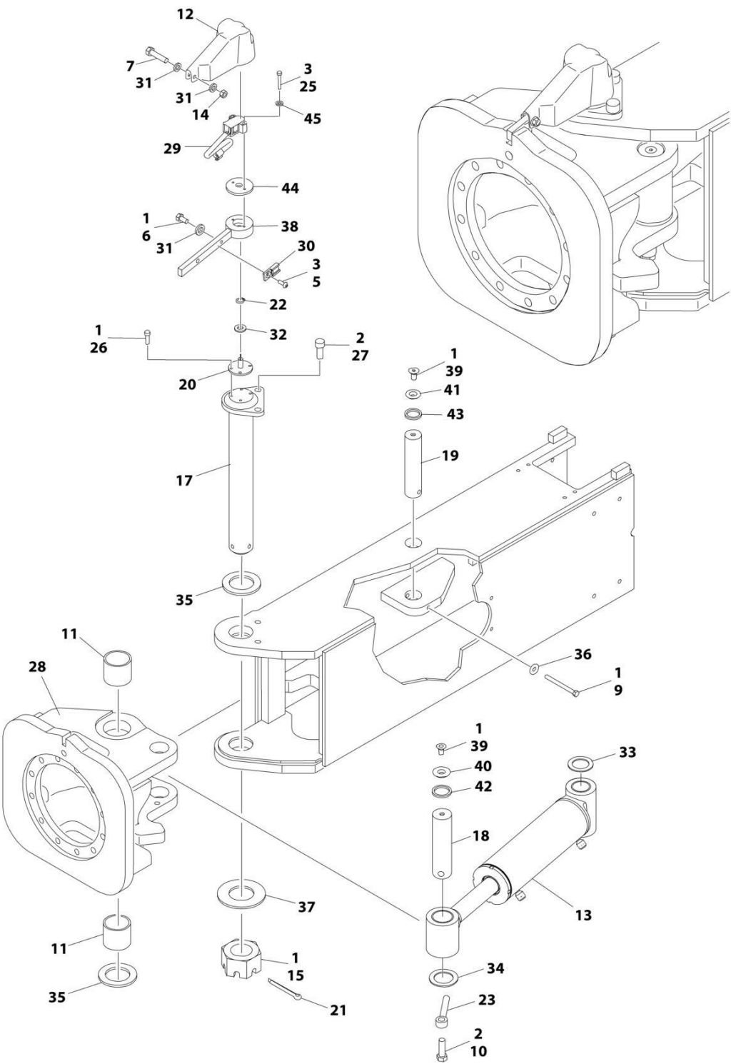
FIGURE 1-4. STEER INSTALLATION
