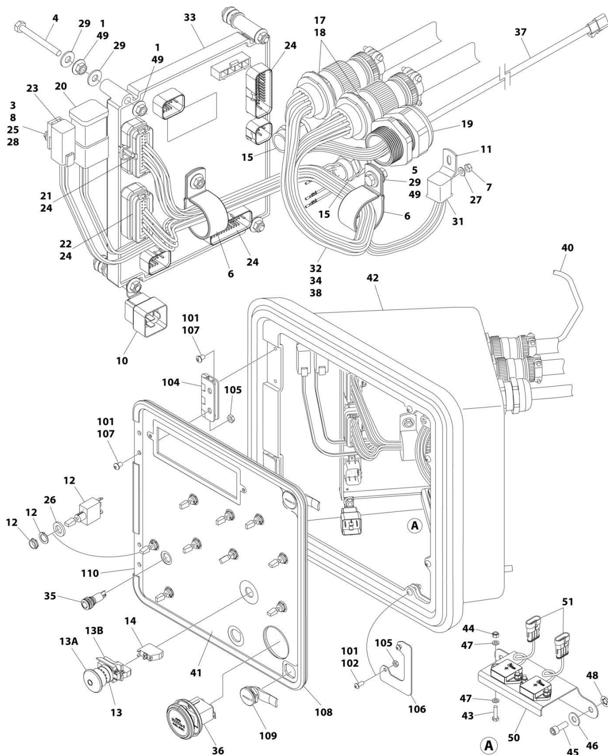
FIGURE 2-39. GROUND CONTROL ASSEMBLY - WITH DEUTZ TD2011 AND DEUTZ TCD2.9L4 ENGINES - WITH MECHANICAL HOUR METER (WITH TOWER STOW) (ALL SPECS EXCEPT CE & UK CA SPECS)
