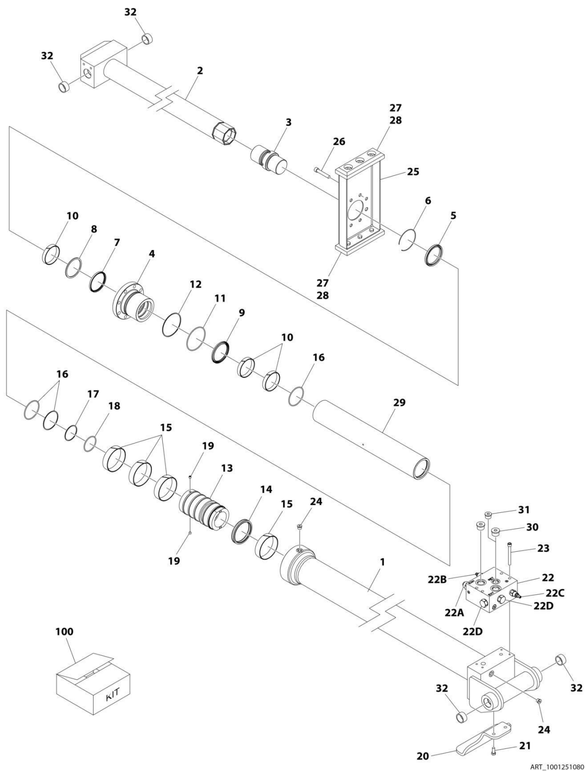
FIGURE 6-8. TELESCOPE CYLINDER ASSEMBLY - MAIN BOOM
