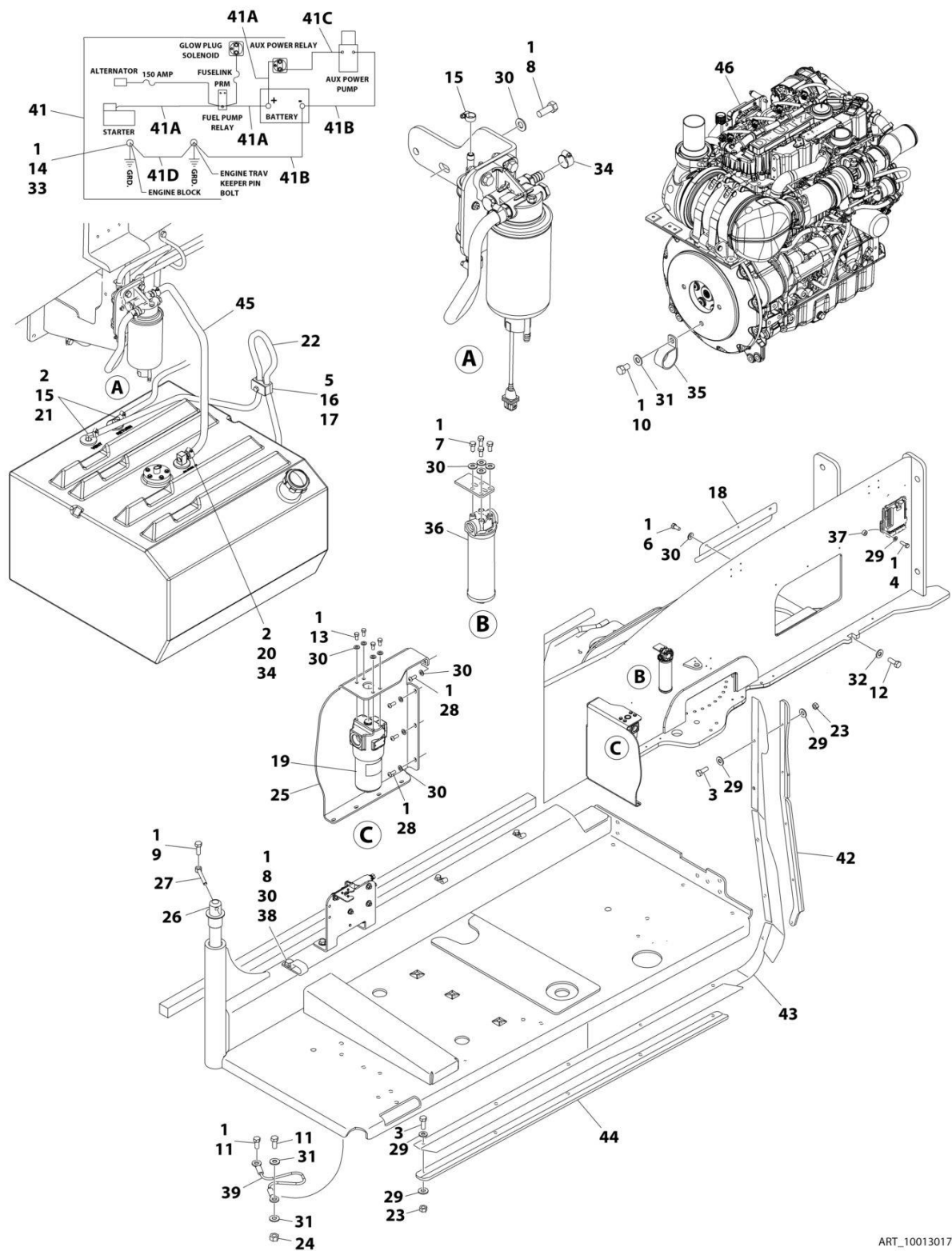
FIGURE 3-35. DEUTZ D2.9L4 - EMR5 ENGINE INSTALLATION WITH PMP PUMPS (WITHOUT COLD WEATHER PLUS PACKAGE)
