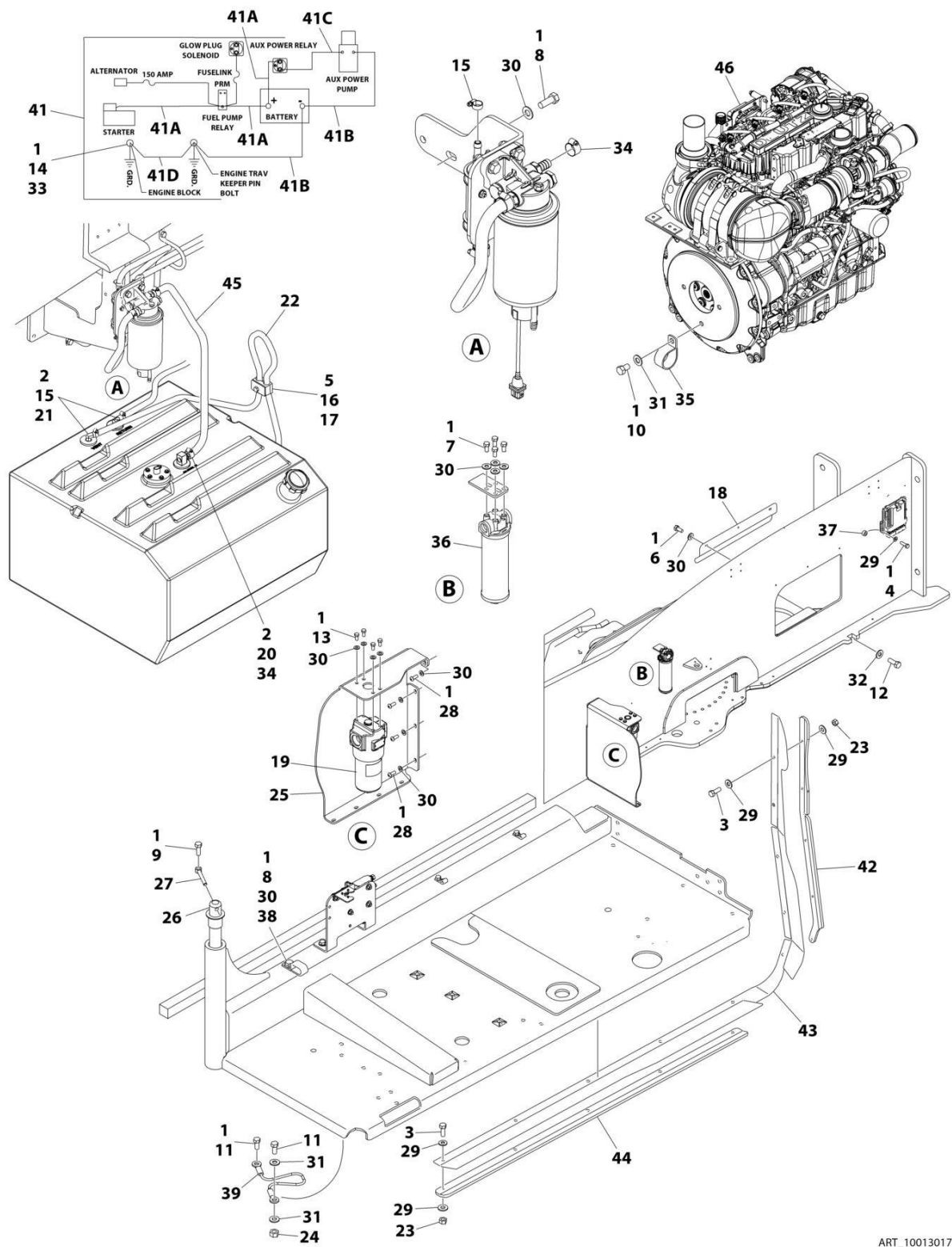
FIGURE 3-36. DEUTZ D2.9L4 - EMR5 ENGINE INSTALLATION WITH PMP PUMPS (WITH COLD WEATHER PLUS PACKAGE)
