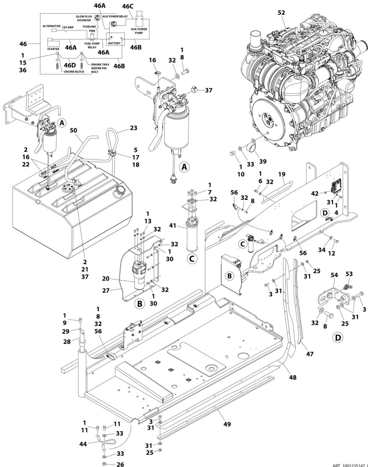
FIGURE 3-49. DEUTZ TCD2.9L4 (STAGE V) ENGINE INSTALLATION - WITH REXROTH PUMP (WITHOUT COLD WEATHER PLUS PACKAGE)
