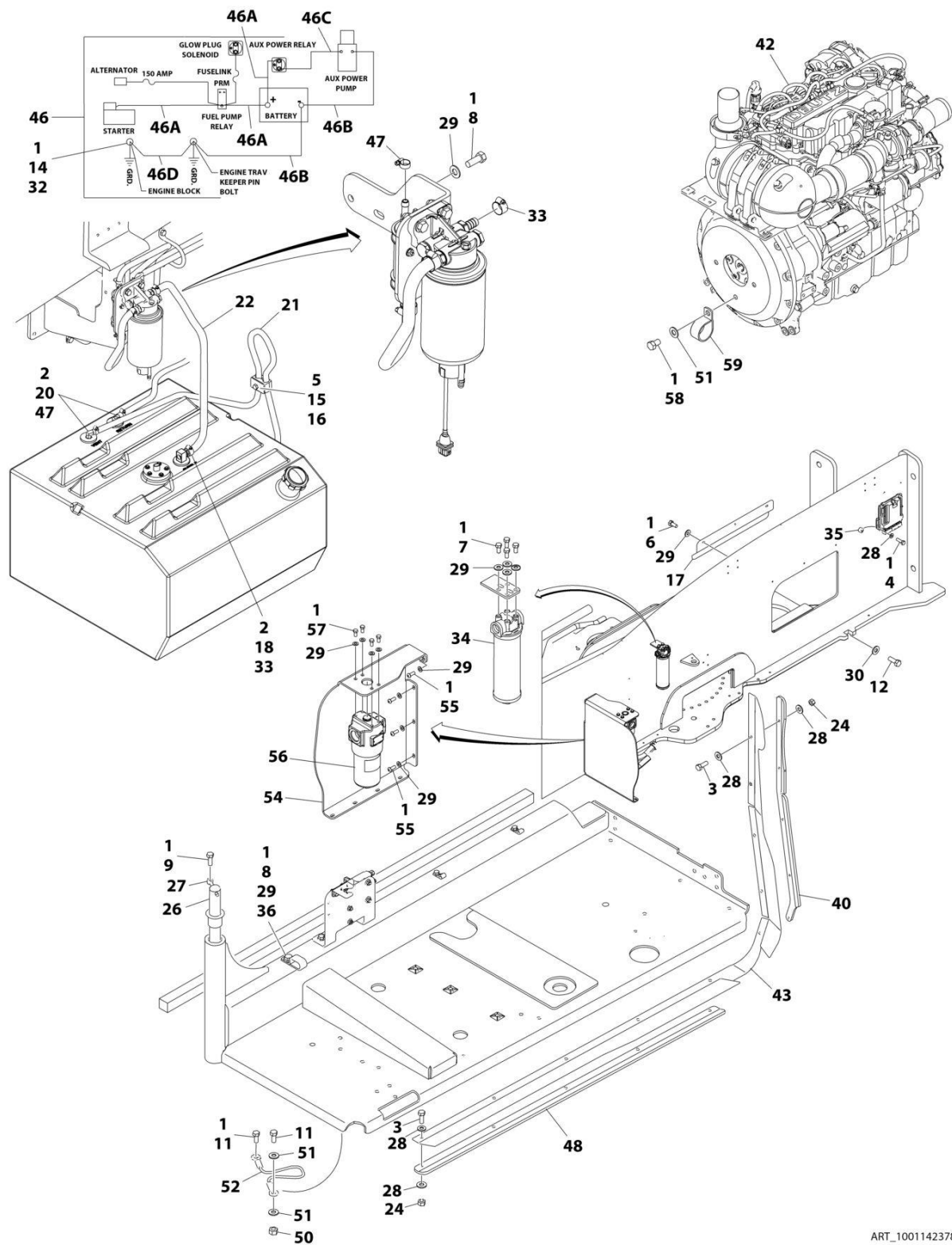
FIGURE 3-23. DEUTZ TCD2.9L4 EMR4 ENGINE INSTALLATION - WITH SAUER PUMPS (WITH COLD WEATHER PLUS PACKAGE)
