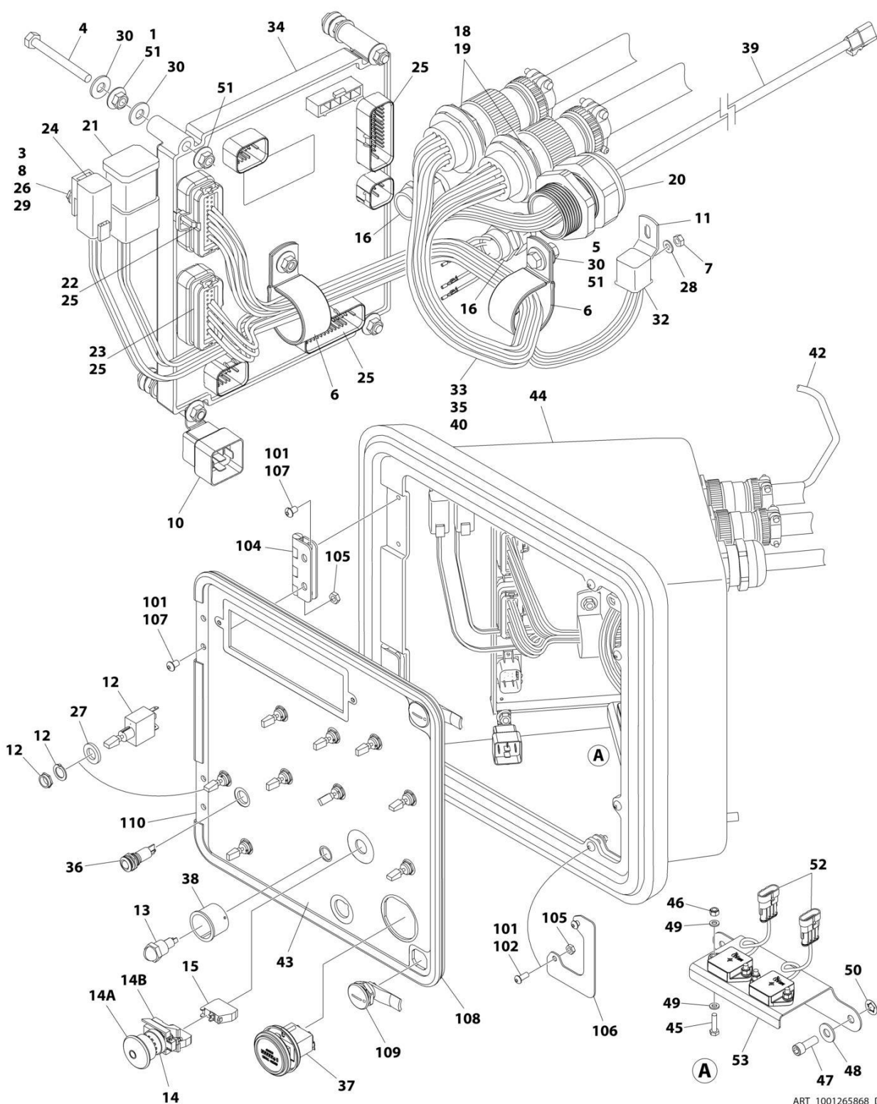
FIGURE 2-41. GROUND CONTROL ASSEMBLY - DEUTZ TD2011 ENGINES (WITH TOWER STOW) (CE & UK CA SPECS)
