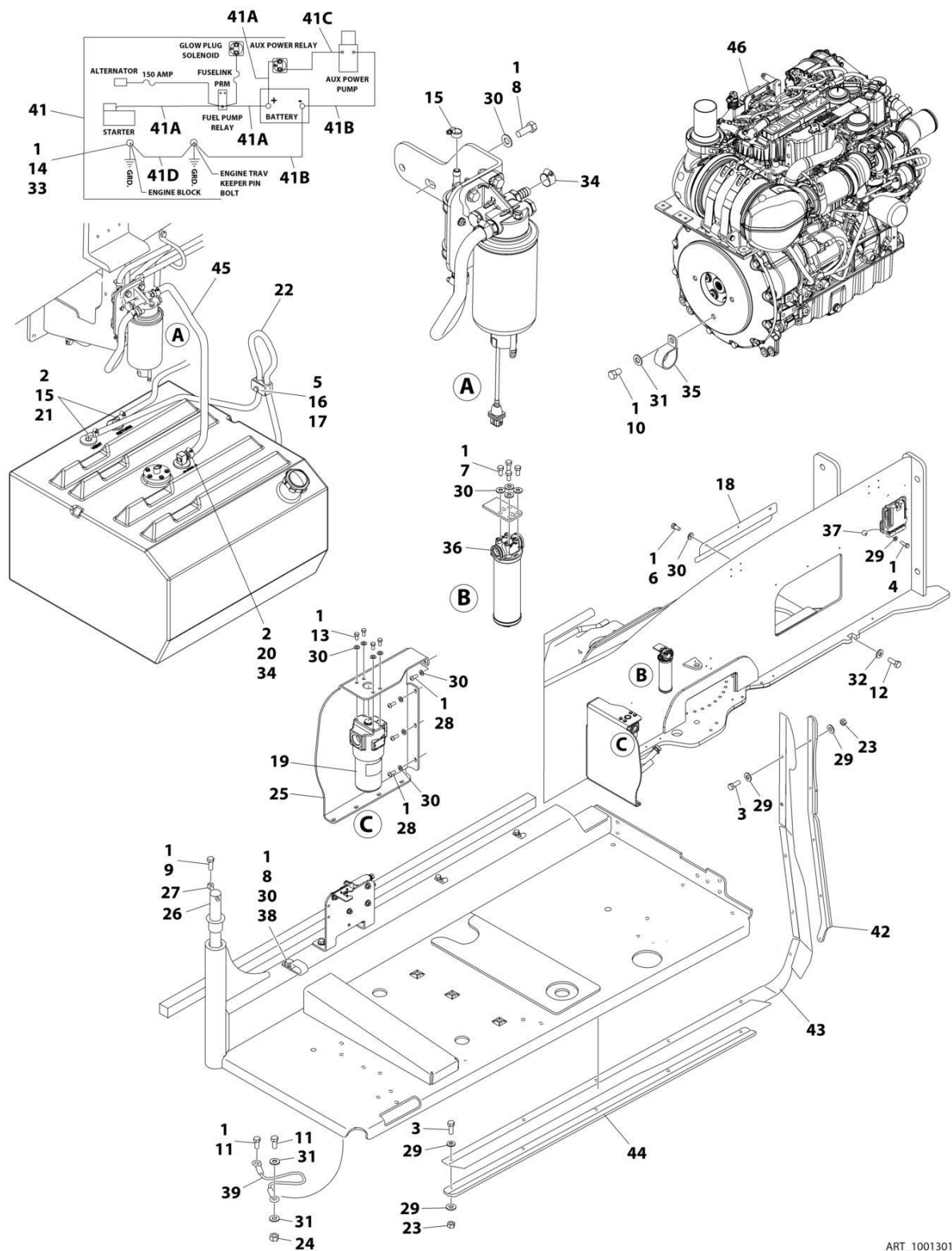
FIGURE 3-29. DEUTZ D2.9L4 - EMR5 ENGINE INSTALLATION WITH REXROTH PUMPS (WITHOUT COLD WEATHER PLUS PACKAGE)
