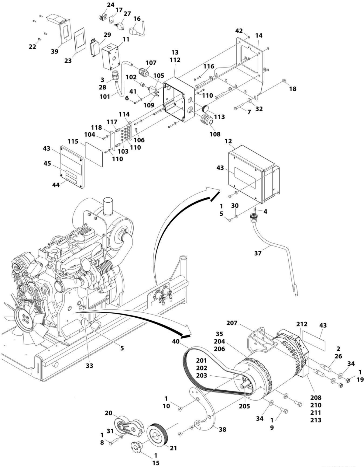
FIGURE 3-76. 4000W GENERATOR INSTALLATION - 60HZ SPEC (DEUTZ TCD2.9L4 ENGINES)
