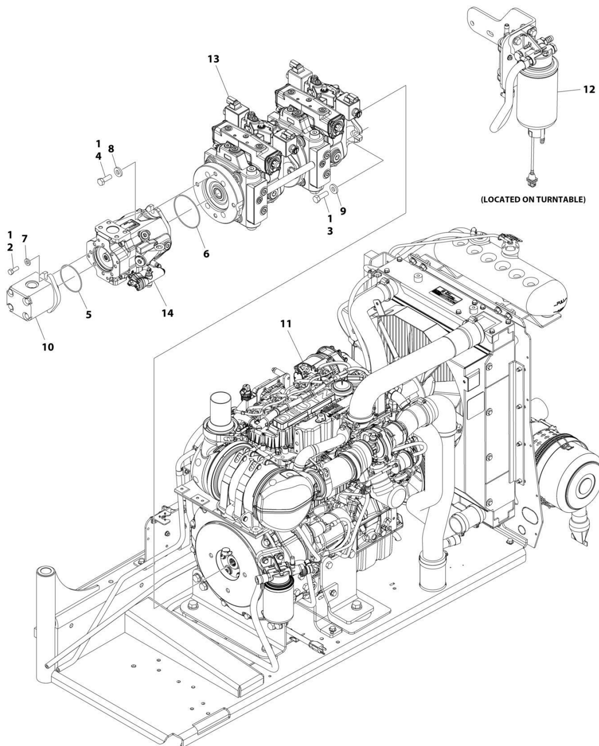
FIGURE 3-26. DEUTZ D2.9L4 (EMR4) ENGINE SUB-ASSEMBLY WITH PMP PUMP AND STEEL HOODS (WITH COLD WEATHER PLUS PACKAGE)
