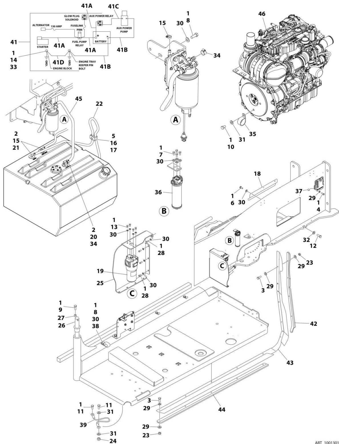
FIGURE 3-30. DEUTZ D2.9L4 - EMR5 ENGINE INSTALLATION WITH REXROTH PUMPS (WITH COLD WEATHER PLUS PACKAGE)
