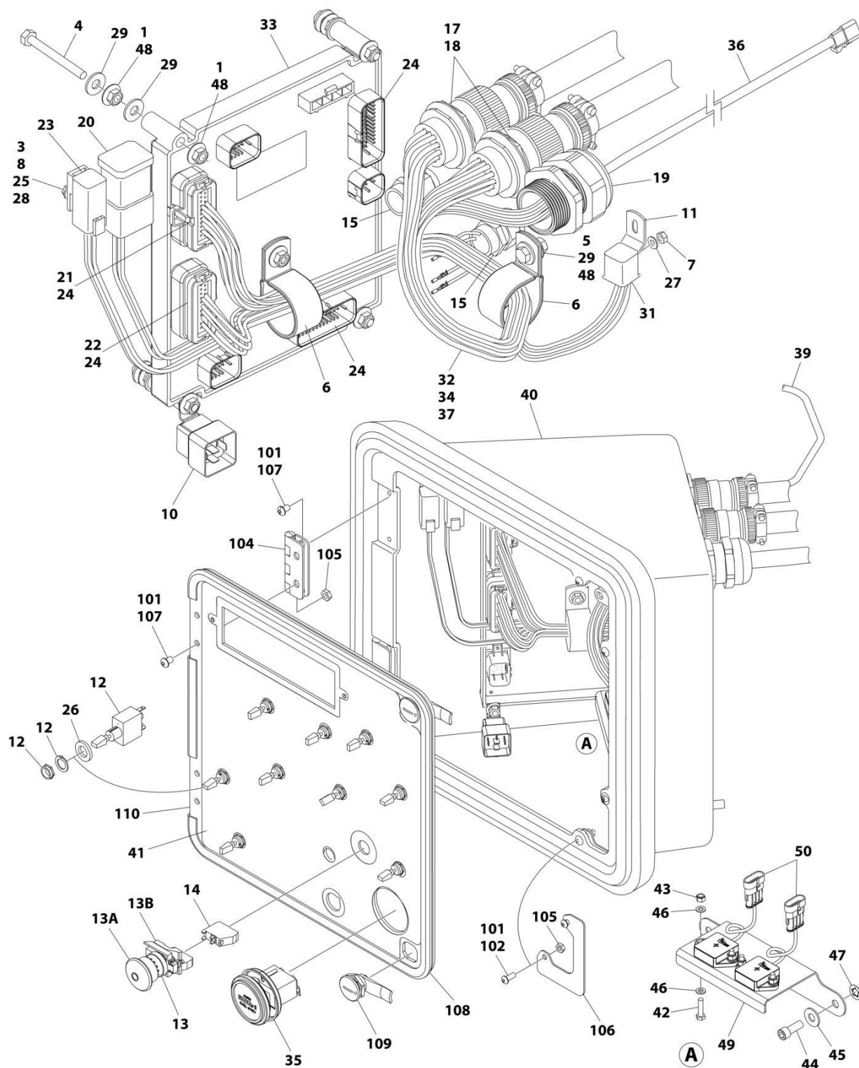
FIGURE 2-36. GROUND CONTROL ASSEMBLY - WITH DEUTZ TD2011 AND DEUTZ TCD2.9L4 ENGINES - WITH MECHANICAL HOUR METER (WITHOUT TOWER STOW) (ALL SPECS EXCEPT CE & UK CA SPECS)
