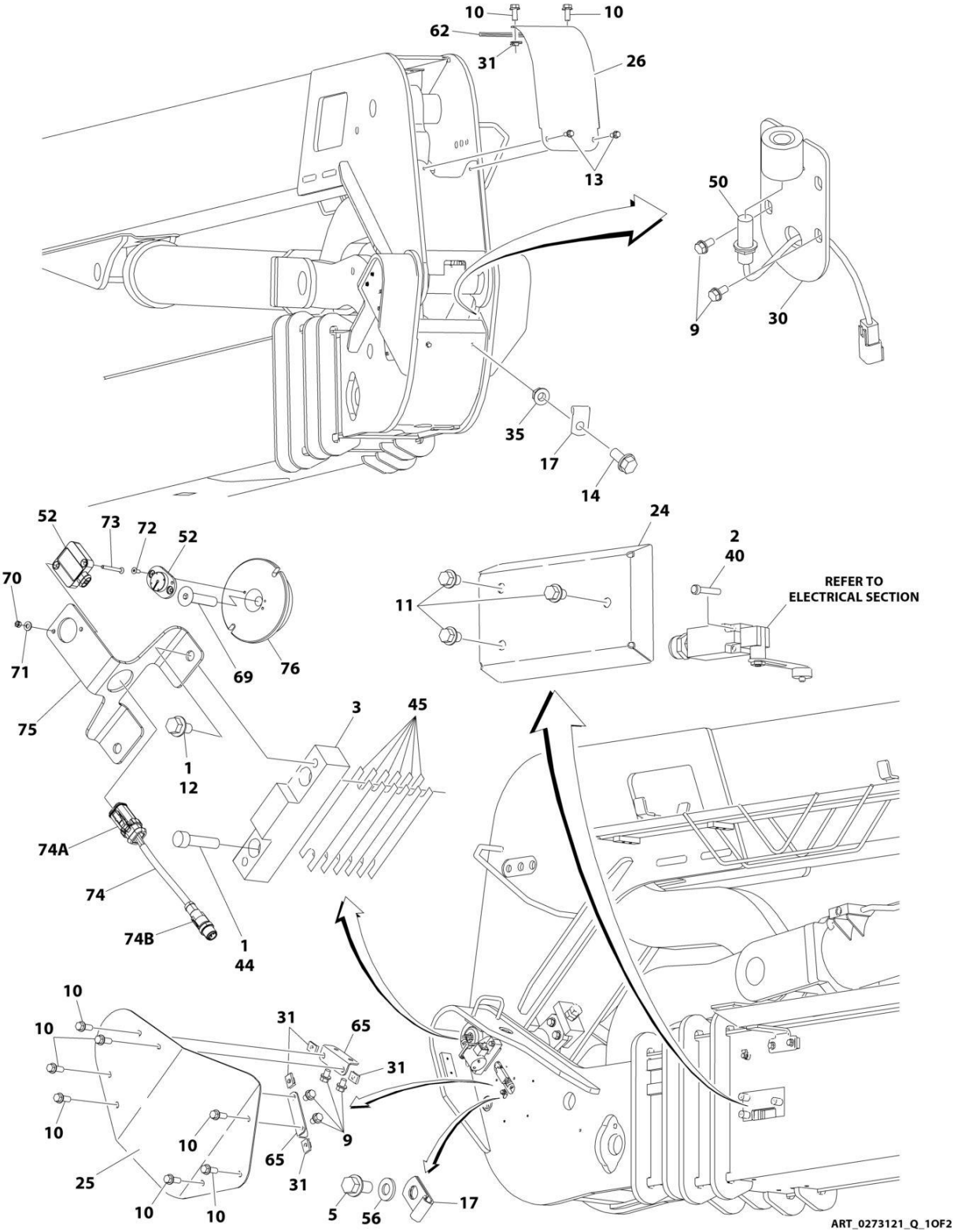
FIGURE 4-10. BOOM SENSORS AND SWITCHES INSTALLATION
