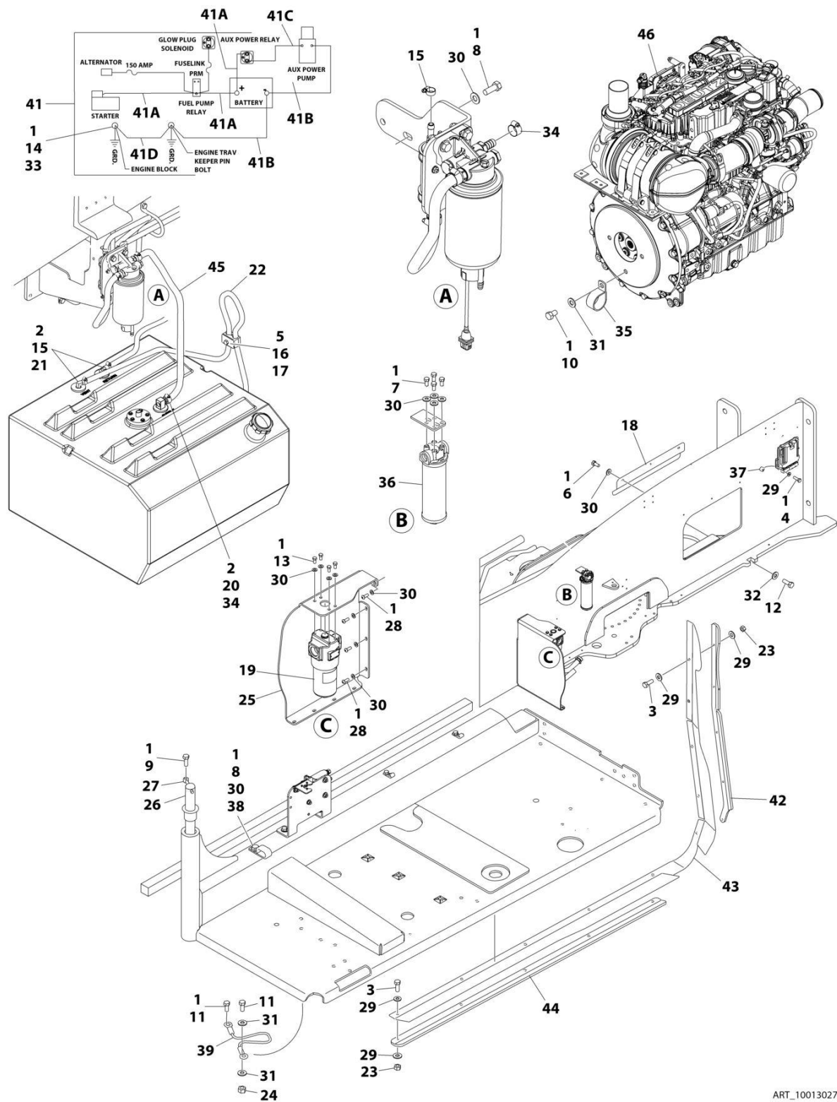
FIGURE 3-34. DEUTZ D2.9L4 - EMR5 ENGINE INSTALLATION WITH SAUER PUMPS (WITH COLD WEATHER PLUS PACKAGE)
