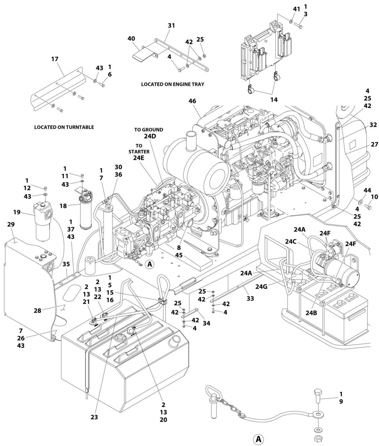
FIGURE 3-3. DEUTZ TD2011 ENGINE INSTALLATION - WITH REXROTH PUMP (WITH GENERATOR AND WITHOUT COLD WEATHER PLUS PACKAGE)
