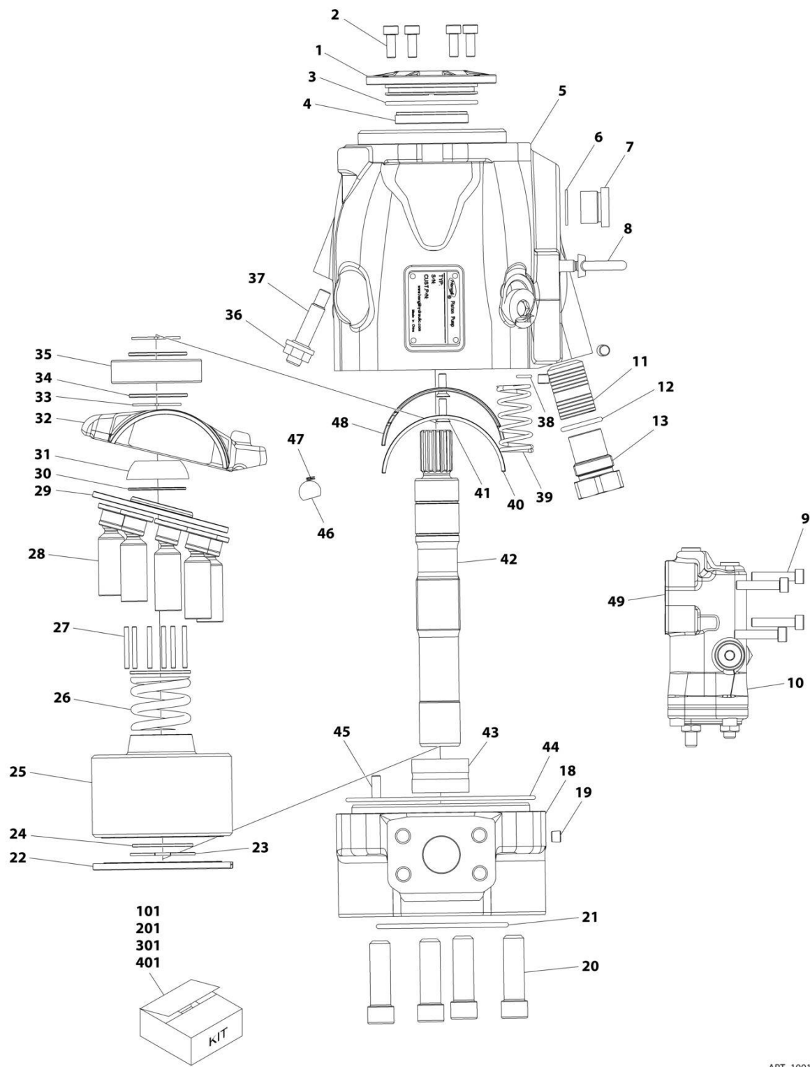
FIGURE 3-48. PUMP ASSEMBLY - HYDRAULIC PISTON
