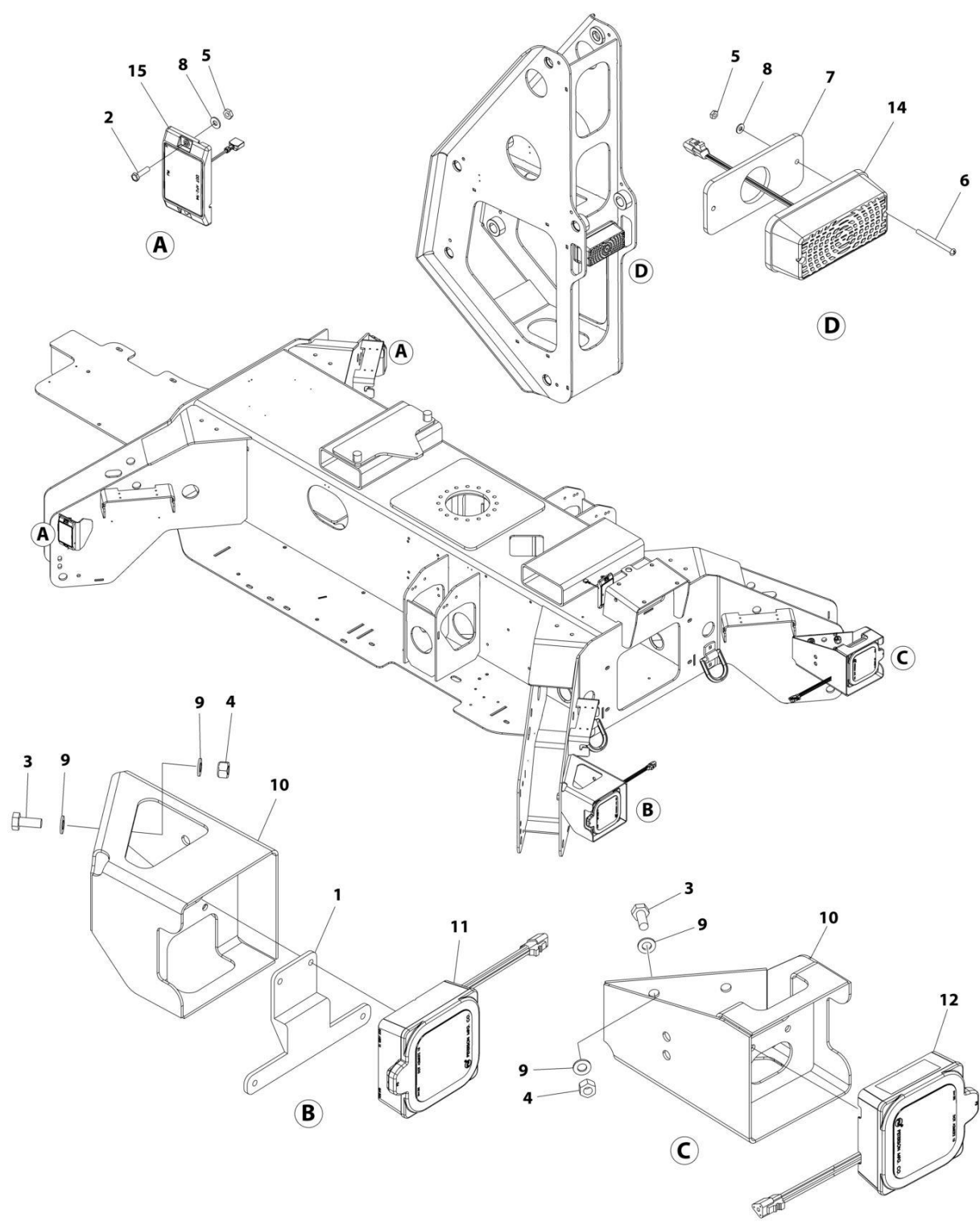
FIGURE 1-23. TAILLIGHTS AND MARKERS INSTALLATION
