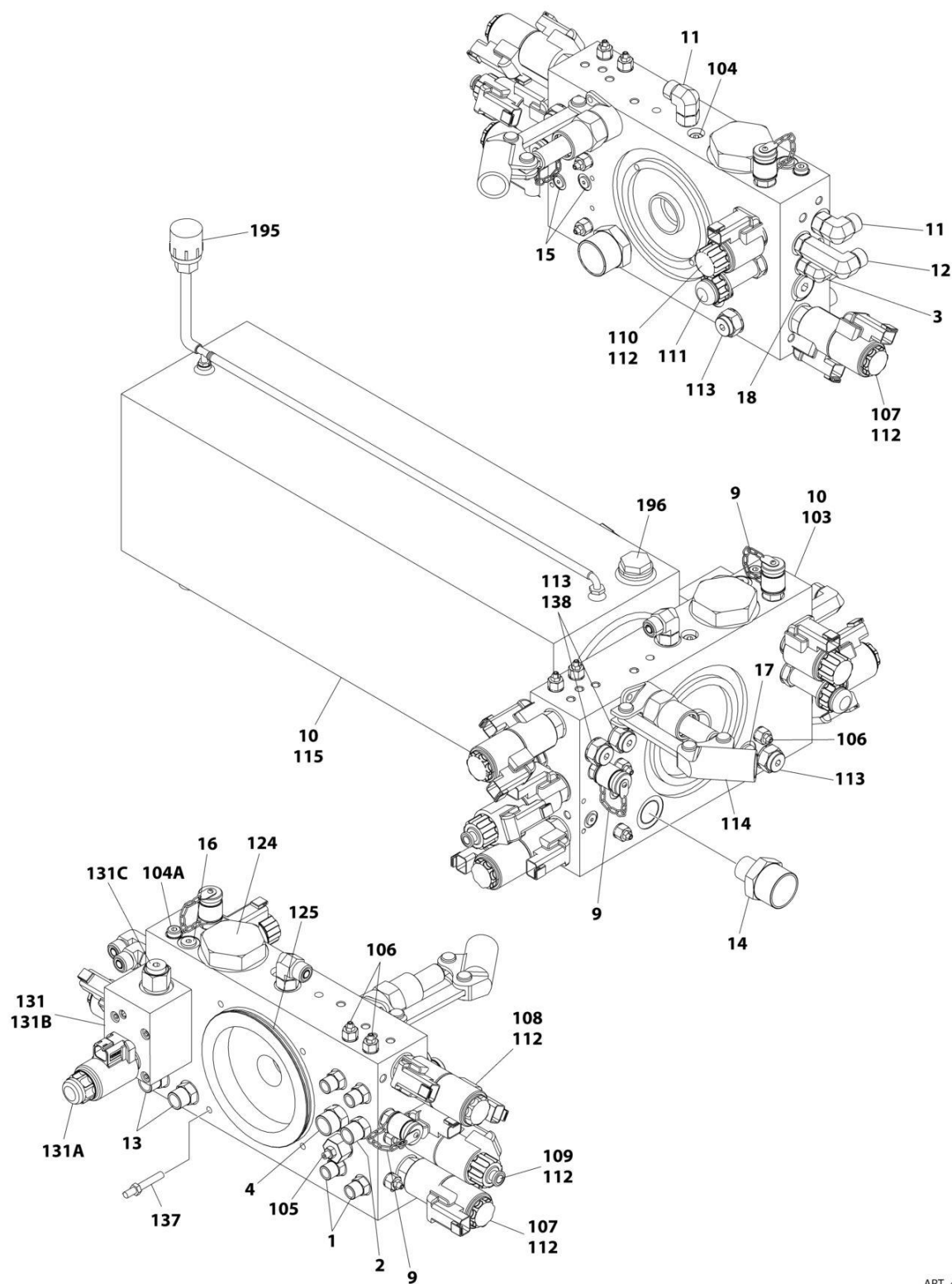
FIGURE 1-14. CONTROL VALVE ASSEMBLY (GAS POWERED MACHINES) (T350)
