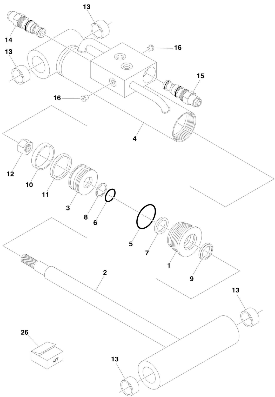
FIGURE 5-4. PLATFORM LEVEL CYLINDER ASSEMBLY
