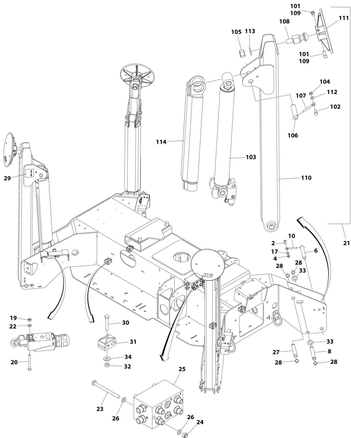
FIGURE 1-20. OUTRIGGERS INSTALLATION
