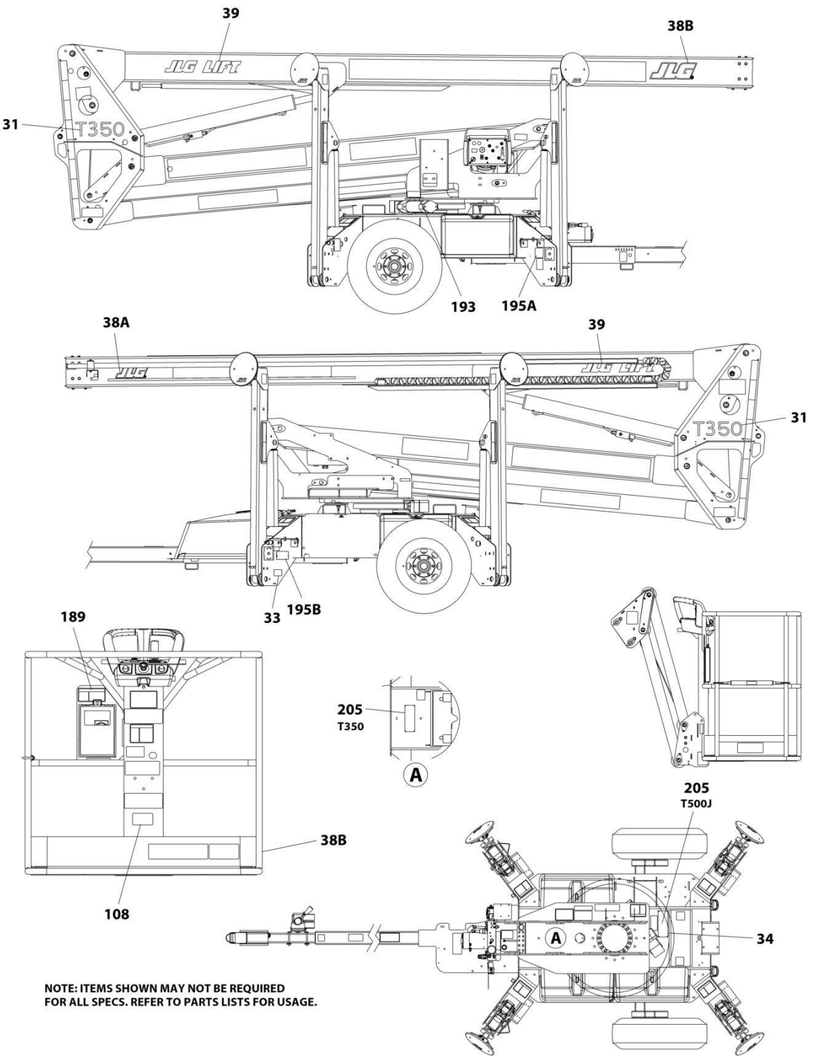
FIGURE 8-7. DECAL INSTALLATION - OPTIONS
