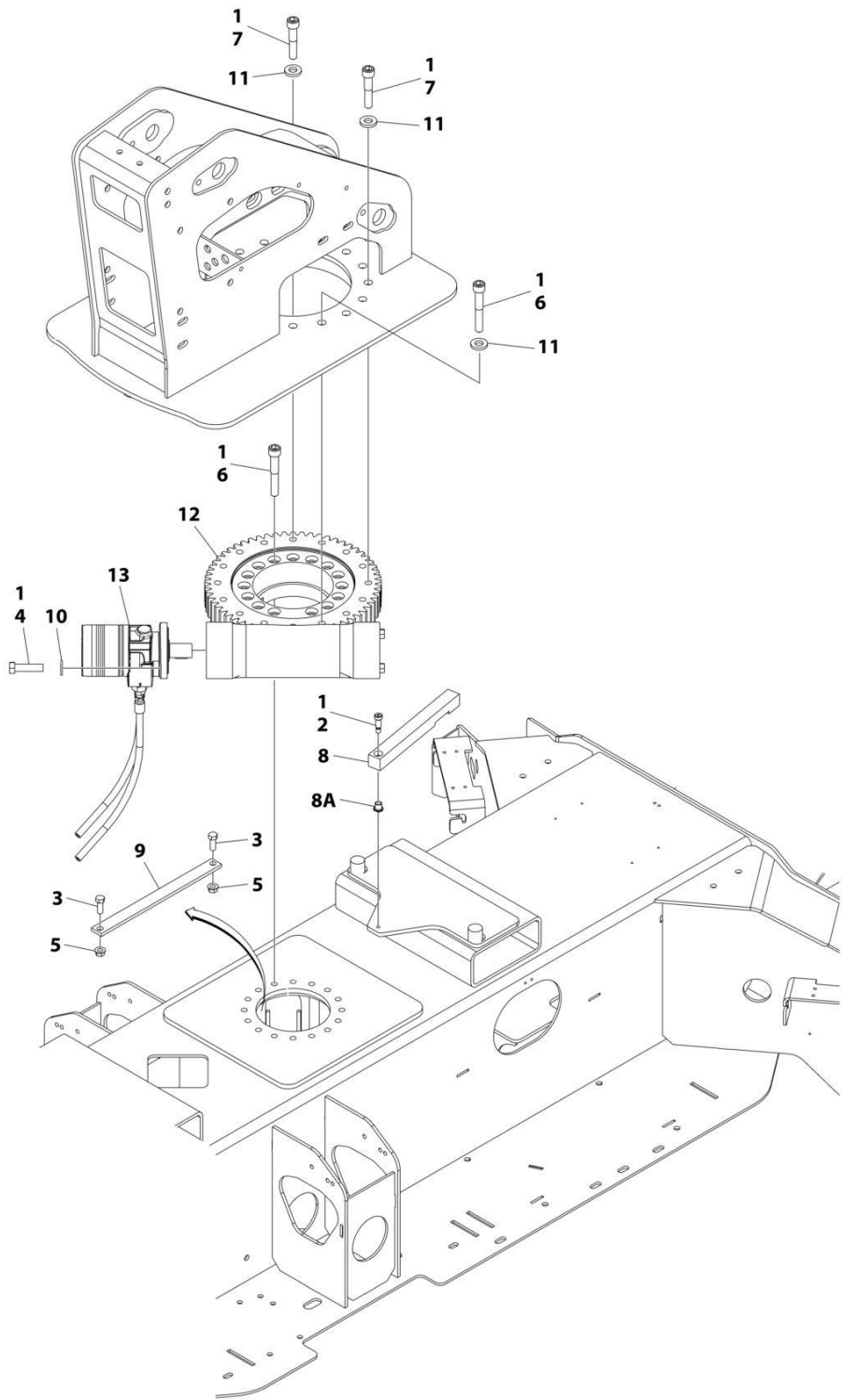
FIGURE 2-4. TURNTABLE BEARING INSTALLATION (WITH JING WEI BEARING/ WITH ZHENJIANG MOTOR)
