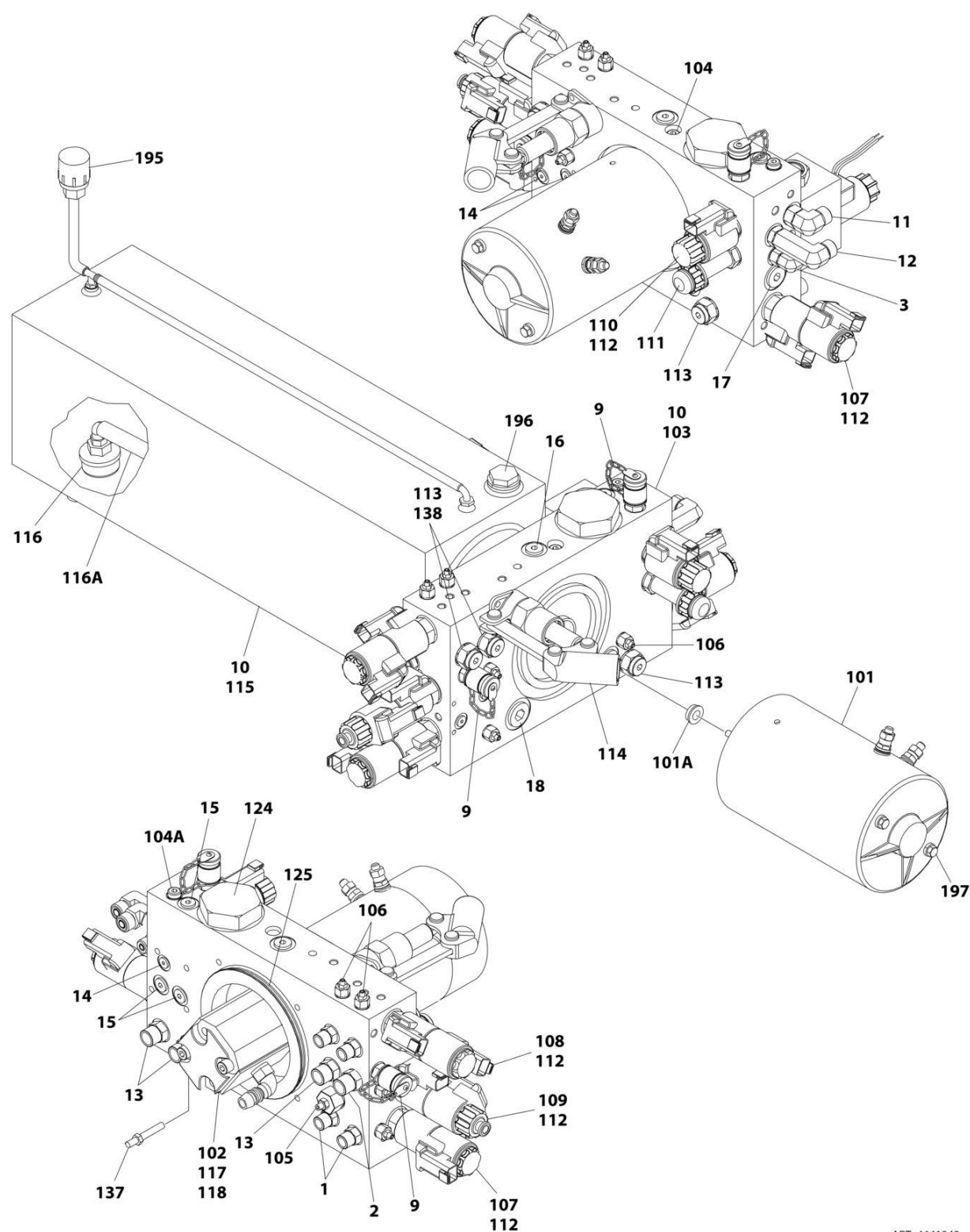
FIGURE 1-13. CONTROL VALVE ASSEMBLY (ELECTRIC POWERED MACHINES) (ET350)
