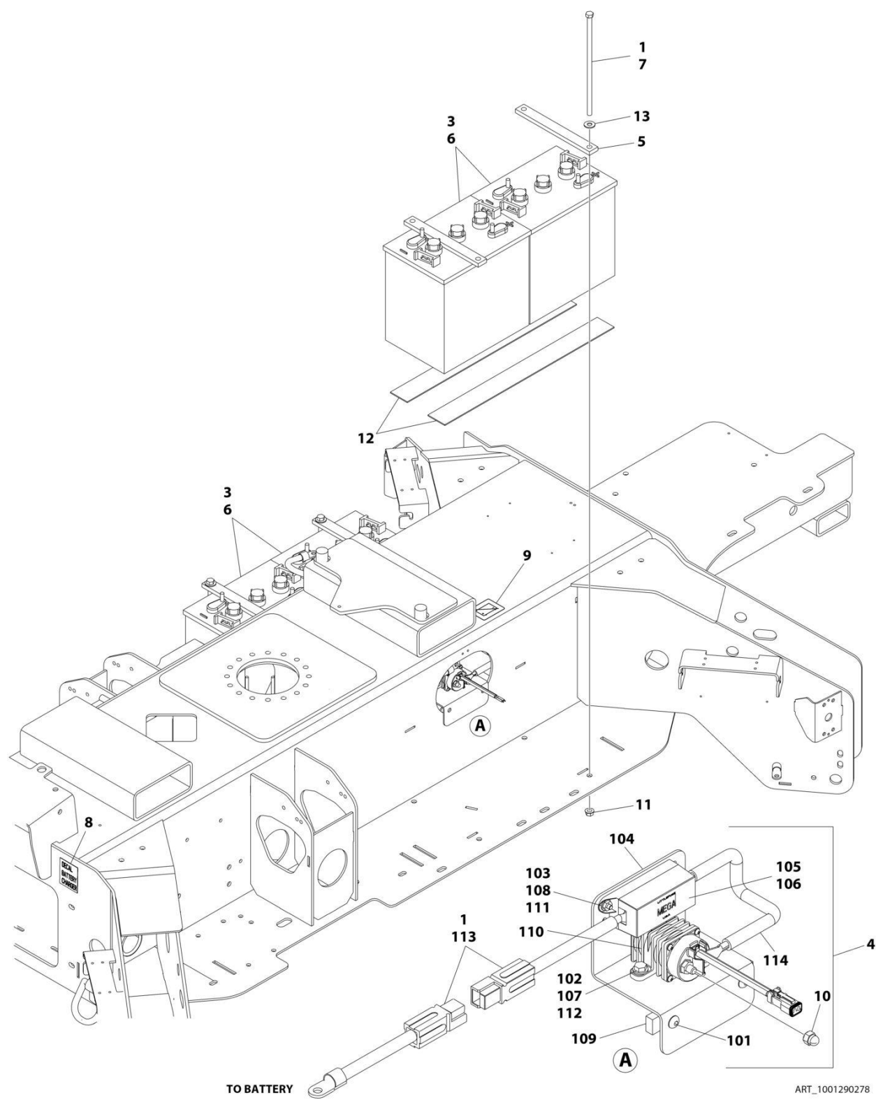
FIGURE 1-4. BATTERIES INSTALLATION
