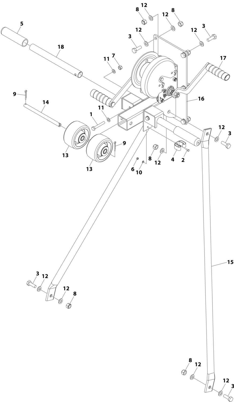
FIGURE 2-1. WINCH INSTALLATION - MANUAL
