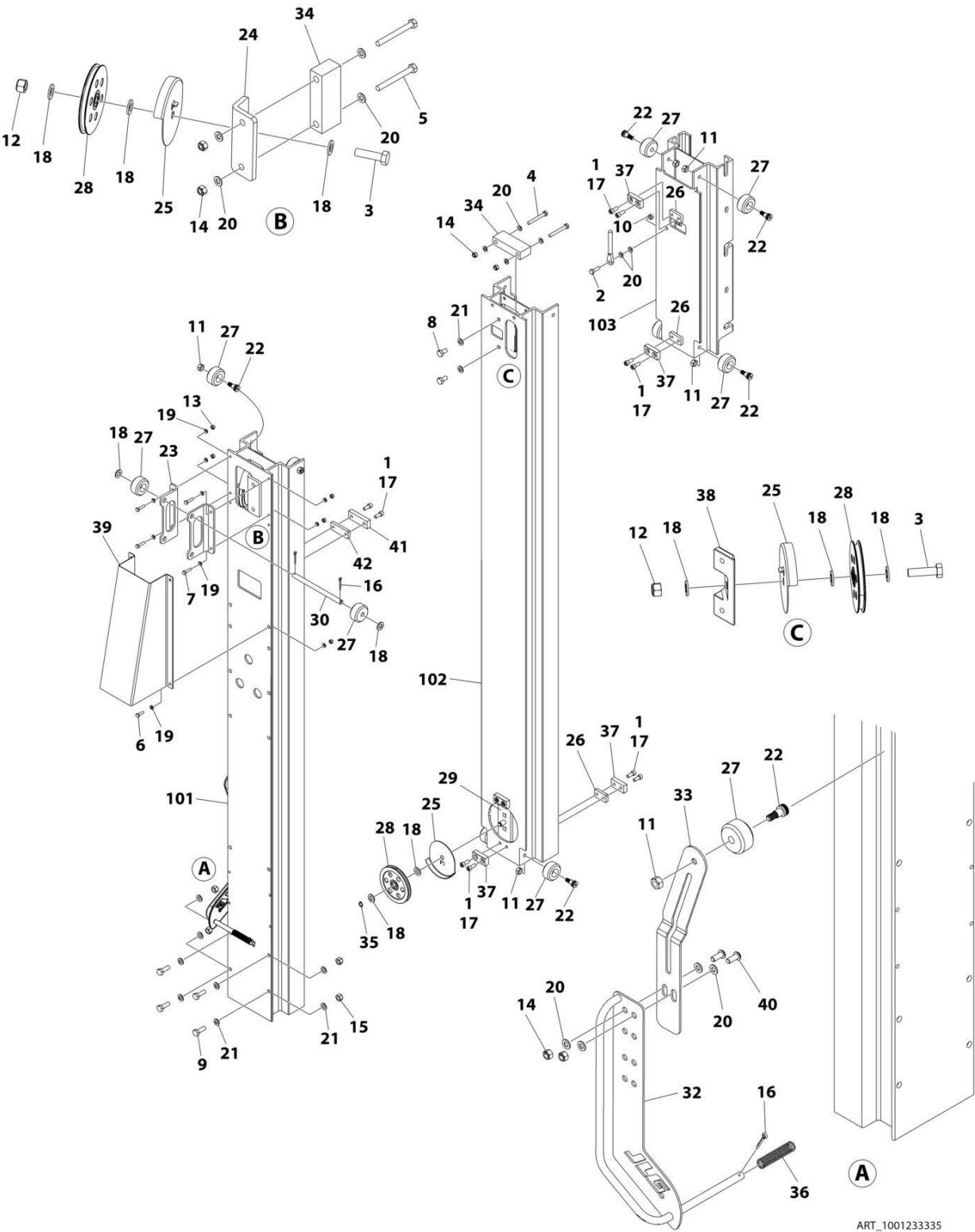
FIGURE 3-1. MAST ASSEMBLY (10ML)
