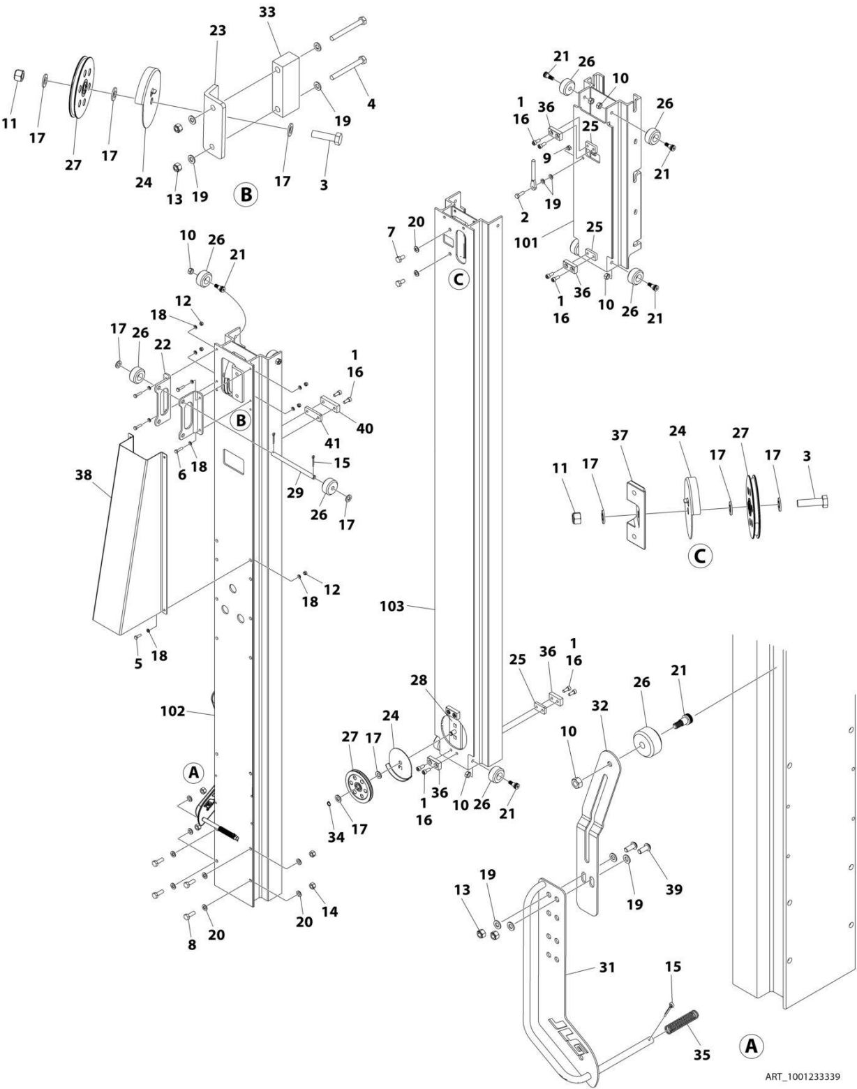
FIGURE 3-2. MAST ASSEMBLY (12MLC)
