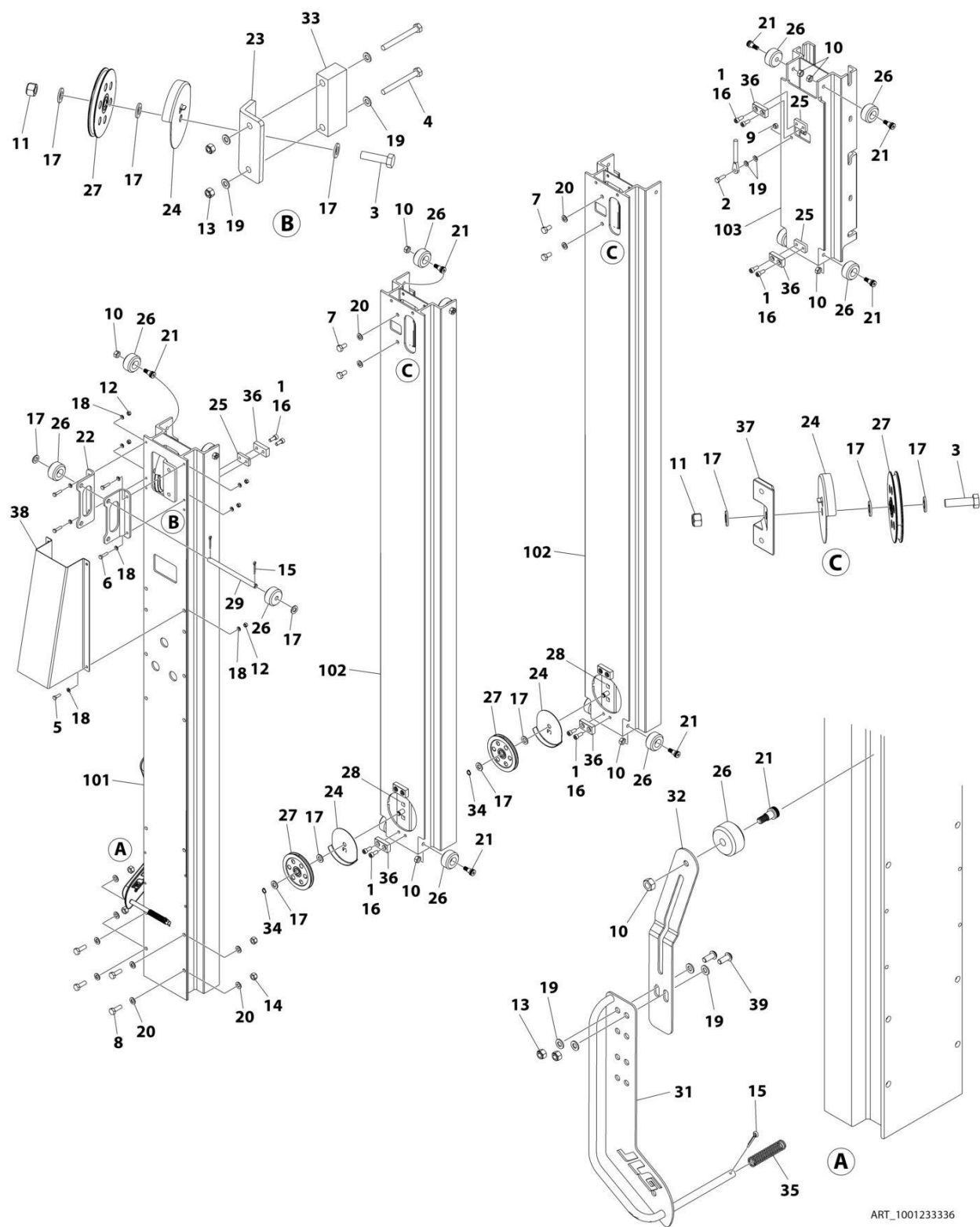
FIGURE 3-3. MAST ASSEMBLY (15ML)
