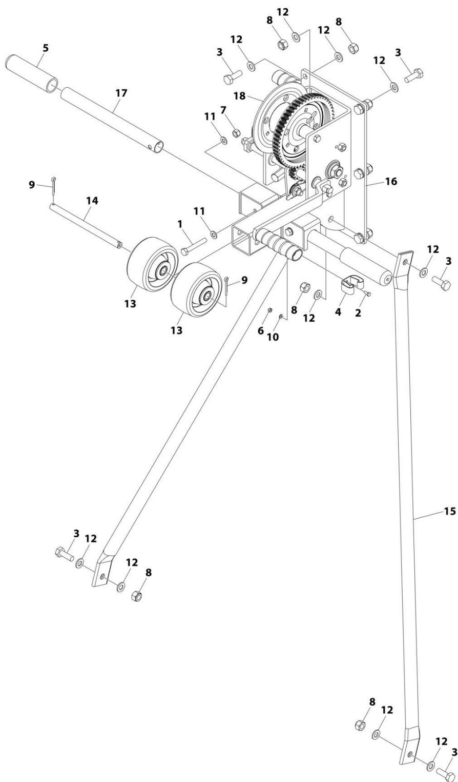
FIGURE 2-2. WINCH INSTALLATION - DRILL DRIVEN
