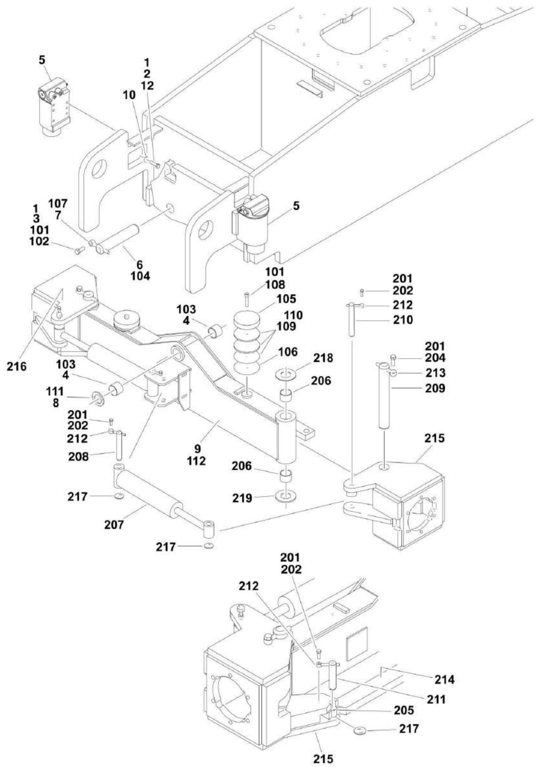
FIGURE 1-4. 4WD FRONT AXLE AND STEERING INSTALLATION (SN 0300075606 through 0300087000)
