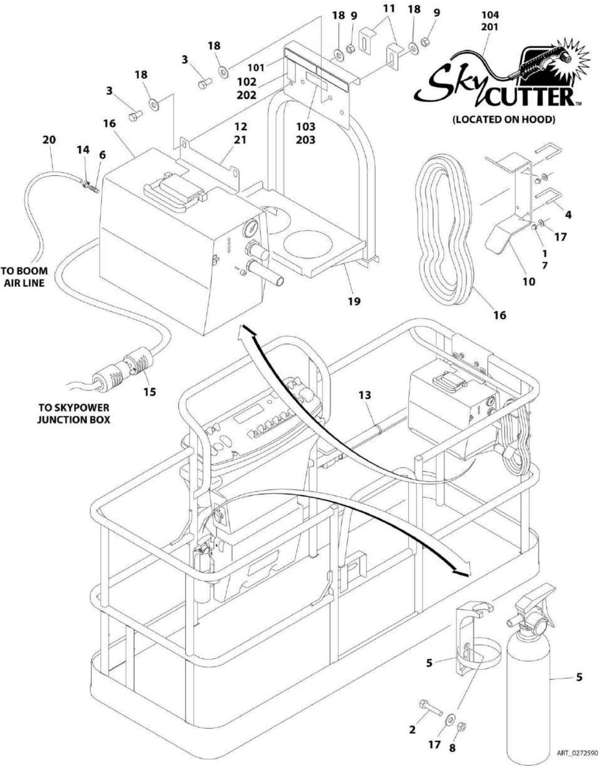
FIGURE 4-17. SKYCUTTER INSTALLATION
