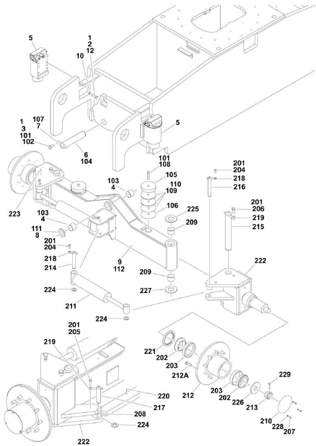
FIGURE 1-2. 2WD FRONT AXLE AND STEERING INSTALLATION (SN 0300075606 through 0300087000)
