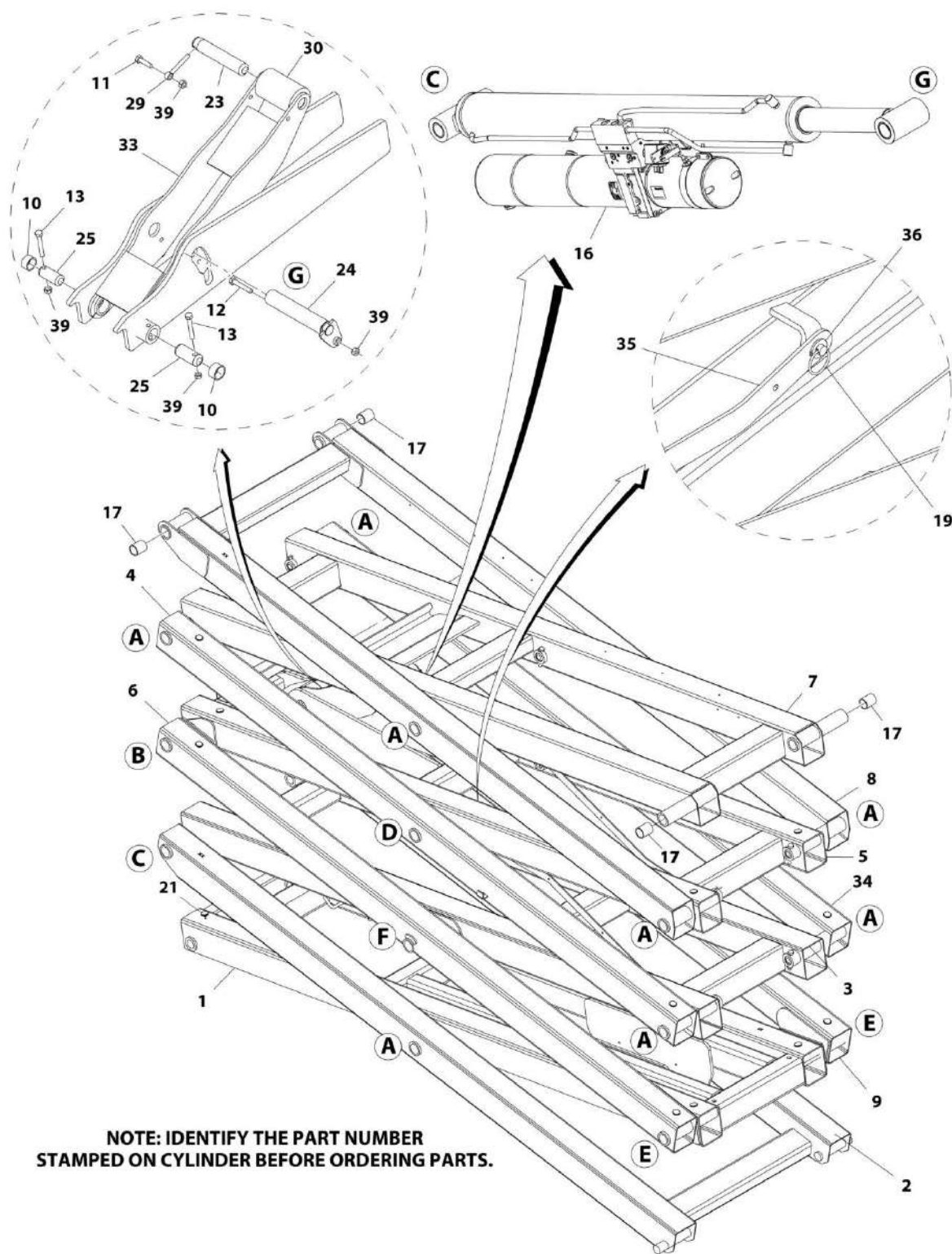
FIGURE 3-26. SCISSOR ARMS ASSEMBLY - 3246ES BIODEGRADABLE HYDRAULIC OIL (USA BUILT MACHINES) (SN 0200239382 through 0200241220)
