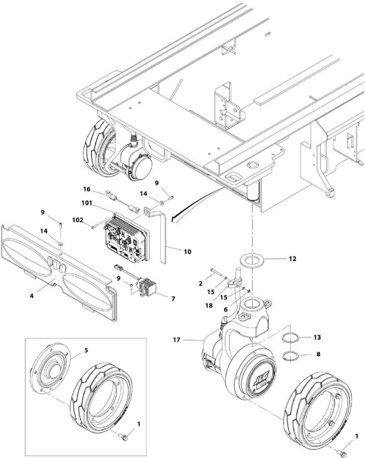
FIGURE 1-4. DRIVE HUB AND MODULE INSTALLATION (BELGIUM BUILT MACHINES ONLY)
