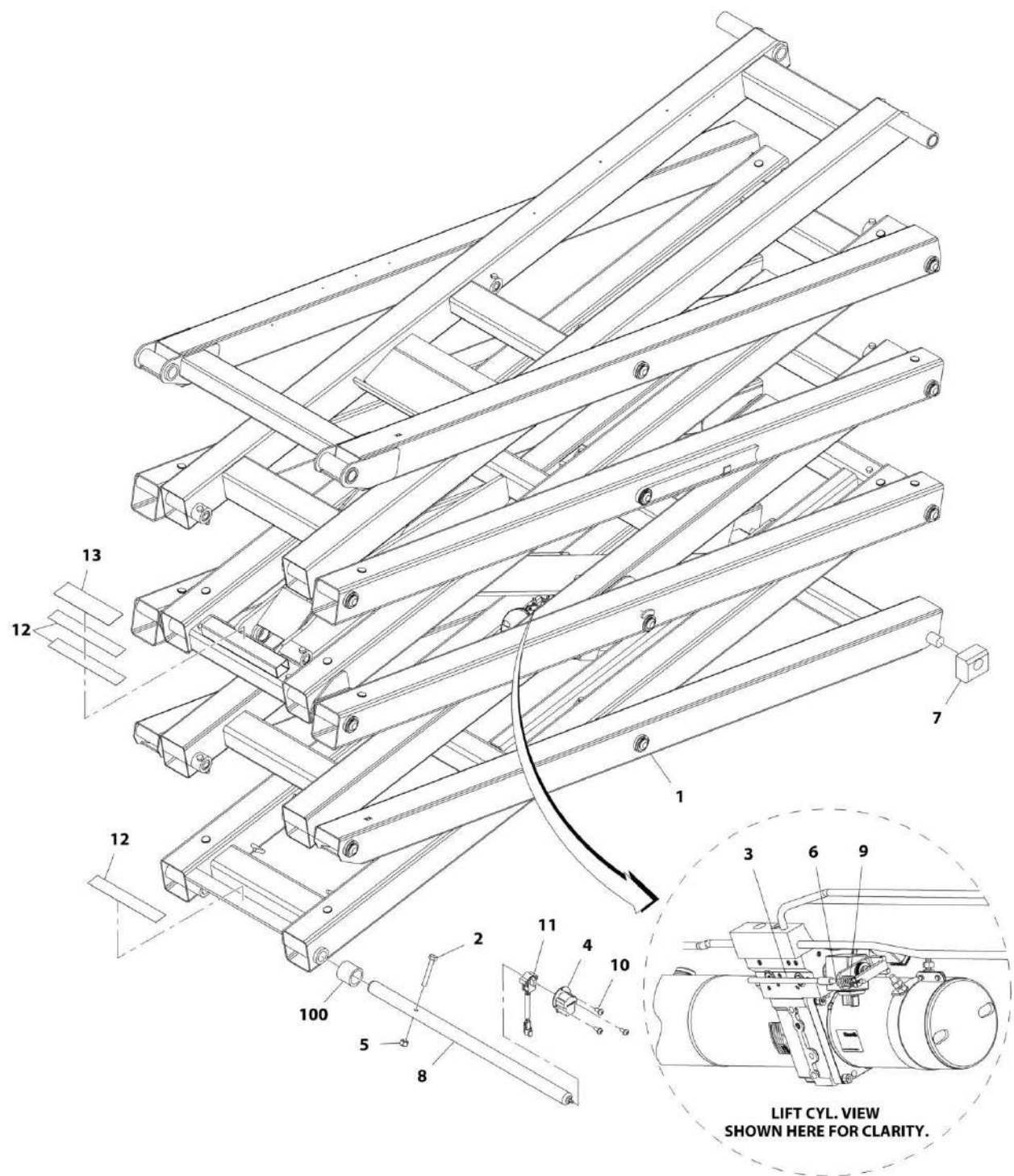
FIGURE 3-25. SCISSORS ARMS INSTALLATION - 3246ES BIODEGRADEABLE HYDRAULIC OIL (USA BUILT MACHINES) (SN 0200239382 through 0200241220)
