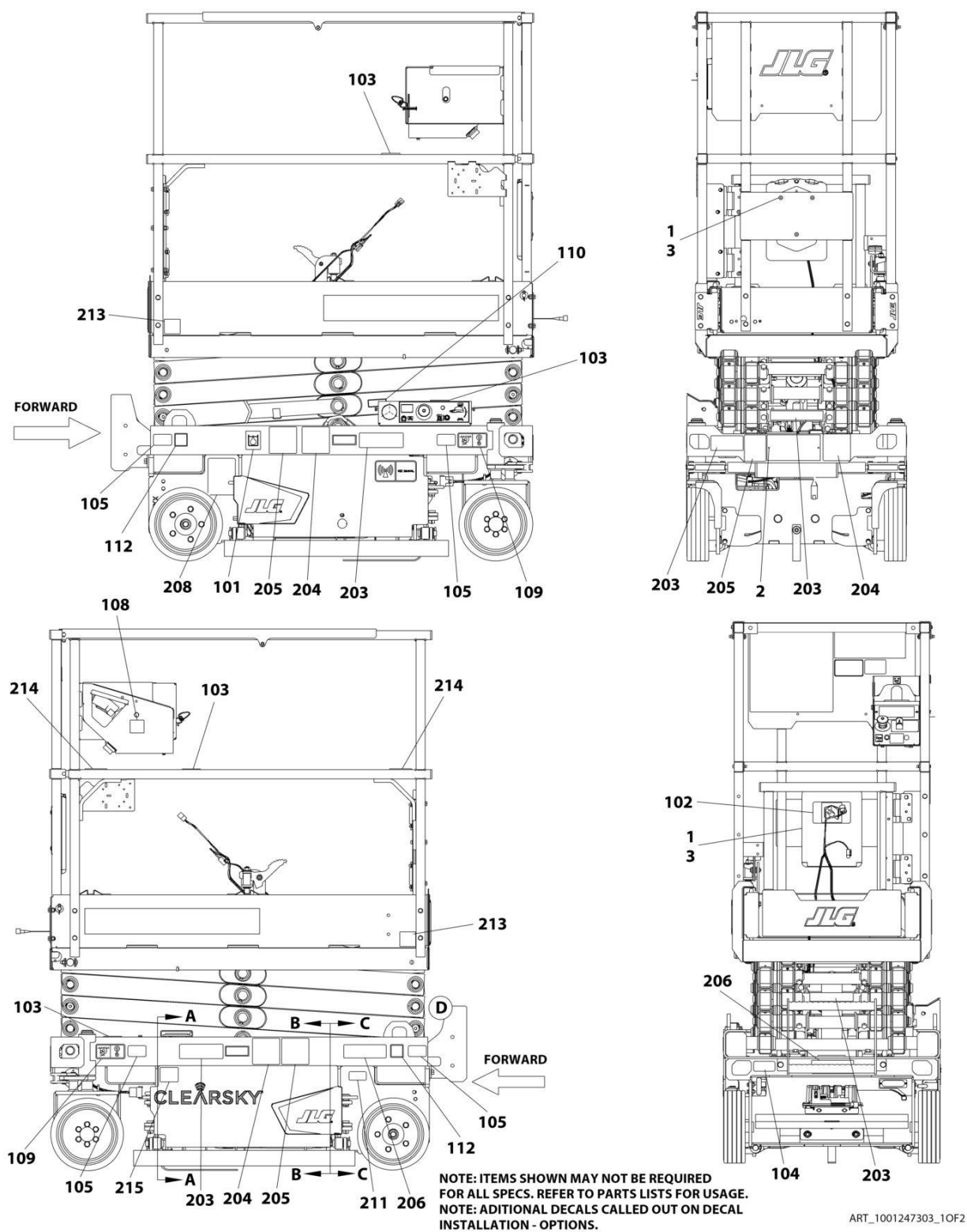
FIGURE 8-4. DECAL INSTALLATION (CHINA SPECS)
