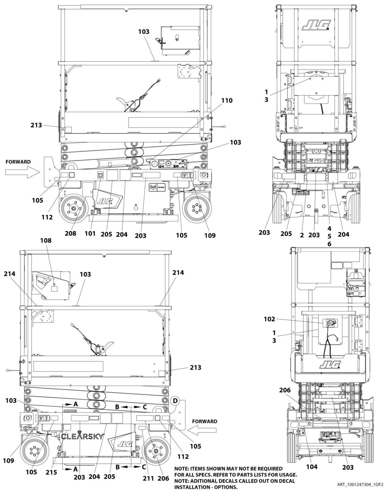
FIGURE 8-6. DECAL INSTALLATION (JAPANESE SPECS)
