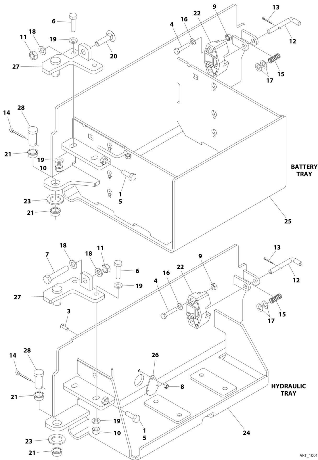
FIGURE 2-13. DOORS INSTALLATION
