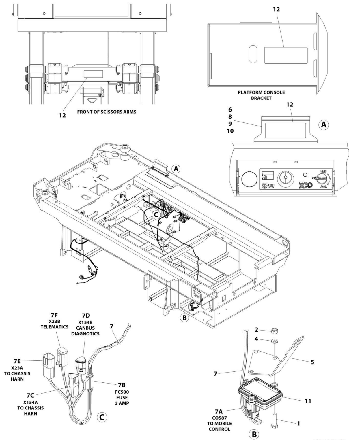
FIGURE 2-10. MOBILE CONTROL INSTALLATION
