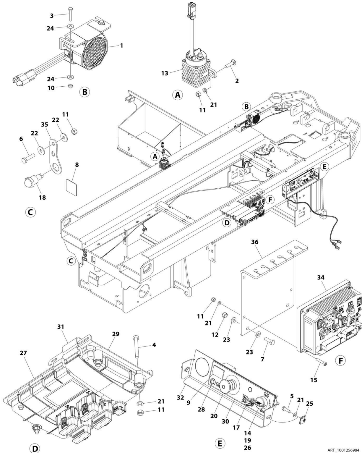
FIGURE 2-4. ELECTRICAL COMPONENTS INSTALLATION (MACHINES WITH SN STARTING WITH B2 & M2) (Prior to SN B200079218, Prior to SN M200064560, SN M200064738 through M200064741, SN M200064828 through M200064838, SN M200064924 through M200064927, Including M200064659, M200064755 and M200064851)
