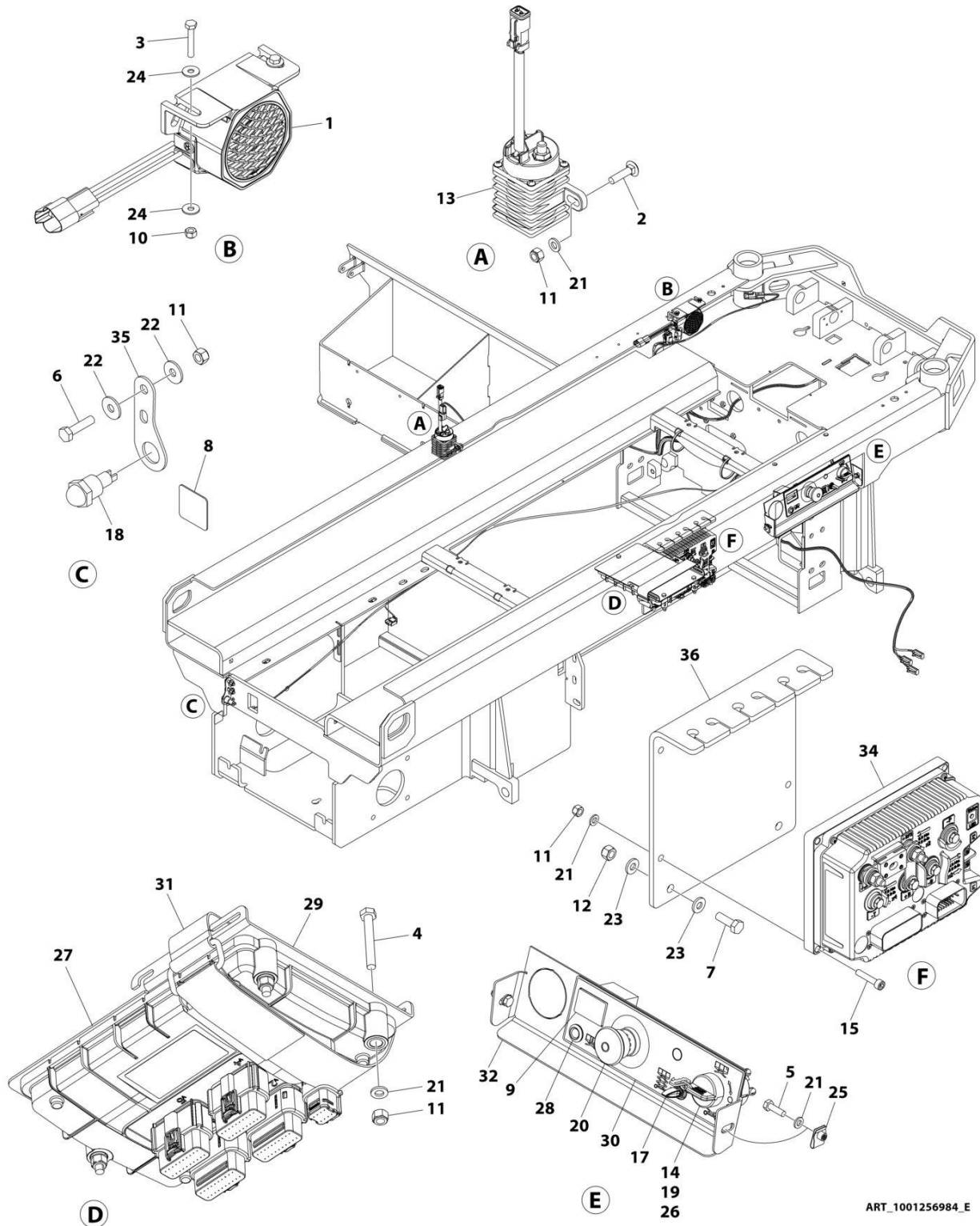
FIGURE 2-5. ELECTRICAL COMPONENTS INSTALLATION (MACHINES WITH SN STARTING WITH B2 & M2) (SN B200079218 to Present, SN M200064560 to Present, Except SN M200064738 through M200064741, Except SN M200064828 through M200064838, Except SN M200064924 through M200064927, Excluding M200064659, M200064755 and M200064851)
