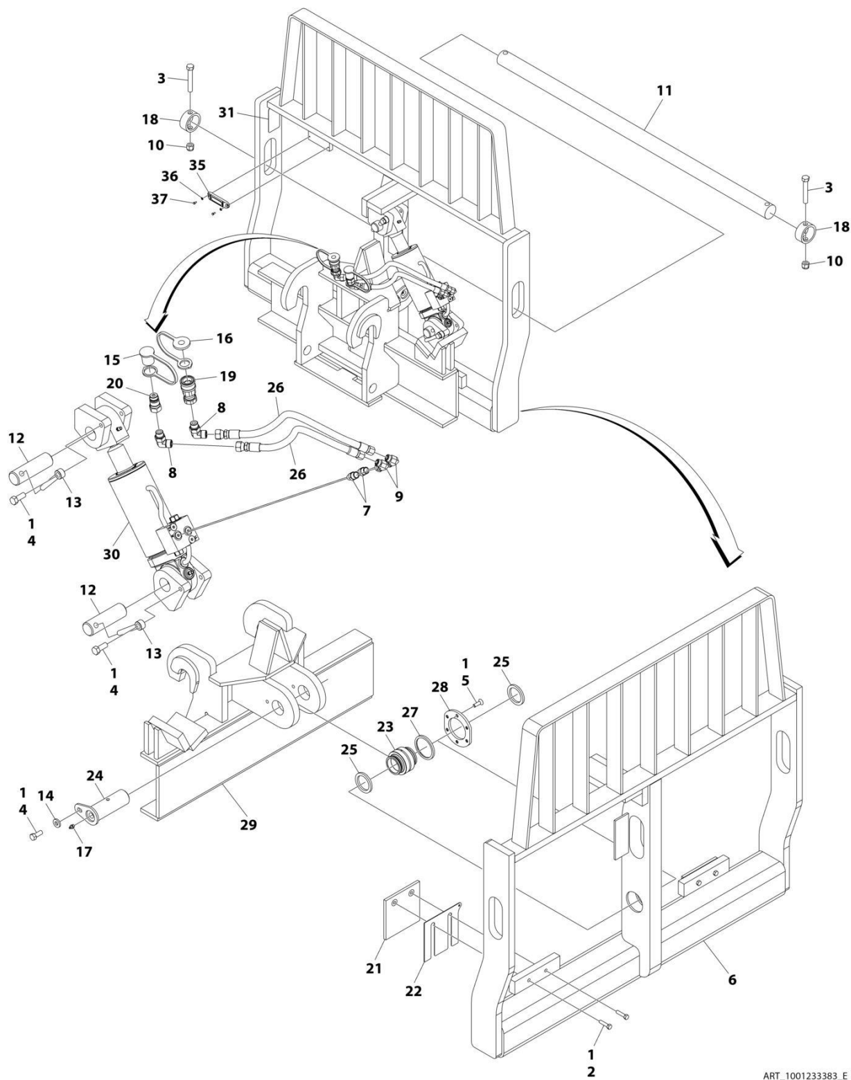
FIGURE 3-21. CARRIAGE ASSEMBLY - 50IN SIDE TILT (Prior to SN 0160116805)
