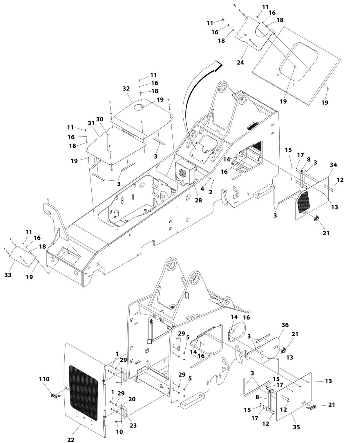
FIGURE 1-6. FRAME COVERS INSTALLATION, 85HP (LS)
