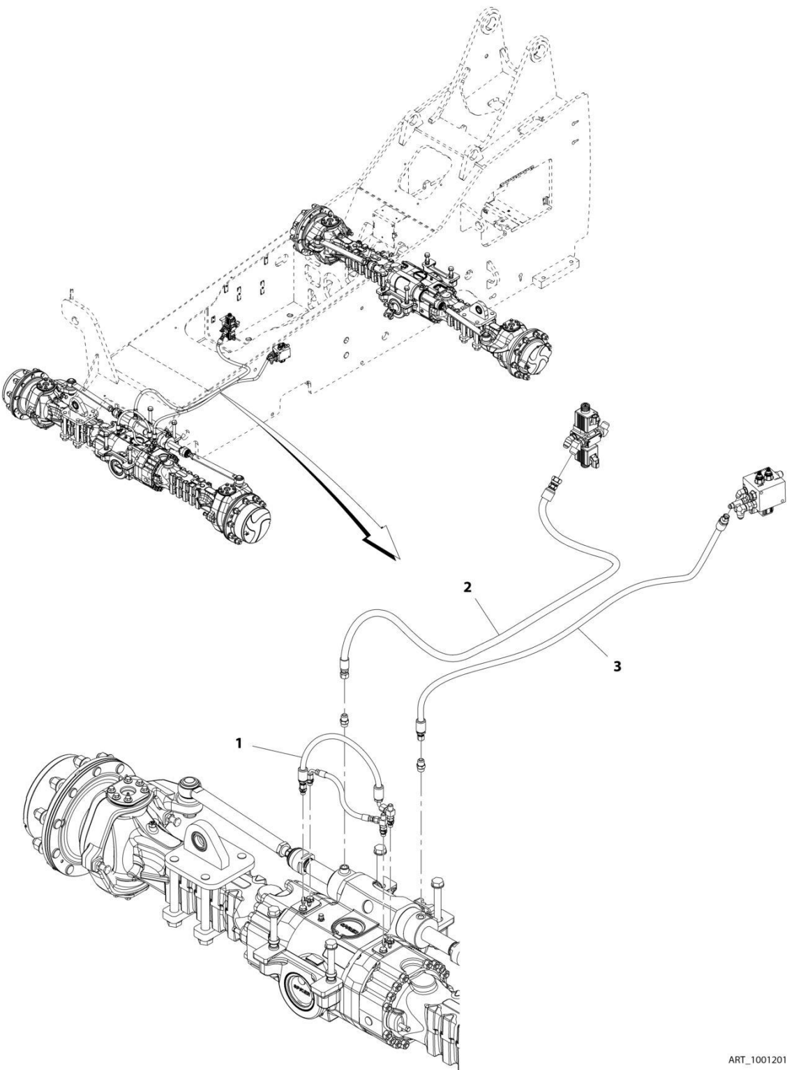
FIGURE 8-3. AXLE (FRONT) HYDRAULICS INSTALLATION
