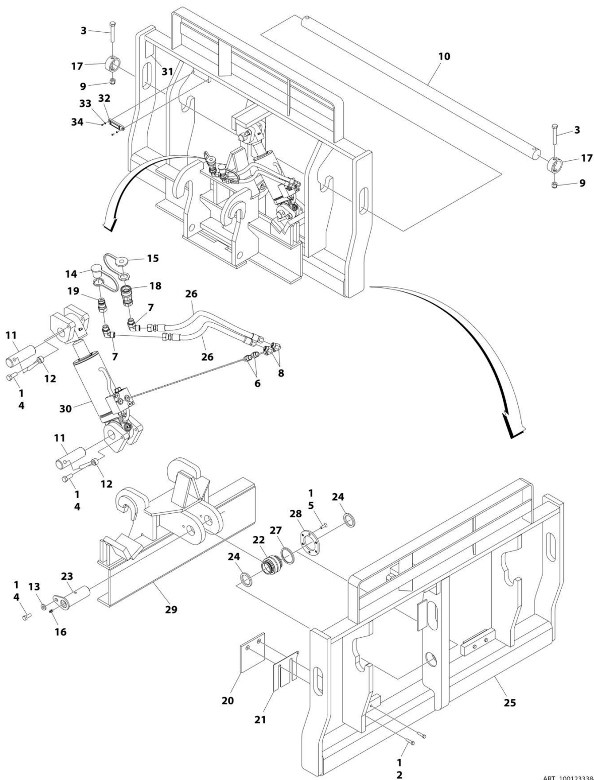
FIGURE 3-24. CARRIAGE ASSEMBLY - 60IN SIDE TILT (Prior to SN 0160116805)
