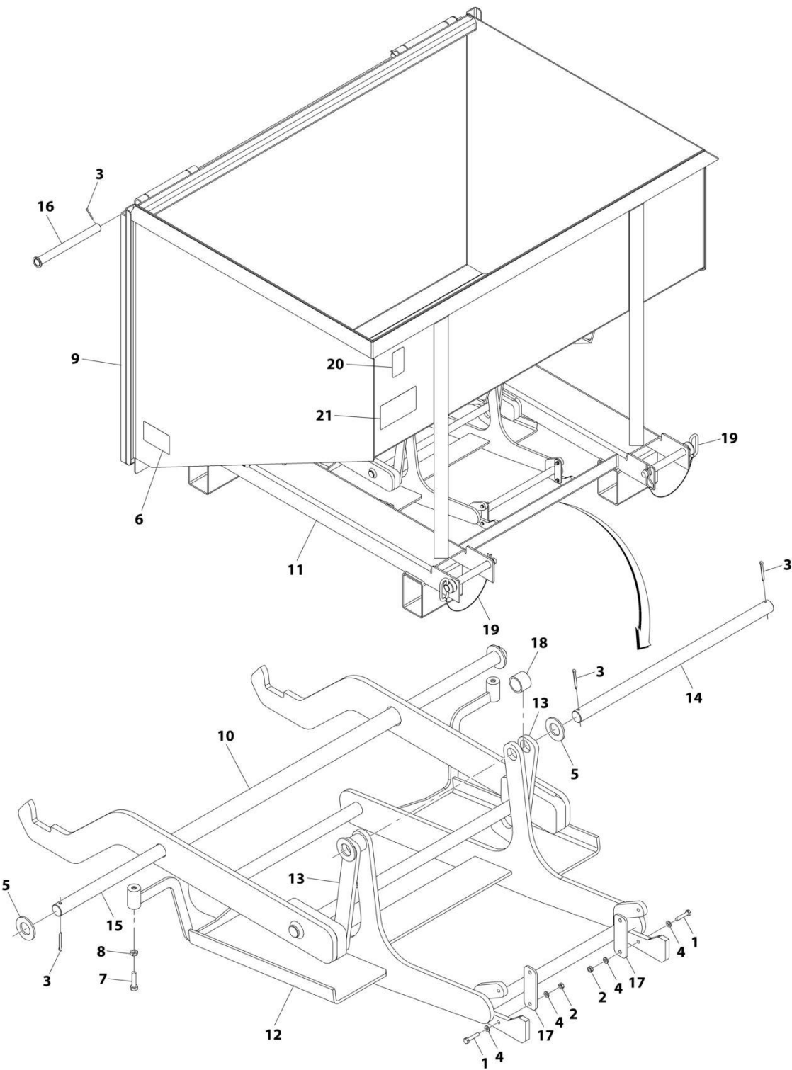
FIGURE 3-56. TRASH HOPPER - FORK MOUNTED
