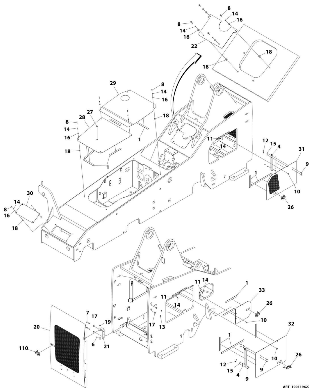
FIGURE 1-5. FRAME COVERS INSTALLATION, 74HP (ULS)
