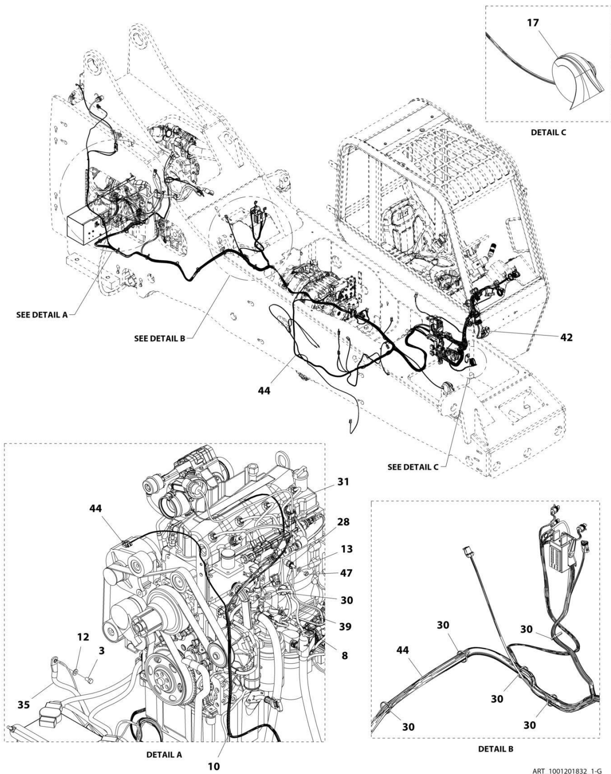
FIGURE 10-2. ELECTRICAL INSTALLATION, 85HP (LS)
