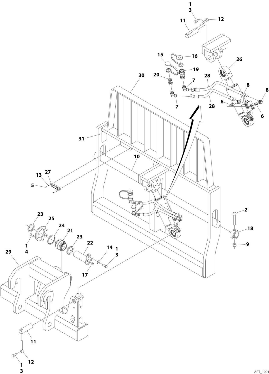
FIGURE 3-22. CARRIAGE ASSEMBLY - 50IN SIDE TILT (SN 0160116805 to Present)
