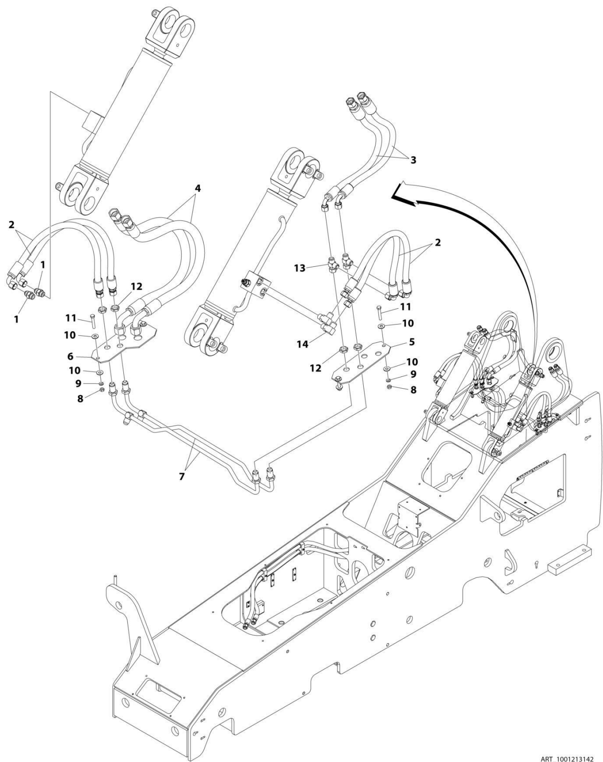
FIGURE 8-23. REAR BULKHEAD TO COMPENSATION CYLINDERS HYDRAULICS
