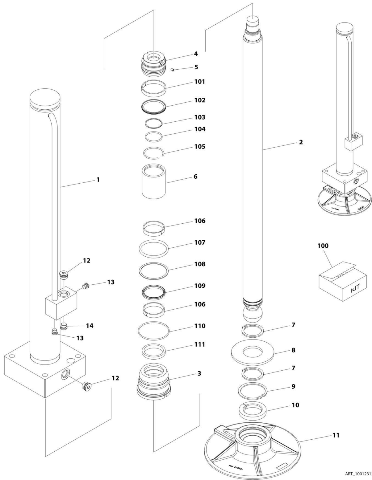
FIGURE 6-4. LEVELING JACK CYLINDER ASSEMBLY
