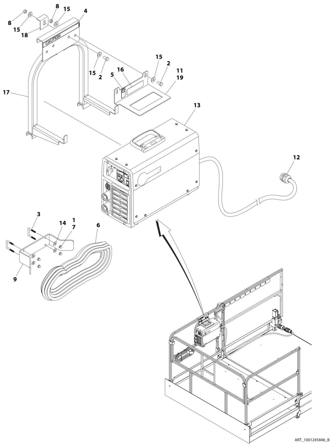
FIGURE 5-11. SKYWELDER INSTALLATION (OPTIONAL) (CE & UK CA SPECS)
