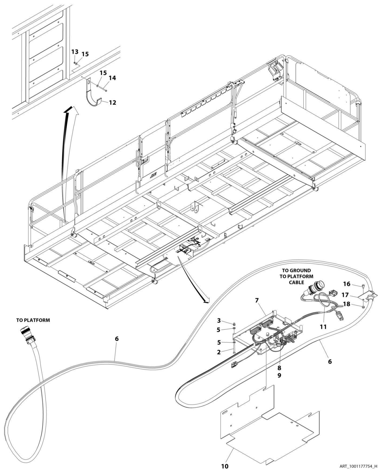
FIGURE 5-8. PLATFORM MODULE INSTALLATION
