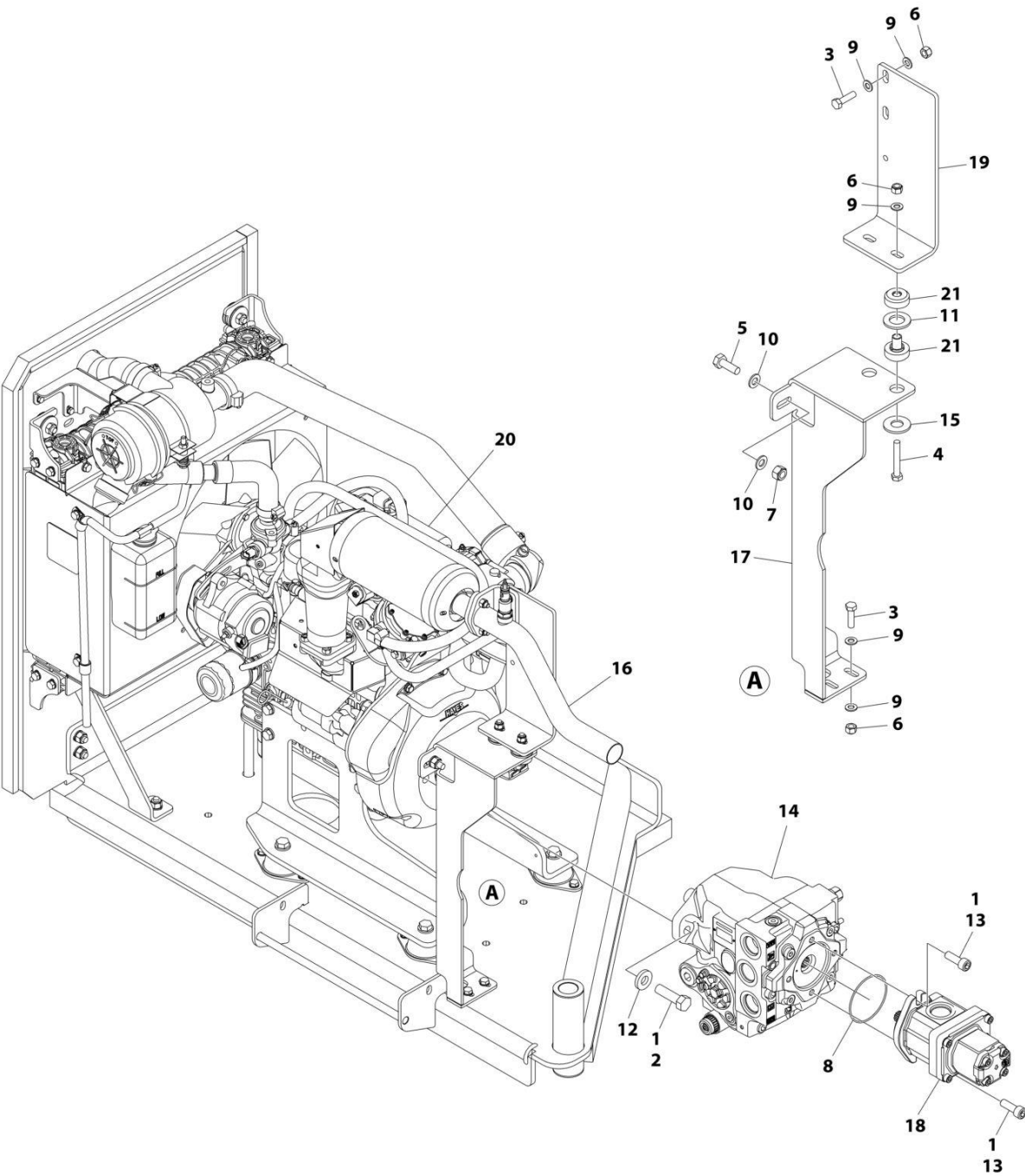
FIGURE 3-14. ENGINE AND PUMP SUB-ASSEMBLY - KUBOTA GASOLINE WITH GENERATOR
