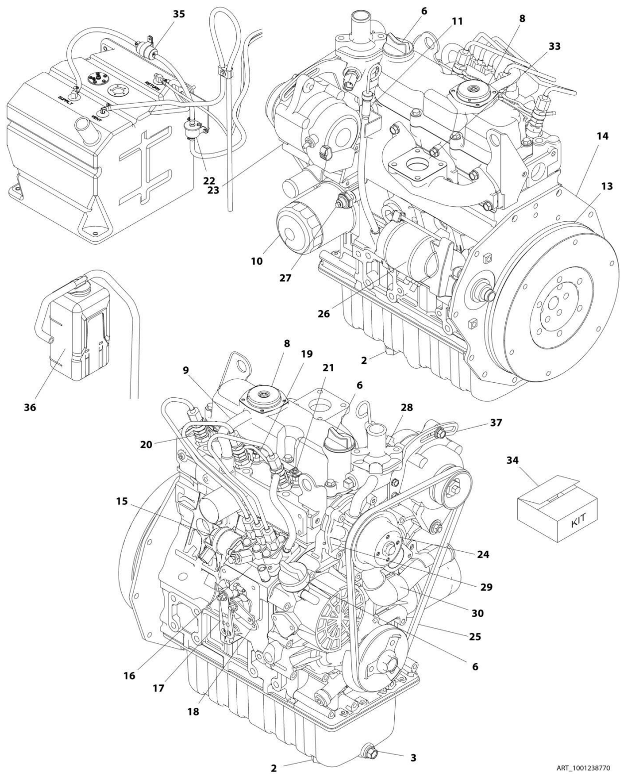
FIGURE 3-9. ENGINE COMPONENTS - KUBOTA DIESEL T4F
