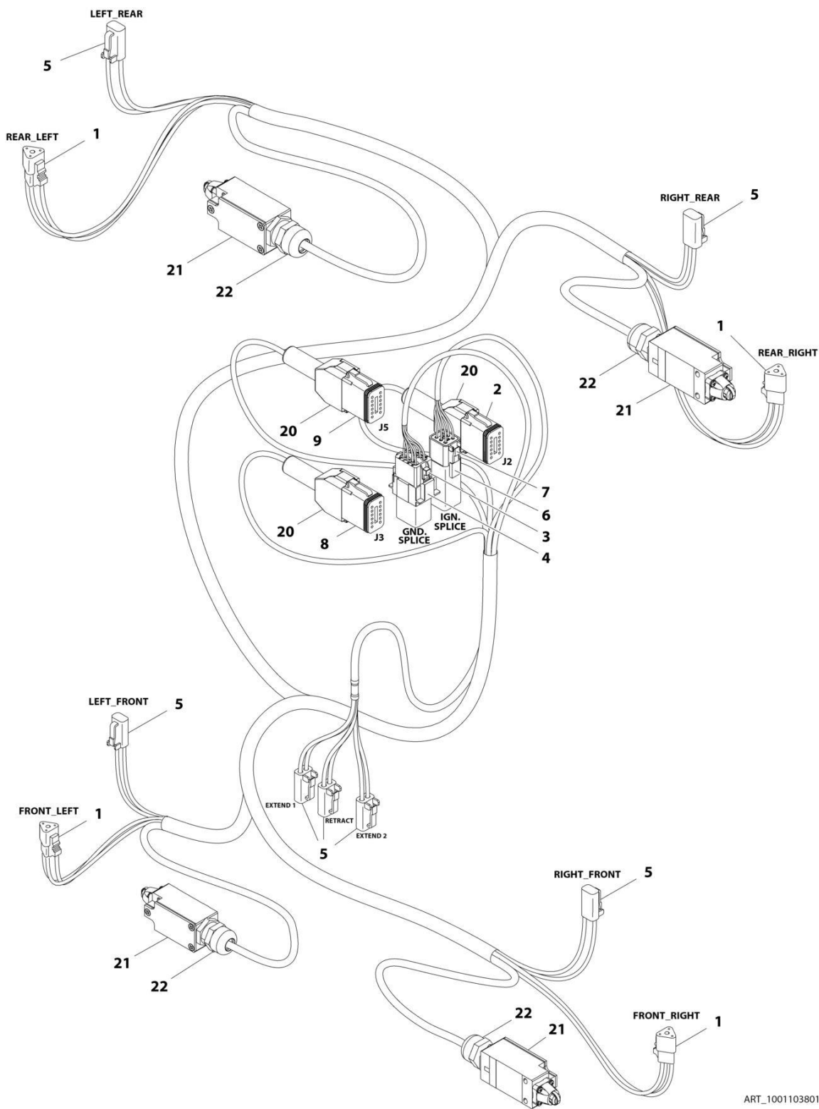
FIGURE 8-29. LEVELING JACK HARNESS
