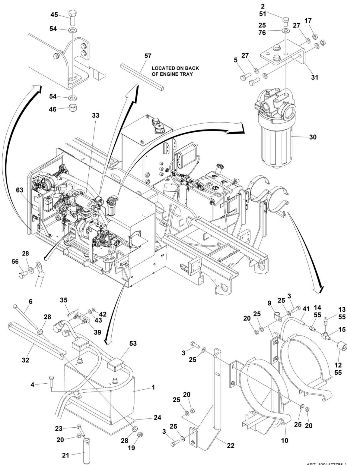
FIGURE 3-10. ENGINE INSTALLATION - KUBOTA GASOLINE
