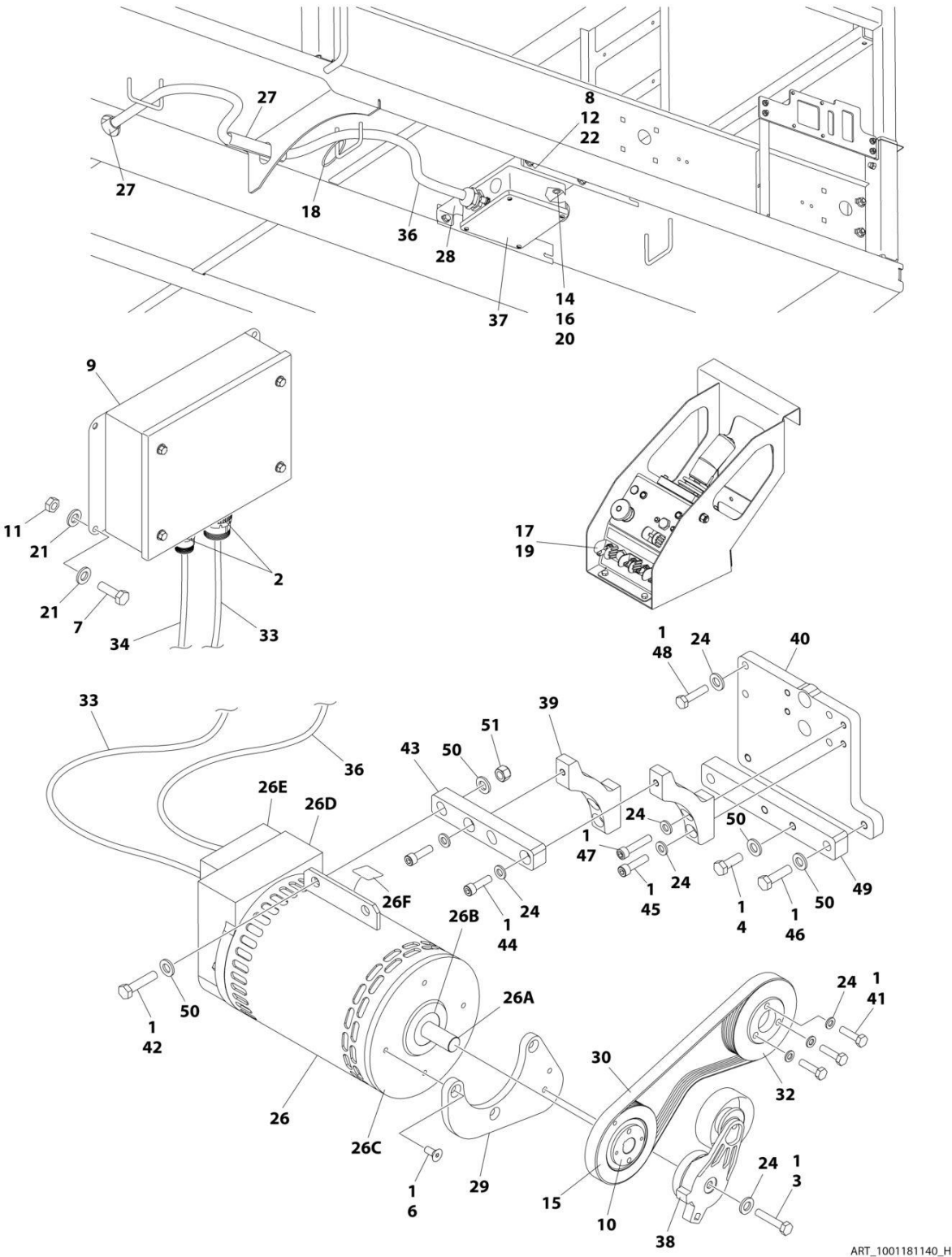
FIGURE 3-26. GENERATOR INSTALLATION - 7500W (KUBOTA DIESEL STAGE III)
