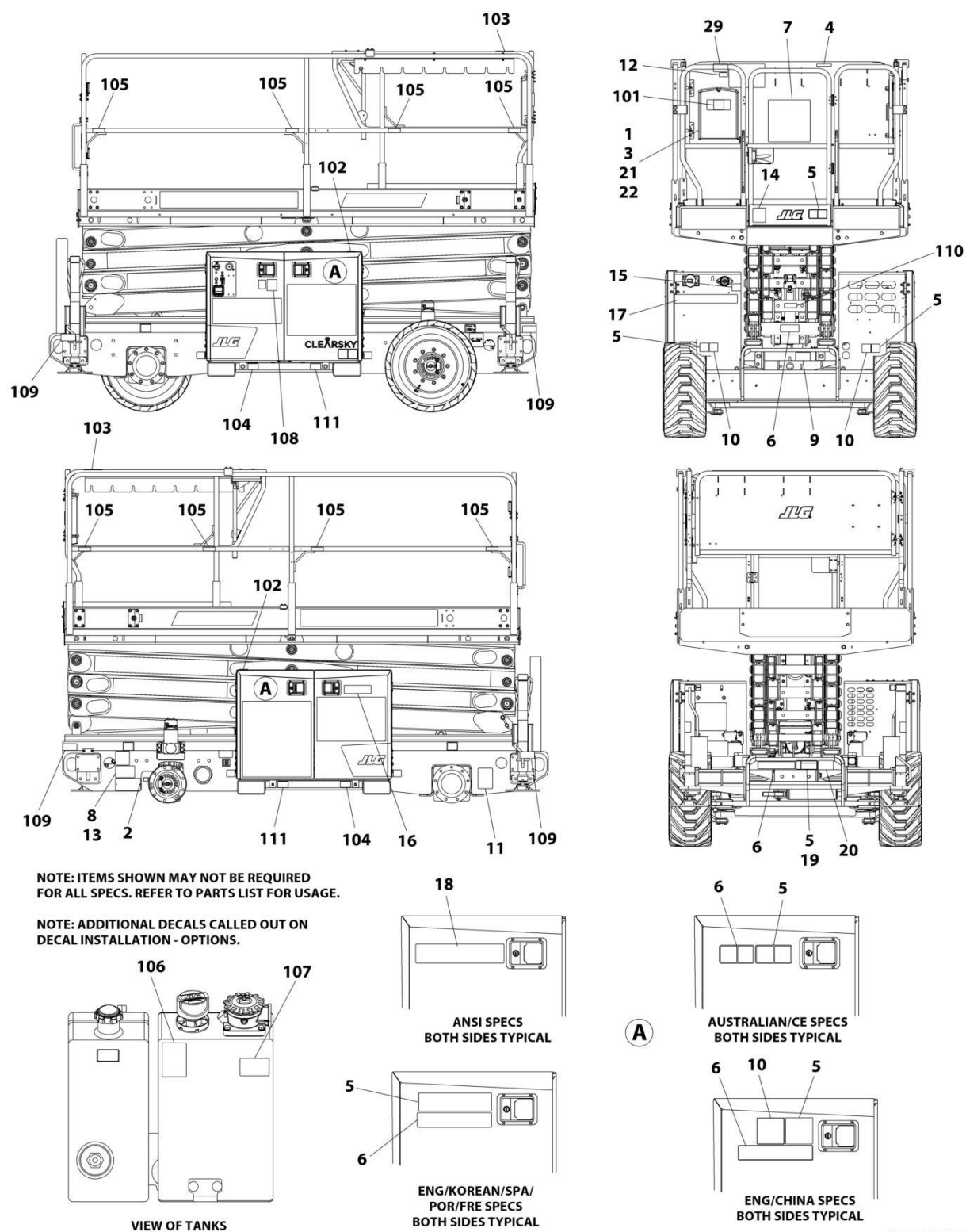
FIGURE 9-3. RT4069 DECAL INSTALLATION - BRAZIL SPECS (SPANISH/PORTUGUESE LANGUAGES)
