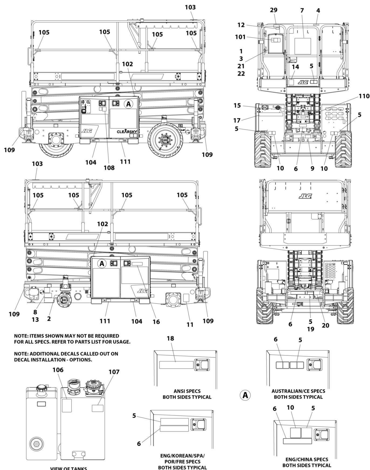
FIGURE 9-7. RT4069 DECAL INSTALLATION - LATIN AMERICAN SPECS (ENGLISH/KSPANISH LANGUAGES)
