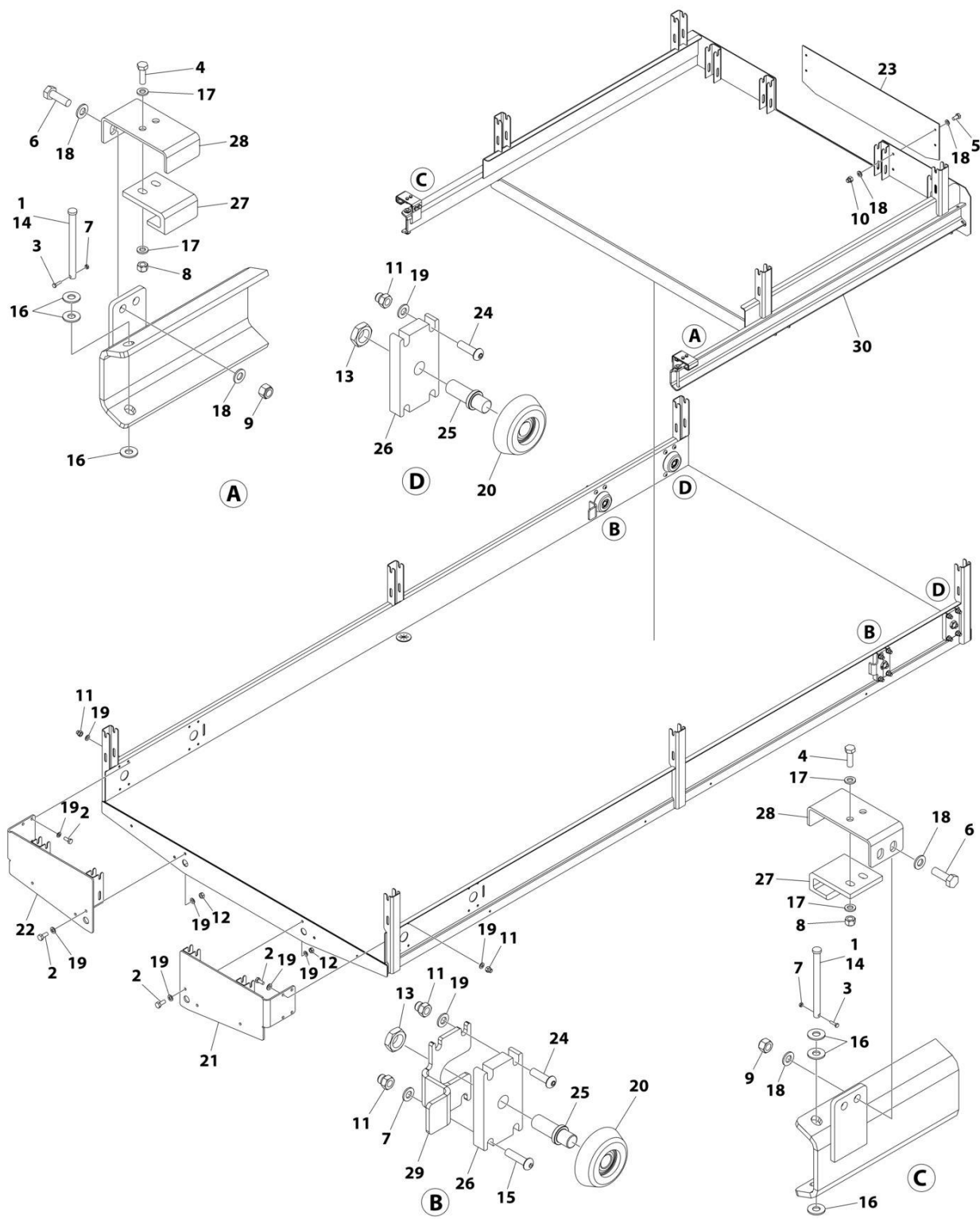
FIGURE 5-3. PLATFORM EXTENSION INSTALLATION (SINGLE) (SN M200067004 to Present, SN M200066376 to Present, Prior to SN M200087444, Prior to SN M200087471, Excluding M200067504)
