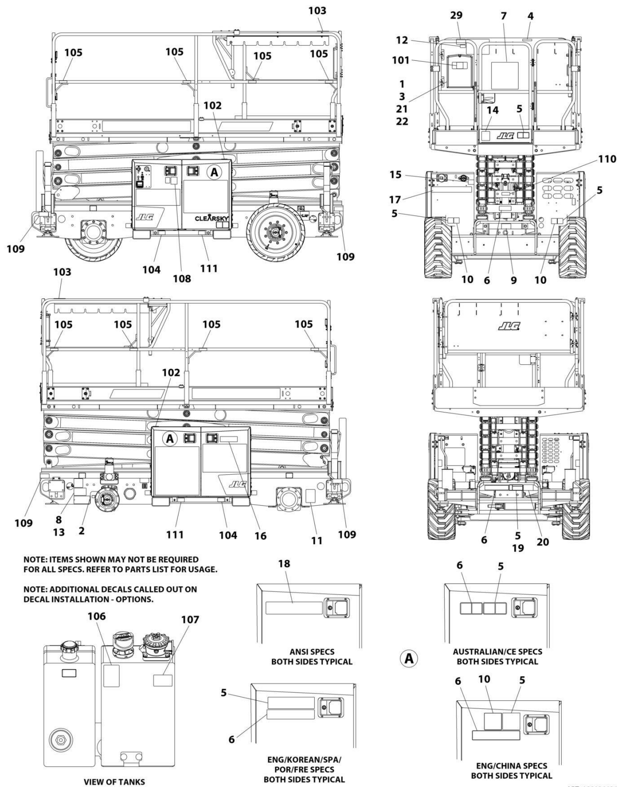
FIGURE 9-12. RT4769 DECAL INSTALLATION - CSA SPECS (ENGLISH/FRENCH LANGUAGES)
