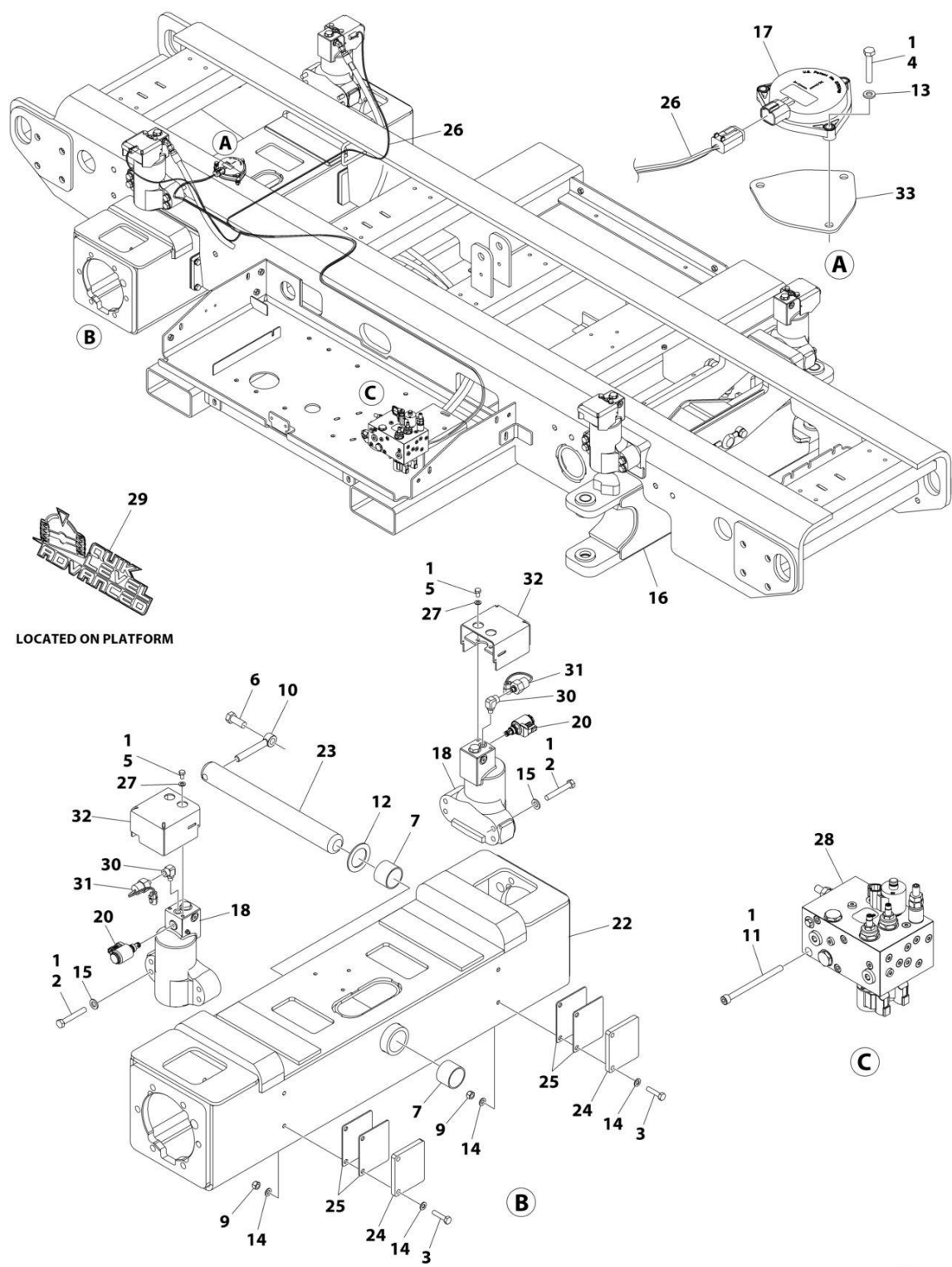
FIGURE 1-3. AXLE INSTALLATION - DUAL OSCILLATING
