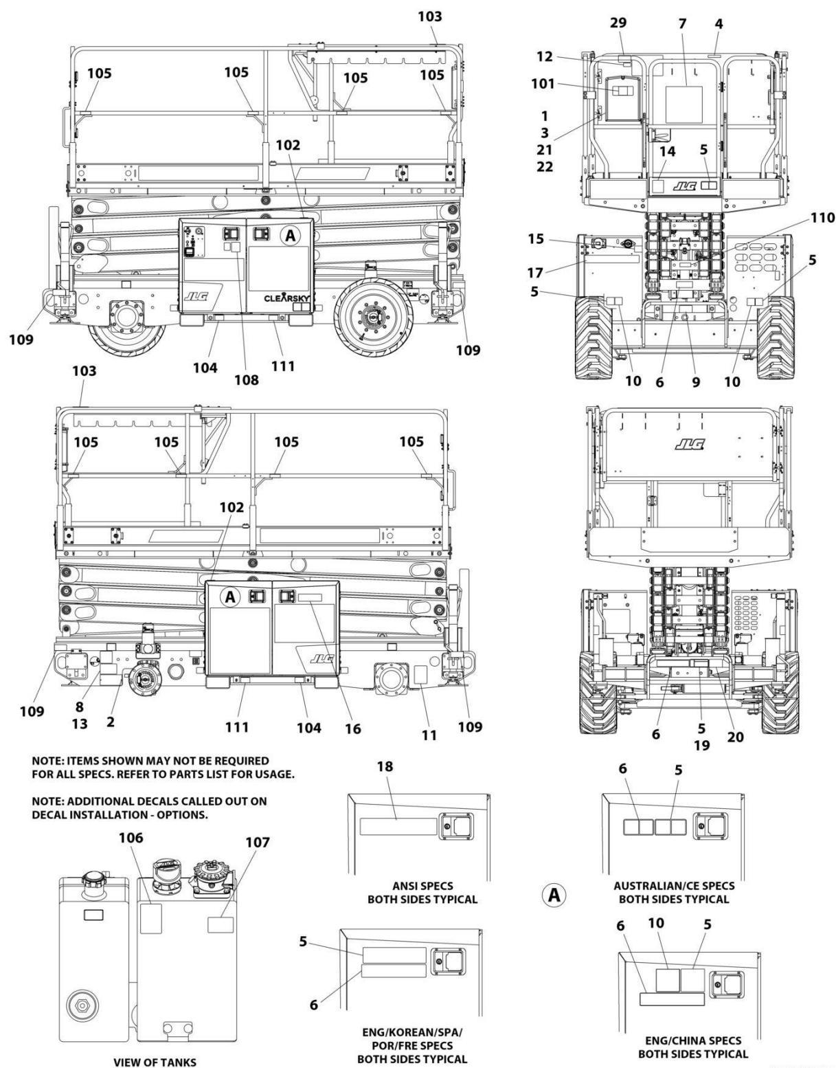
FIGURE 9-9. RT4769 DECAL INSTALLATION - AUSTRALIAN,CE & UK CA SPECS (ENGLISH LANGUAGE)
