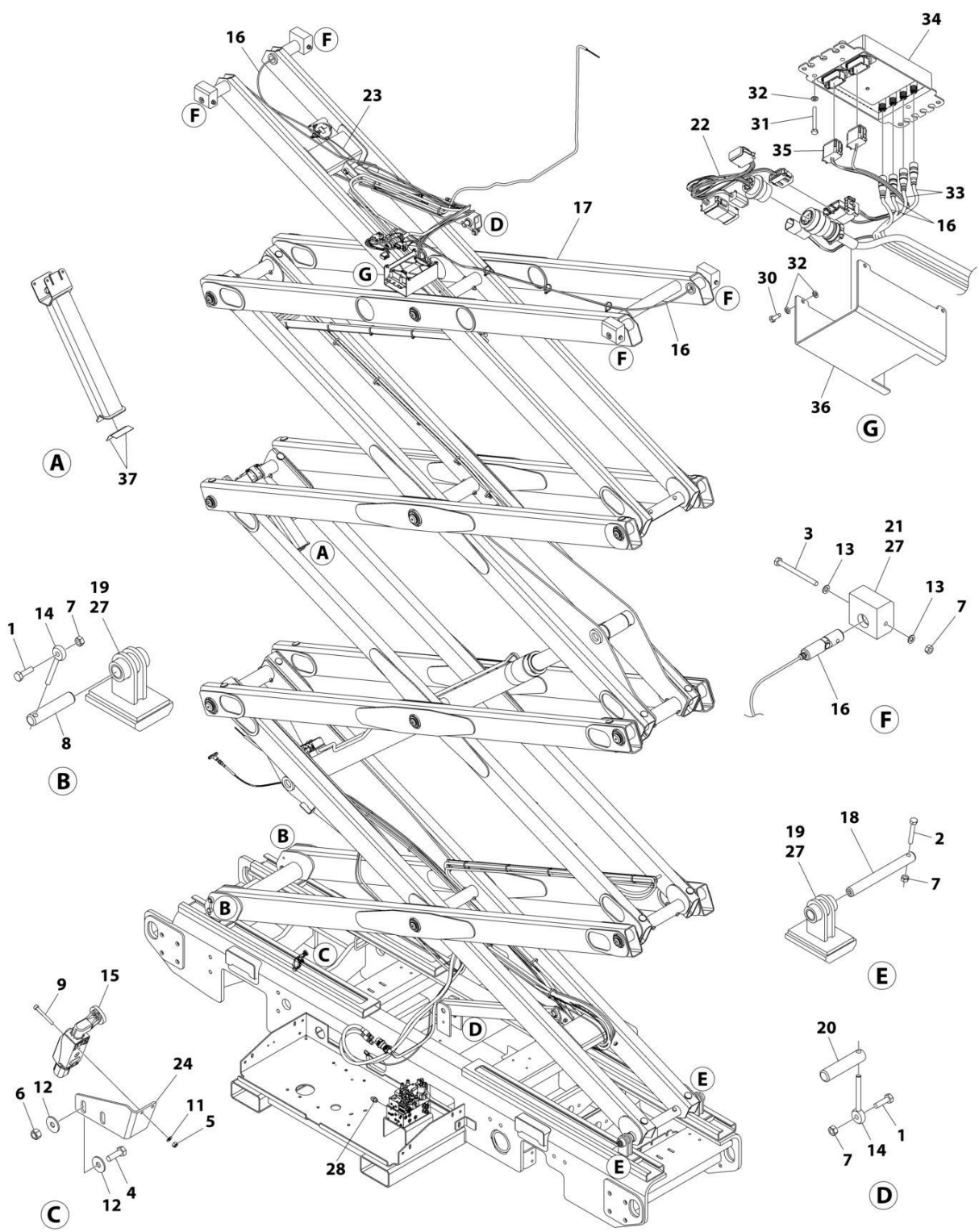
FIGURE 4-1. RT4069 ARMS INSTALLATION
