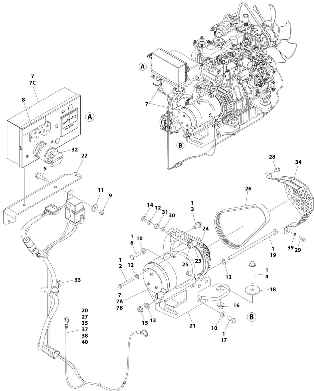
FIGURE 3-25. GENERATOR INSTALLATION - 2500W/60HZ (DIESEL MACHINES) (SN M200076032 to Present)
