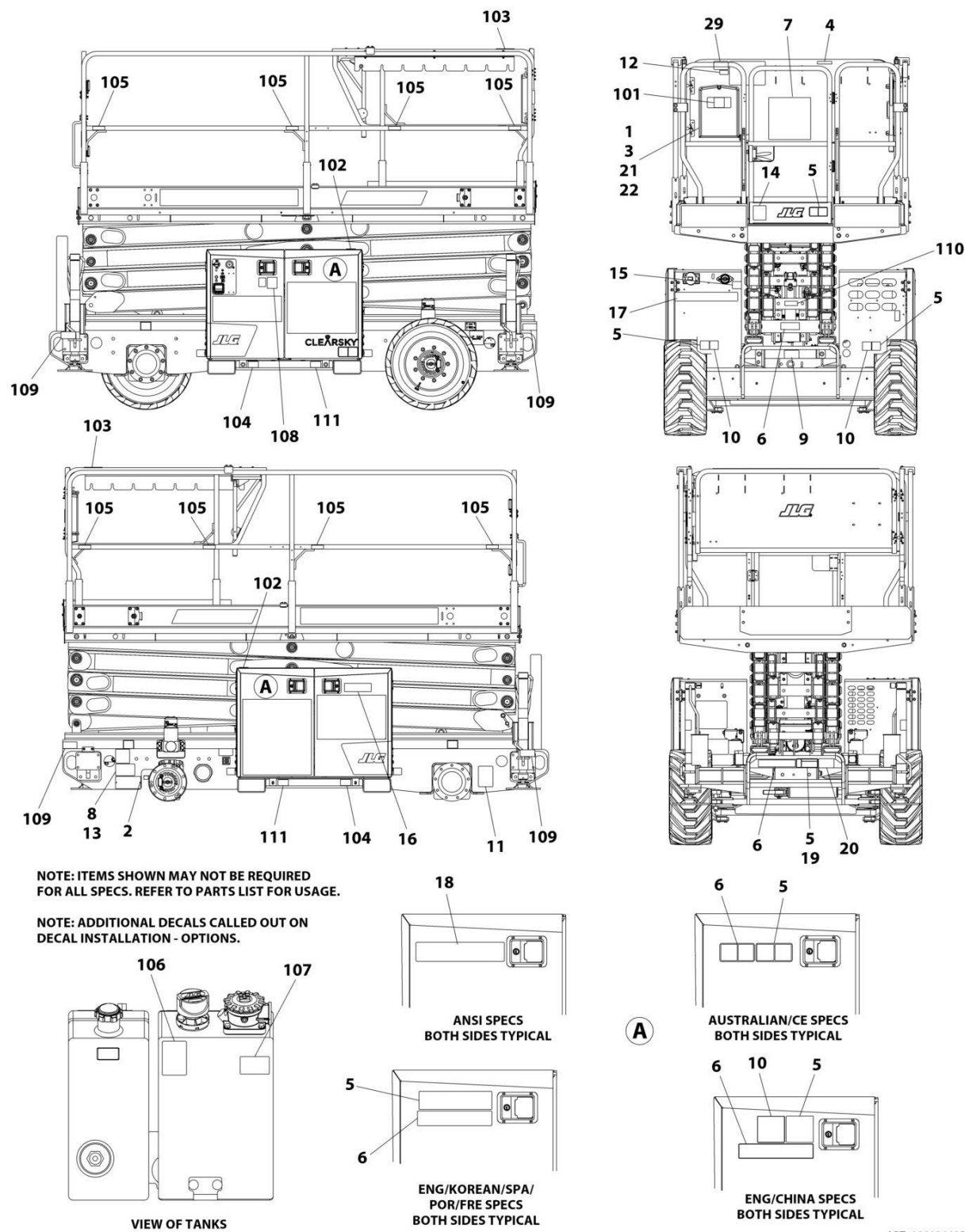
FIGURE 9-8. RT4769 DECAL INSTALLATION - ANSI SPECS (ENGLISH LANGUAGE)
