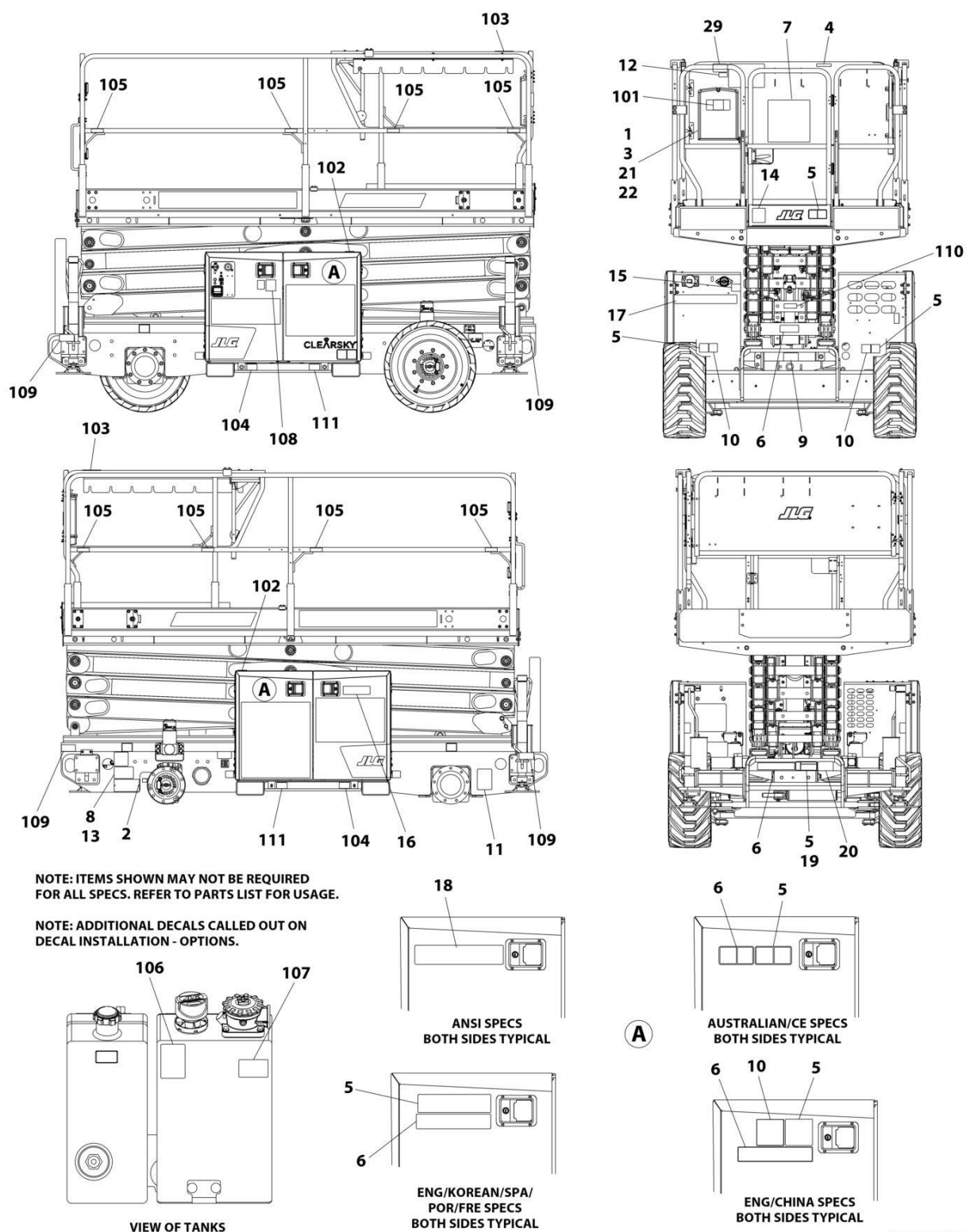
FIGURE 9-11. RT4769 DECAL INSTALLATION - CHINA SPECS (ENGLISH/CHINESE LANGUAGES)
