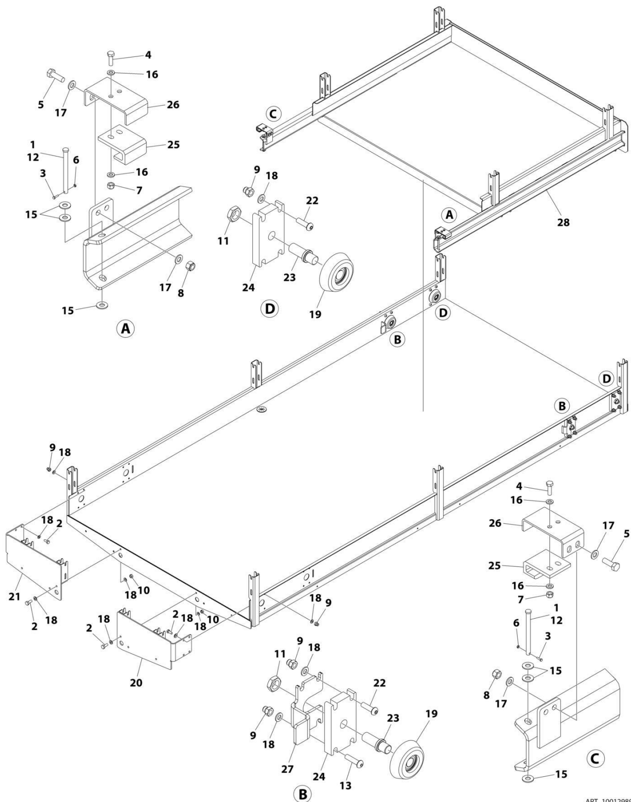
FIGURE 5-4. PLATFORM EXTENSION INSTALLATION (SINGLE) (SN M200087470 to Present, SN M200087545 to Present)
