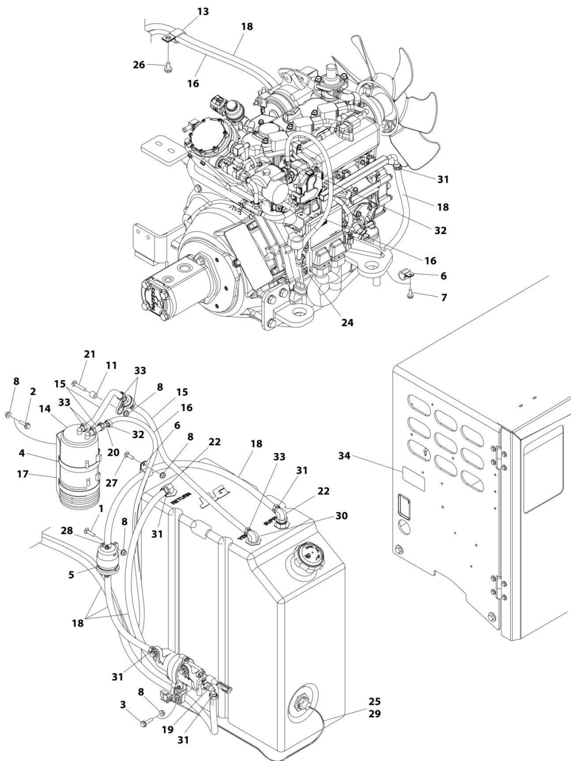
FIGURE 3-17. ENGINE FUEL LINES INSTALLATION - DUAL FUEL (Prior to SN M200084784, Prior to SN M200084488)
