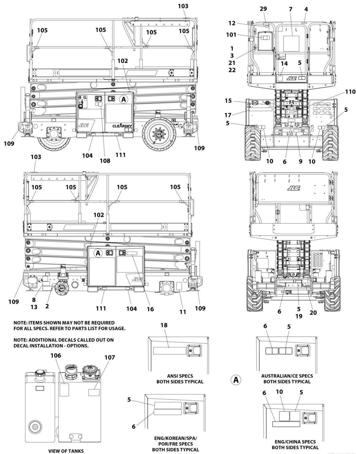
FIGURE 9-6. RT4069 DECAL INSTALLATION - KOREAN SPECS (ENGLISH/KOREAN LANGUAGES)
