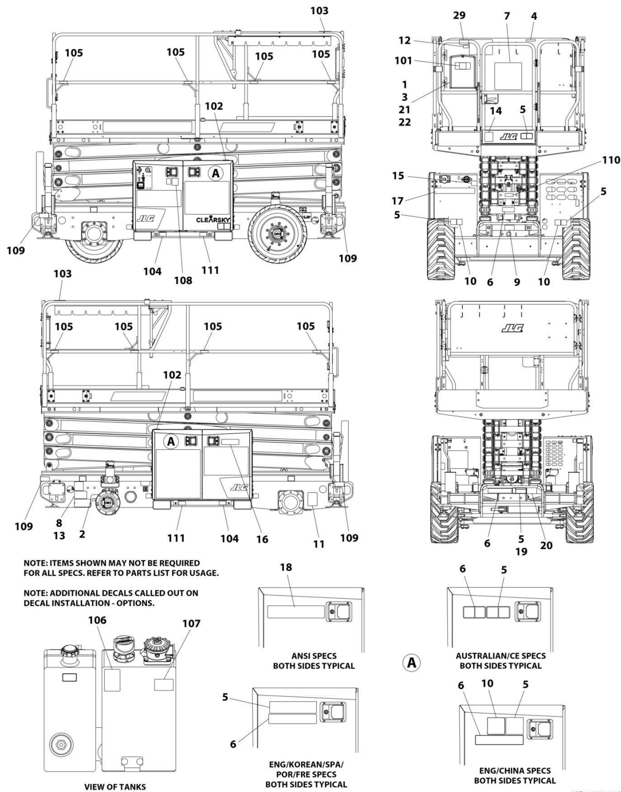
FIGURE 9-13. RT4769 DECAL INSTALLATION - KOREAN SPECS (ENGLISH/KOREAN LANGUAGES)
