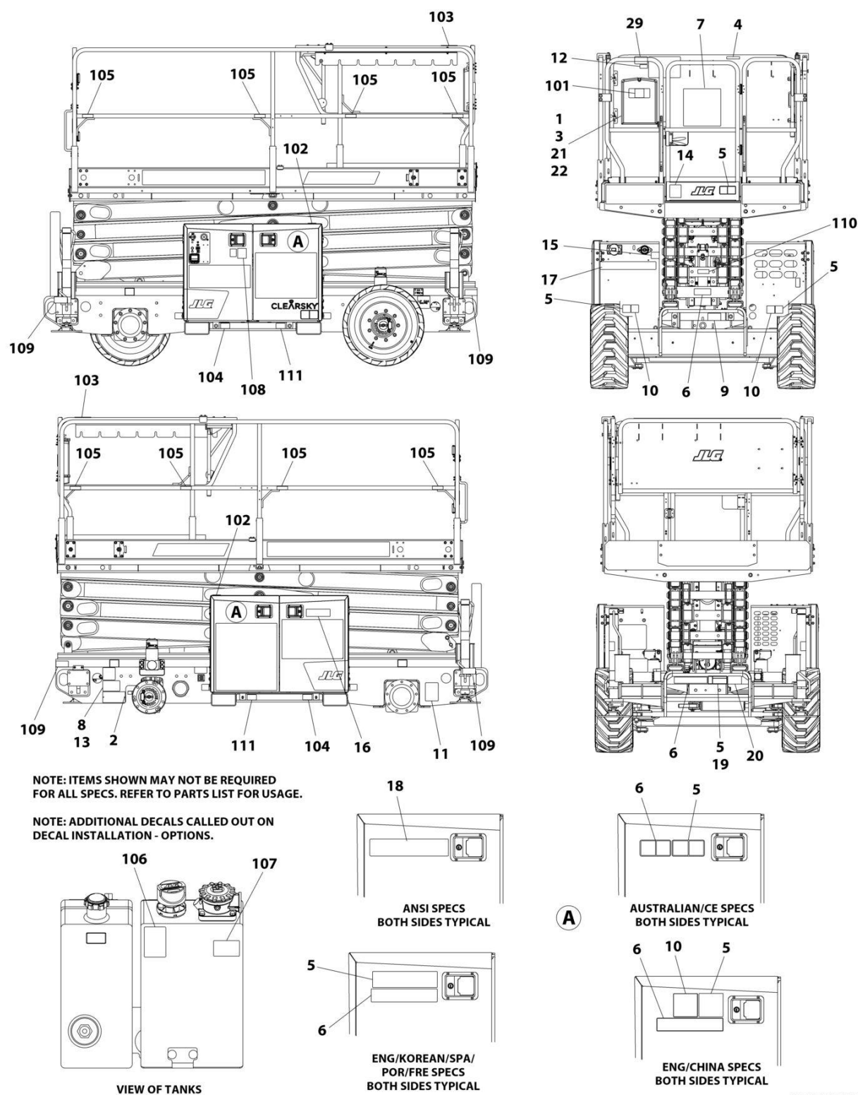
FIGURE 9-2. RT4069 DECAL INSTALLATION - AUSTRALIAN,CE & UK CA SPECS (ENGLISH LANGUAGE)
