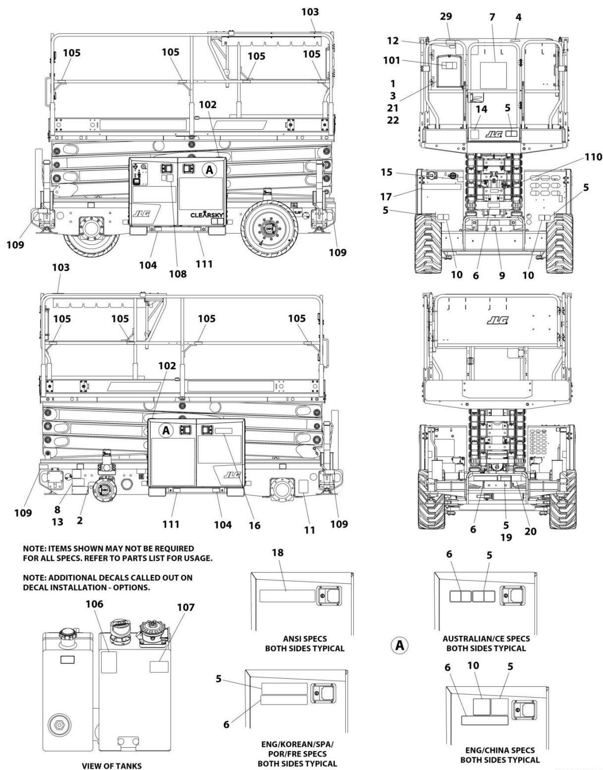
FIGURE 9-14. RT4769 DECAL INSTALLATION - LATIN AMERICAN SPECS (ENGLISH/KSPANISH LANGUAGES)
