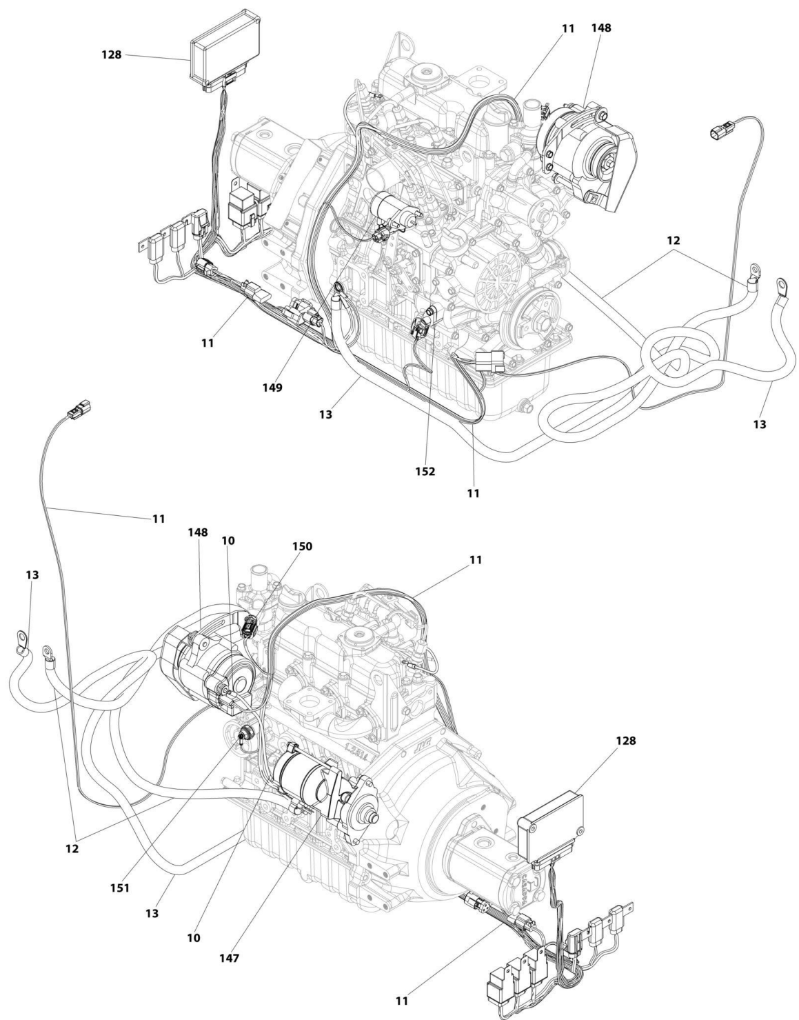
ART_RT3369-ELECTRICAL_ENGINE-KUBOTAT126D
