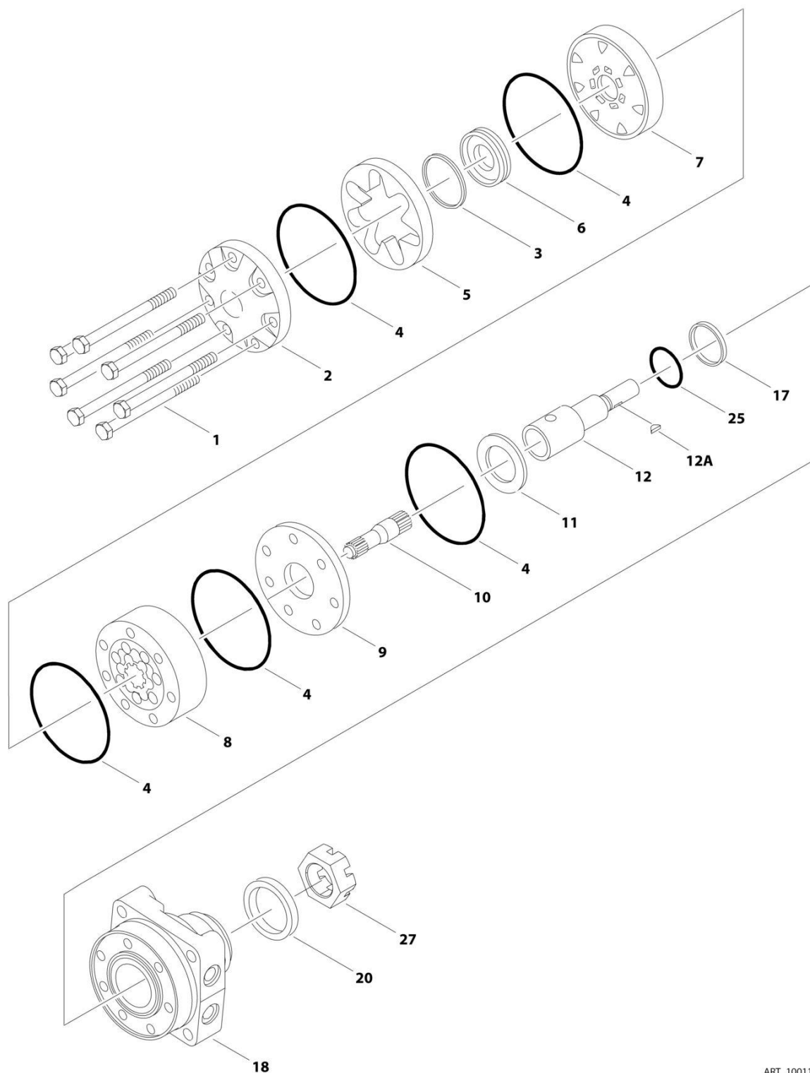
FIGURE 1-4. DRIVE MOTOR ASSEMBLY (Prior to SN B200079563, Prior to SN M200065756, Prior to SN 1200041017)
