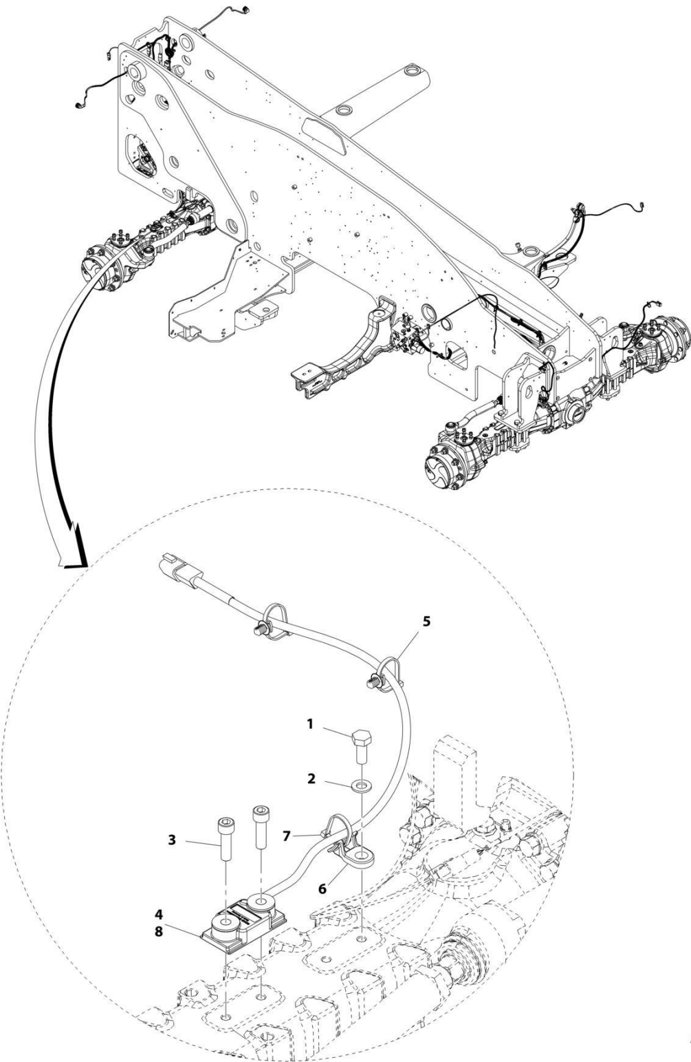
FIGURE 10-51. LSI SENSOR INSTALLATION
