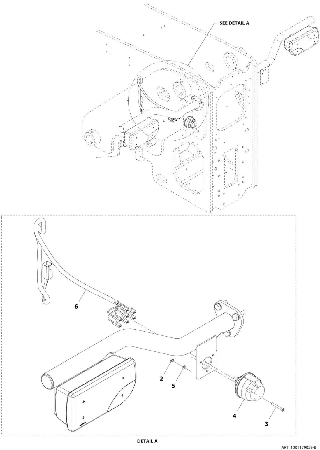
FIGURE 10-62. TRAILER ELECTRICS INSTALLATION
