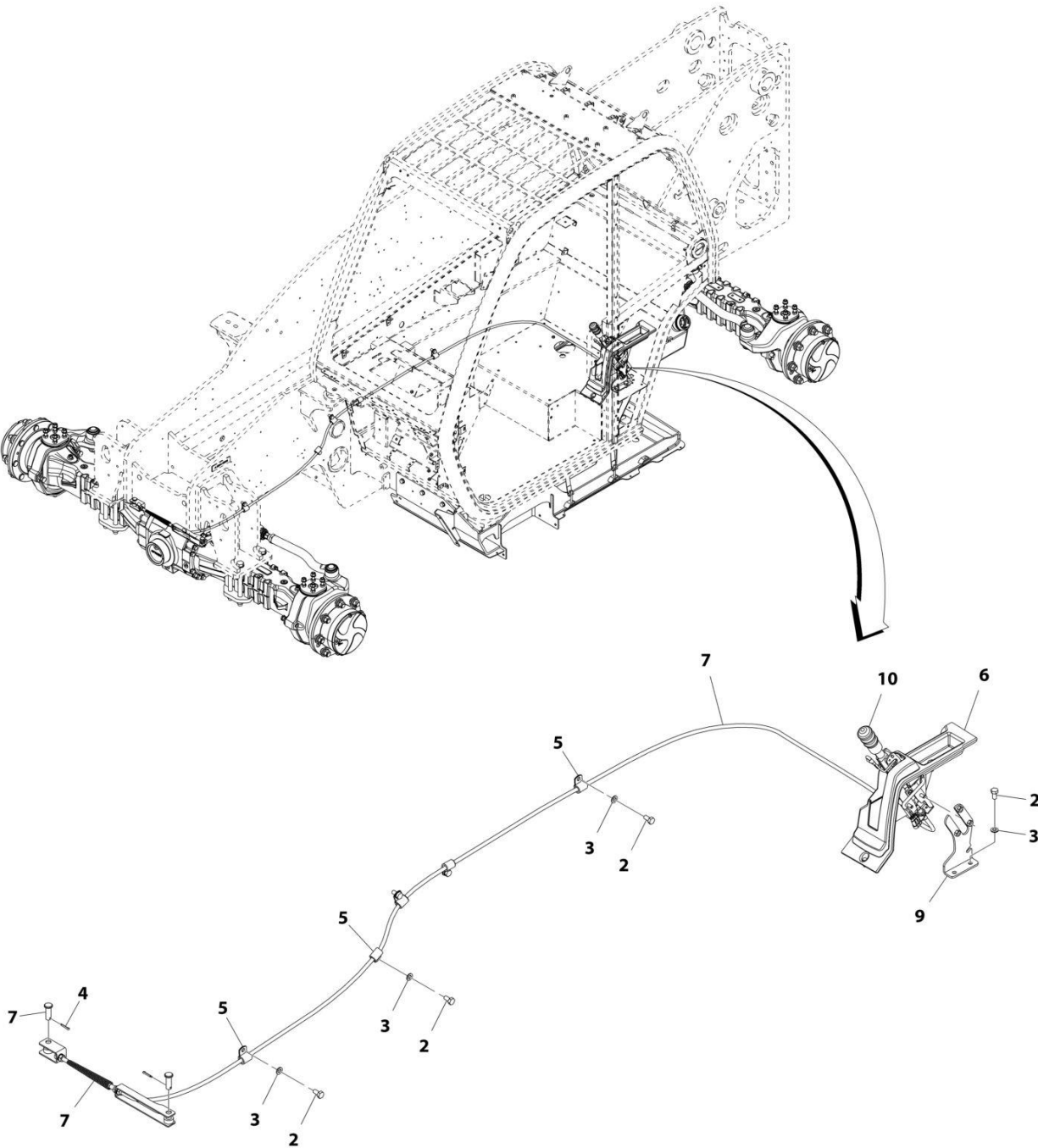
FIGURE 7-8. PARKING BRAKE INSTALLATION (CABLE - STANDARD)
