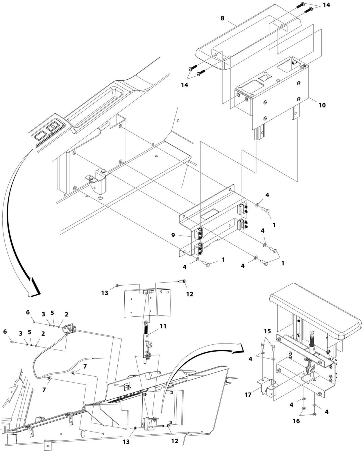
FIGURE 6-23. ADJUSTABLE ARMREST INSTALLTION (SN 0160112883 to Present)
