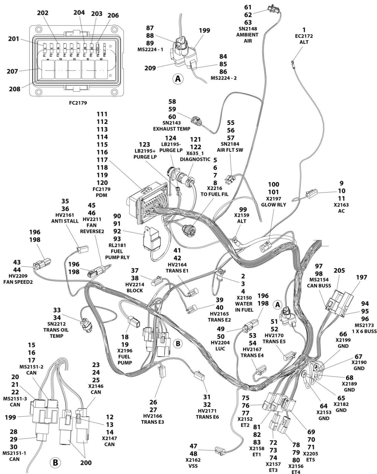
FIGURE 10-30. ENGINE HARNESS (ULS)
