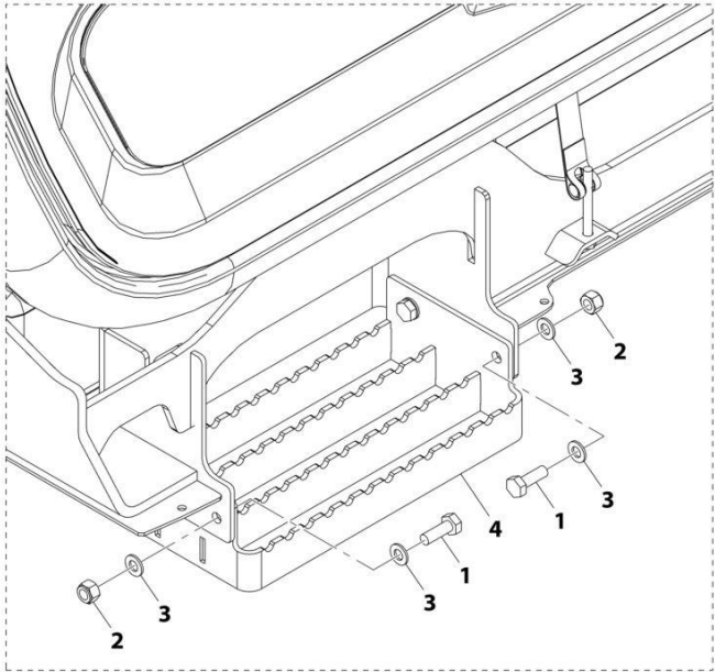
DETAIL A
