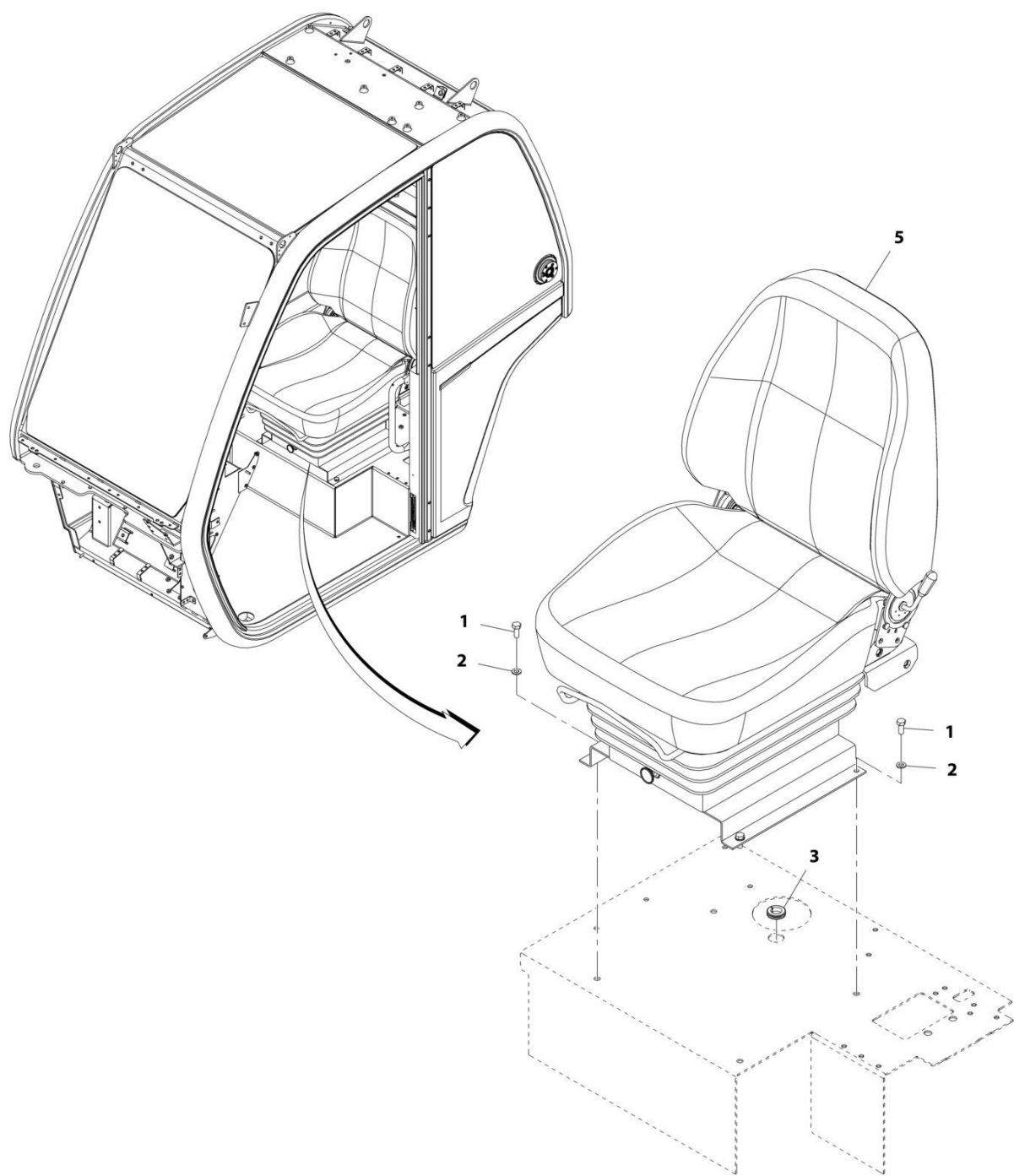
FIGURE 6-36. SEAT INSTALLATION (AIR SUSPENSION - STANDARD) (Prior to SN 0160112883)
