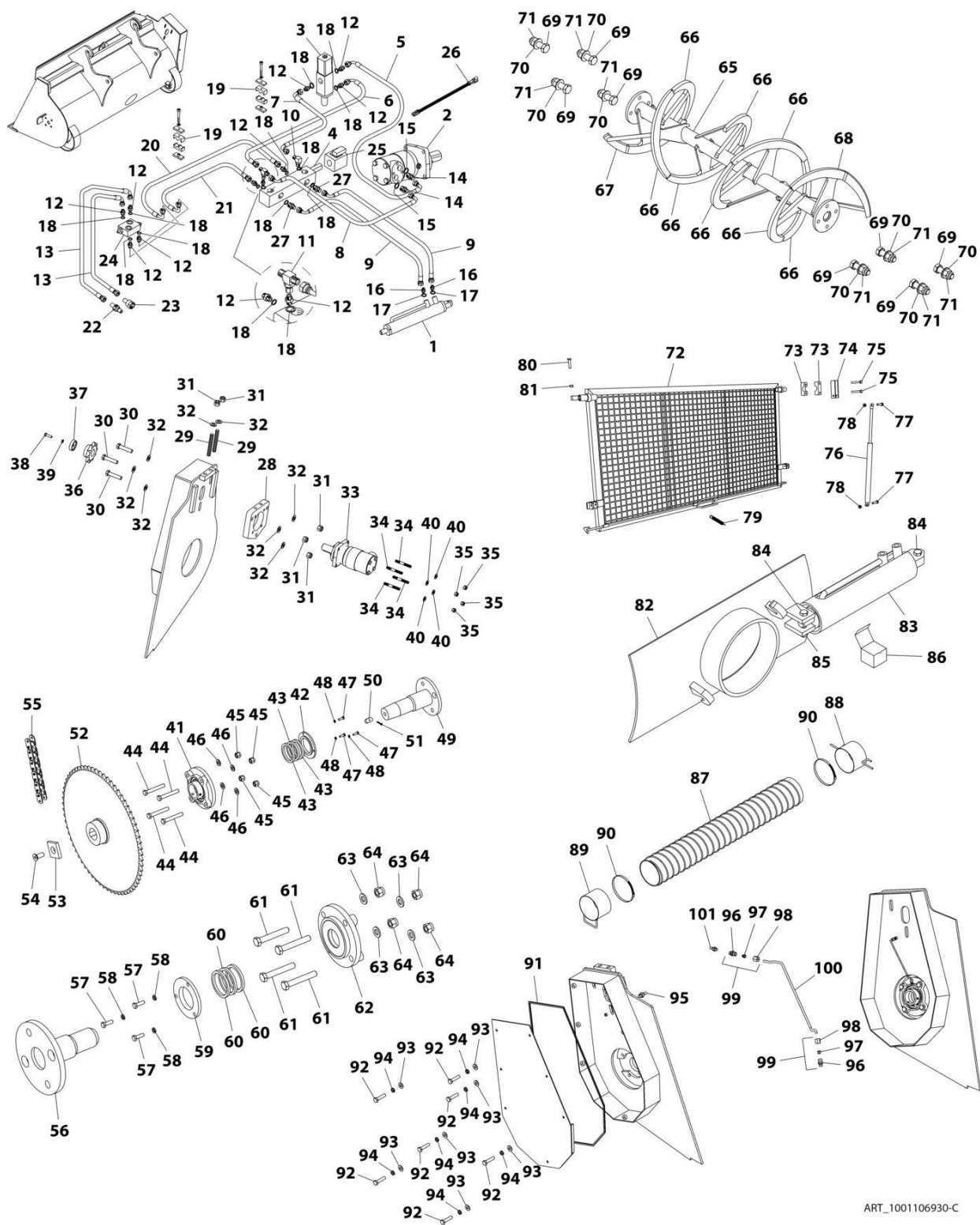
FIGURE 3-17. BUCKET (CONCRETE)
