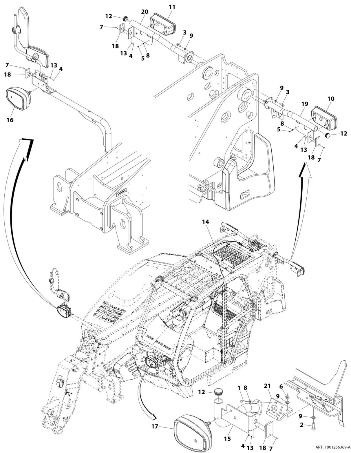
FIGURE 10-38. LIGHTS - DIP LIGHTS INSTALLATION (RH)
