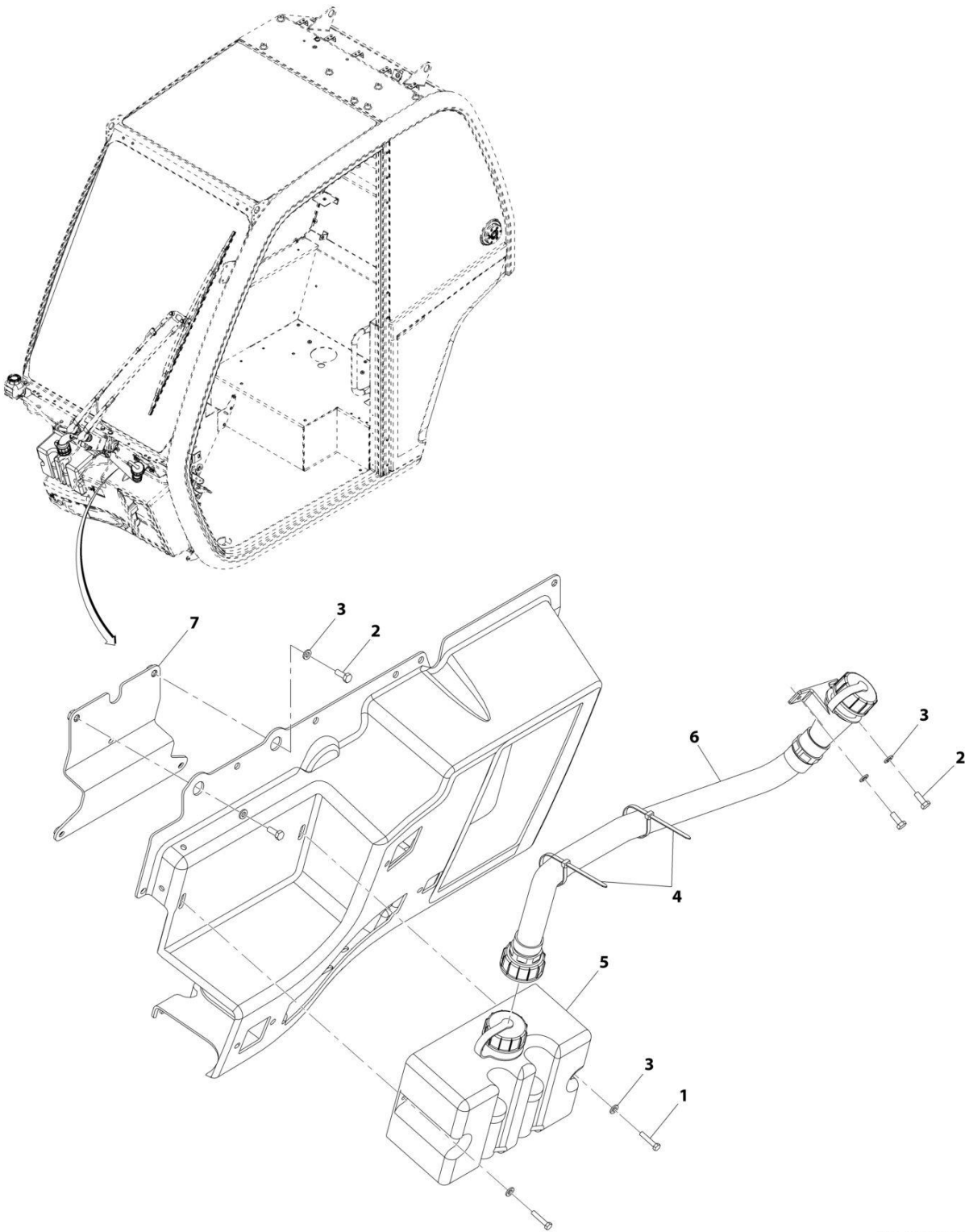
FIGURE 6-34. WASHER TANK INSTALLATION
