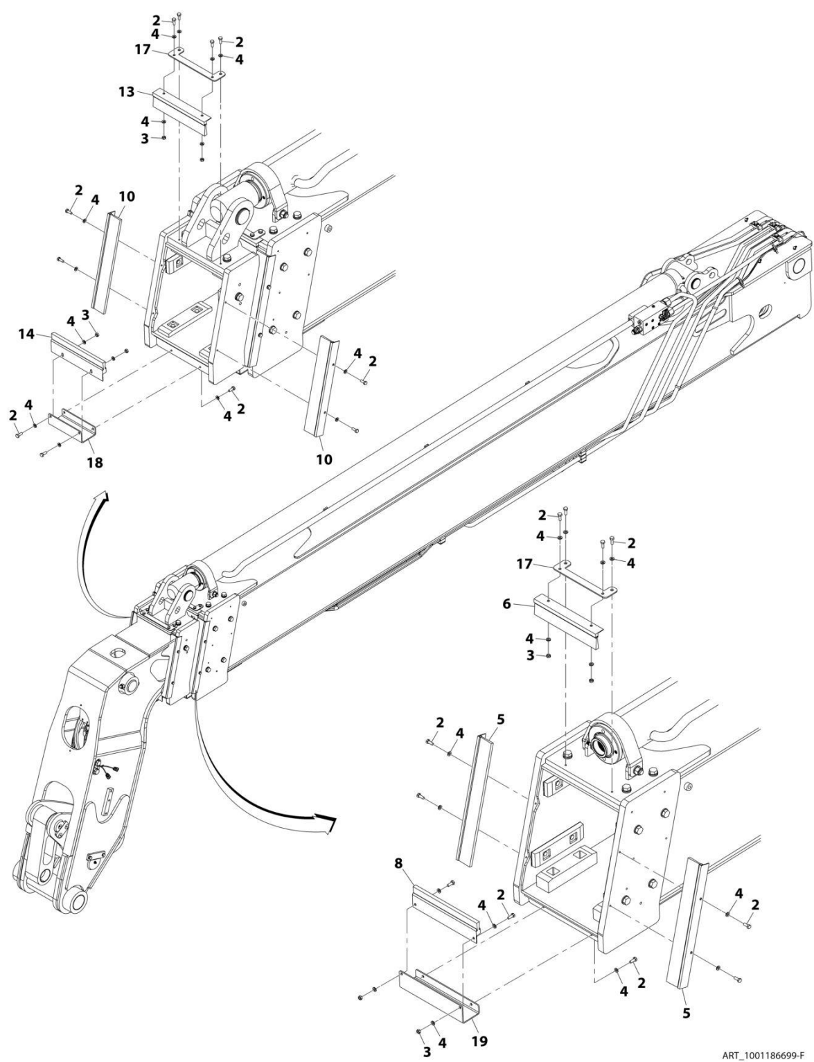
FIGURE 2-14. BOOM BRUSHES INSTALLATION
