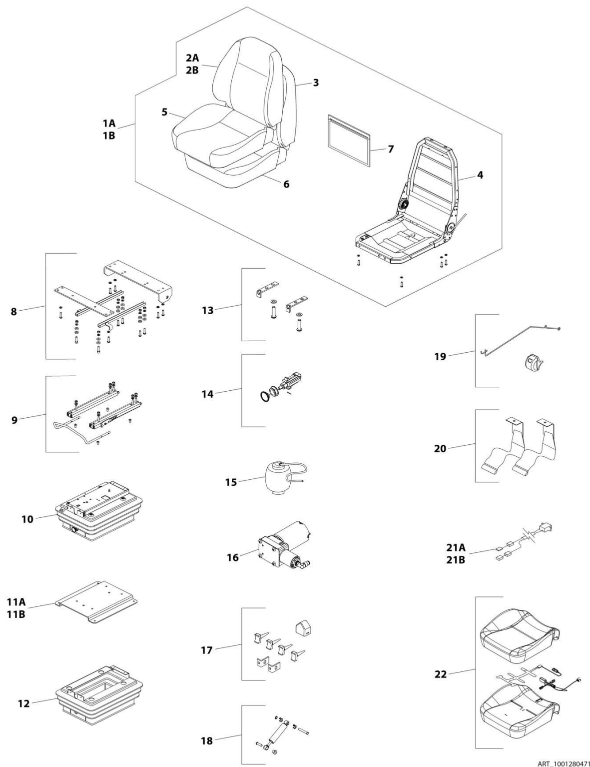
FIGURE 6-39. SEAT ASSEMBLY (AIR SUSPENSION - STANDARD) (SN 0160112883 to Present)
