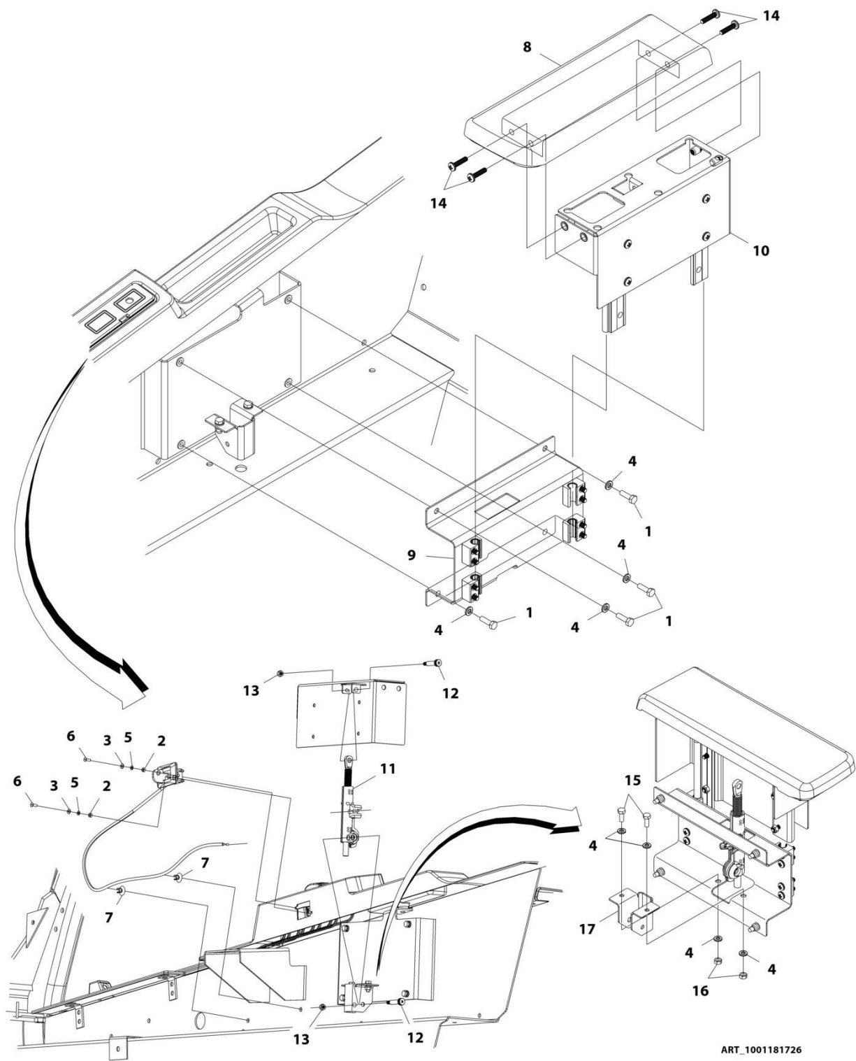
FIGURE 6-22. ADJUSTABLE ARMREST INSTALLTION (Prior to SN 0160112883)
