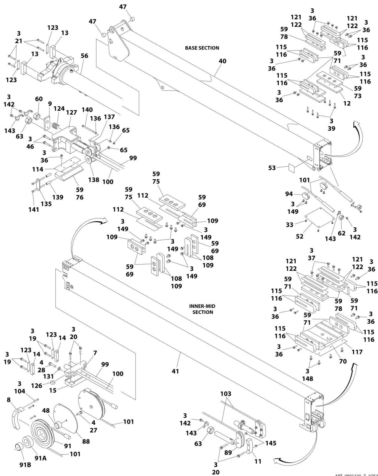
FIGURE 4-10. BOOM ASSEMBLY - WITHOUT COLD WEATHER PLUS PACKAGE (1200SJP) (SN 0300296108 to Present, SN B300016940 to Present, Including 030026105 and B300016704)
