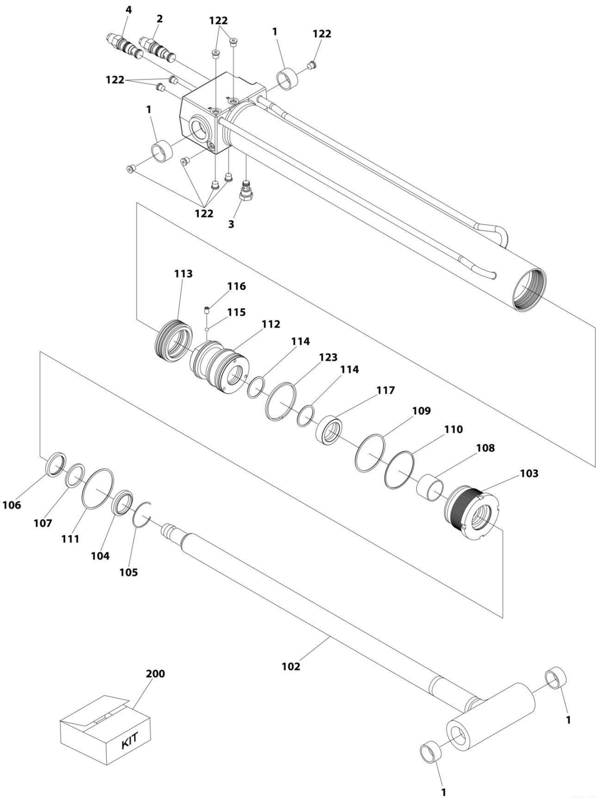
FIGURE 6-7. JIB CYLINDER ASSEMBLY - WITH OR WITHOUT COLD WEATHER PLUS PACKAGE
