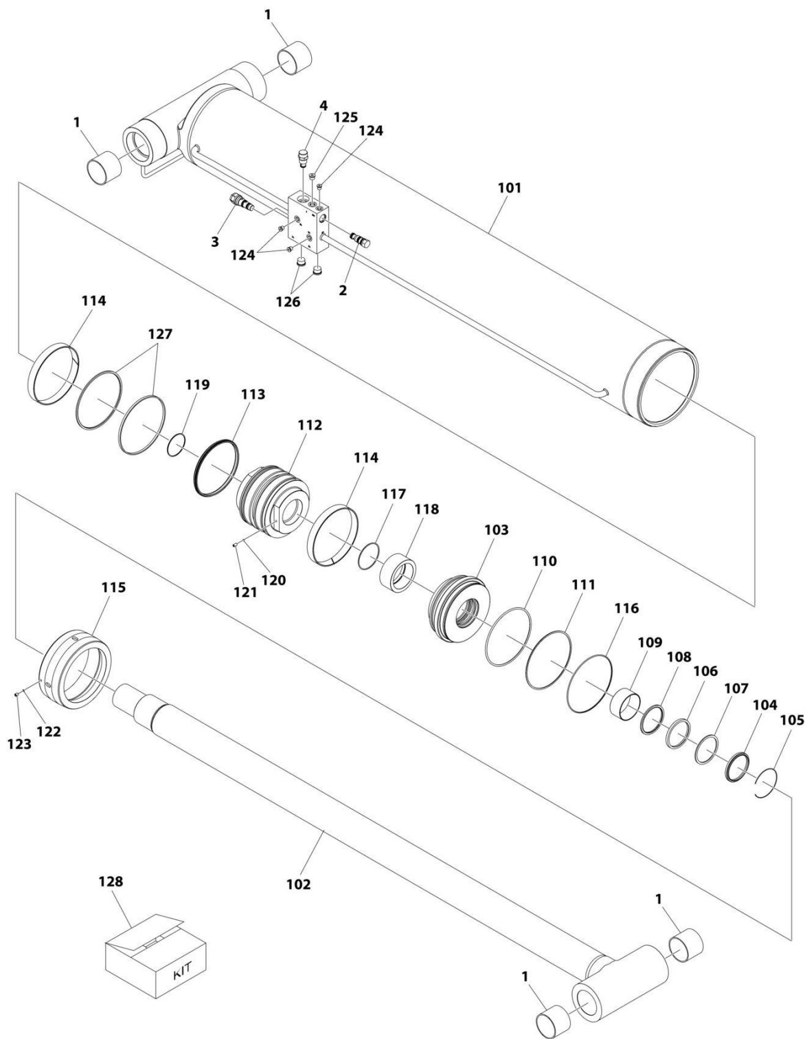
FIGURE 6-6. LIFT CYLINDER ASSEMBLY (Excluding B300016796, B300016807, B300016833 and B300016836)
