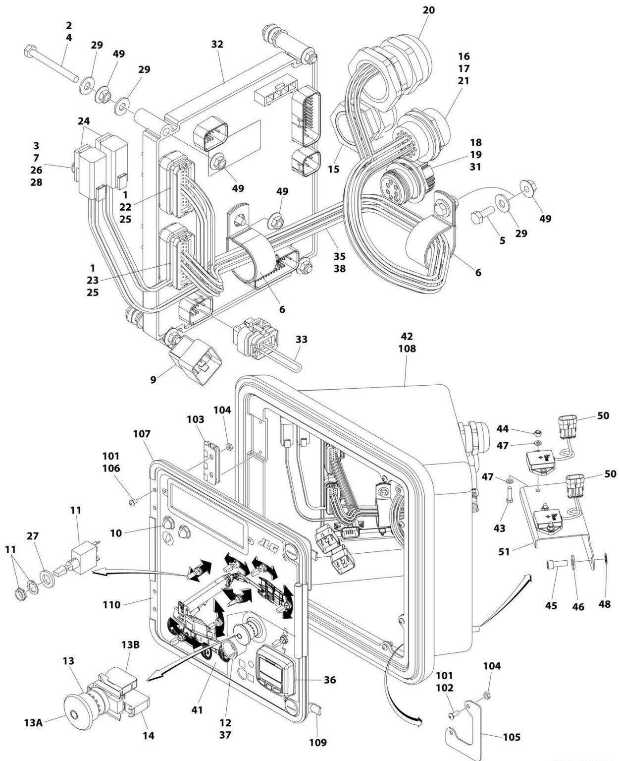
FIGURE 2-38. GROUND CONTROL BOX ASSEMBLY - DEUTZ TCD2.9L4 STAGE V ENGINES (Prior to SN 0300298064, Prior to SN B300017880, Excluding 0300287515, B300016940, B300017007 and B300017072)
