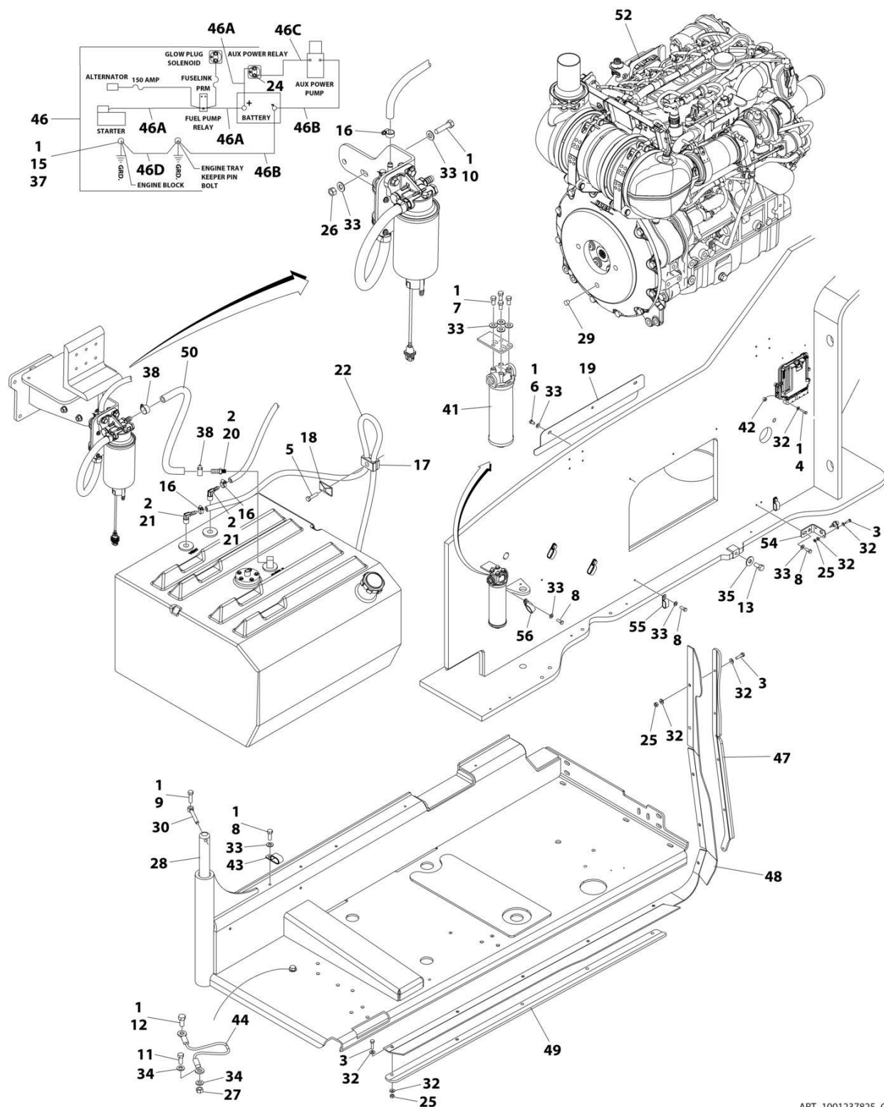
FIGURE 3-36. DEUTZ TCD2.9L4 (STAGE V) ENGINE INSTALLATION - WITH REXROTH PUMPS AND ABS HOODS (WITHOUT COLD WEATHER PLUS PACKAGE)
