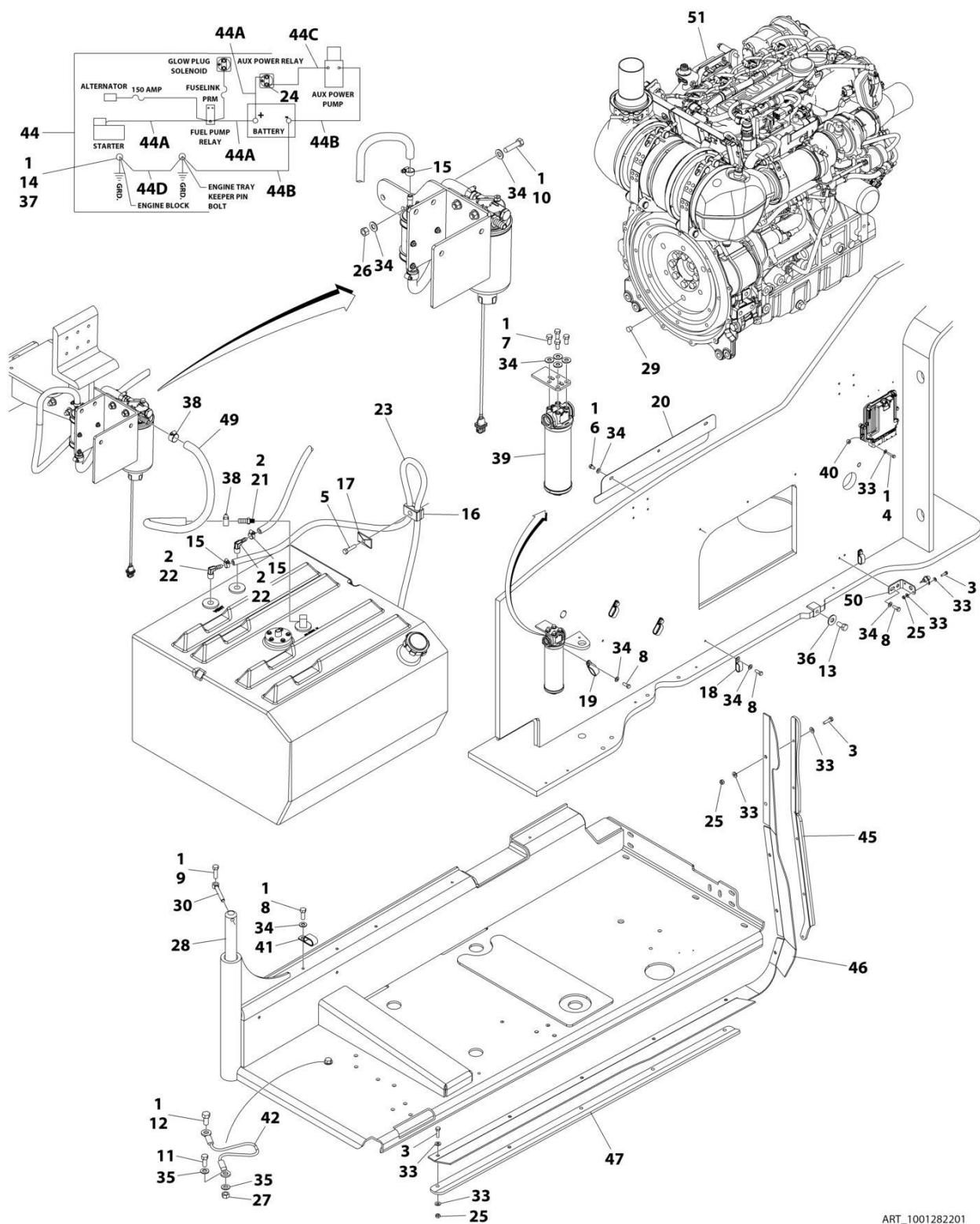
FIGURE 3-41. DEUTZ TCD2.9L4 (CHINA IV) ENGINE INSTALLATION - WITH SAUER PUMPS
