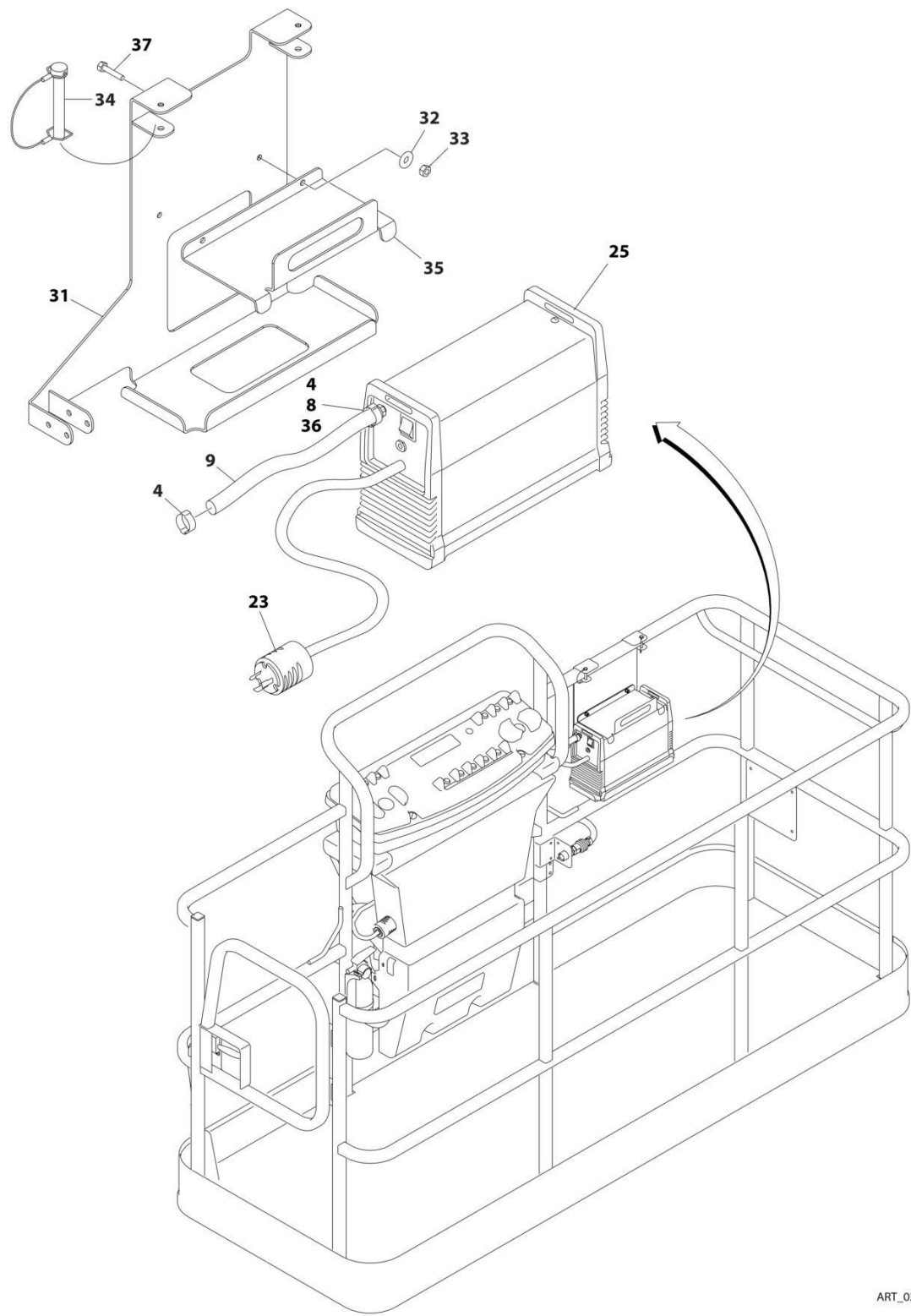
FIGURE 5-46. SKYWELDER/SKYCUTTER COMBO INSTALLATION (60HZ) (ANSI, ANSI EXPORT, CHINA, CSA AND JAPANESE SPECS)
