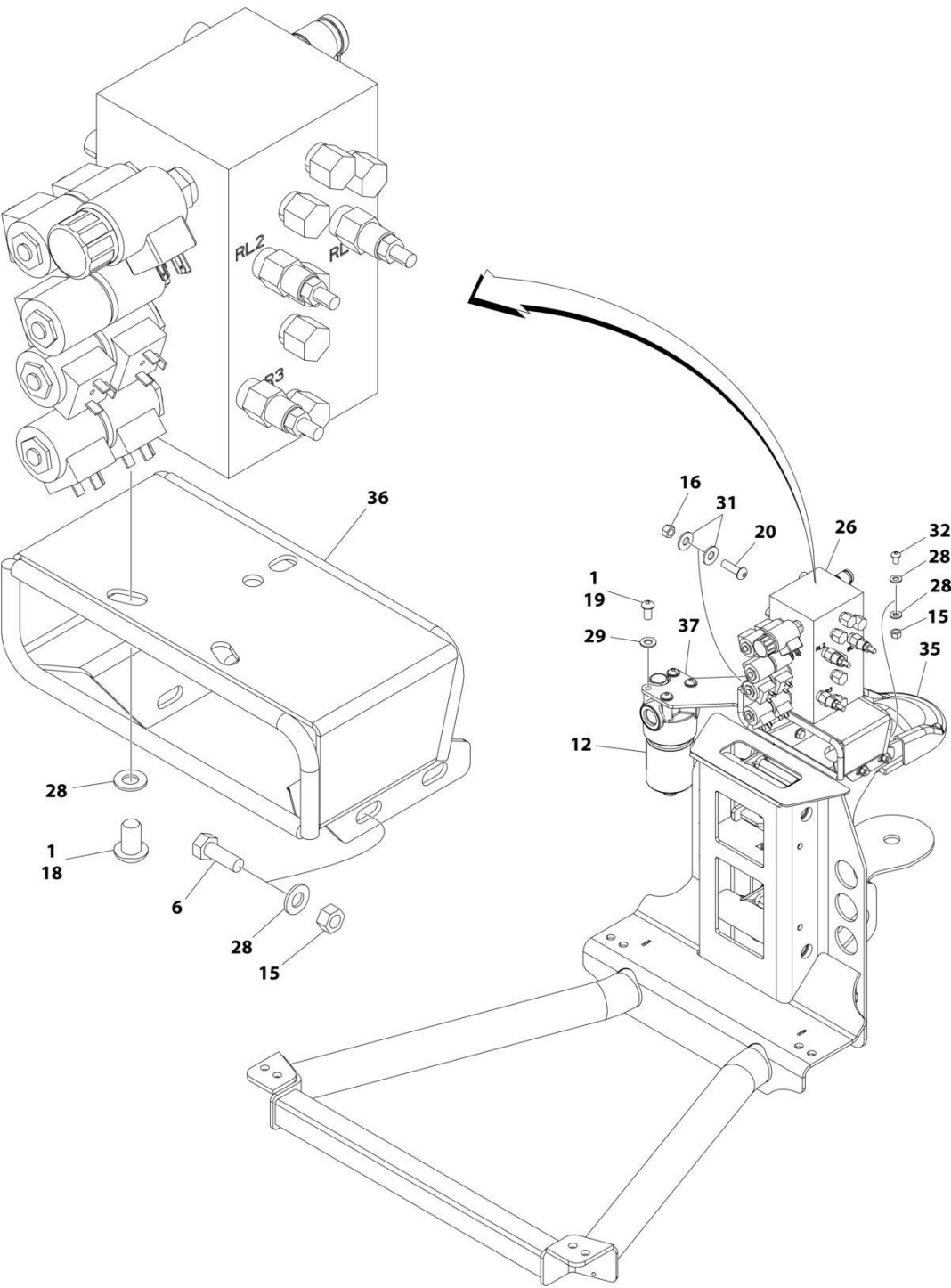
FIGURE 4-22. CONTROL VALVE INSTALLATION
