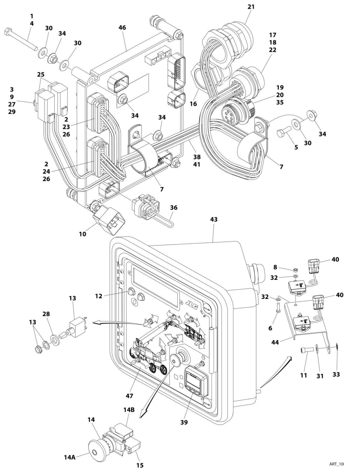
FIGURE 2-40. GROUND CONTROL BOX ASSEMBLY - DEUTZ TCD2.9L4 CHINA IV ENGINES (Prior to SN 0300298064, Prior to SN B300017880, Excluding 0300287515, B300016940, B300017007 and B300017072)
