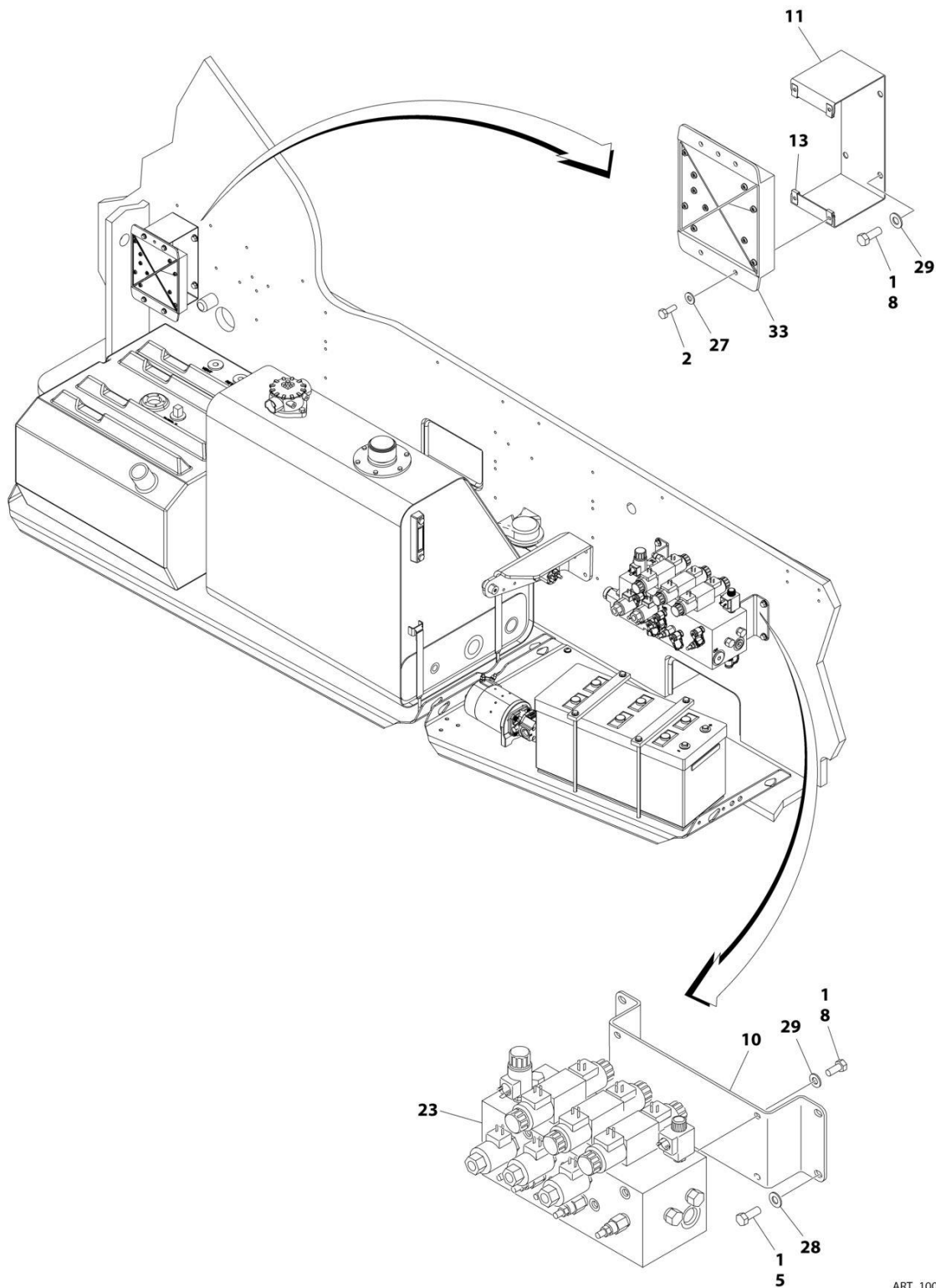
FIGURE 2-1. TURNTABLE VALVES INSTALLATION (Prior to SN 0300298064, Prior to SN B300017880, Excluding 0300287515, B300016940, B300017007 and B300017072)
