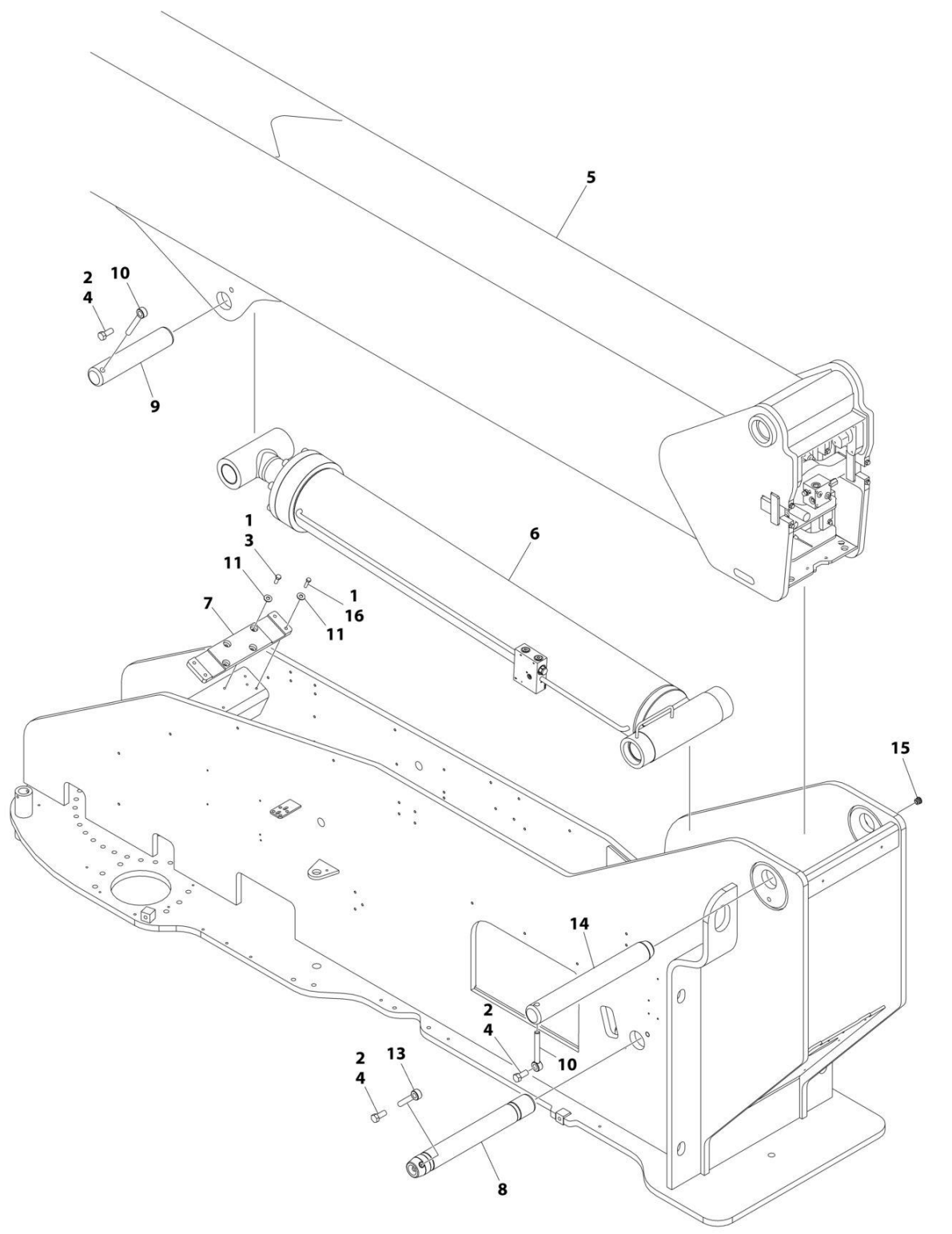
FIGURE 4-8. BOOM INSTALLATION - WITH COLD WEATHER PLUS PACKAGE (1350SJP) (Excluding B300016796, B300016807, B300016833 and B300016836)
