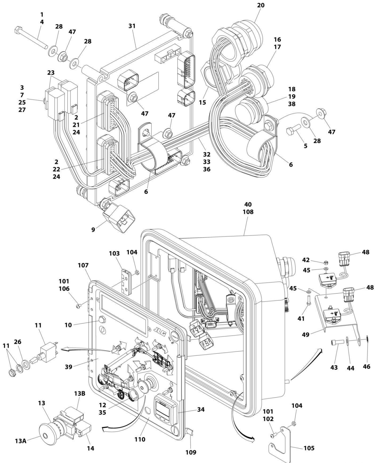
FIGURE 2-37. GROUND CONTROL BOX ASSEMBLY - DEUTZ TD2011 ENGINES (SN 0300298064 to Present, SN B300017880 to Present, Including 0300287515, B300016940, B300017007 and B300017072)
