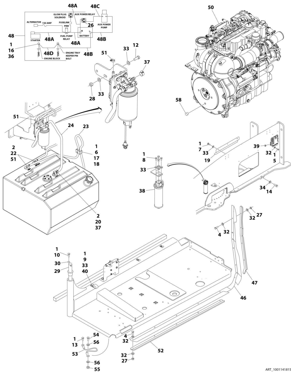
FIGURE 3-24. DEUTZ TCD2.9L4 ENGINE INSTALLATION - WITH REXROTH PUMPS AND STEEL HOODS (WITH COLD WEATHER PLUS PACKAGE)
