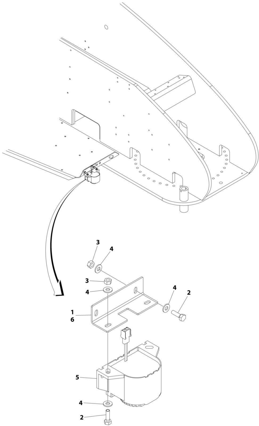
FIGURE 2-47. ALARM AMBIENT (WHITE NOISE) INSTALLATION (ALARM WITH HORIZONTAL BAR GRILLE)
