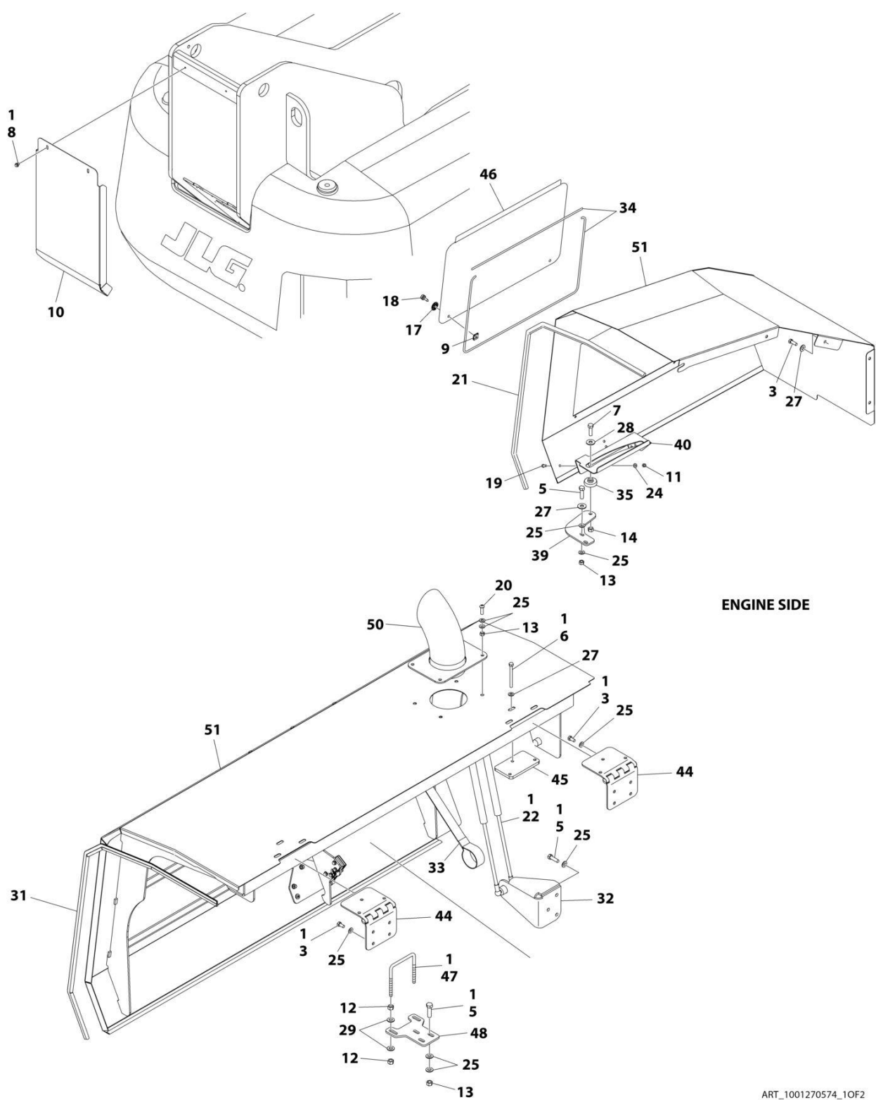
FIGURE 2-58. HOOD INSTALLATION - DEUTZ TCD2.9L (CHINA IV) ENGINES (STEEL)
