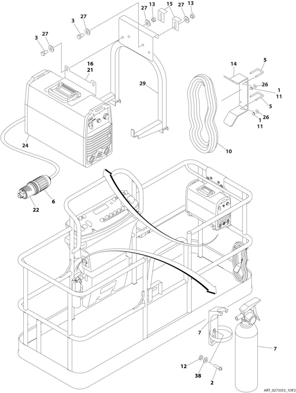
FIGURE 5-47. SKYWELDER/SKYCUTTER COMBO INSTALLATION (60HZ) (ANSI, ANSI EXPORT, CHINA, CSA AND JAPANESE SPECS)
