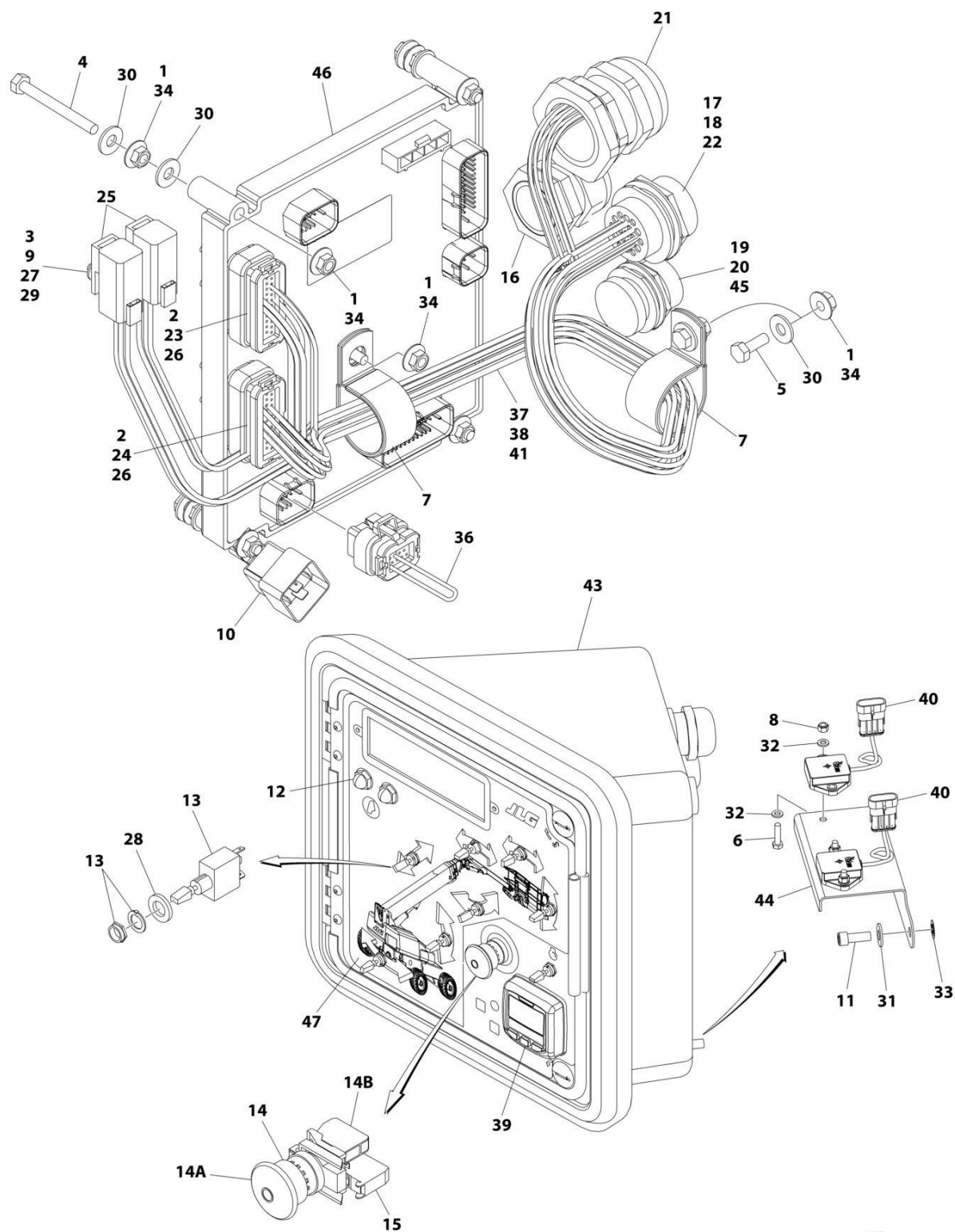
FIGURE 2-41. GROUND CONTROL BOX ASSEMBLY - DEUTZ TCD2.9L4 CHINA IV ENGINES (SN 0300298064 to Present, SN B300017880 to Present, Including 0300287515, B300016940, B300017007 and B300017072)
