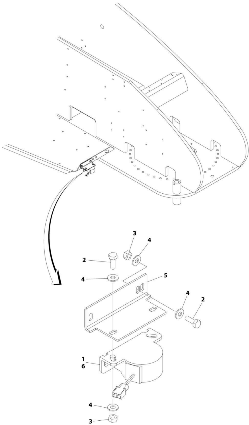
FIGURE 2-48. ALARM AMBIENT (WHITE NOISE) INSTALLATION (ALARM WITH CROSS HATCH GRILLE)
