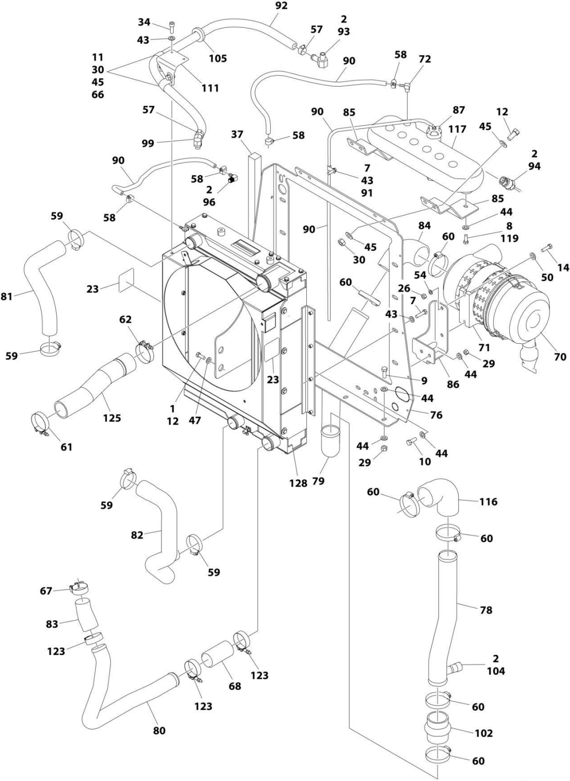
FIGURE 3-44. ENGINE ASSEMBLY - DEUTZ TCD2.9L4 (CHINA IV) (SN 0300297979 to Present, SN B300017842 to Present, SN B300016940 through B300016942, Including 0300287515, B300017007 and B300017072)
