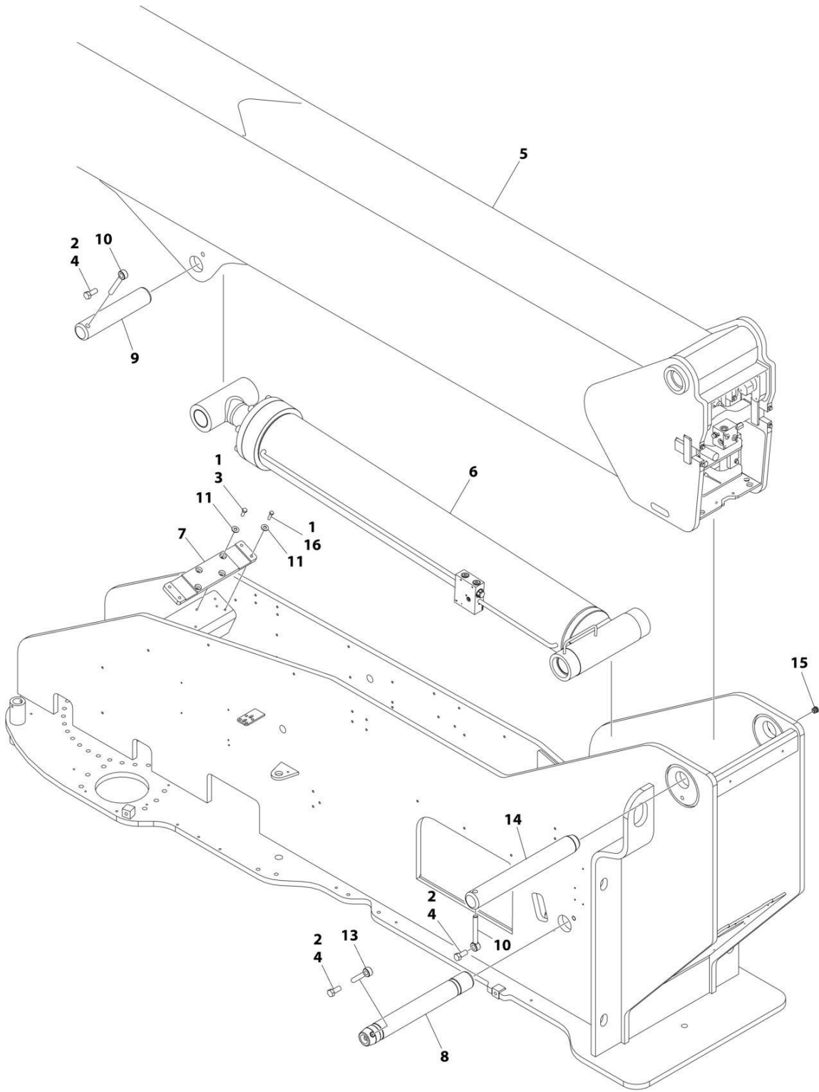
FIGURE 4-2. BOOM INSTALLATION - WITHOUT COLD WEATHER PLUS PACKAGE (1200SJP) (Excluding B300016796, B300016807, B300016833 and B300016836)
