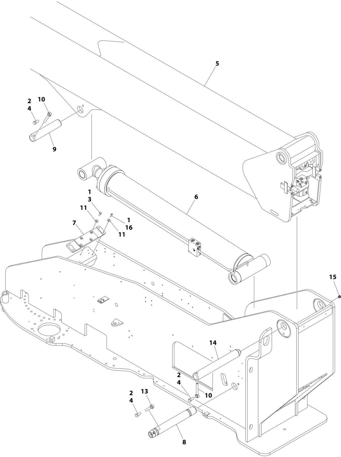
FIGURE 4-1. BOOM INSTALLATION - WITHOUT COLD WEATHER PLUS PACKAGE (1200SJP) (Including B300016796, B300016807, B300016833 and B300016836)
