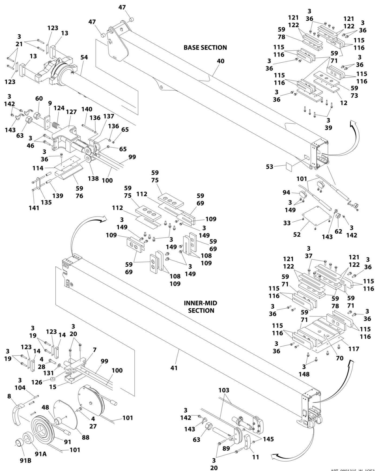
FIGURE 4-13. BOOM ASSEMBLY - WITHOUT COLD WEATHER PLUS PACKAGE (1350SJP)
