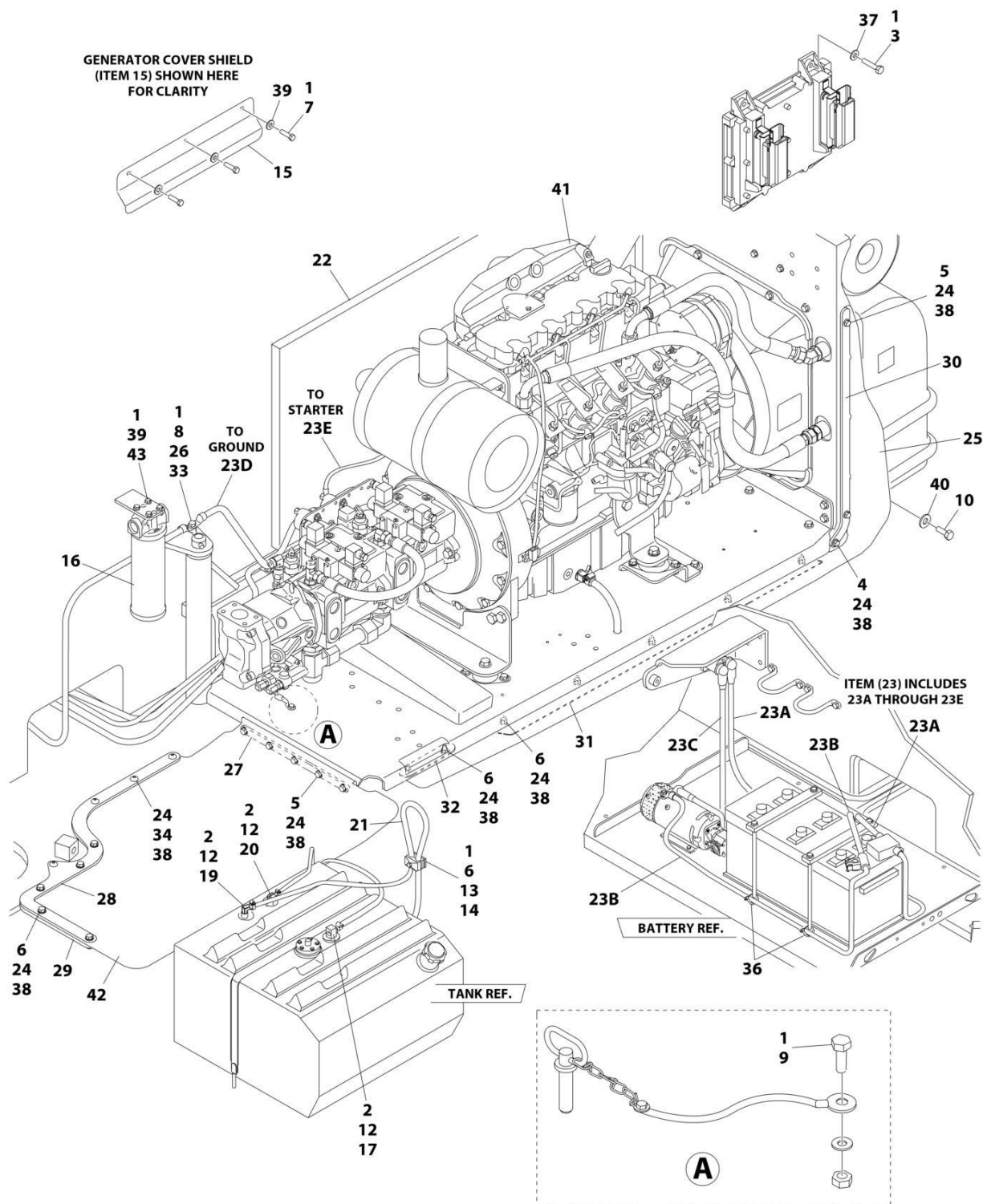
FIGURE 3-3. DEUTZ TD2011 ENGINE INSTALLATION - WITH REXROTH PUMPS AND STEEL HOOD (WITHOUT SKYPOWER AND WITHOUT COLD WEATHER PLUS PACKAGE)
