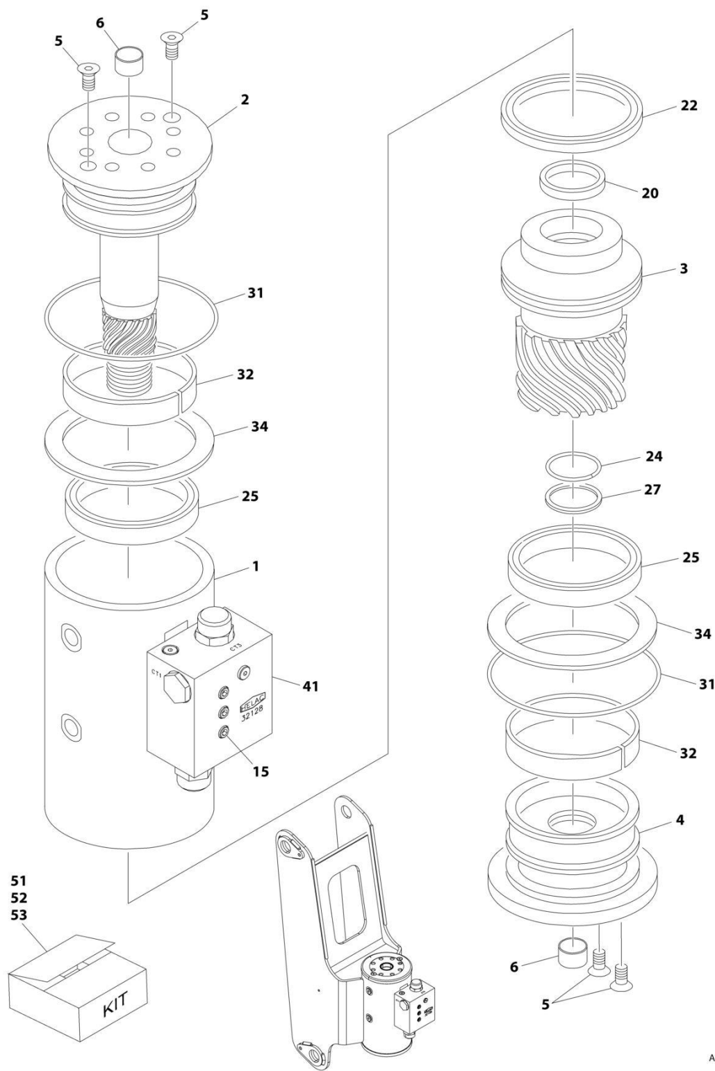
FIGURE 4-16. PLATFORM ROTATE ASSEMBLY
