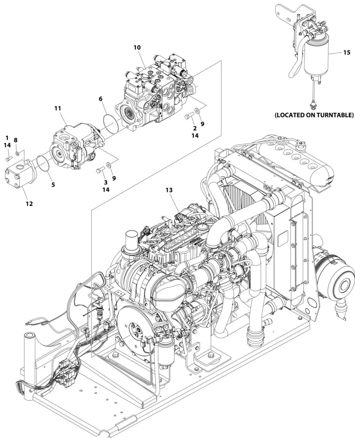
FIGURE 3-30. DEUTZ TCD2.9L4 ENGINE SUB-ASSEMBLY - WITH SAUER PUMP (WITHOUT COLD WEATHER PLUS PACKAGE)
