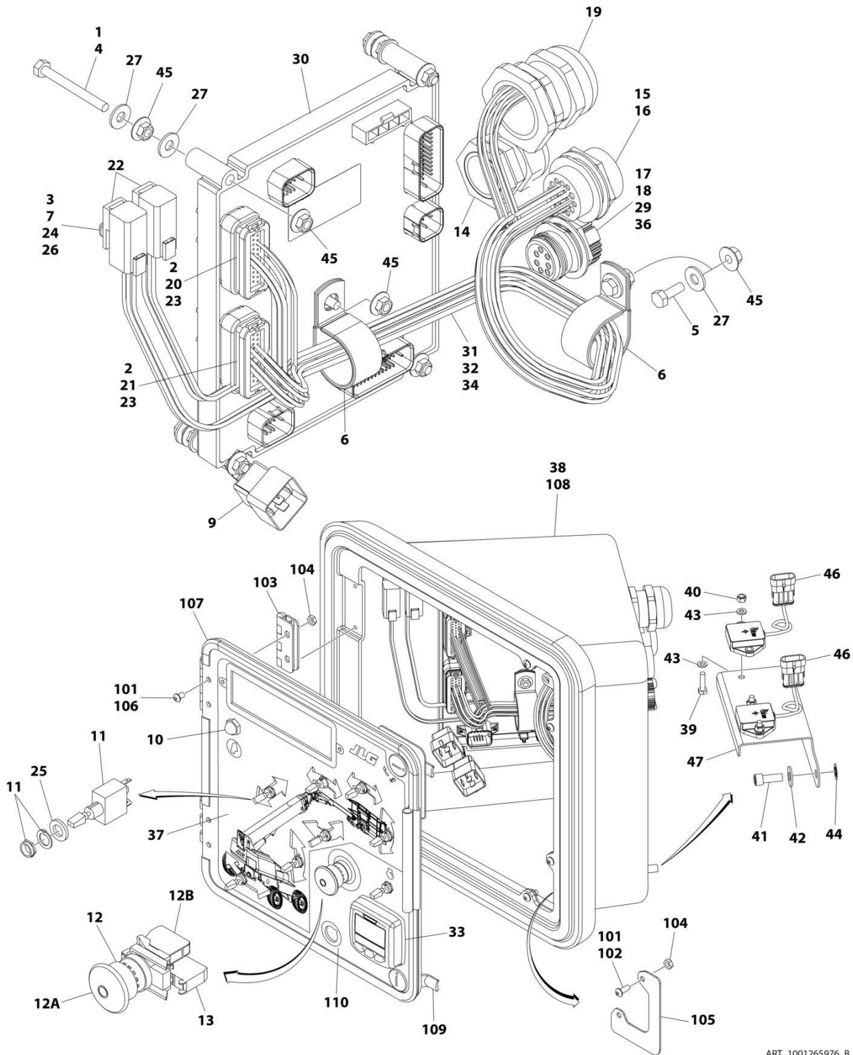
FIGURE 2-33. GROUND CONTROL BOX ASSEMBLY - DEUTZ TCD2.9L4 ENGINES - WITH DIGITAL DISPLAY (Prior to SN 0300298064, Prior to SN B300017880, Excluding 0300287515, B300016940, B300017007 and B300017072)
