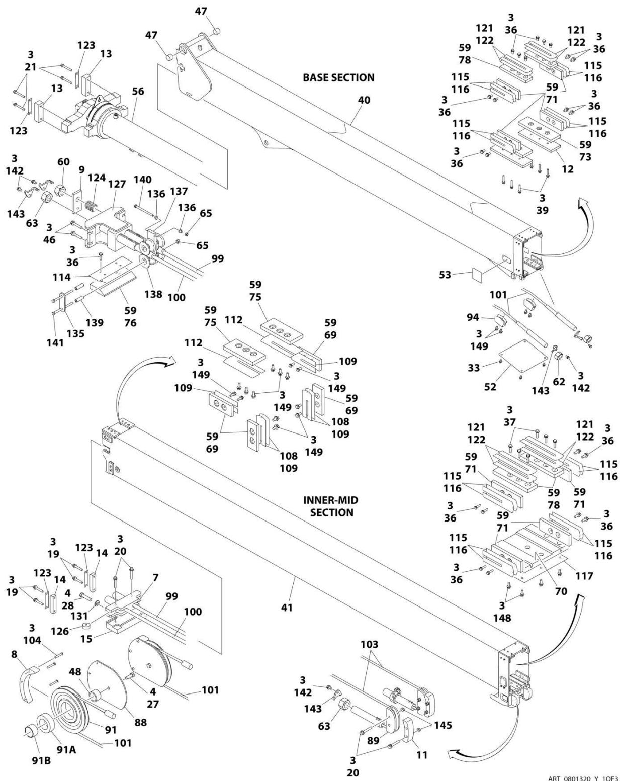
FIGURE 4-9. BOOM ASSEMBLY - WITHOUT COLD WEATHER PLUS PACKAGE (1200SJP) (Prior to SN 0300296108, Prior to SN B300016940, Excluding 030026105 and B300016704)
