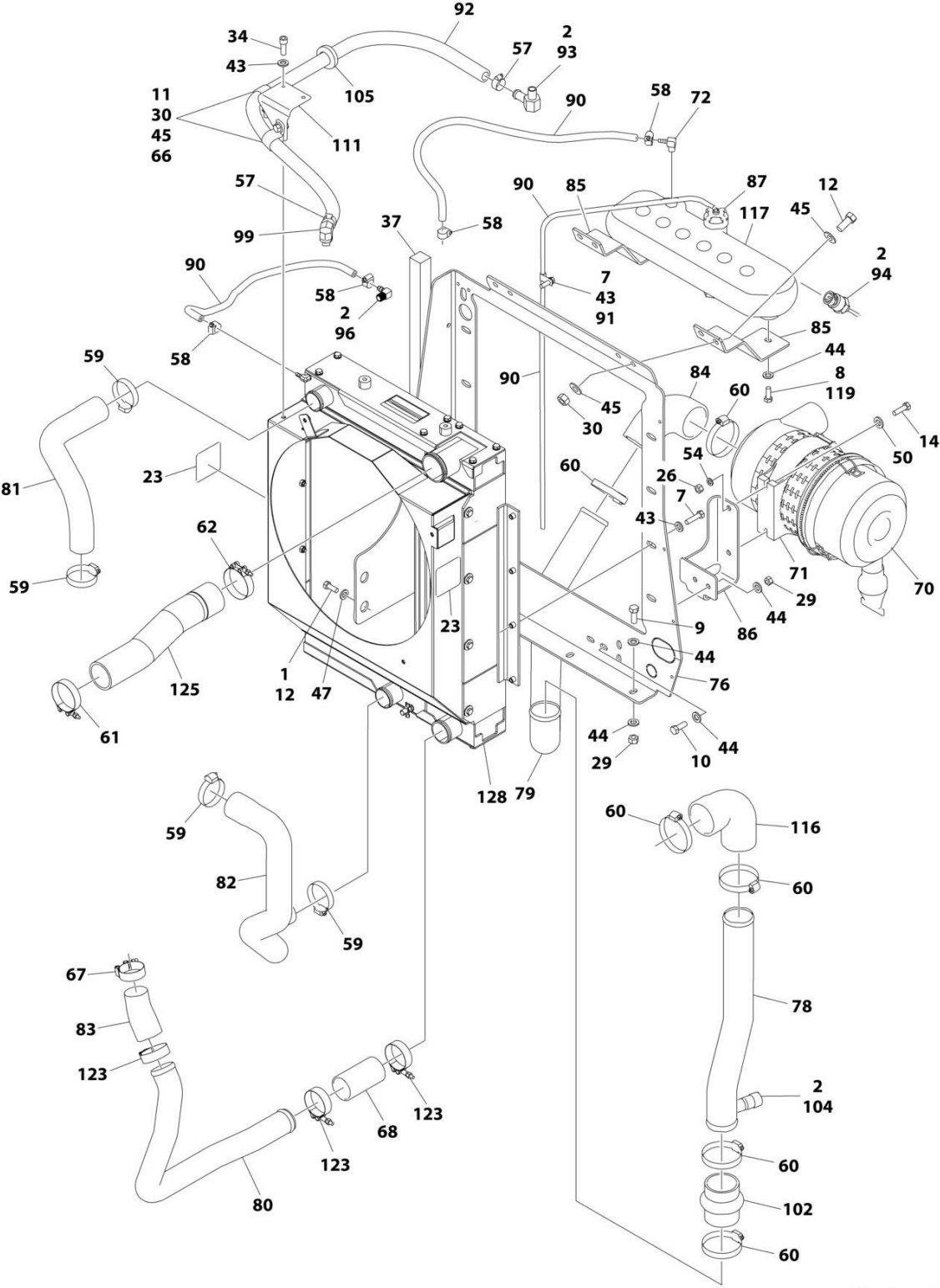
FIGURE 3-43. ENGINE ASSEMBLY - DEUTZ TCD2.9L4 (CHINA IV) (Prior to SN 0300297979, Prior to SN B300017842, Except SN B300016940 through B300016942, Excluding 0300287515, B300017007 and B300017072)
