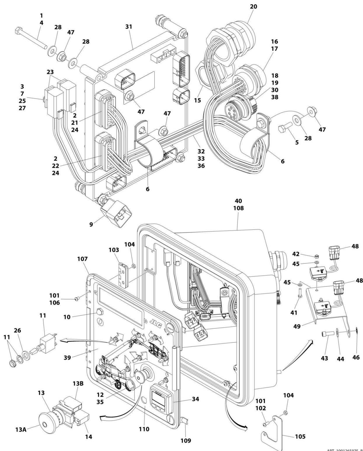
FIGURE 2-36. GROUND CONTROL BOX ASSEMBLY - DEUTZ TD2011 ENGINES (Prior to SN 0300298064, Prior to SN B300017880, Excluding 0300287515, B300016940, B300017007 and B300017072)
