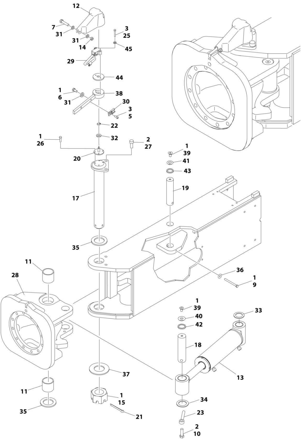
FIGURE 1-3. STEER INSTALLATION
