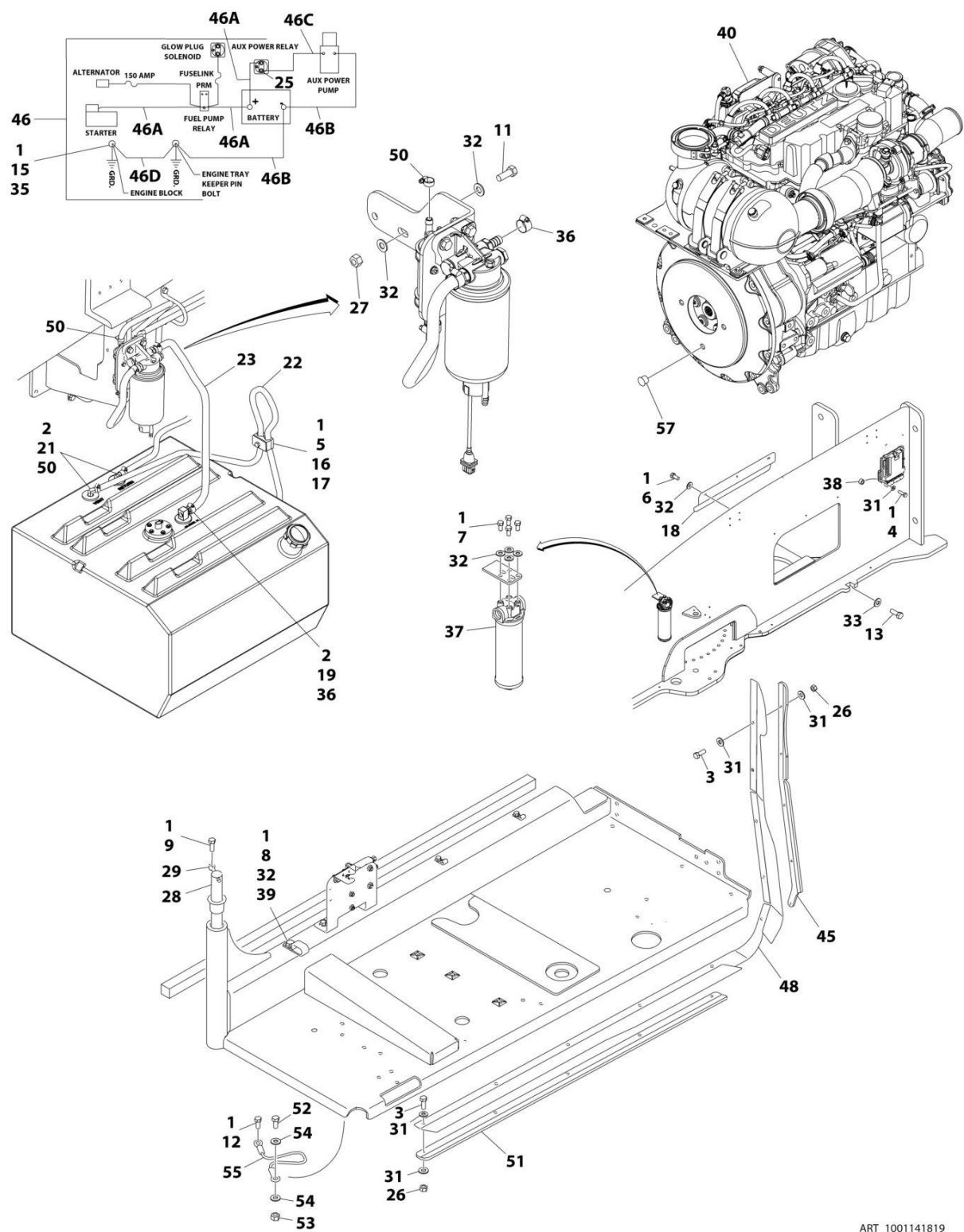
FIGURE 3-22. DEUTZ TCD2.9L4 ENGINE INSTALLATION - WITH REXROTH PUMPS AND ABS HOODS (WITHOUT COLD WEATHER PLUS PACKAGE)
