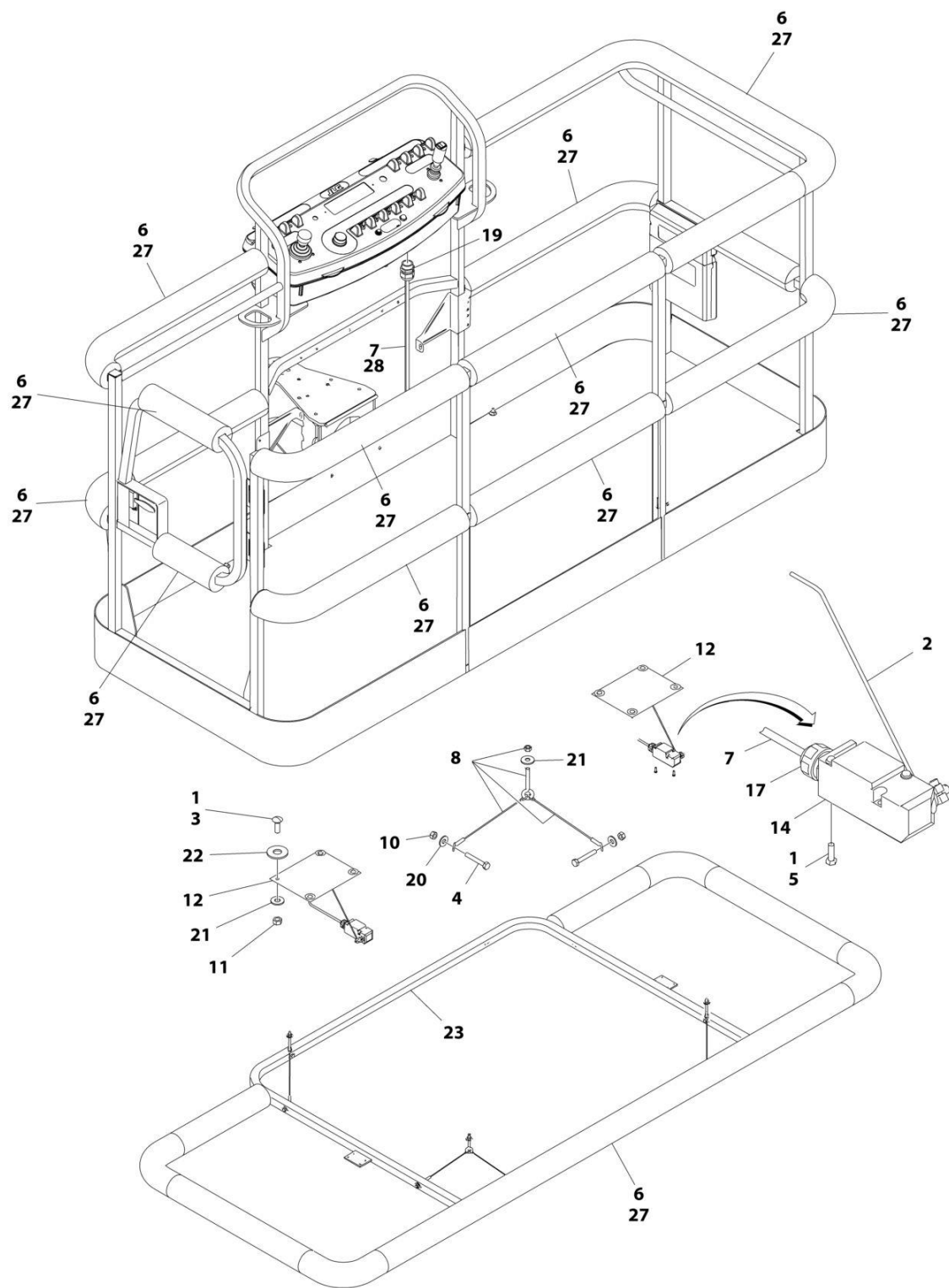
FIGURE 5-48. SOFT TOUCH SYSTEM INSTALLATION - 8FT/2.4M PLATFORMS (ALL SPECS) (1350SJP)
