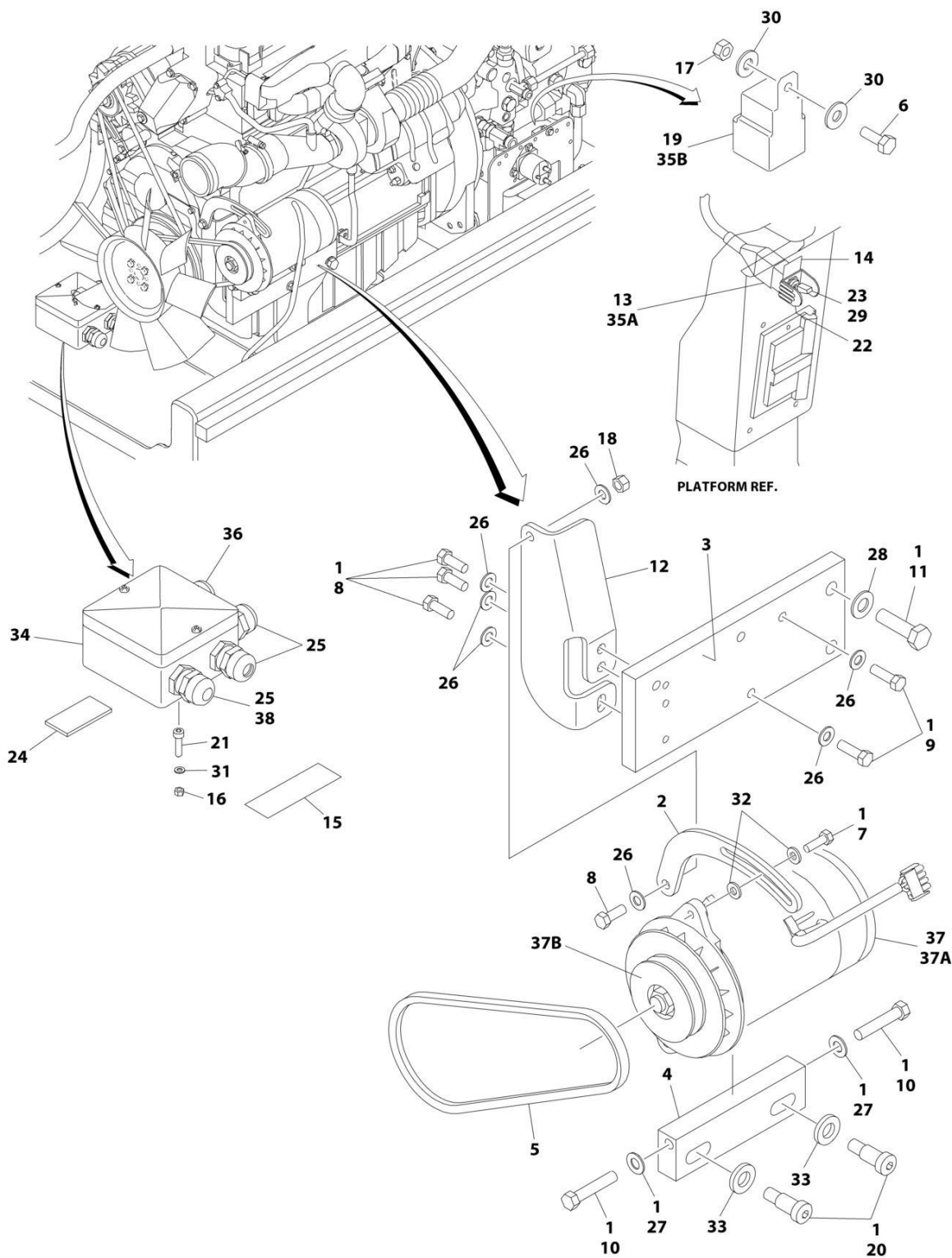
FIGURE 3-60. 2500W GENERATOR INSTALLATION - 50HZ SPEC (DEUTZ TD2011 ENGINES) (OPTIONAL)
