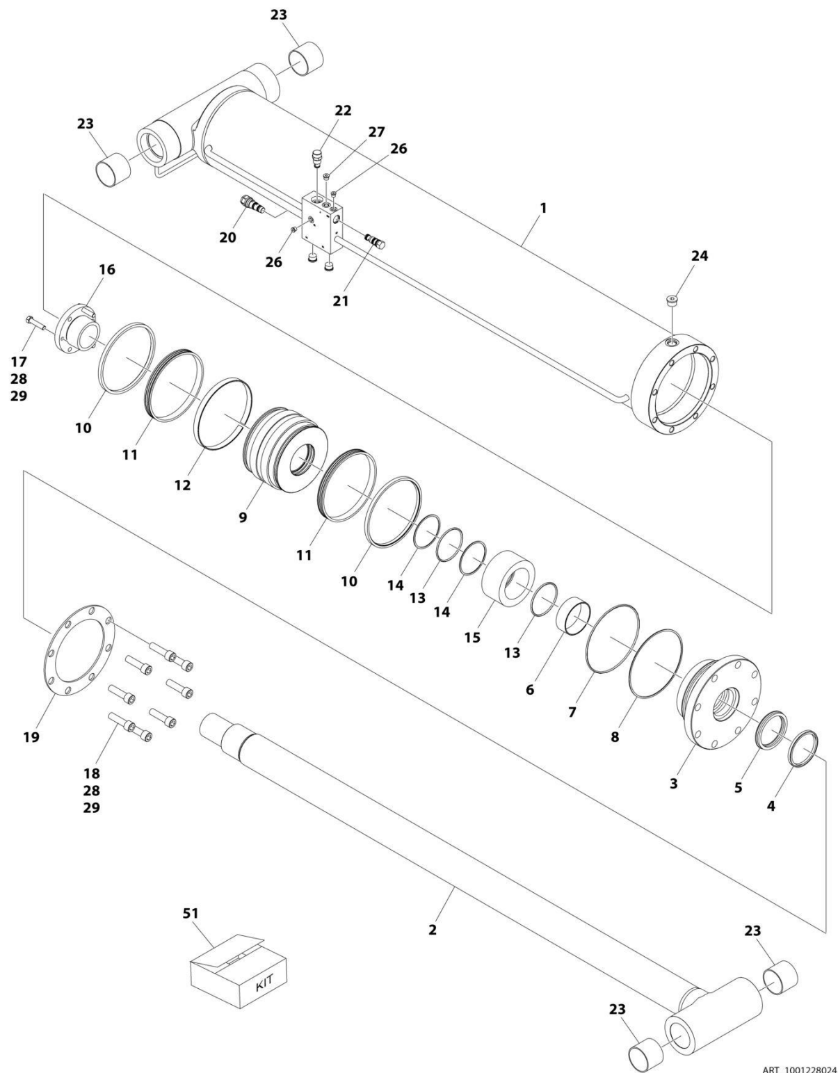
FIGURE 6-5. LIFT CYLINDER ASSEMBLY (Including B300016796, B300016807, B300016833 and B300016836)
