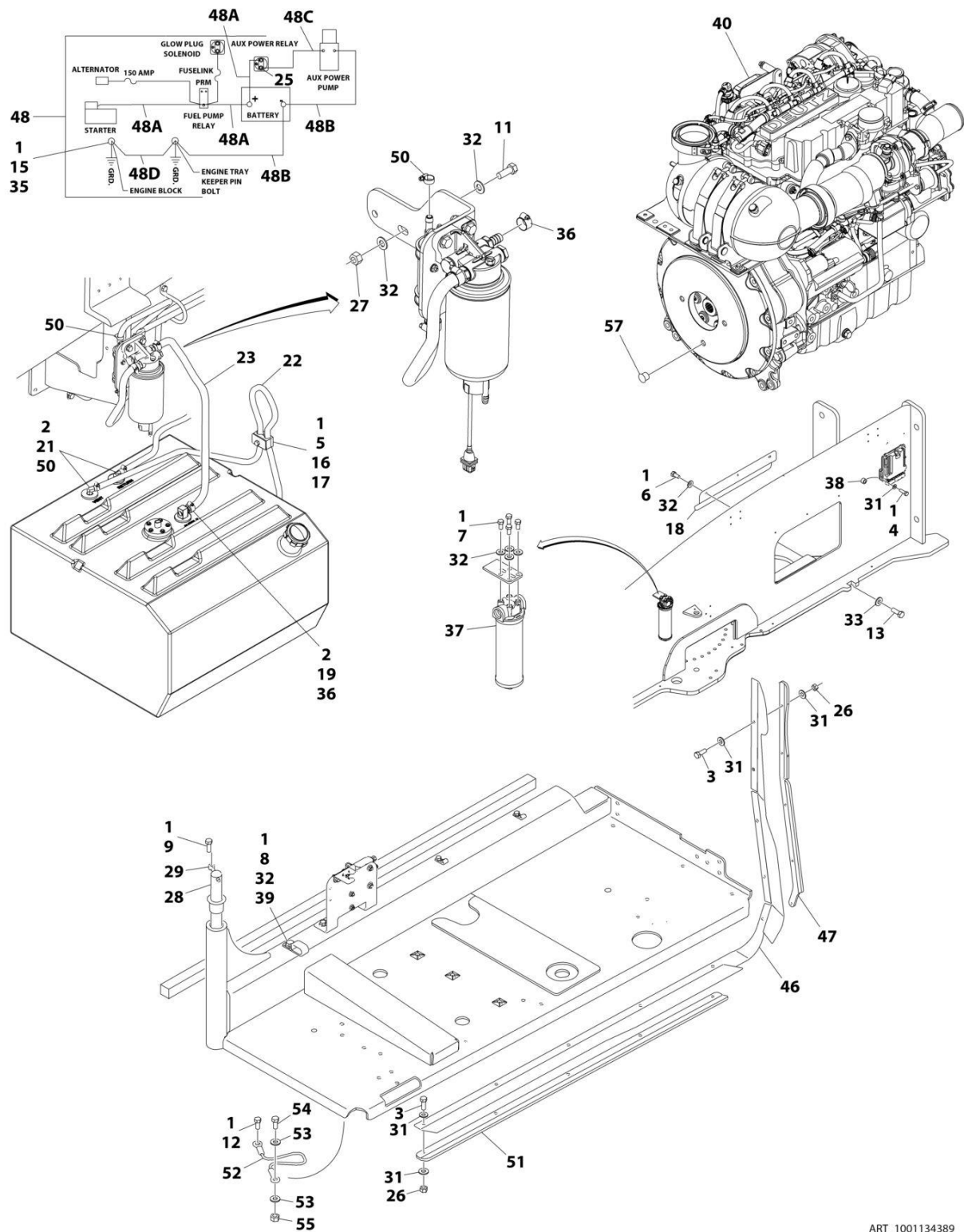
FIGURE 3-26. DEUTZ TCD2.9L4 ENGINE INSTALLATION - WITH SAUER PUMPS AND STEEL HOODS (WITHOUT COLD WEATHER PLUS PACKAGE)
