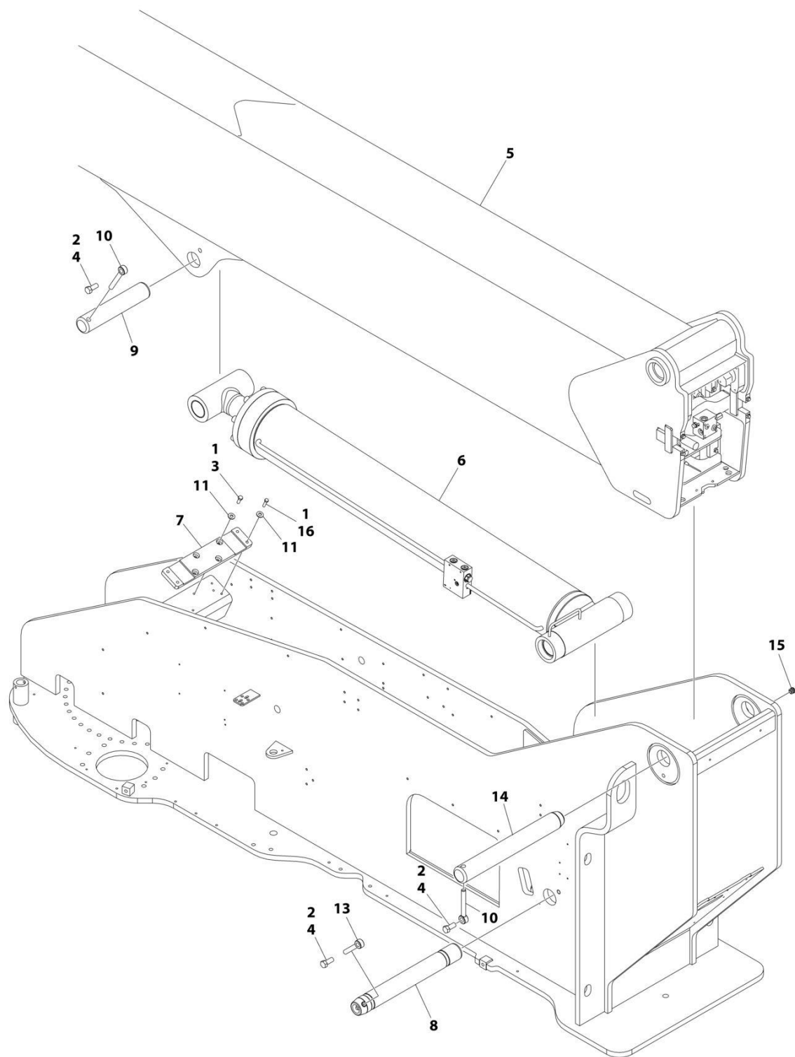
FIGURE 4-7. BOOM INSTALLATION - WITH COLD WEATHER PLUS PACKAGE (1350SJP) (Including B300016796, B300016807, B300016833 and B300016836)
