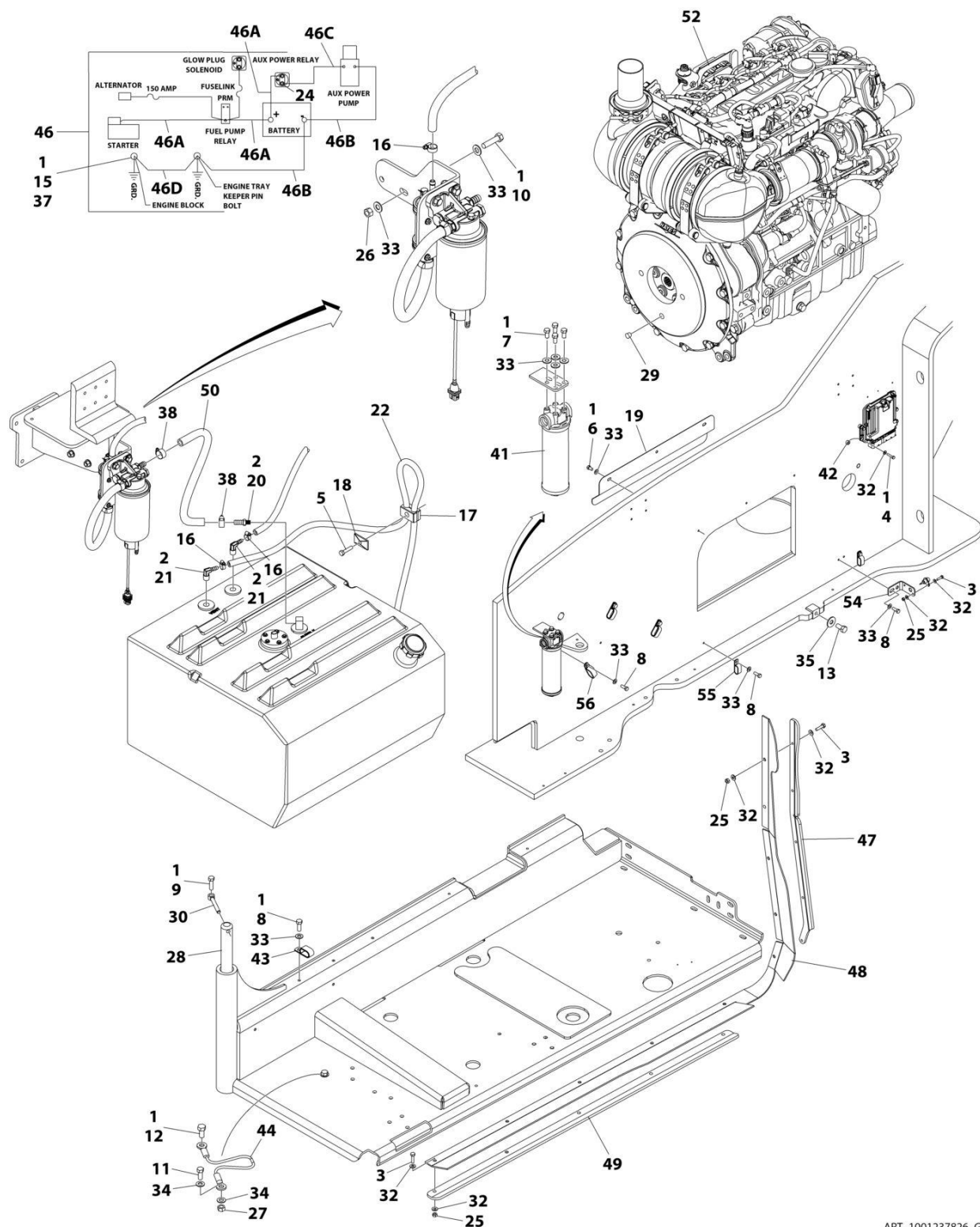
FIGURE 3-35. DEUTZ TCD2.9L4 (STAGE V) ENGINE INSTALLATION - WITH SAUER PUMPS AND ABS HOODS (WITHOUT COLD WEATHER PLUS PACKAGE)
