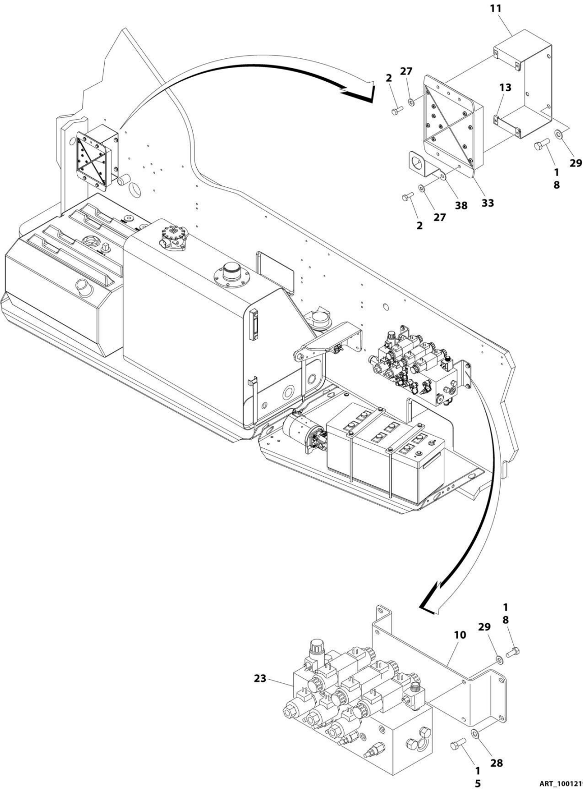
FIGURE 2-2. TURNTABLE VALVES INSTALLATION (SN 0300298064 to Present, SN B300017880 to Present, Including 0300287515, B300016940, B300017007 and B300017072)
