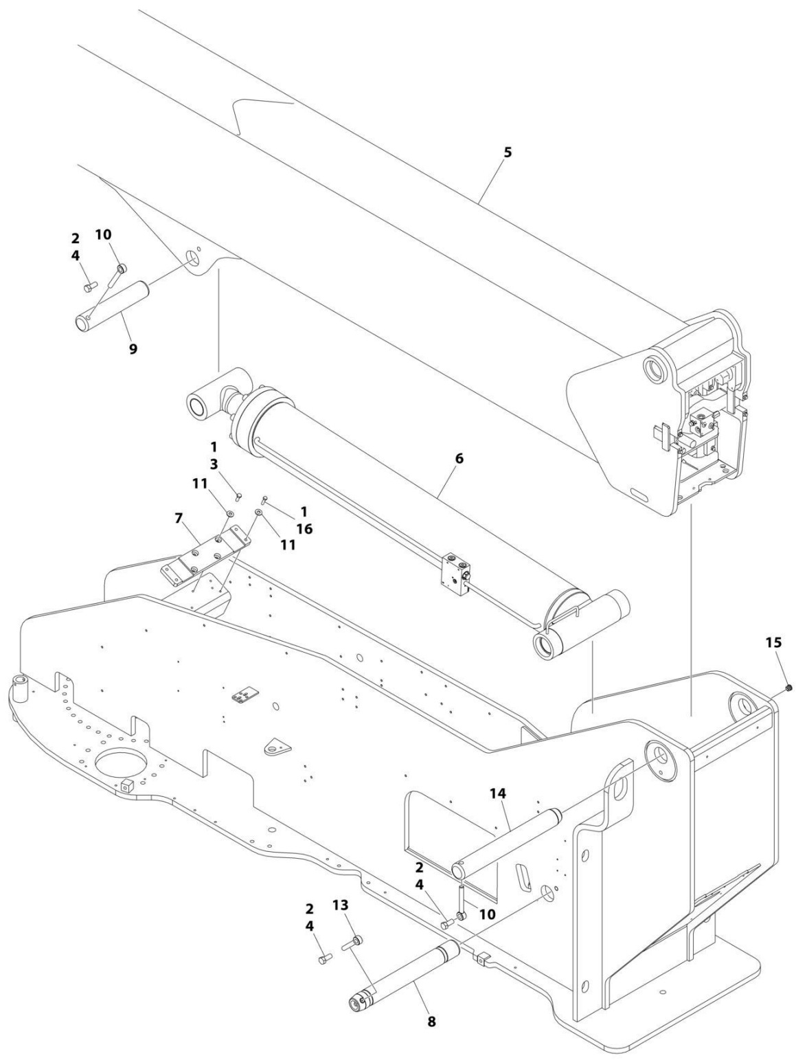
FIGURE 4-4. BOOM INSTALLATION - WITH COLD WEATHER PLUS PACKAGE (1200SJP) (Excluding B300016796, B300016807, B300016833 and B300016836)
