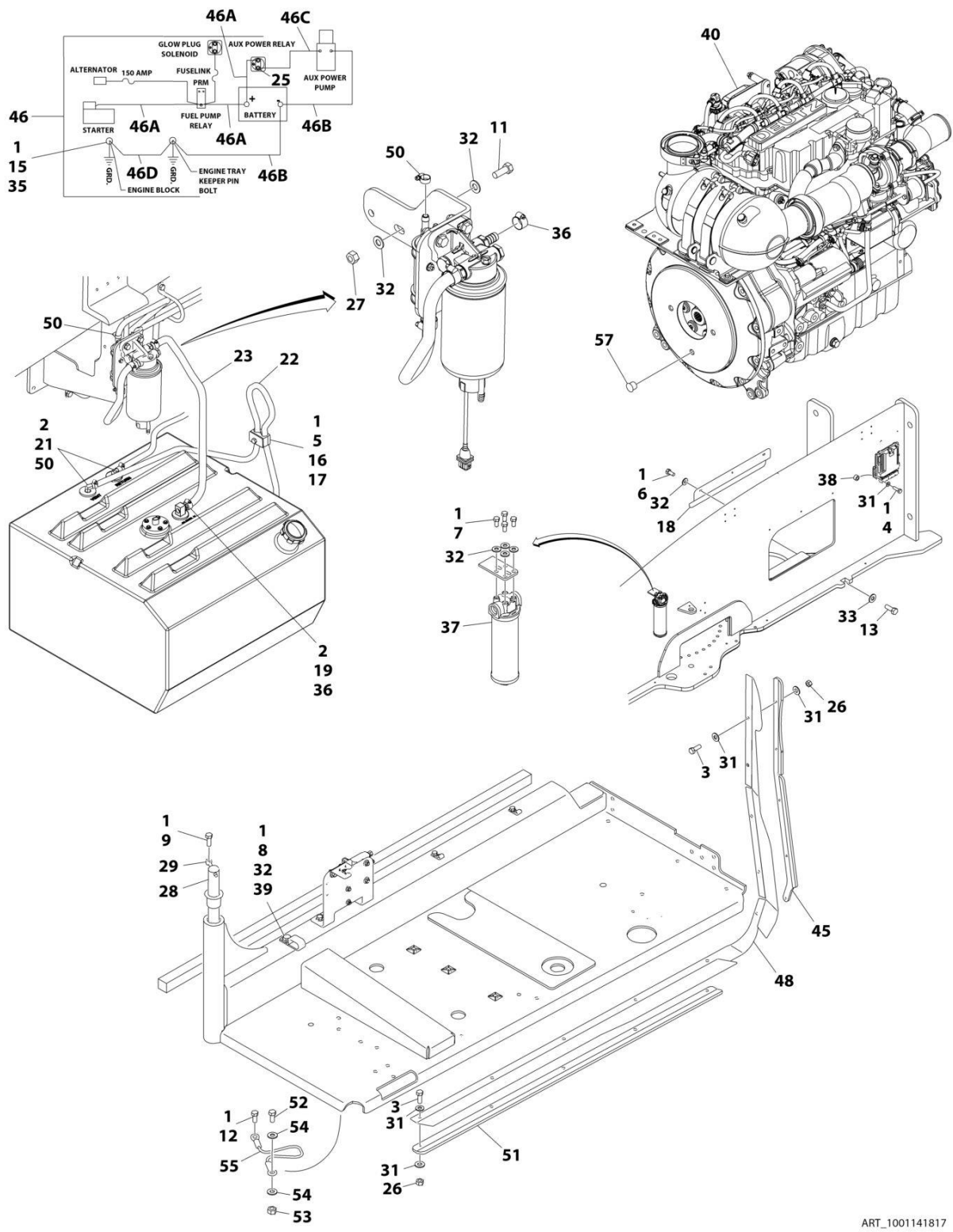
FIGURE 3-25. DEUTZ TCD2.9L4 ENGINE INSTALLATION - WITH SAUER PUMPS AND ABS HOODS (WITHOUT COLD WEATHER PLUS PACKAGE)
