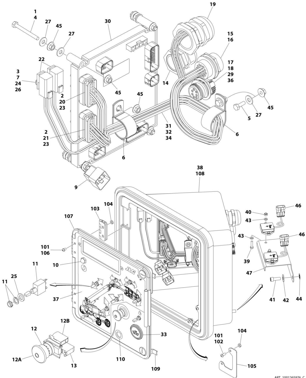
FIGURE 2-34. GROUND CONTROL BOX ASSEMBLY - DEUTZ TCD2.9L4 ENGINES - WITH MECHANICAL HOUR METER (Prior to SN 0300298064, Prior to SN B300017880, Excluding 0300287515, B300016940, B300017007 and B300017072)
