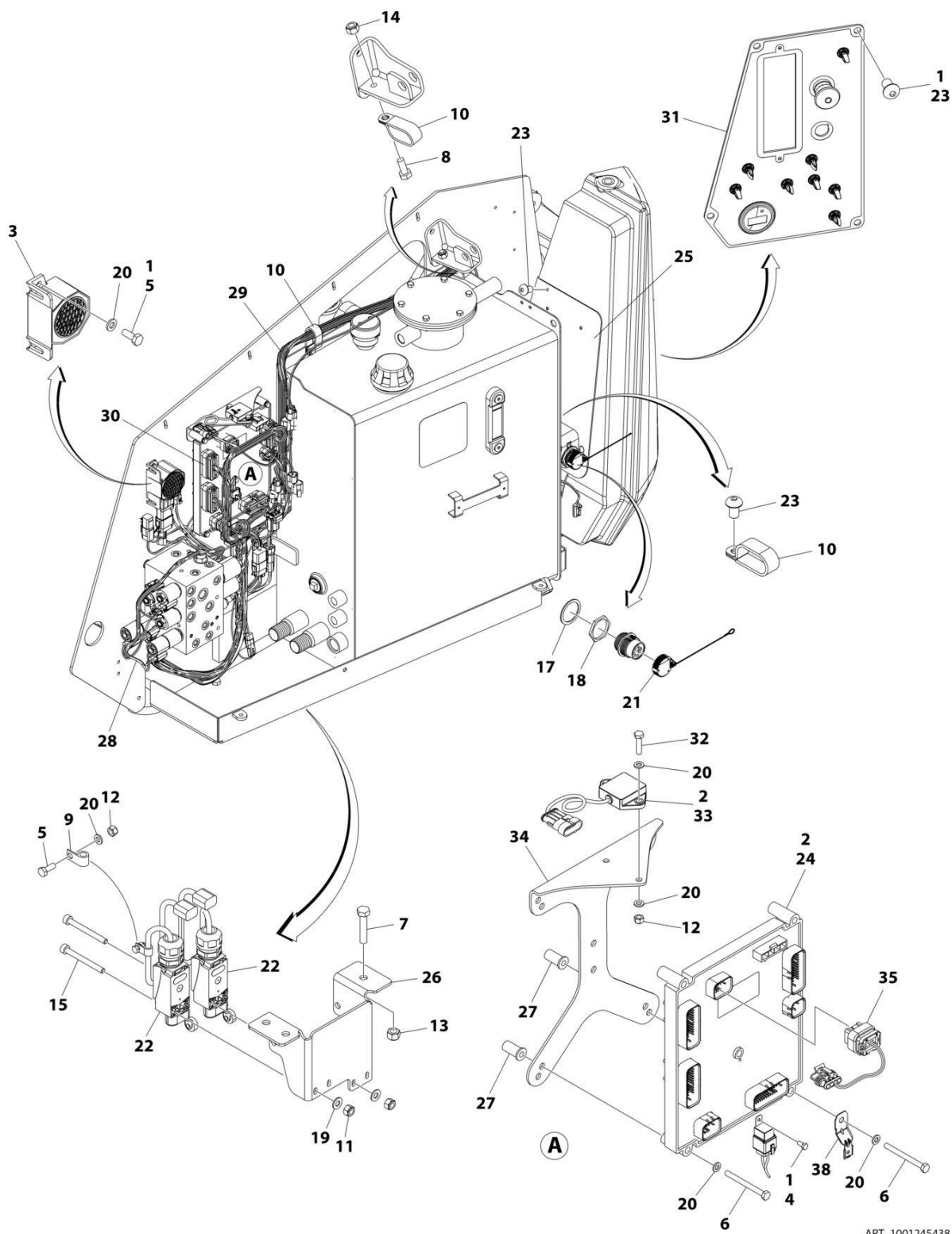
FIGURE 2-12. ELECTRICAL COMPONENTS INSTALLATION (ALL SPECS EXCEPT CE & UK CA)
