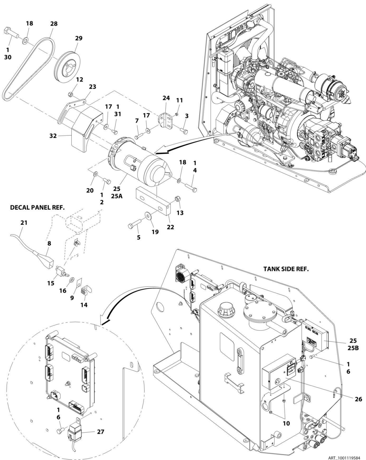
FIGURE 3-24. 3500W GENERATOR INSTALLATION - KUBOTA ENGINE MACHINES 220V/60HZ GENERATOR (ANSI EXPORT, CHINA AND CSA SPECS)
