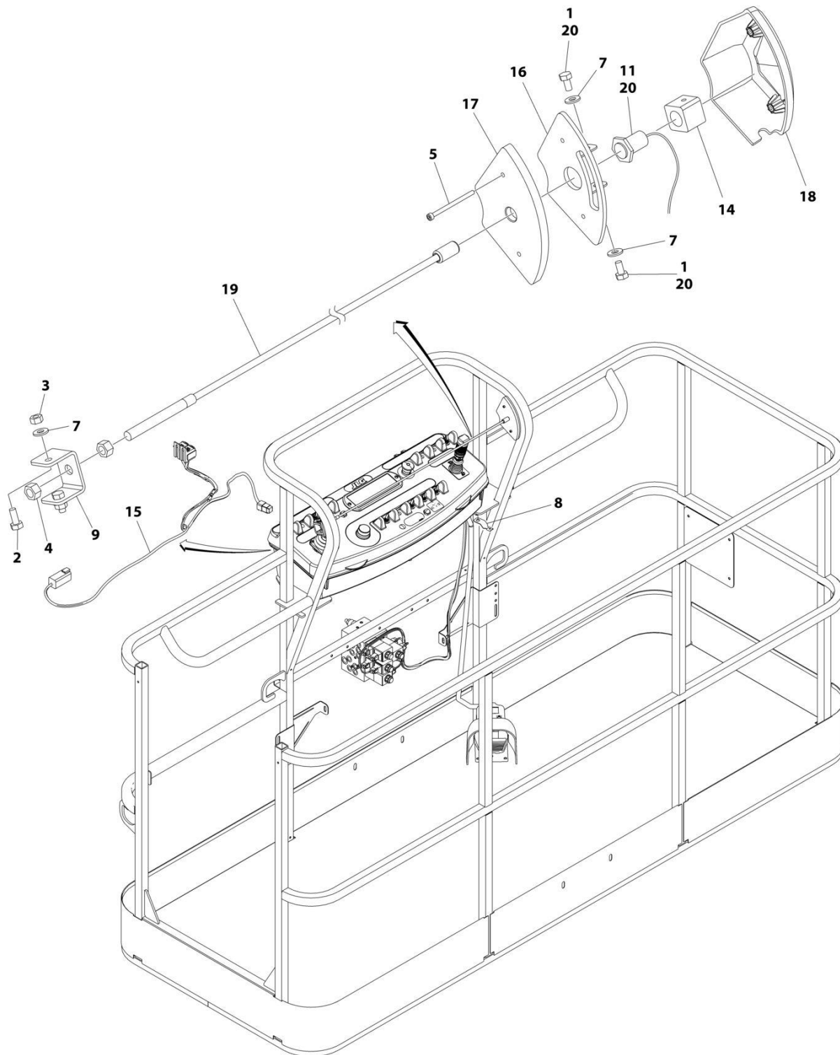
FIGURE 5-17. SKYLINE INSTALLATION
