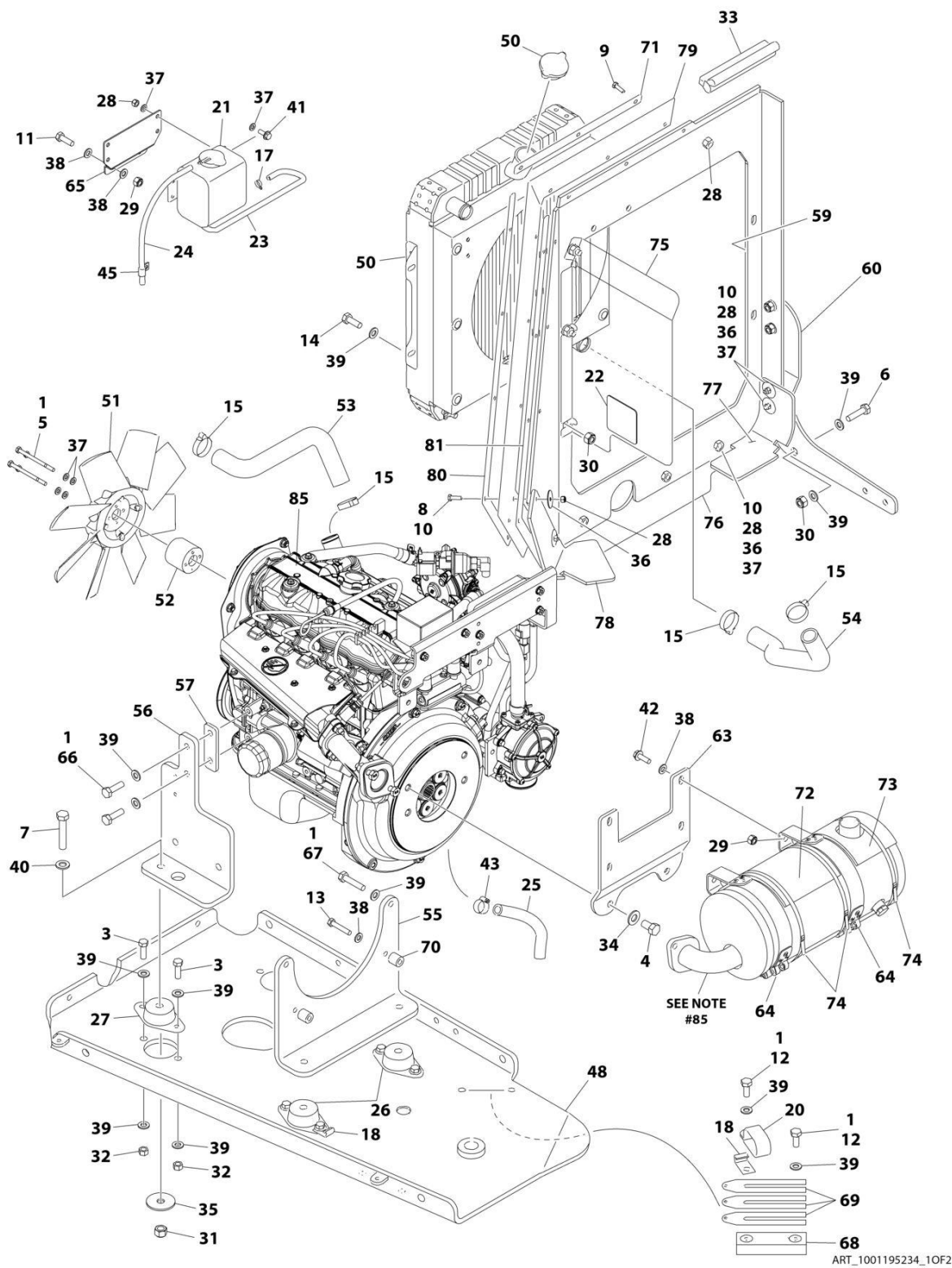
FIGURE 3-4. GM ENGINE ASSEMBLY
