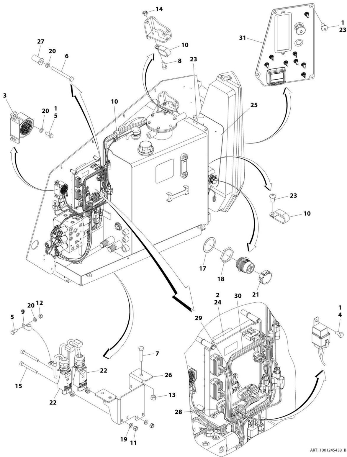
FIGURE 2-11. ELECTRICAL COMPONENTS INSTALLATION (ALL SPECS EXCEPT CE & UK CA) (Prior to SN 0300291111)
