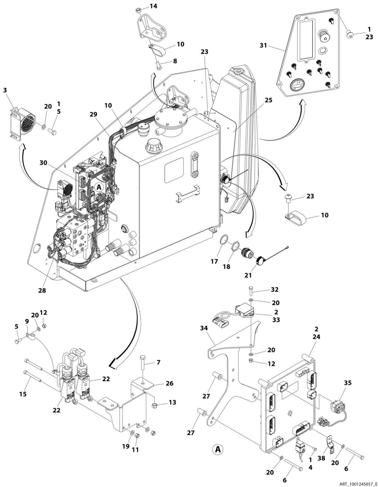
FIGURE 2-14. ELECTRICAL COMPONENTS INSTALLATION (CE & UK CA SPEC)
