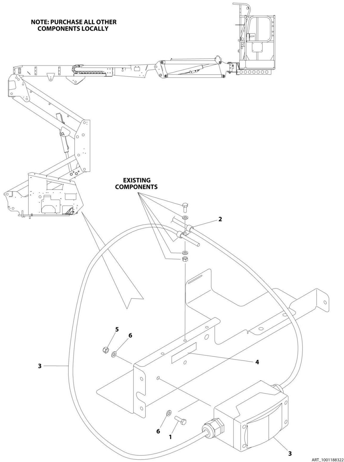
FIGURE 8-31. BREAKER BOX INSTALLATION
