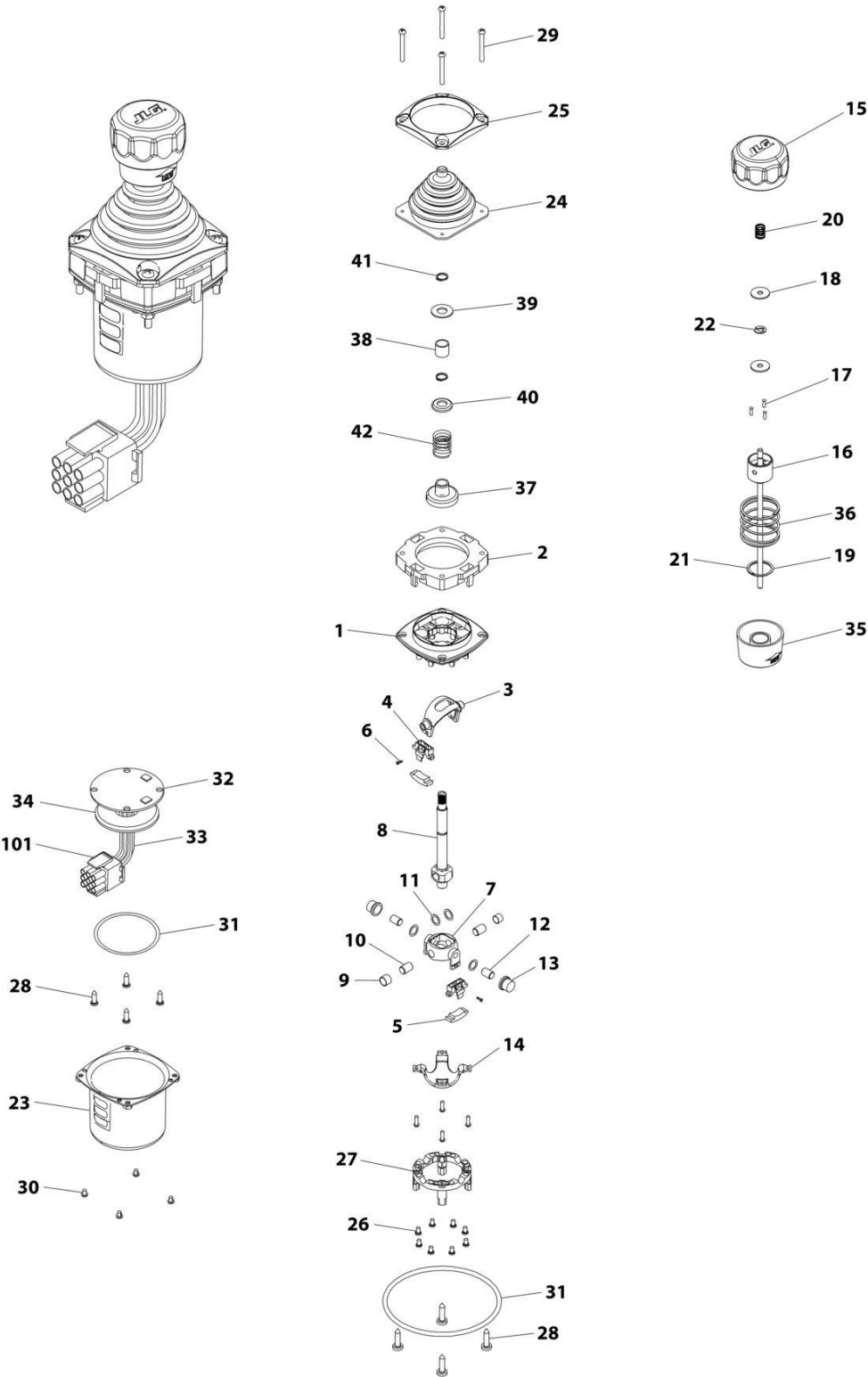
FIGURE 5-10. LIFT/SWING CONTROLLER ASSEMBLY
