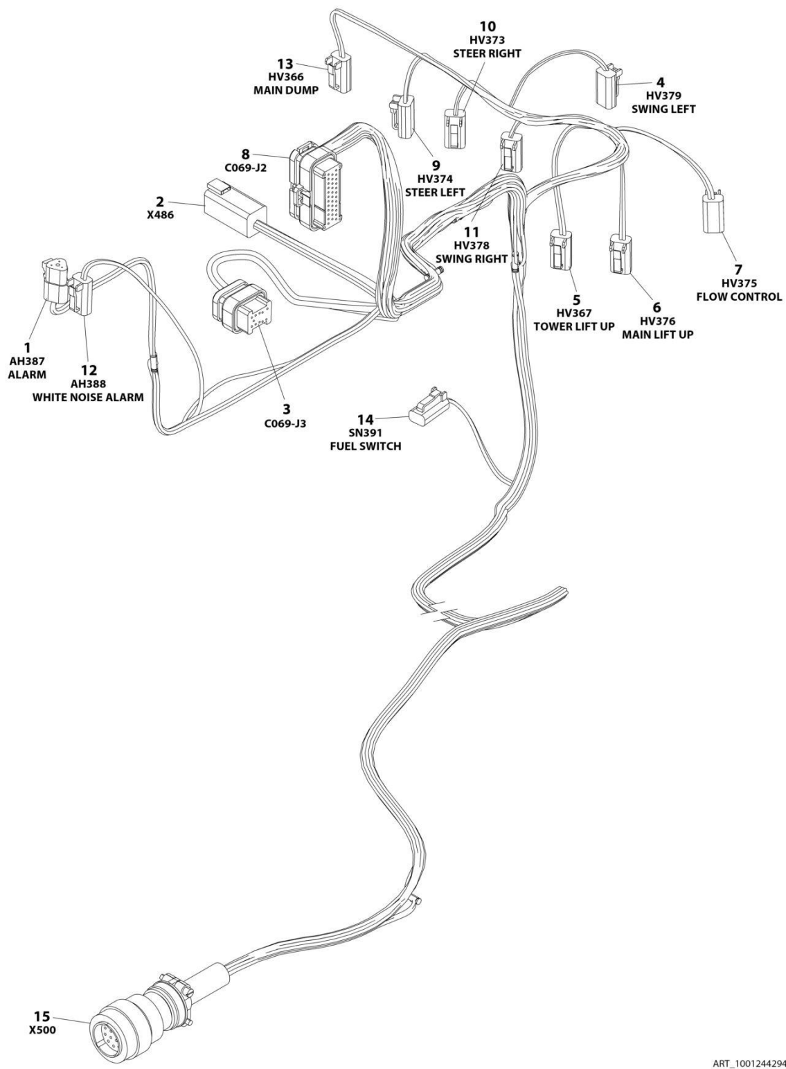
FIGURE 8-49. VALVE HARNESS - MAIN VALVE (Prior to SN B300017683, Including B300017688)
