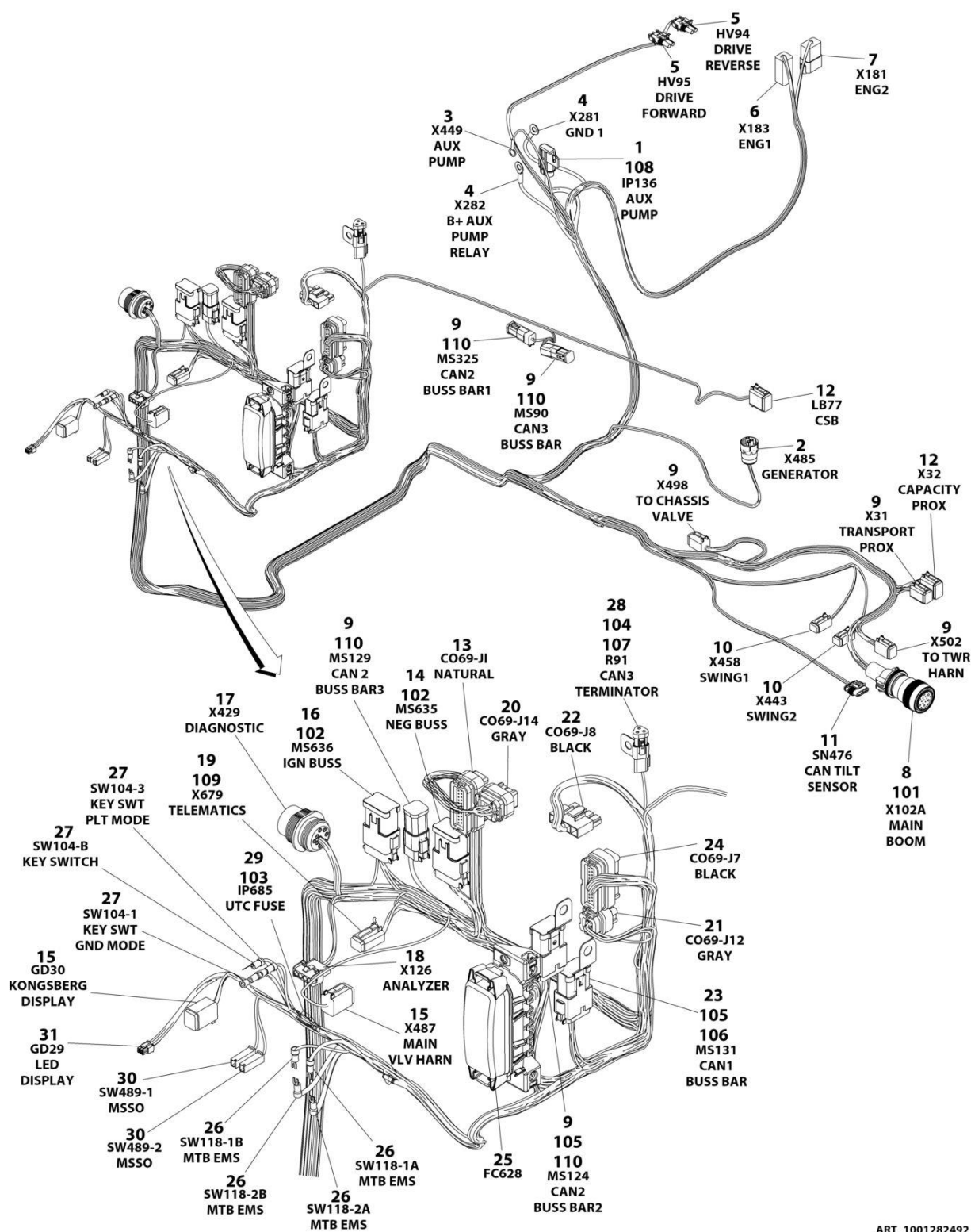
FIGURE 8-47. TURNTABLE HARNESS (SN B300017683 to Present, Excluding B300017688)
