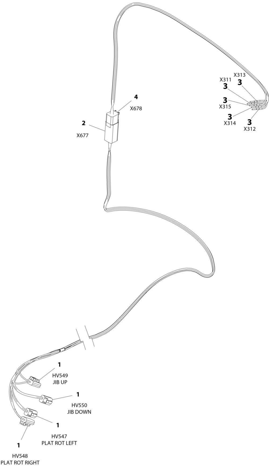
FIGURE 8-51. VALVE HARNESS - PLATFORM VALVE
