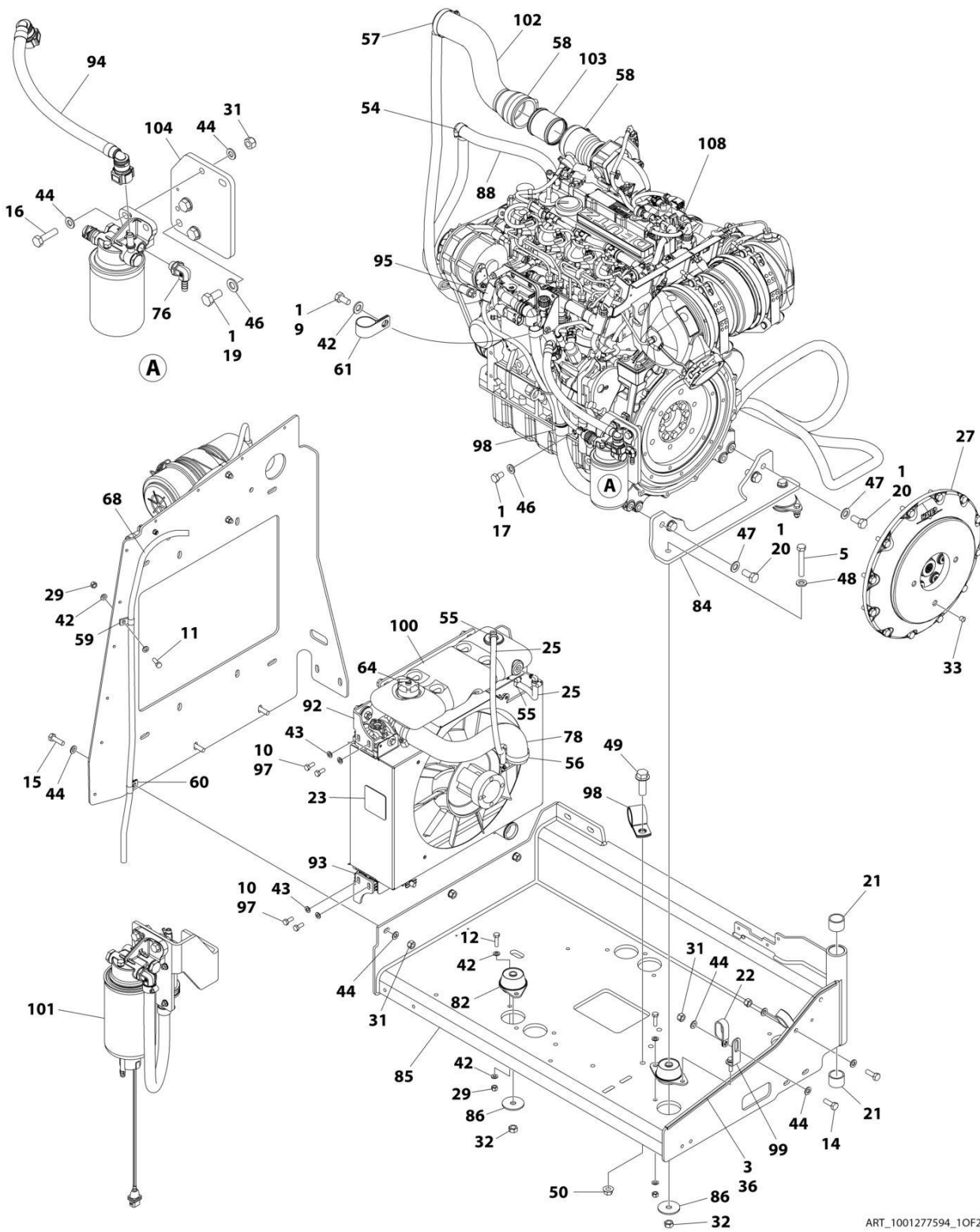
FIGURE 3-7. ENGINE ASSEMBLY – DEUTZ D2.9L4 ENGINE (STAGE V) (CE & UK CA SPECS)
