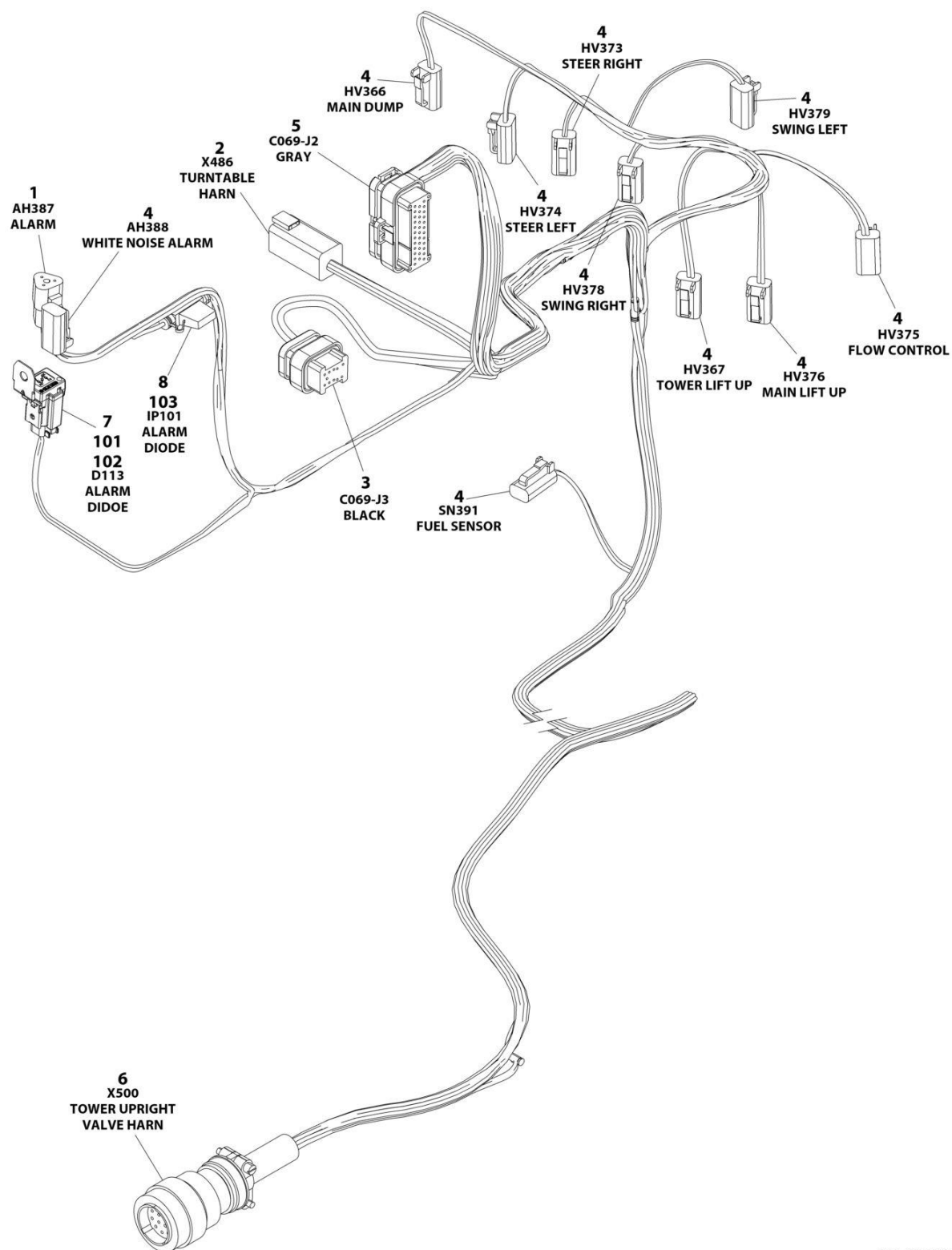
FIGURE 8-50. VALVE HARNESS - MAIN VALVE (SN B300017683 to Present, Excluding B300017688)
