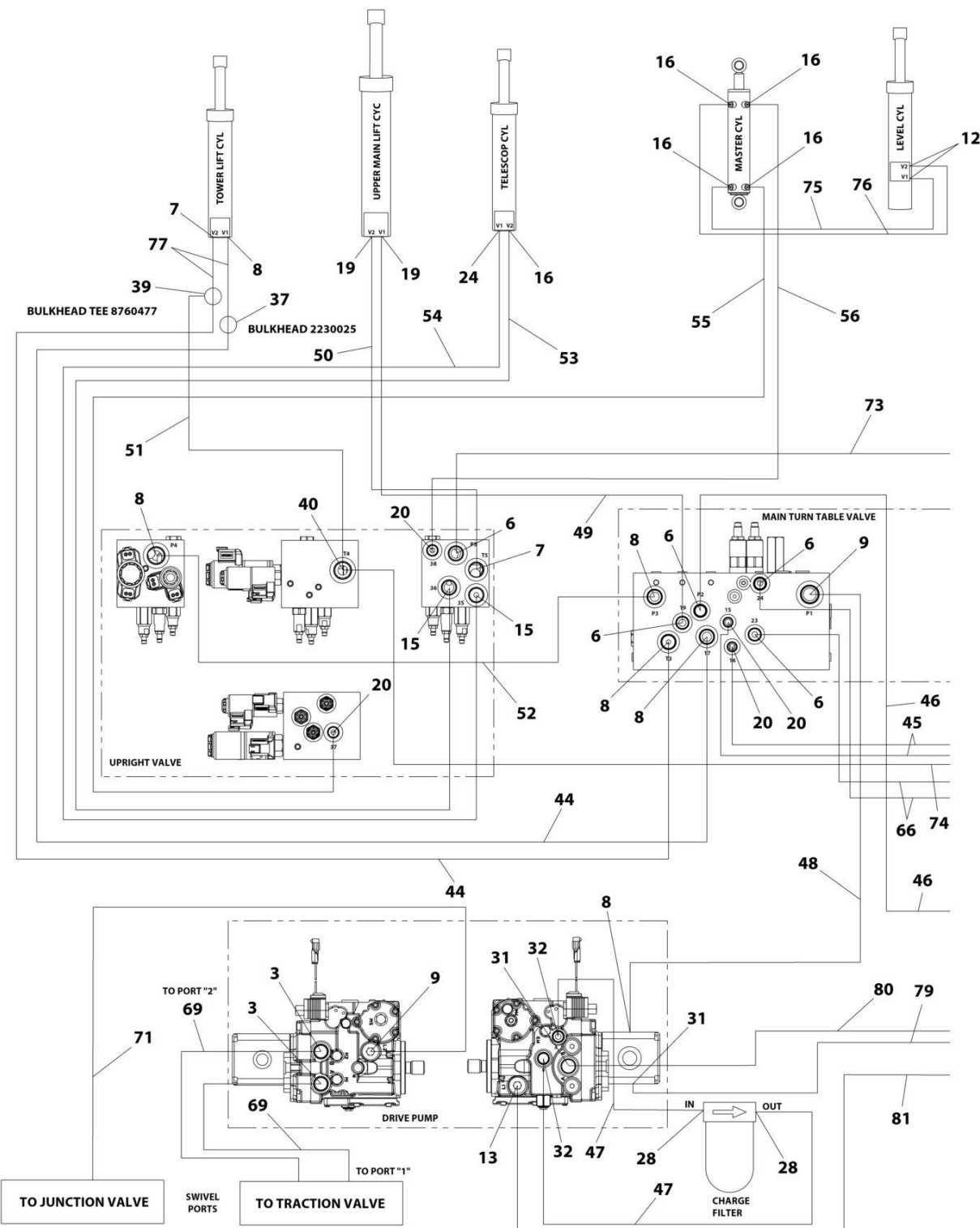
FIGURE 7-1. HYDRAULIC SYSTEM INSTALLATION
