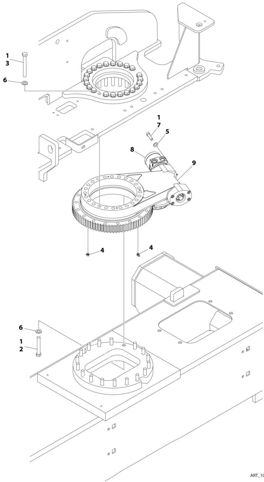
FIGURE 2-4. SWING DRIVE AND TURNTABLE BEARING INSTALLATION (Prior to SN B300018363, Including B300018382, B300018383 and B300018451)
