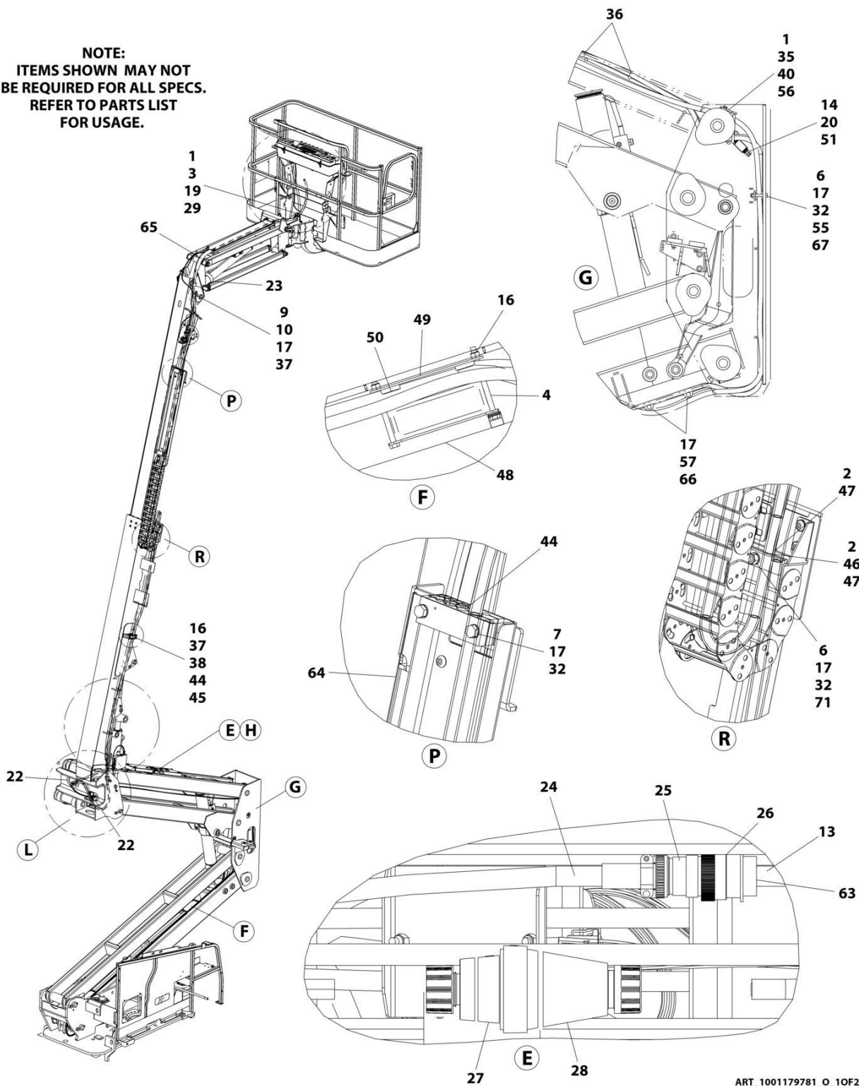
FIGURE 8-19. BOOM CABLES & CLAMPS INSTALLATION (7500W SKYPOWER GENERATOR)
