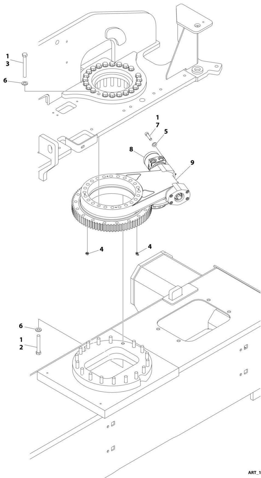
FIGURE 2-5. SWING DRIVE AND TURNTABLE BEARING INSTALLATION (SN B300018363 to Present, Excluding B300018382, B300018383 and B300018451)
