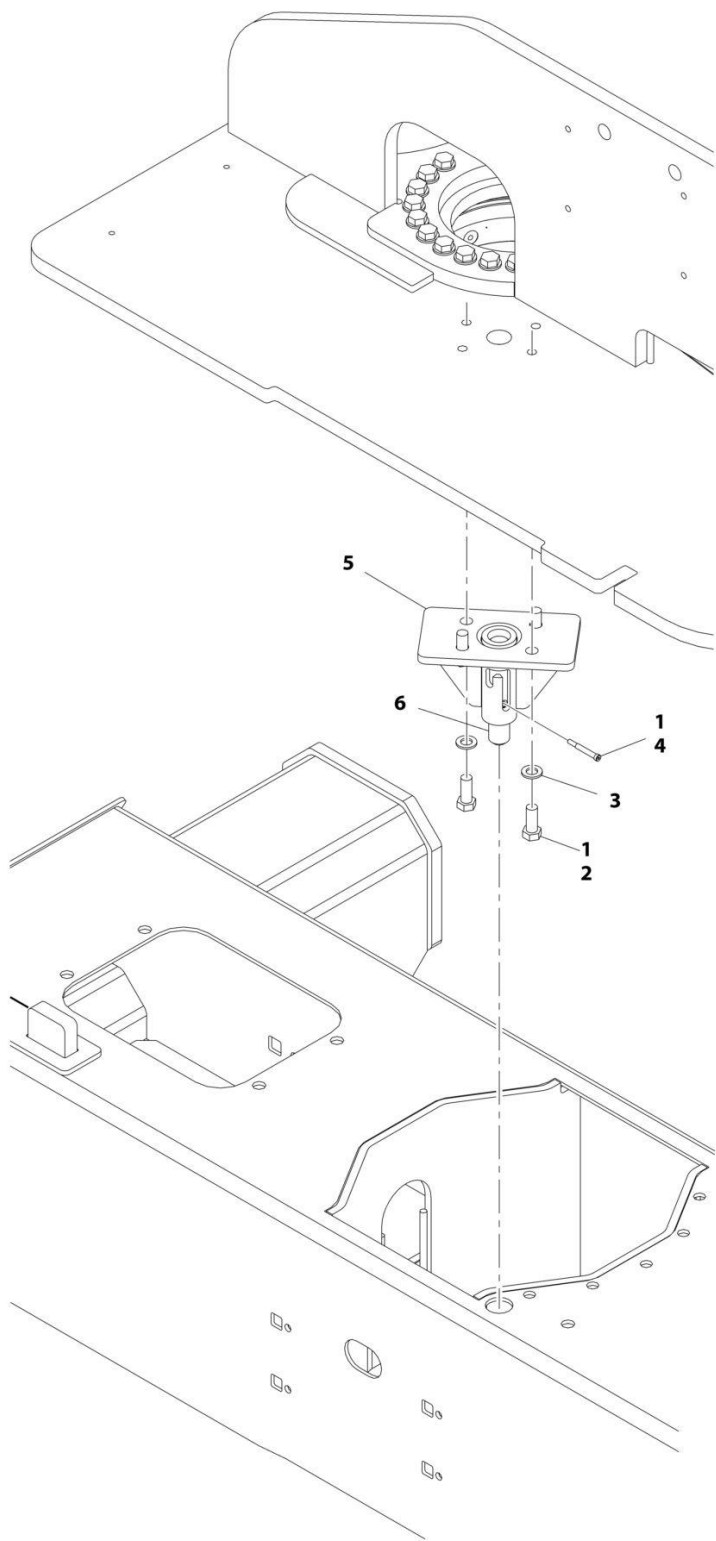
FIGURE 2-10. TURNTABLE LOCK INSTALLATION
