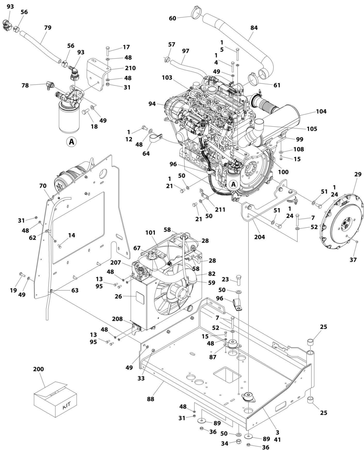
FIGURE 3-15. ENGINE ASSEMBLY - DEUTZ D2.9L4 ENGINE (CHINA IV)
