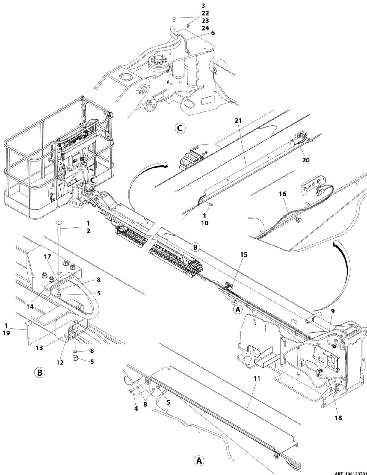
FIGURE 8-26. CABLES AND CLAMPS INSTALLATION - 400S HC3 WITH 7500W GENERATOR
