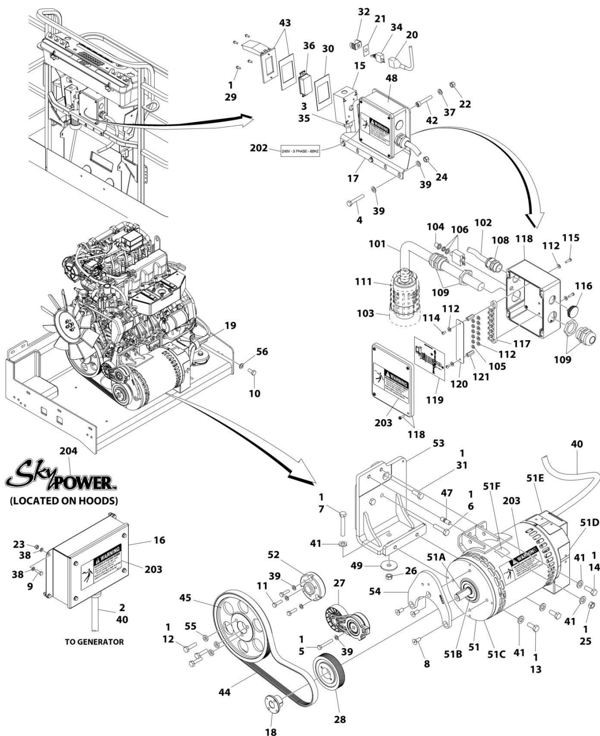
FIGURE 3-51. 7500W/60HZ SKYPOWER GENERATOR INSTALLATION - KUBOTA ENGINES
