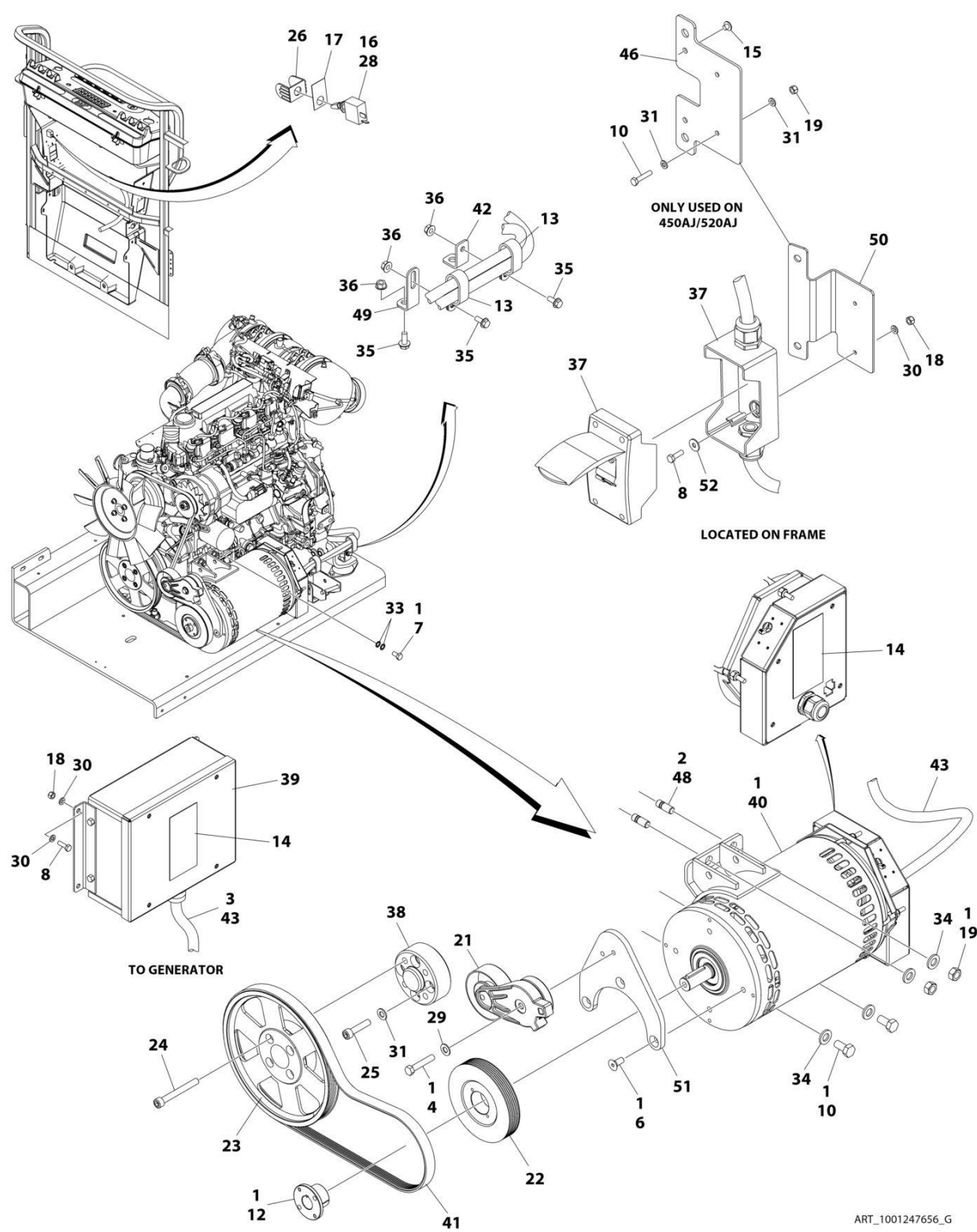
FIGURE 3-47. 4000W/50HZ GENERATOR INSTALLATION (DEUTZ D2.9L4 (STAGE V) ENGINES)
