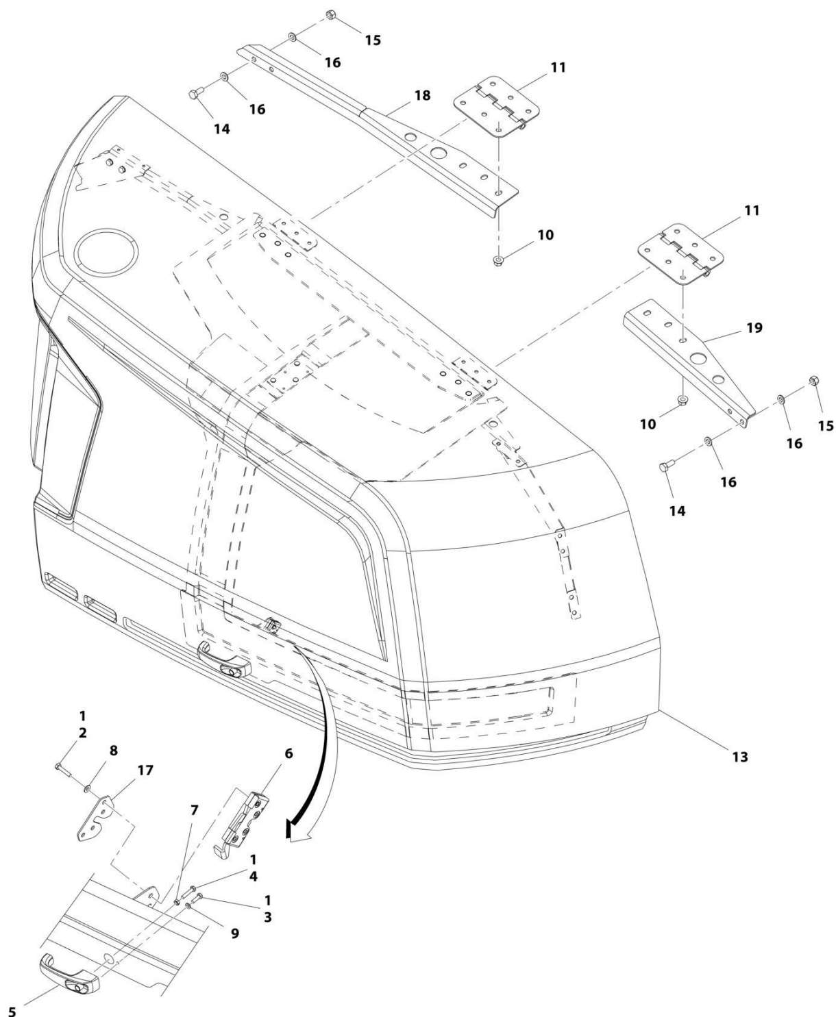
FIGURE 2-49. HOOD ASSEMBLY - ENGINE SIDE (ABS)
