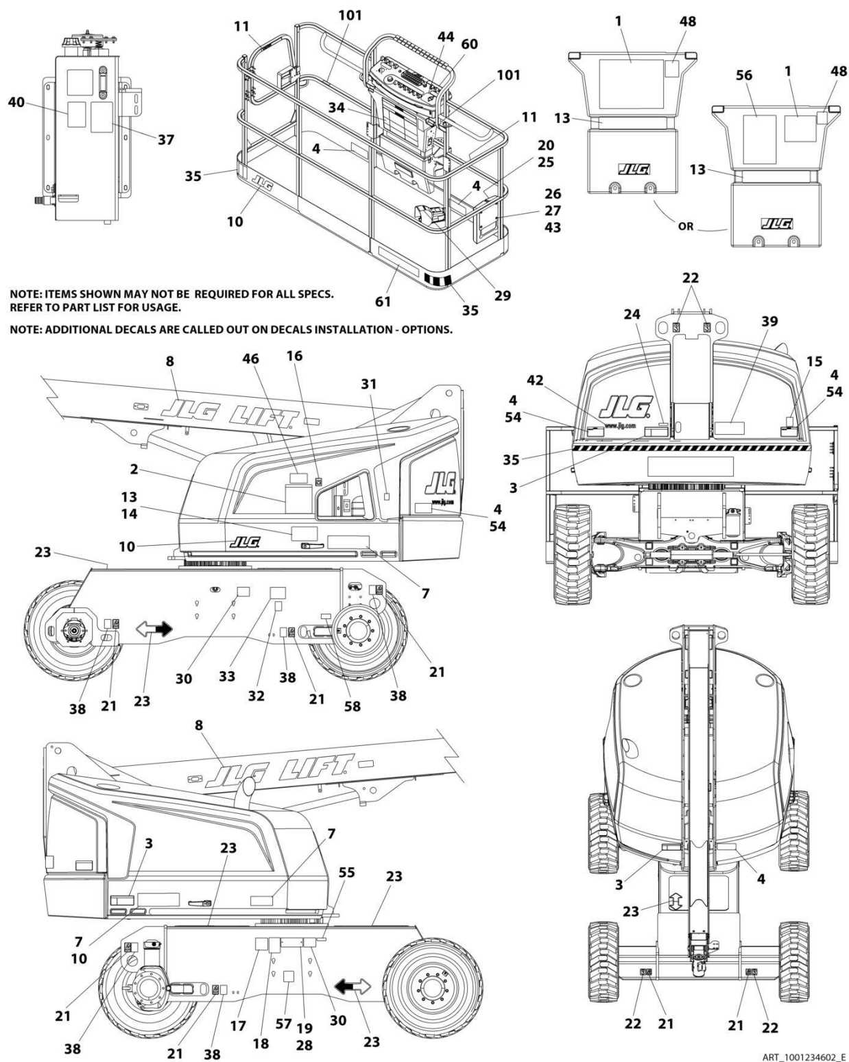
FIGURE 9-10. DECAL INSTALLATION - KOREAN SPECS
