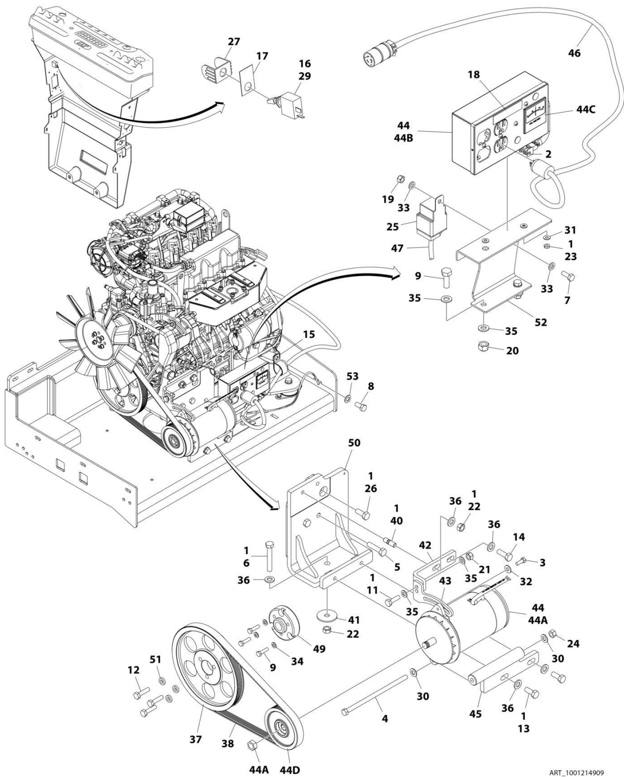
FIGURE 3-43. 2500W/110V/60HZ GENERATOR INSTALLATION - KUBOTA ENGINES
