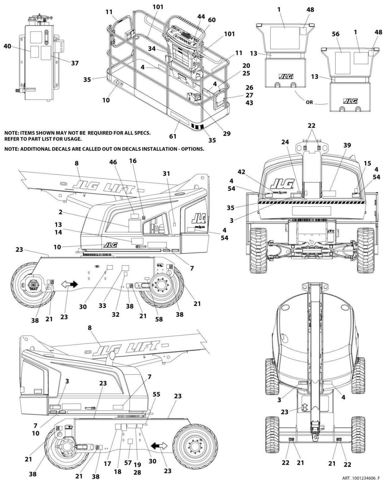
FIGURE 9-4. DECAL INSTALLATION - BRAZIL SPECS
