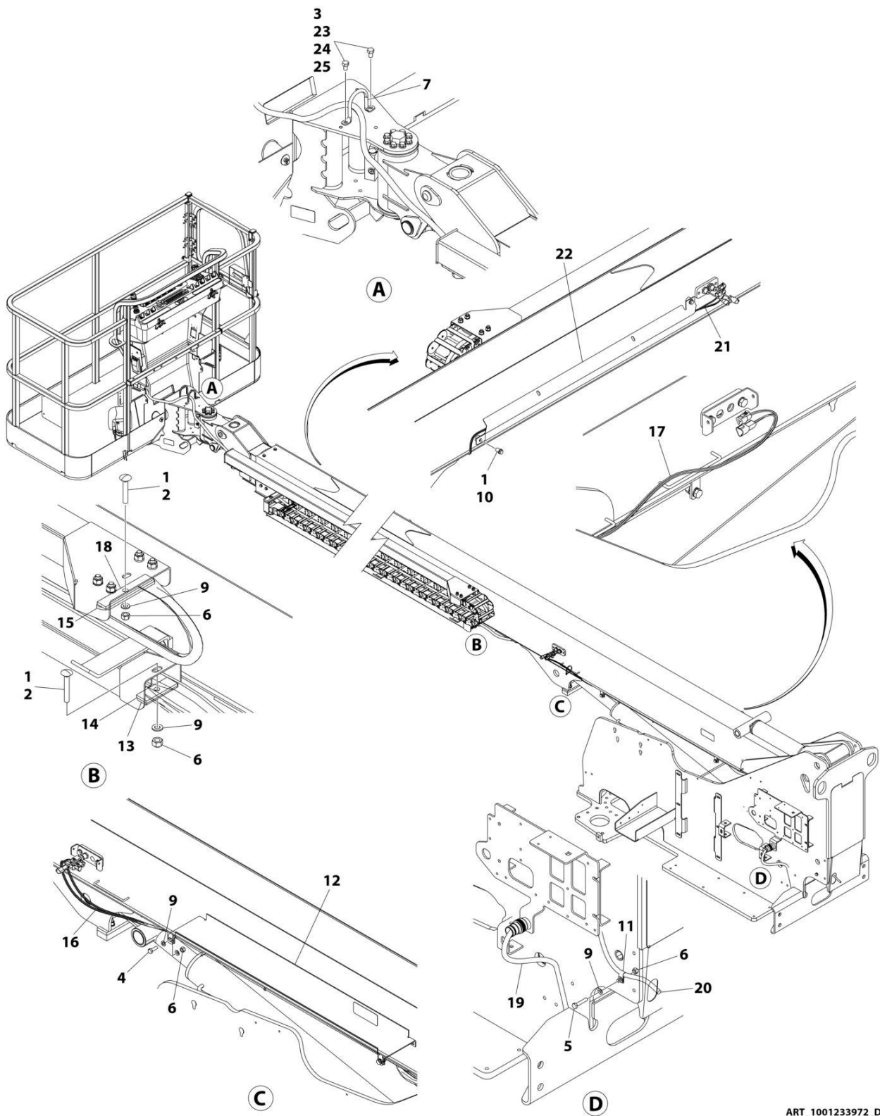
FIGURE 8-24. CABLES AND CLAMPS INSTALLATION - 400S HC3 WITH 4000W/50HZ GENERATOR
