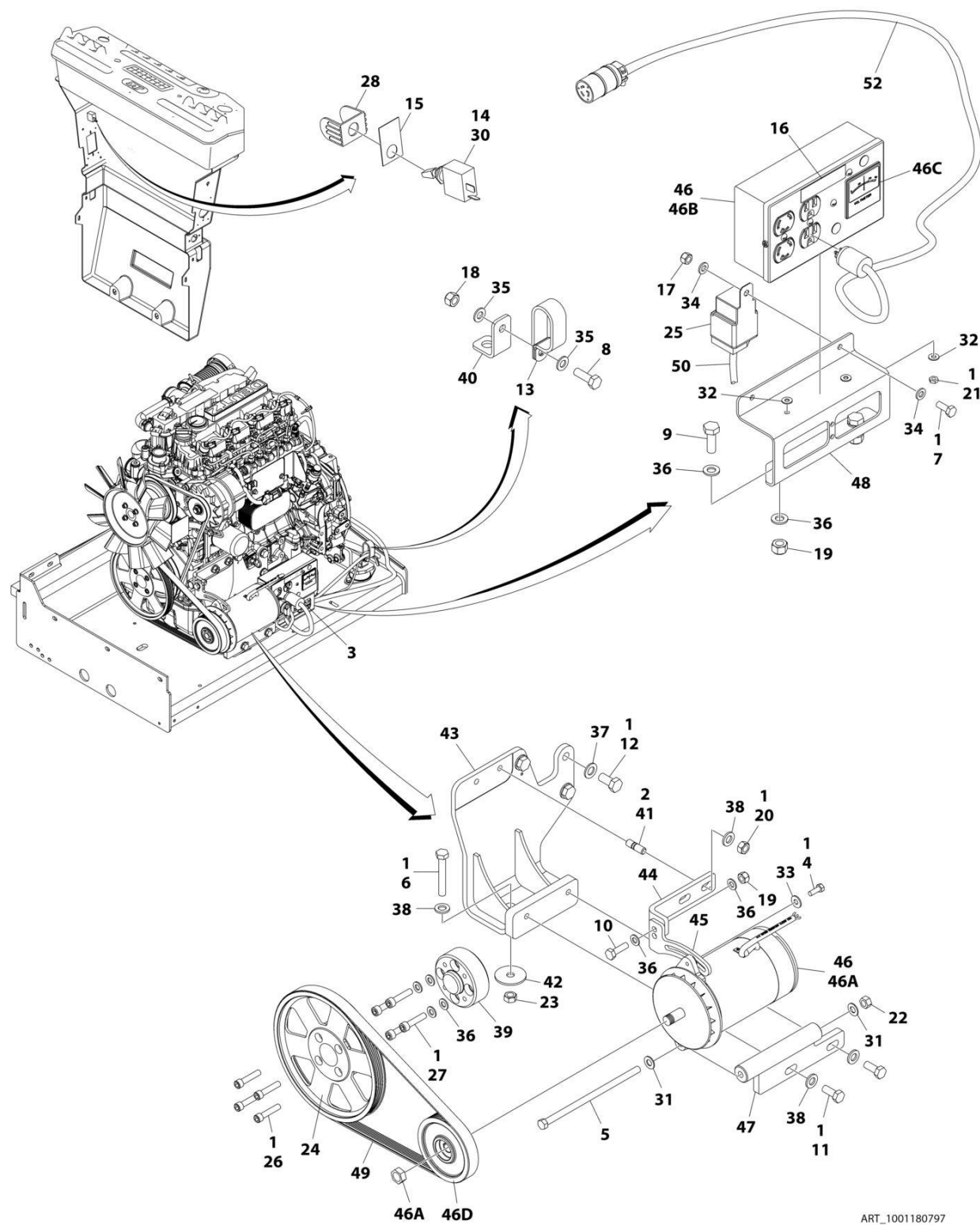
FIGURE 3-42. 2500W/110V/60HZ GENERATOR INSTALLATION - DEUTZ D2.9L4 ENGINES
