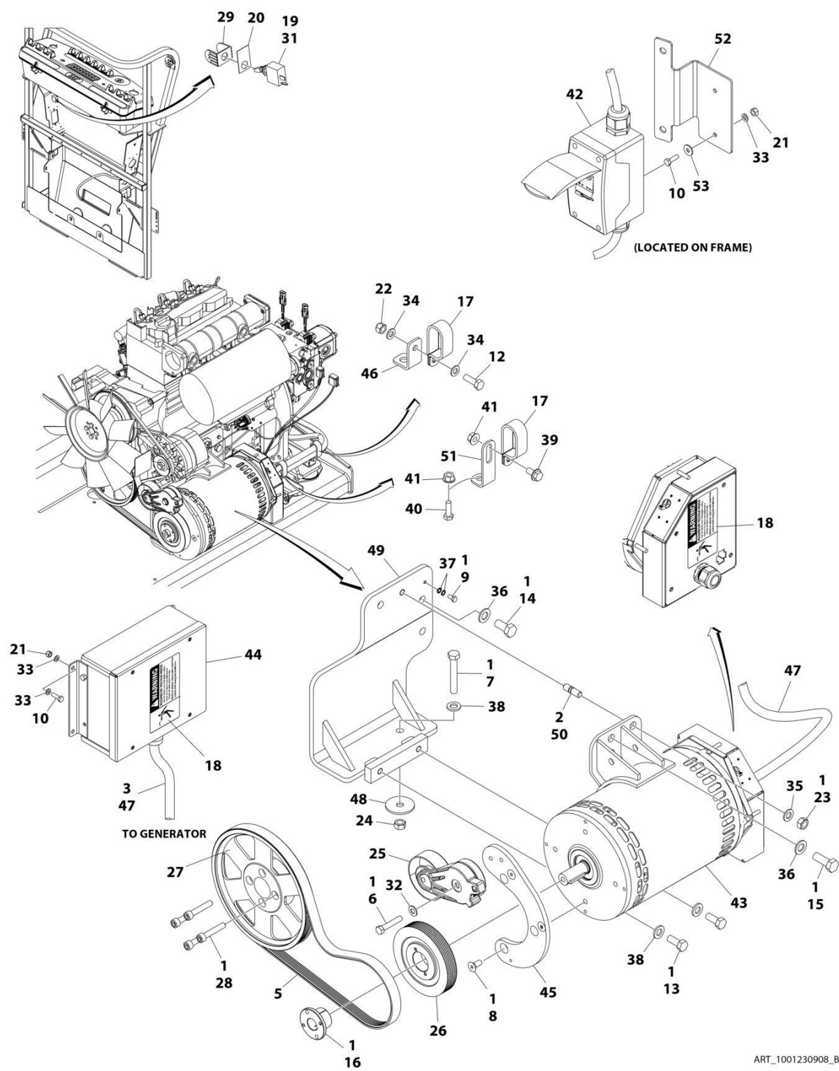
FIGURE 3-44. 4000W/50HZ GENERATOR INSTALLATION - DEUTZ D2011 ENGINES
