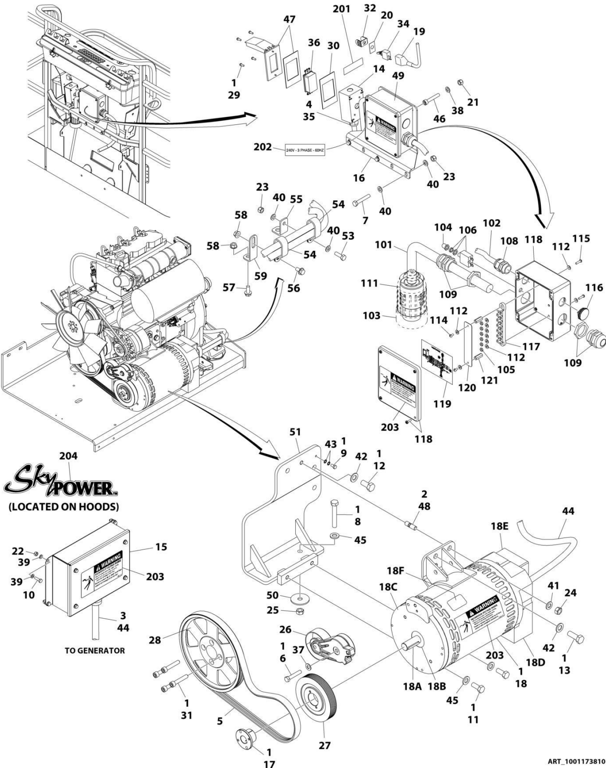
FIGURE 3-49. 7500W/60HZ SKYPOWER GENERATOR INSTALLATION - DEUTZ D2011 ENGINES
