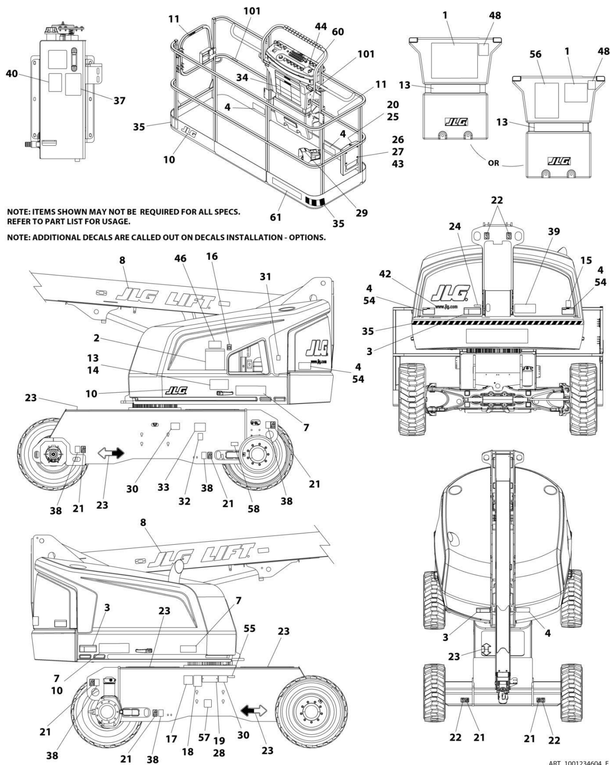
FIGURE 9-7. DECAL INSTALLATION - CSA SPECS (DIESEL MACHINES)
