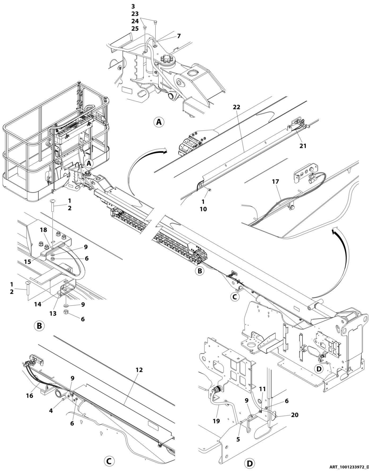
FIGURE 8-23. CABLES AND CLAMPS INSTALLATION - 400S HC3 WITH 2500W GENERATOR OR NO GENERATOR
