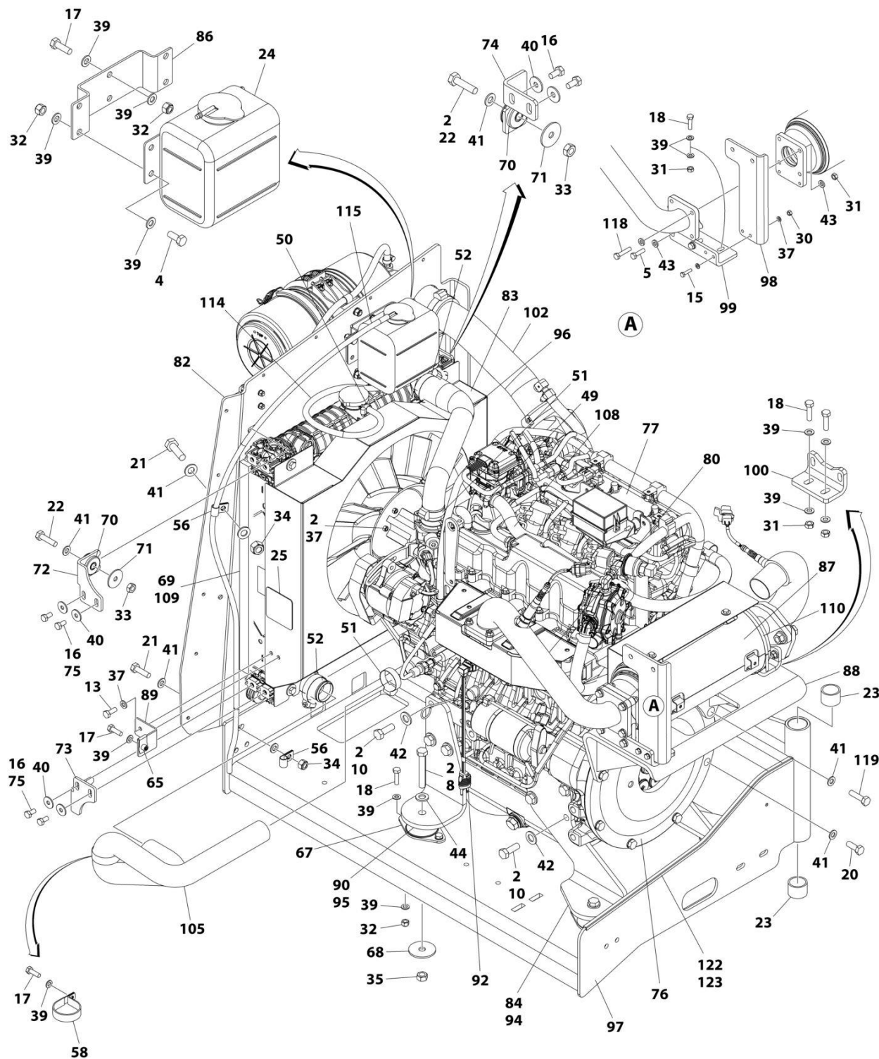
FIGURE 3-31. KUBOTA ENGINE ASSEMBLY (WITH ARCTIC PACKAGE)
