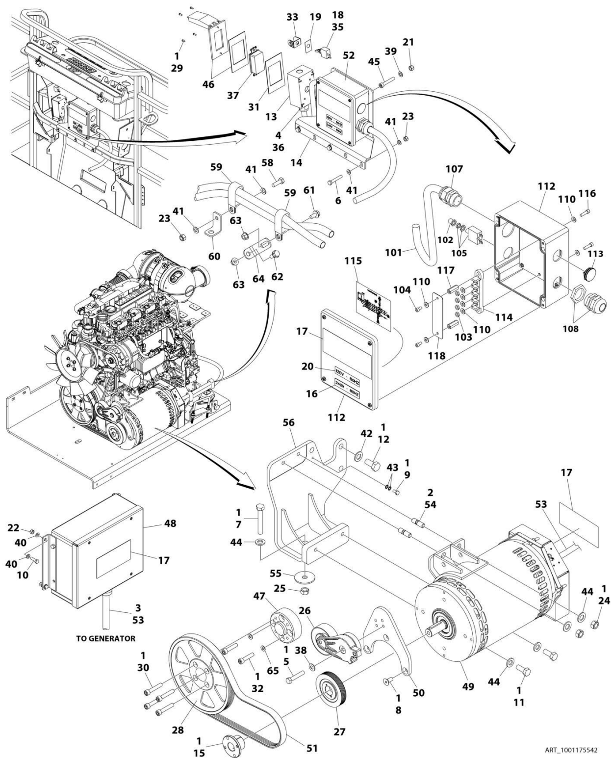
FIGURE 3-46. 4000W/60HZ GENERATOR INSTALLATION - DEUTZ D2.9L4 ENGINES
