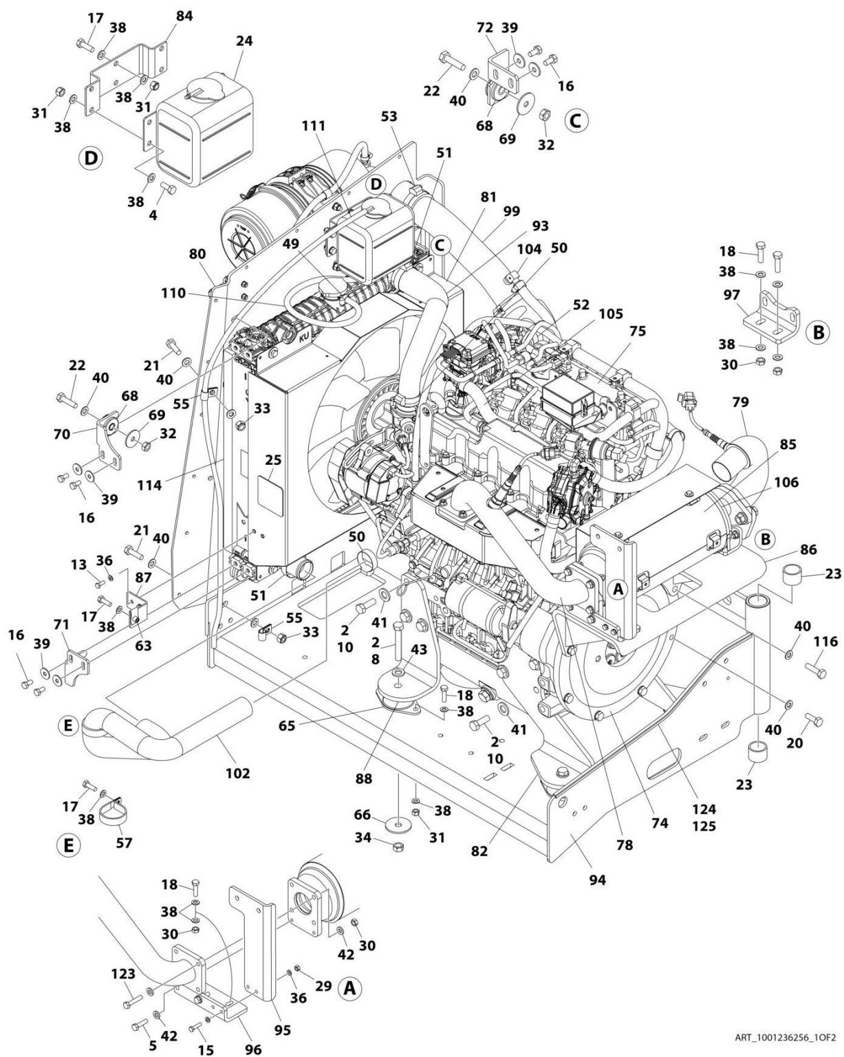
FIGURE 3-28. KUBOTA ENGINE ASSEMBLY (WITHOUT ARCTIC PACKAGE)
