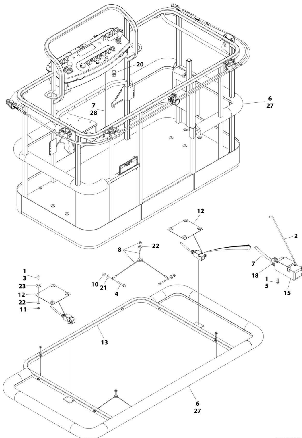
FIGURE 5-28. SOFT TOUCH SYSTEM INSTALLATION - 6FT/1.83M FALL ARREST PLATFORM (MACHINES WITH SN STARTING WITH 03 ONLY)
